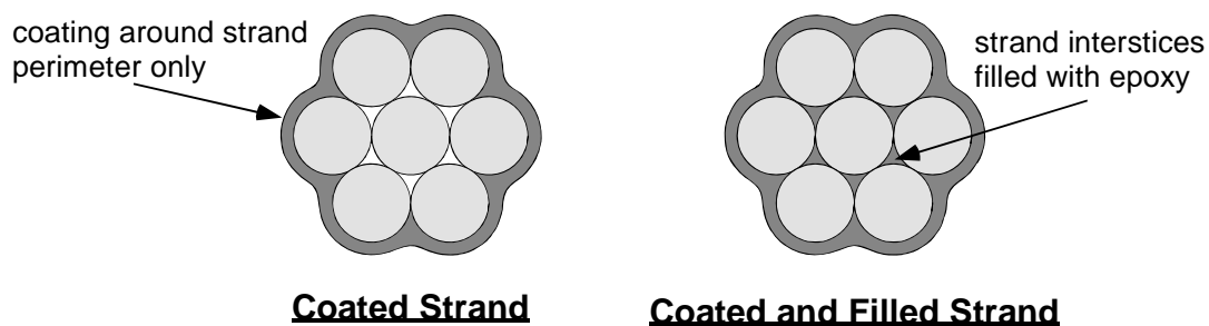
Figure 2.29 - Epoxy Coated Strand Types
