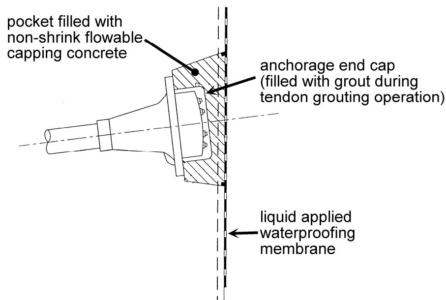
Figure 2.30 -Multi-Layer Corrosion Protection for Buried Post-Tensioning Anchorages 2.78
