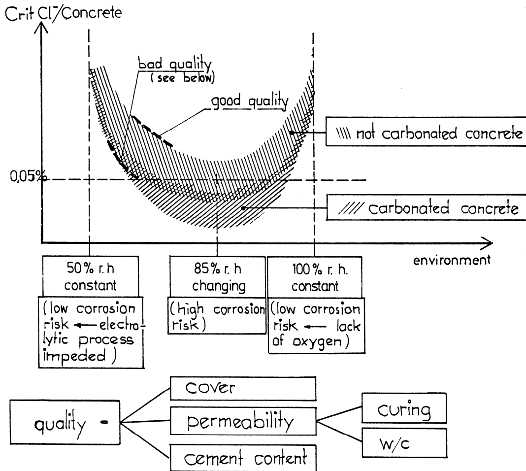
Figure 2.12 - CEB Critical Chloride Ion Content for Corrosion 2.1
