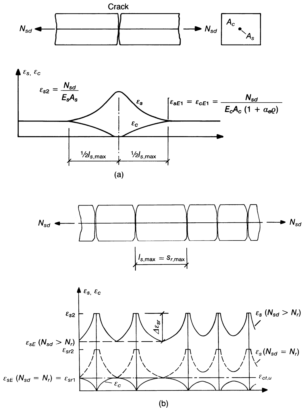
Figure 2.39 - Strains for Calculating Crack Widths Under MC 90: (a) For Single Crack Formation, (b) for Stabilized Cracking (from Ref. 2.124)
