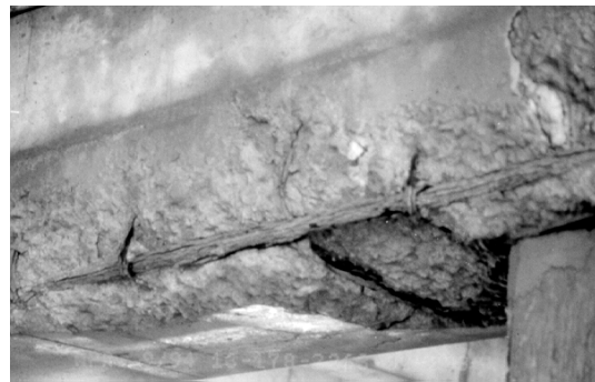
(b) Atmospheric Zone - Bent Cap
