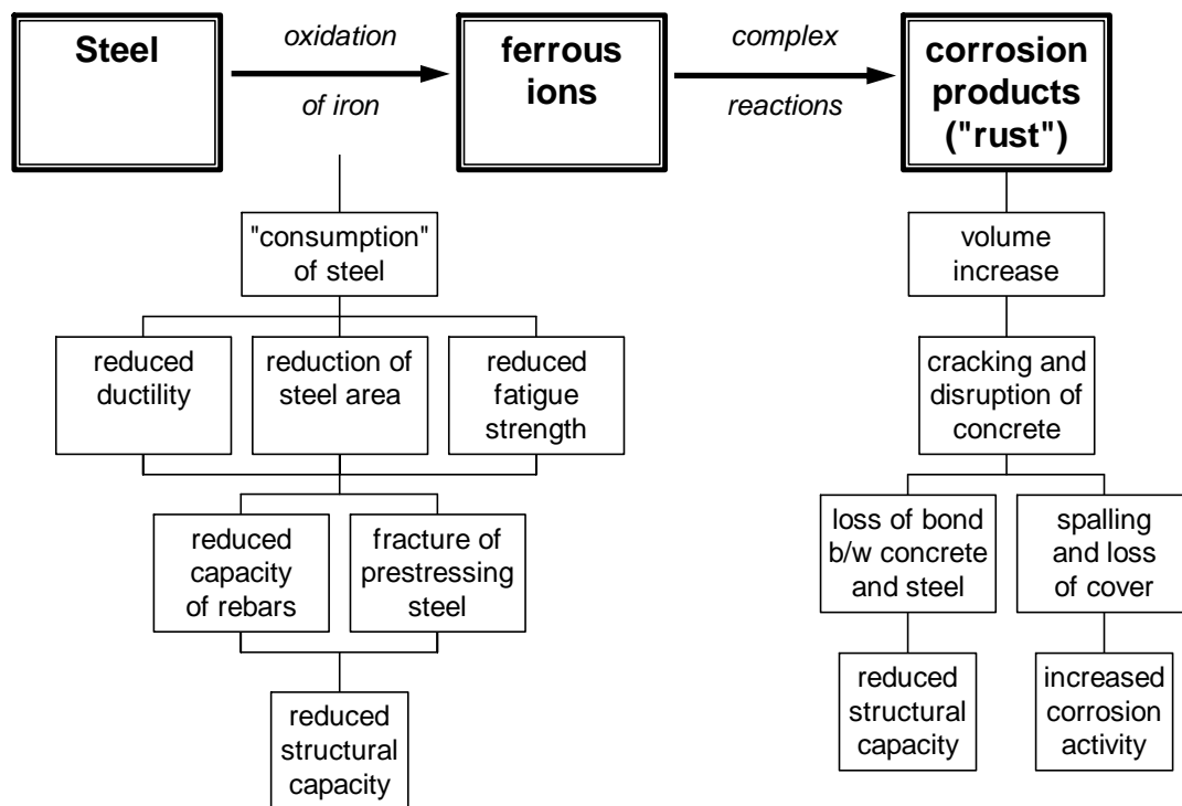
Figure 2.5 - Deterioration Mechanism for Corrosion of Steel in Concrete
