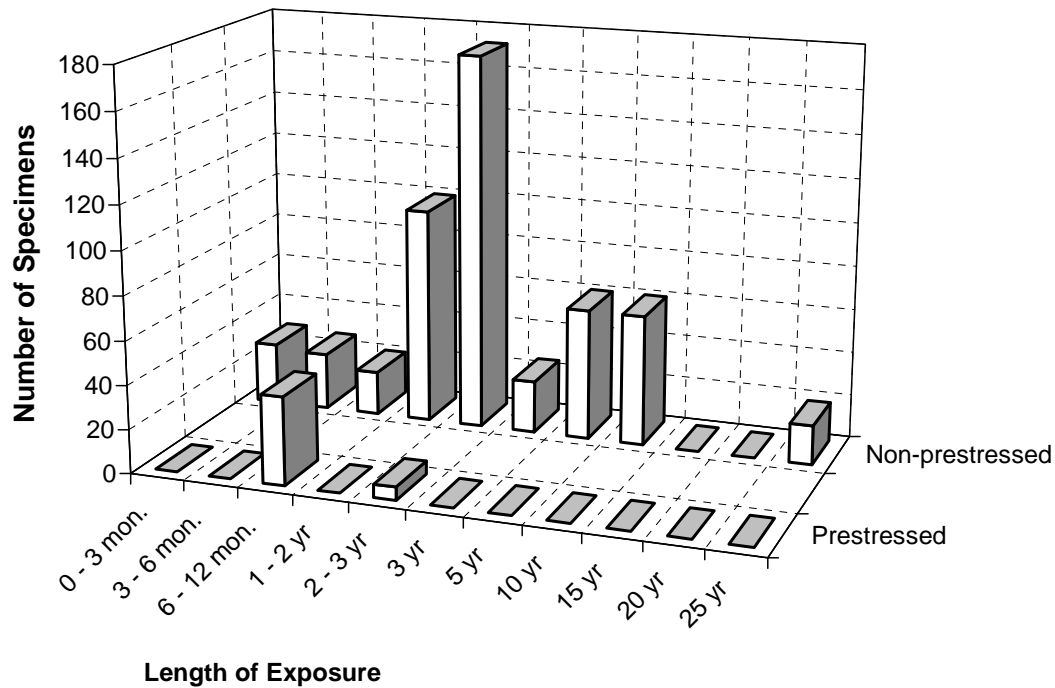
Figure 2.18 - Summary of Corrosion Studies Considering Crack Width
