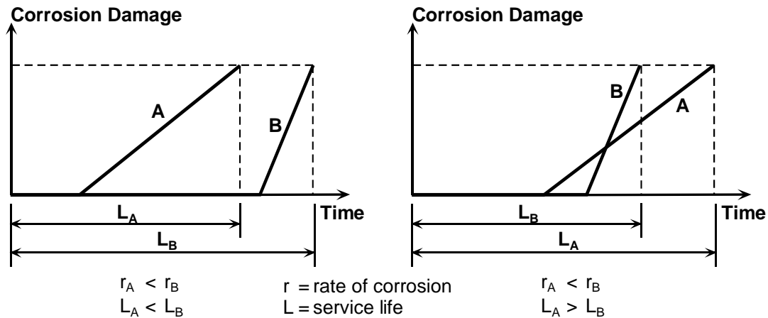
Figure 2.9 - Effect of Time to Corrosion and Corrosion Rate on Service Life (adapted from Ref. 2.12)
