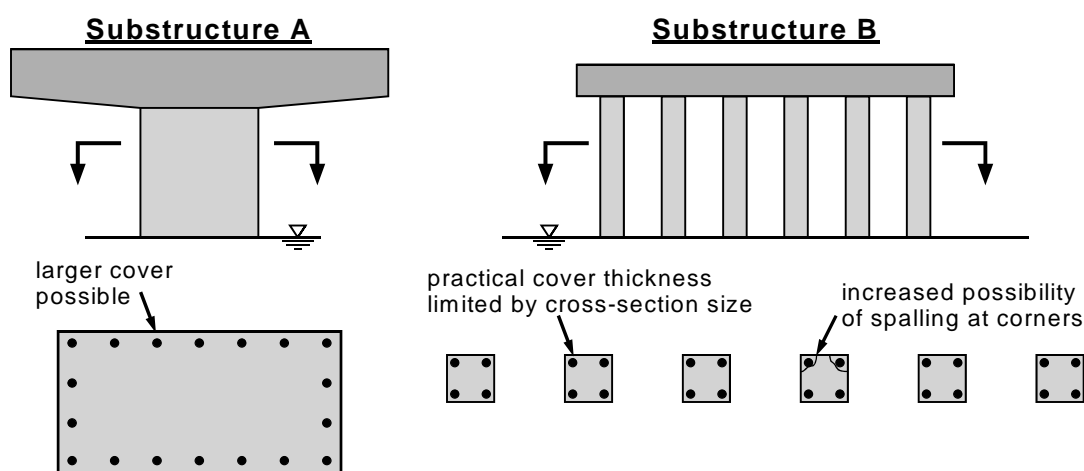
Figure 2.26 - Geometry Effects on Durability for Alternate Substructure Designs
