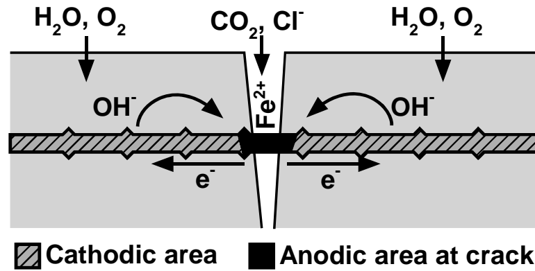
Figure 2.7 - Macrocell Corrosion at a Crack
