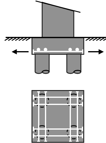
Figure 1.6 - Applications of Post-Tensioning in Bridge Substructures
