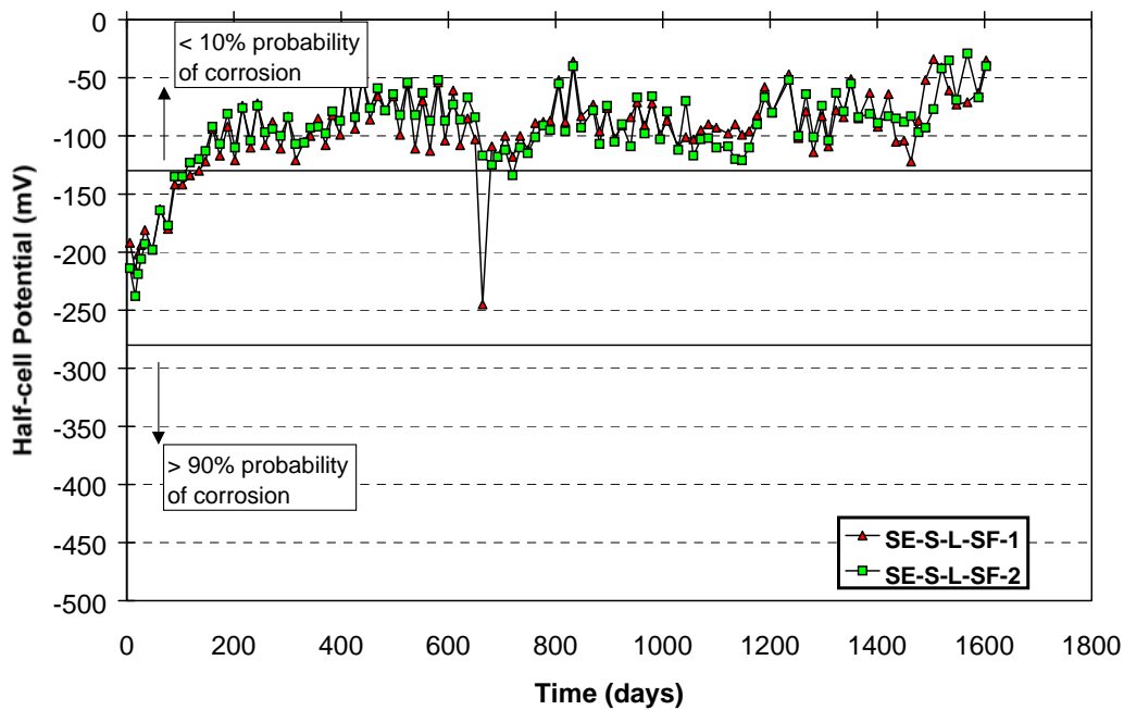
Figure E.35 - Half-Cell Potential Readings: SE-S-L-SF
