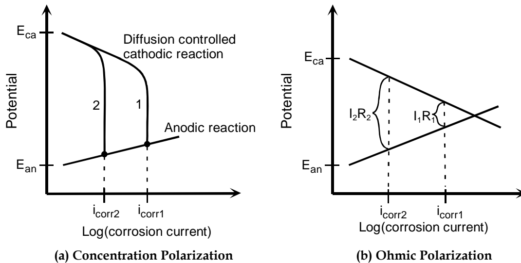
Figure 2.11 – Common Polarization Effects in Concrete Structures 2,11
