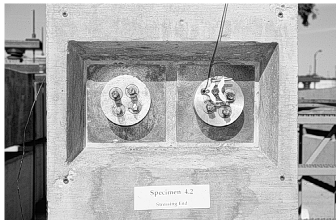
Figure 3.29 - Anchorage Pocket Immediately Before Capping
