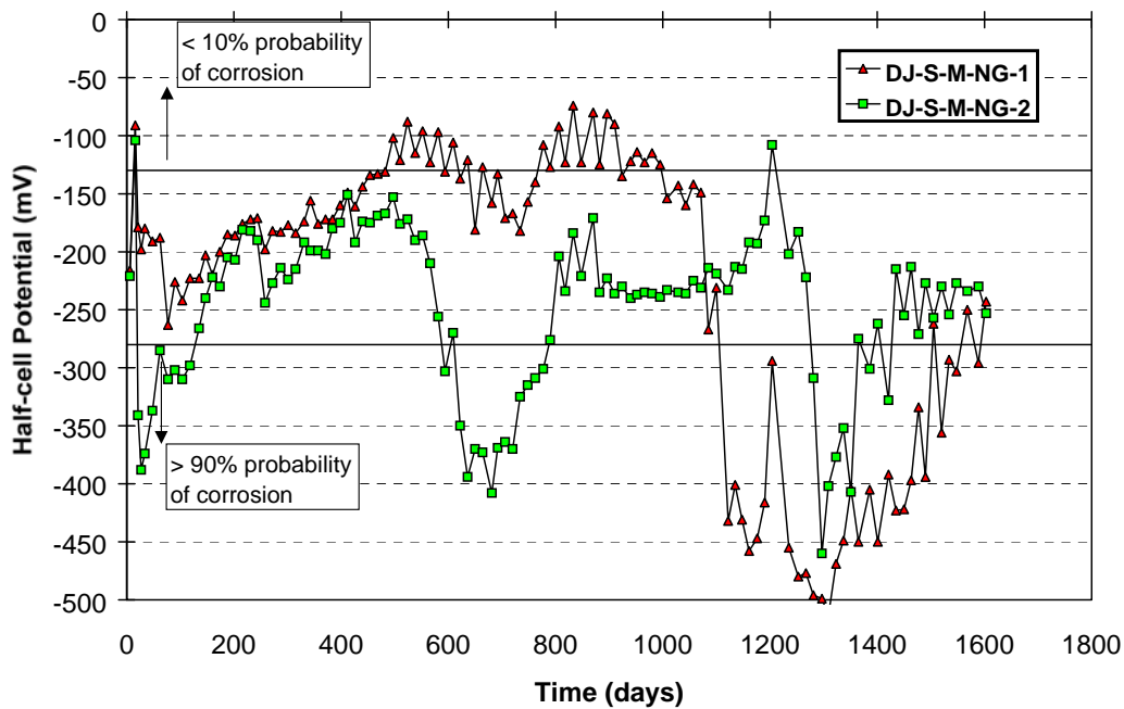
Figure E.21 - Half-Cell Potential Readings: DJ-S-M-NG
