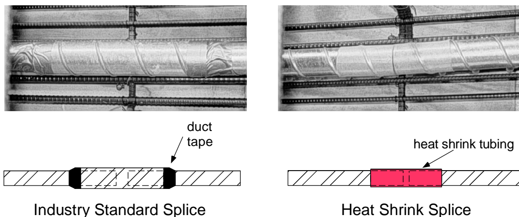
Figure 3.16 - Duct Splices
