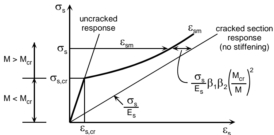
Figure 2.37 - Mean Reinforcement Strain, \epsilon_{sm} , Accounting for the Contribution of Concrete in Tension (MC 78)
