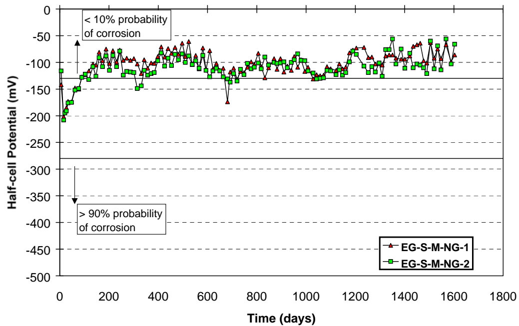
Figure E.37 - Half-Cell Potential Readings: EG-S-M-NG
