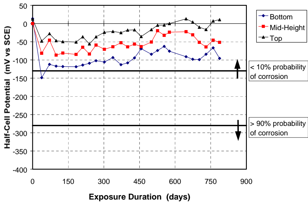
Figure D.10 - Average Half-Cell Potentials: Column DJ-TC-S
