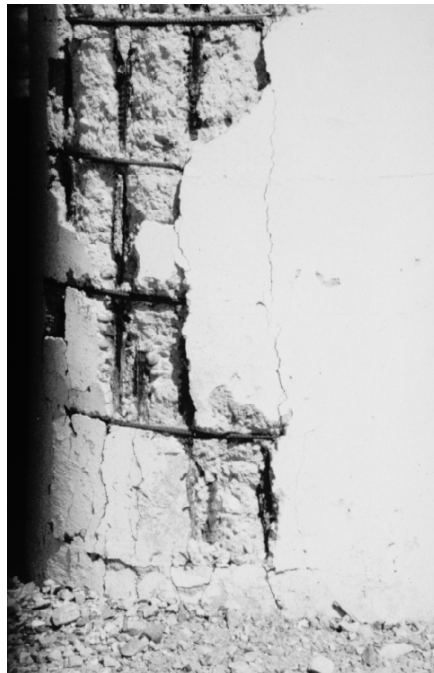
Figure 2.25 - Column Corrosion Resulting from Splashing Adjacent to Roadway
