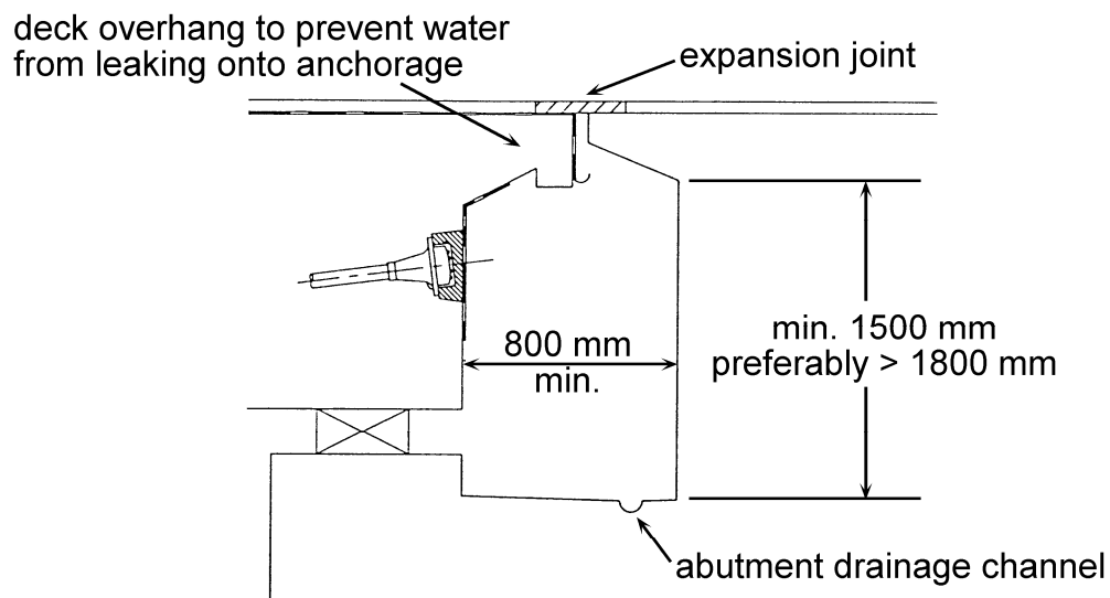
Figure 2.31 - Member End Details for Anchorage Corrosion Protection 2.78
