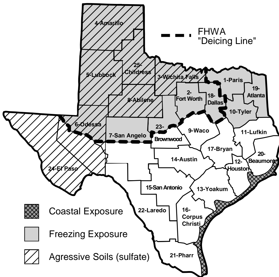
Figure 2.4 - Substructure Exposure Conditions for the State of Texas
