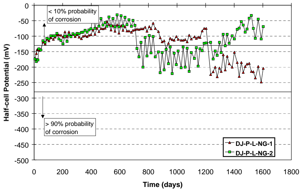
Figure E.23 - Half-Cell Potential Readings: DJ-P-L-NG
