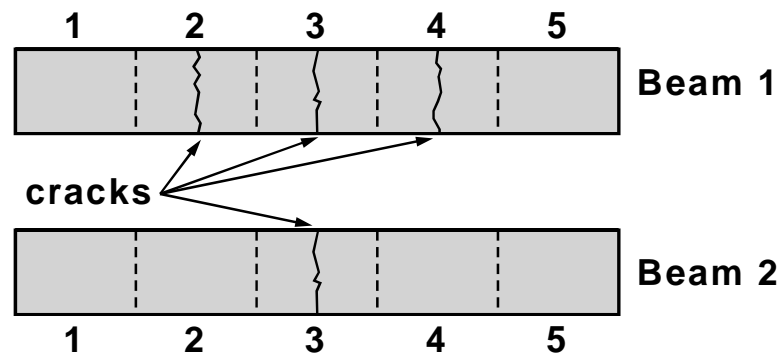
Figure 2.19 - Beams for Effect of Cracking Illustration
