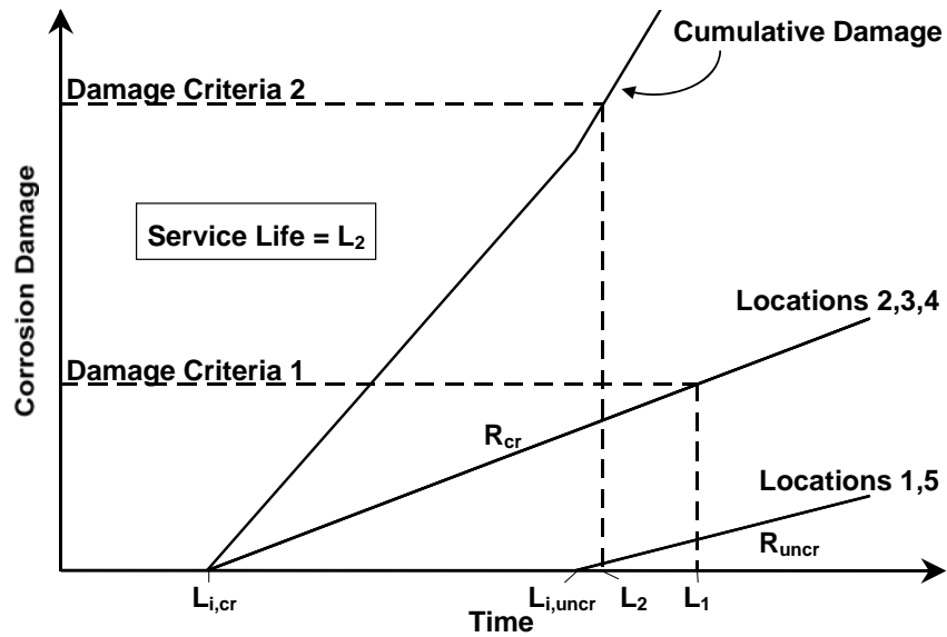
Figure 2.20 - Corrosion Damage Plot for Beam 1
