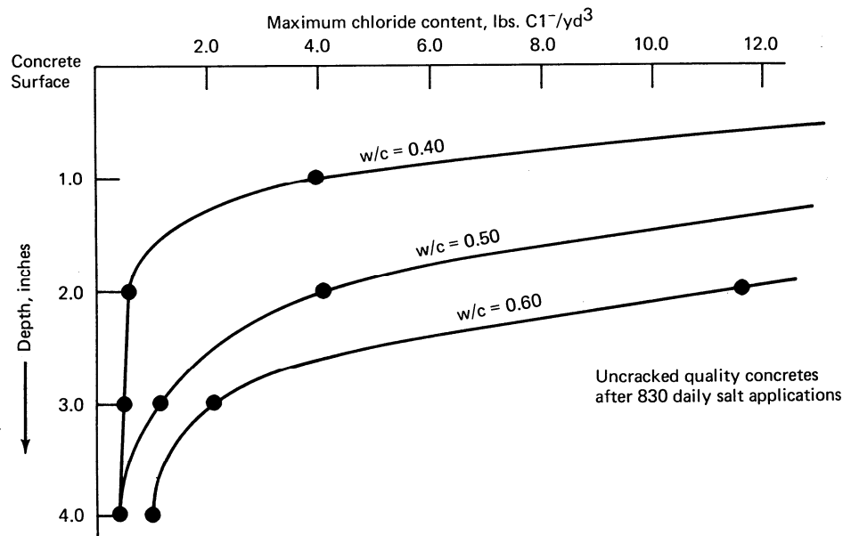
Figure 2.27 - Effect of Water-Cement Ratio on Chloride Ion Penetration 2.41
