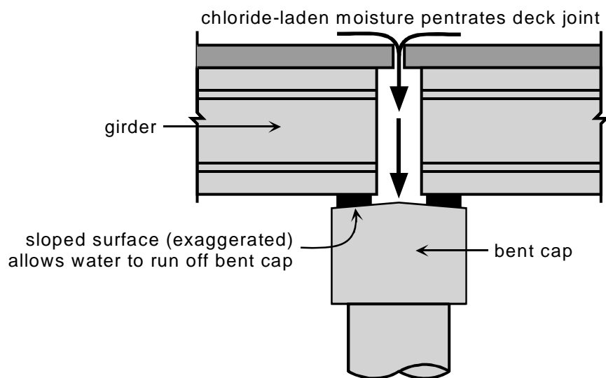
Figure 2.24 - Sloped Bent Cap to Promote Run-Off (adapted from Ref. 2.1)
