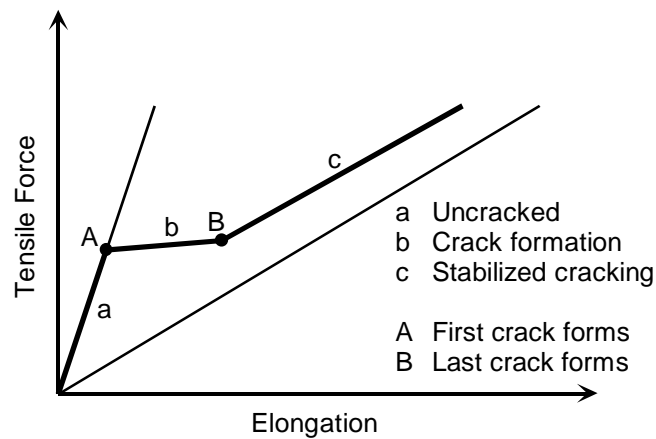
Figure 2.38 - Idealized Phases of Cracking Behavior for a Reinforced Concrete Tension Tie (adapted from Ref. 2.124)
