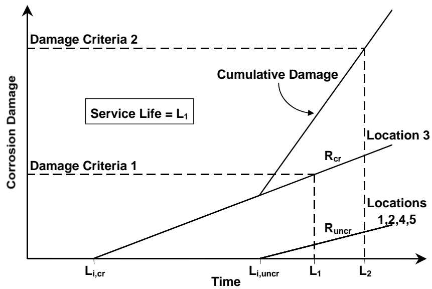
Figure 2.21 - Corrosion Damage Plot for Beam 2
