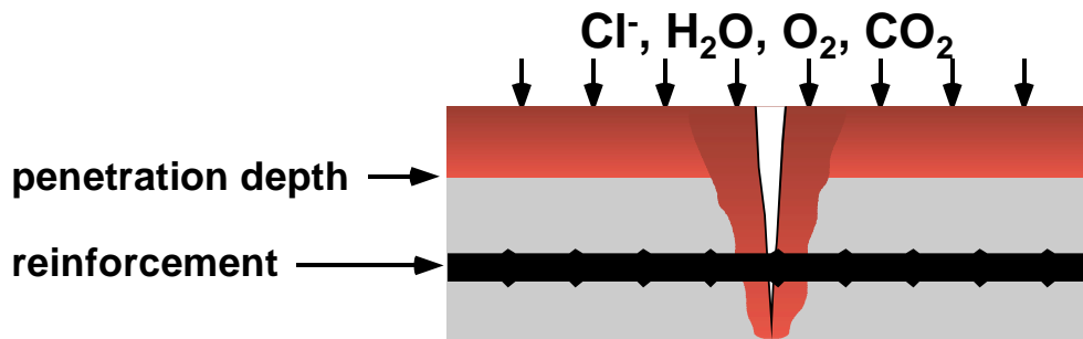
Figure 2.14 - Point of View 1: Increased Penetration of Moisture and Chlorides at Crack Location Accelerates the Onset and Severity of Corrosion
