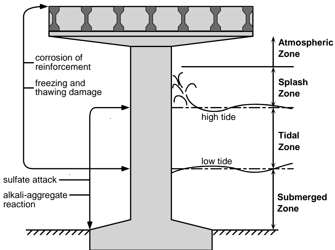
Figure 2.1 - Substructure Exposure Zones and Forms of Deterioration in Coastal Seawater Exposures
