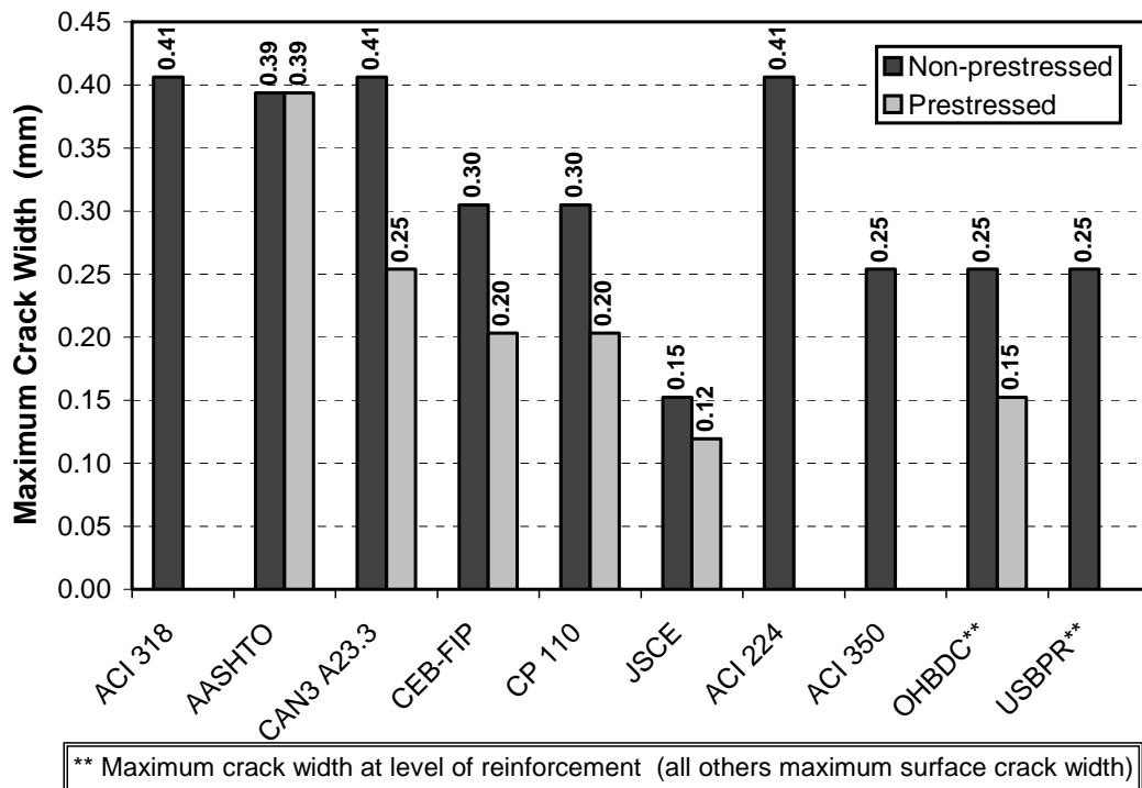
Figure 2.16 - Comparison of Allowable Crack Widths: Mild Exposure
