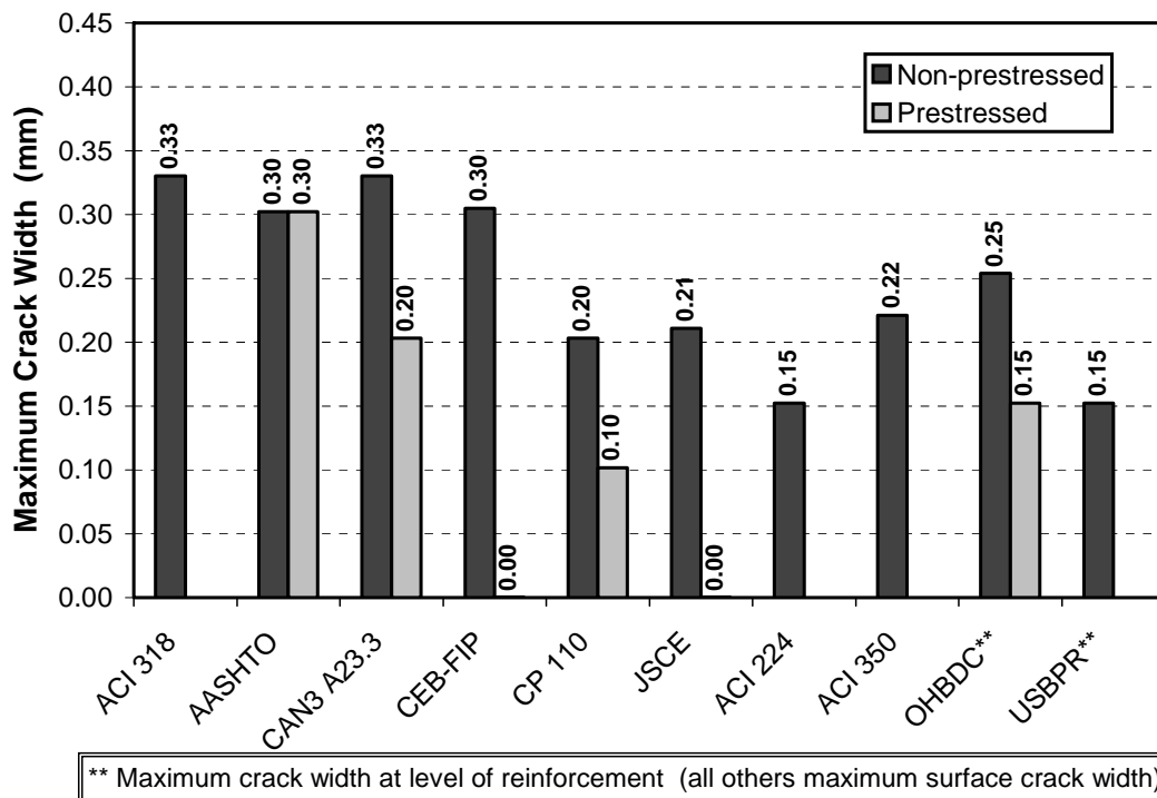
Figure 2.17 - Comparison of Allowable Crack Widths: Severe Exposure
