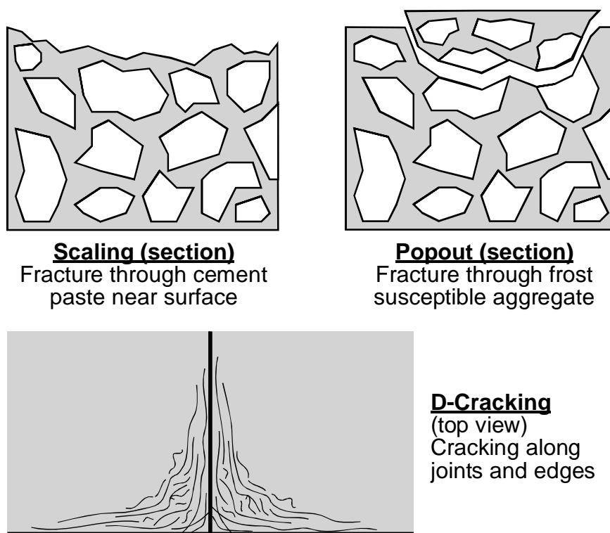
Figure 2.34 - Forms of Freezing and Thawing Damage
