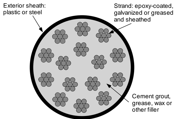
Figure 2.32 - External Post-Tensioning Tendon Corrosion Protection
