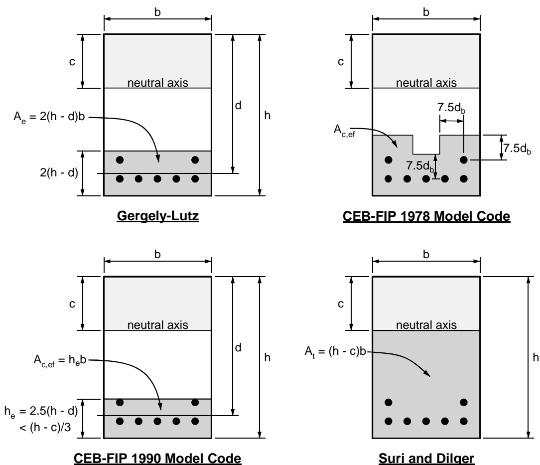
Figure 2.36 - Calculation of Effective Concrete Area in Tension for Various Models
