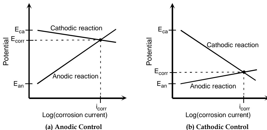
Figure 2.10 - Electrochemical Processes Under Activation Polarization 2,11
