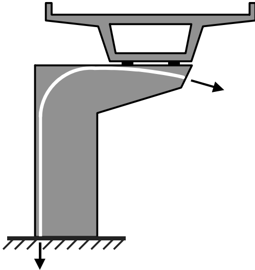
(a) Cantilever Substructure
