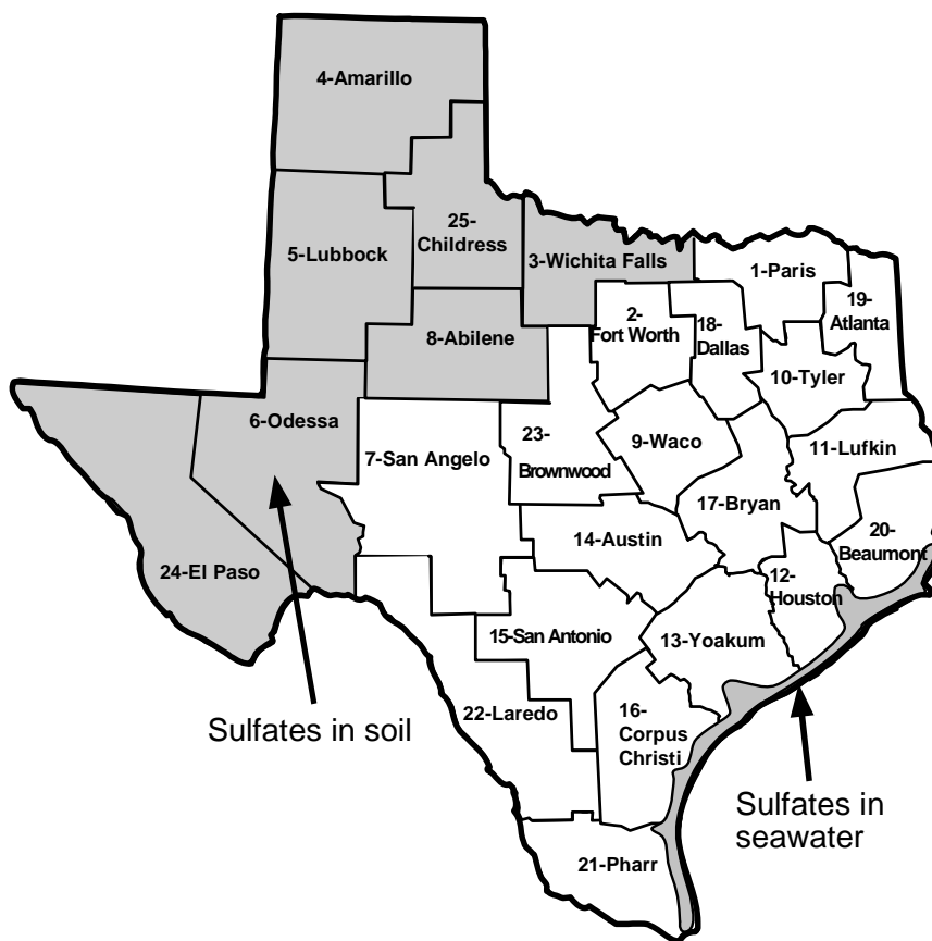
Figure 2.33 - Possible Sulfate Attack Exposure Conditions in Texas 2,2
