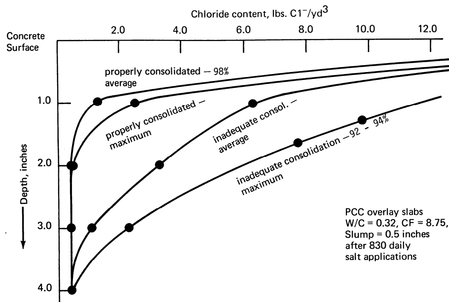
Figure 2.28 - Effect of Consolidation on Chloride Ion Penetration 2.41
