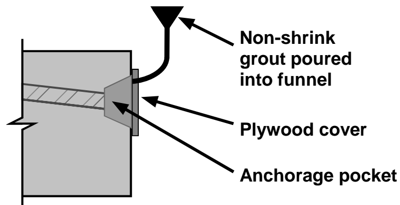
Figure 3.30 - Capping End Anchorages
