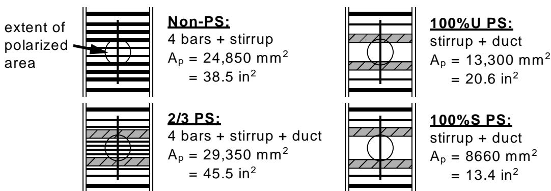
Figure 3.43 - Polarized Steel Surface Areas for PR-Monitor
