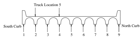
Figure 5.24 Unsymmetrical loading for Truck Locations 1 and 5
