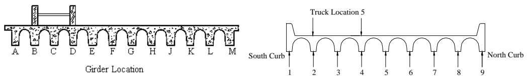
Figure 6.4 1968 Load Pattern Equivalent to Truck Location 5 [4]
