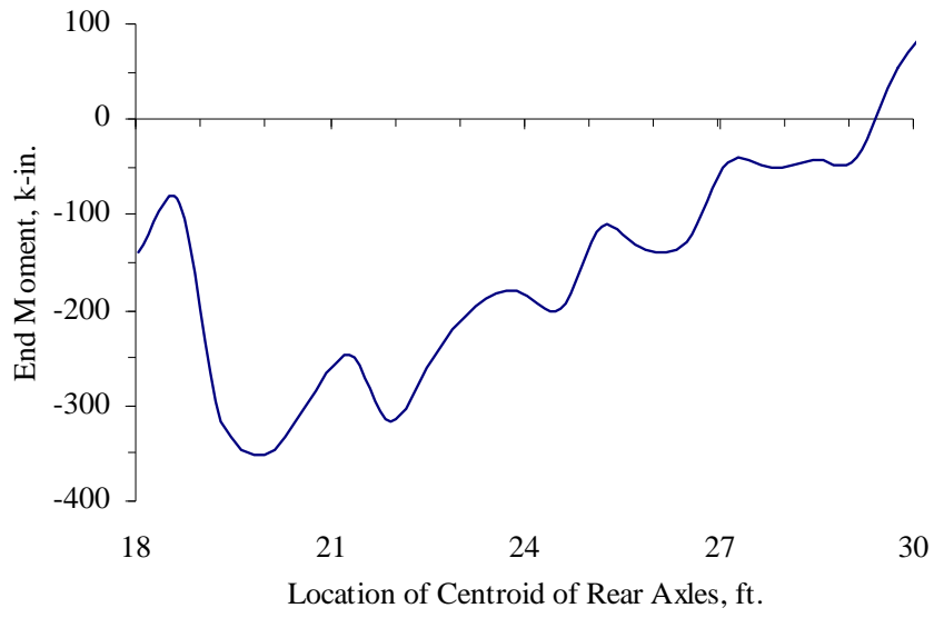
Figure 5.39 End Moment at East Support, Test Series 1
