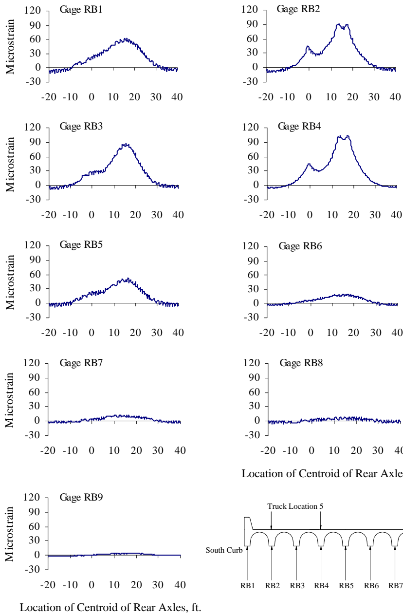
Figure A.21 Reinforcing Bar Strains at Mid-span, Test Series 3, Truck Location 5, Pass 1
