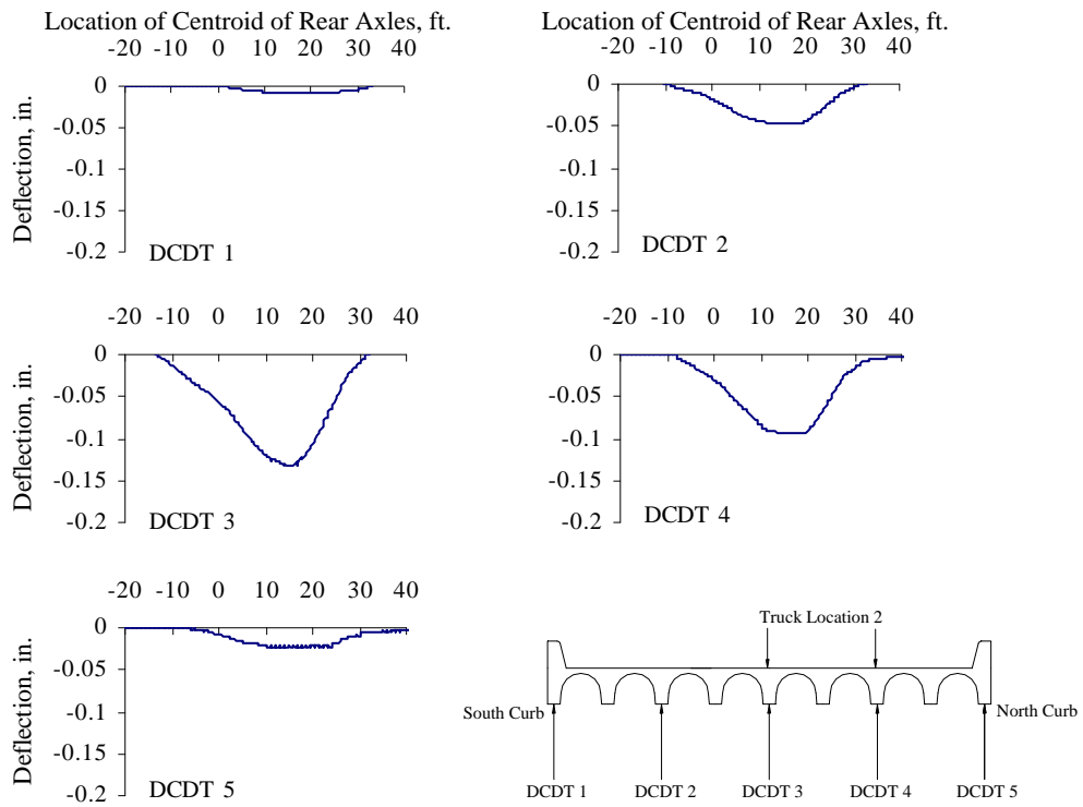
Figure G.15 Vertical Deflections Measured at Mid-span, Test Series 3, Truck Location 2, Pass 1
