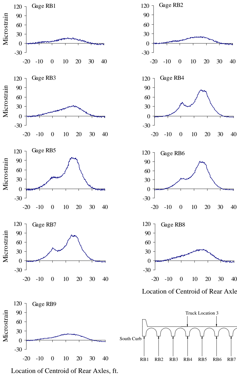
Figure A.8 Reinforcing Bar Strains at Mid-span, Test Series 2, Truck Location 3, Pass 2
