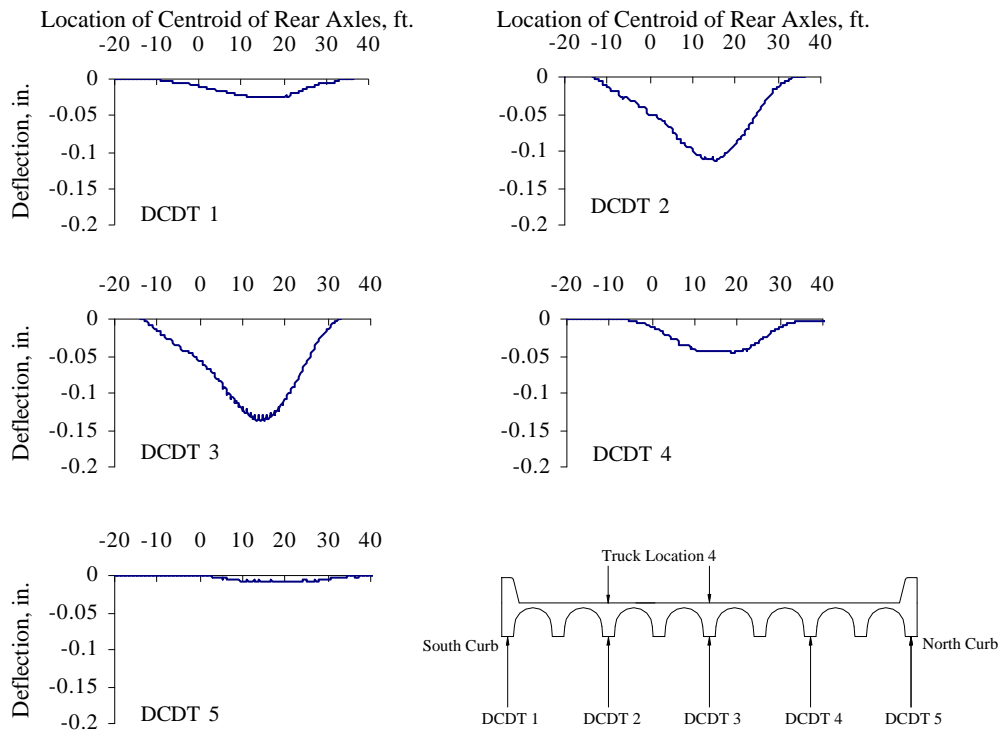
Figure G.10 Vertical Deflections Measured at Mid-span, Test Series 2, Truck Location 4, Pass 2
