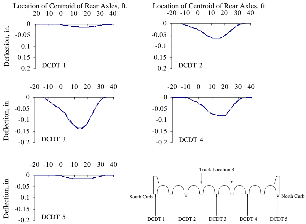
Figure G.8 Vertical Deflections Measured at Mid-span, Test Series 2, Truck Location 3, Pass 2
