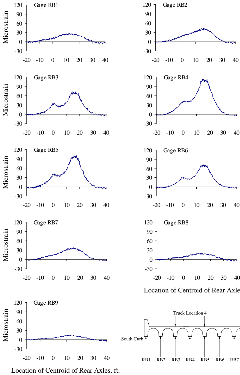
Figure A.10 Reinforcing Bar Strains at Mid-span, Test Series 2, Truck Location 4, Pass 2
