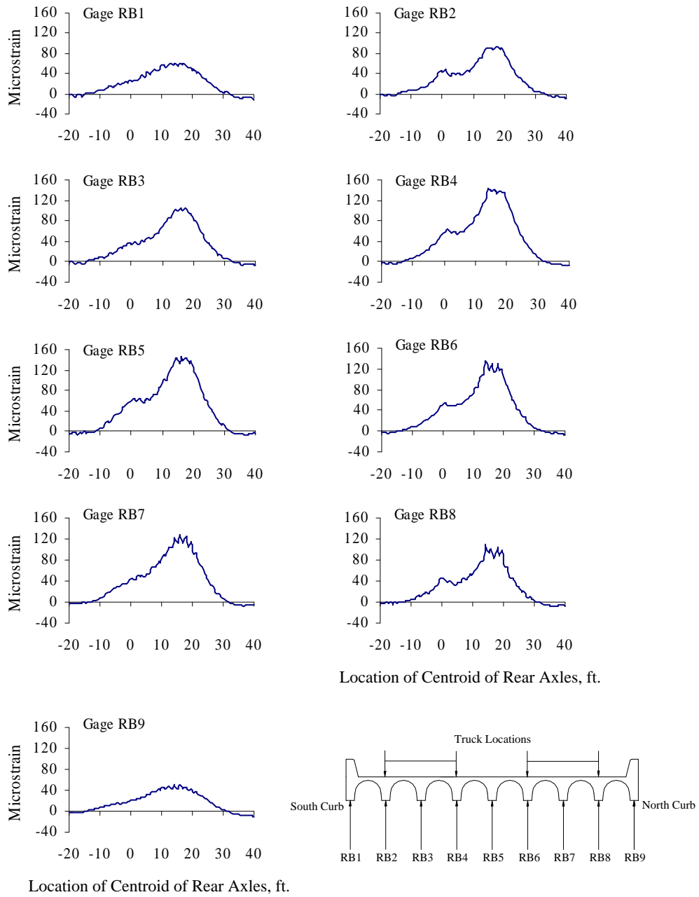
Figure A.1 Reinforcing Bar Strains at Mid-span, Test Series 1, Pass 1
