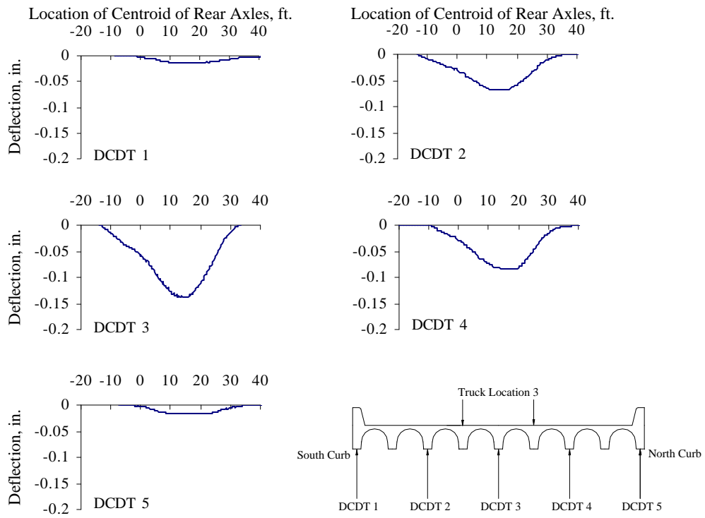
Figure G.7 Vertical Deflections Measured at Mid-span, Test Series 2, Truck Location 3, Pass 1
