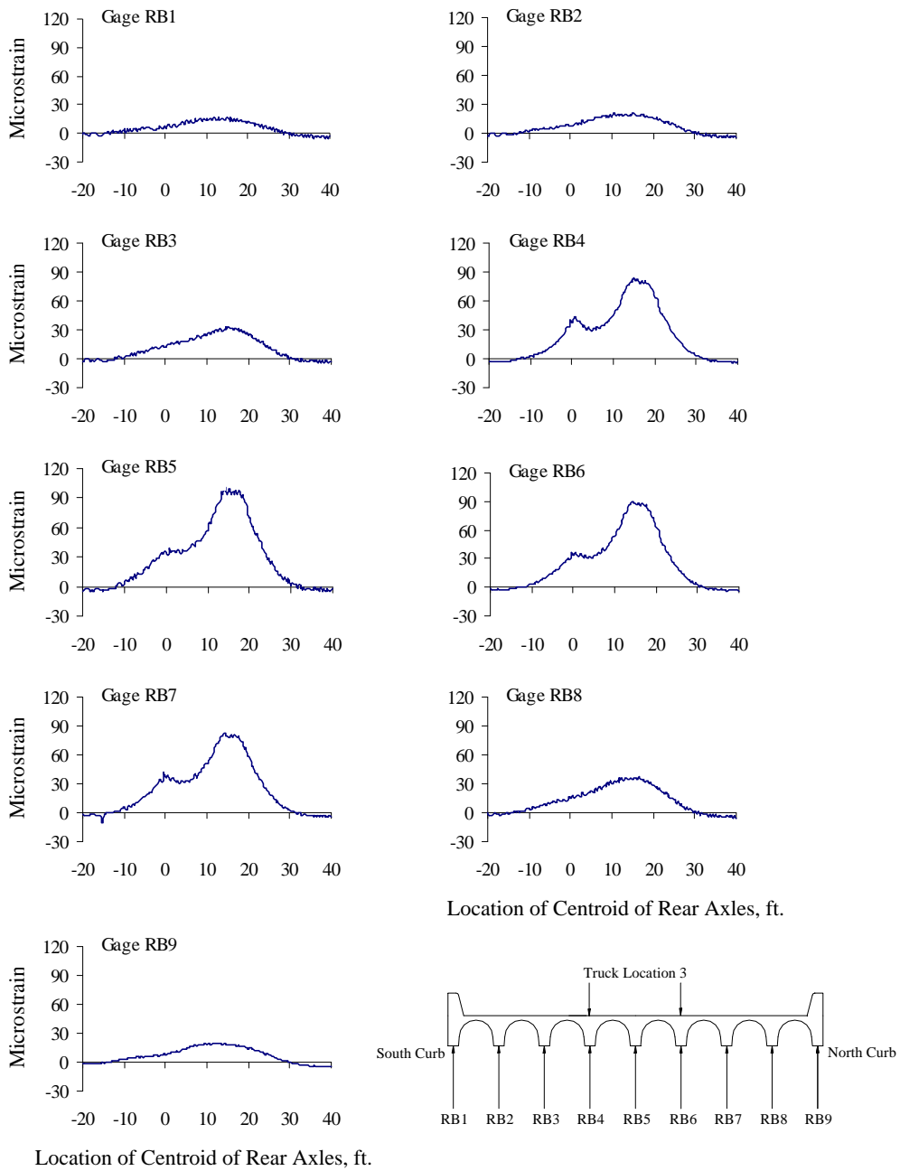
Figure A.7 Reinforcing Bar Strains at Mid-span, Test Series 2, Truck Location 3, Pass 1
