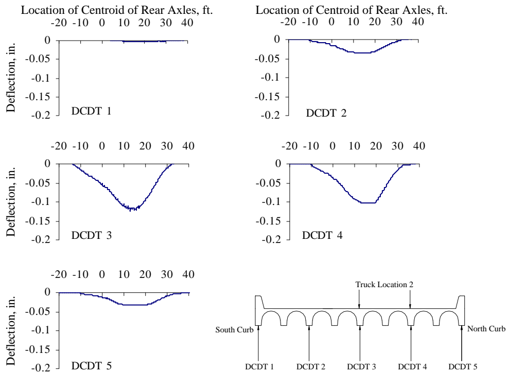
Figure G.6 Vertical Deflections Measured at Mid-span, Test Series 2, Truck Location 2, Pass 2
