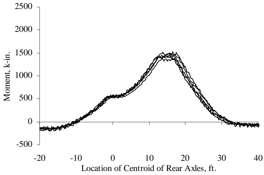
Figure 5.21 Total Moment Lines at Mid-span for Test Series 3
