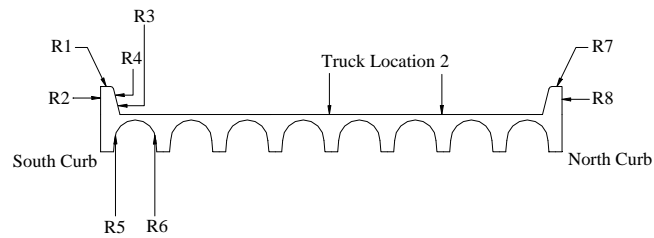
Figure C.6 Curb Strains at Mid-span, Test Series 2, Truck Location 2, Pass 2
