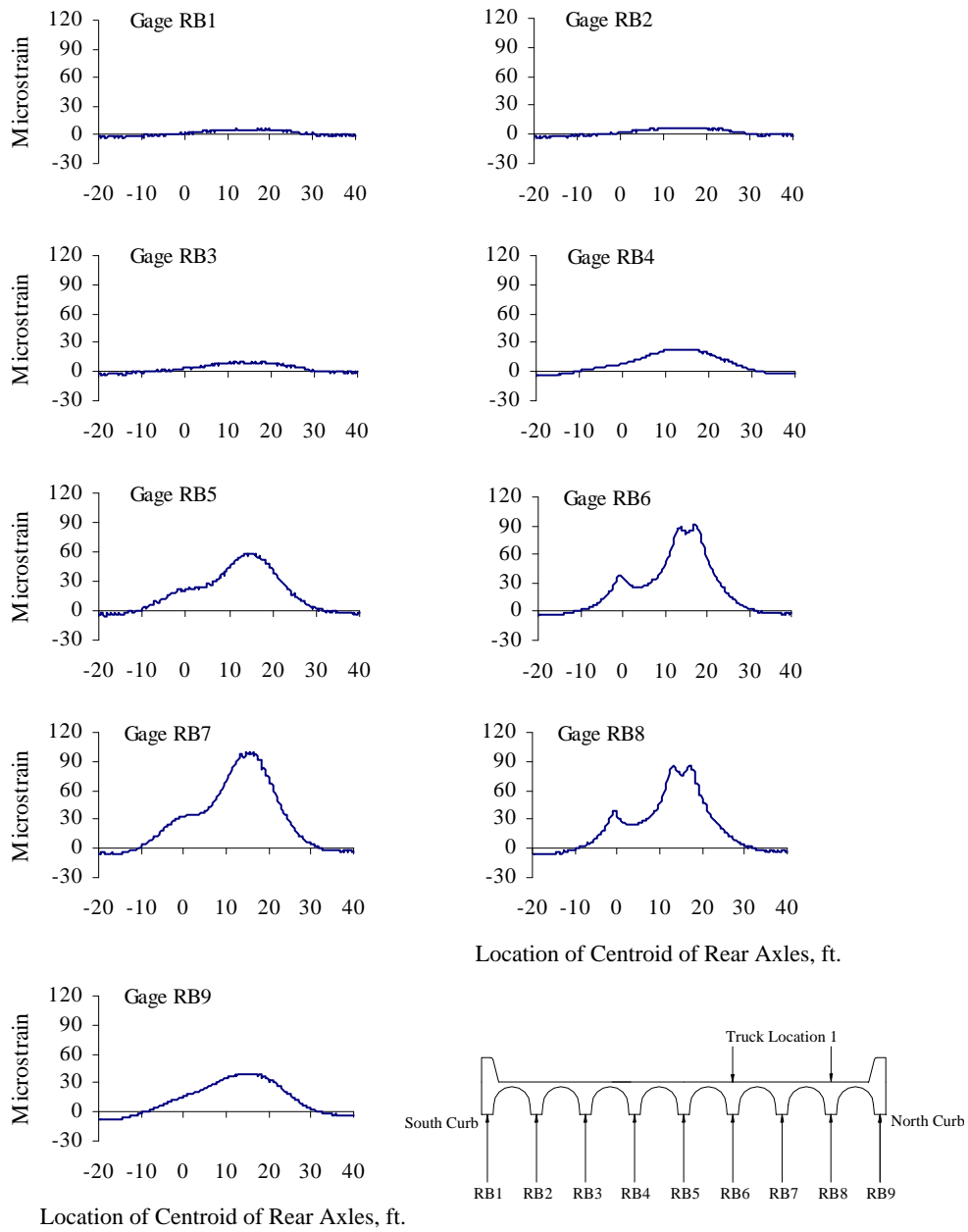
Figure A.13 Reinforcing Bar Strains at Mid-span, Test Series 3, Truck Location 1, Pass 1
