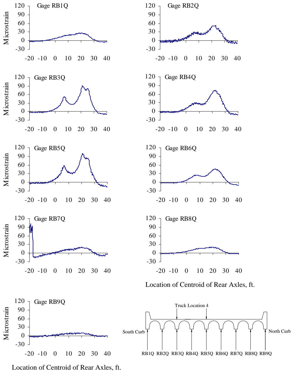
Figure B.20 Reinforcing Bar Strains at Quarter-span, Test Series 3, Truck Location 4, Pass 2
