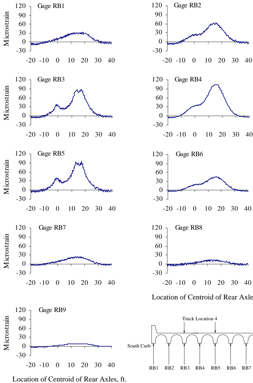
Figure A.20 Reinforcing Bar Strains at Mid-span, Test Series 3, Truck Location 4, Pass 2
