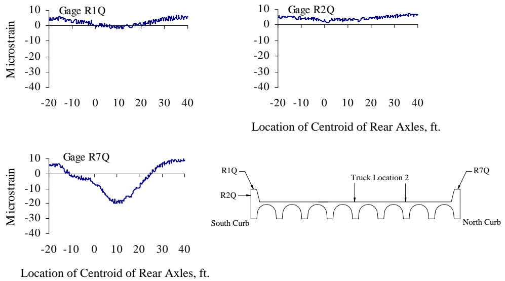
Figure D.6 Curb Strains at Quarter-span, Test Series 2, Truck Location 2, Pass 2
