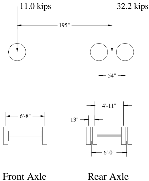
Figure 3.17 Sketch of Configuration of Truck 1
