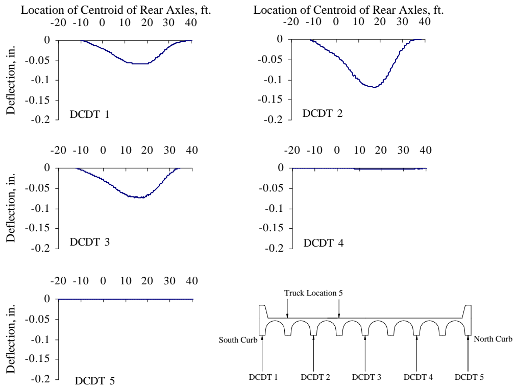
Figure G.22 Vertical Deflections Measured at Mid-span, Test Series 3, Truck Location 5, Pass 2
