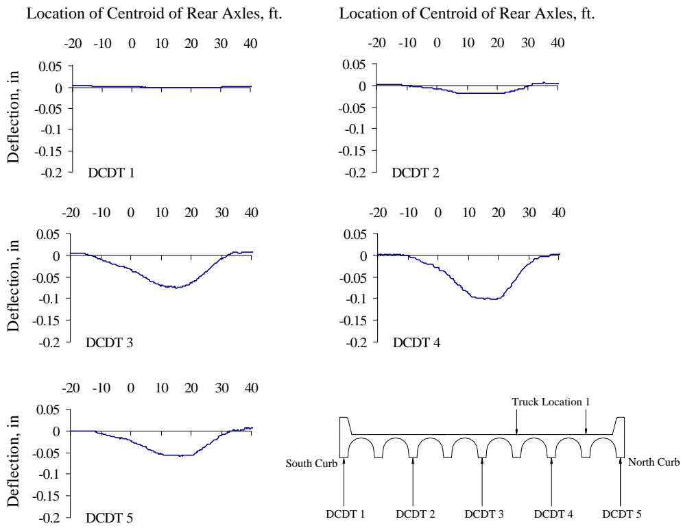
Figure 4.32 Vertical Deflections Measured at Mid-span, Test Series 2, Truck Location 1, Pass 1
