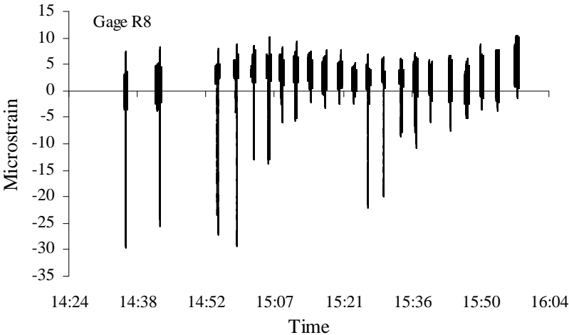
Figure 4.3 Drift in Wire Strain Gage not Exposed to Sunlight, Test Series 1 through 3
