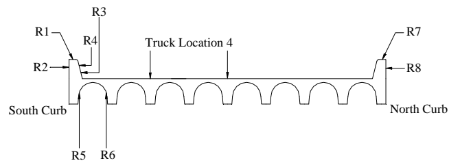
Figure C.20 Curb Strains at Mid-span, Test Series 3, Truck Location 4, Pass 2
