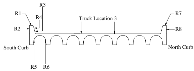
Figure C.7 Curb Strains at Mid-span, Test Series 2, Truck Location 3, Pass 1
