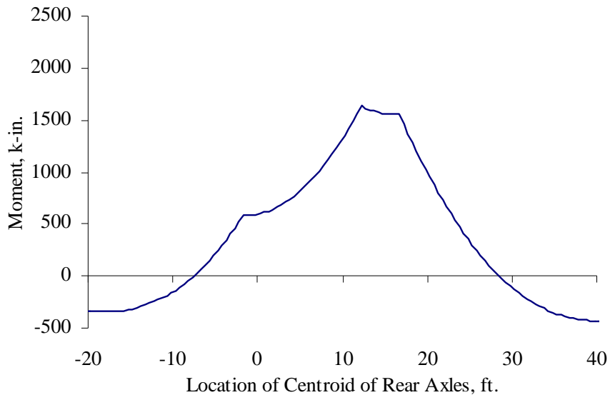
Figure 5.3 Moment Line at Mid-span for a Continuous Beam
