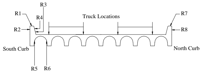
Figure C.2 Curb Strains at Mid-span, Test Series 1, Pass 2
