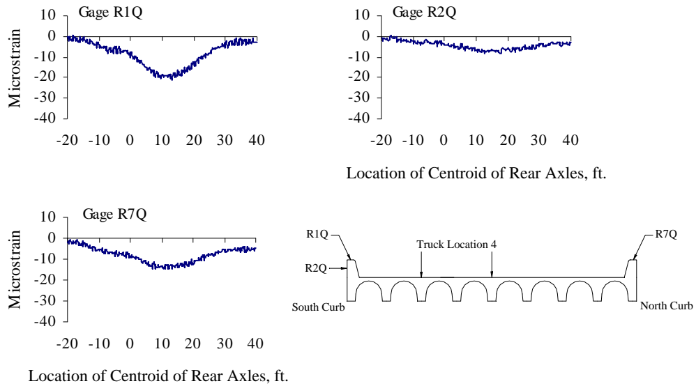
Figure D.9 Curb Strains at Quarter-span, Test Series 2, Truck Location 4, Pass 1
