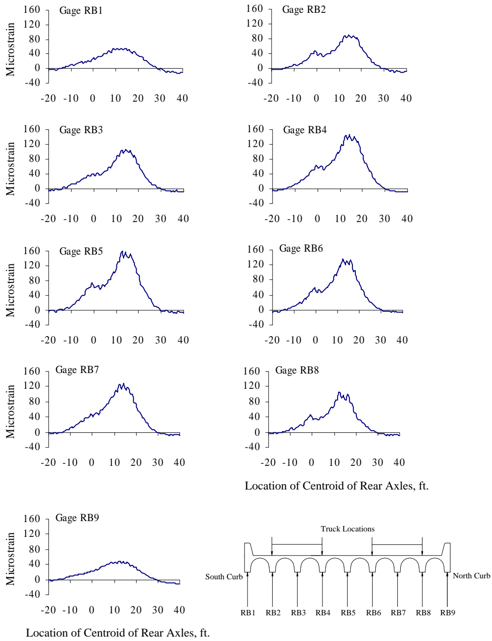
Figure A.2 Reinforcing Bar Strains at Mid-span, Test Series 1, Pass 2
