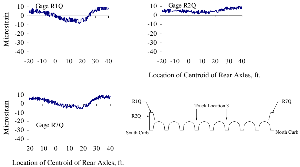
Figure D.18 Curb Strains at Quarter-span, Test Series 3, Truck Location 3, Pass 2
