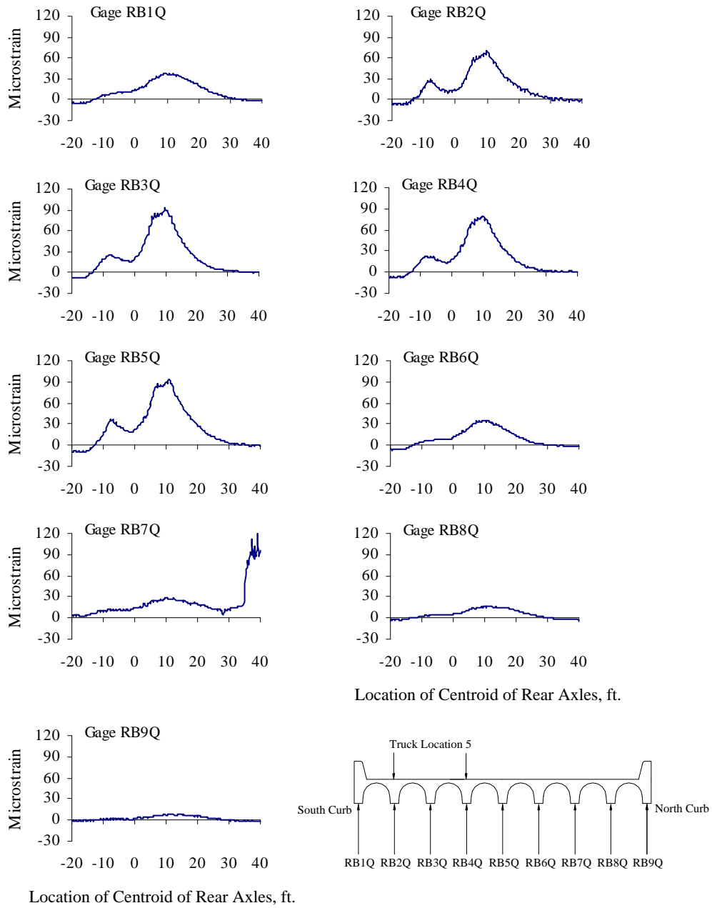
Figure B.12 Reinforcing Bar Strains at Quarter-span, Test Series 2, Truck Location 5, Pass 2
