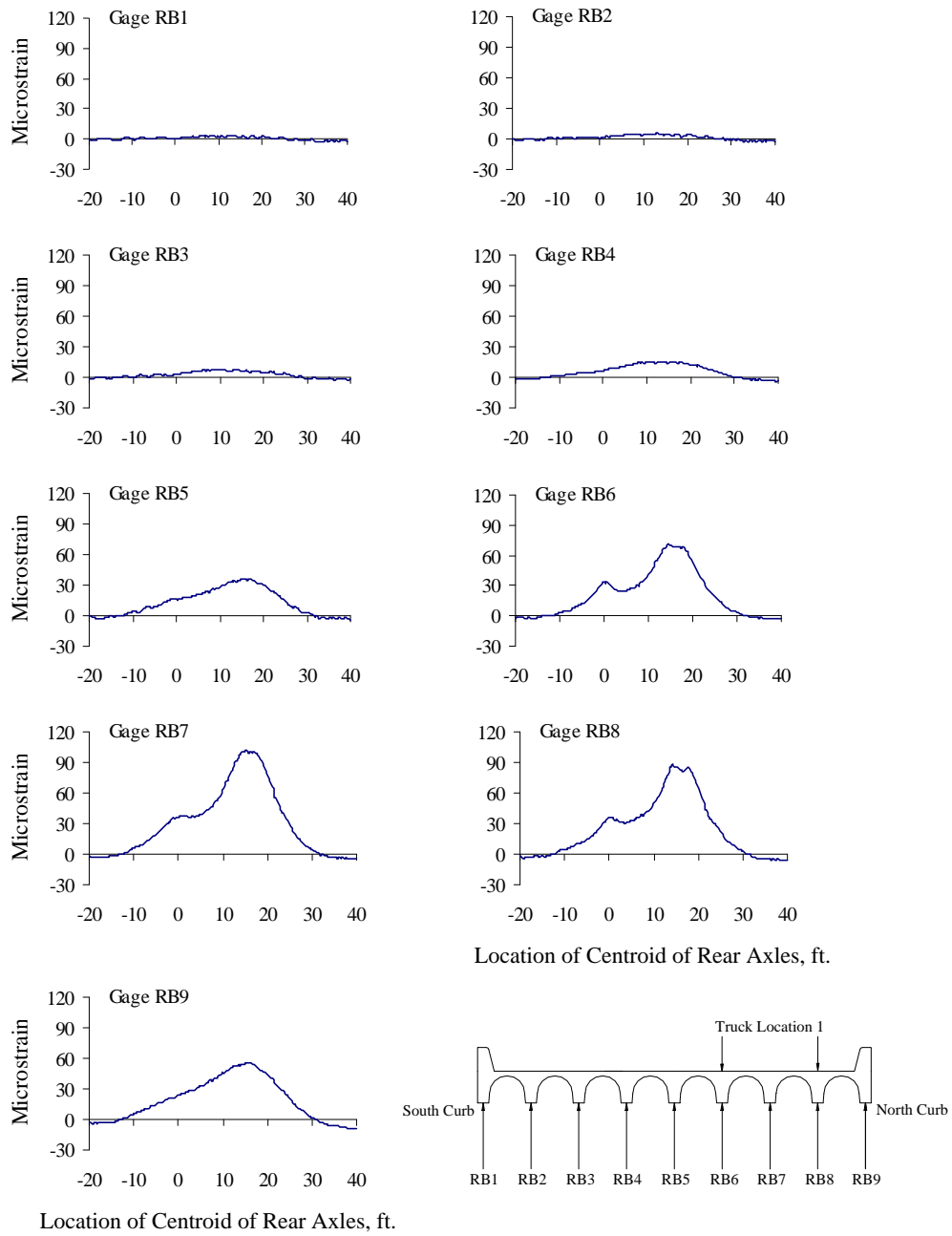
Figure A.4 Reinforcing Bar Strains at Mid-span, Test Series 2, Truck Location 1, Pass 2
