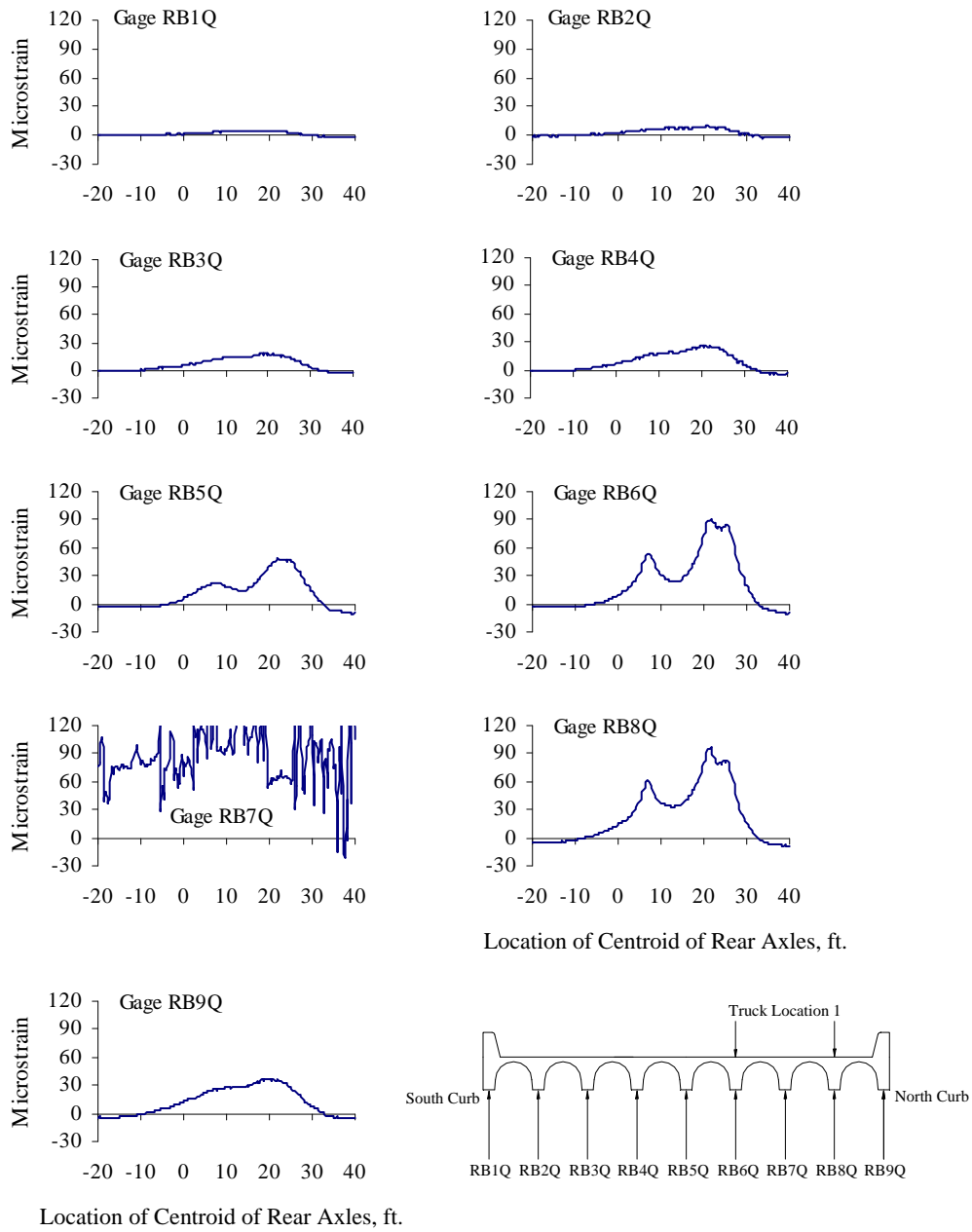
Figure B.14 Reinforcing Bar Strains at Quarter-span, Test Series 3, Truck Location 1, Pass 2
