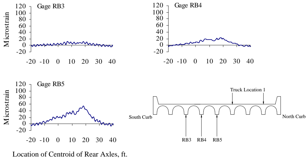
Figure A.25 Reinforcing Bar Strains at Mid-span, Test Series 5, Truck Location 1, Pass 1
