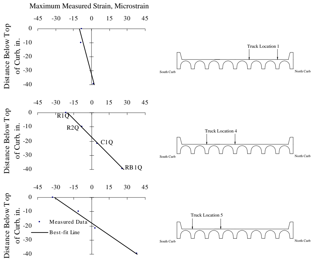
Figure 4.30 Measured Strain Gradients within South Curb at Quarter-span
