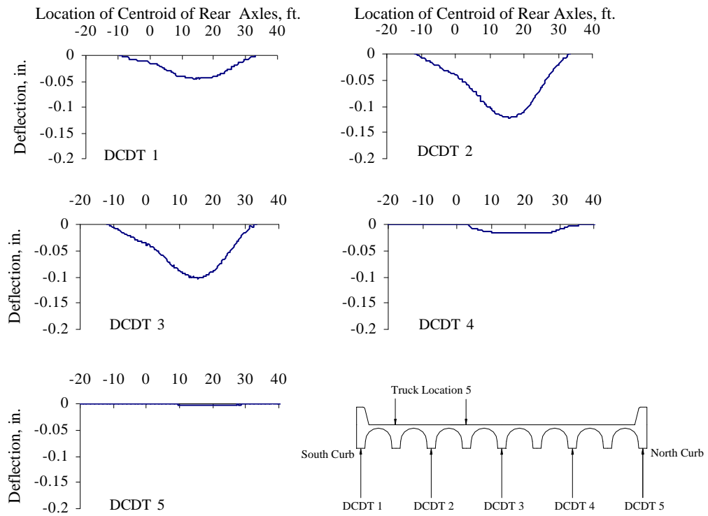
Figure G.11 Vertical Deflections Measured at Mid-span, Test Series 2, Truck Location 5, Pass 1
