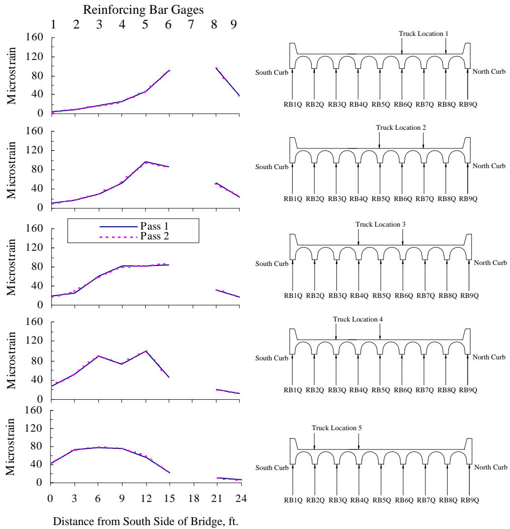
Figure 4.20 Profiles of Maximum Reinforcing Bar Strains at Quarter-span for Test Series 3
