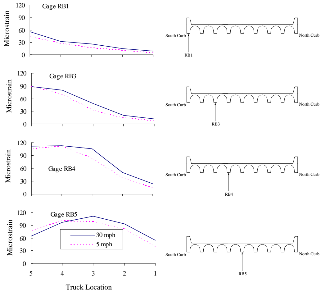
Figure 4.16 Comparison of Maximum Strains at Mid-span for 30 mph and 5 mph Runs
