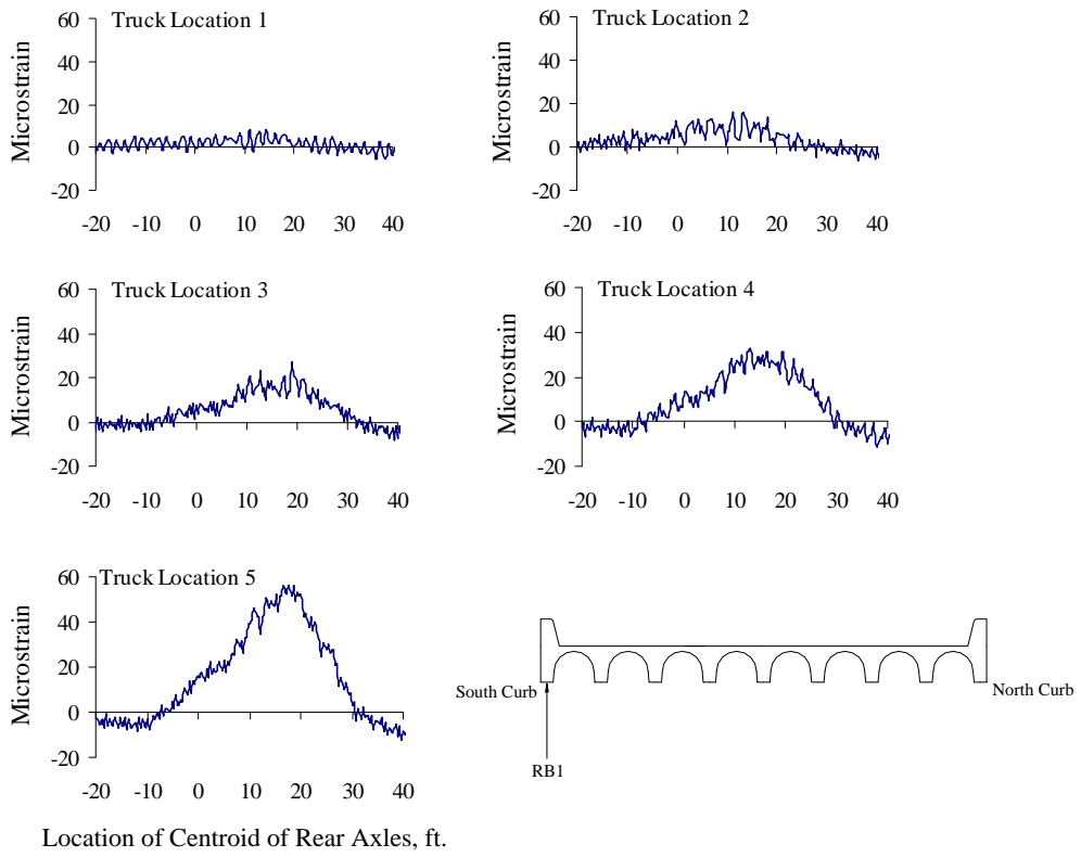
Figure A.24 Strains for Gage RB1 at Mid-span, Test Series 4, Pass 2
