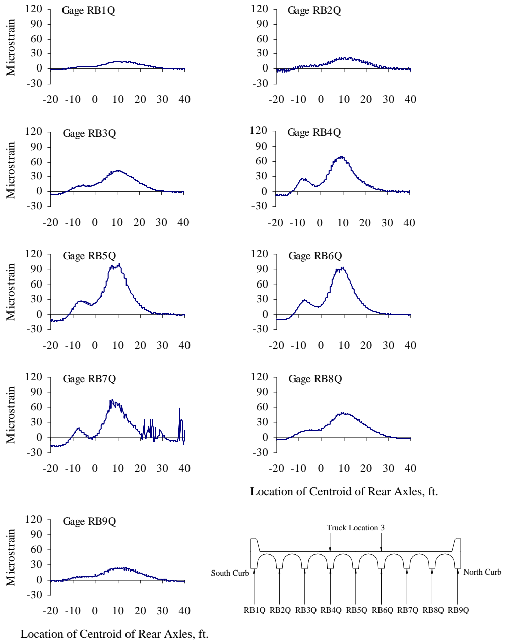
Figure B.8 Reinforcing Bar Strains for Quarter-span, Test Series 2, Truck Location 3, Pass 2
