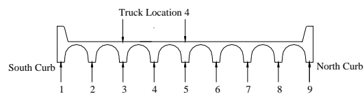
Figure 5.25 Unsymmetrical Loading for Truck Locations 2 and 4
