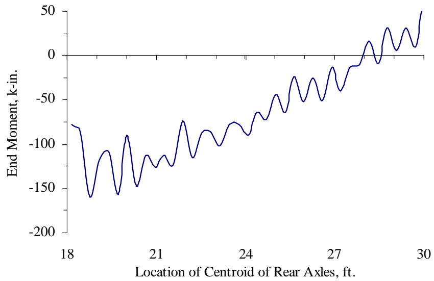
Figure 5.43 End Moment at East Support, Test Series 2, Truck Location 4
