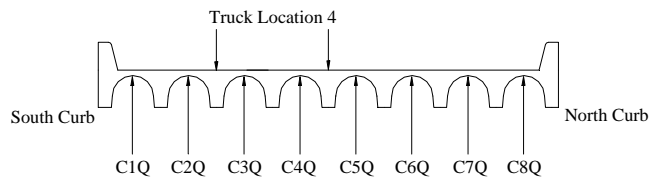
Figure F.9 Crown Strains at Quarter-span, Test Series 2, Truck Location 4, Pass 1
