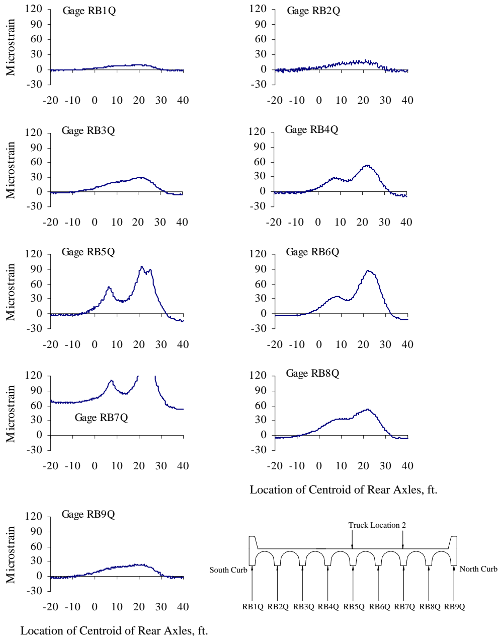
Figure B.16 Reinforcing Bar Strains at Quarter-span, Test Series 3, Truck Location 2, Pass 2
