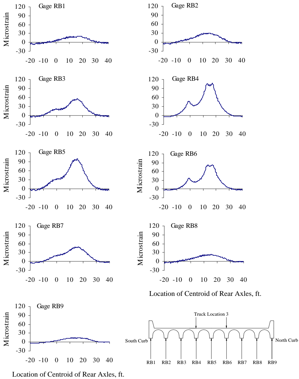
Figure A.17 Reinforcing Bar Strains at Mid-span, Test Series 3, Truck Location 3, Pass 1
