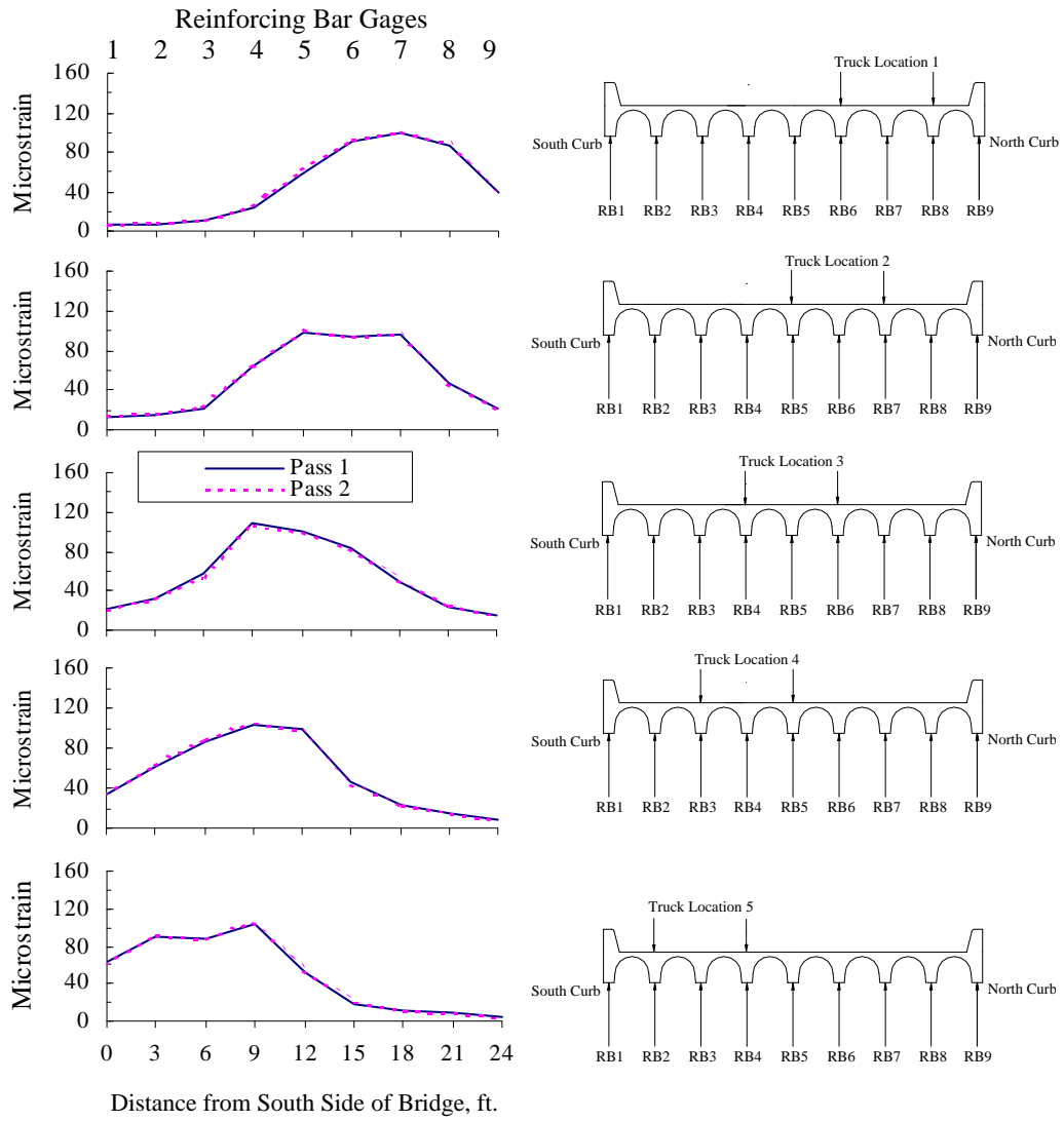
Figure 4.14 Profiles of Maximum Reinforcing Bar Strains at Mid-span for Test Series 3
