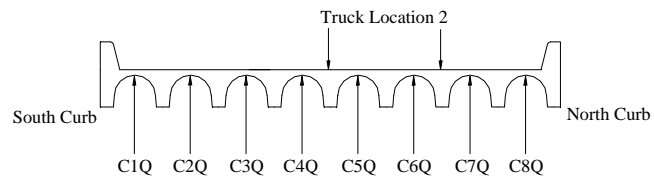
Figure F.5 Crown Strains at Quarter-span, Test Series 2, Truck Location 2, Pass 1
