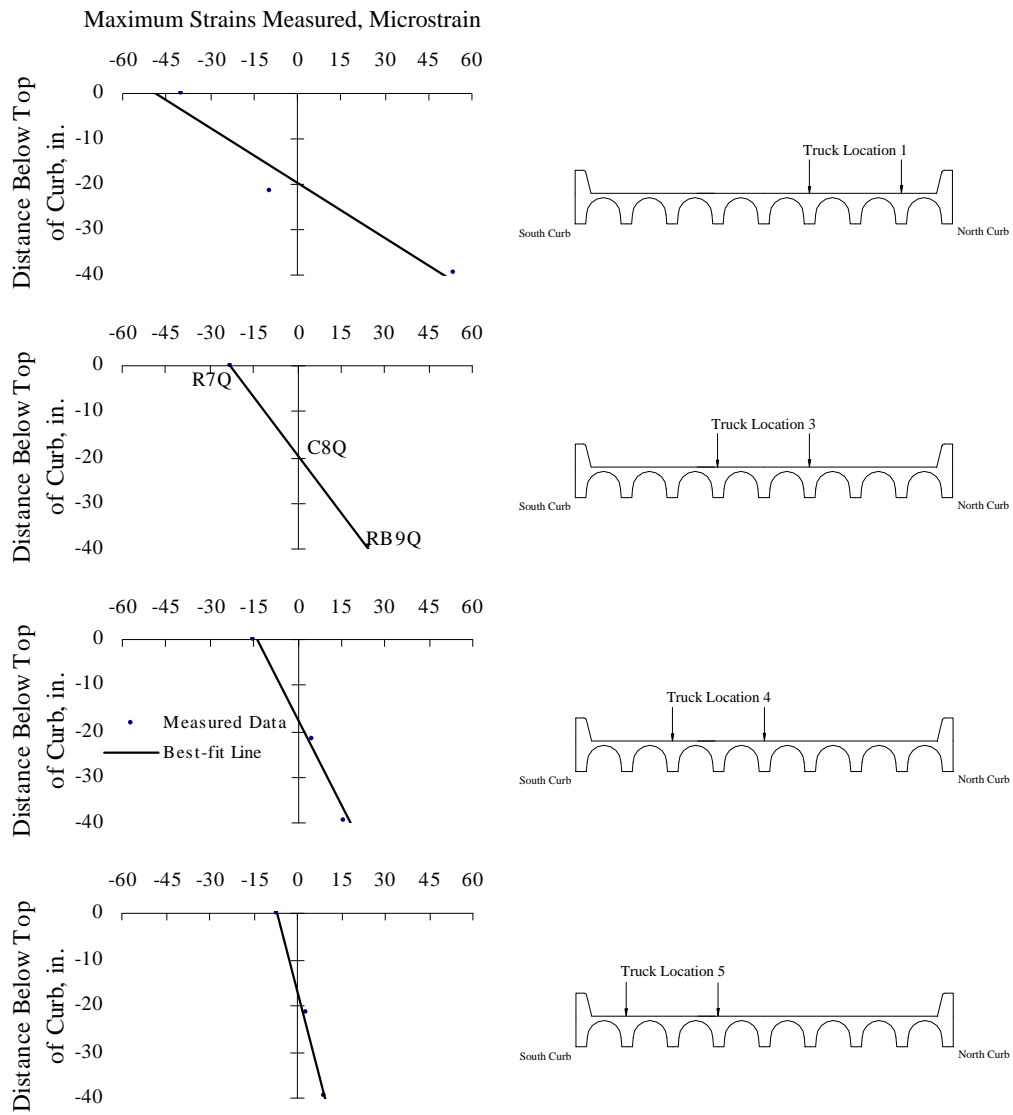
Figure 4.31 Measured Strain Gradients within North Curb at Quarter-span
