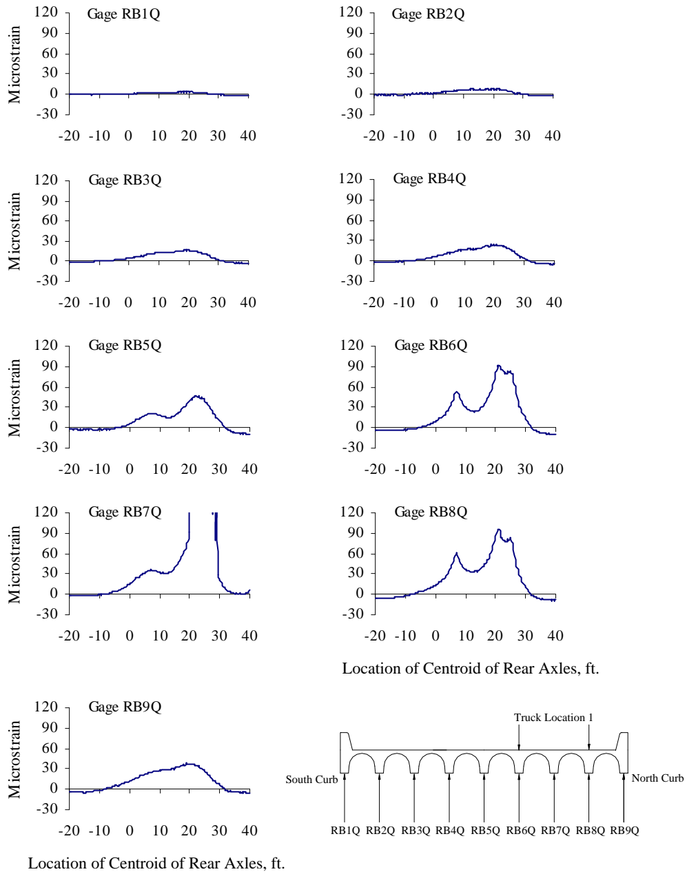
Figure B.13 Reinforcing Bar Strains at Quarter-span, Test Series 3, Truck Location 1, Pass 1
