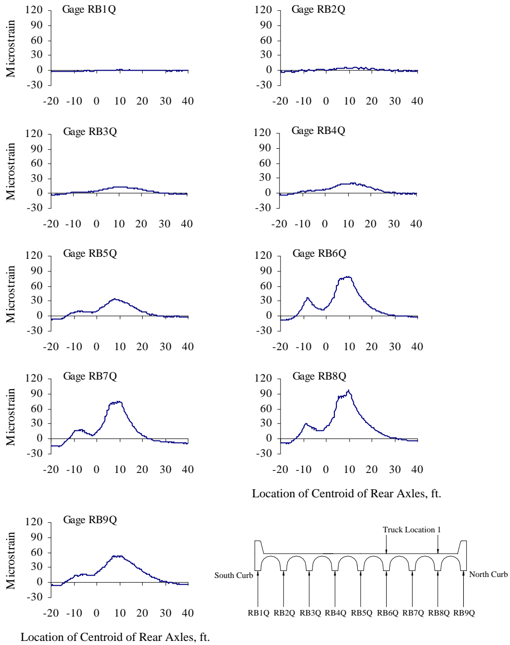
Figure B.4 Reinforcing Bar Strains at Quarter-span, Test Series 2, Truck Location 1, Pass 2
