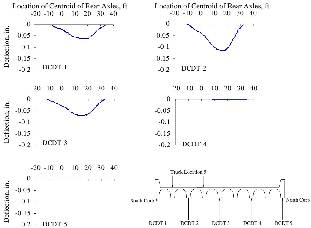
Figure G.21 Vertical Deflections Measured at Mid-span, Test Series 3, Truck Location 5, Pass 1
