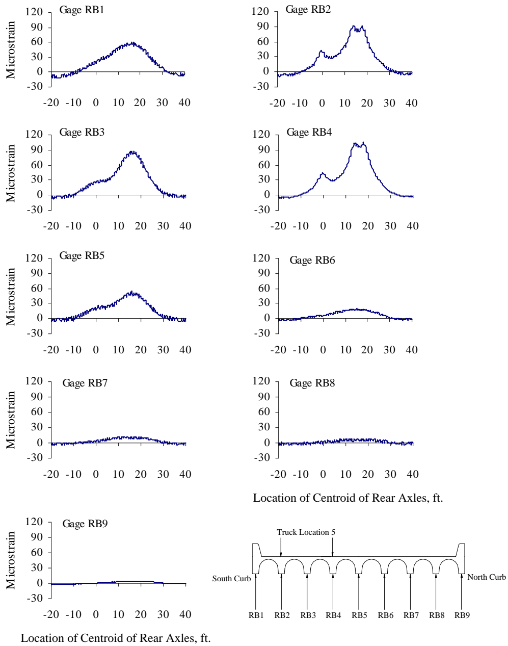
Figure A.22 Reinforcing Bar Strains at Mid-span, Test Series 3, Truck Location 5, Pass 2
