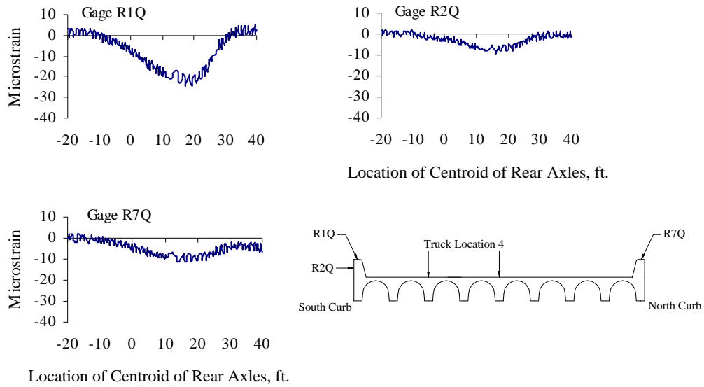
Figure D.19 Curb Strains at Quarter-span, Test Series 3, Truck Location 4, Pass 1
