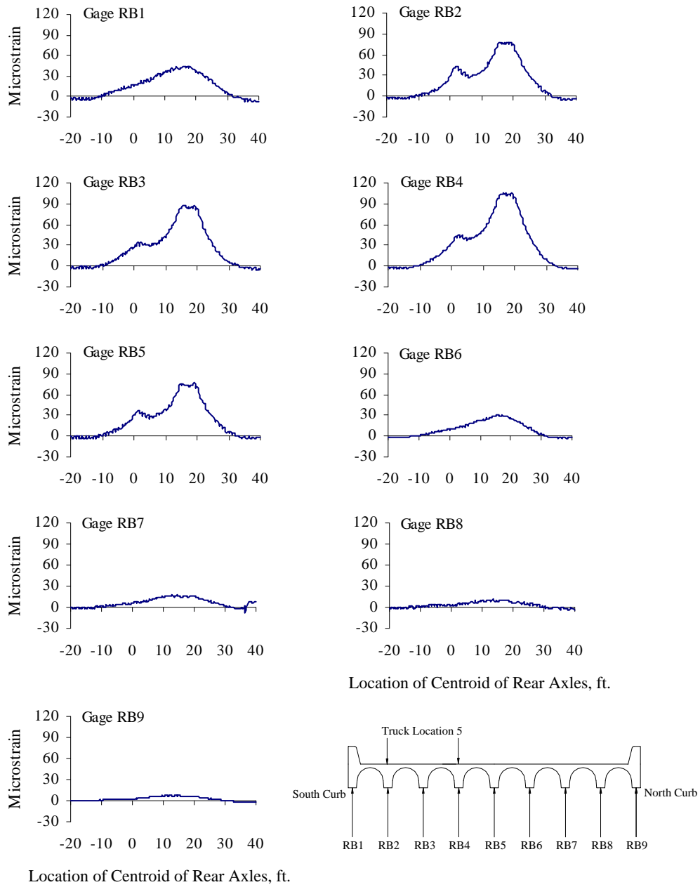
Figure A.11 Reinforcing Bar Strains at Mid-span, Test Series 2, Truck Location 5, Pass 1
