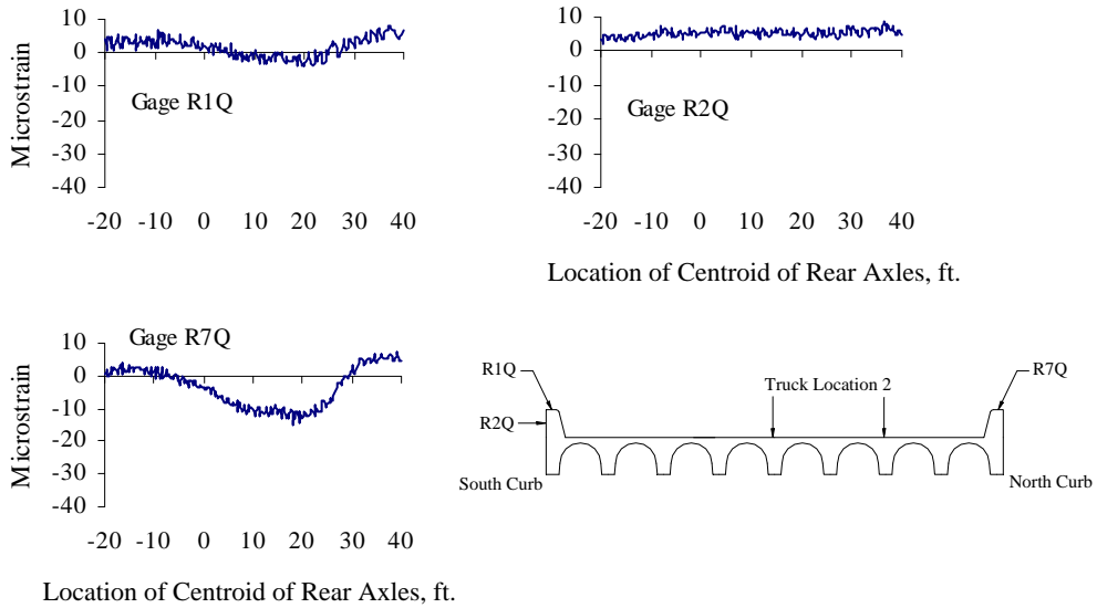
Figure D.16 Curb Strains at Quarter-span, Test Series 3, Truck Location 2, Pass 2
