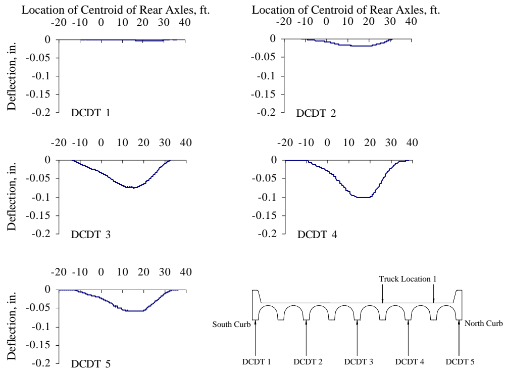
Figure G.3 Vertical Deflections Measured at Mid-span, Test Series 2, Truck Location 1, Pass 1
