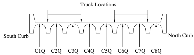
Figure F.1 Crown Strains at Quarter-span, Test Series 1, Pass 1
