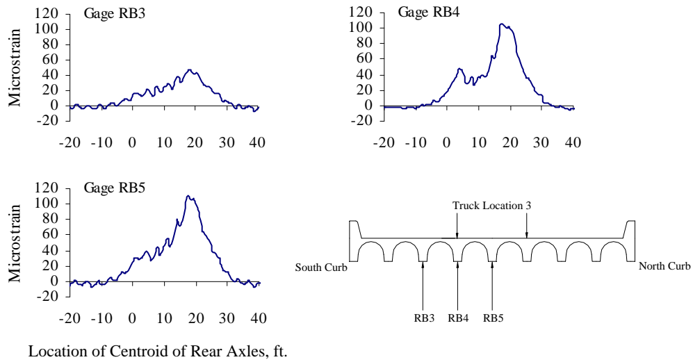
Figure A.30 Reinforcing Bar Strains at Mid-span, Test Series 5, Truck Location 3, Pass 2
