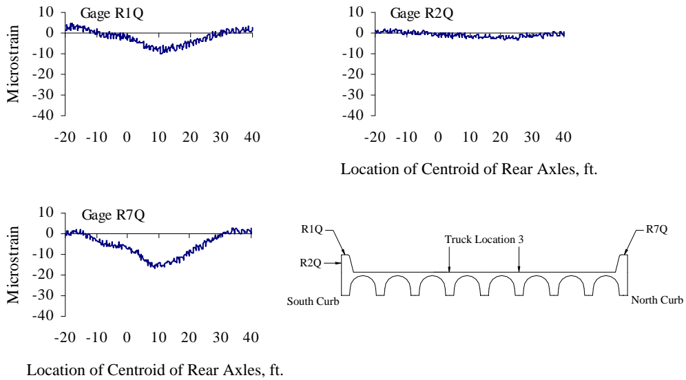
Figure D.8 Curb Strains at Quarter-span, Test Series 2, Truck Location 3, Pass 2
