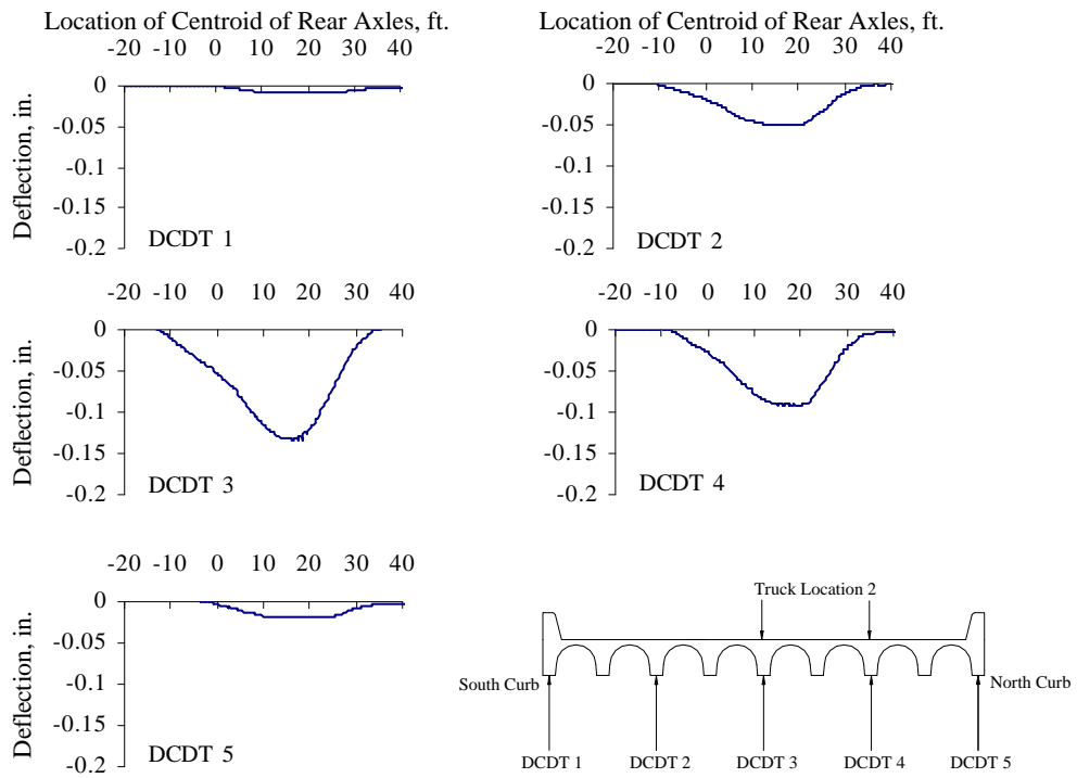
Figure G.16 Vertical Deflections Measured at Mid-span, Test Series 3, Truck Location 2, Pass 2
