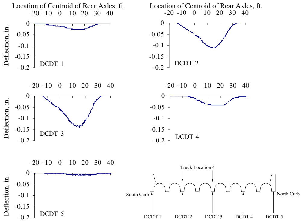
Figure G.9 Vertical Deflections Measured at Mid-span, Test Series 2, Truck Location 4, Pass 1
