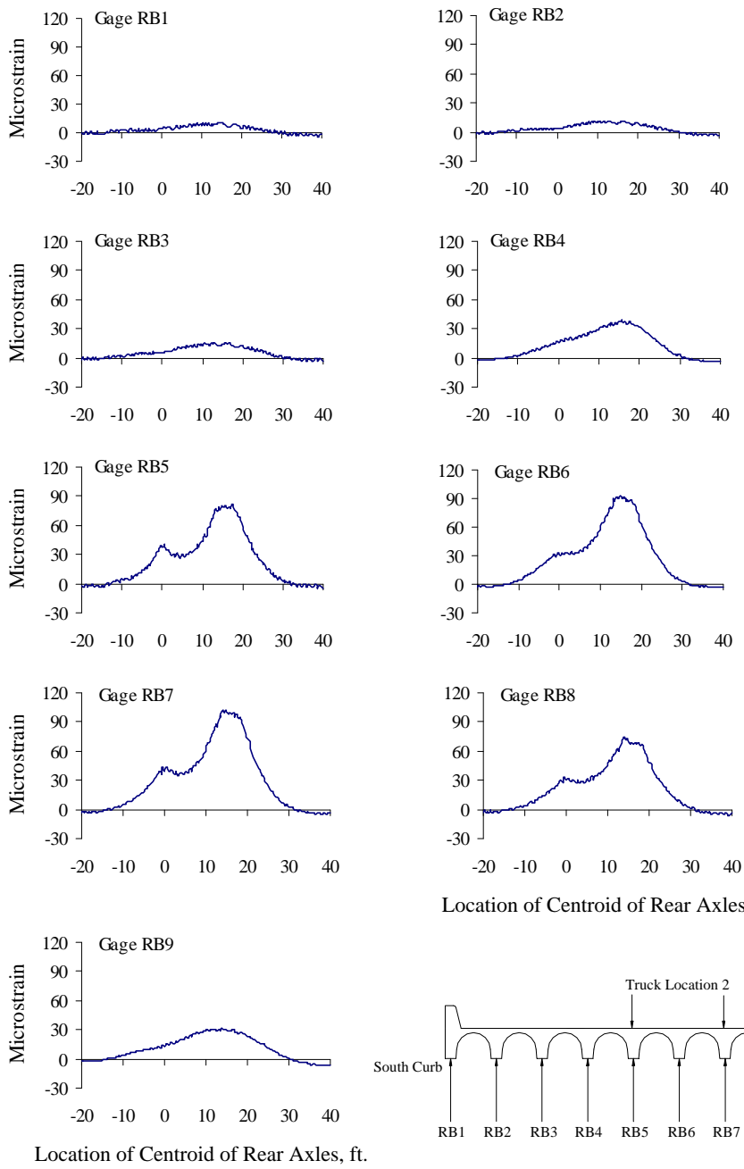
Figure A.6 Reinforcing Bar Strains at Mid-span, Test Series 2, Truck Location 2, Pass 2
