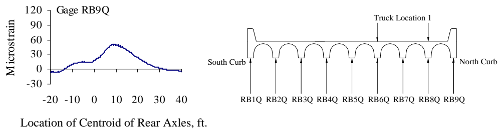
Figure 4.17 Reinforcing Bar Strains at Quarter-span, Test Series 2, Truck Location 1, Pass 1
