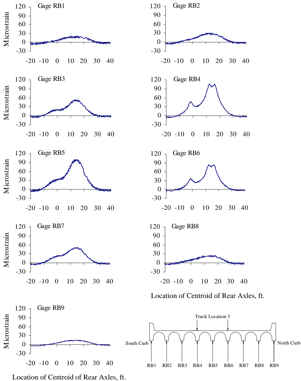
Figure A.18 Reinforcing Bar Strains at Mid-span, Test Series 3, Truck Location 3, Pass 2
