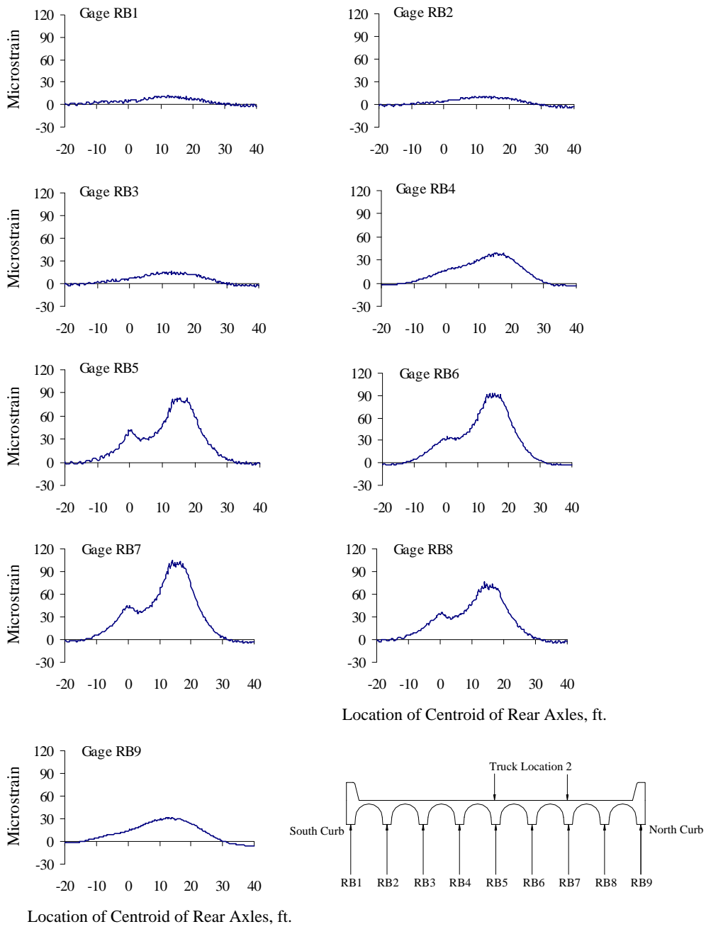
Figure A.5 Reinforcing Bar Strains at Mid-span, Test Series 2, Truck Location 2, Pass 1
