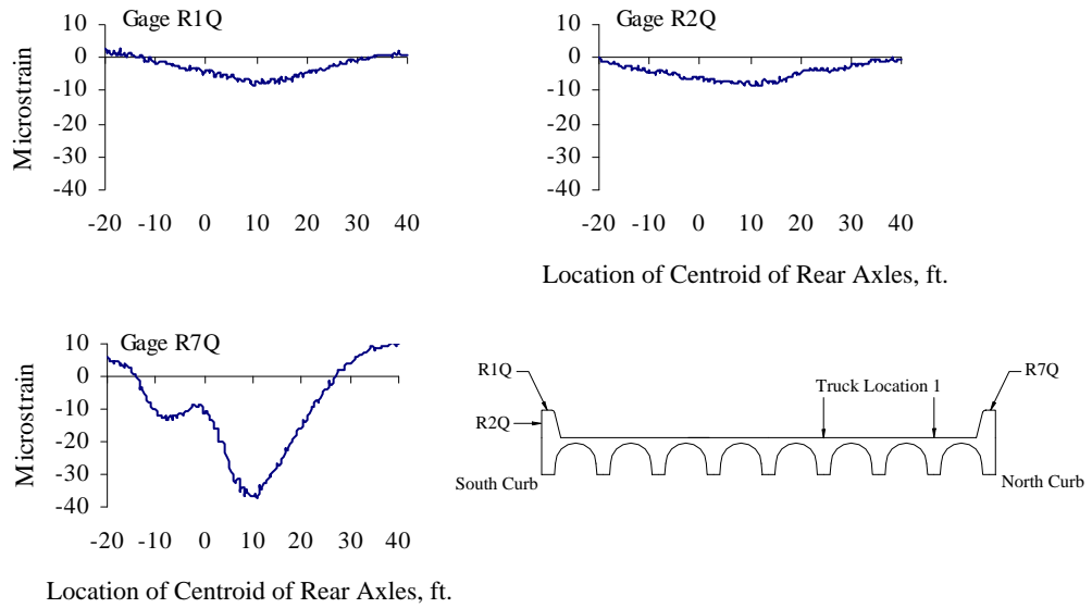
Figure D.3 Curb Strains at Quarter-span, Test Series 2, Truck Location 1, Pass 1
