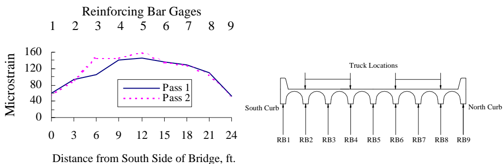
Figure 4.12 Profile of Maximum Reinforcing Bar Strains at Mid-span for Test Series 1
