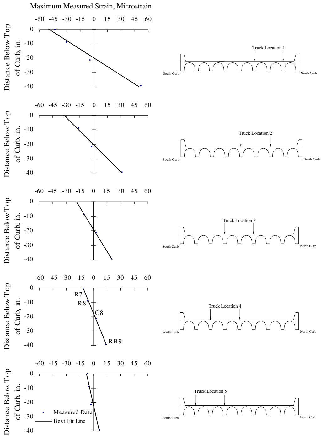
Figure 4.29 Measured Strain Gradients within North Curb at Mid-span
