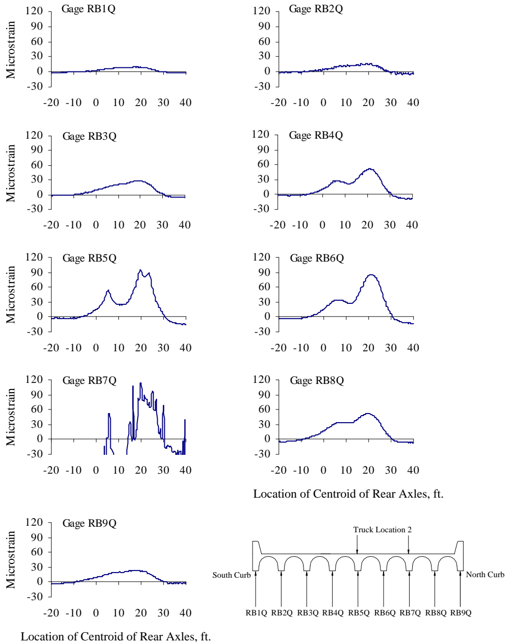
Figure B.15 Reinforcing Bar Strains at Quarter-span, Test Series 3, Truck Location 2, Pass 1
