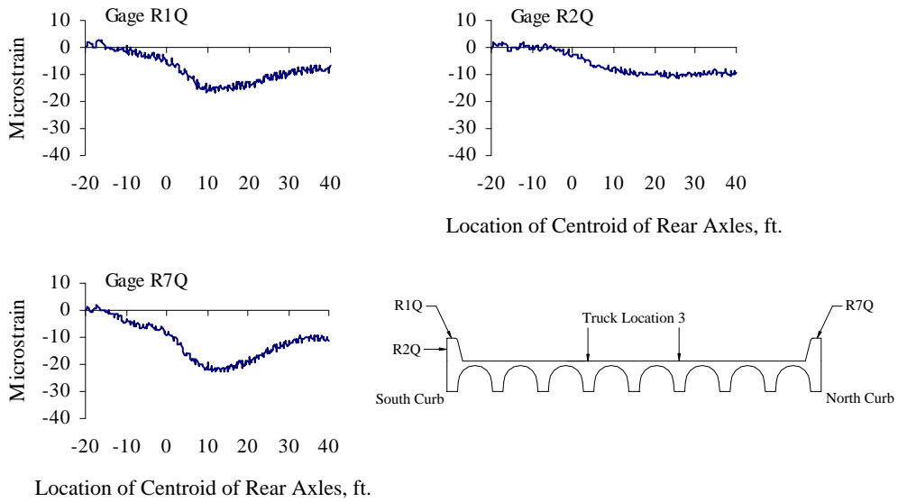
Figure D.7 Curb Strains at Quarter-span, Test Series 2, Truck Location 3, Pass 1
