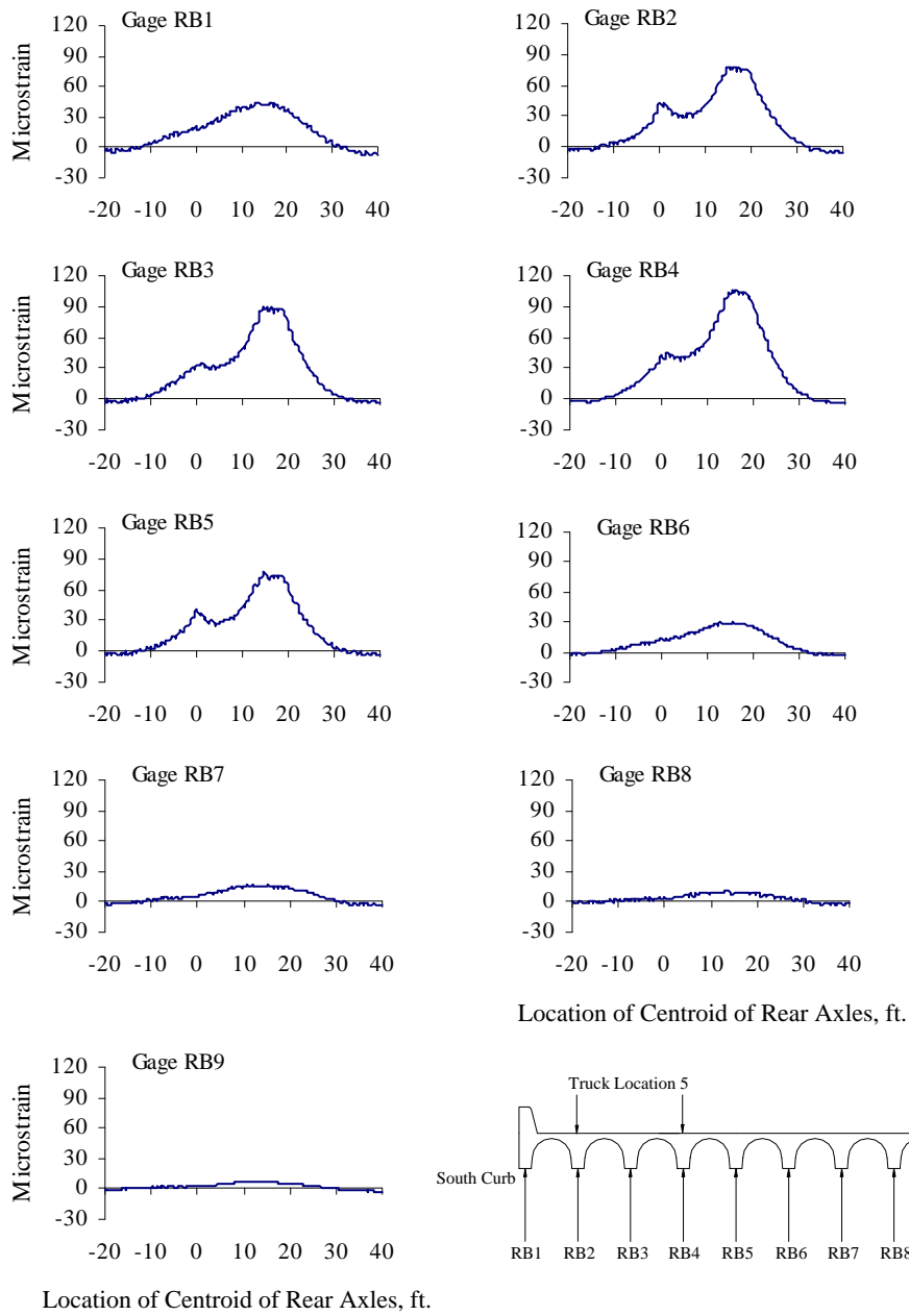
Figure A.12 Reinforcing Bar Strains at Mid-span, Test Series 2, Truck Location 5, Pass 2
