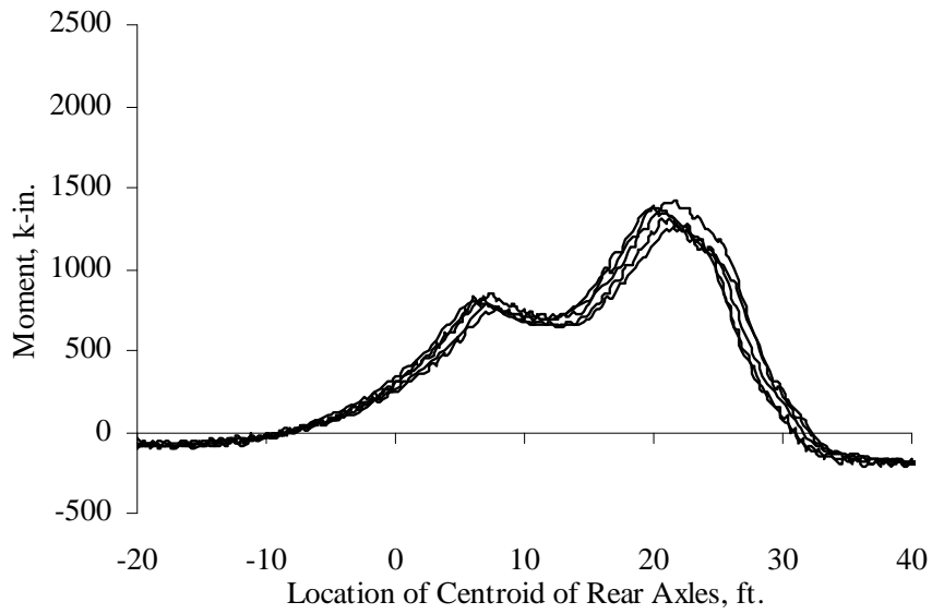
Figure 5.22 Total Moment Lines at Quarter-span for Test Series 3
