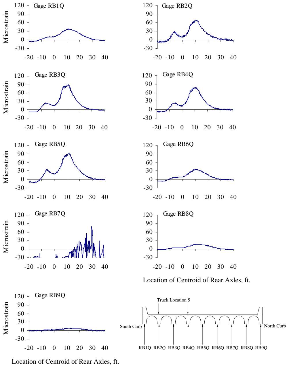
Figure B.11 Reinforcing Bar Strains at Quarter-span, Test Series 2, Truck Location 5, Pass 1
