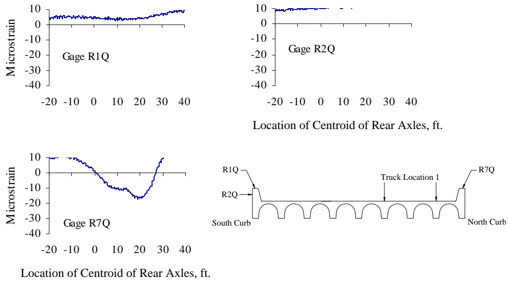
Figure D.13 Curb Strains at Quarter-span, Test Series 3, Truck Location 1, Pass 1
