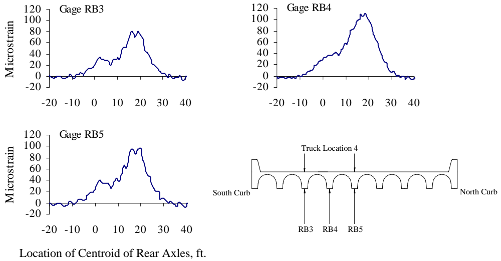
Figure A.32 Reinforcing Bar Strains at Mid-span, Test Series 5, Truck Location 4, Pass 2
