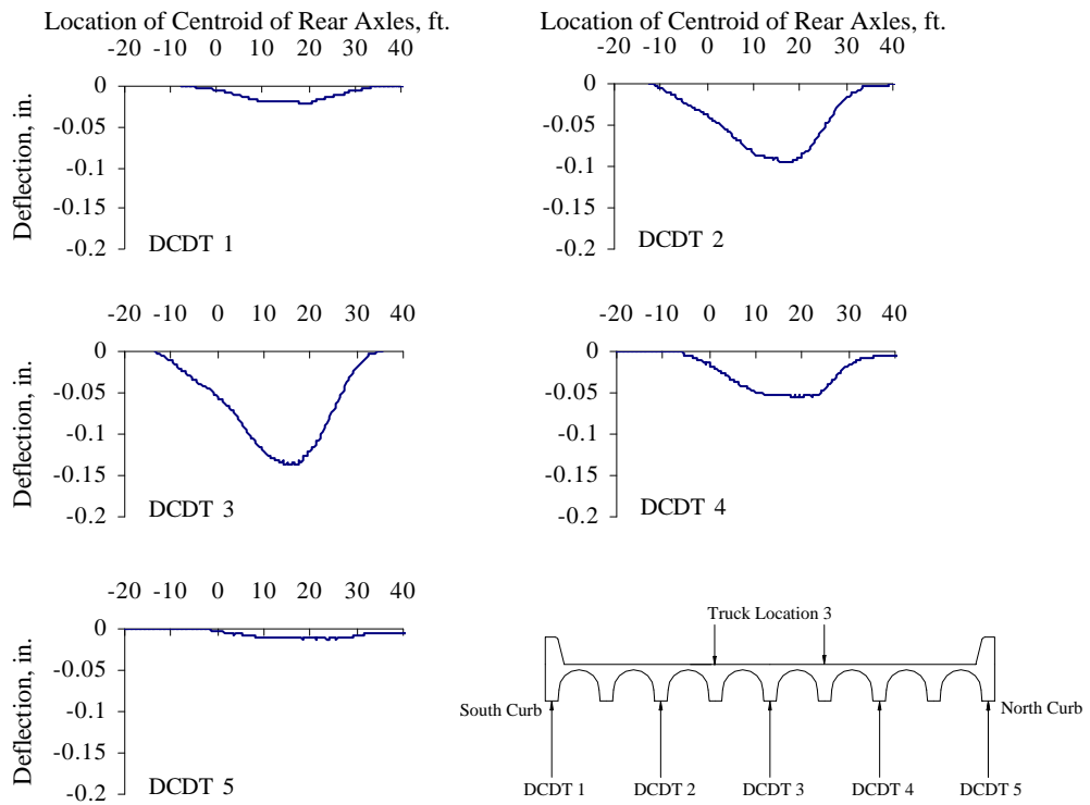
Figure G.17 Vertical Deflections Measured at Mid-span, Test Series 3, Truck Location 3, Pass 1
