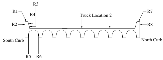
Figure C.5 Curb Strains at Mid-span, Test Series 2, Truck Location 2, Pass 1
