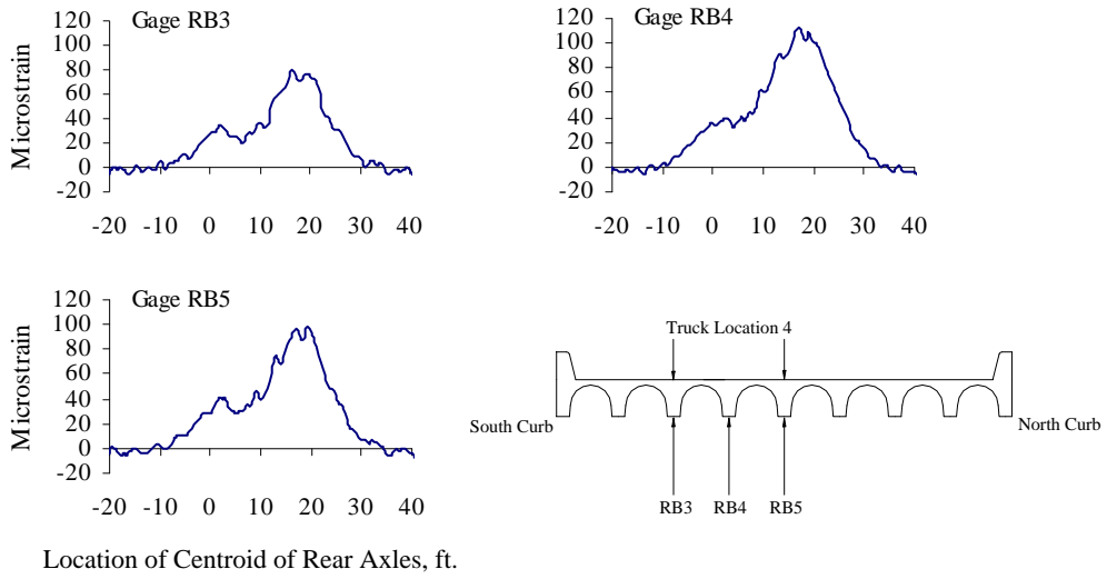
Figure A.31 Reinforcing Bar Strains at Mid-span, Test Series 5, Truck Location 4, Pass 1
