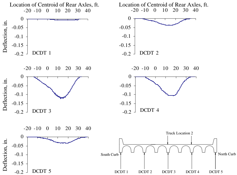
Figure G.5 Vertical Deflections Measured at Mid-span, Test Series 2, Truck Location 2, Pass 1
