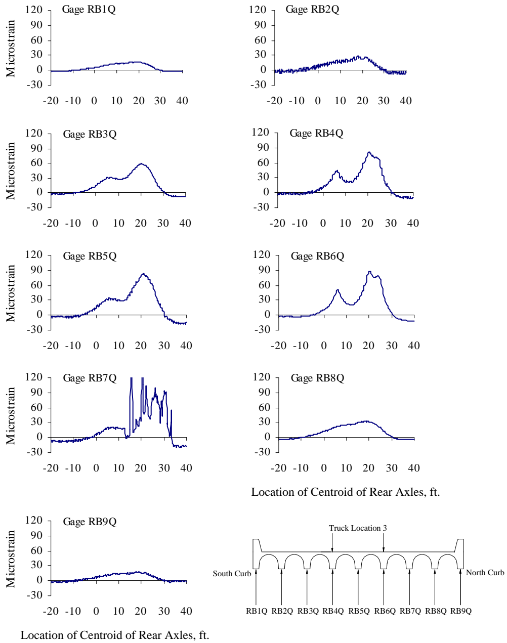
Figure B.18 Reinforcing Bar Strains at Quarter-span, Test Series 3, Truck Location 3, Pass 2
