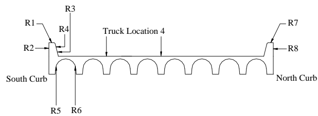
Figure C.10 Curb Strains at Mid-span, Test Series 2, Truck Location 4, Pass 2
