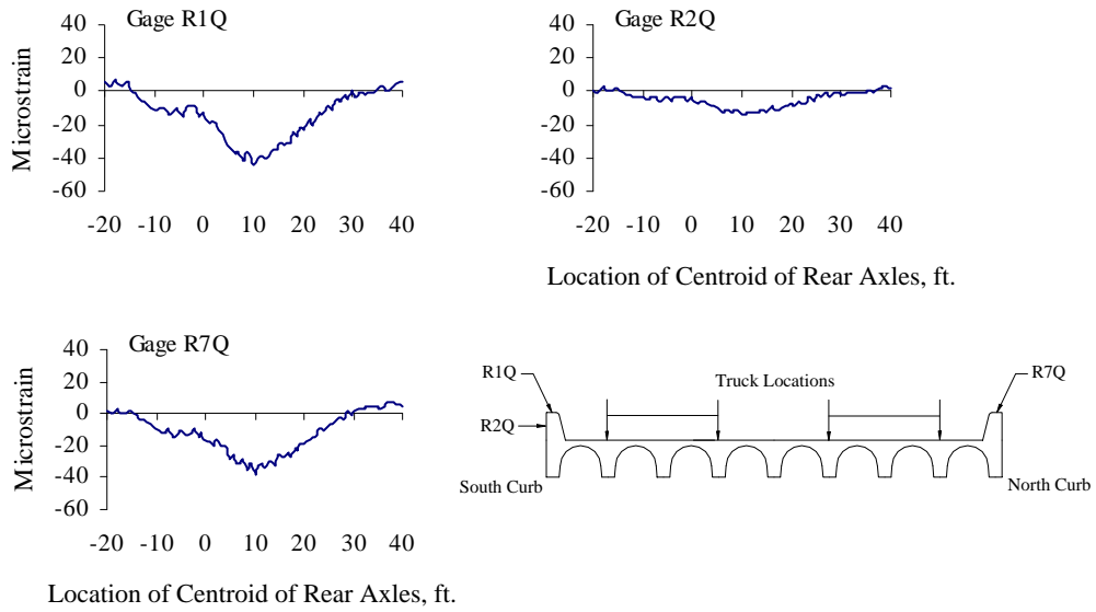
Figure D.1 Curb Strains at Quarter-span, Test Series 1, Pass 1
