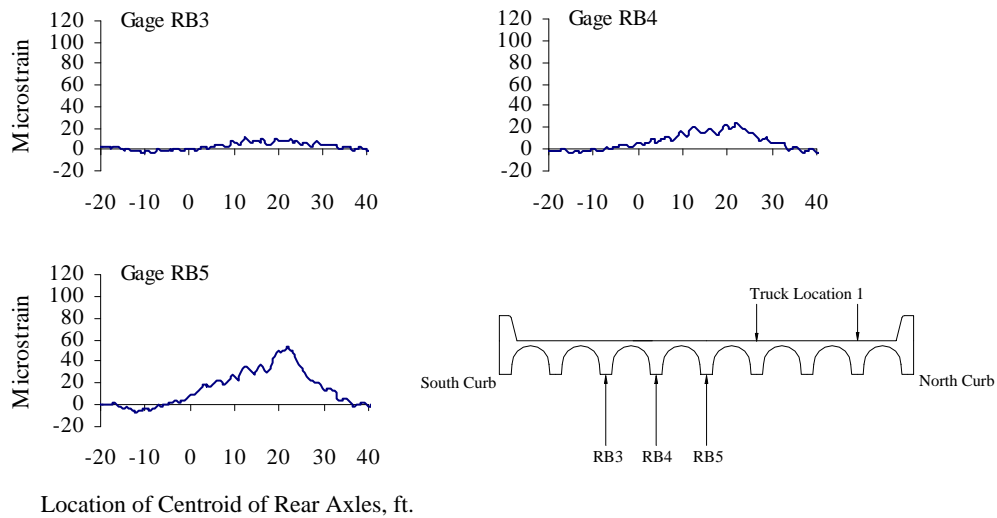
Figure A.26 Reinforcing Bar Strains at Mid-span, Test Series 5, Truck Location 1, Pass 2
