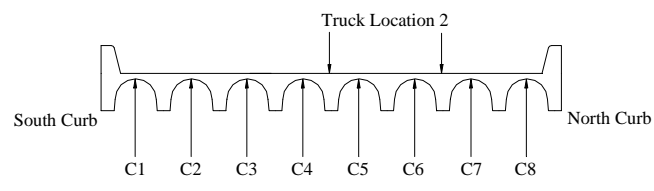
Figure E.15 Crown Strains at Mid-span, Test Series 3, Truck Location 2, Pass 1
