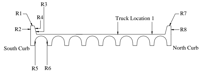
Figure C.14 Curb Strains at Mid-span, Test Series 3, Truck Location 1, Pass 2
