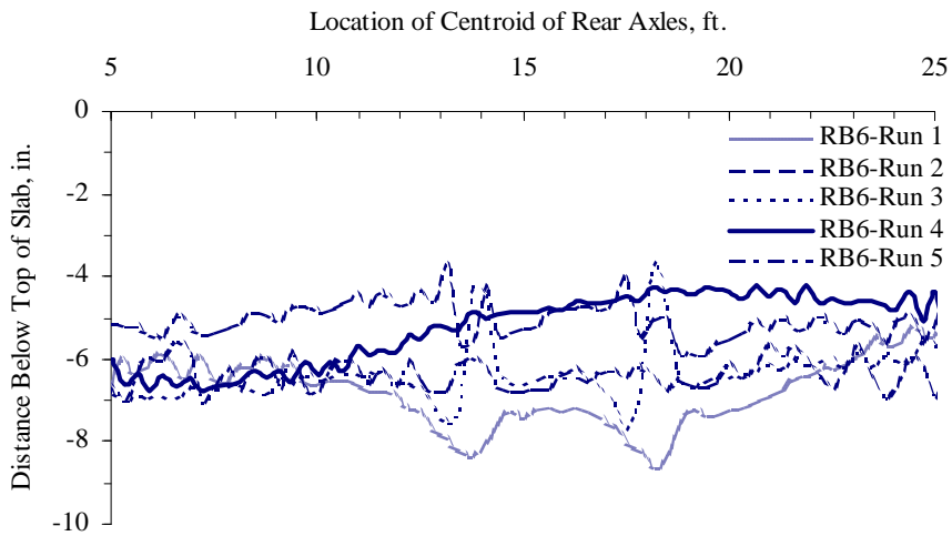
Figure 5.12 Variation in Neutral Axis Depth Calculated from Measured Strains for an Interior Girder at Mid-span
