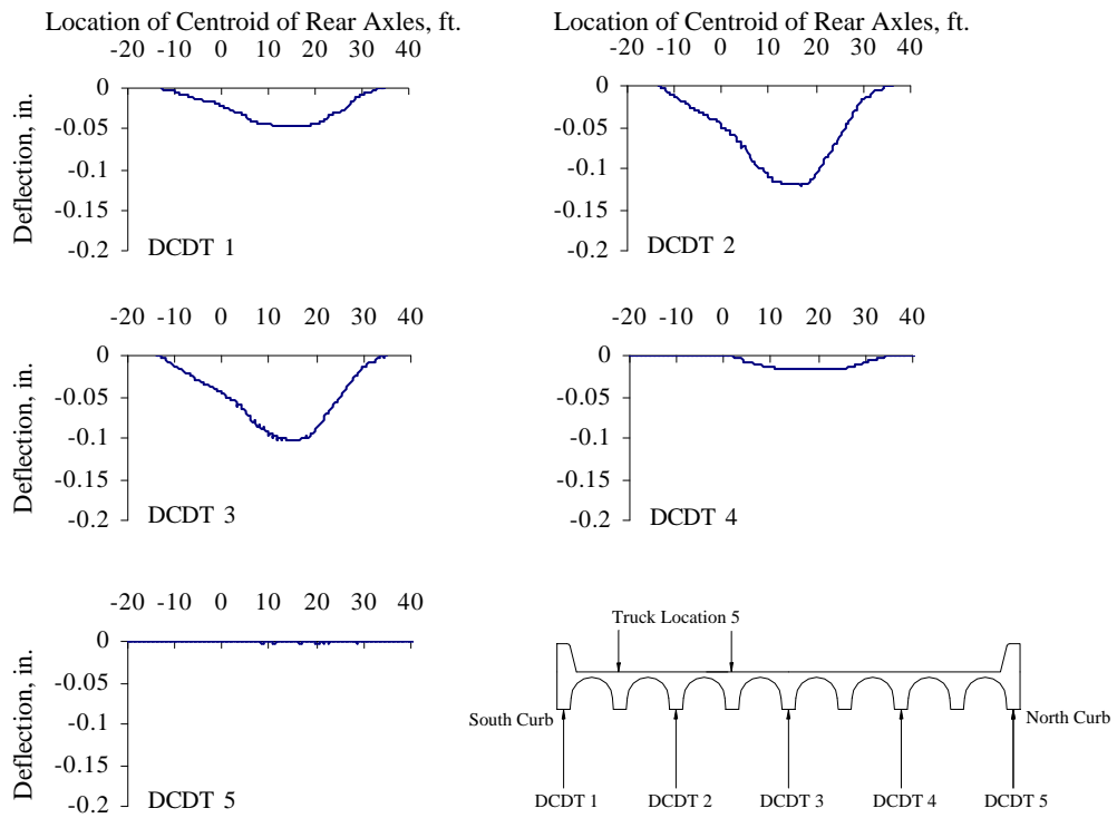
Figure G.12 Vertical Deflections Measured at Mid-span, Test Series 2, Truck Location 5, Pass 2
