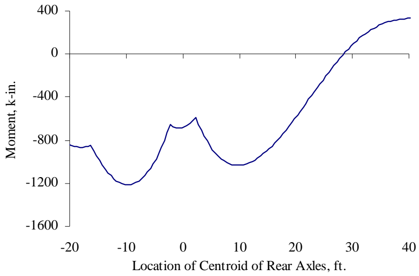
Figure 5.5 Moment Line at East Support for a Continuous Beam
