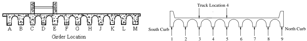
Figure 6.3 1968 Load Pattern Equivalent to Truck Location 4 [4]
