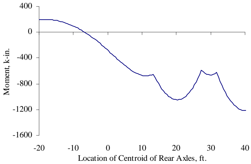
Figure 5.6 Moment Line at West Support for a Continuous Beam
