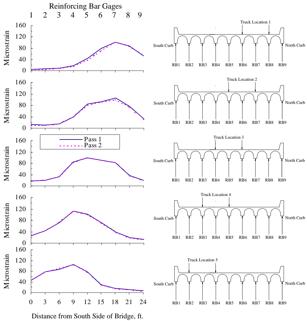
Figure 4.13 Profiles of Maximum Reinforcing Bar Strains at Mid-span for Test Series 2
