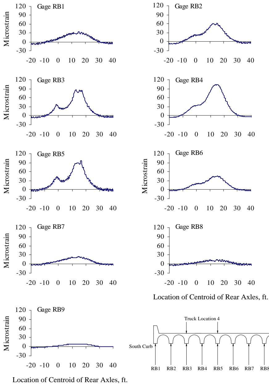
Figure A.19 Reinforcing Bar Strains at Mid-span, Test Series 3, Truck Location 4, Pass 1
