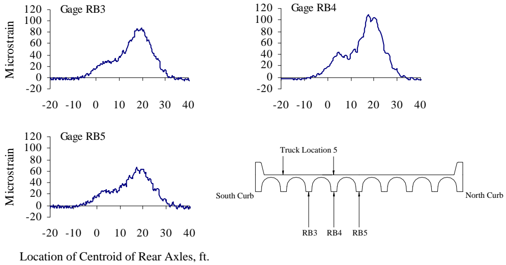
Figure A.33 Reinforcing Bar Strains at Mid-span, Test Series 5, Truck Location 5, Pass 1
