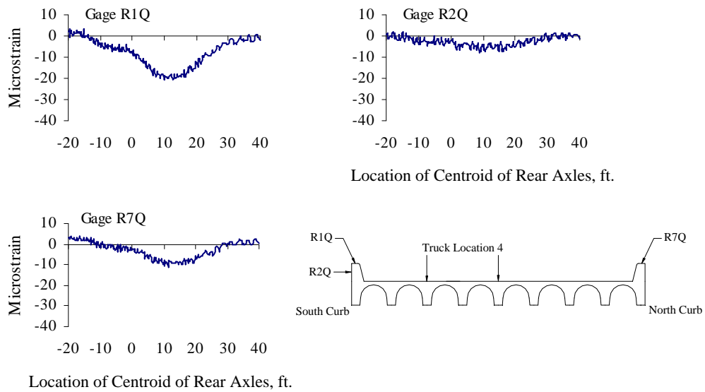
Figure D.10 Curb Strains at Quarter-span, Test Series 2, Truck Location 4, Pass 2
