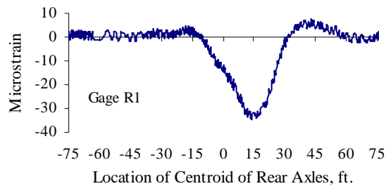
Figure 4.8 Response History for Gage R1 during Test Series 2, Truck Location 5, Pass 1
