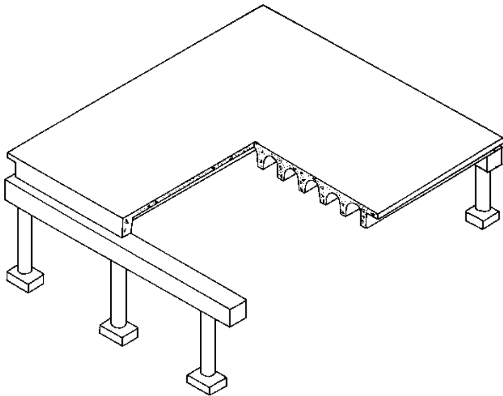
Figure 1.1 Typical Pan-Girder Span [3]
