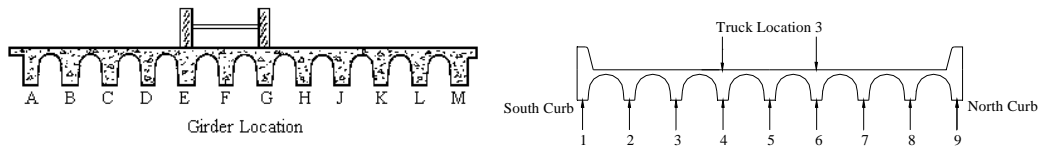
Figure 6.2 1968 Load Pattern Equivalent to Truck Location 3 [4]
