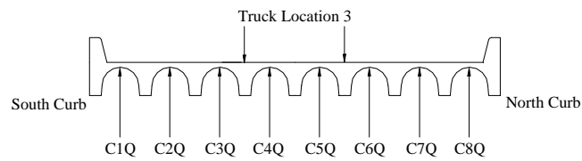
Figure F.7 Crown Strains at Quarter-span, Test Series 2, Truck Location 3, Pass 1
