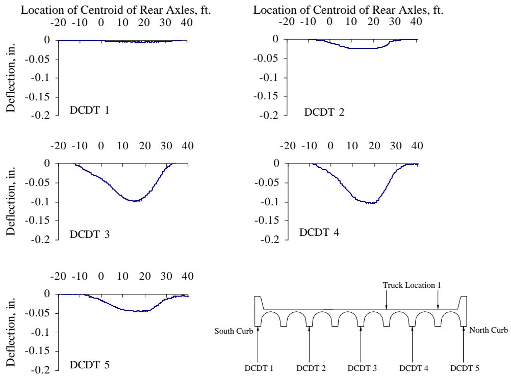
Figure G.14 Vertical Deflections Measured at Mid-span, Test Series 3, Truck Location 1, Pass 2
