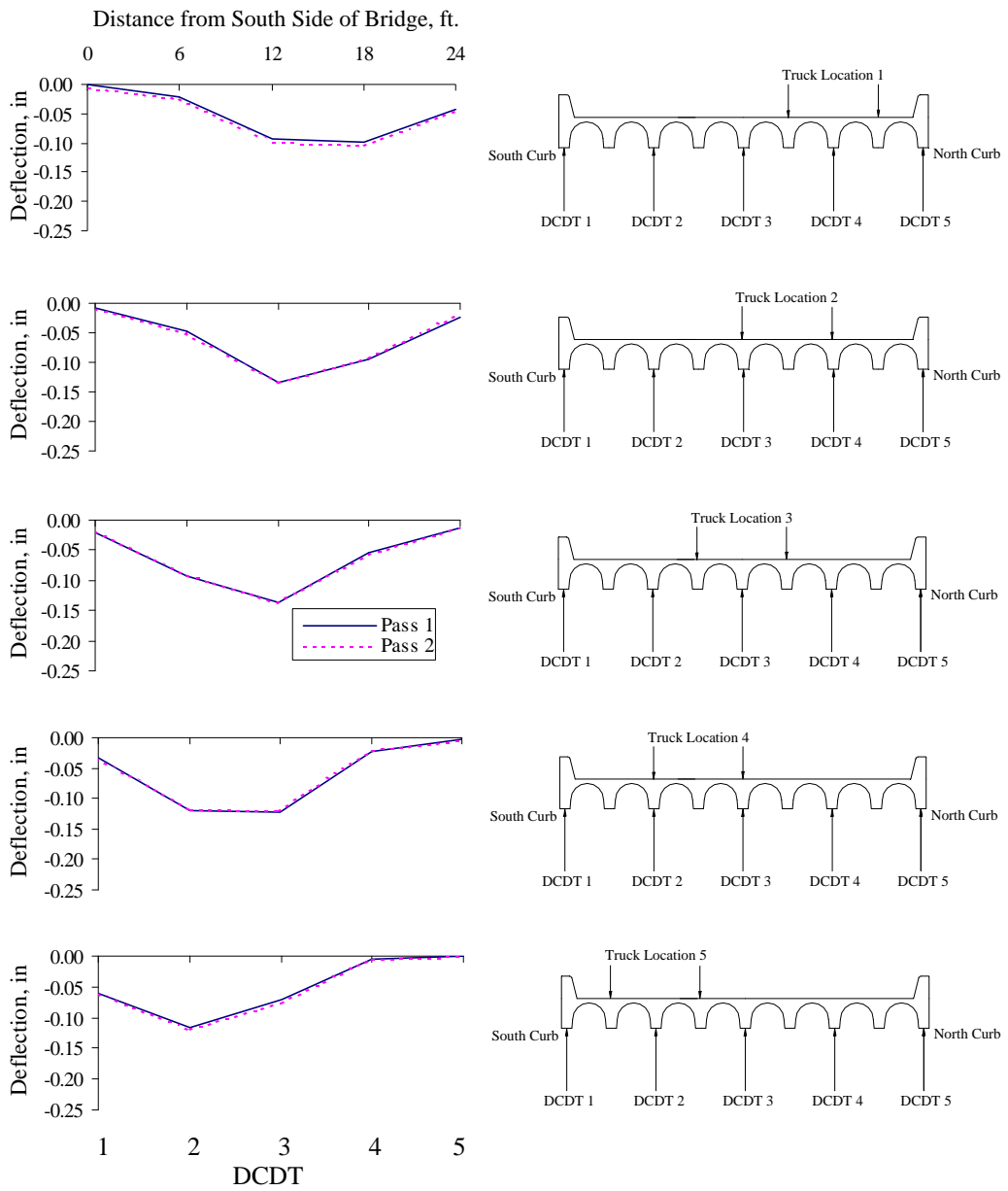
Figure 4.35 Profiles of Maximum Vertical Deflections at Mid-span for Test Series 3
