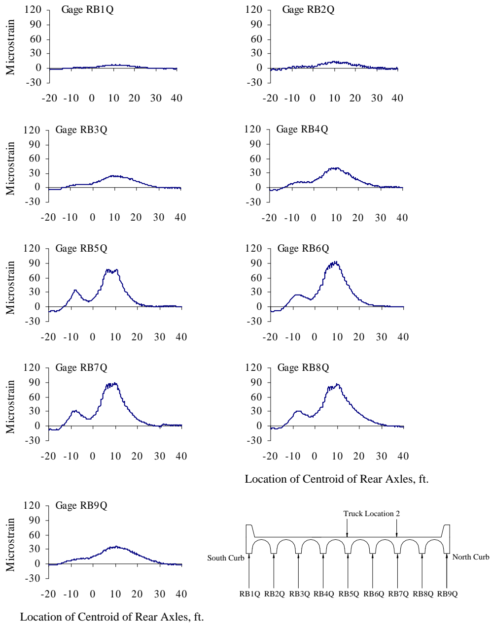
Figure B.5 Reinforcing Bar Strains at Quarter-span, Test Series 2, Truck Location 2, Pass 1
