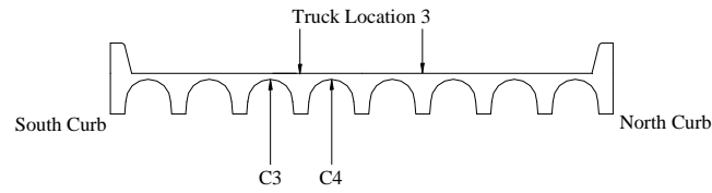
Figure E.28 Crown Strains at Mid-span, Test Series 5, Truck Location 3, Pass 2
