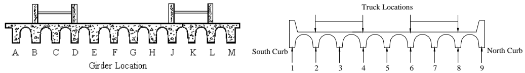
Figure 6.1 1968 Load Pattern Equivalent to Test Series 1 [4]
