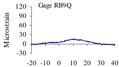
Figure B.9 Reinforcing Bar Strains at Quarter-span, Test Series 2, Truck Location 4, Pass 1
