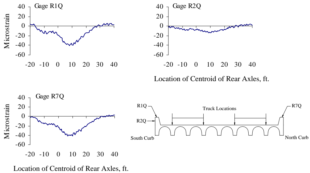
Figure D.2 Curb Strains at Quarter-span, Test Series 1, Pass 2
