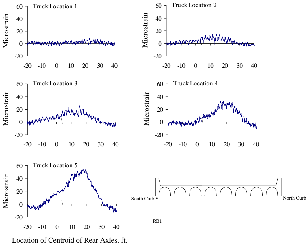
Figure A.23 Strains for Gage RB1 at Mid-span, Test Series 4, Pass 1
