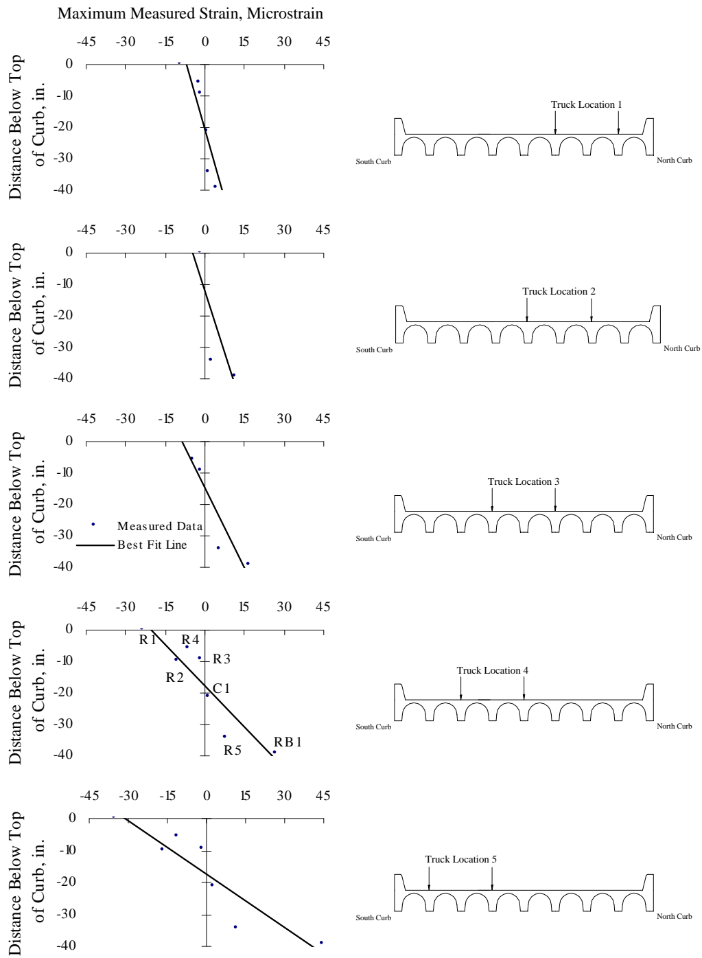
Figure 4.28 Measured Strain Gradients within South Curb at Mid-span
