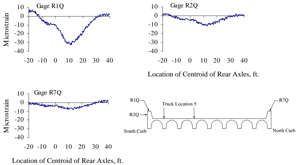
Figure D.12 Curb Strains at Quarter-span, Test Series 2, Truck Location 5, Pass 2
