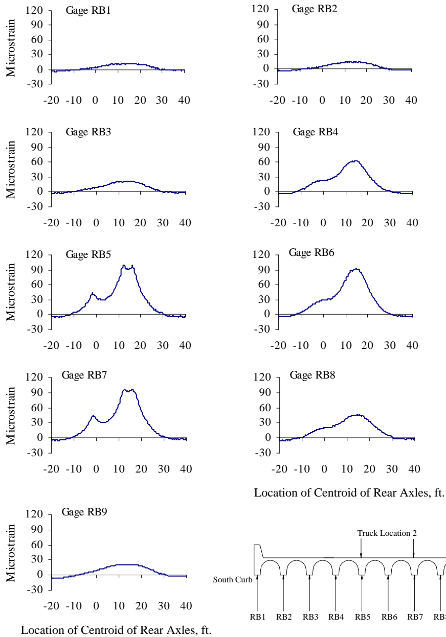
Figure A.15 Reinforcing Bar Strains at Mid-span, Test Series 3, Truck Location 2, Pass 1
