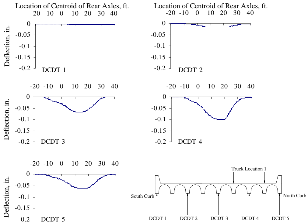
Figure G.4 Vertical Deflections Measured at Mid-span, Test Series 2, Truck Location 1, Pass 2
