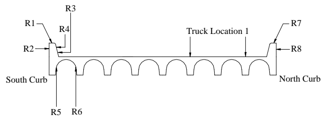
Figure C.3 Curb Strains at Mid-span, Test Series 2, Truck Location 1, Pass 1
