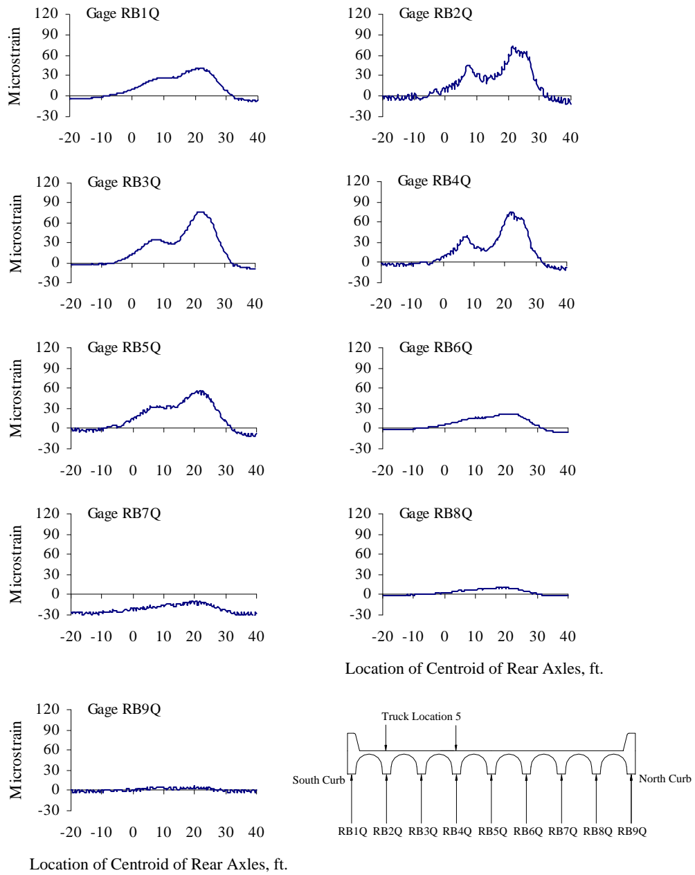
Figure B.21 Reinforcing Bar Strains at Quarter-span, Test Series 3, Truck Location 5, Pass 1
