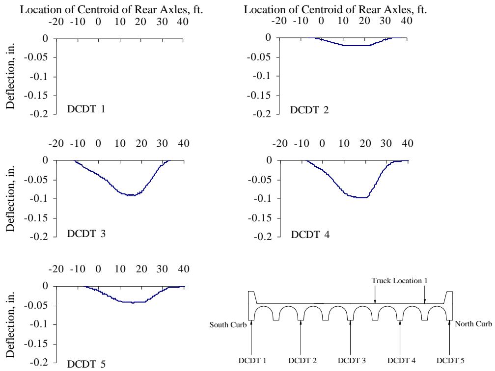
Figure G.13 Vertical Deflections Measured at Mid-span, Test Series 3, Truck Location 1, Pass 1
