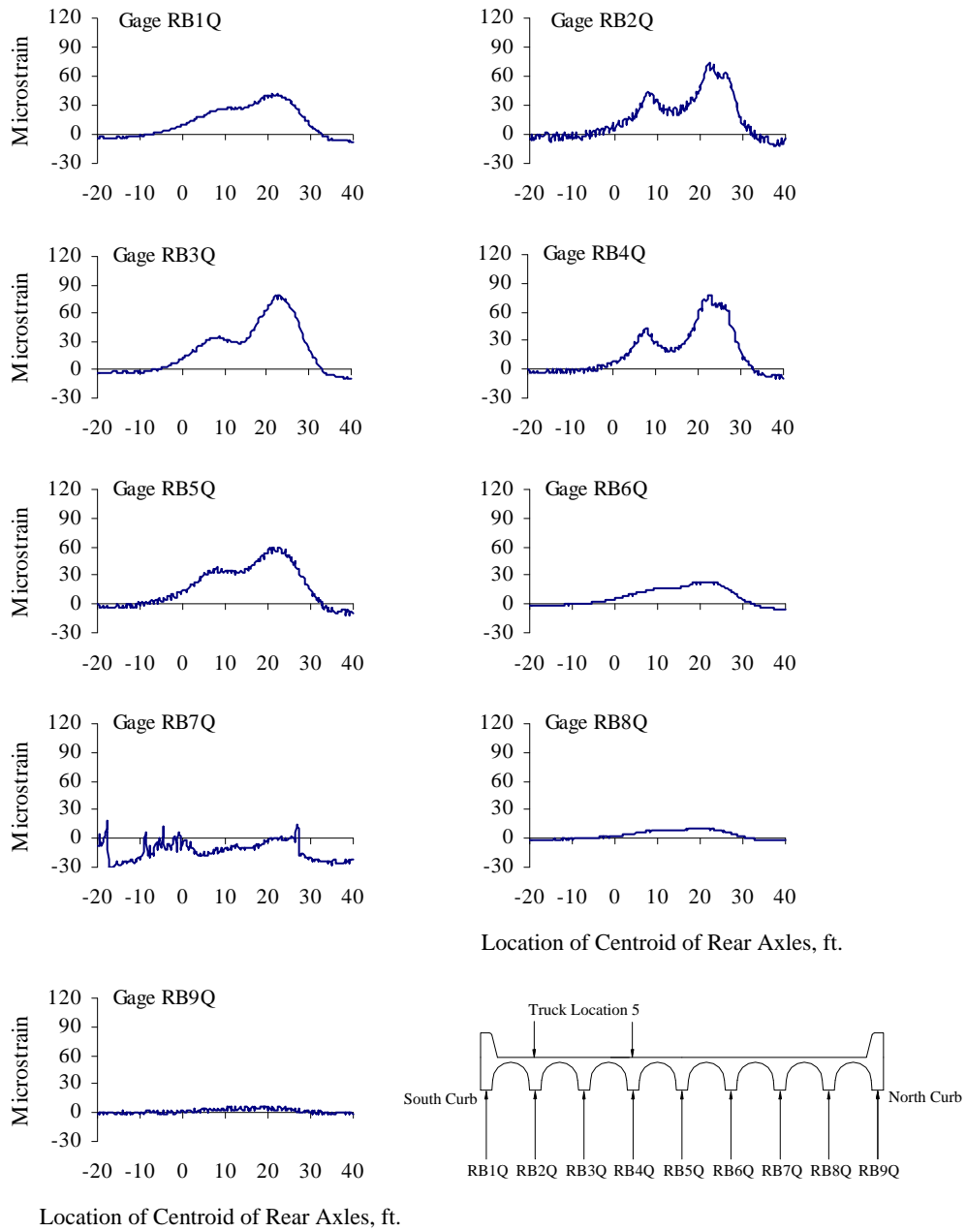
Figure B.22 Reinforcing Bar Strains at Quarter-span, Test Series 3, Truck Location 5, Pass 2
