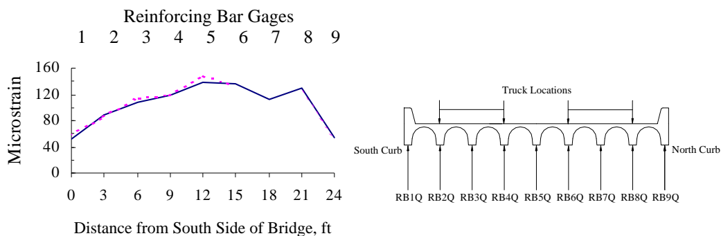
Figure 4.18 Profile of Maximum Reinforcing Bar Strains at Quarter-span for Test Series 1
