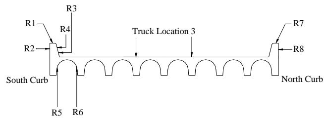
Figure C.8 Curb Strains at Mid-span, Test Series 2, Truck Location 3, Pass 2
