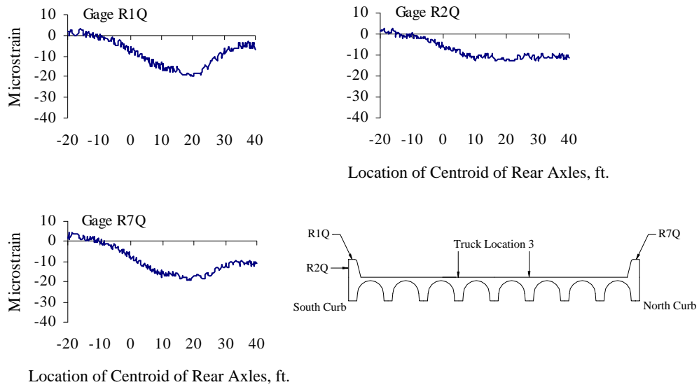
Figure D.17 Curb Strains at Quarter-span, Test Series 3, Truck Location 3, Pass 1
