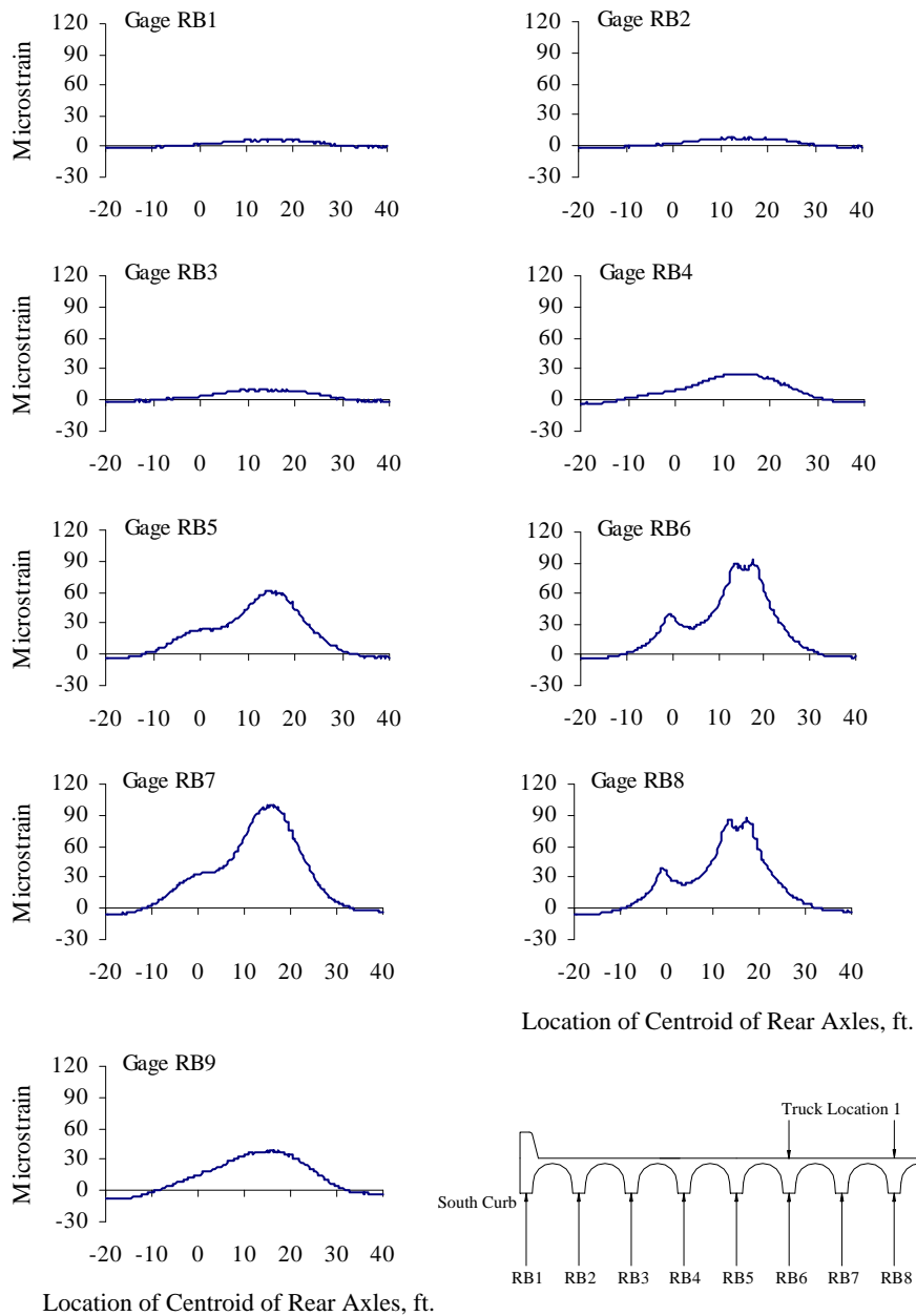
Figure A.14 Reinforcing Bar Strains at Mid-span, Test Series 3, Truck Location 1, Pass 2
