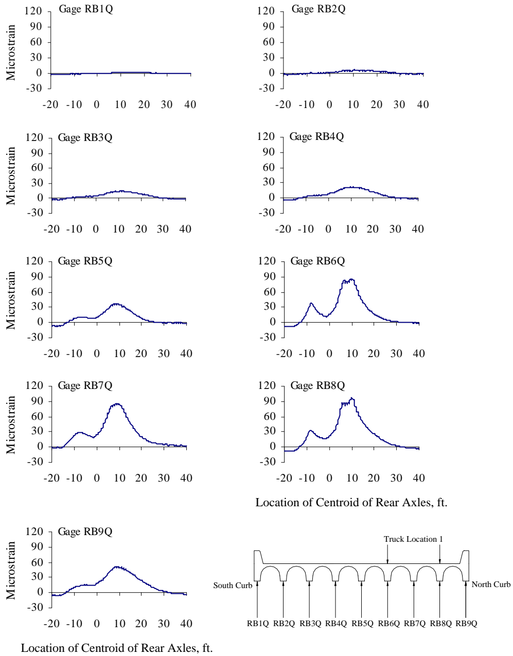
Figure B.3 Reinforcing Bar Strains at Quarter-span, Test Series 2, Truck Location 1, Pass 1
