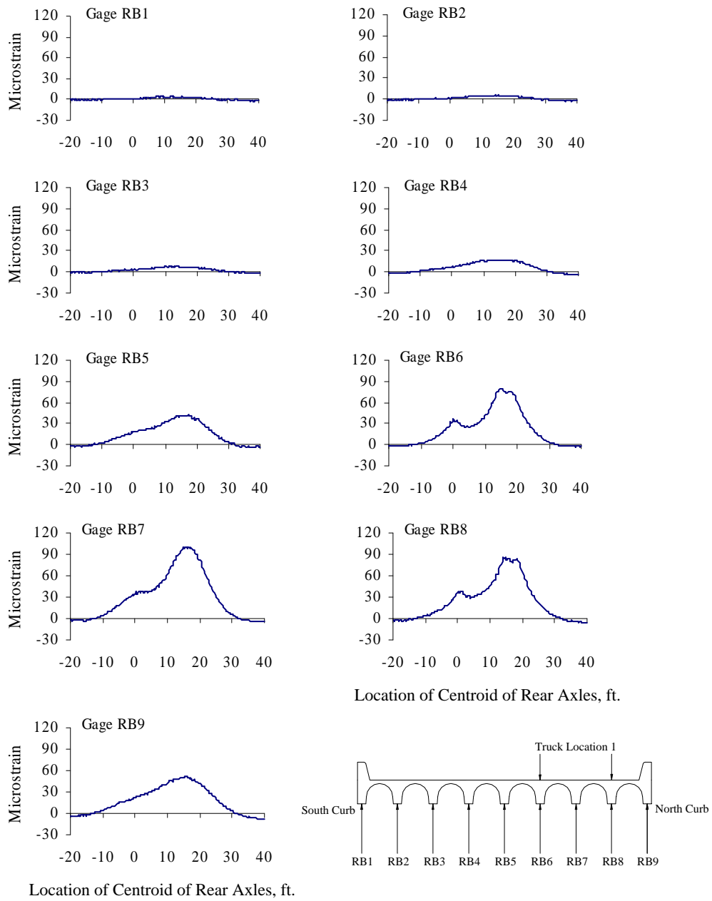
Figure A.3 Reinforcing Bar Strains at Mid-span, Test Series 2, Truck Location 1, Pass 1
