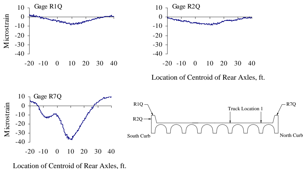
Figure 4.23 Curb Strains at Quarter-span, Test Series 2, Truck Location 1, Pass 1
