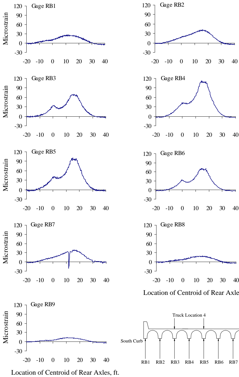
Figure A.9 Reinforcing Bar Strains at Mid-span, Test Series 2, Truck Location 4, Pass 1
