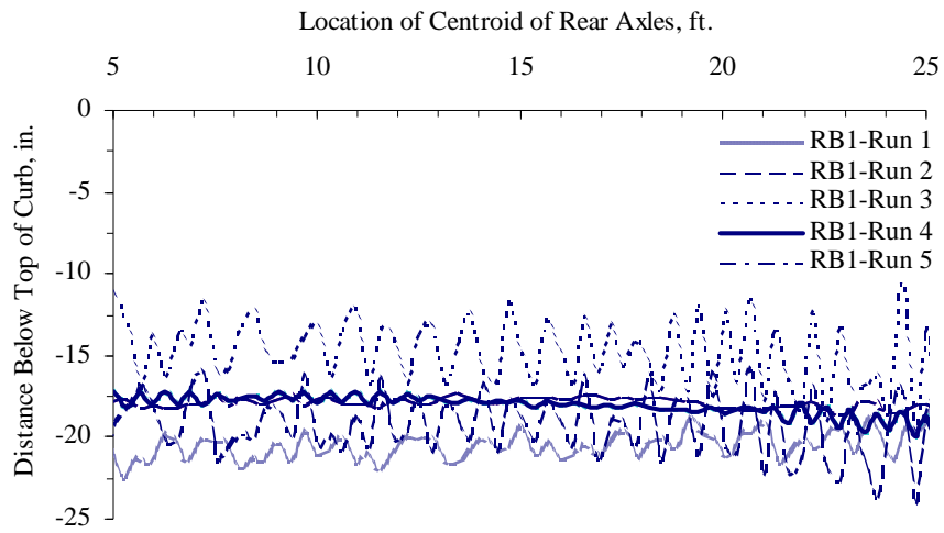
Figure 5.11 Variation in Neutral Axis Depth Calculated from Measured Strains for South Exterior Girder at Mid-span
