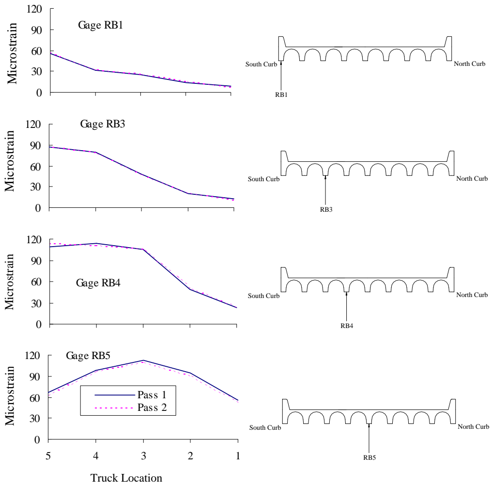
Figure 4.15 Profiles of Maximum Reinforcing Bar Strains at Mid-span for Test Series 4 and 5
