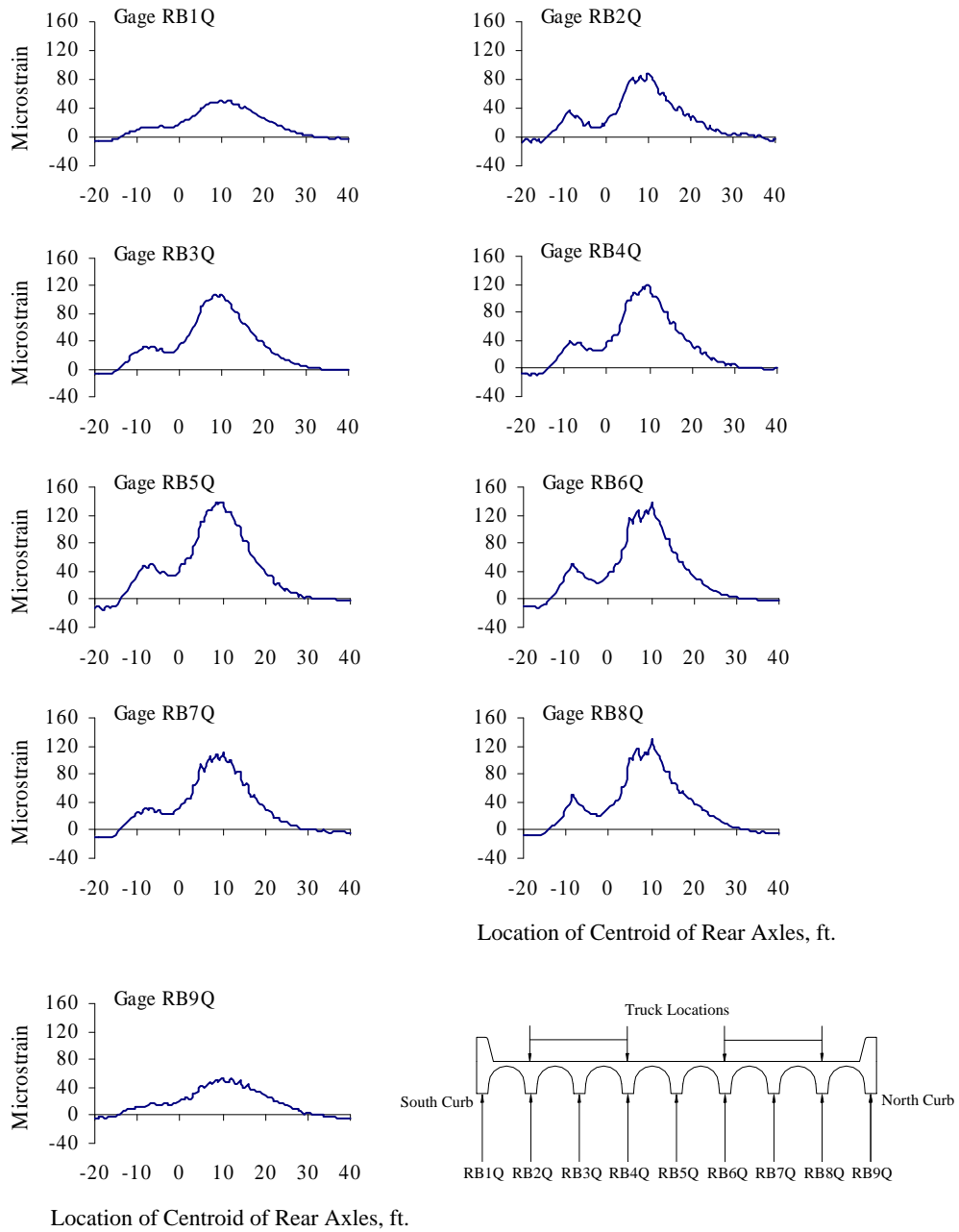
Figure B.1 Reinforcing Bar Strains at Quarter-span, Test Series 1, Pass 1
