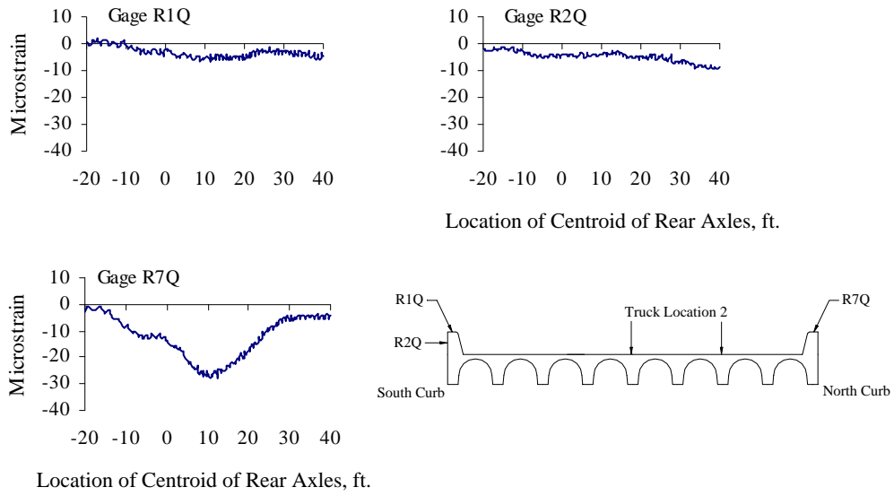
Figure D.5 Curb Strains at Quarter-span, Test Series 2, Truck Location 2, Pass 1
