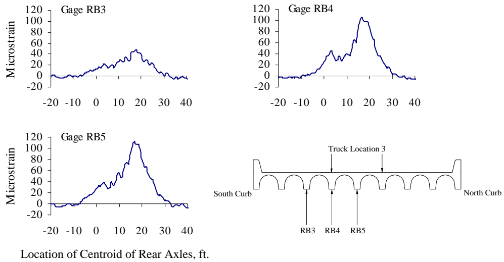
Figure A.29 Reinforcing Bar Strains at Mid-span, Test Series 5, Truck Location 3, Pass 1
