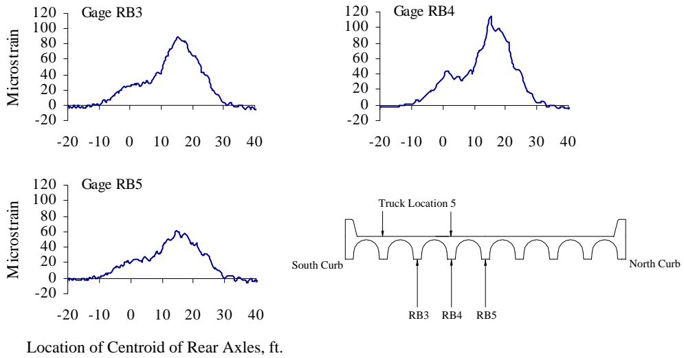
Figure A.34 Reinforcing Bar Strains at Mid-span, Test Series 5, Truck Location 5, Pass 2
