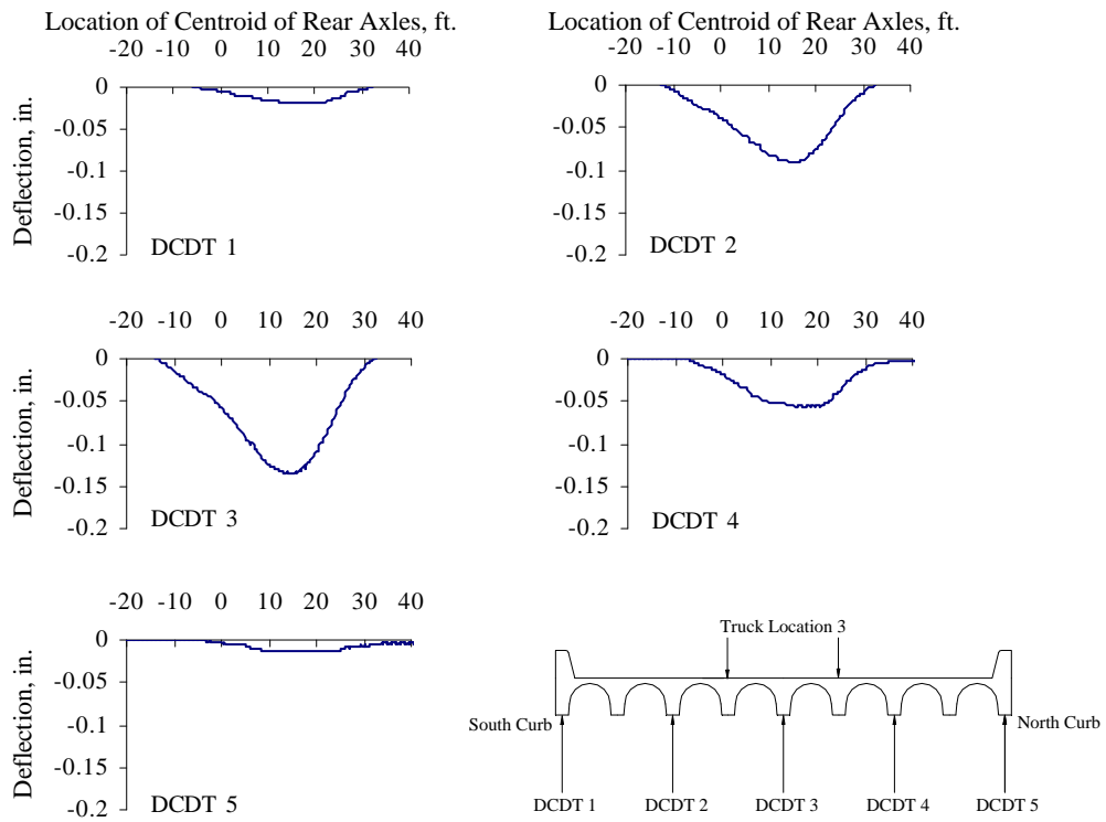
Figure G.18 Vertical Deflections Measured at Mid-span, Test Series 3, Truck Location 3, Pass 2
