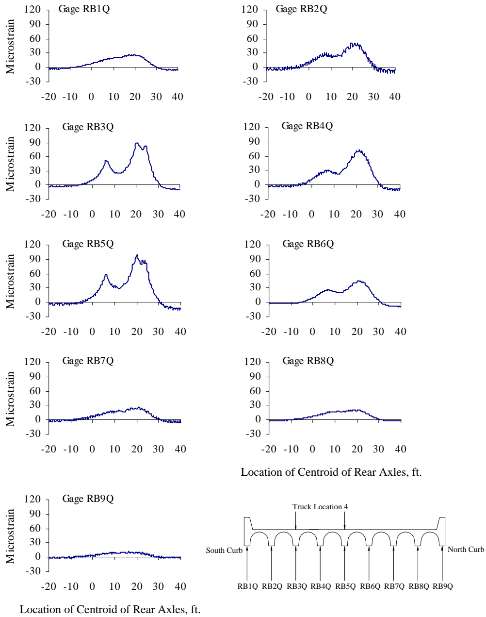
Figure B.19 Reinforcing Bar Strains at Quarter-span, Test Series 3, Truck Location 4, Pass 1
