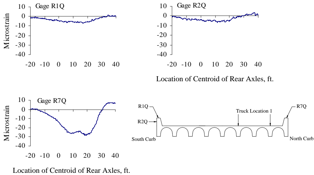
Figure D.14 Curb Strains at Quarter-span, Test Series 3, Truck Location 1, Pass 2
