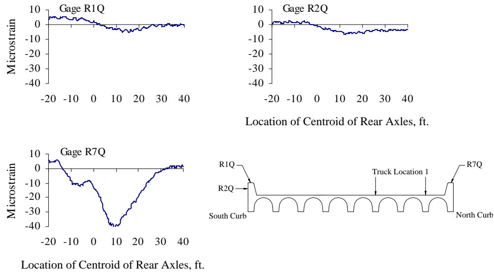
Figure D.4 Curb Strains at Quarter-span, Test Series 2, Truck Location 1, Pass 2
