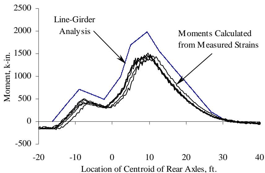
Figure 5.28 Comparison of Measured Moment Lines at Quarter-span with Line-Girder Analysis of a Simply-supported Beam, Test Series 2
