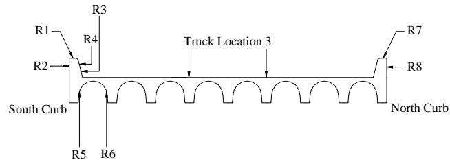
Figure C.17 Curb Strains at Mid-span, Test Series 3, Truck Location 3, Pass 1
