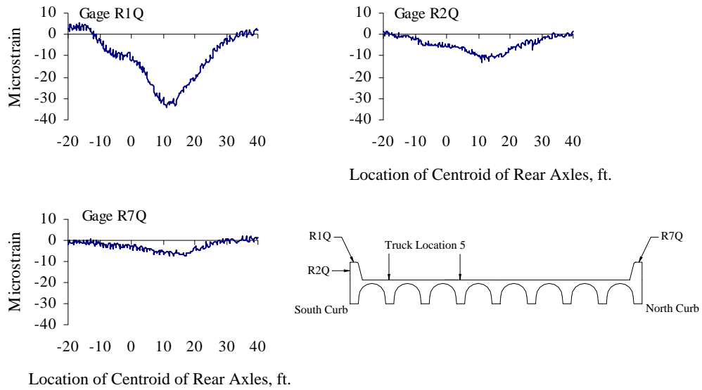
Figure D.11 Curb Strains at Quarter-span, Test Series 2, Truck Location 5, Pass 1
