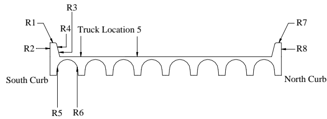
Figure C.11 Curb Strains at Mid-span, Test Series 2, Truck Location 5, Pass 1
