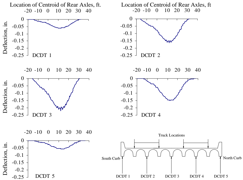
Figure G.2 Vertical Deflections Measured at Mid-span, Test Series 1, Pass 2
