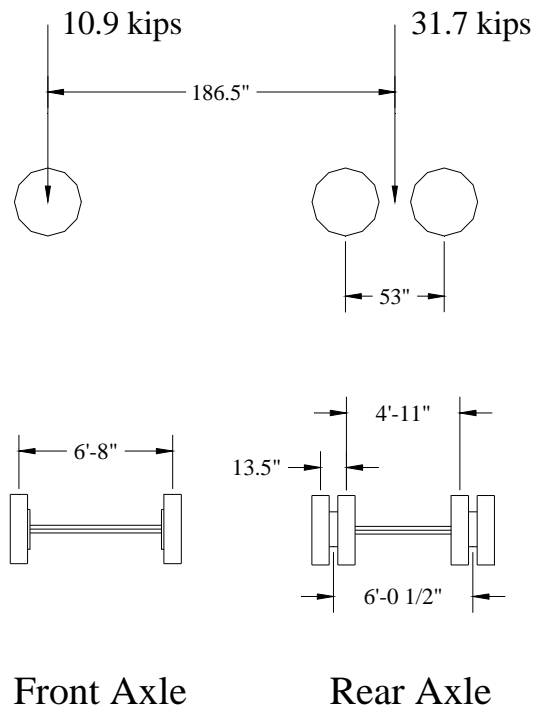
Figure 3.18 Sketch of Configuration of Truck 2
