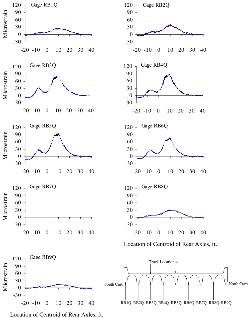
Figure B.10 Reinforcing Bar Strains at Quarter-span, Test Series 2, Truck Location 4, Pass 2
