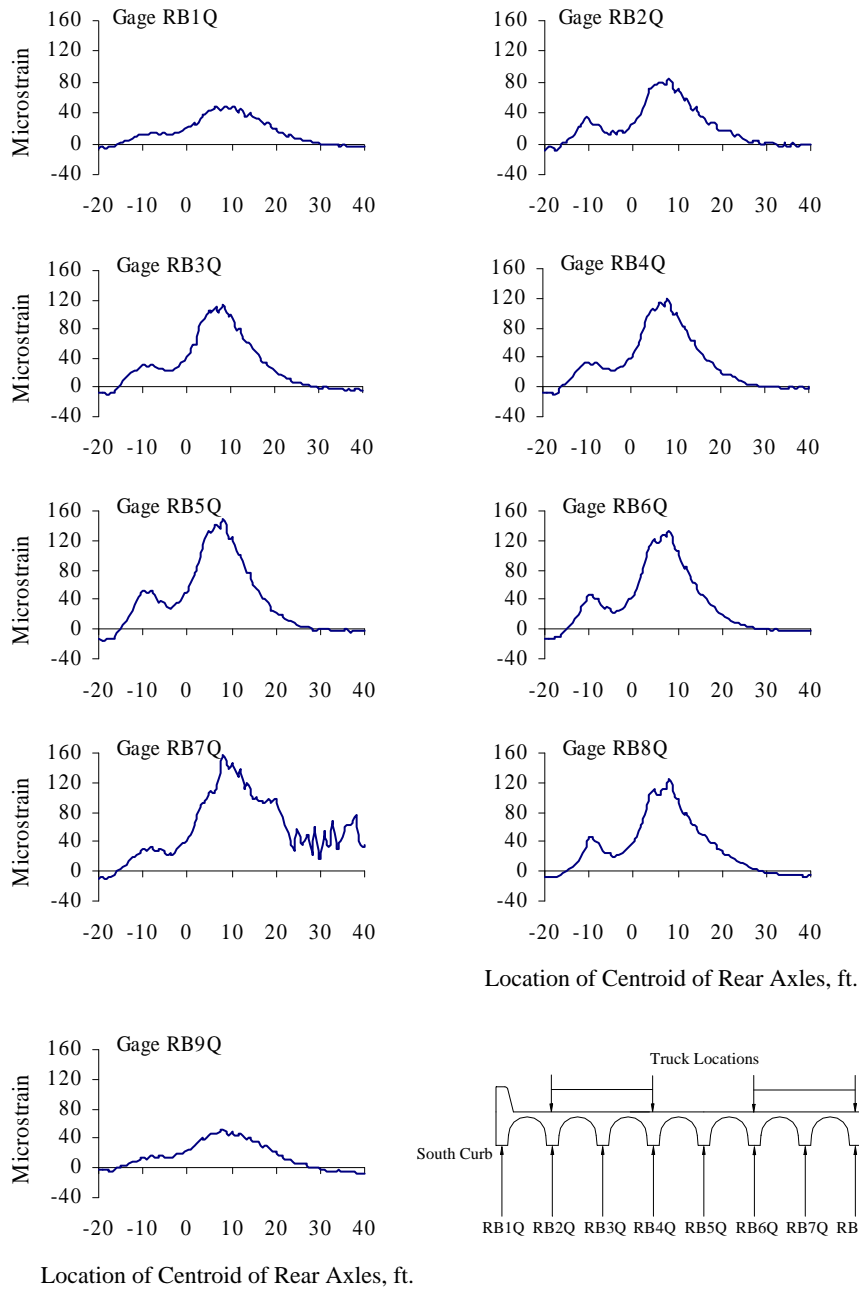
Figure B.2 Reinforcing Bar Strains at Quarter-span, Test Series 1, Pass 2
