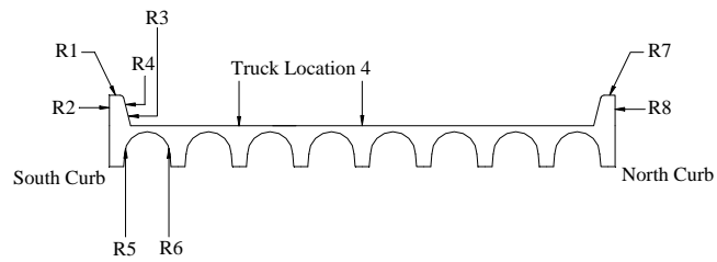
Figure C.9 Curb Strains at Mid-span, Test Series 2, Truck Location 4, Pass 1
