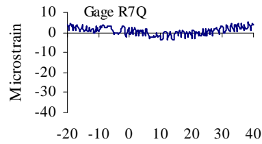
Figure D.21 Curb Strains at Quarter-span, Test Series 3, Truck Location 5, Pass 1
