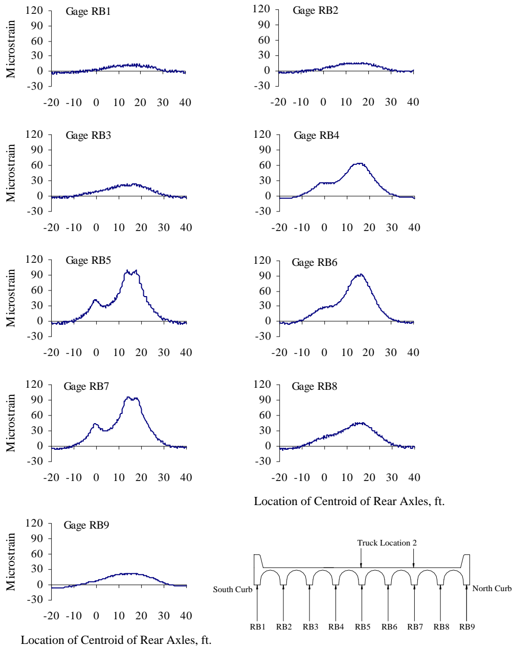
Figure A.16 Reinforcing Bar Strains at Mid-span, Test Series 3, Truck Location 2, Pass 2
