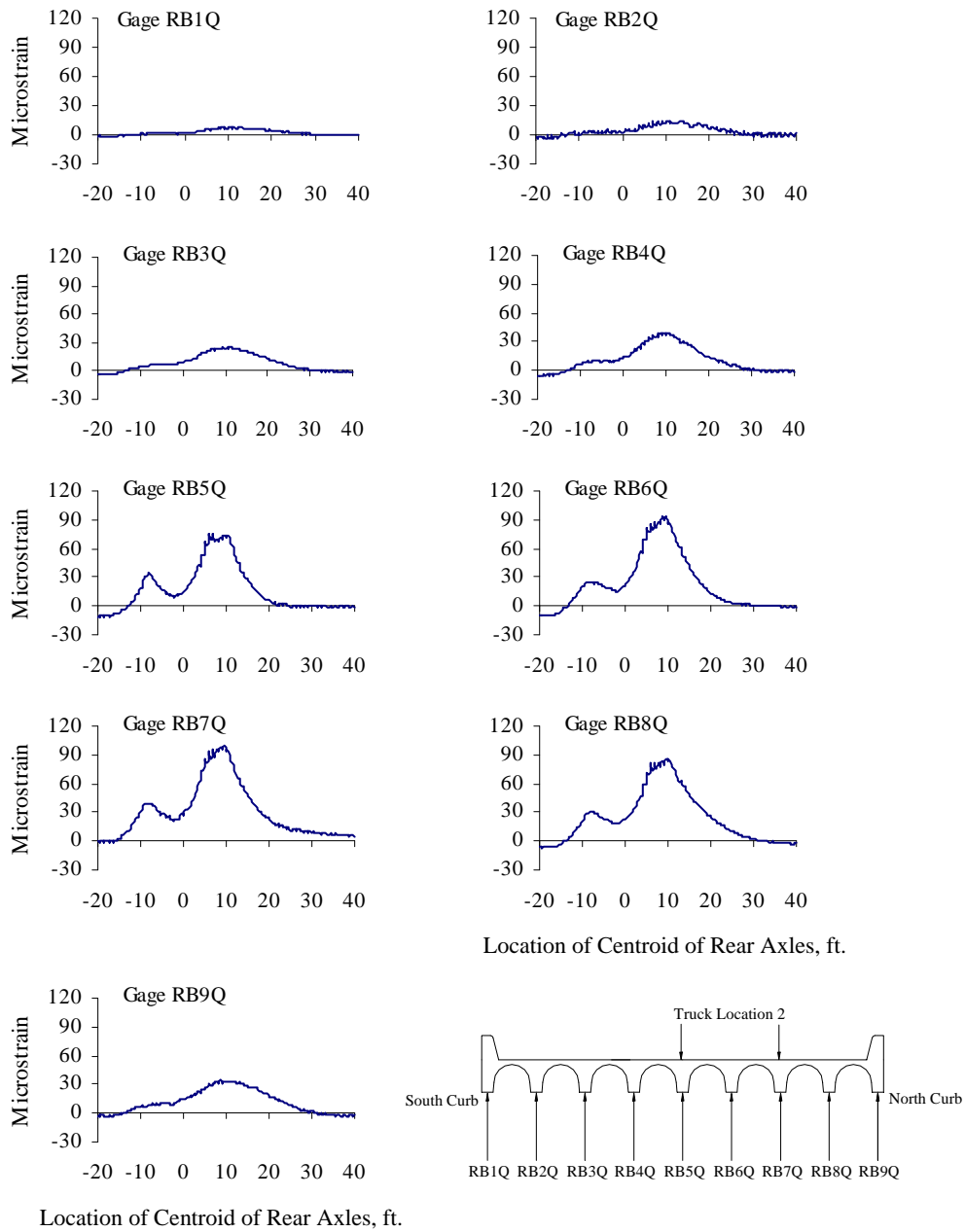
Figure B.6 Reinforcing Bar Strains at Quarter-span, Test Series 2, Truck Location 2, Pass 2
