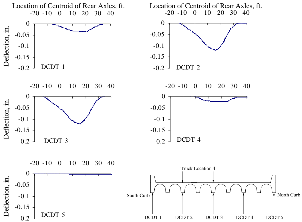
Figure G.19 Vertical Deflections Measured at Mid-span, Test Series 3, Truck Location 4, Pass 1
