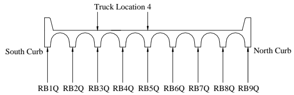
Figure B.9 Reinforcing Bar Strains at Quarter-span, Test Series 2, Truck Location 4, Pass 1
