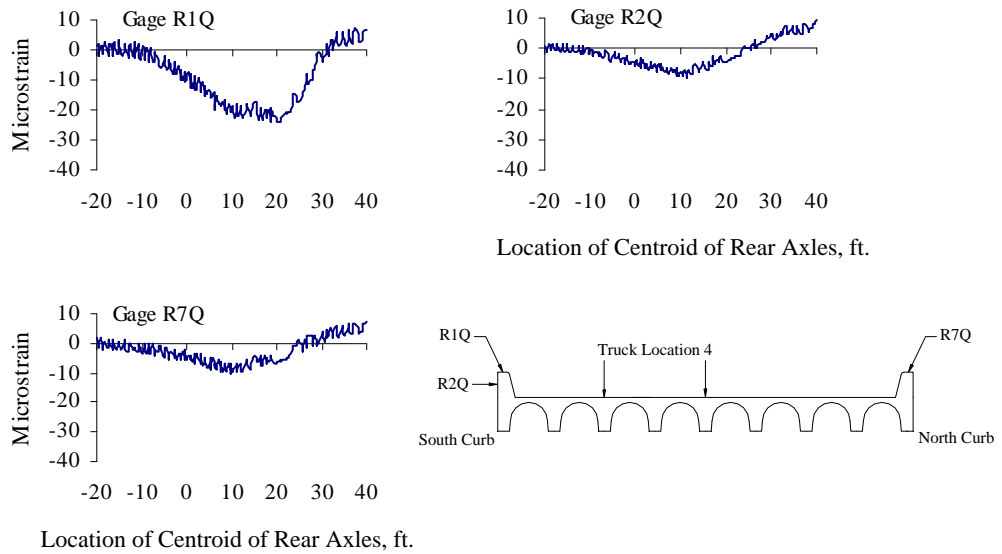
Figure D.20 Curb Strains at Quarter-span, Test Series 3, Truck Location 4, Pass 2
