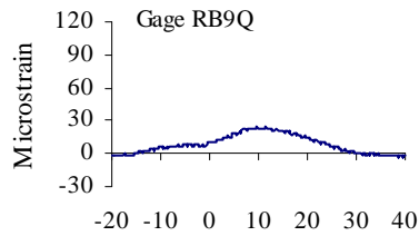
Figure B.7 Reinforcing Bar Strains at Quarter-span, Test Series 2, Truck Location 3, Pass 1
