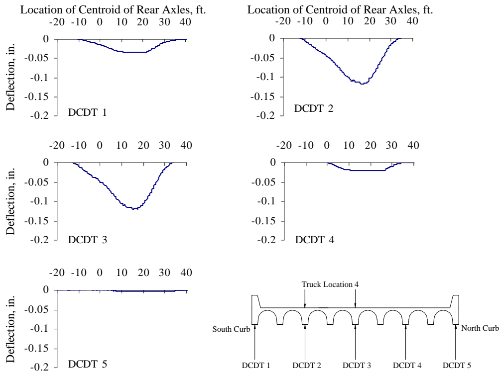
Figure G.20 Vertical Deflections Measured at Mid-span, Test Series 3, Truck Location 4, Pass 2
