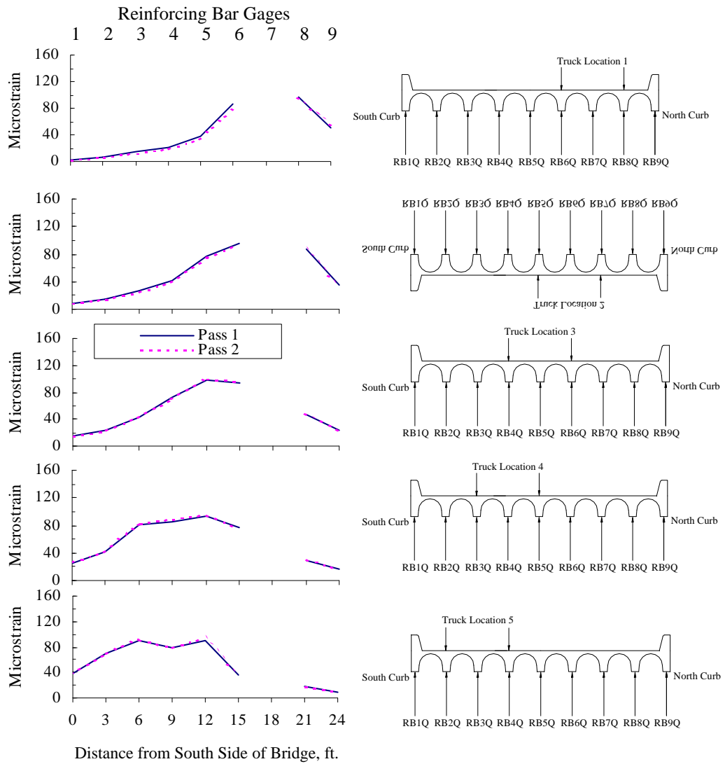
Figure 4.19 Profiles of Maximum Reinforcing Bar Strains at Quarter-span for Test Series 2
