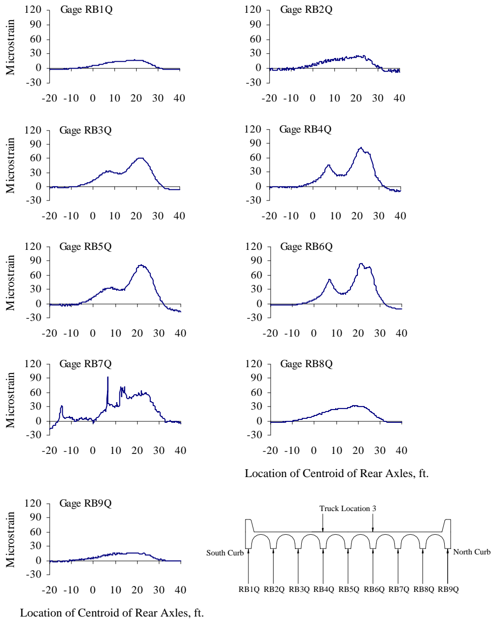
Figure B.17 Reinforcing Bar Strains at Quarter-span, Test Series 3, Truck Location 3, Pass 1
