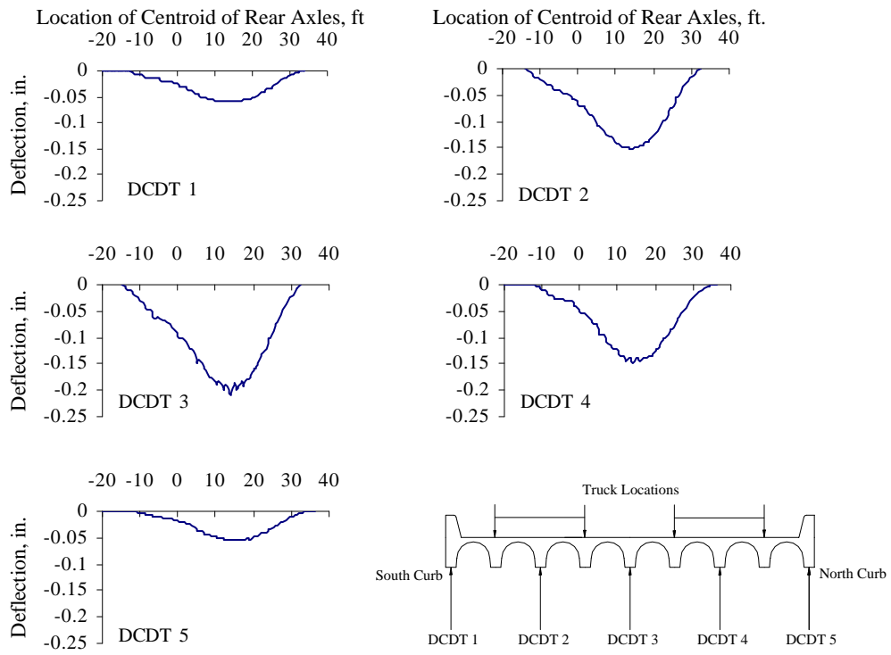
Figure G.1 Vertical Deflections Measured at Mid-span, Test Series 1, Pass 1
