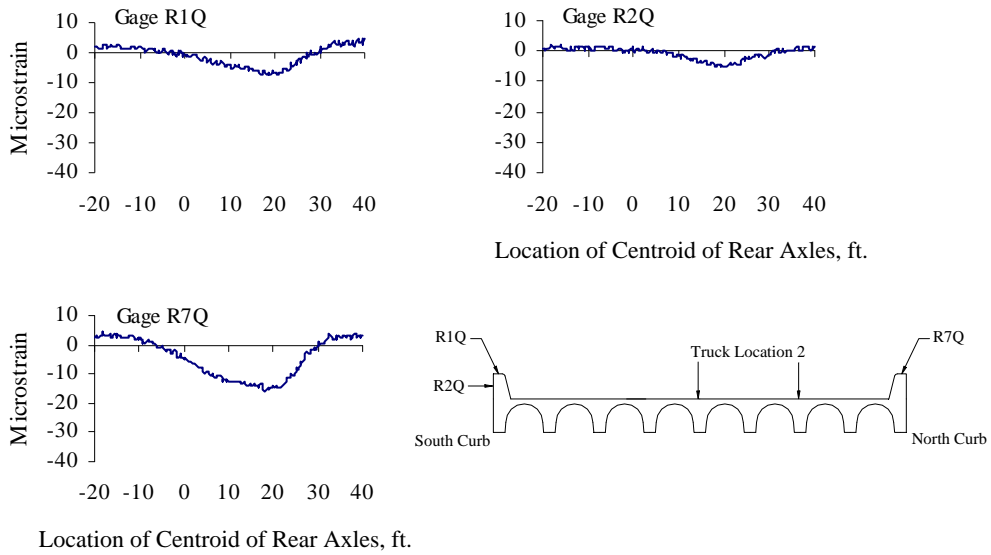
Figure D.15 Curb Strains at Quarter-span, Test Series 3, Truck Location 2, Pass 1
