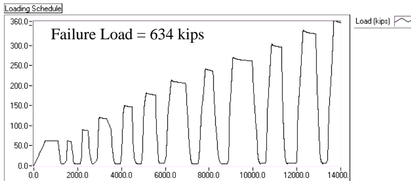
b) Amplitude vs. Time for G1WS
