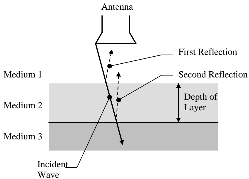
Figure 5.1 - Propagation of Electromagnetic Waves through Media of Different Dielectric Constants
