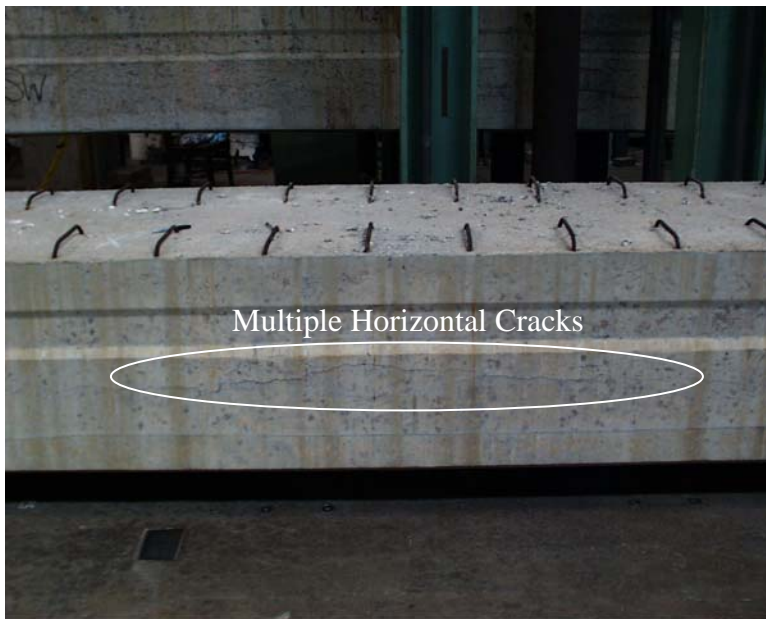
Figure 3.9 - Damage at Interior Blockout on BG3
