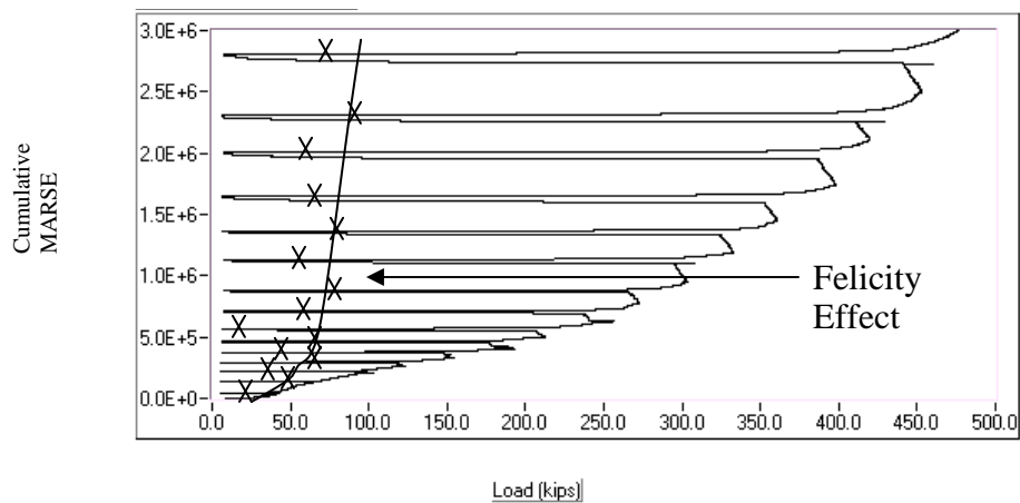
Figure 4.52 - Cumulative MARSE vs. Load for G1ES
