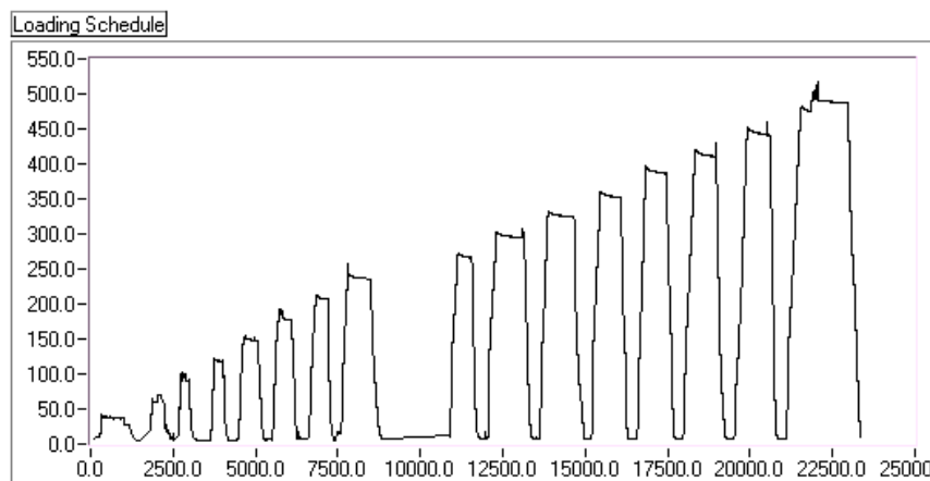
Figure 4.51 - Loading Schedule for G1ES
