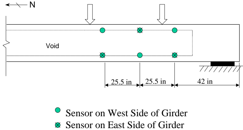
Figure 4.26 - Sensor Locations on all Shear Specimens
