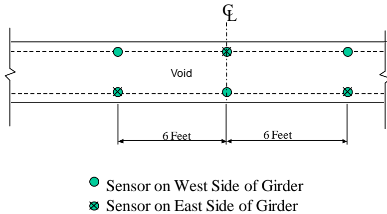
Figure 4.16 – Plan View of Sensor Locations on Box Girder Specimens
