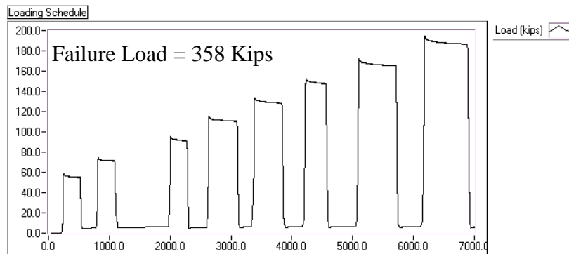
b) Amplitude vs Time for BG2S
