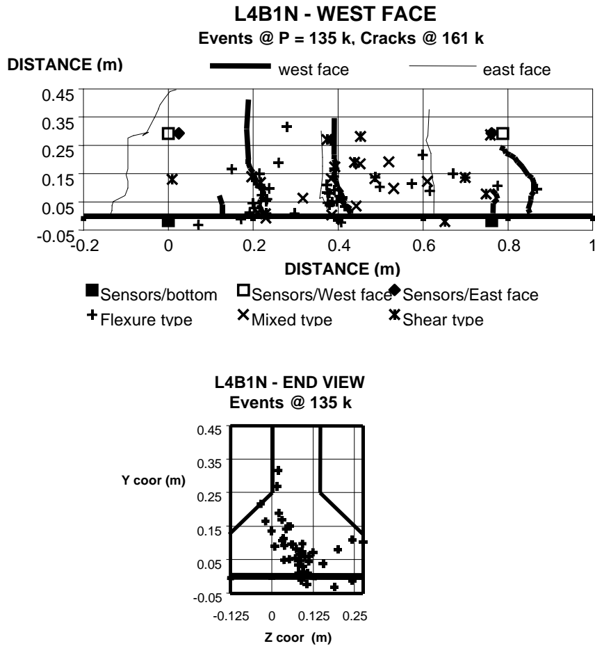
Figure 4.5 - Moment Tensor Results on Prestressed Girder (Yezpe 1997)
