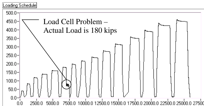
Figure 4.44 - Loading Schedule for G2ES
