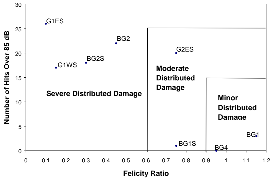
Figure 4.55 – Proposed Evaluation Criteria and Test Results
