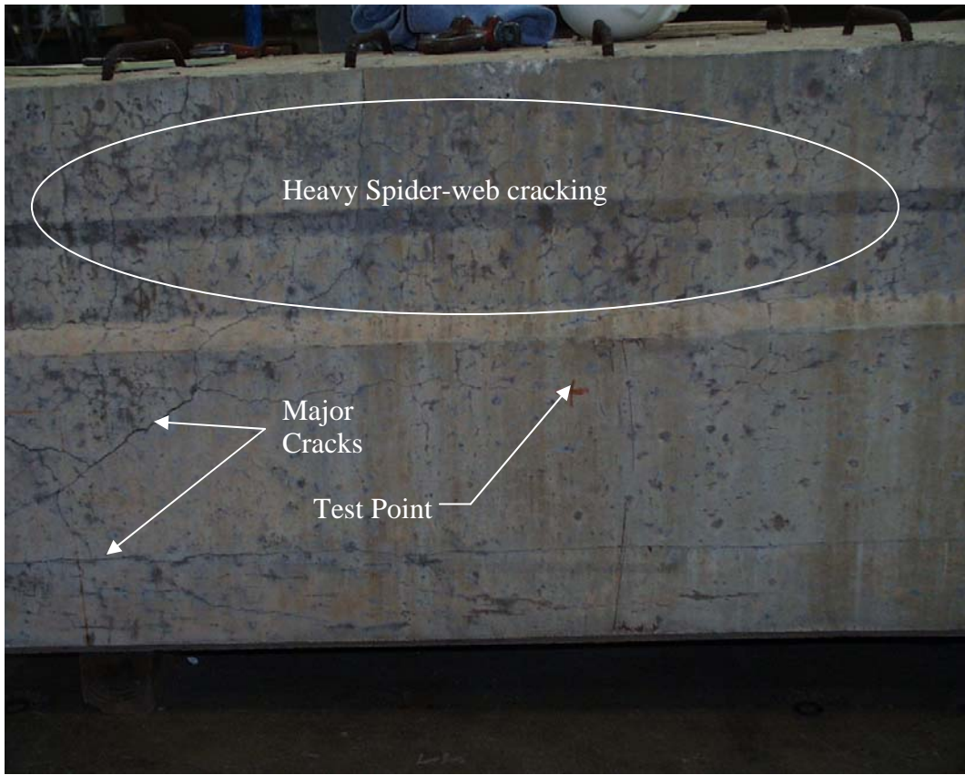
Figure 6.7 - Photo of the Test Point 3 feet from the North End of BG3
