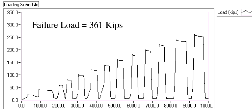
b) Amplitude vs Time for BG4S
