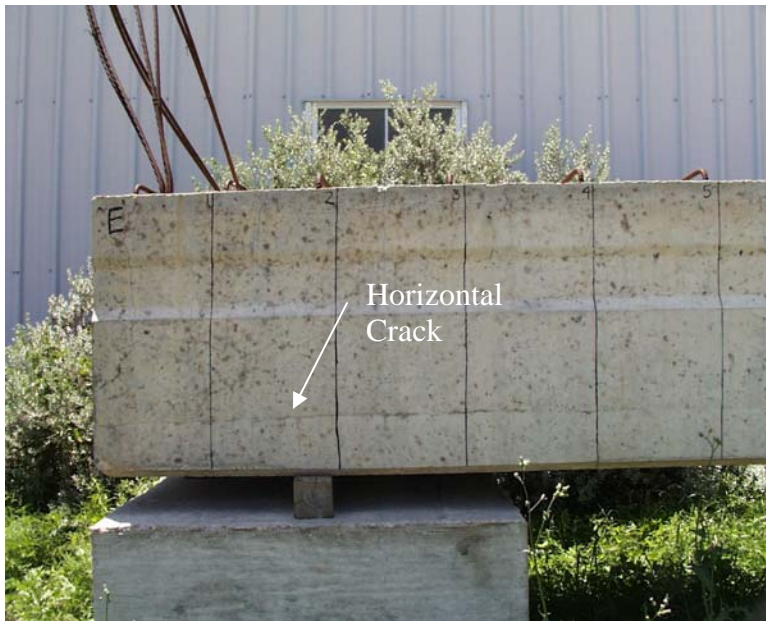
Figure 3.2 - Side of BG1 at A-End
