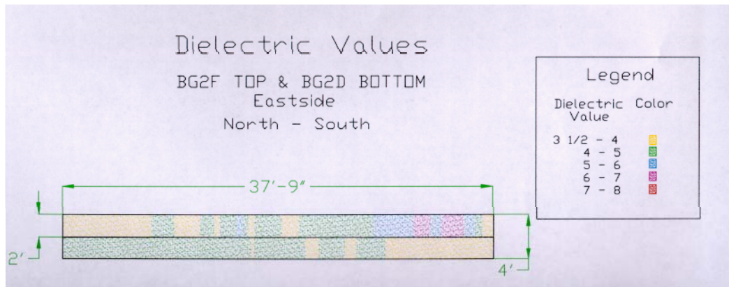
Figure 5.5 - Dielectric Values on East Side of BG2 at the A-End
