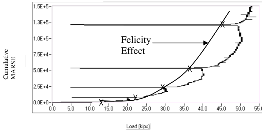
Figure 4.21 - Cumulative MARSE vs. Load for BG4
