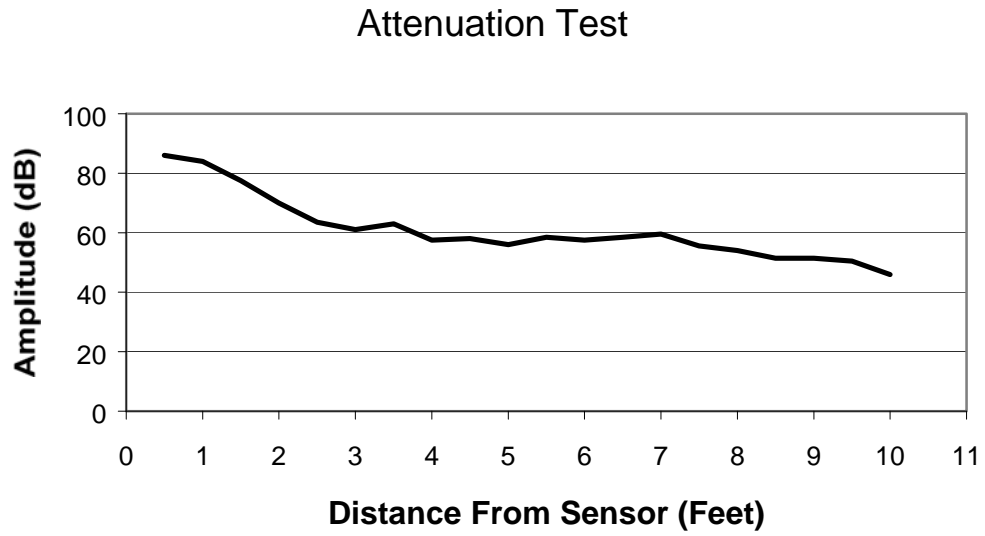
Figure 4.15 - Attenuation Curve for R6I Sensor
