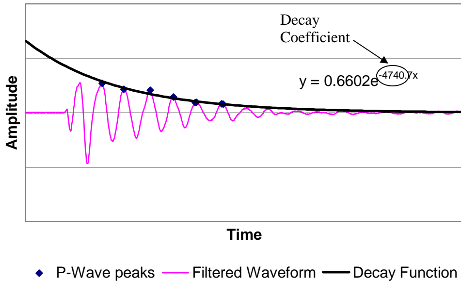
Figure 6.4 - Calculation of the Decay Coefficient
