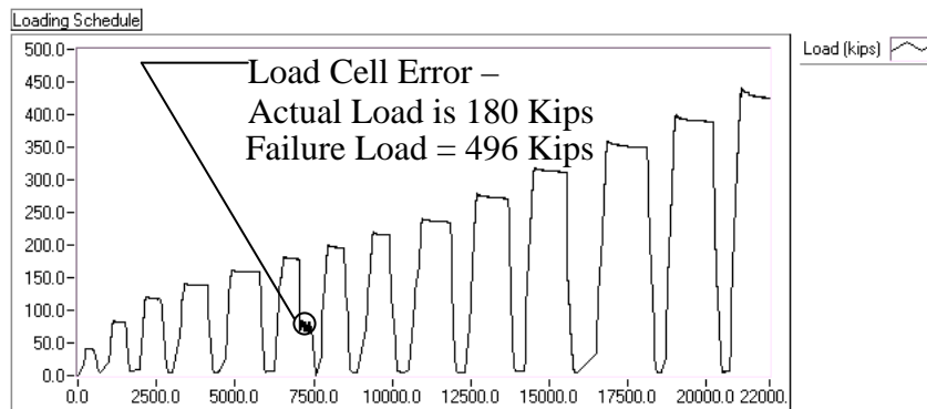
c) Load vs. Time for G2ES
