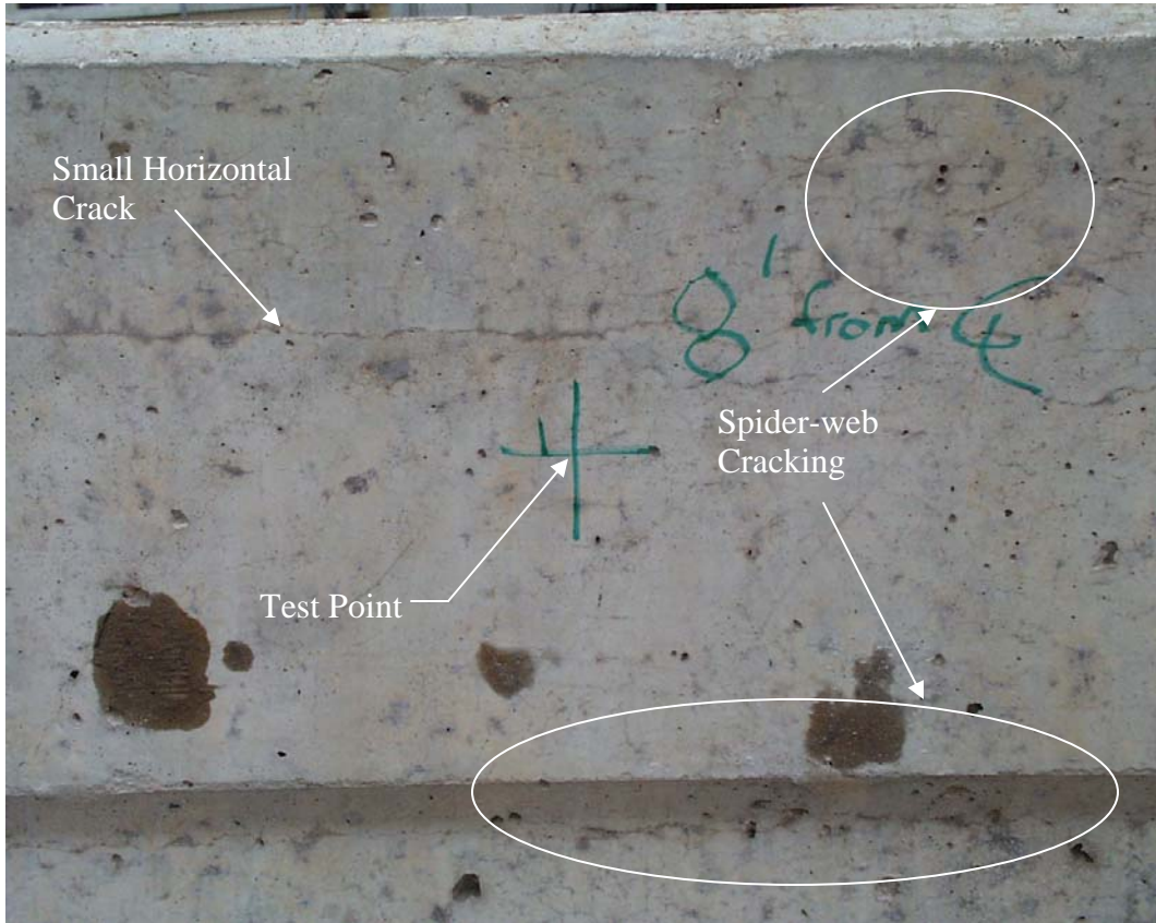
Figure 6.5 - Photo of the Test Point 8 feet from Centerline on BG1
