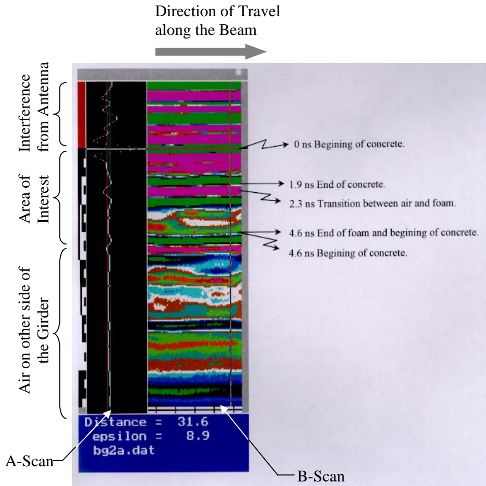
Figure 5.2 - Typical A-Scan and B-Scan From Sample BG2
