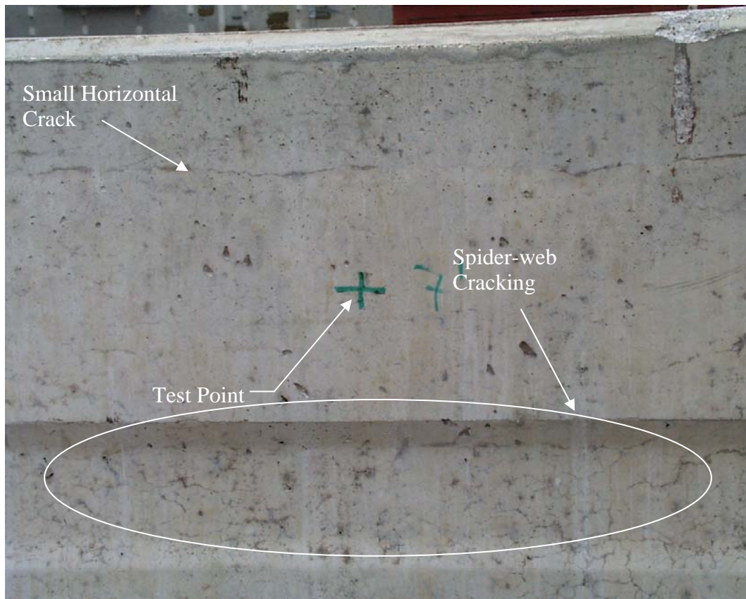
Figure 6.6 - Photo of the Test Point 7 feet from the South End of BG1
