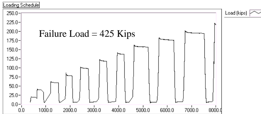
b) Amplitude vs Time for BG1S
