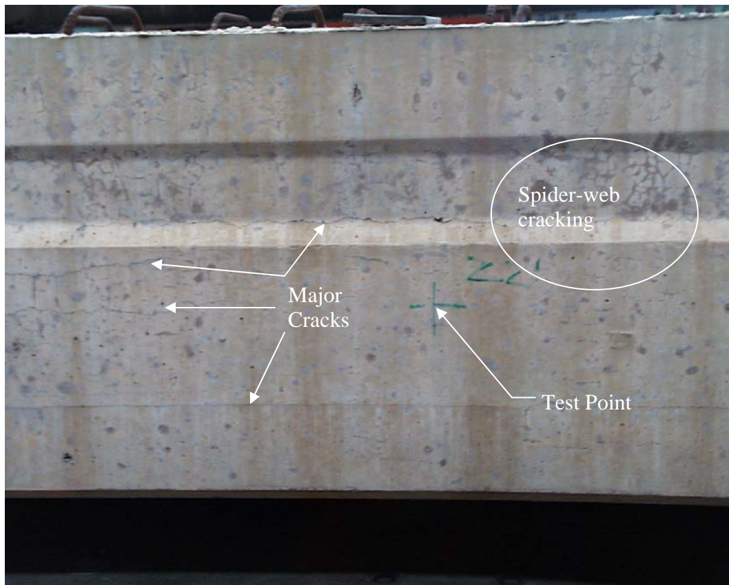
Figure 6.8 - Photo of the Test Point 22 feet from the South End of BG3
