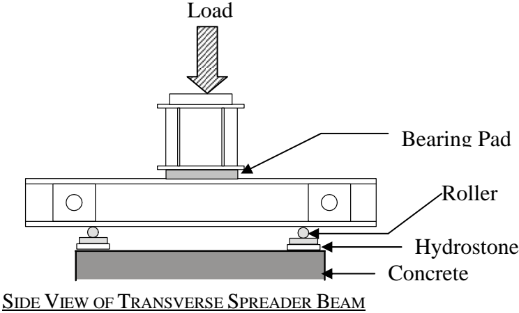
Figure 4.12 - Detail of Spreader Beams used in Flexure Tests
