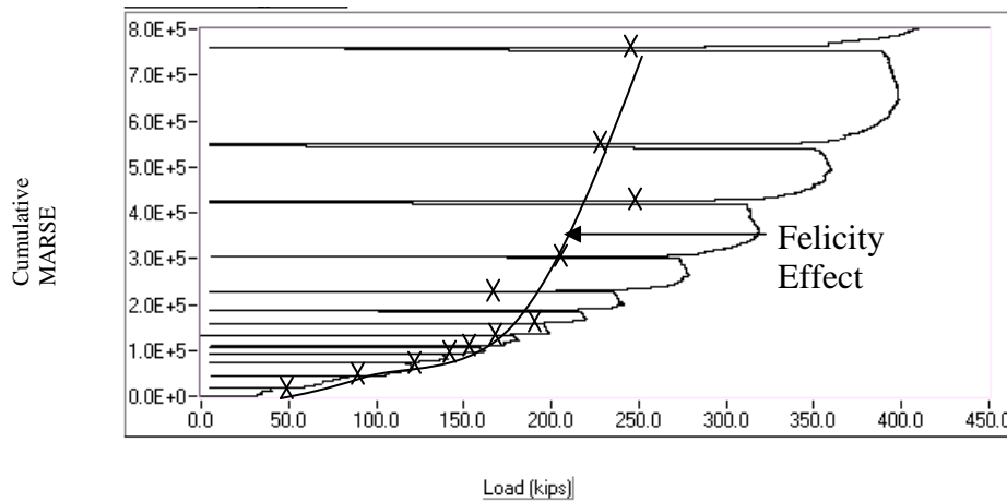
Figure 4.45 - Cumulative MARSE vs. Load for G2ES
