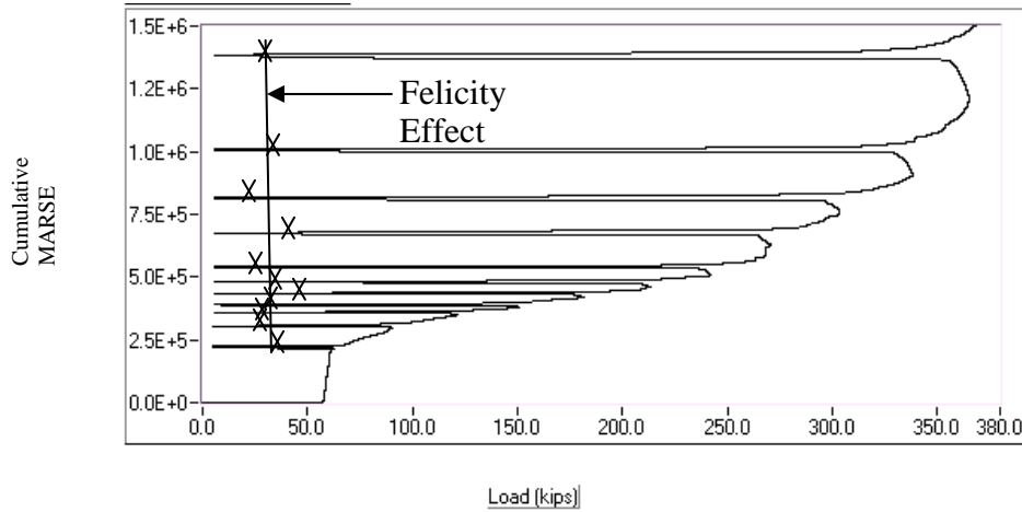
Figure 4.49 - Cumulative MARSE vs. Load for G1WS
