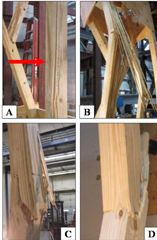
Figure 5.83 Post Failures A) Back Left B) Back Right C) Front Left D) Front Right
