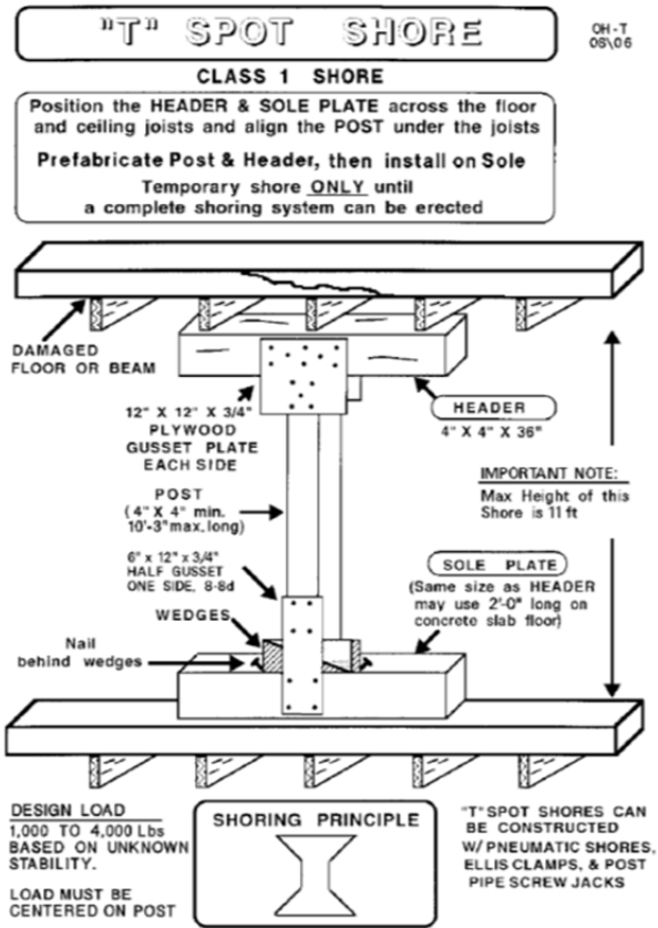
Figure 2.5 Standard Class 1 Shore ( USACE FOG 2009 )
