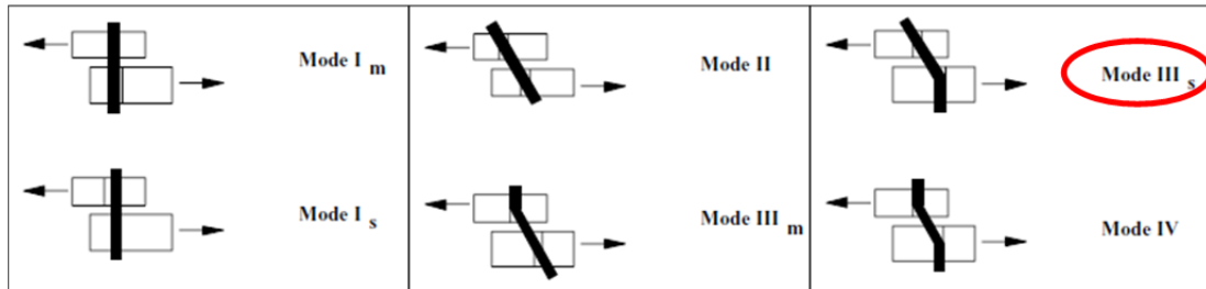
Figure 6.7 PLP Controlling Single Shear Yield Mode (NDS 2005)
