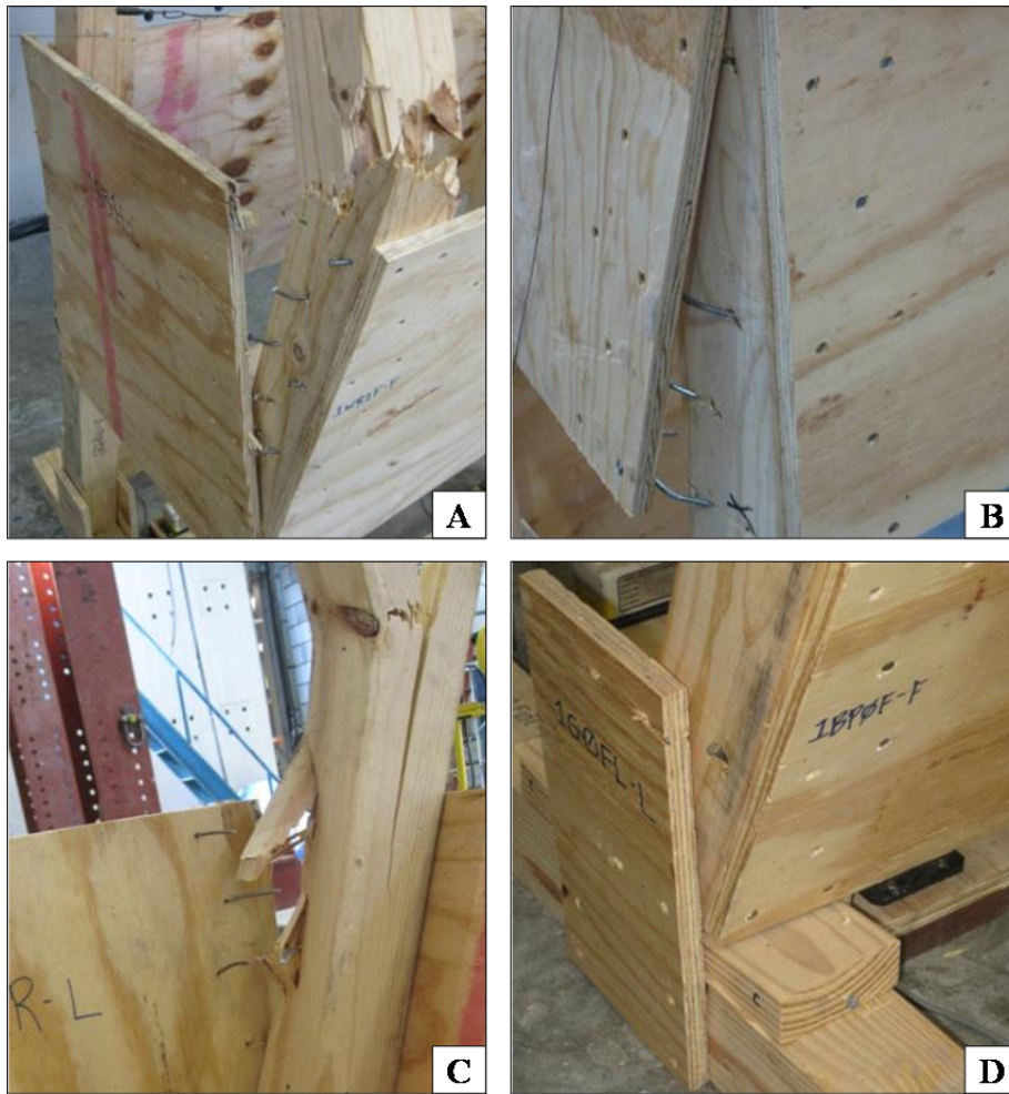
Figure 5.7 Connection Failures A) Pull Through B) Pullout C) Post Splintering D) Half-Gusset Rotation and Pull Through
