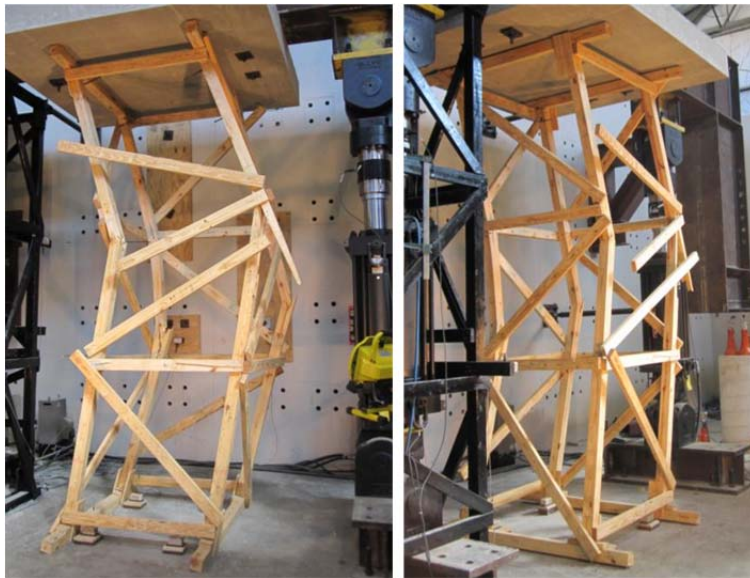
Figure 5.22 Specimen 4 Failure Photographs at Conclusion of Test
