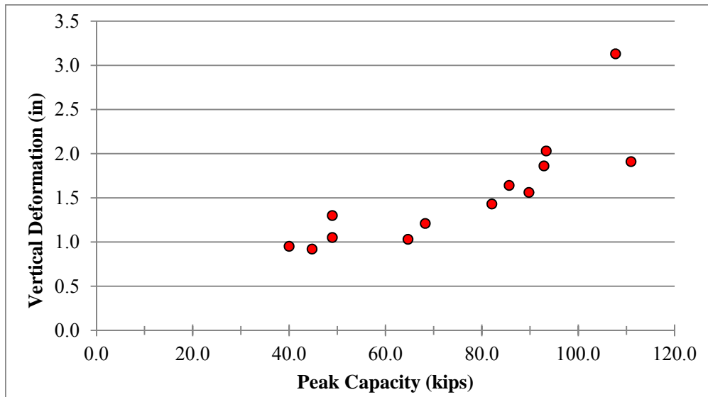
Figure 6.4 Vertical Deformation at Peak Capacity
