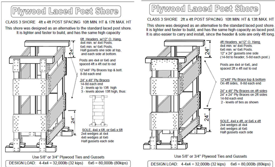
Figure 2.9 Plywood Laced Post Shore Specifications, 4ft x 4ft Base (Left), 2ft x 4ft Base (Right), (USACE FOG 2011)
