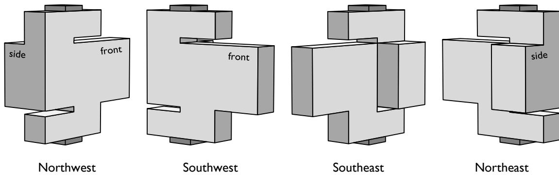
Figure 7-31: Modified push-off specimen viewed from four corners.
