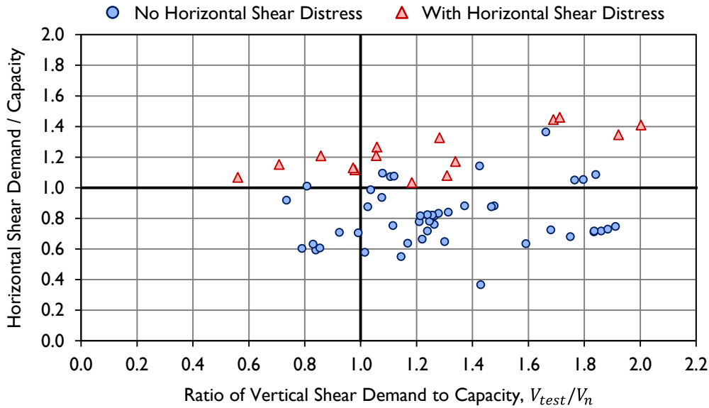
Figure 7-23: Ratios of vertical and horizontal shear demand to capacity for specimens in the HSED.
