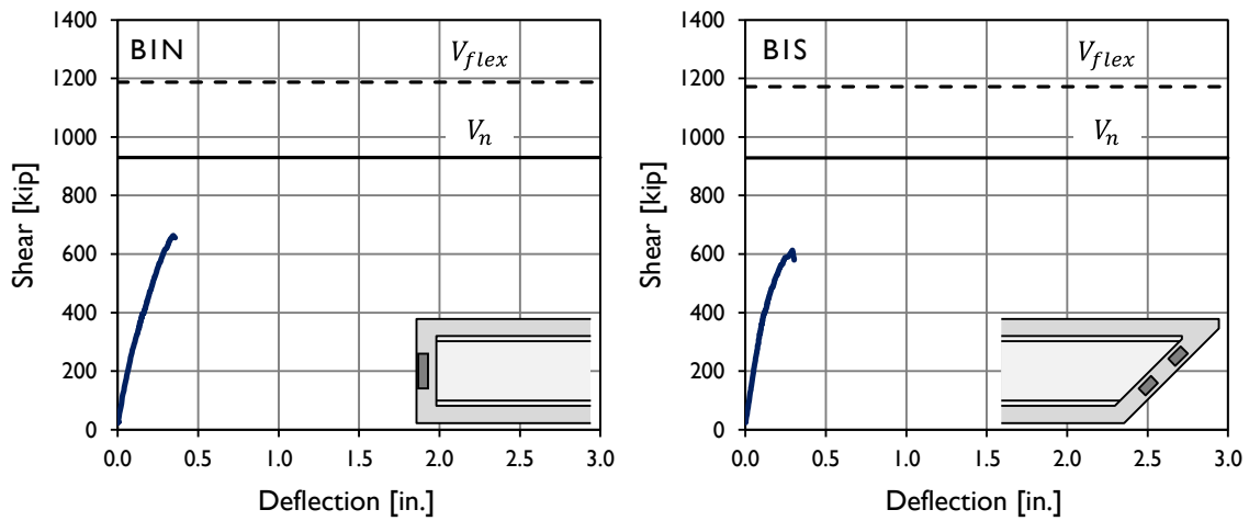
Figure B-45: Shear-deflection plot for specimens B1N and B1S.
