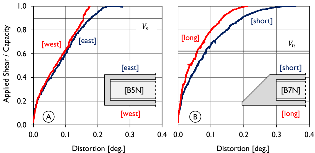
Figure 6-11: Typical distortion measured in the two webs of a rectangular and skewed beam.
