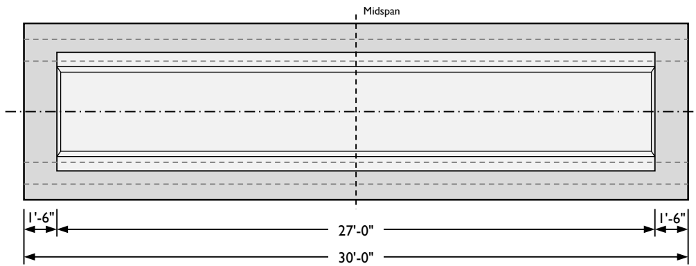
PLAN VIEW – Beam 3
