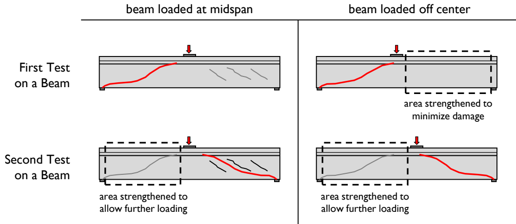
Figure 3-20: Schematic of how and when external post-tensioned clamps were used to aid in achieving a second failure within one beam.
