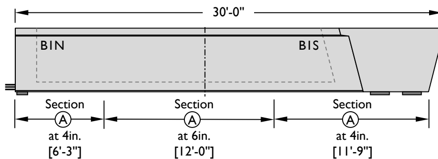
Figure 4-2: (ii) Elevation view of Beam 1.
