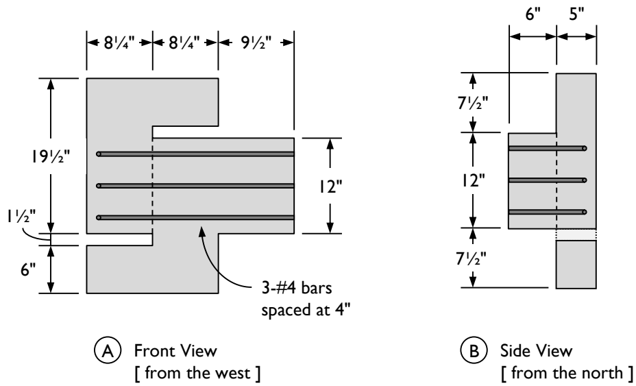
Figure 7-30: Dimensions and interface reinforcing bar locations in modified push-off specimens.
