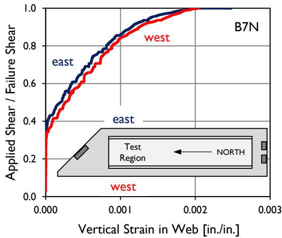
Figure B-37: Vertical strains measured in the webs of test specimen B7N during loading.
