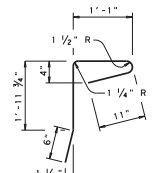
BARS X (#4)
