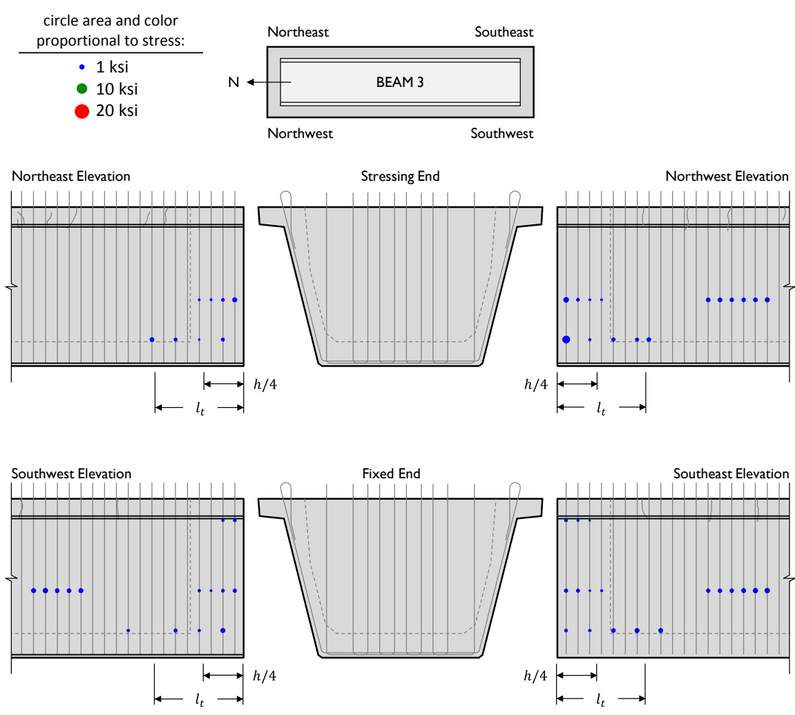
Figure B-3: Magnitude and location of cracking and stresses induced in reinforcement at prestress transfer for Beam 3.
