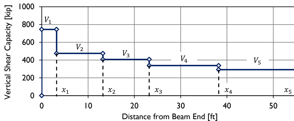
Figure 7-38: Typical vertical shear capacity plot.
