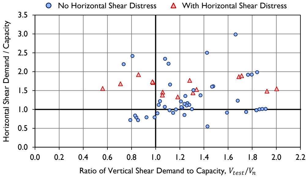
Figure 7-24: HSR-SPR plot for specimens in the HSED with calculations for capacity performed using the ACI (2008) shear-friction equation.
