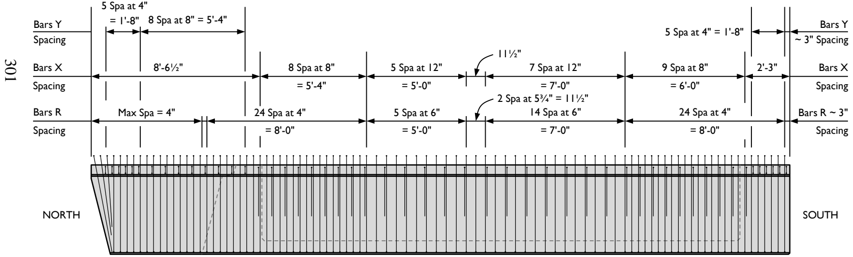
PLAN VIEW – Beam 7
