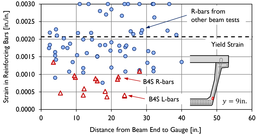
Figure 6-27: Measured strains in web reinforcing bars at bottom flange-to-web interface just before failure.
