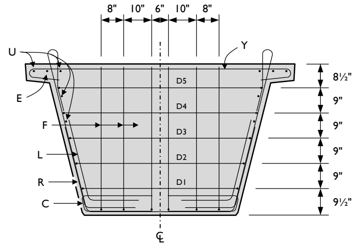
SECTION D-D - Beam 6
