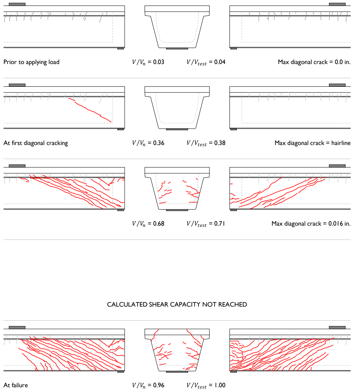
Figure B-20: Cracks observed during testing of specimen B3N.
