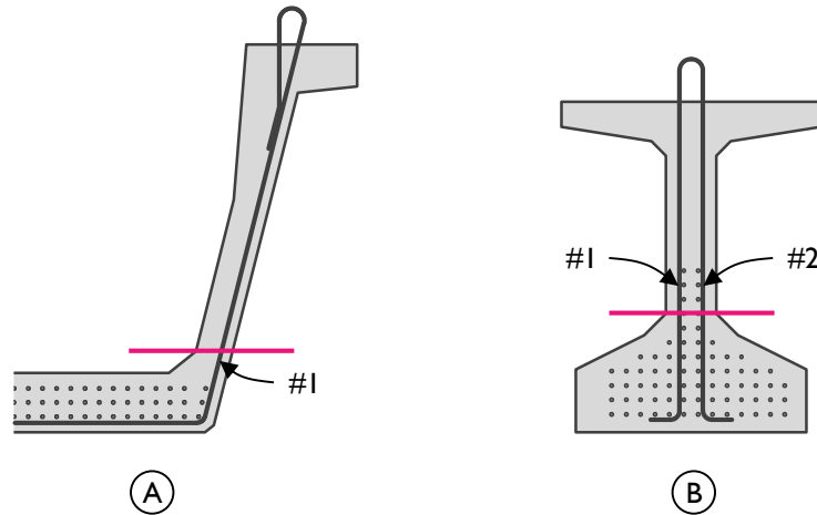
Figure 7-27: (A) Typical U-Beam and (B) I-Beam bottom flange-to-web interface and reinforcing.
