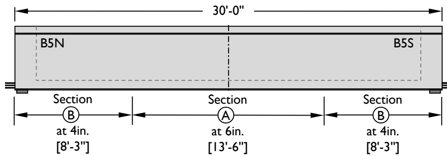
Figure 5-6: (i) Elevation view of Beam 5.
