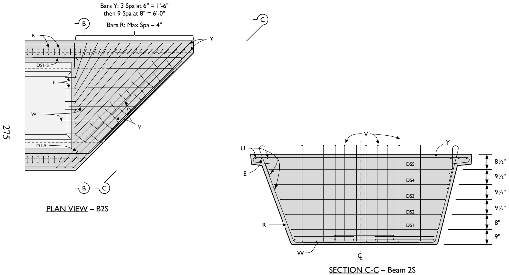
Figure A-14: Beam 2 south end region plan view and cross-sections
