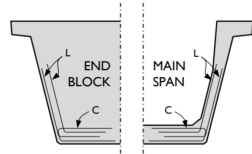
CROSS-SECTIONS – Beam 6
