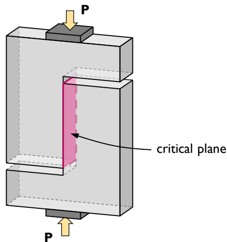
Figure 7-26: Typical push-off specimen as described in literature.
