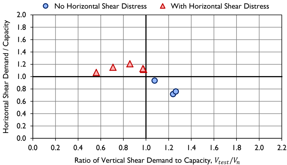
Figure 7-36: Summary of comparison between horizontal and vertical shear demand and capacity for Texas U-Beams, with correction factor in horizontal shear capacity calculation.
