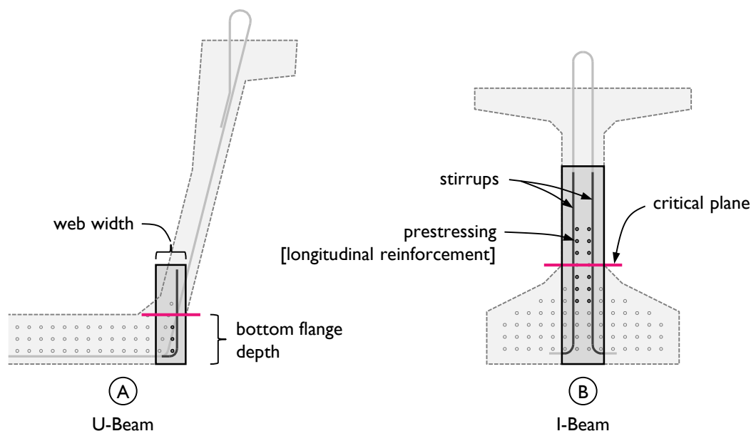
Figure 7-28: Critical interface of push-off specimens based on the reinforcement of (A) a standard Texas U-Beam and (B) an I-Beam (Tx 46).
