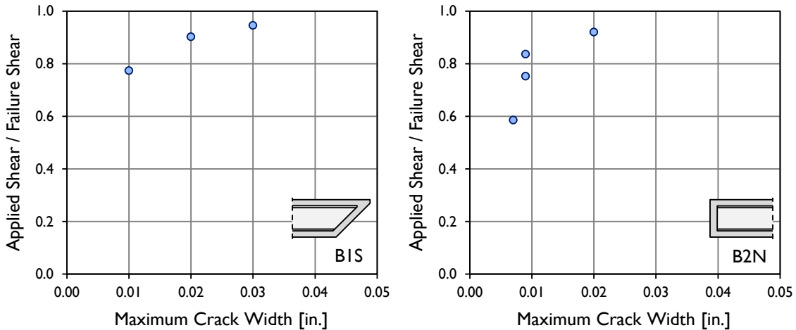
Figure B-28: Maximum crack widths measured in test specimens B1S and B2N.
