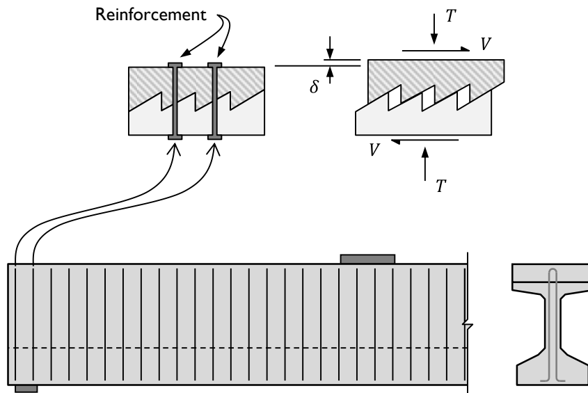
Figure 7-33: Elevation view of a beam and the shear-friction model.
