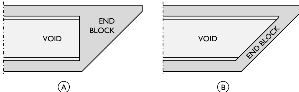
Figure 3-3: Plan view of end block options in skewed U-Beams: (A) square void with triangular end block, and (B) skewed void with square end block.
