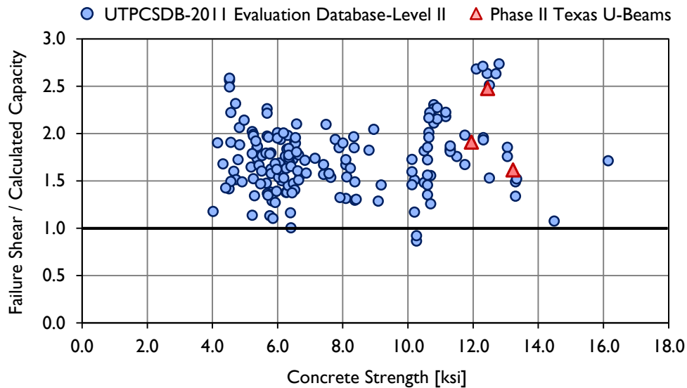
Figure 6-34: Texas U-Beam failure shear-to-calculated shear ratios (capacity calculated using the AASHTO Segmental Procedure (2010) with no limit on K ), compared to other UTPCSDB-2011 data points.
