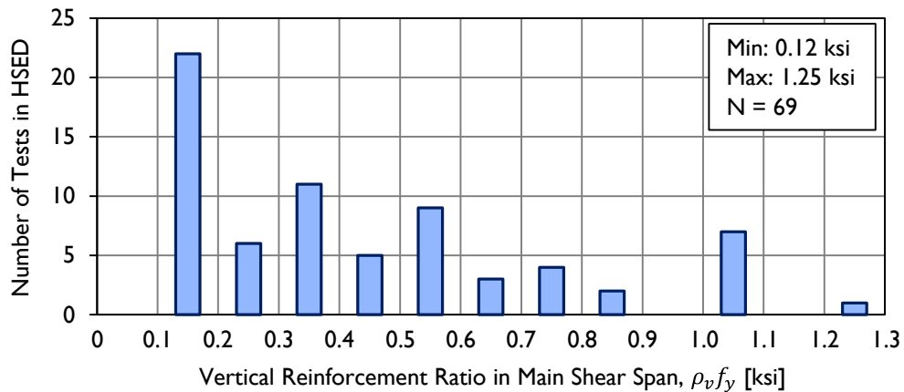
Figure 7-22: Distribution of vertical reinforcement ratio for specimens in the HSED.
