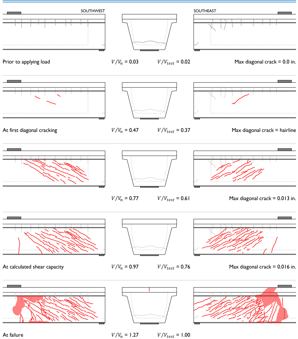
Figure B-25: Cracks observed during testing of specimen B6S.
