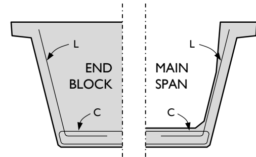
CROSS-SECTIONS – Beam 5
