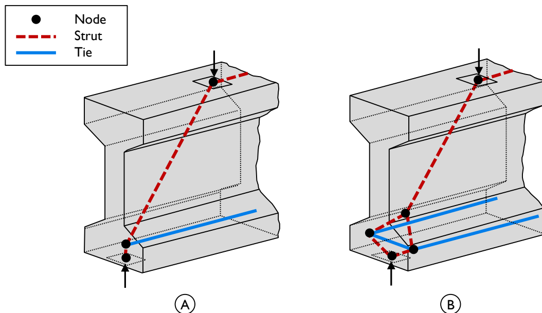
Figure 2-15: Strut-and-tie model for beam with (A) fully bonded tendons and (B) significant numbers of unbounded tendons located beneath the web (from Hamilton, Llanos, and Ross, 2009).
