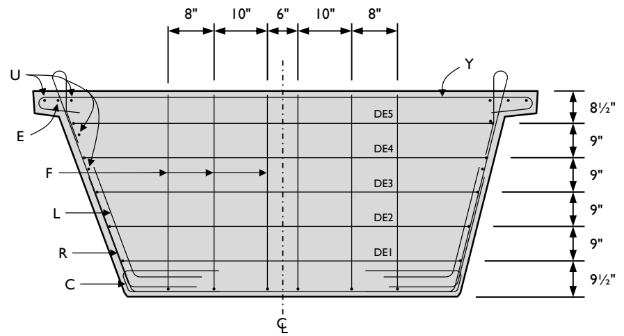
Figure A-36: Beam 7 north end-region plan views and cross-sections (1 of 2).
