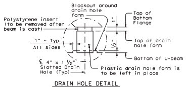
DRAIN HOLE DETAIL
