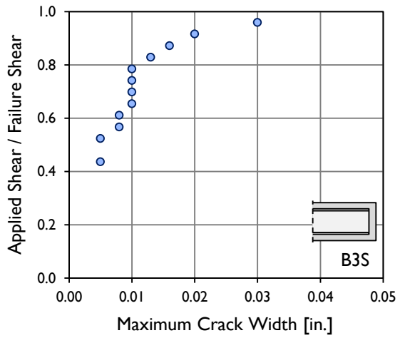
Figure B-29: Maximum crack widths measured in test specimens B3N and B3S.
