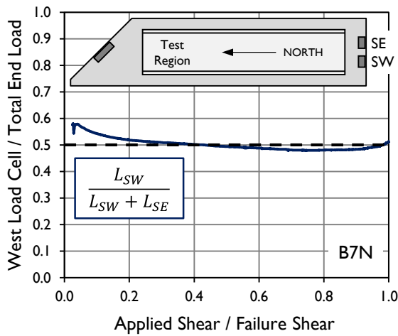
Figure B-15: Distribution of load into two bearing pads during testing of specimen B7N.
