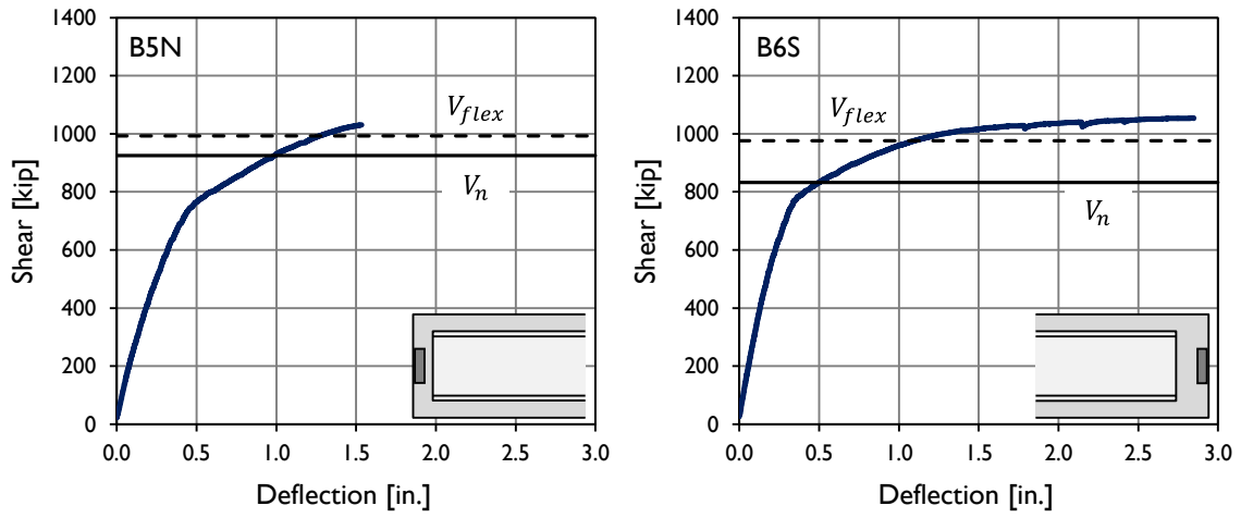
Figure B-49: Shear-deflection plot for specimens B5N and B6S.
