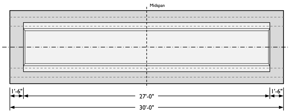
PLAN VIEW – Beam 5
