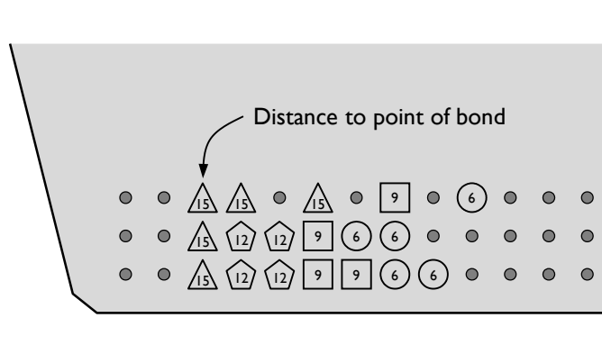
Figure A-16: Distance from beam end to point of bond for strands in Beam 3.
