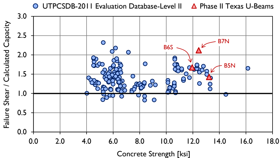
Figure 6-32: Texas U-Beam failure shear-to-calculated shear ratios (capacity calculated using ACI Detailed Method (2008)), compared to other UTPCSDB-2011 data points.
