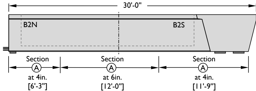
Figure 4-5: (ii) Elevation view of Beam 2.
