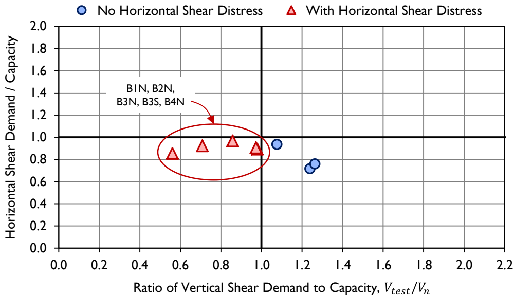
Figure 7-25: Summary of comparison between horizontal and vertical shear demand and capacity for Texas U-Beams.
