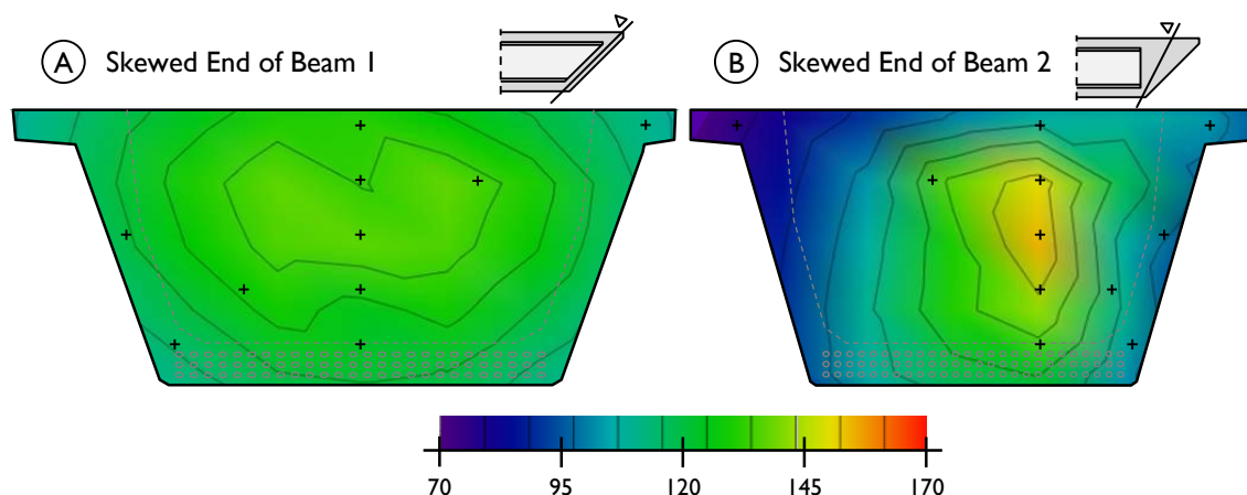
Figure 6-7: Temperatures measured through the cross sections of the skewed end blocks of Beam 1 and Beam 2 at time of maximum temperature reading.
