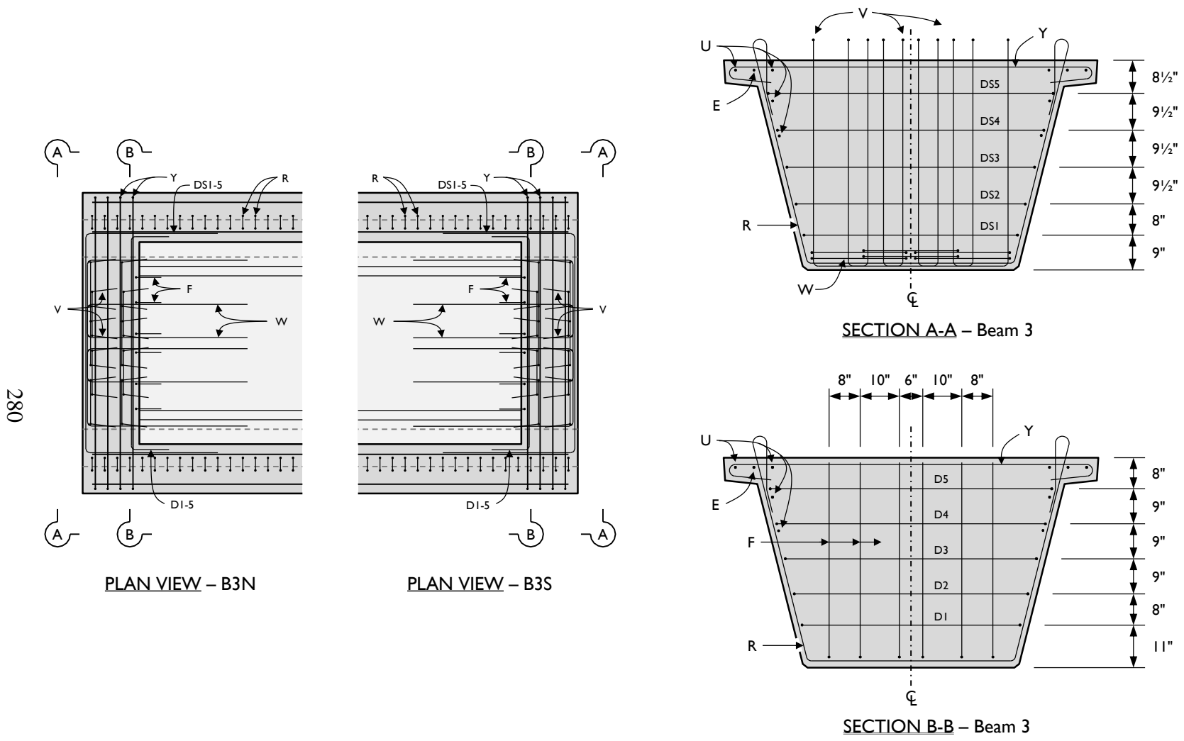
Figure A-18: Beam 3 end-region plan views and cross-sections.
