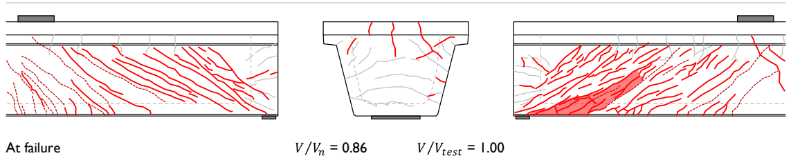
Figure B-22: Cracks observed during testing of specimen B4N.
