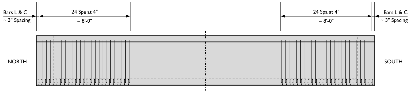
ELEVATION VIEW – Beam 5 Supplementary Reinforcement
