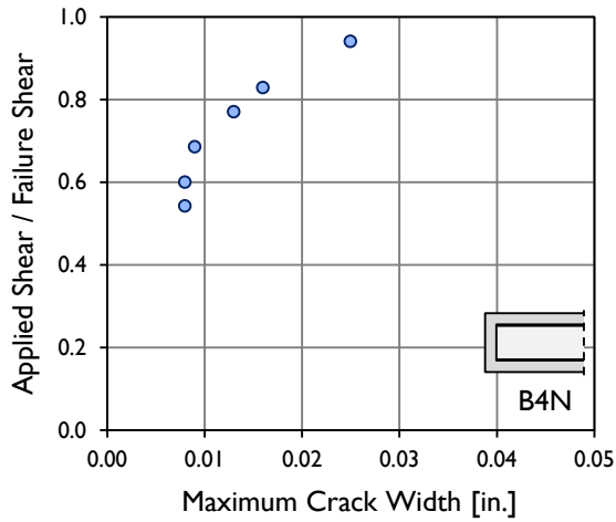
Figure B-30: Maximum crack widths measured in test specimens B4N and B4S.
