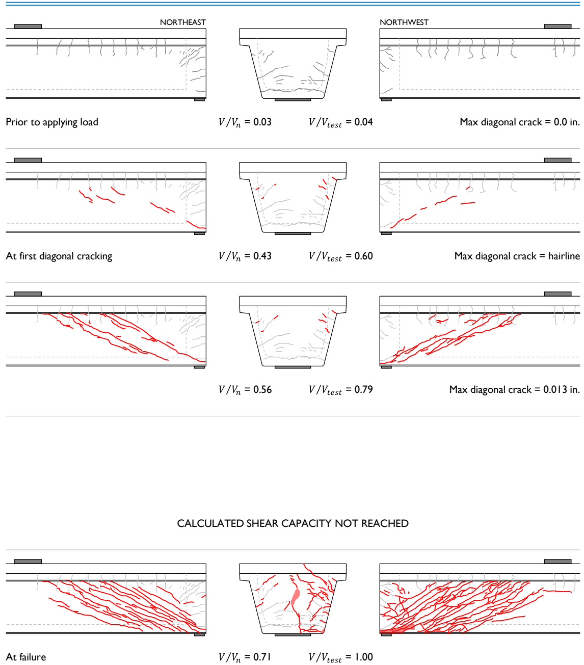
Figure B-17: Cracks observed during testing of specimen B1N.
