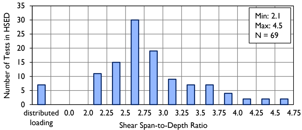
Figure 7-21: Distribution of shear span-to-depth ratio used in tests in the HSED.
