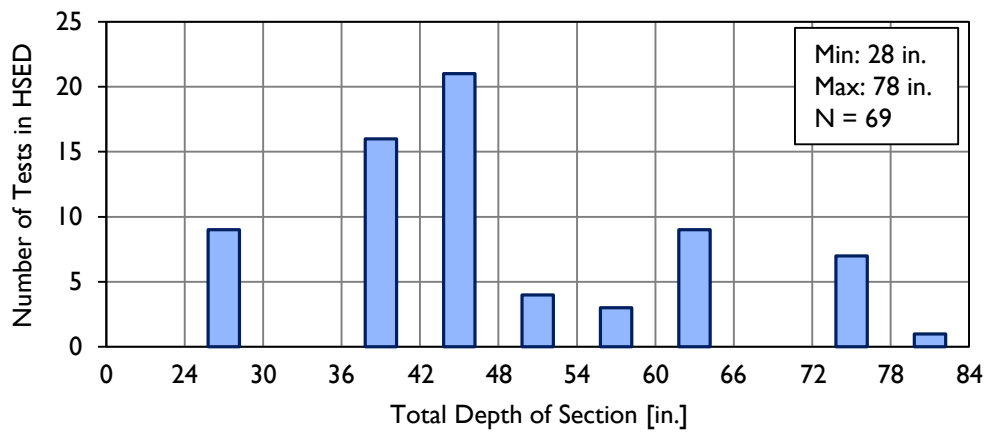
Figure 7-20: Distribution of specimen size in the HSED.
