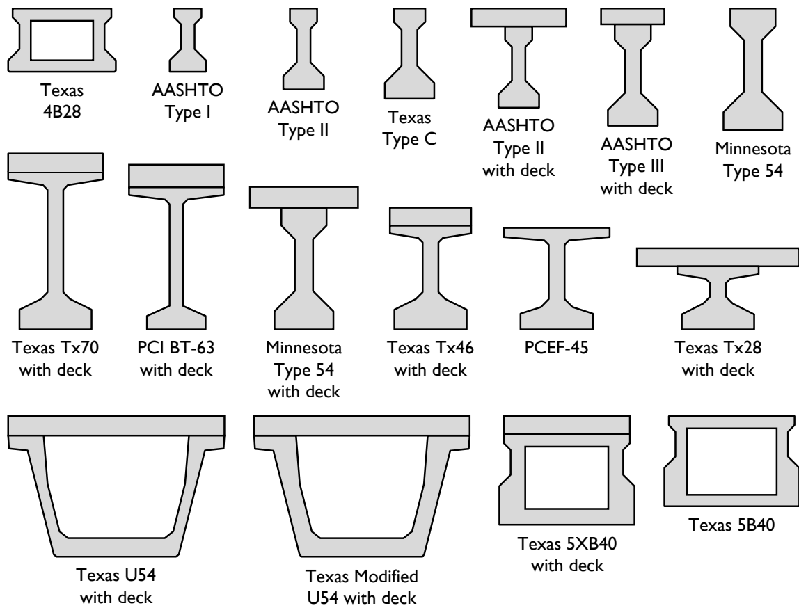
Figure 7-18: Beam shapes included in the Horizontal Shear Evaluation Database.
