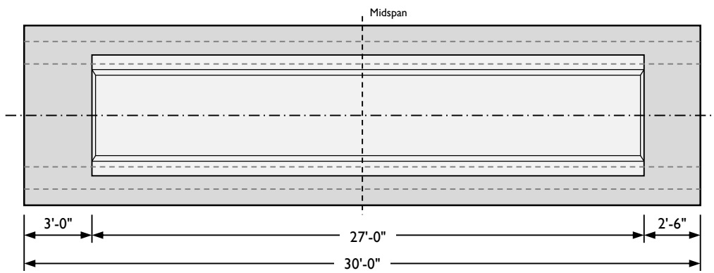
PLAN VIEW – Beam 6
