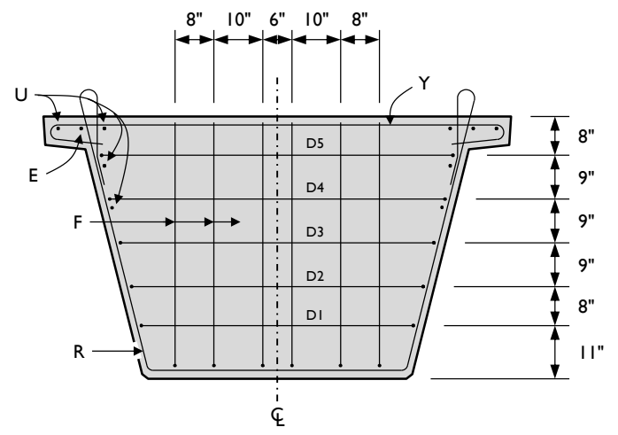
Figure A-9: Beam 1 north end-region plan view and cross-sections.
