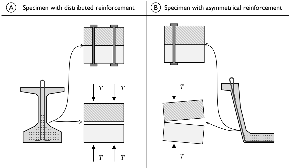
Figure 7-34: Cross-sectional view of shear-friction specimens with (A) distributed and (B) asymmetrical reinforcement.
