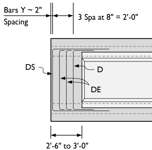
Figure 6-36: Reinforcing bar changes in the end block.
