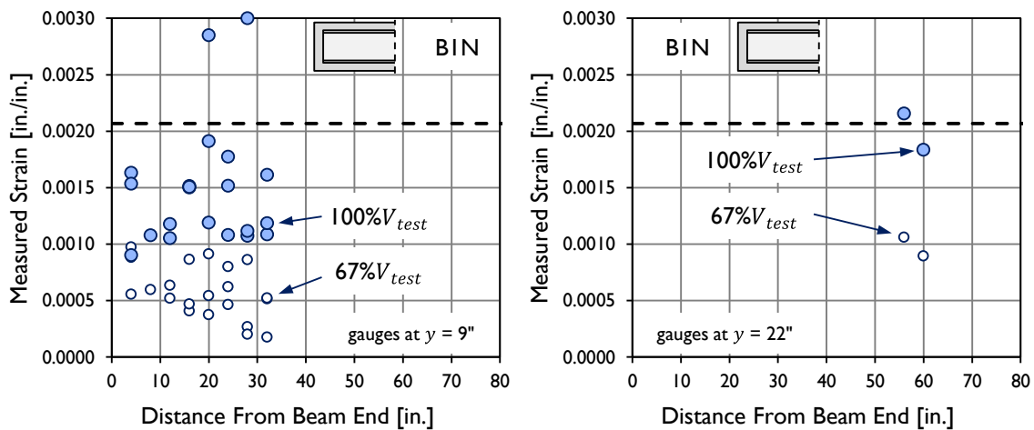
Figure B-38: Strain measured in reinforcing bars during load-testing of specimen BIN.
