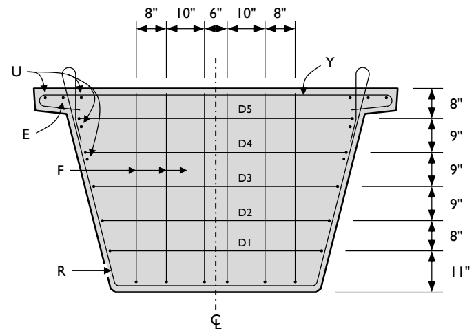
Figure A-6: Beam 0 end-region plan views and cross-sections.
