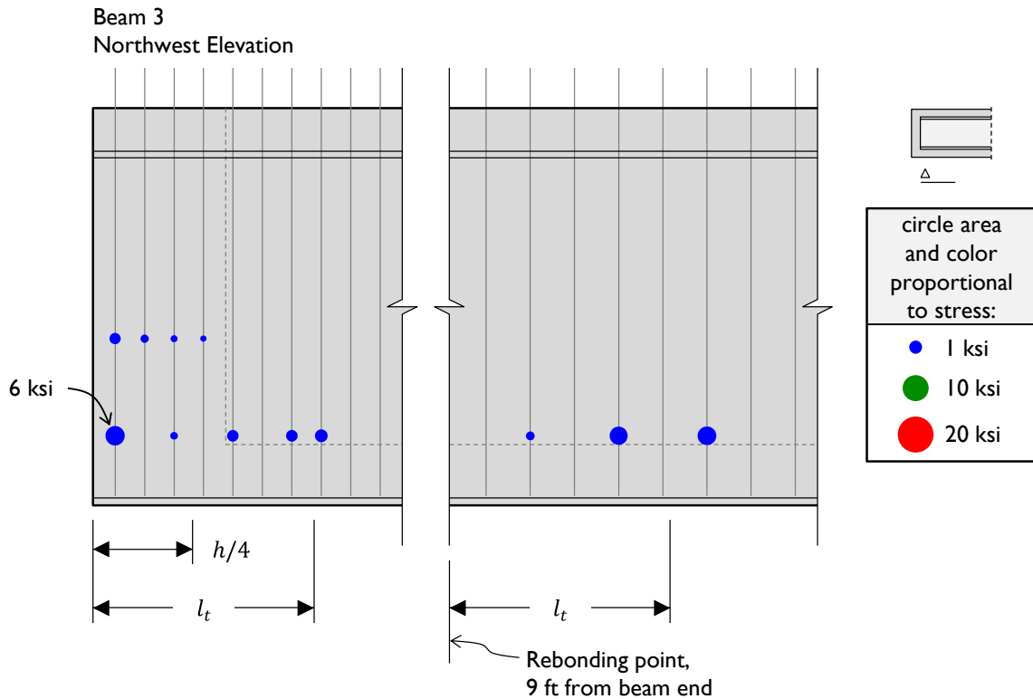
Figure 6-4: Typical beam end region in beam with debonded strands (B3N).
