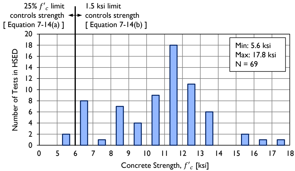
Figure 7-19: Distribution of concrete strength for specimens in the HSED.
