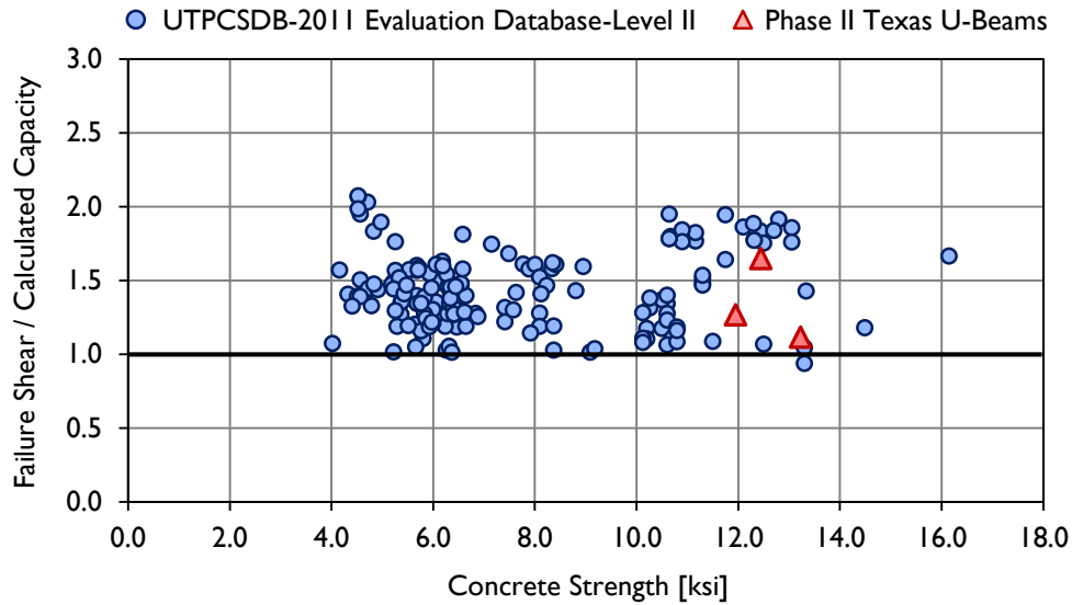
Figure 6-33: Texas U-Beam failure shear-to-calculated shear ratios (capacity calculated using AASHTO General Procedure (2010)), compared to other UTPCSDB-2011 data points.
