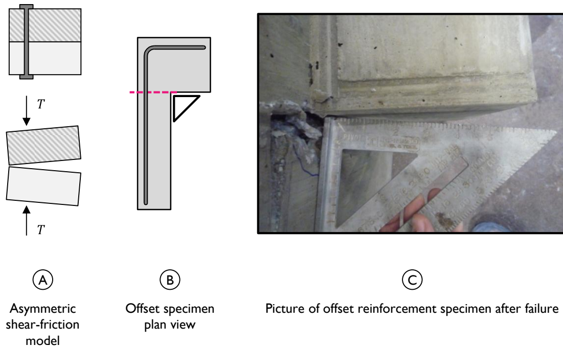
Figure 7-35: Observations of asymmetric opening of shear-friction interface.
