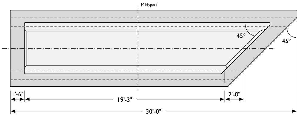
PLAN VIEW – Beam I
