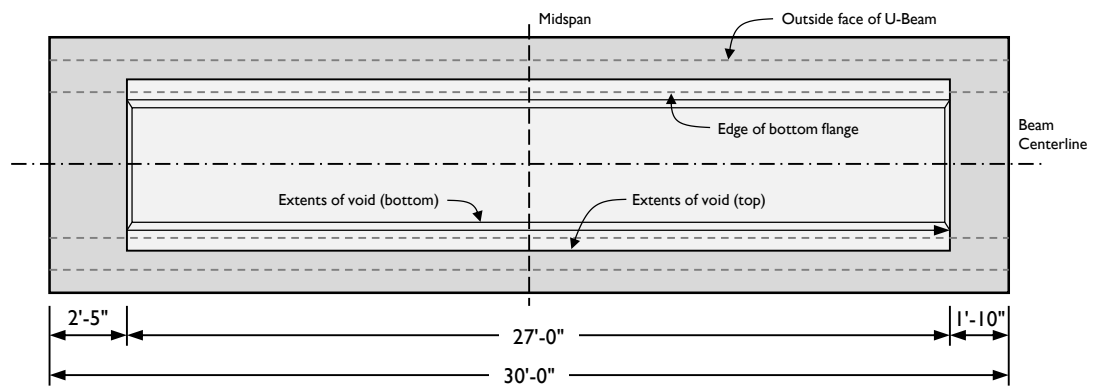
PLAN VIEW – Beam 0
