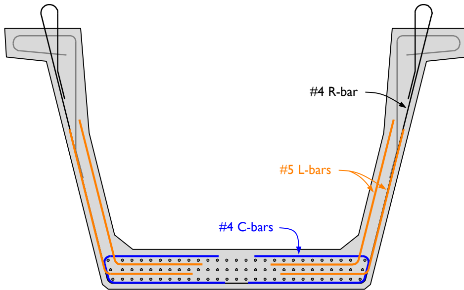
Figure 6-35: Key reinforcing bars in the recommended new Texas U-Beam design.
