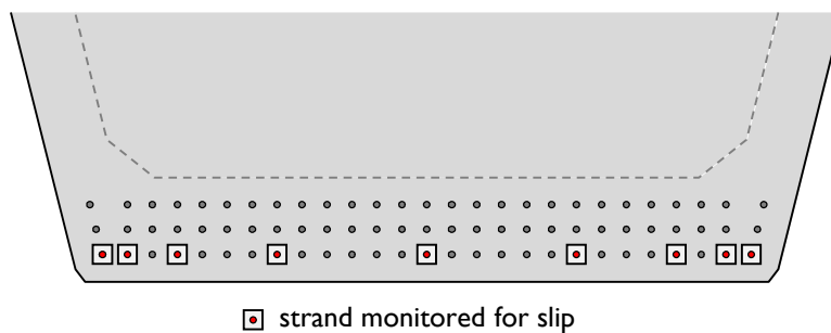
Figure 3-18: Typical locations for strand slip gauges during shear testing.
