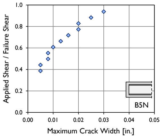
Figure B-31: Maximum crack widths measured in test specimens B5N and B6S.
