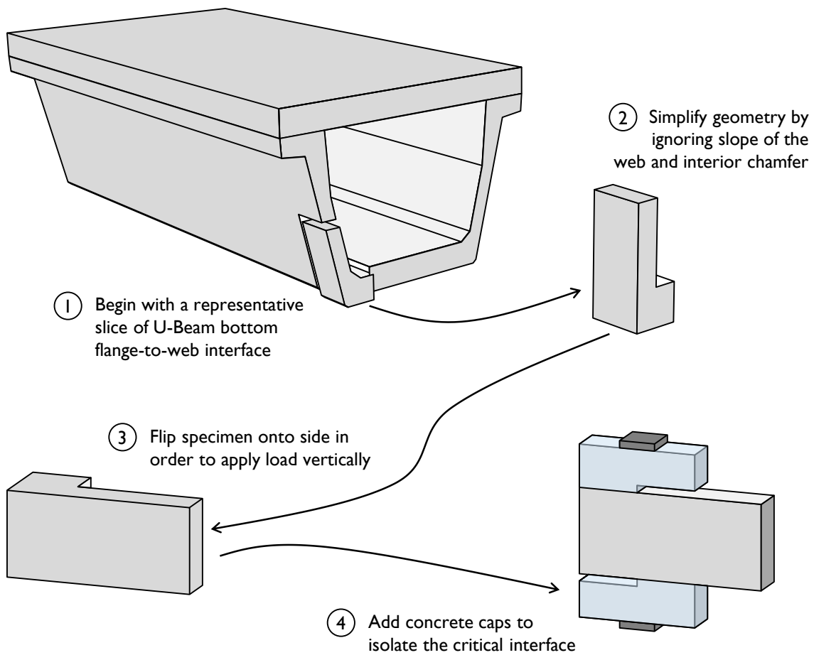
Figure 7-29: Steps taken to design the modified push-off specimens used.
