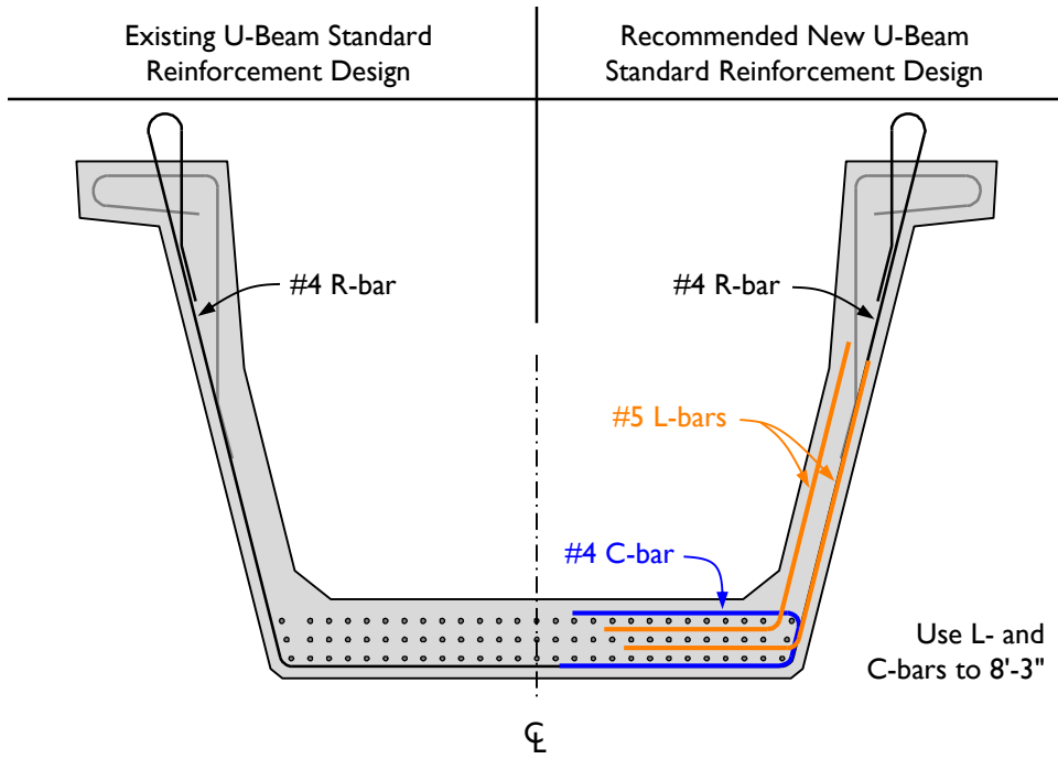
Figure 8-1: Existing and recommended U-Beam standard reinforcement.
