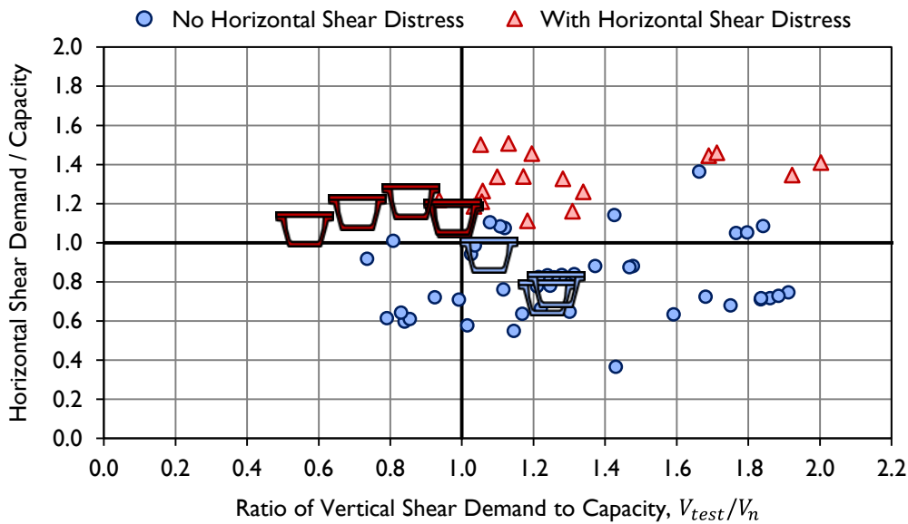
Figure 7-37: Ratio of horizontal shear demand to capacity for all points in the HSED.
