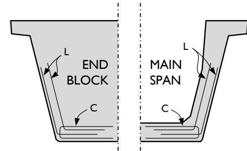
CROSS-SECTIONS – Beam 4
