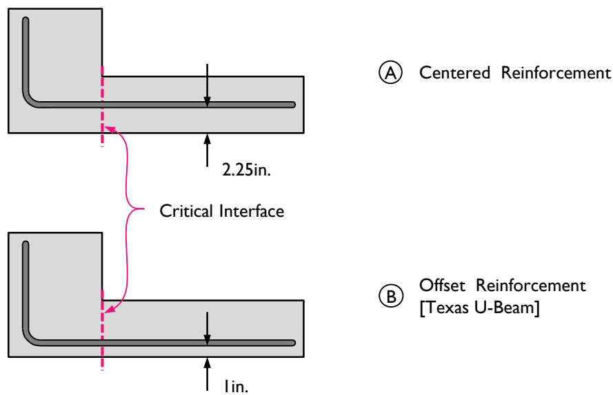
Figure 7-32: Placement of reinforcing bars crossing critical plane in modified push-off specimens.
