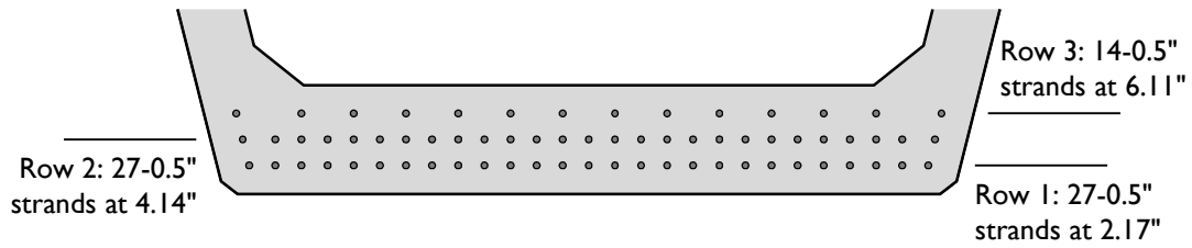
Figure A-4: Prestressing strand positions for Beam 0.
