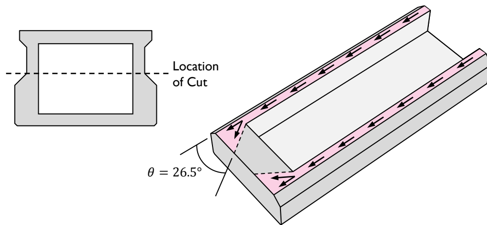
Figure 7-13: Area of concrete involved in resisting horizontal shear in beams in end blocks.
