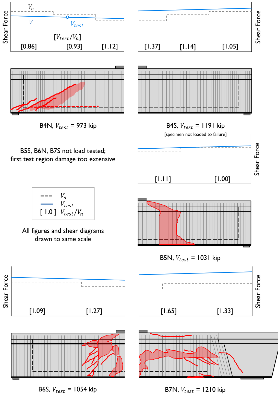
Figure 6-31: Summary of Phase II U-Beam shear tests.
