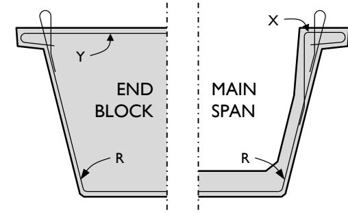
CROSS-SECTIONS – Beam 3
