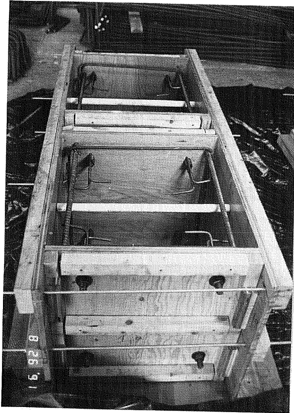
Figure 3.11 Formwork with reinforcement and inserts in place.
