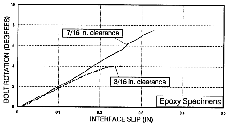
Figure 4.86 Rotation-slip plots for monotonic tests (connections with epoxy).
