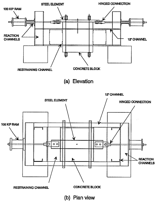
Figure 3.27 Plan view and elevation of test frame.
