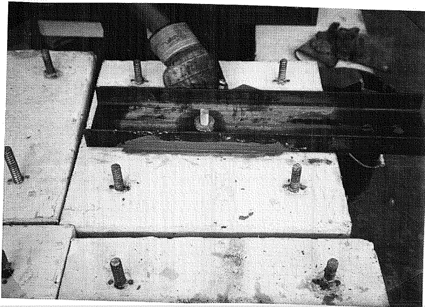
Figure 3.25 Specimen during removal of excess grout at interface.
