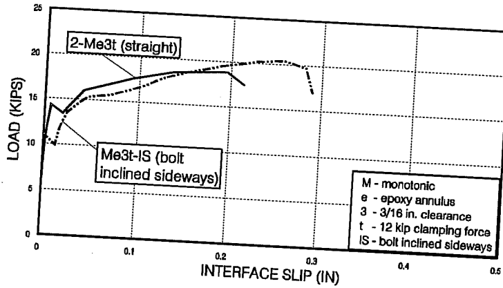
Figure 4.27 Effect of 4 degree bolt inclination perpendicular to the direction of loading (specimens with epoxy-filled annulus and 3/16 in. hole clearance).
