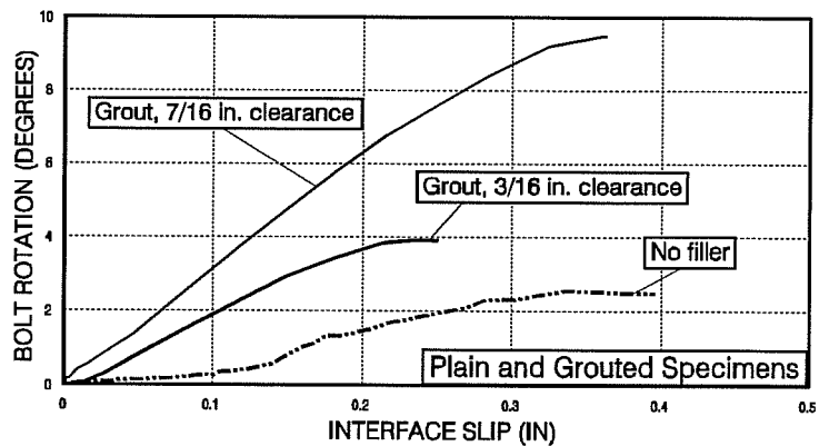
Figure 4.85 Rotation-slip plots for monotonic tests (plain test and connections with grout).
