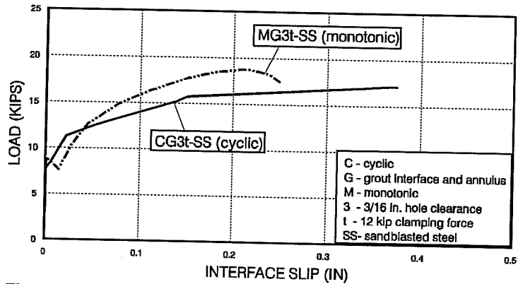
Figure 4.58 Comparison of response envelope & monotonic load-slip plot for the effect of cyclic loading (tests with non-shrink grout & 3/16 in. hole clearance).
