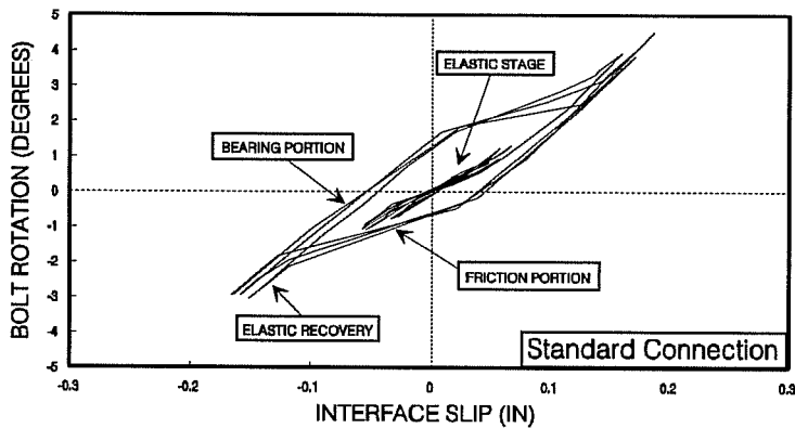
Figure 4.87 Typical rotation-slip plot for cyclic tests with standard washers – Test 2-Ce7t-SP.
