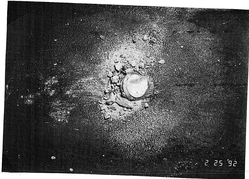
Figure 4.55 Crushed concrete into annulus of steel element by excessive bolt deformation – Test CN3h-WN.
