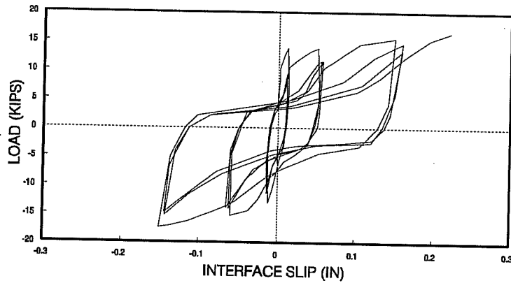
Figure 4.45 Load-slip plot – Test Ce3t-SP.
