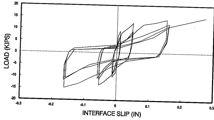
Figure 4.39 Load-slip plot – Test CG7T-SS.
