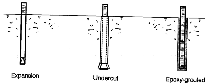
Figure 2.4 Types of retrofit anchors.
