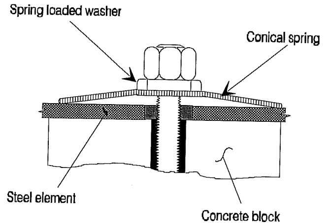
Figure 2.7 Spring-loaded connection.
