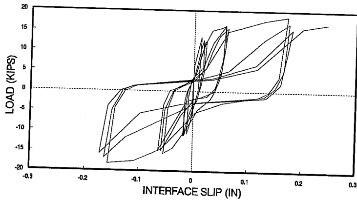
Figure 4.41 Load-slip plot – Test Ce3t.
