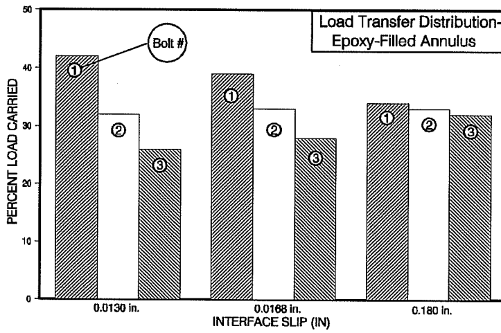
Figure 5.9 Estimated percentage of load resisted by bolts in sample connection with an epoxy-filled annulus (Case I).
