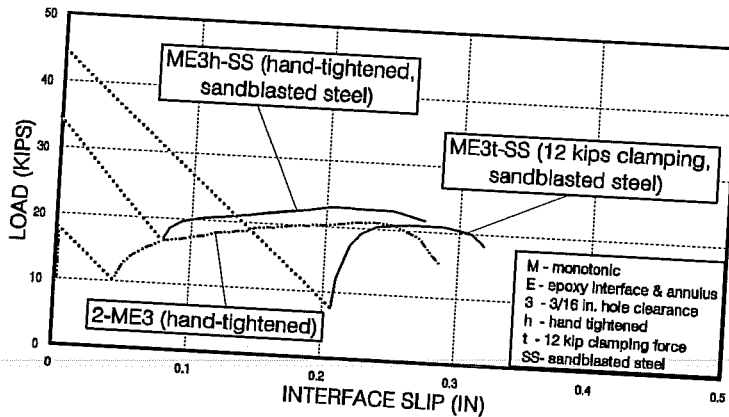
Figure 4.29 Effect of interface epoxy (3/16 in. hole clearance).
