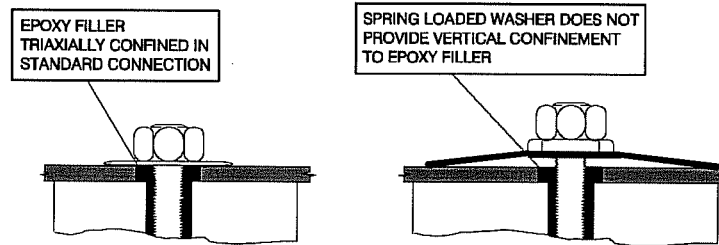
Figure 4.81 Schematic of state of confinement of filler with different washer types.
