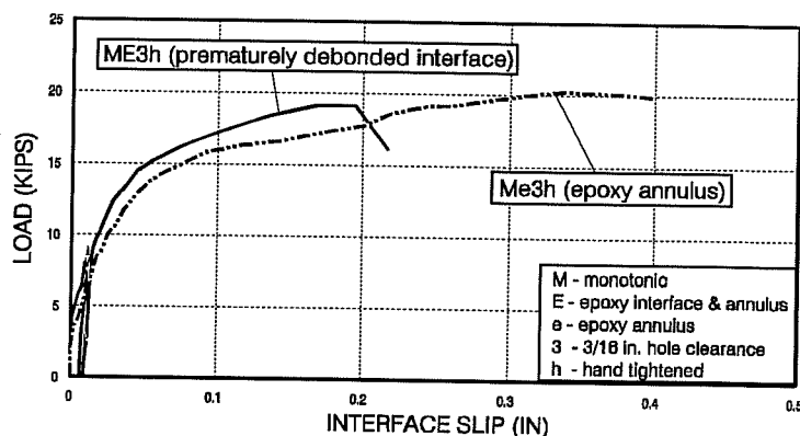
Figure 4.30 Comparison of test with debonded epoxy interface and test with epoxy-filled annulus (hand-tightened tests with 3/16 in. hole clearance).
