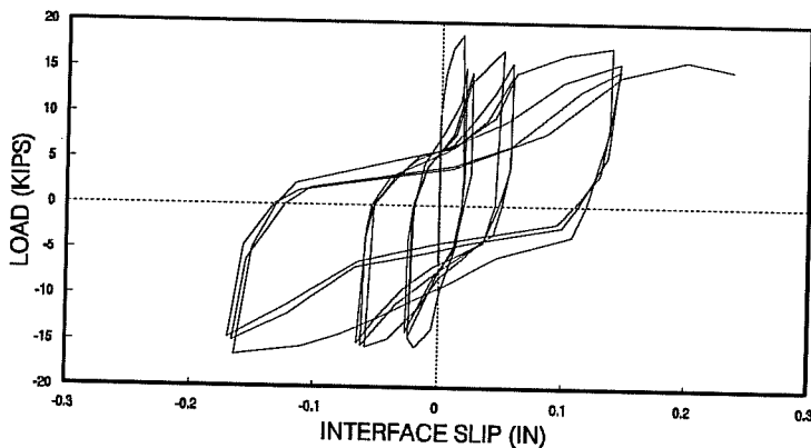
Figure 4.47 Load-slip plot – Test Ce3T-SP.
