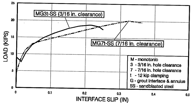
Figure 4.9 Effect of hole clearance (tests with grout in the annulus and interface).
