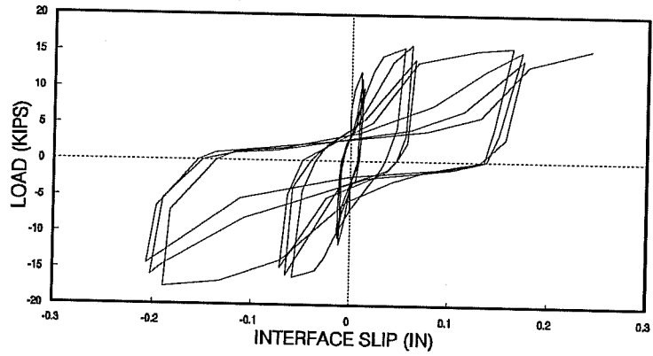
Figure 4.43 Load-slip plot – Test Ce3T.
