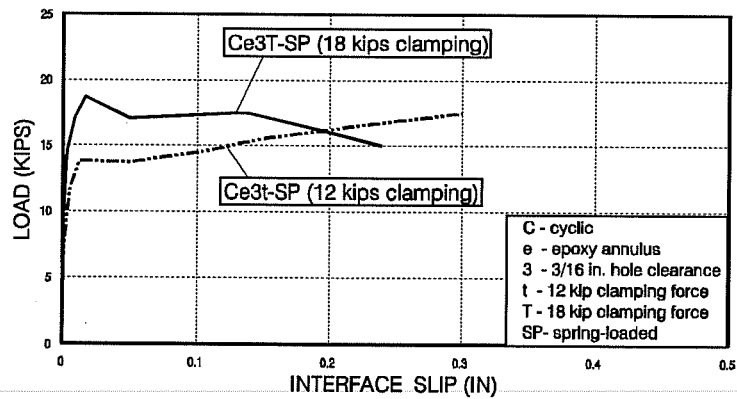
Figure 4.82 Response envelopes for the effect of increased clamping force (tests with spring-loaded washer and 3/16 in. hole clearance).
