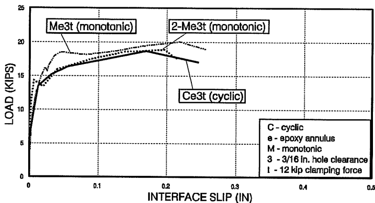
Figure 4.72 Comparison of response envelope & monotonic load-slip plot for the effect of cyclic loading (tests with epoxy-filled annulus & 3/16 in. hole clearance).
