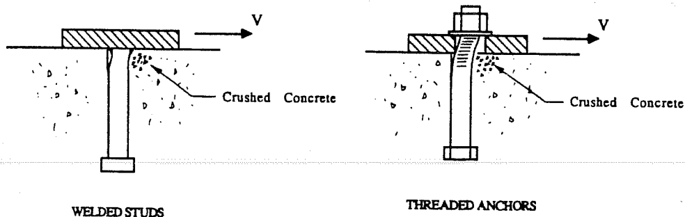
Figure 2.6 Deformations of welded studs and threaded anchors in shear. 19
