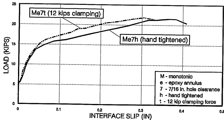
Figure 4.21 Effect of clamping force (specimens with epoxy-filled annulus and 7/16 in. hole clearance).
