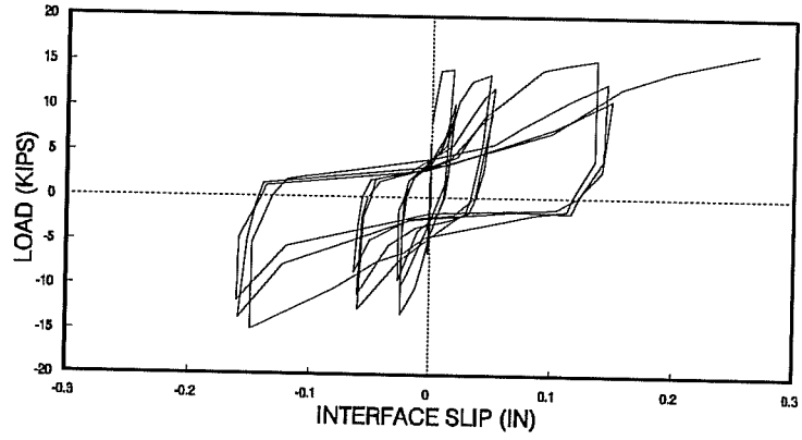
Figure 4.42 Load-slip plot – Test Ce7t.
