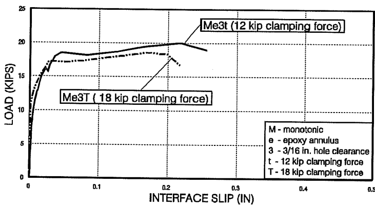
Figure 4.17 Effect of increased clamping force to 18 kips (tests with epoxy-filled annulus and 3/16 in. hole clearance).
