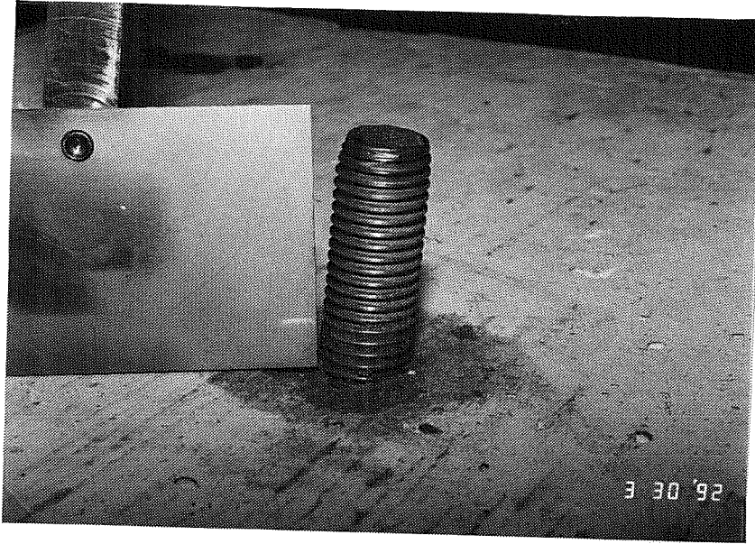
Figure 3.6 Anchor bolt with initial inclination.
