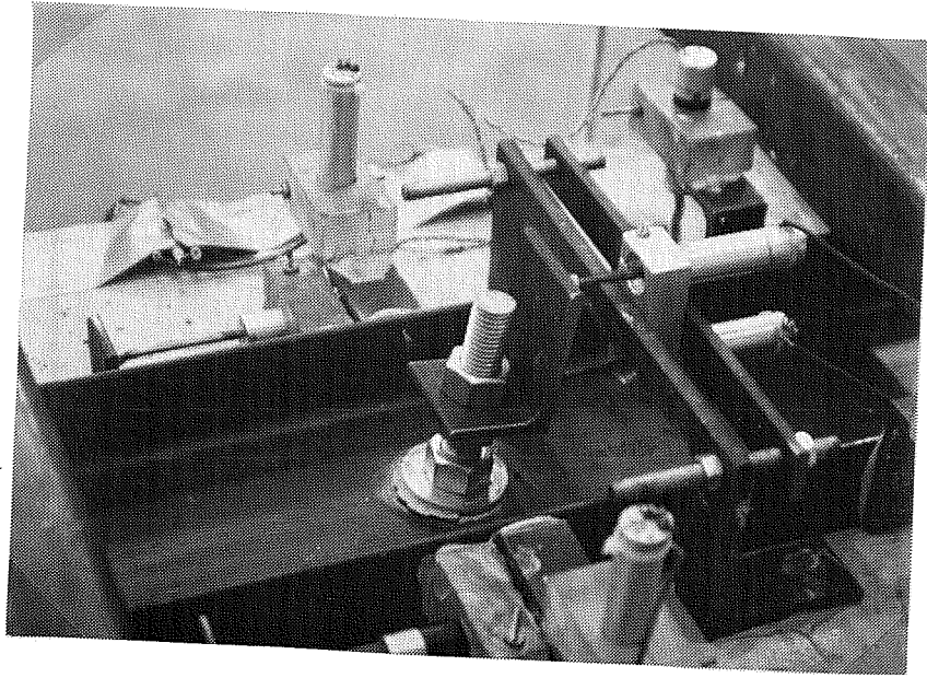
Figure 4.4 Anchor bolt rotation at large relative slip of the steel element.
