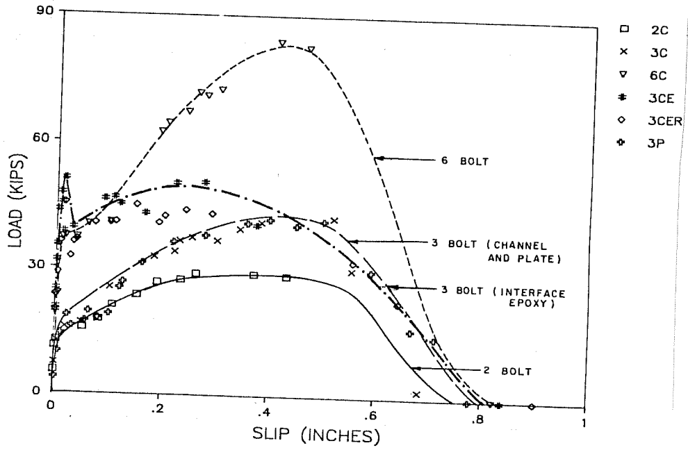
Figure 2.9 Envelopes of response in tests conducted by Wiener. 45
