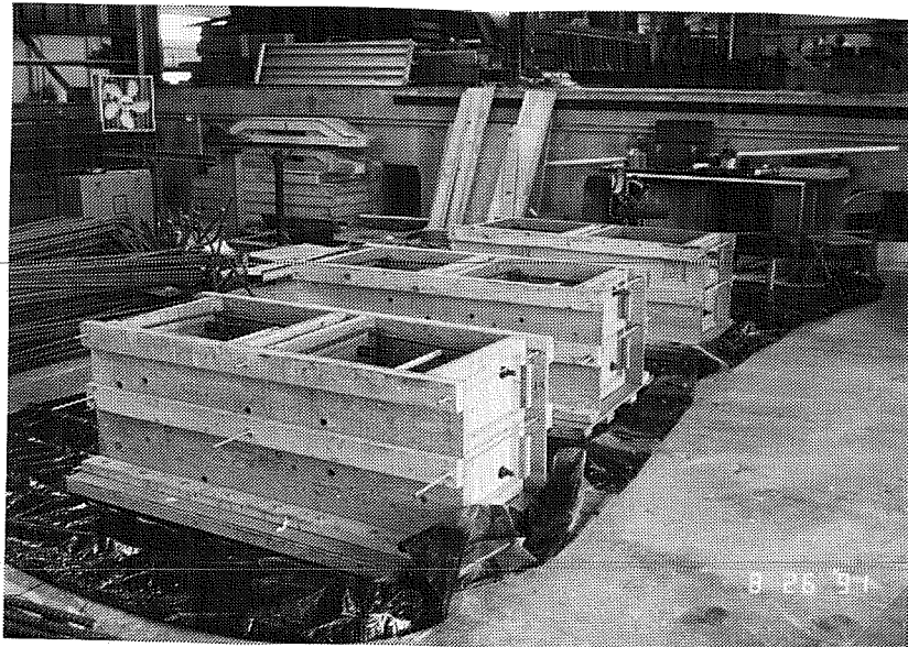
Figure 3.12 Completed formwork.
