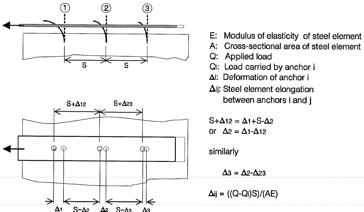
Figure 5.5 Schematic of distribution of deformations in multiple-anchor steel-to-concrete connection.
