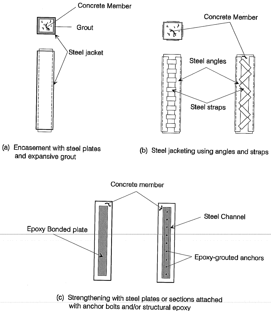
Figure 2.2 Steel jacking techniques.
