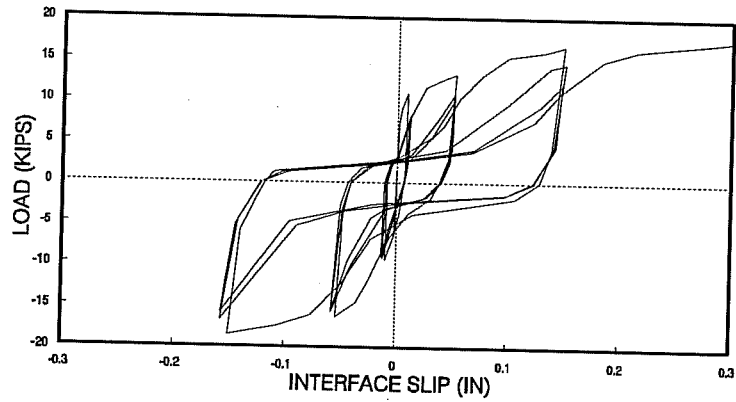
Figure 4.44 Load-slip plot – Test Ce3t-IB.
