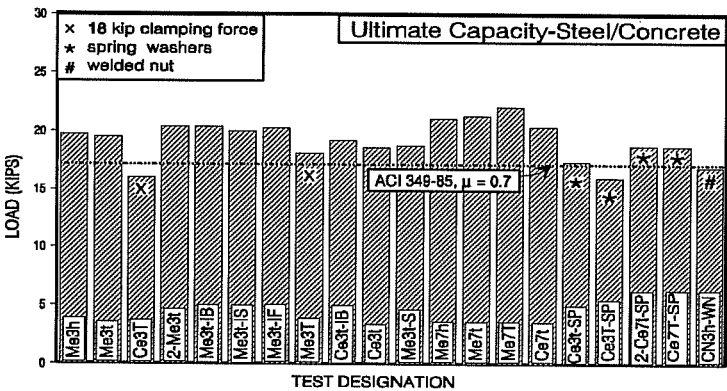
Figure 5.4 Comparison of measured capacities for tests without grout at the interface and ACI 349-85 shear friction strengths.
