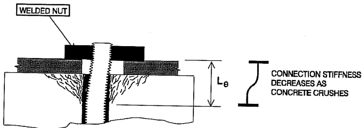
Figure 4.52 Schematic of behavior of welded nut connection.
