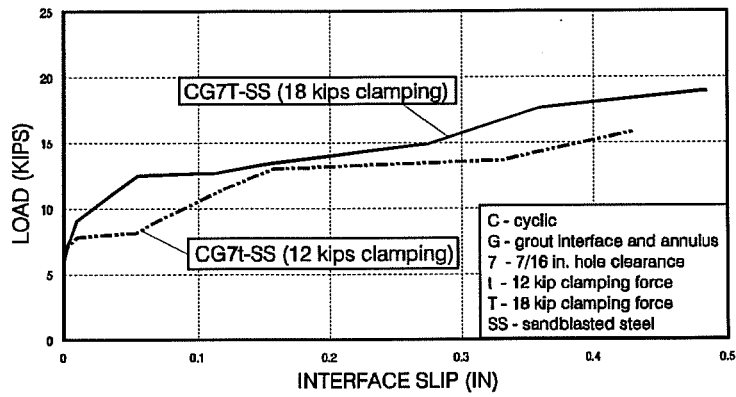
Figure 4.64 Response envelopes for the effect of increased clamping force (tests with non-shrink grout and 7/16 in. hole clearance).
