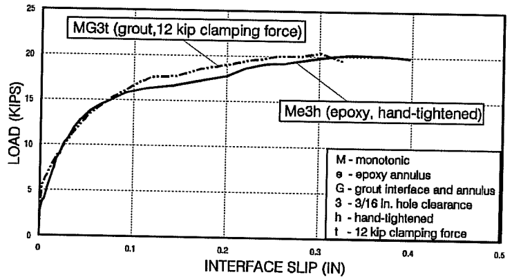
Figure 4.14 Comparison of hand-tightened test filled with epoxy versus torqued connection with non-shrink grout.
