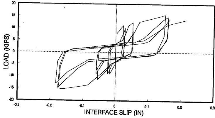
Figure 4.36 Load-slip plot – Test CG3t-SS.
