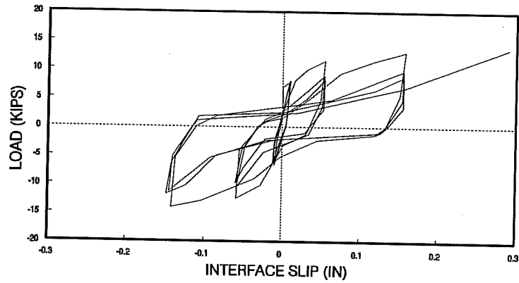
Figure 4.37 Load-slip plot – Test CG7t-SS.
