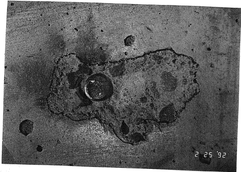
Figure 4.54 Crushing of concrete after removal of loose material – Test CN3h-WN.
