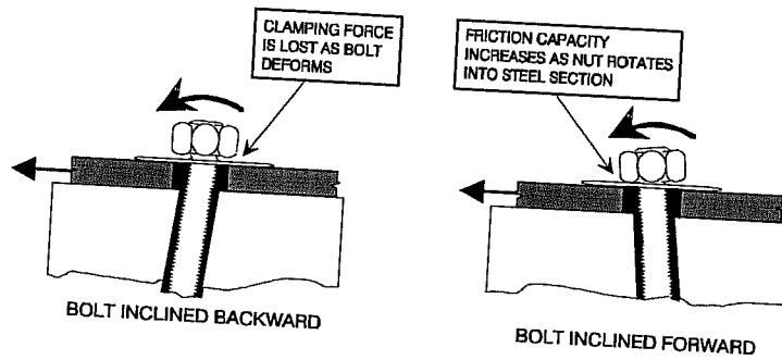
Figure 4.28 Schematic of behavior of inclined anchors.
