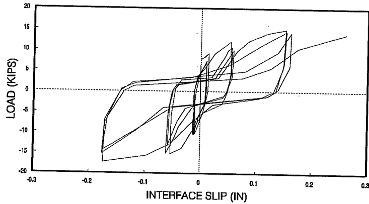
Figure 4.38 Load-slip plot – Test CG3T-SS.
