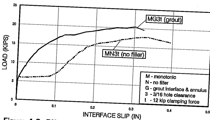
Figure 4.3 Effect of grout in the annulus and interface.
