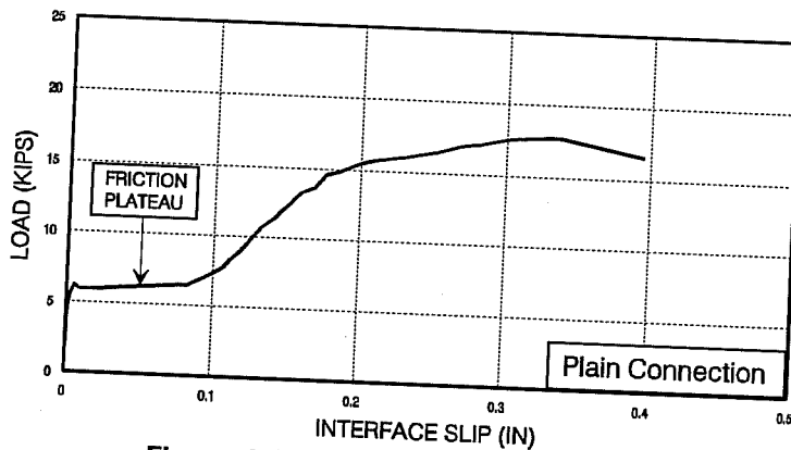
Figure 4.2 Load-slip plot-test MN3t.
