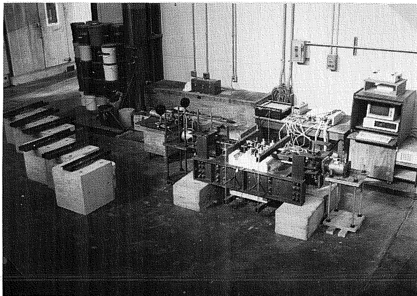
Figure 3.28 Overall view of test set-up with specimens ready for testing.
