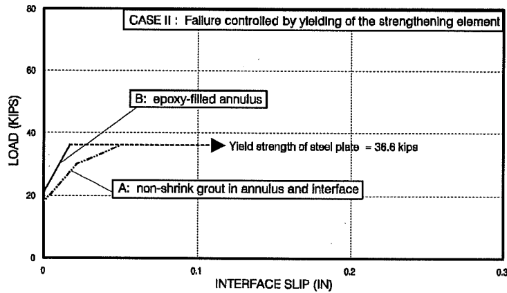
Figure 5.8 Load-interface slip response of analyzed multi-anchor connection (Case II).
