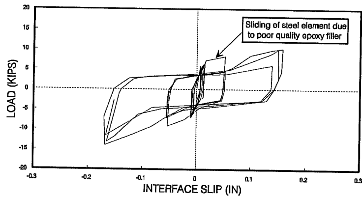
Figure 4.49 Load-slip plot – Test Ce7t-SP.
