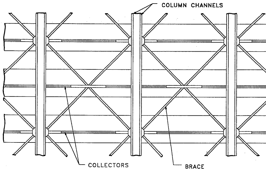
Figure 2.1 Steel bracing retrofit scheme. 11
