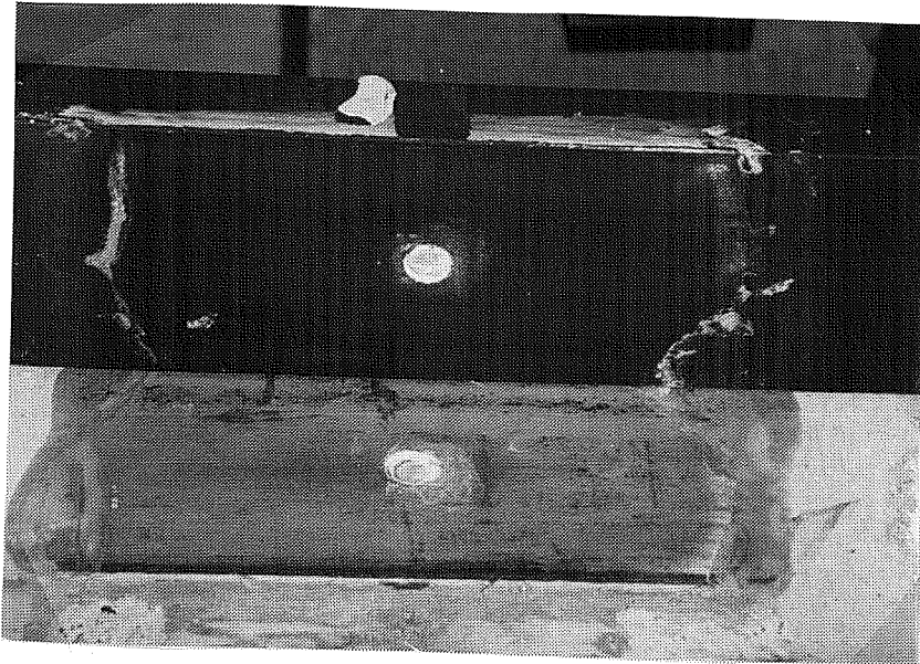
Figure 4.31 Epoxy interface completely debonded from steel section – Test 2-ME3h.
