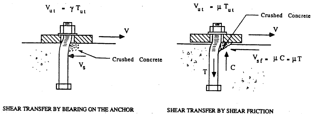
Figure 2.5 Anchor bolt shear transfer mechanisms. 19
