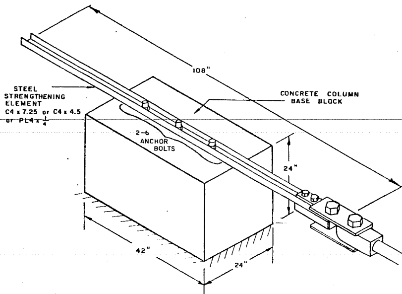
Figure 2.8 Test setup used in previous research on steel-to-concrete connections. 45
