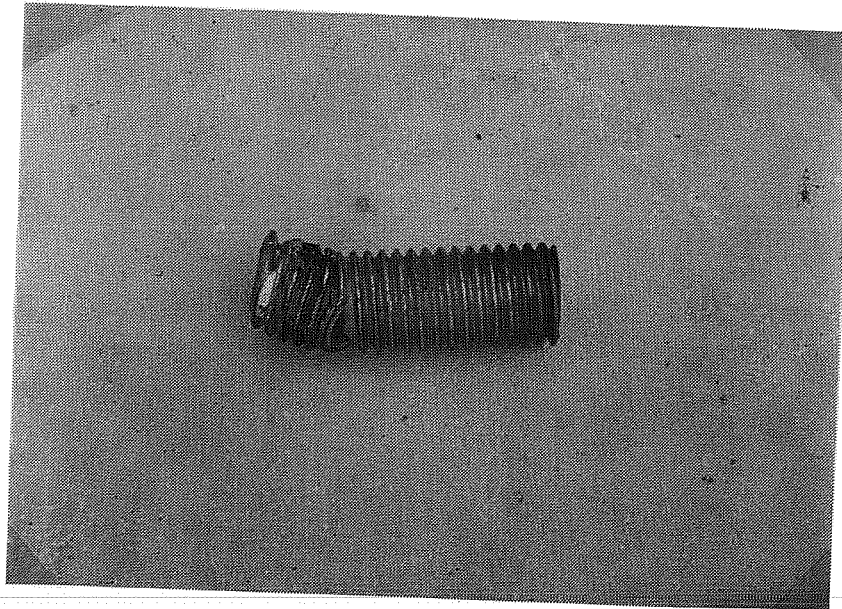
Figure 4.57 Top portion of failed anchor bolt – Test CN3h-WN.
