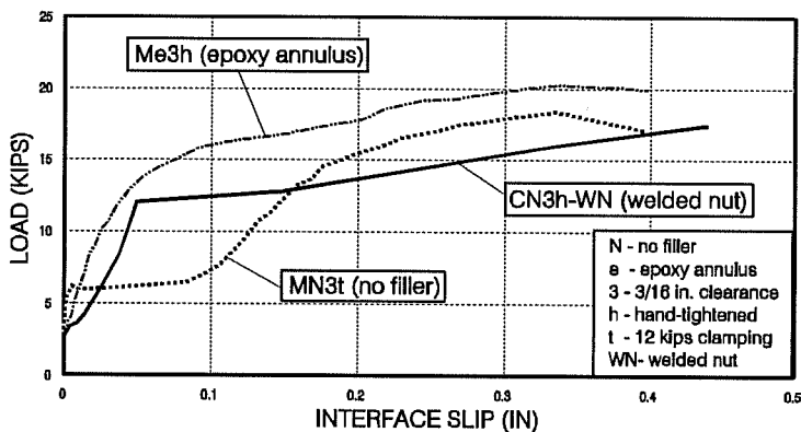
Figure 4.84 Response envelope for welded detail and load-slip plots for epoxy-filled and plain connections.
