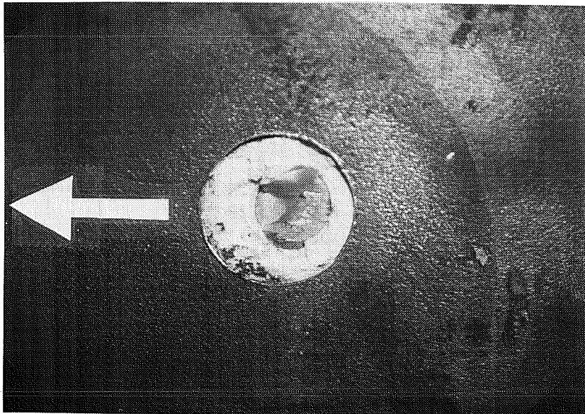
Figure 4.76 Plastic deformation of adhesive in annulus (anchor bolt originally in center) – closeup view.
