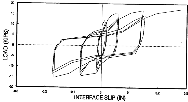
Figure 4.48 Load-slip plot – Test Ce7T-SP.
