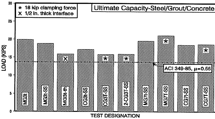
Figure 5.3 Comparison of measured capacities for tests with non-shrink grout and ACI 349-85 shear friction strengths.
