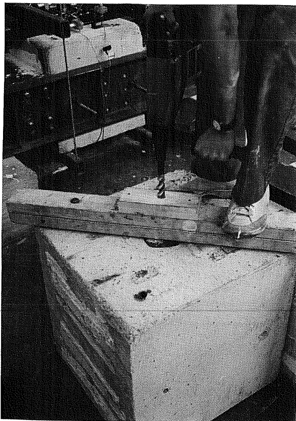
Figure 3.14 Concrete drilling with wooden guide in place.
