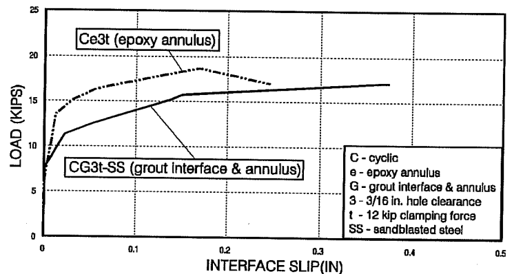
Figure 4.70 Response envelope for test with epoxy-filled annulus and test with non-shrink grout having similar details (3/16 in. hole clearance).
