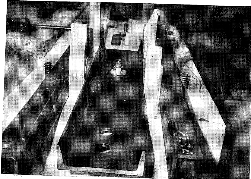
Figure 3.22 Channel held in position with wooden wedges while curing.
