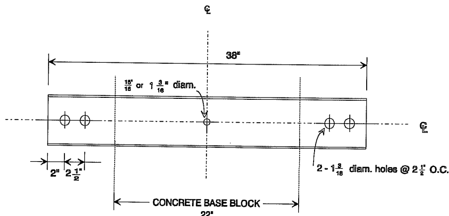
Figure 3.13 Schematic of steel element machining details.
