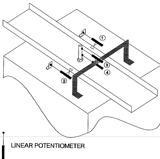
Figure 3.31 Schematic of linear potentiometer layout.
