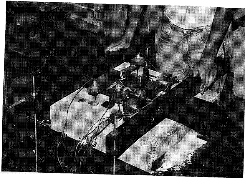
Figure 3.30 Close up view of specimen ready for testing with instrumentation in place.
