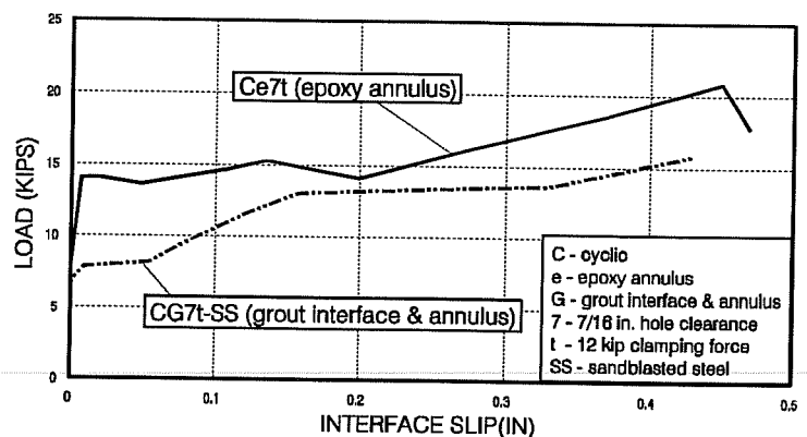
Figure 4.71 Response envelope for test with epoxy-filled annulus and test with non-shrink grout having similar details (7/16 in. hole clearance).
