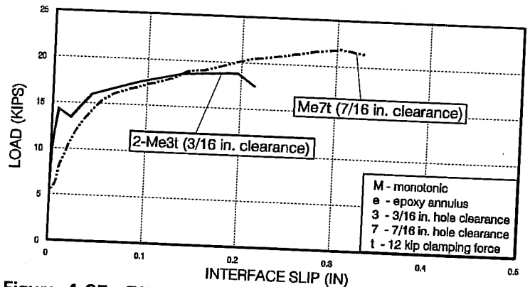
Figure 4.25 Effect of hole clearance (tests with epoxy-filled annulus and 12 kip clamping force).
