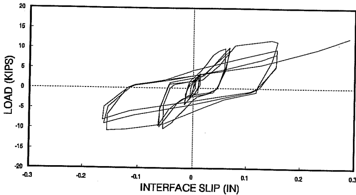
Figure 4.51 Load-slip plot – Test CN3h-WN.
