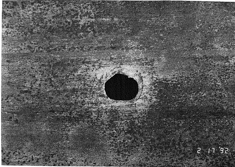
Figure 4.61 Crushing of grout in annulus after removal of loose material – Test CG7T-SS.
