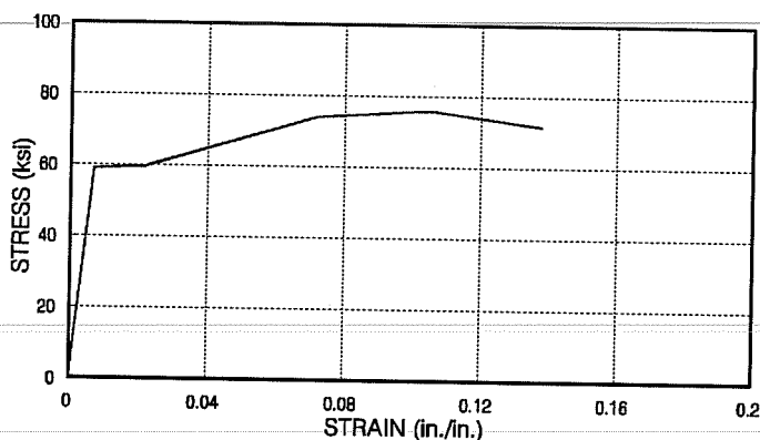
Figure 3.9 Stress-strain curve for threaded rod.
