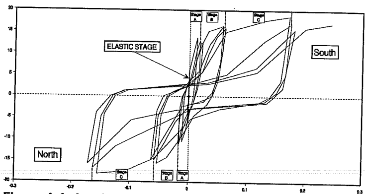
Figure 4.1 Load stages performed in typical cyclic test.
