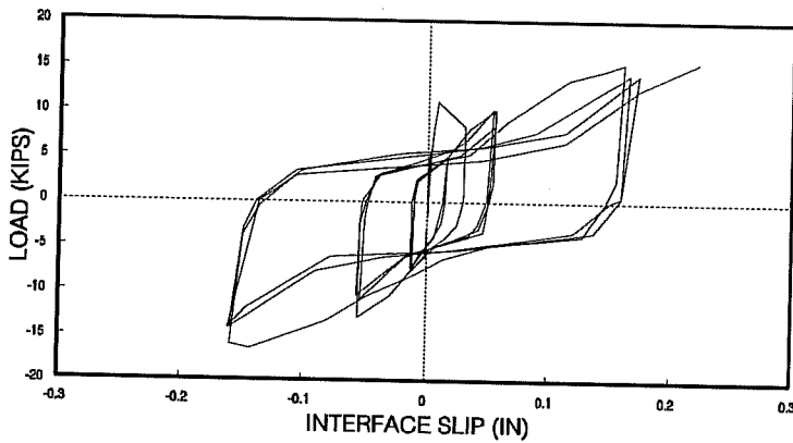
Figure 4.46 Load-slip plot – 2-Test Ce7t-SP.
