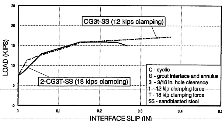
Figure 4.63 Response envelopes for the effect of increased clamping force (tests with non-shrink grout and 3/16 in. hole clearance).
