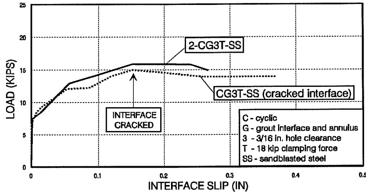
Figure 4.65 Response envelopes for the effect of grout interface cracking.
