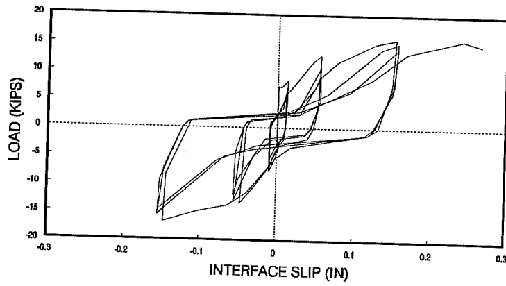
Figure 4.40 Load-slip plot – Test 2-CG3T-SS.
