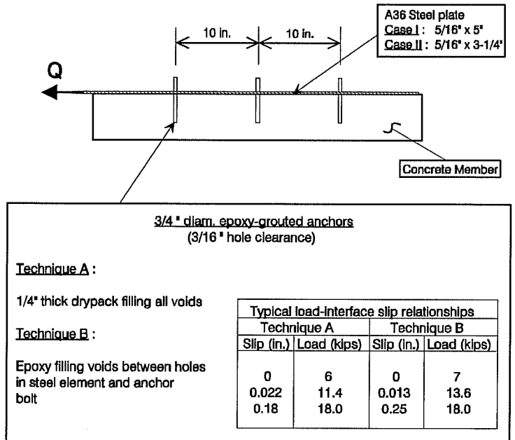
Figure 5.6 Details of sample multiple-anchor steel-to-concrete connection.
