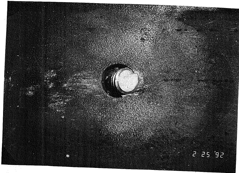
Figure 4.56 Anchor failure by kinking after bending in double curvature – Test CN3h-WN (viewed from bottom of steel section).
