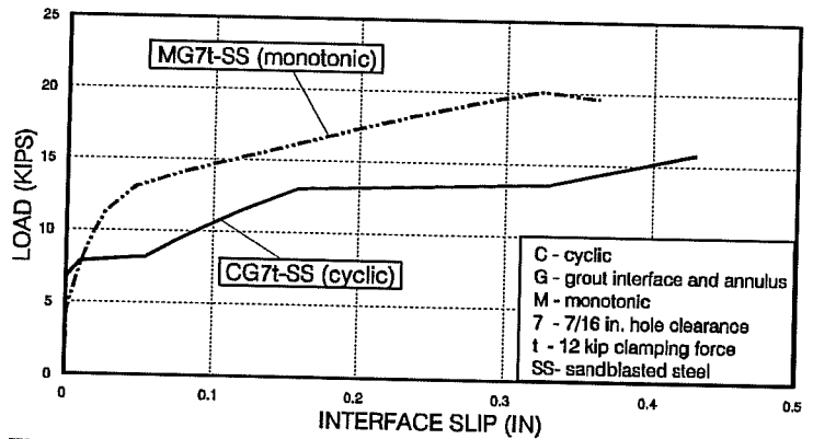
Figure 4.59 Comparison of response envelope & monotonic load-slip plot for the effect of cyclic loading (tests with non-shrink grout & 7/16 in. hole clearance).
