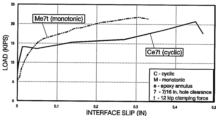
Figure 4.73 Comparison of response envelope & monotonic load-slip plot for the effect of cyclic loading (tests with epoxy-filled annulus & 7/16 in. hole clearance).
