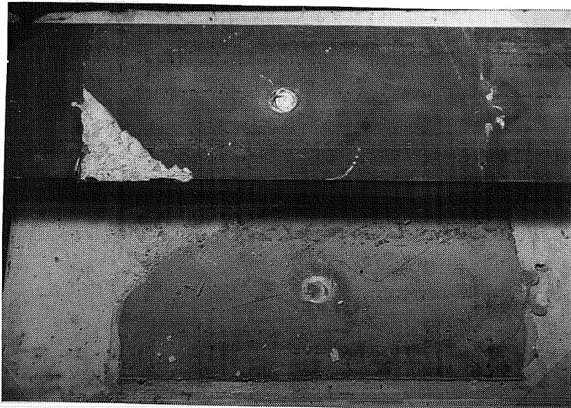
Figure 4.32 Concrete bonded to steel section by epoxy – Test ME3h-SS.
