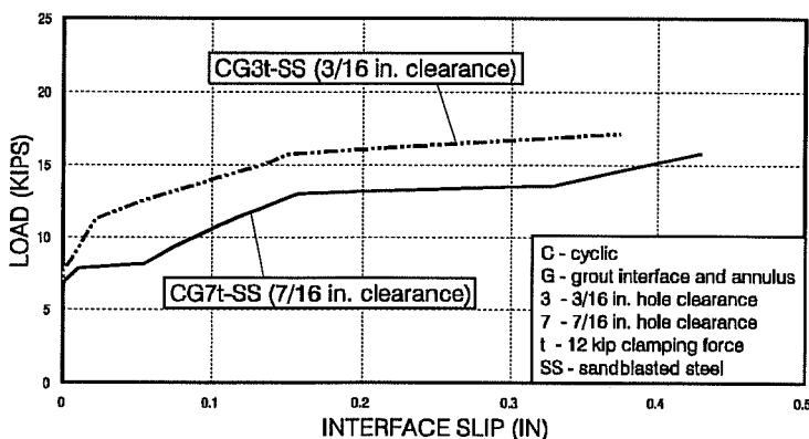
Figure 4.62 Response envelopes for the effect of hole clearance (tests with non-shrink grout and 12 kip clamping force).
