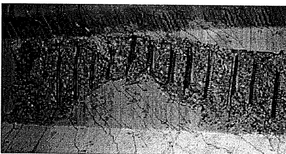
Figure 4.4 Explosive shear-compression failure (Beam NSC-2-N)
