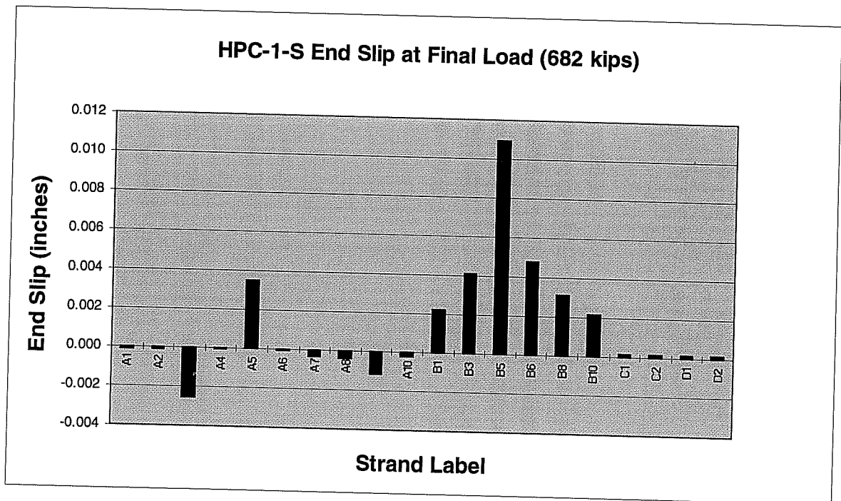
Fig. D-10 End slip of beam end HPC-1-S after development length test
