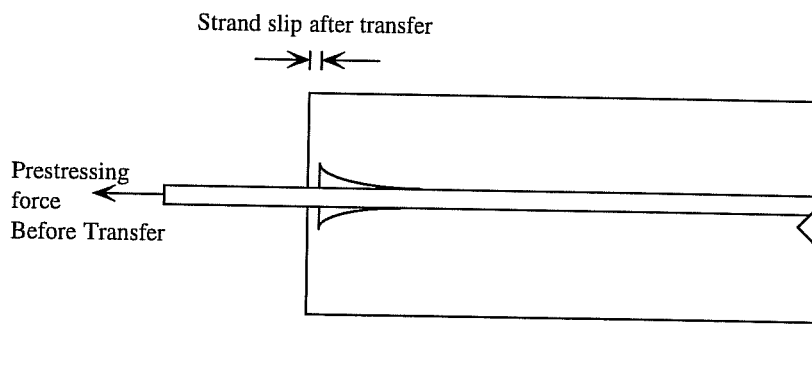
Figure 2.2 Transfer of prestress 8
