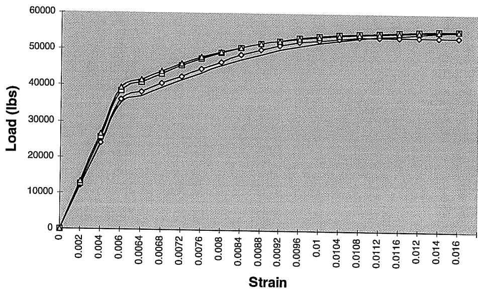
Tensile Test Curves of 0.6 inch-Grade 270 Low Relaxation Strand
