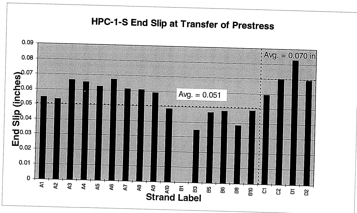
Fig. D-2 End slip of beam end HPC-1-S at transfer
