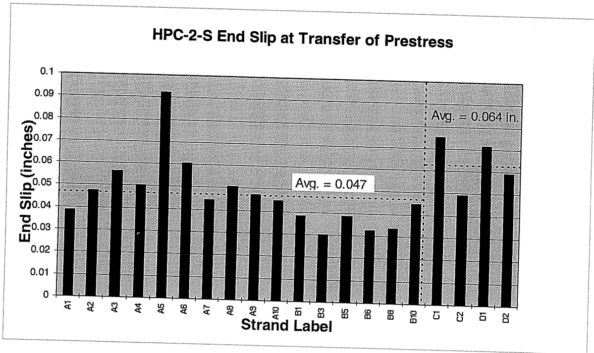
Fig. D-4 End slip of beam end HPC-2-S at transfer
