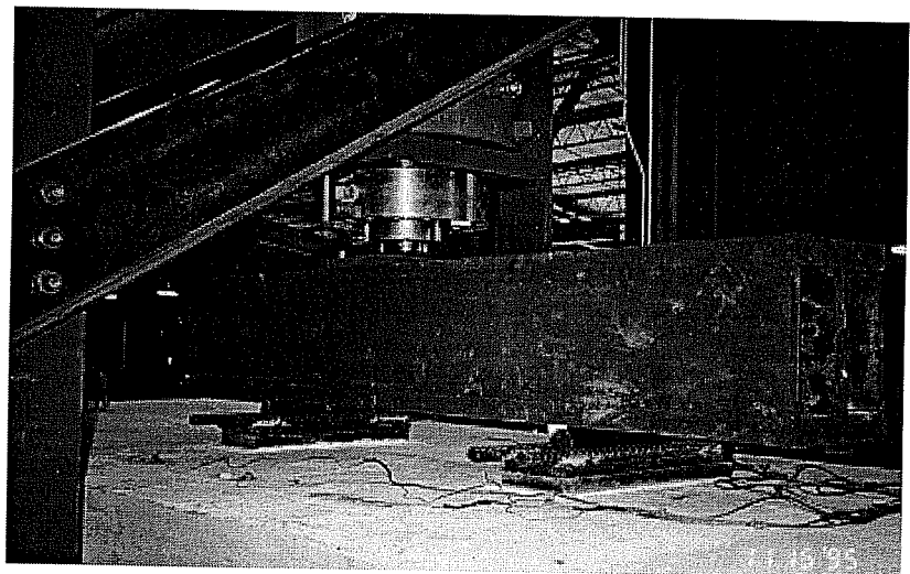
Figure 3.5 Two-point loading system
