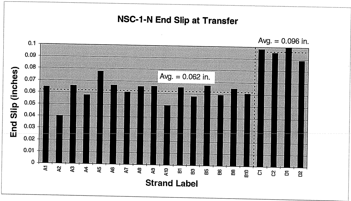
Fig. D-5 End slip of beam end NSC-1-N at transfer
