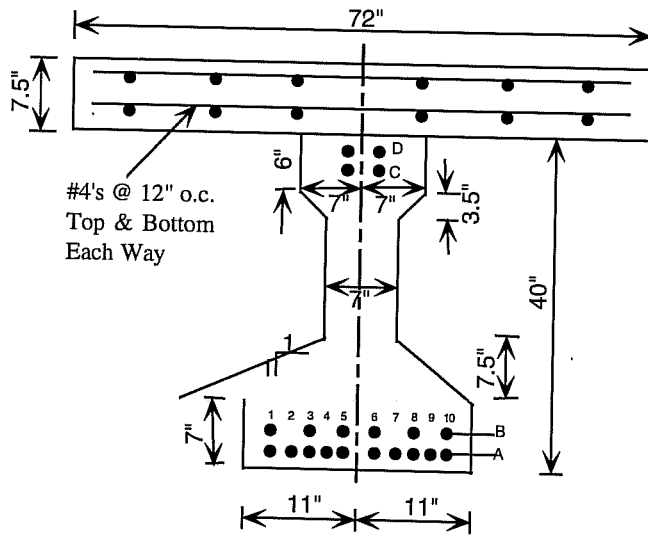
Figure 3.1 Texas Type C girder with composite deck
