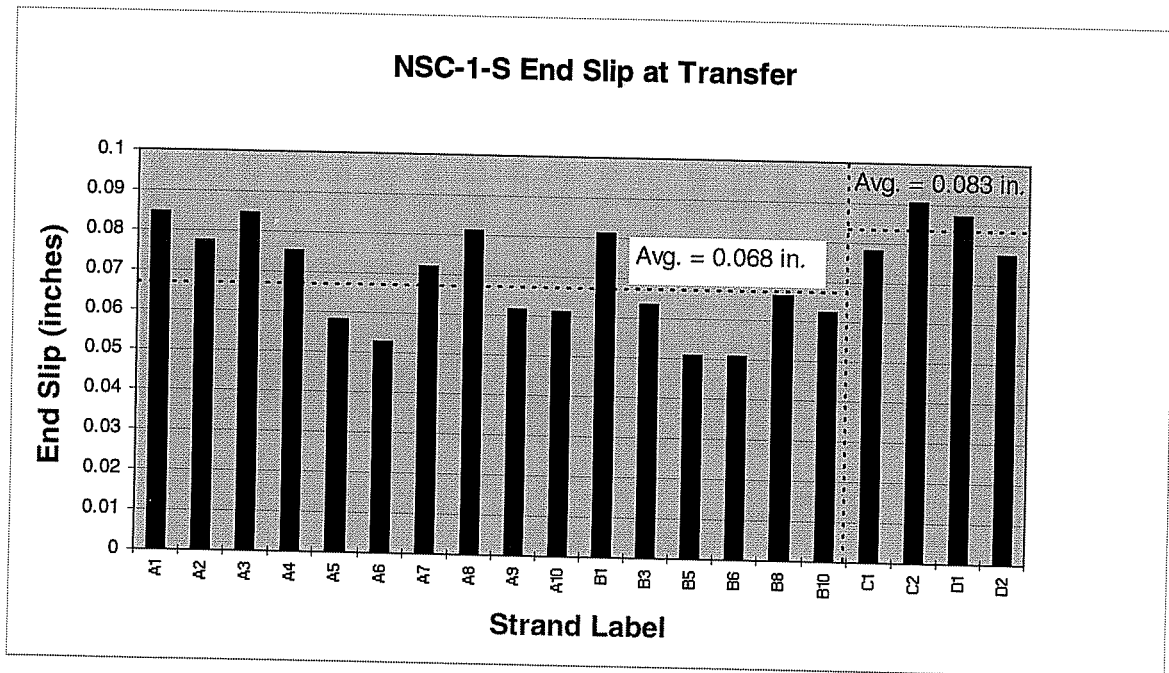
Fig. D-6 End slip of beam end NSC-1-S at transfer
