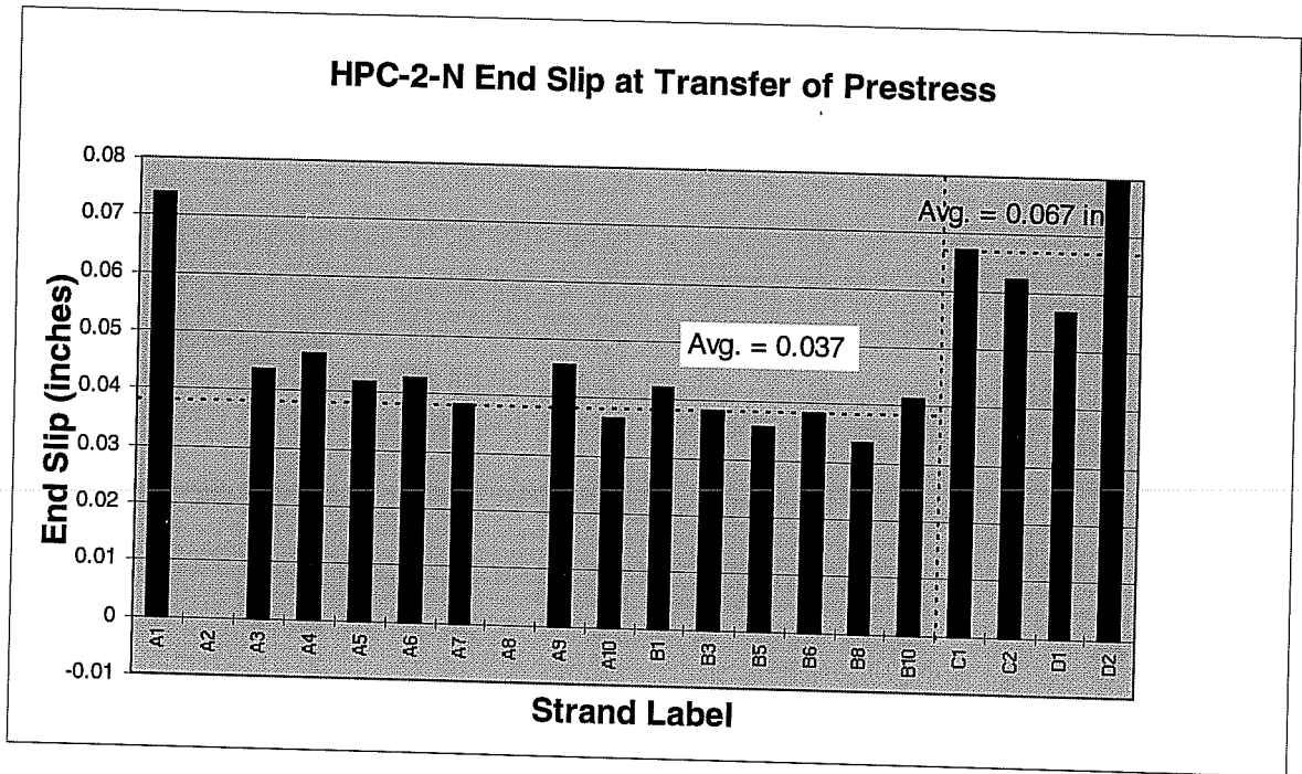
Fig. D-3 End slip of beam end HPC-2-N at transfer
