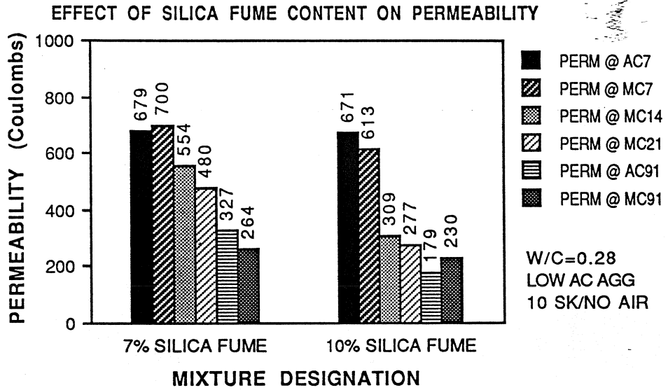
Figure 5.32 Effect of Silica Fume Content on Permeability
