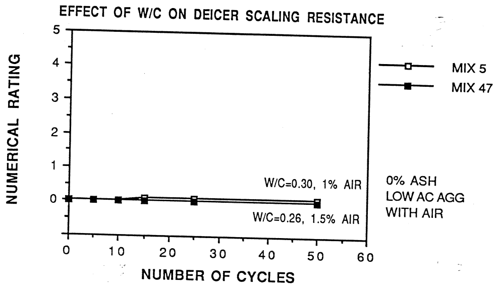
Figure 6.13 Effect of W/C Ratio on Deicer Scaling Resistance
