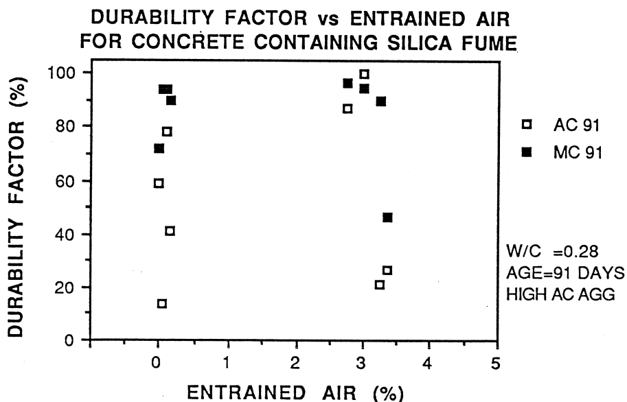
Figure 8.12 Durability Factor vs Entrained Air Content
