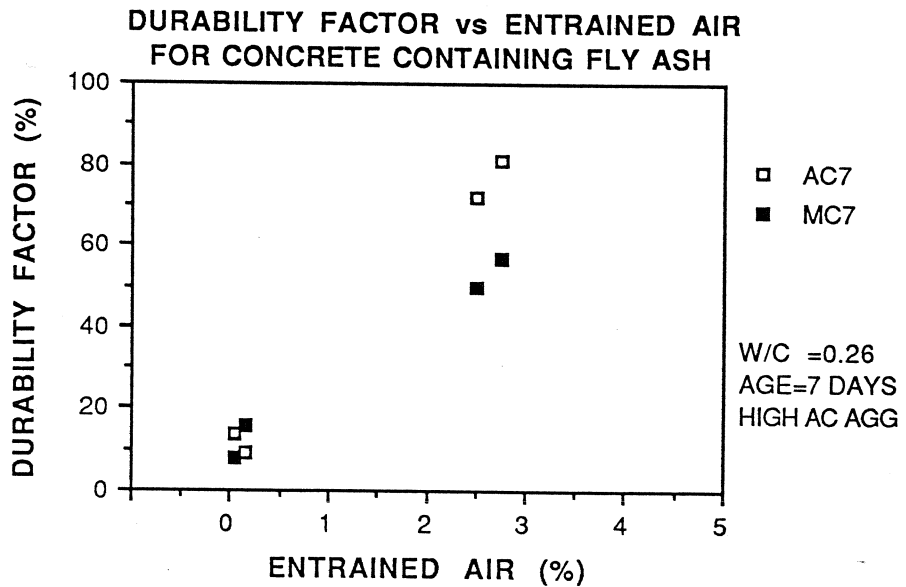
Figure 8.7 Durability Factor vs Entrained Air Content
