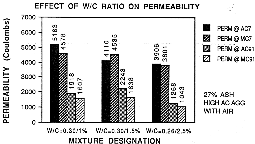
Figure 5.19 Effect of Water/Cement Ratio on Permeability
