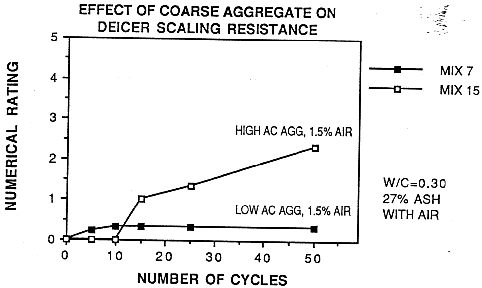
Figure 6.27 Effect of Coarse Aggregate on Scaling Resistance
