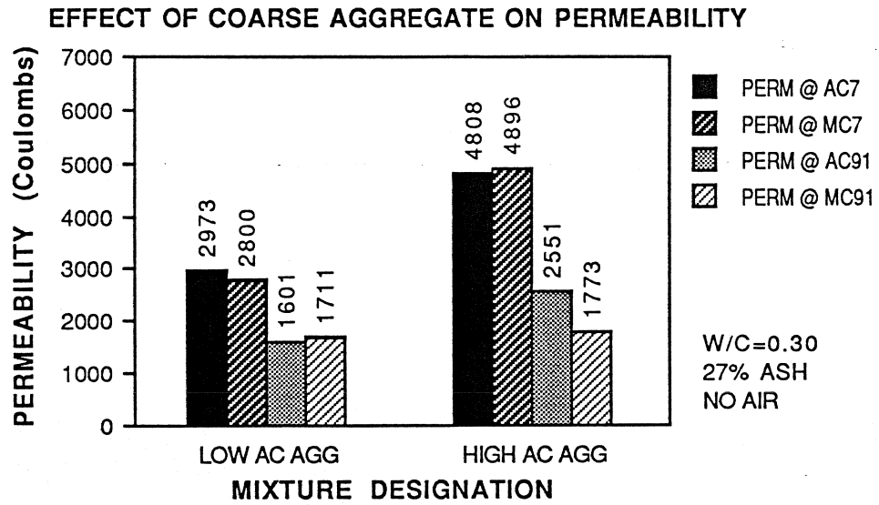
Figure 5.22 Effect of Coarse Aggregate on Permeability
