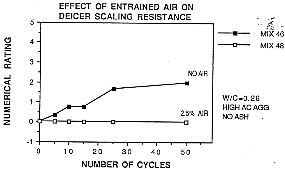
Figure 6.4 Effect of Engrained Air on Deicer Scaling Resistance
