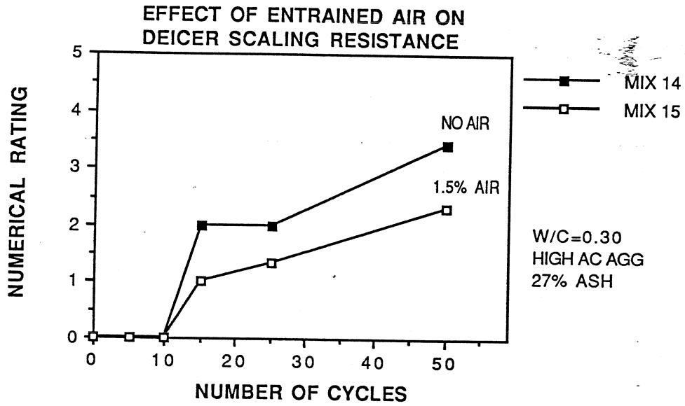
Figure 6.6 Effect of Entrained Air on Deicer Scaling Resistance
