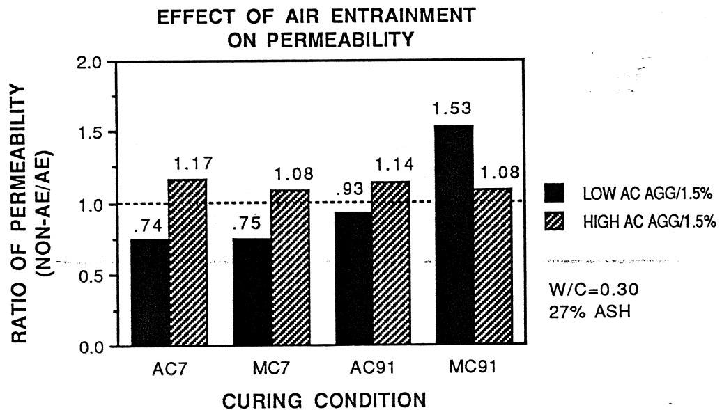
Figure 5.5 Effect of Air Entrainment on Permeability
