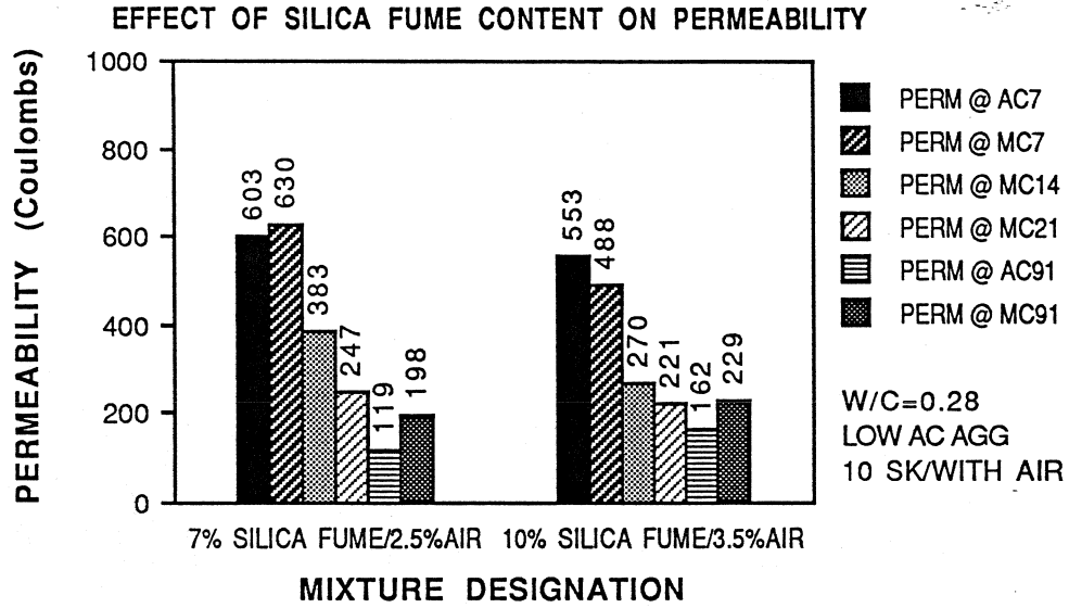
Figure 5.34 Effect of Silica Fume Content on Permeability
