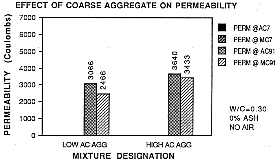
Figure 5.20 Effect of Coarse Aggregate on Permeability
