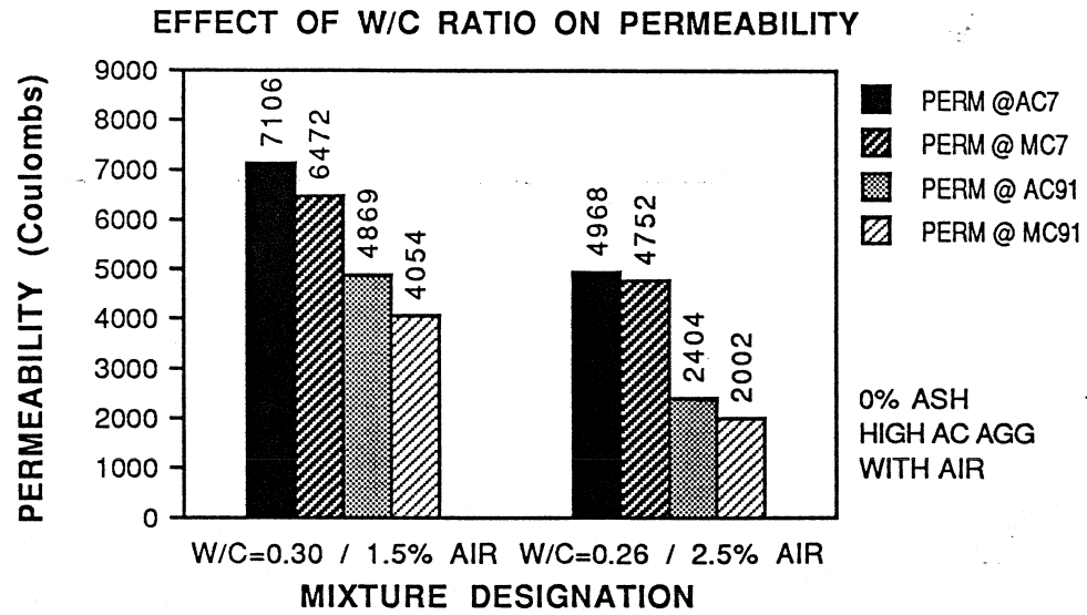
Figure 5.17 Effect of Water/Cement Ratio on Permeability
