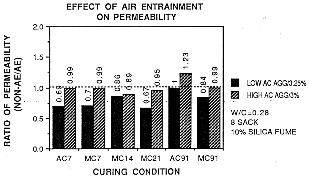
Figure 5.11 Effect of Air Entrainment on Permeability
