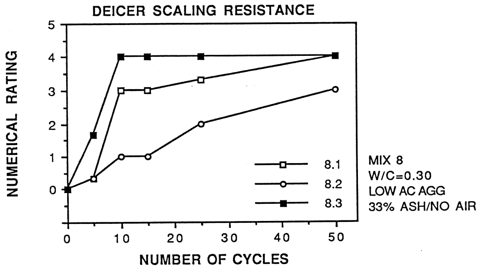
Figure 4.5 Typical Deicer Scaling Plot
