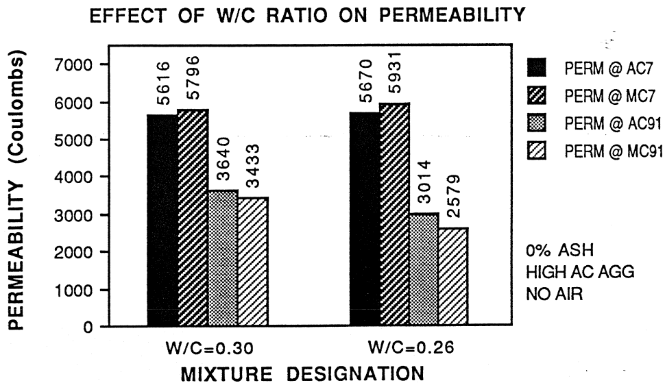
Figure 5.13 Effect of Water/Cement Ratio on Permeability
