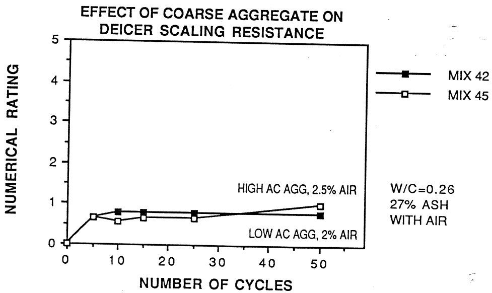
Figure 6.28 Effect of Coarse Aggregate on Scaling Resistance
