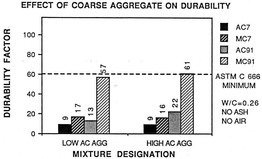
Figure 8.22 Effect of Coarse Aggregate on Durability
