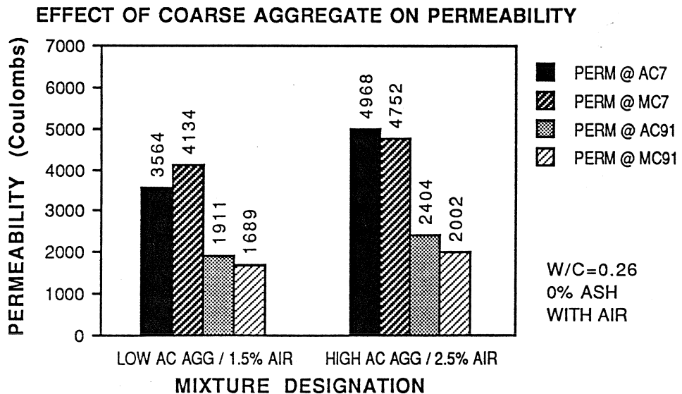
Figure 5.25 Effect of Coarse Aggregate on Permeability
