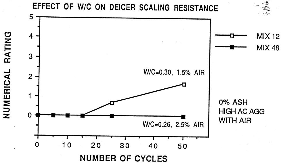
Figure 6.14 Effect of W/C Ratio on Deicer Scaling Resistance
