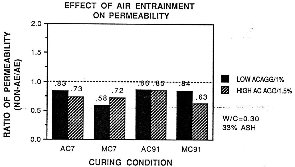
Figure 5.3 Effect of Air Entrainment on Permeability
