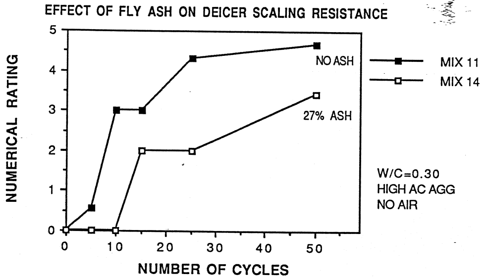
Figure 6.18 Effect of Fly Ash on Deicer Scaling Resistance
