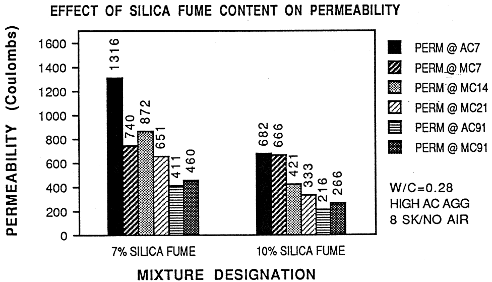
Figure 5.37 Effect of Silica Fume Content on Permeability
