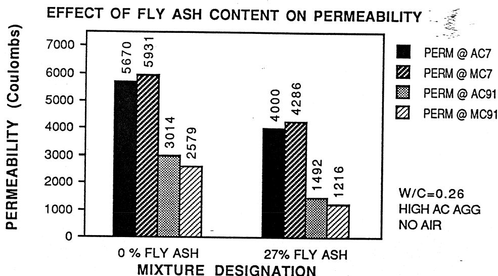
Figure 5.31 Effect of Fly Ash Content on Permeability
