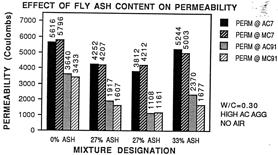
Figure 5.29 Effect of Fly Ash Content on Permeability
