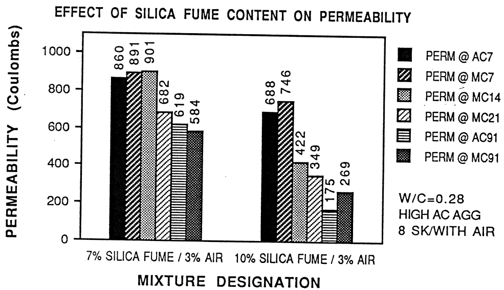
Figure 5.39 Effect of Silica Fume Content on Permeability
