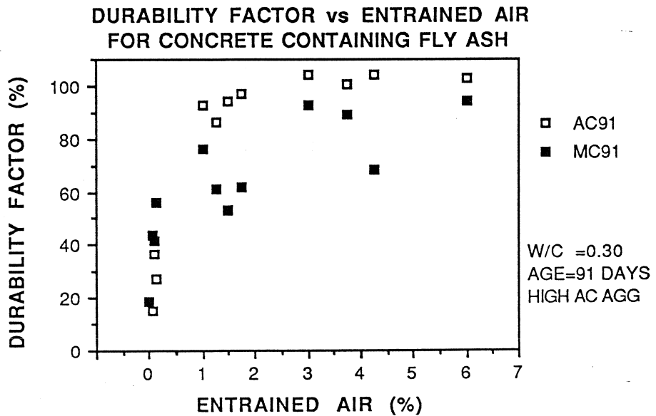
Figure 8.4 Durability Factor vs Entrained Air Content
