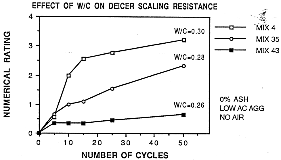
Figure 6.9 Effect of W/C Ratio on Deicer Scaling Resistance.
