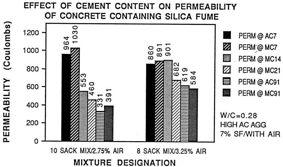
Figure 5.46 Effect of Cement Content on Permeability
