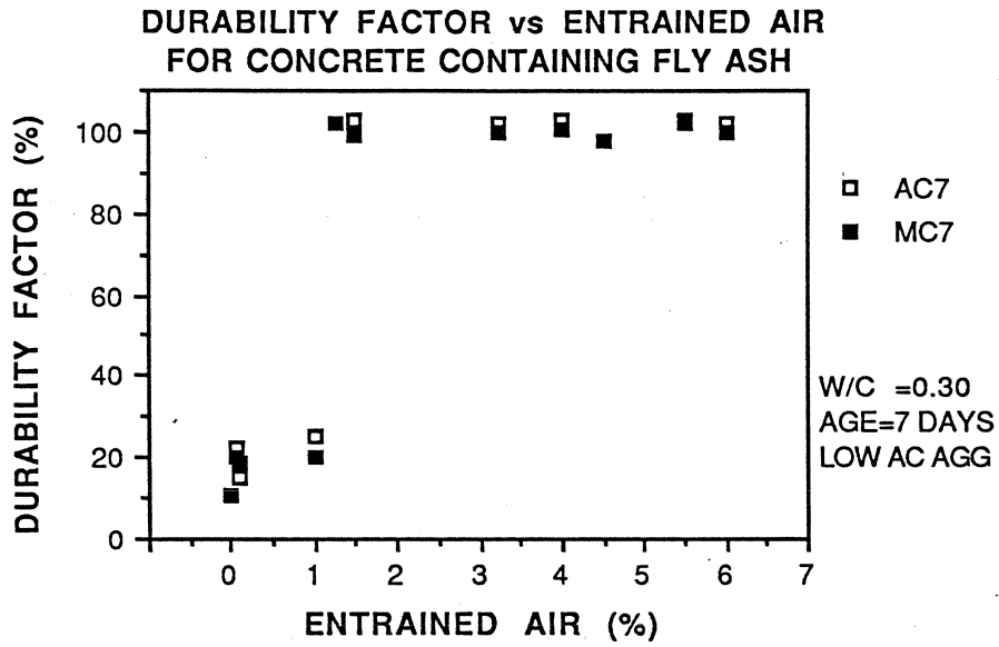
Figure 8.1 Durability Factor vs Entrained Air Content
