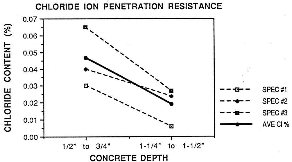
Figure 4.6 Chloride Ion Penetration for a Typical Mix
