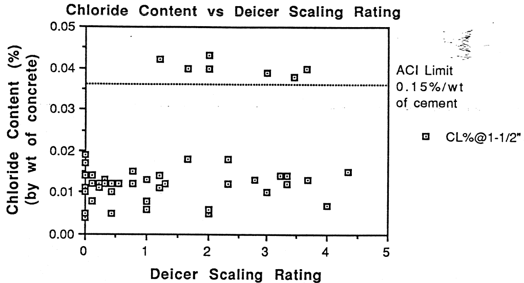
Figure 6.30 Chloride Ion Content vs Deicer Scaling Rating
