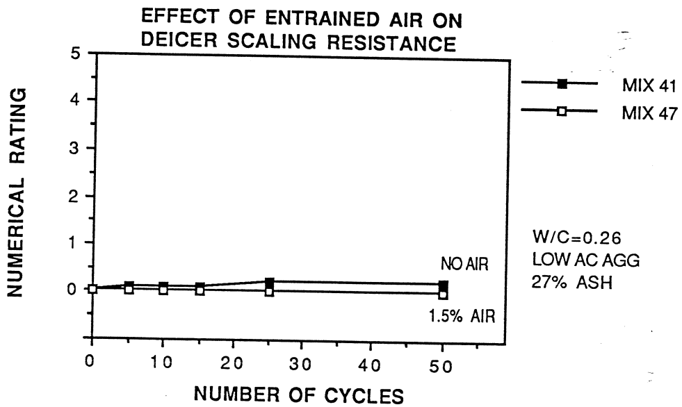
Figure 6.7 Effect of Entrained Air on Deicer Scaling Resistance
