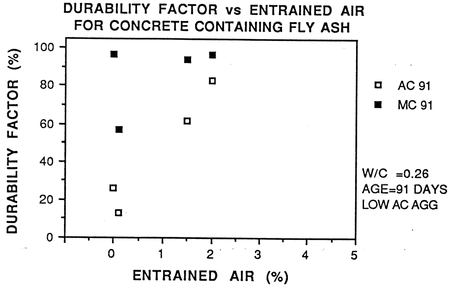
Figure 8.6 Durability Factor vs Entrained Air Content
