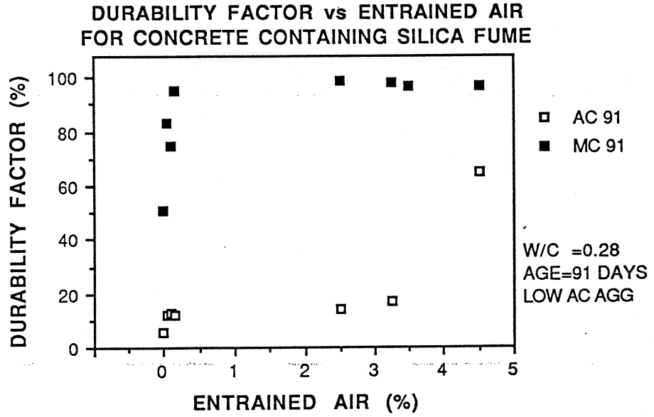
Figure 8.10 Durability Factor vs Entrained Air Content
