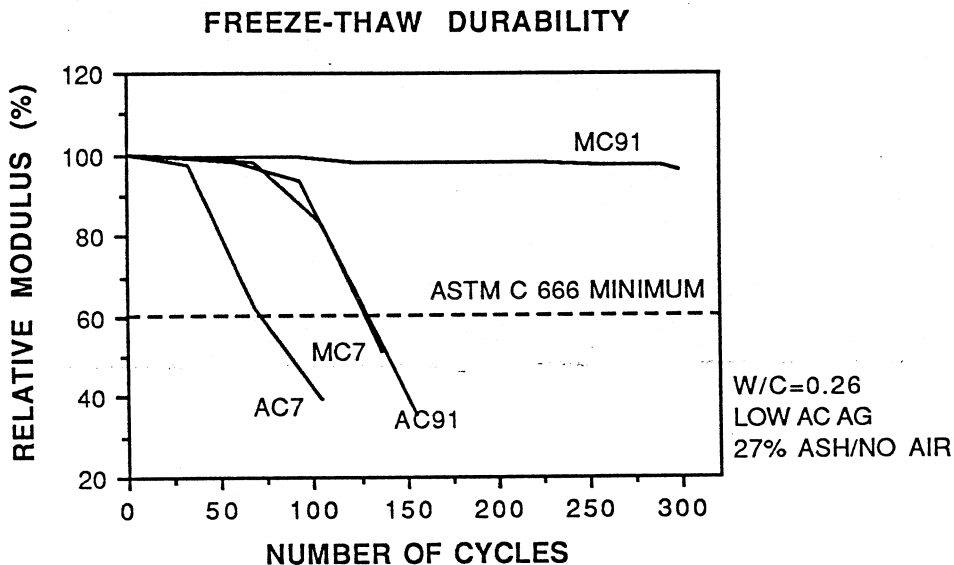
Figure 4.2 Plot of Relative Dynamic Modulus vs. Number of Freeze-Thaw Cycles
