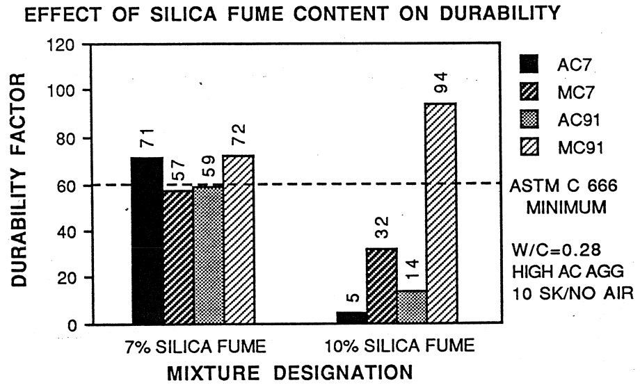
Figure 8.34 Effect of Silica Fume Content on Durability.
