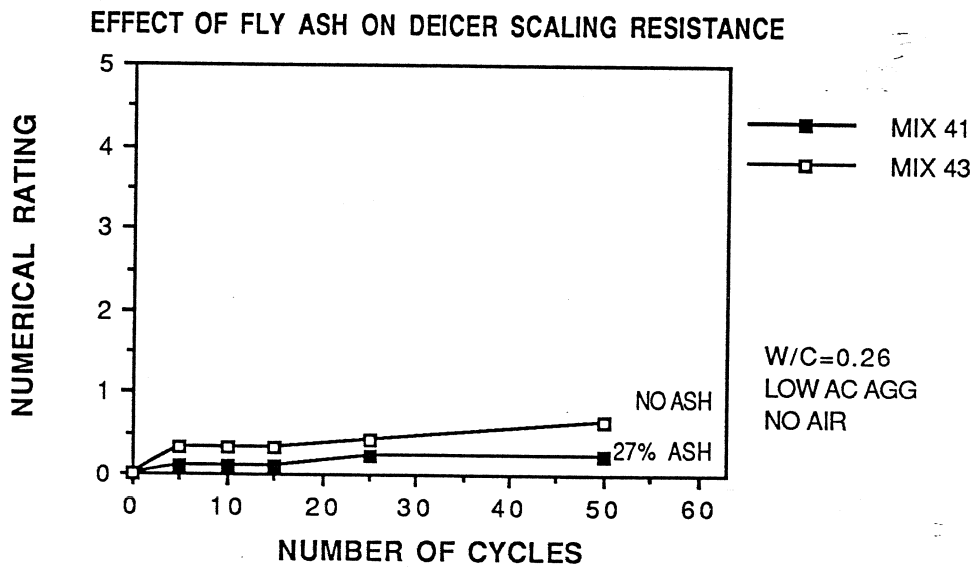
Figure 6.19 Effect of Fly Ash on Deicer Scaling Resistance
