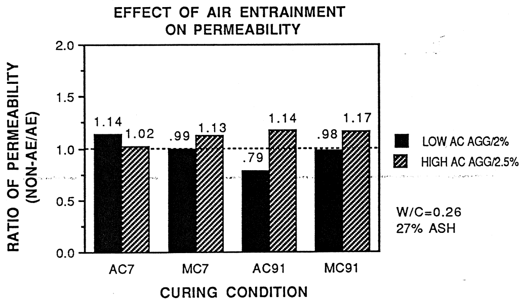
Figure 5.7 Effect of Air Entrainment on Permeability
