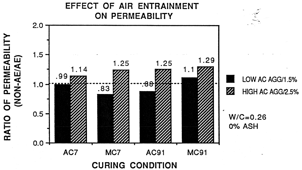
Figure 5.6 Effect of Air Entrainment on Permeability
