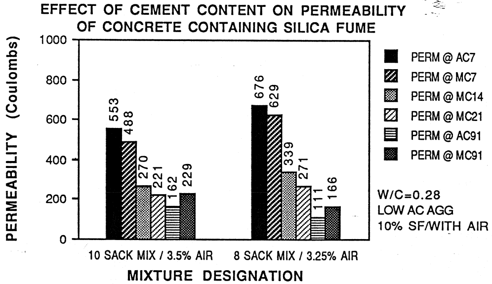
Figure 5.45 Effect of Cement Content on Permeability
