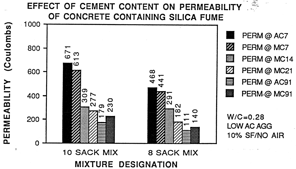
Figure 5.41 Effect of Cement Content on Permeability
