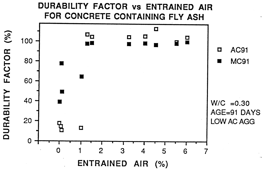
Figure 8.2 Durability Factor vs Entrained Air Content
