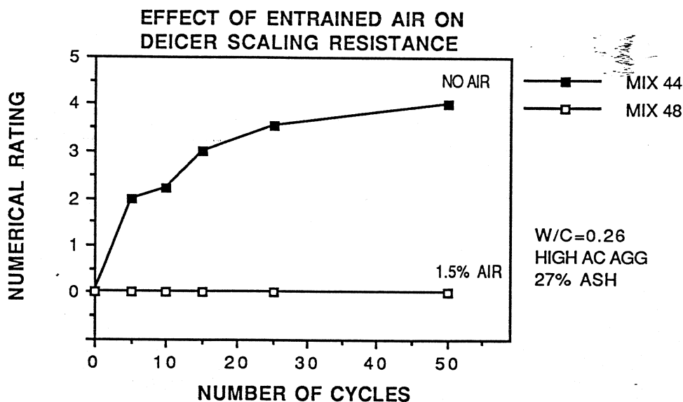
Figure 6.8 Effect of Entrained Air on Deicer Scaling Resistance
