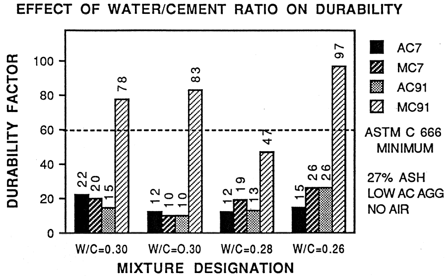
Figure 8.15 Effect of Water/Cement Ratio on Durability
