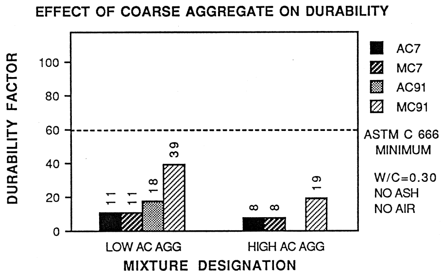
Figure 8.21 Effect of Coarse Aggregate on Durability
