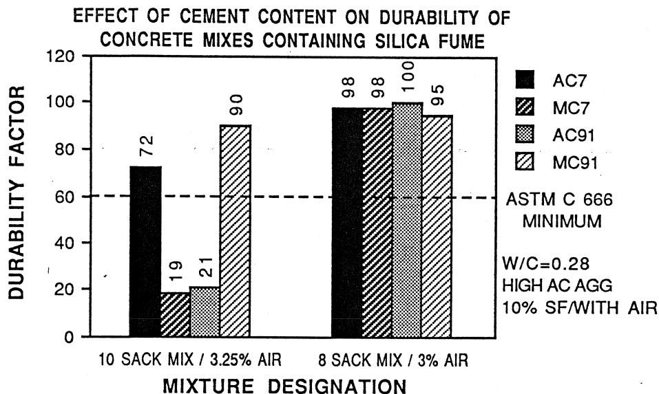
Figure 8.48 Effect of Cement Content on Durability
