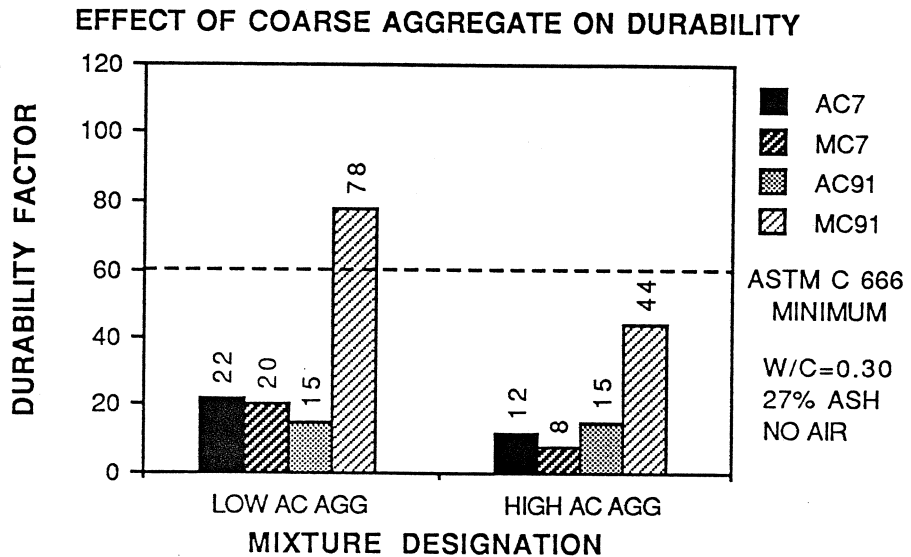
Figure 8.23 Effect of Coarse Aggregate on Durability
