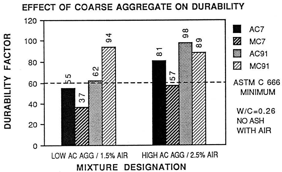
Figure 8.26 Effect of Coarse Aggregate on Durability
