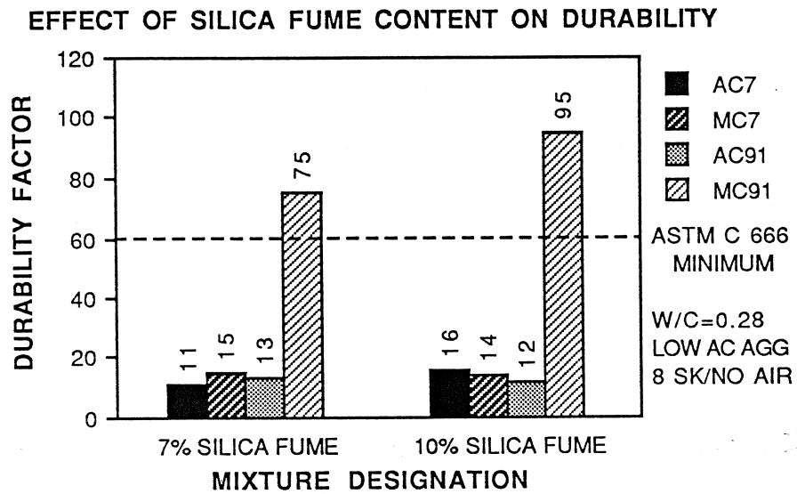
Figure 8.37 Effect of Silica Fume Content on Durability
