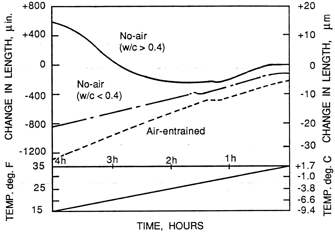
Figure 3.2 Typical Results from Critical Dilation Tests According to ASTM C 671 from Khalil 27 .
