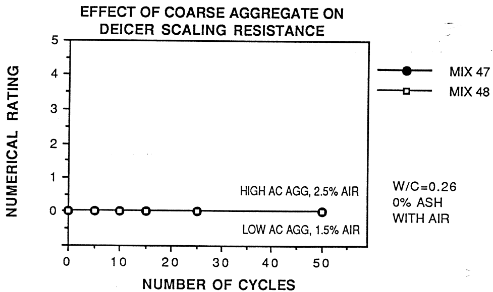
Figure 6.26 Effect of Coarse Aggregate on Scaling Resistance
