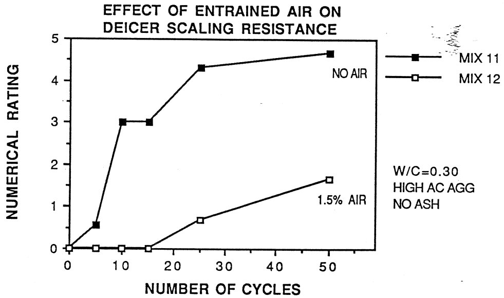
Figure 6.2 Effect of Engrained Air on Deicer Scaling Resistance
