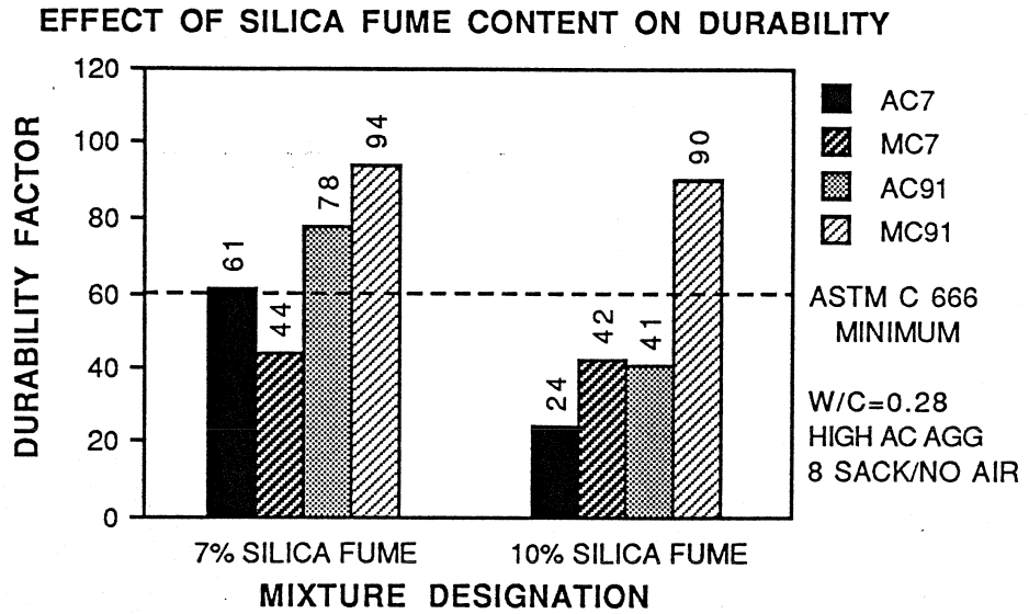
Figure 8.38 Effect of Silica Fume Content on Durability
