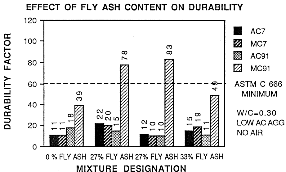
Figure 8.29 Effect of Fly Ash Content on Durability
