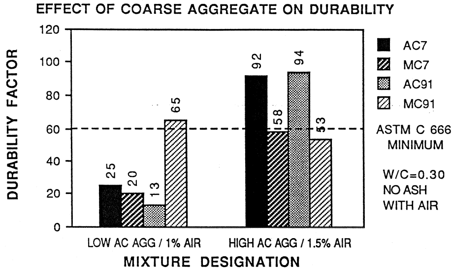
Figure 8.25 Effect of Coarse Aggregate on Durability
