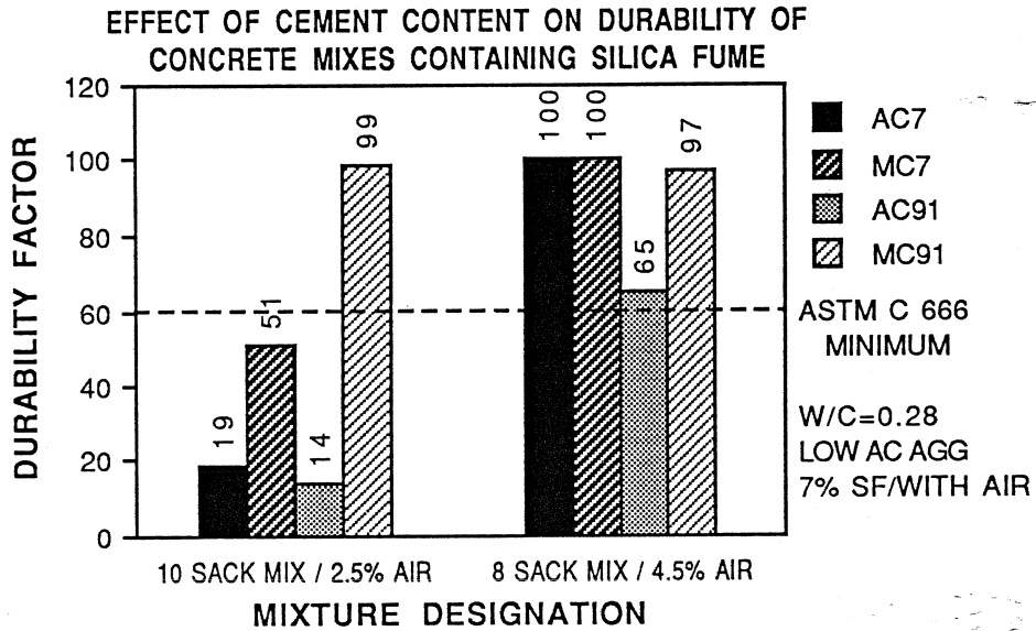
Figure 8.45 Effect of Cement Content on Durability
