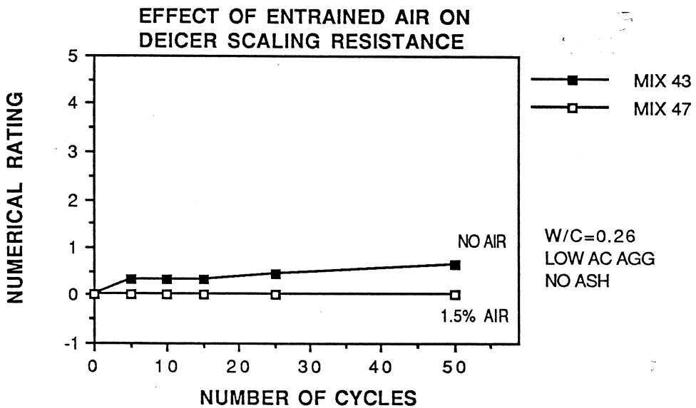
Figure 6.3 Effect of Engrained Air on Deicer Scaling Resistance
