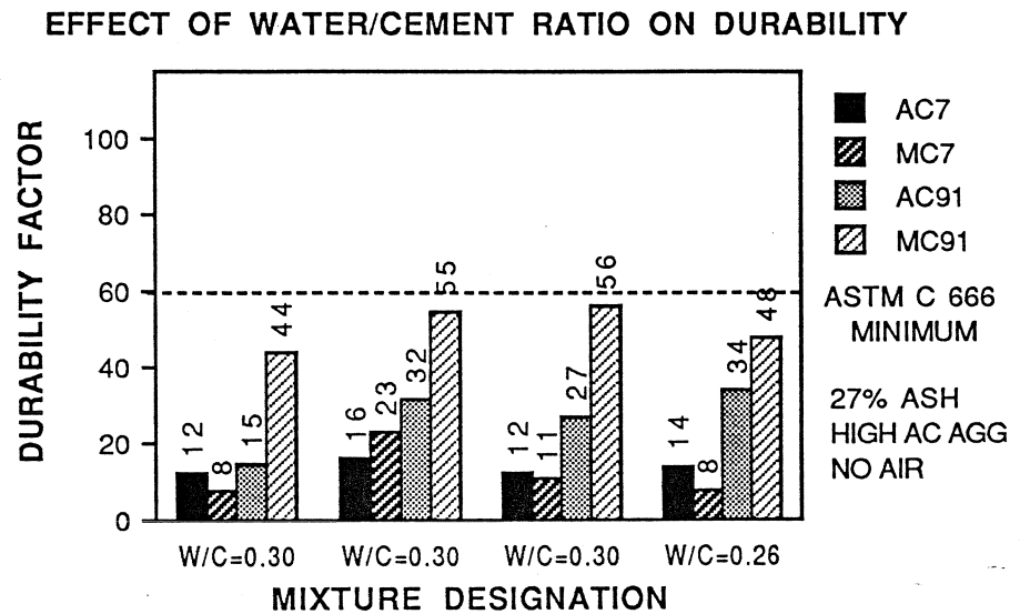
Figure 8.16 Effect of Water/Cement Ratio on Durability
