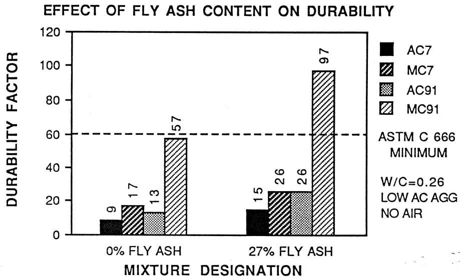
Figure 8.31 Effect of Fly Ash Content on Durability
