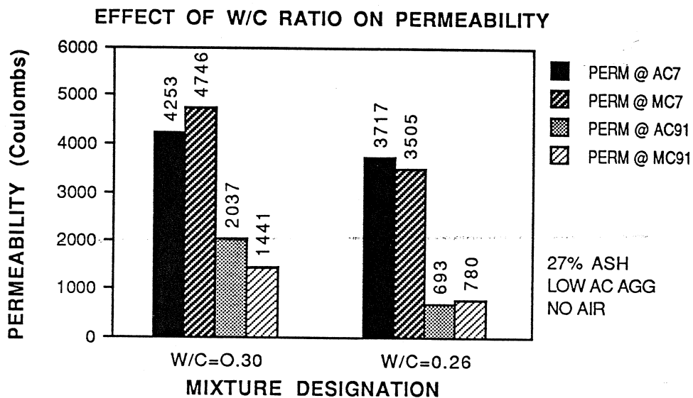
Figure 5.14 Effect of Water/Cement Ratio on Permeability
