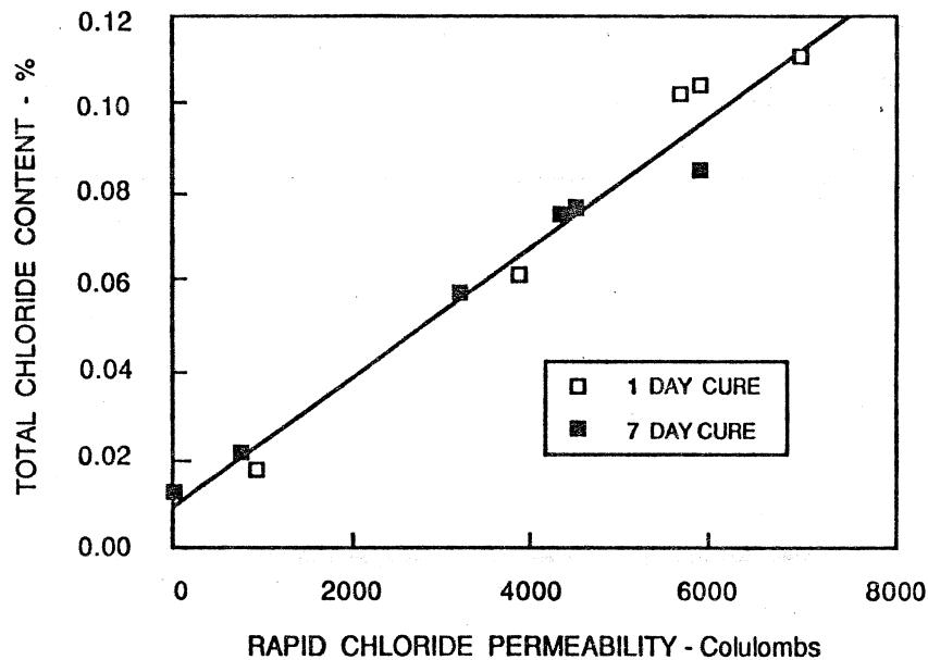
Figure 3.5 Relationship Between Results of Rapid Chloride in Permeability and 90-Day Chloride Ponding Tests from Whiting.
