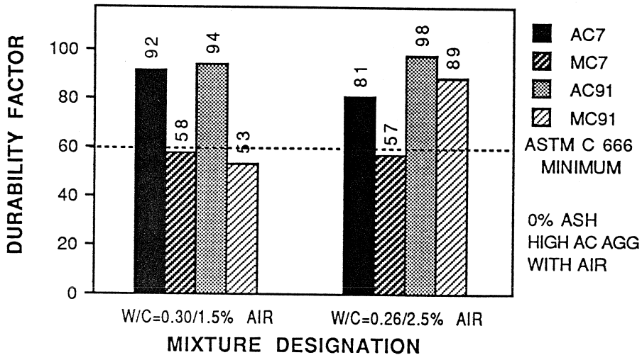
Figure 8.18 Effect of Water/Cement Ratio on Durability
