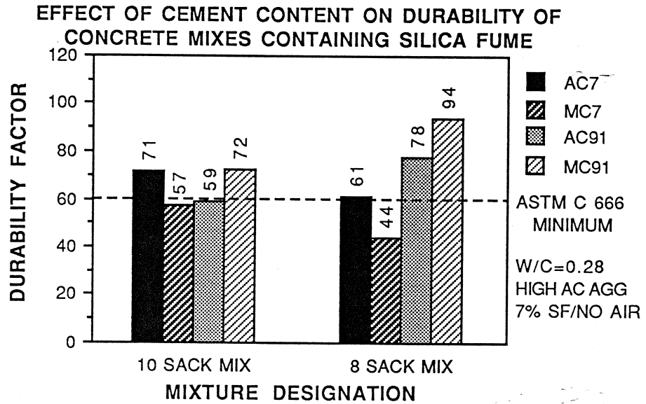
Figure 8.43 Effect of Cement Content on Durability
