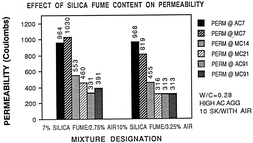
Figure 5.35 Effect of Silica Fume Content on Permeability
