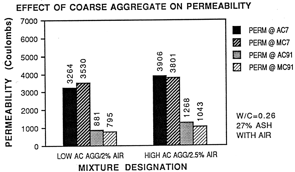
Figure 5.27 Effect of Coarse Aggregate on Permeability
