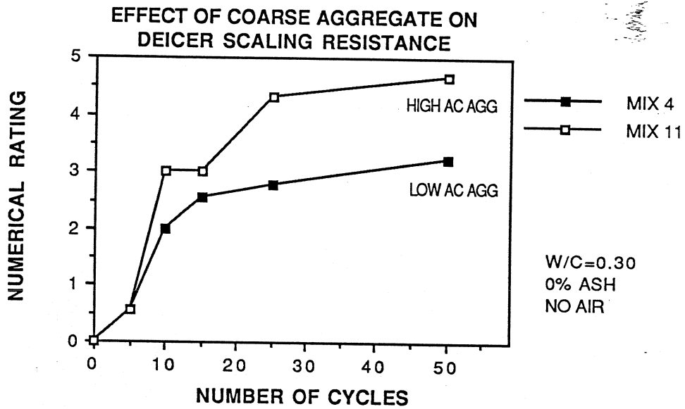
Figure 6.21 Effect of Coarse Aggregate on Scaling Resistance
