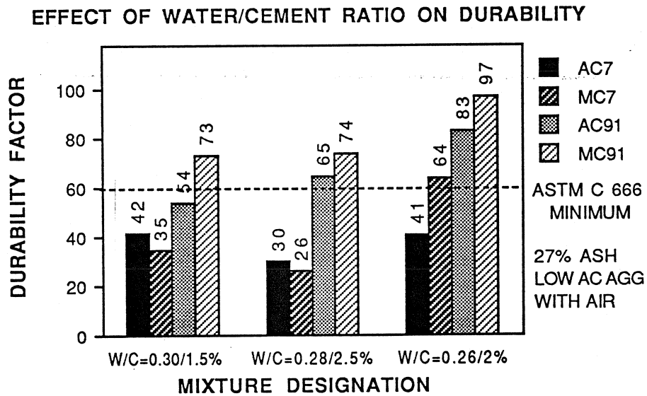
Figure 8.19 Effect of Water/Cement Ratio on Durability
