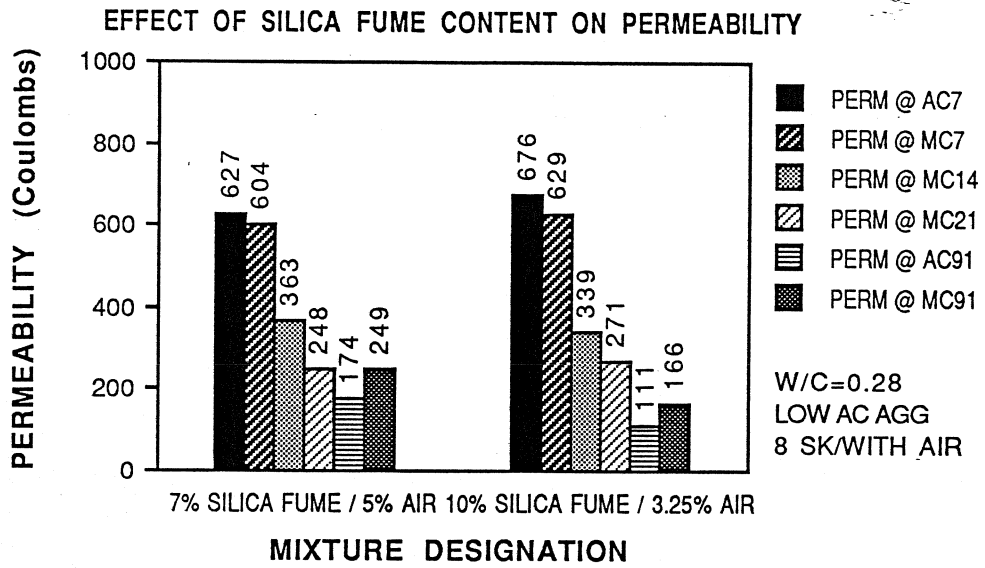
Figure 5.38 Effect of Silica Fume Content on Permeability
