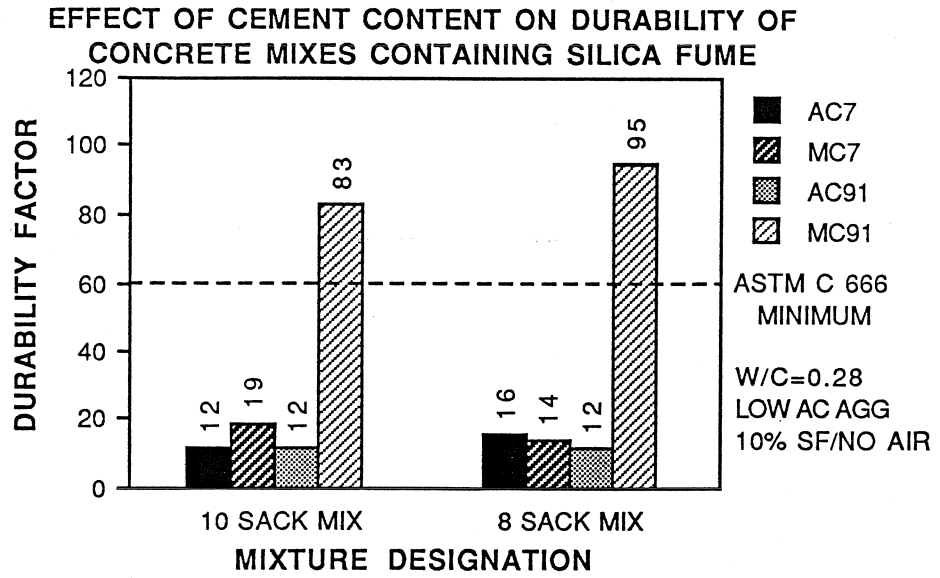
Figure 8.42 Effect of Cement Content on Durability
