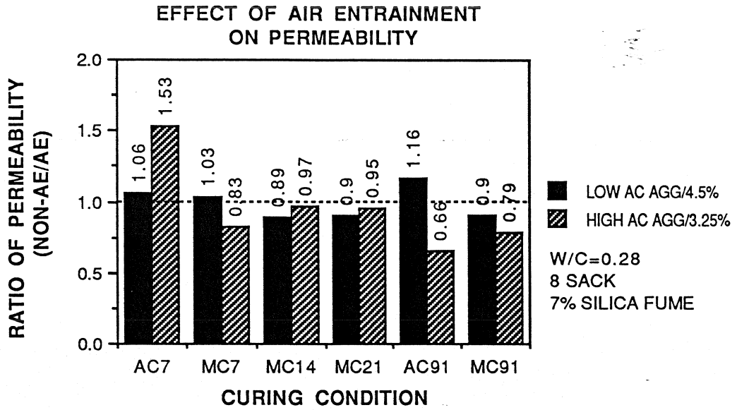
Figure 5.10 Effect of Air Entrainment on Permeability
