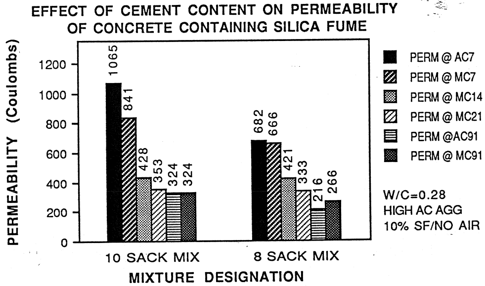
Figure 5.43 Effect of Cement Content on Permeability
