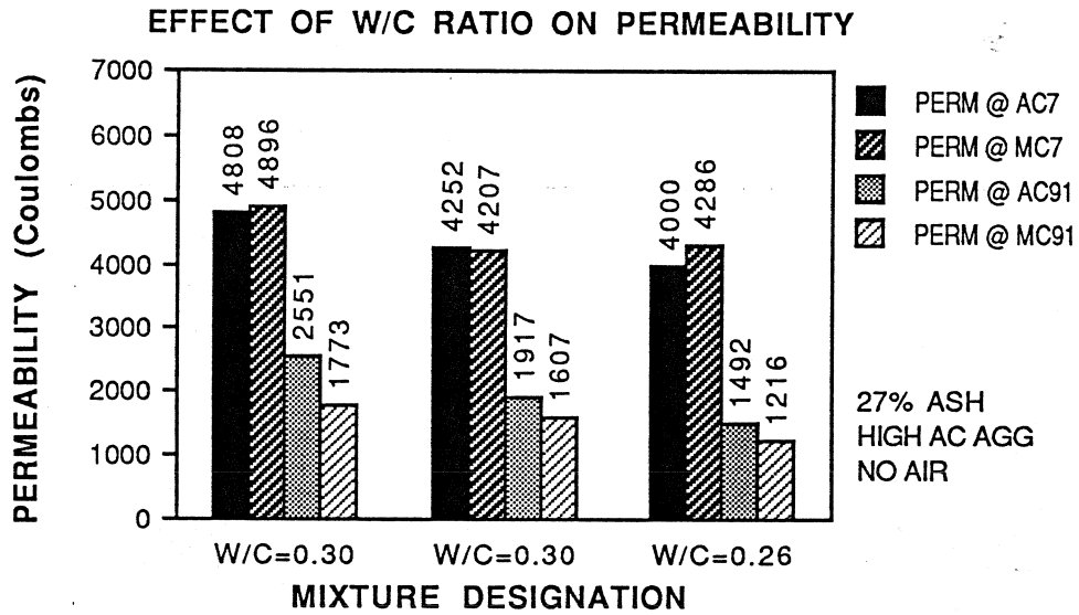
Figure 5.15 Effect of Water/Cement Ratio on Permeability
