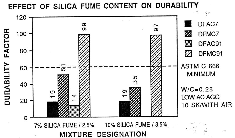
Figure 8.35 Effect of Silica Fume Content on Durability
