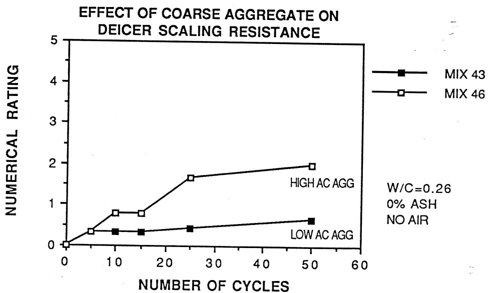
Figure 6.22 Effect of Coarse Aggregate on Scaling Resistance
