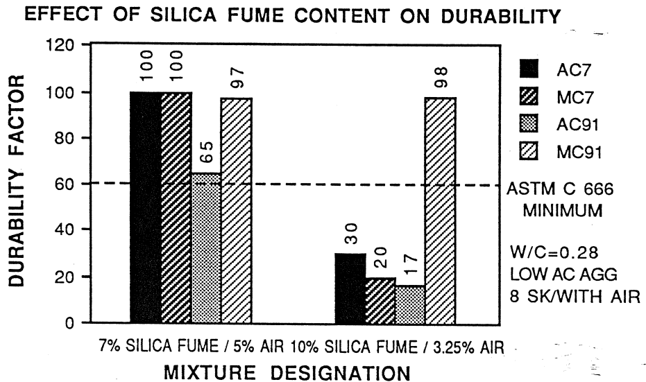
Figure 8.39 Effect of Silica Fume Content on Durability
