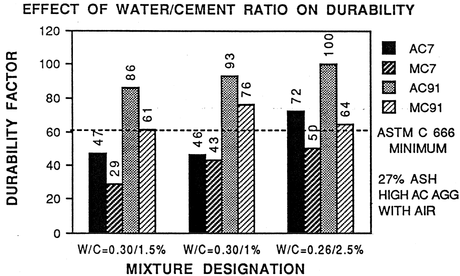
Figure 8.20 Effect of Water/Cement Ratio on Durability
