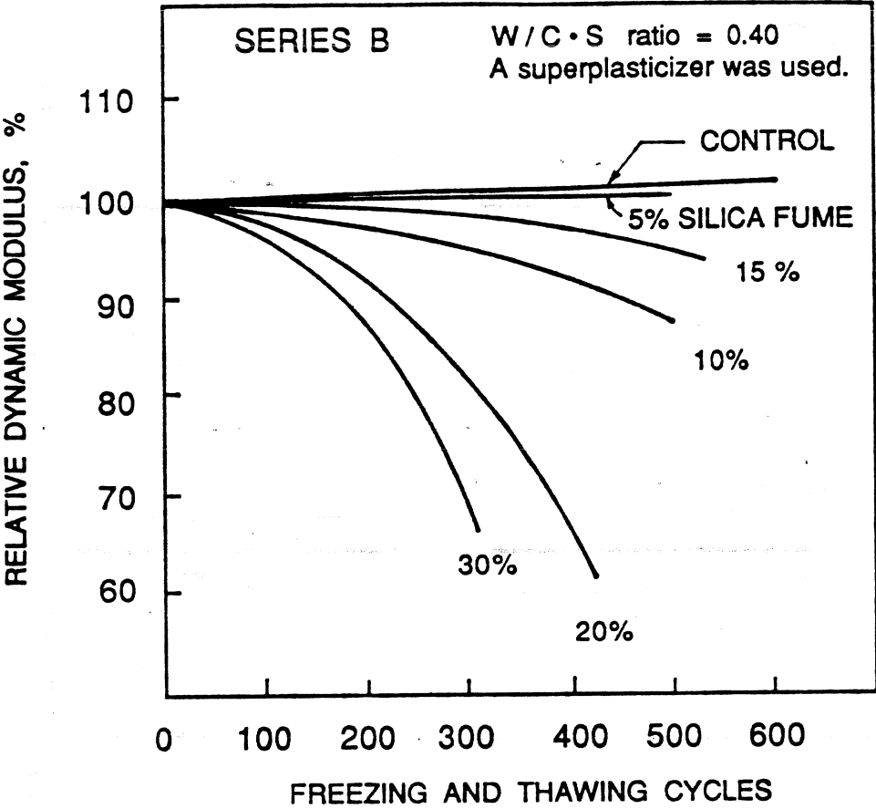
Figure 3.1 Durability Factors vs. Freeze-thaw Cycles for Silica Fume Concrete Mixtures from Malhotra 14 .
