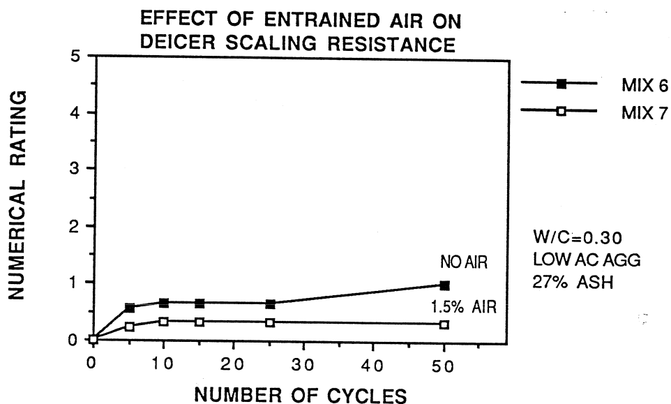
Figure 6.5 Effect of Entrained Air on Deicer Scaling Resistance
