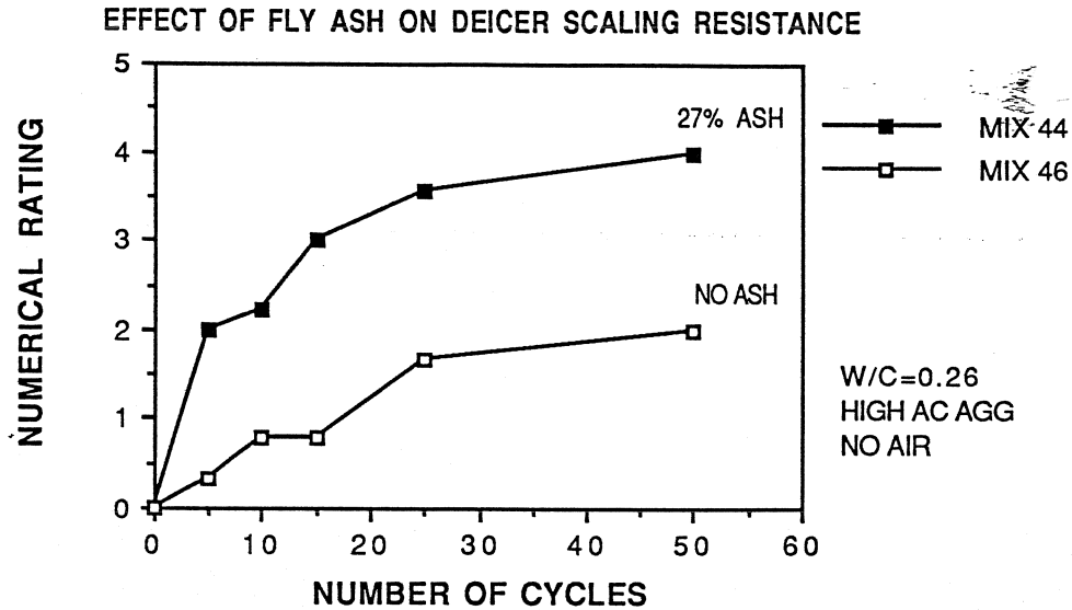
Figure 6.20 Effect of Fly Ash on Deicer Scaling Resistance
