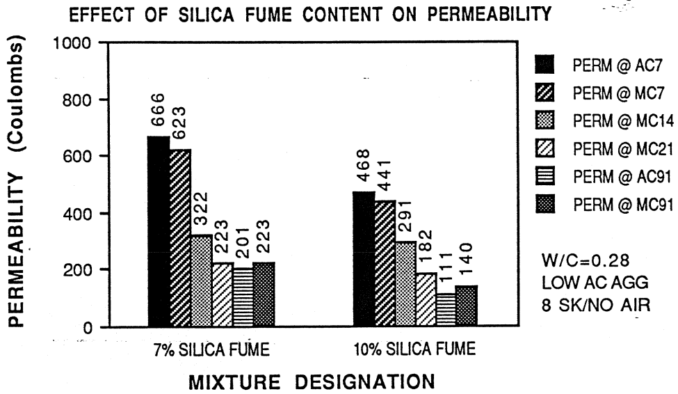
Figure 5.36 Effect of Silica Fume Content on Permeability
