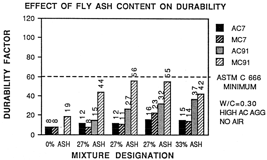
Figure 8.30 Effect of Fly Ash Content on Durability
