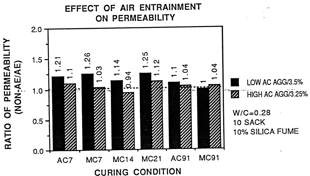
Figure 5.9 Effect of Air Entrainment on Permeability
