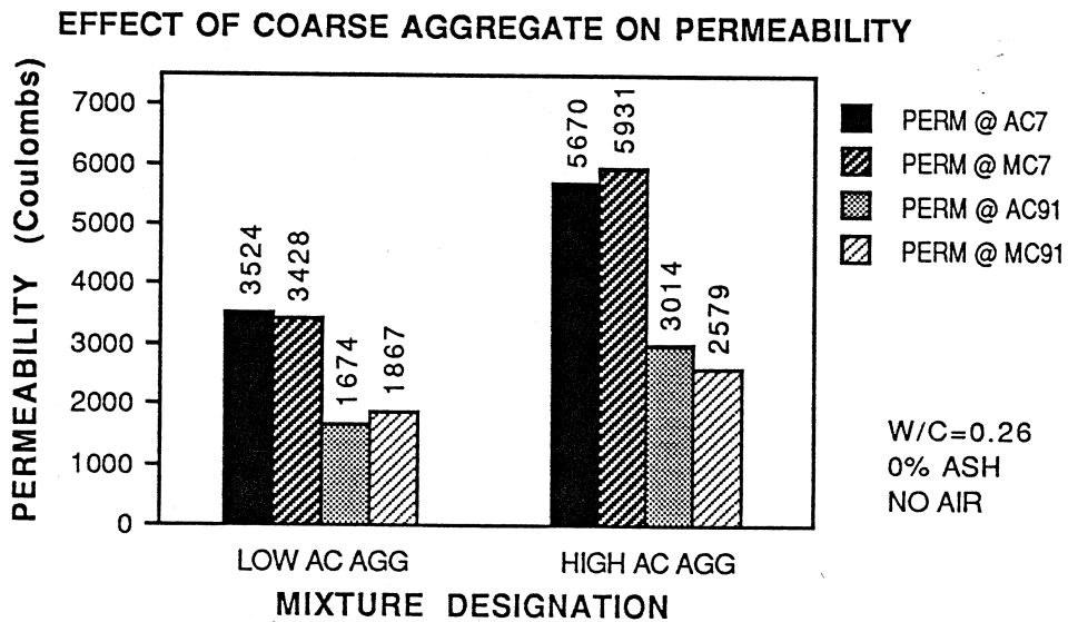
Figure 5.21 Effect of Coarse Aggregate on Permeability
