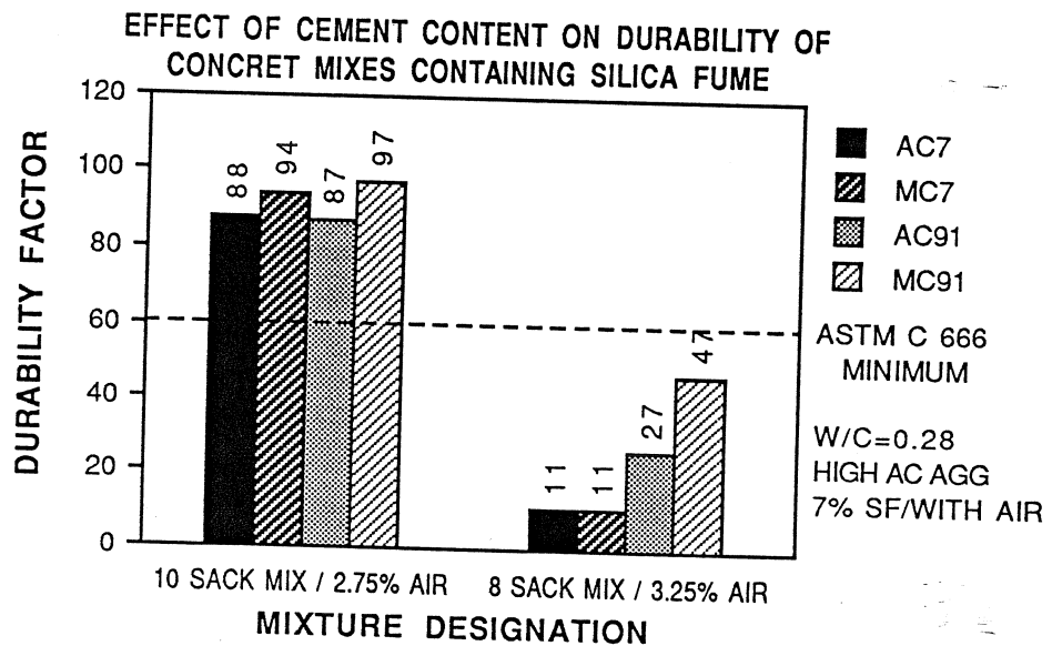
Figure 8.47 Effect of Cement Content on Durability
