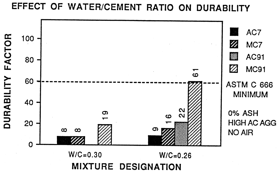
Figure 8.14 Effect of Water/Cement Ratio on Durability
