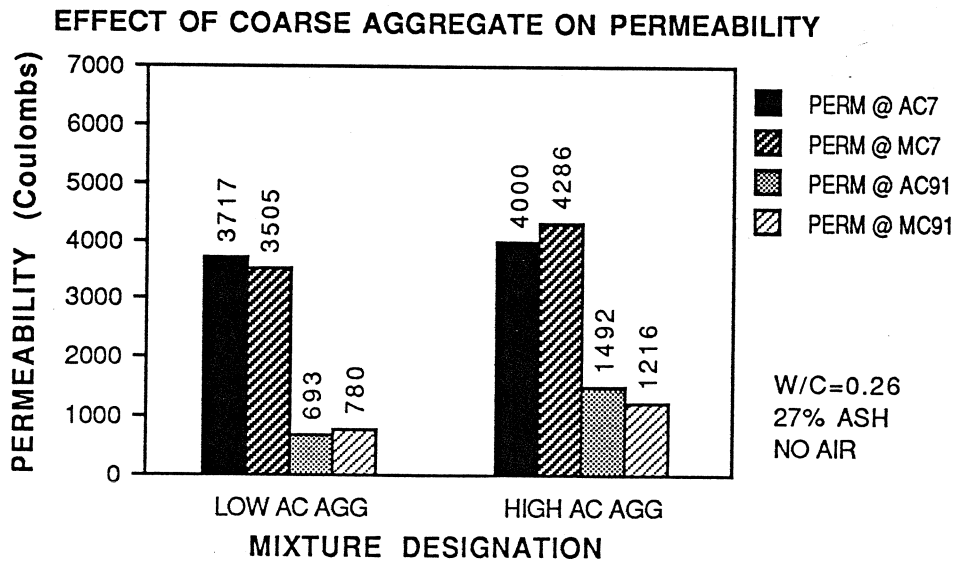
Figure 5.23 Effect of Coarse Aggregate on Permeability
