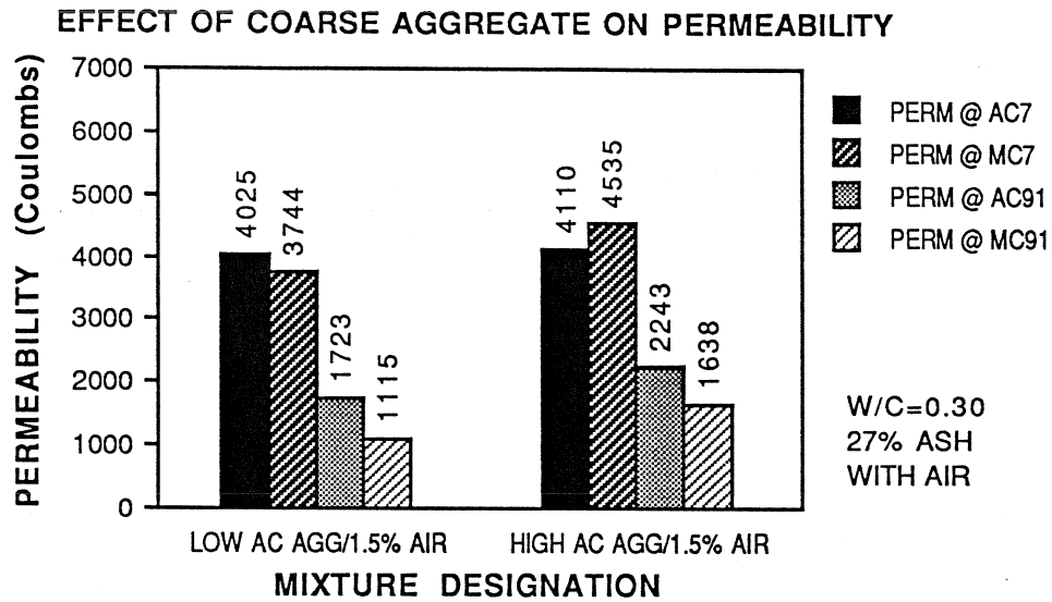
Figure 5.26 Effect of Coarse Aggregate on Permeability
