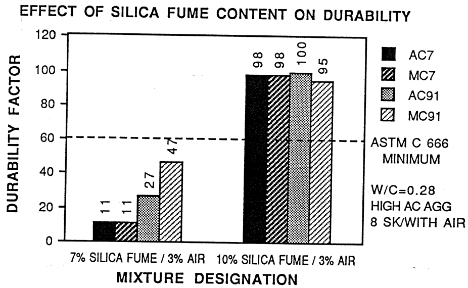
Figure 8.40 Effect of Silica Fume Content on Durability
