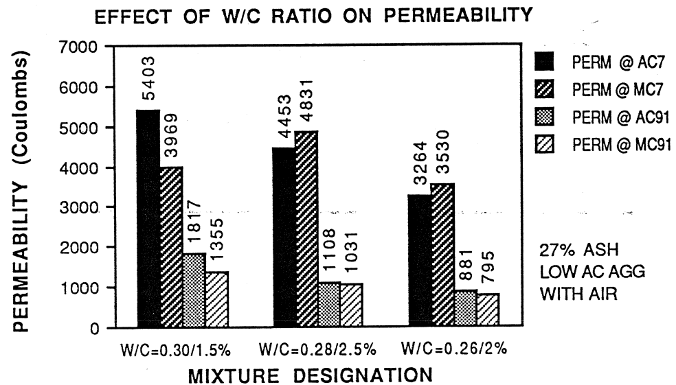
Figure 5.18 Effect of Water/Cement Ratio on Permeability
