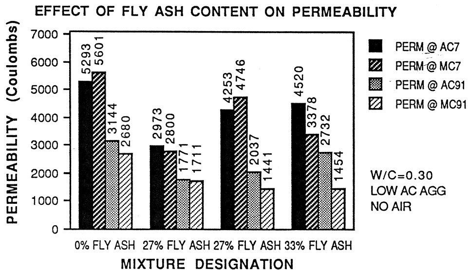
Figure 5.28 Effect of Fly Ash Content on Permeability
