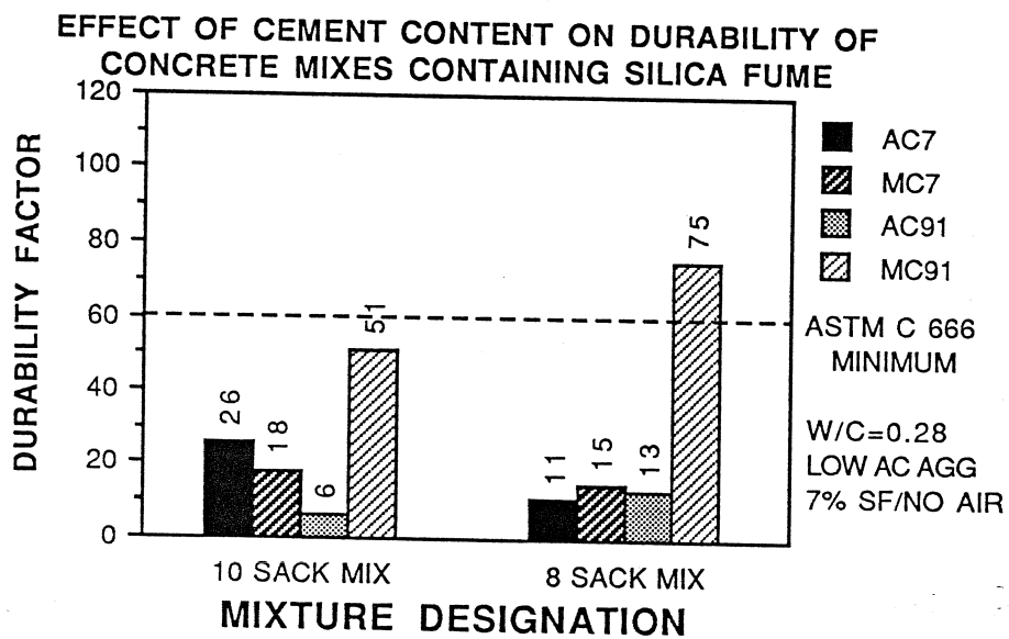
Figure 8.41 Effect of Cement Content on Durability
