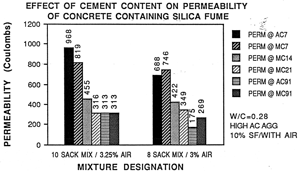
Figure 5.47 Effect of Cement Content on Permeability
