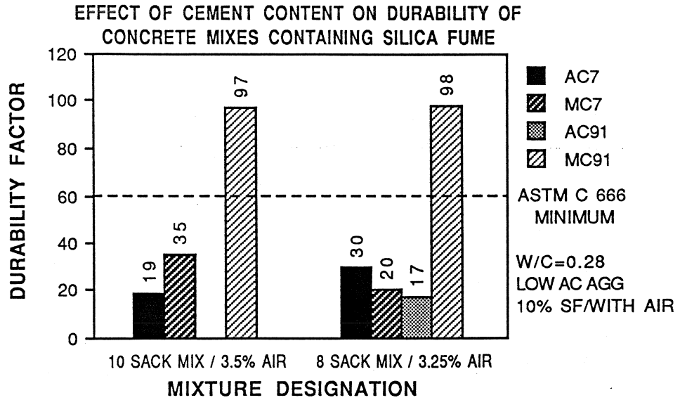
Figure 8.46 Effect of Cement Content on Durability
