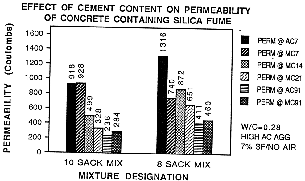
Figure 5.42 Effect of Cement Content on Permeability
