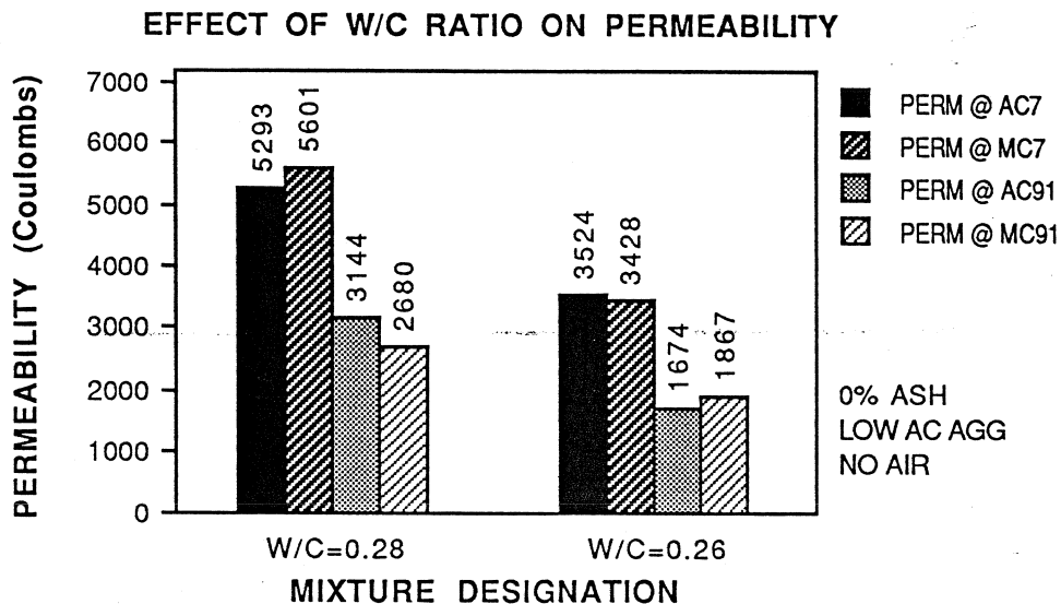
Figure 5.12 Effect of Water/Cement Ratio on Permeability
