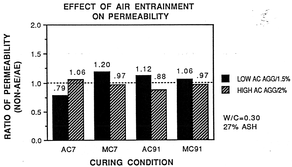
Figure 5.4 Effect of Air Entrainment on Permeability
