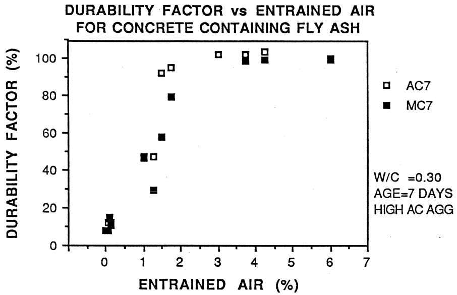
Figure 8.3 Durability Factor vs Entrained Air Content
