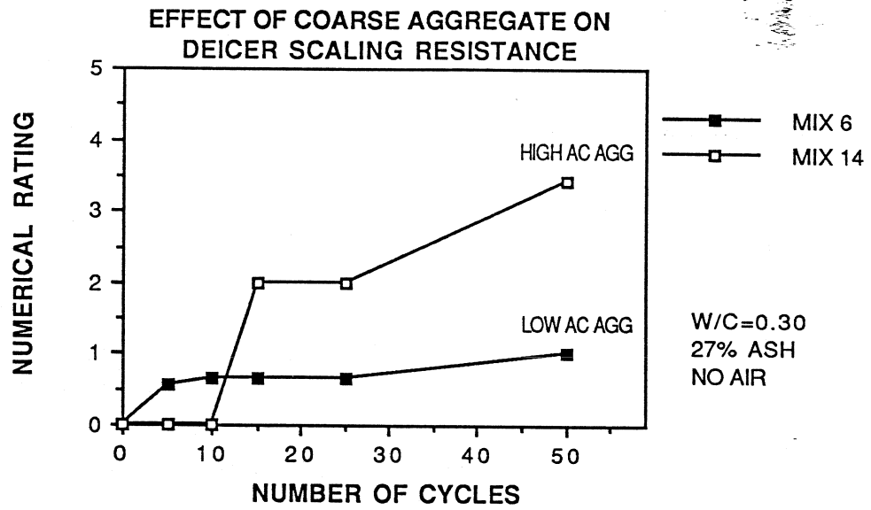
Figure 6.23 Effect of Coarse Aggregate on Scaling Resistance
