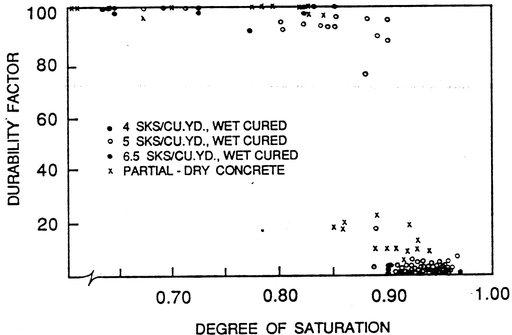
Figure 2.5 Plot of Degree of Saturation vs. Durability 70
