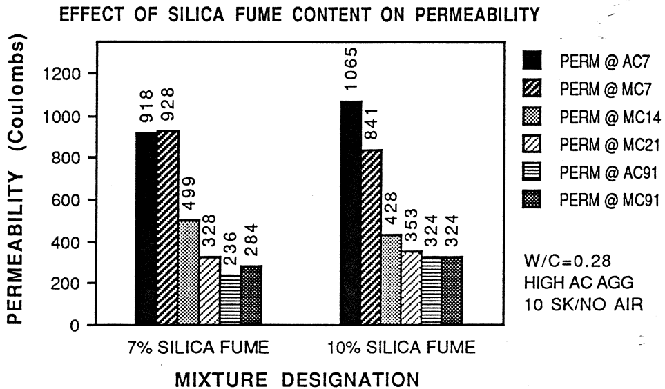
Figure 5.33 Effect of Silica Fume Content on Permeability
