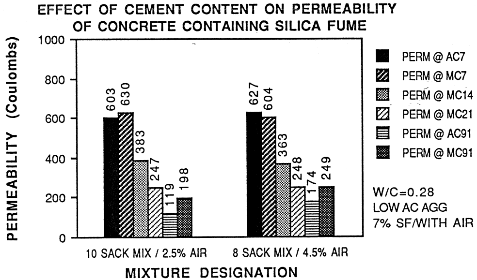
Figure 5.44 Effect of Cement Content on Permeability
