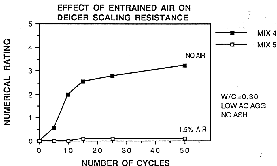
Figure 6.1 Effect of Engrained Air on Deicer Scaling Resistance
