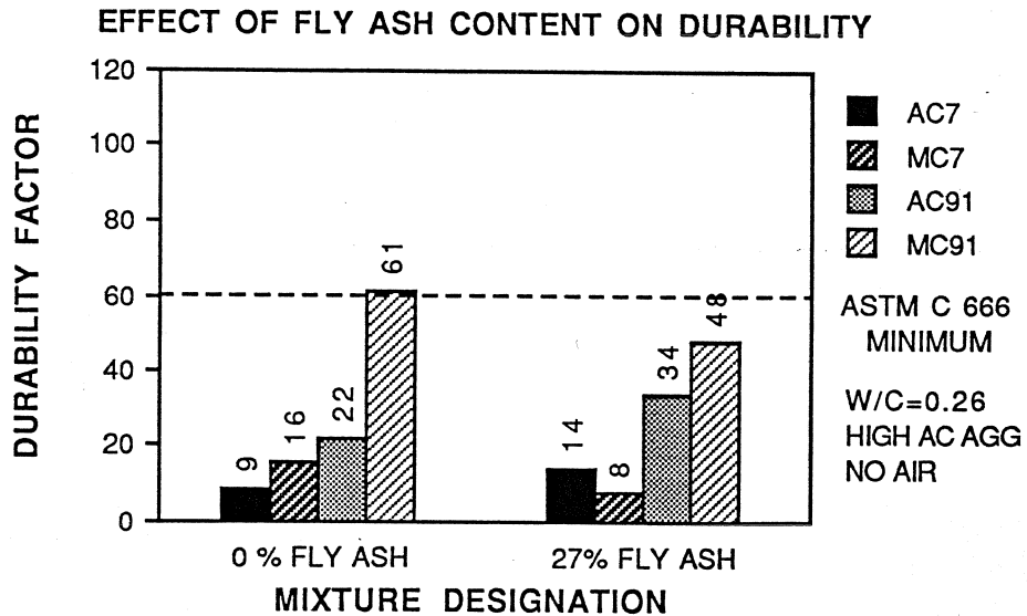
Figure 8.32 Effect of Fly Ash Content on Durability
