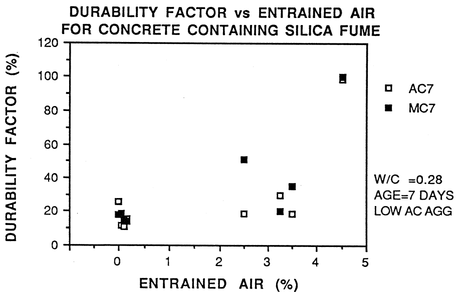
Figure 8.9 Durability Factor vs Entrained Air Content
