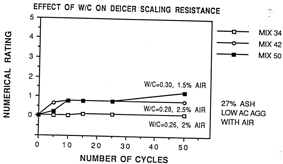
Figure 6.15 Effect of W/C Ratio on Deicer Scaling Resistance
