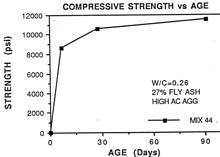
Figure 4.1 Plot of Compressive Strength vs. Age for Mix 44.
