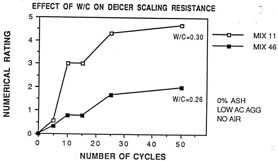
Figure 6.10 Effect of W/C Ratio on Deicer Scaling Resistance
