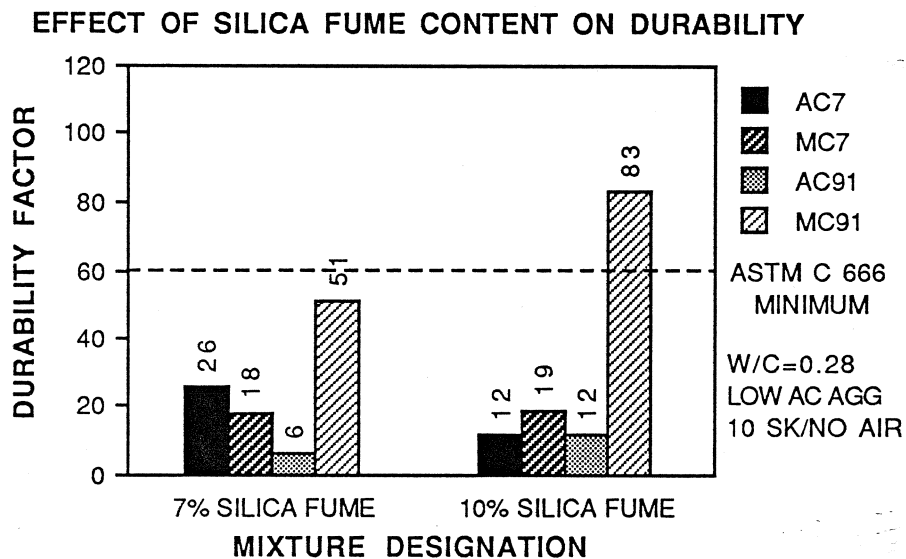
Figure 8.33 Effect of Silica Fume Content on Durability
