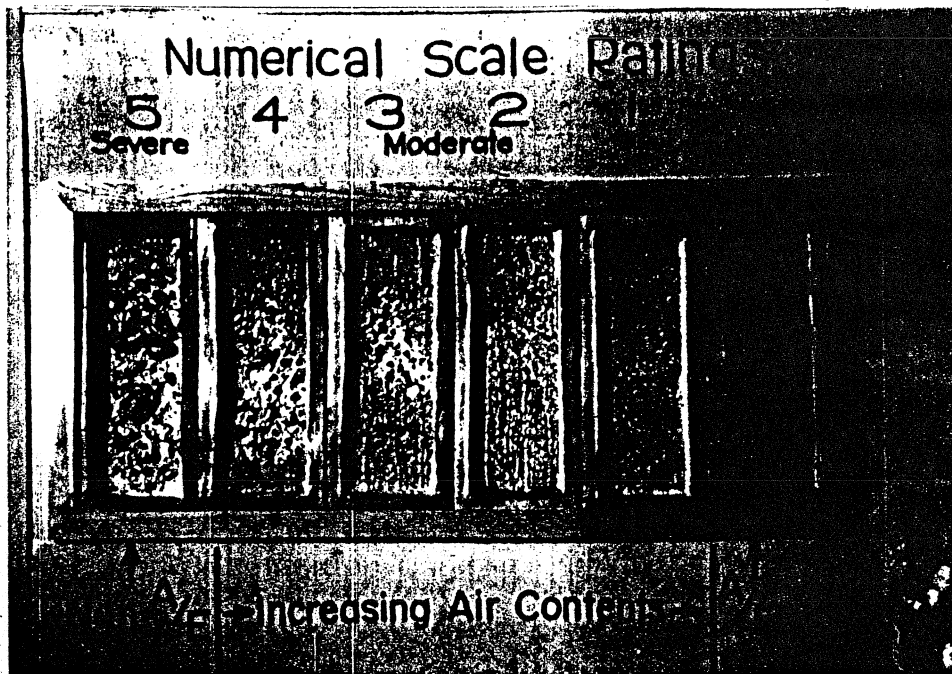
Figure 4.4 Reference Photograph Used in Rating Deicer Scaling Specimens.
