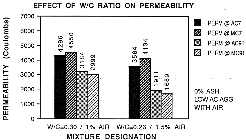
Figure 5.16 Effect of Water/Cement Ratio on Permeability
