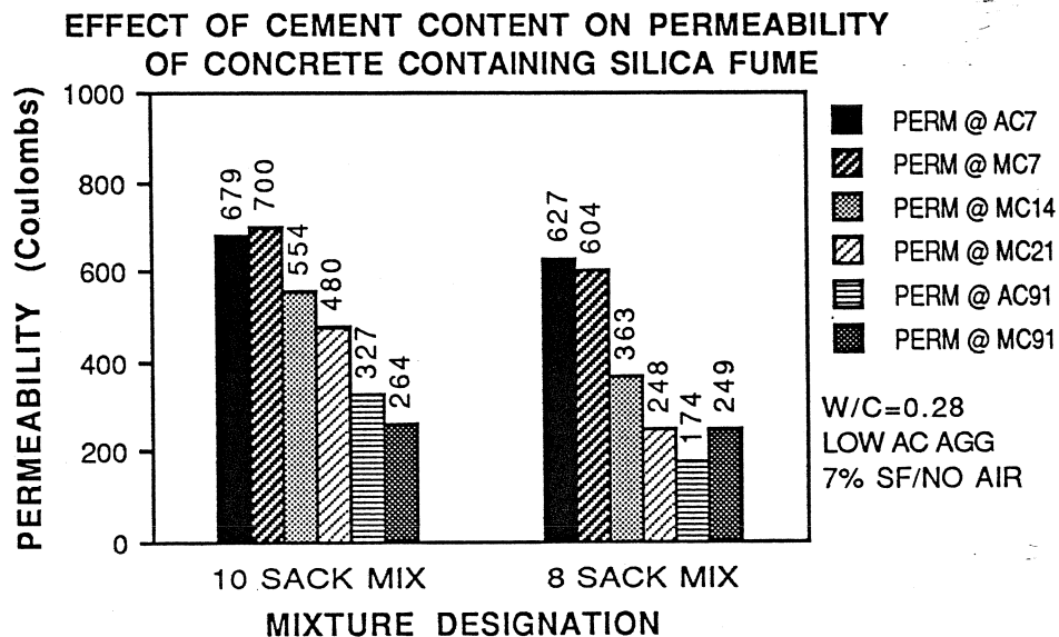
Figure 5.40 Effect of Cement Content on Permeability
