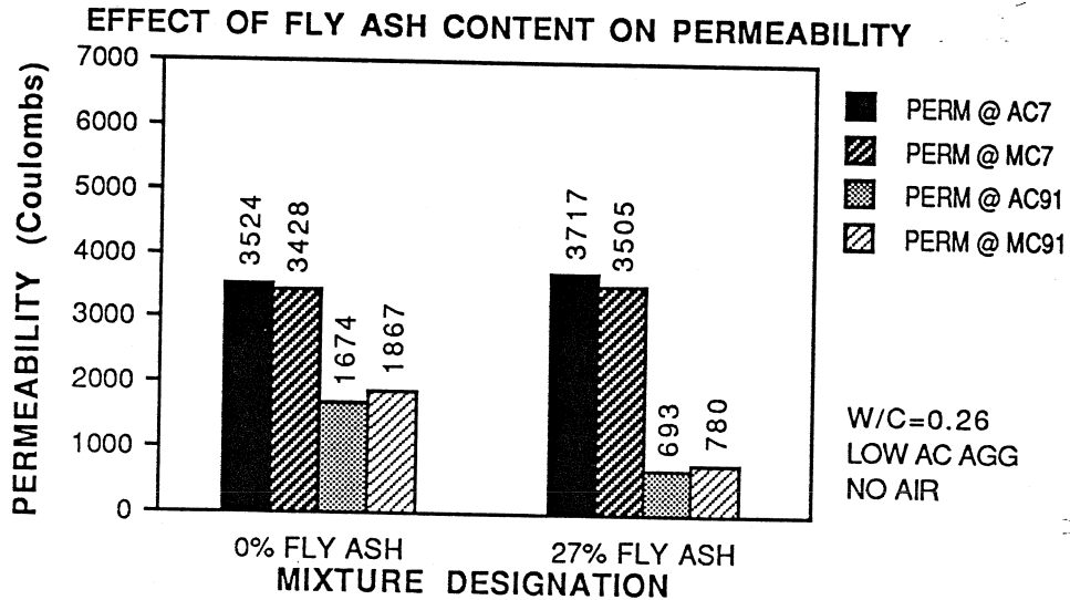
Figure 5.30 Effect of Fly Ash Content on Permeability
