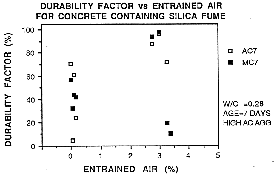
Figure 8.11 Durability Factor vs Entrained Air Content
