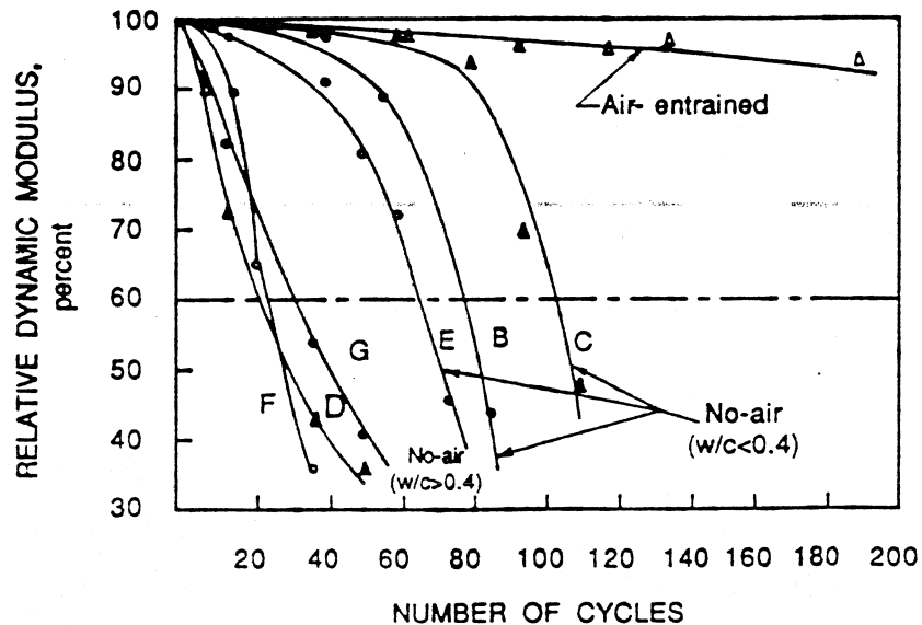
Figure 3.4 Plot of Freeze-Thaw Durability vs. Cycles for Mixes Tested Under ASTM C 666 from Khalil 27 .
