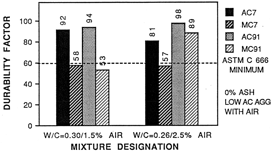
EFFECT OF WATER/CEMENT RATIO ON DURABILITY
