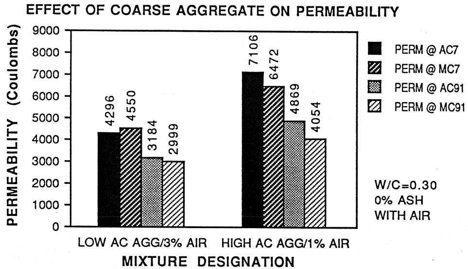
Figure 5.24 Effect of Coarse Aggregate on Permeability
