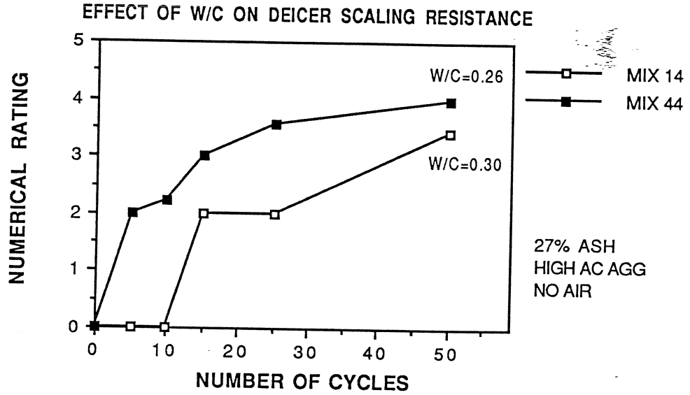
Figure 6.12 Effect of W/C Ratio on Deicer Scaling Resistance
