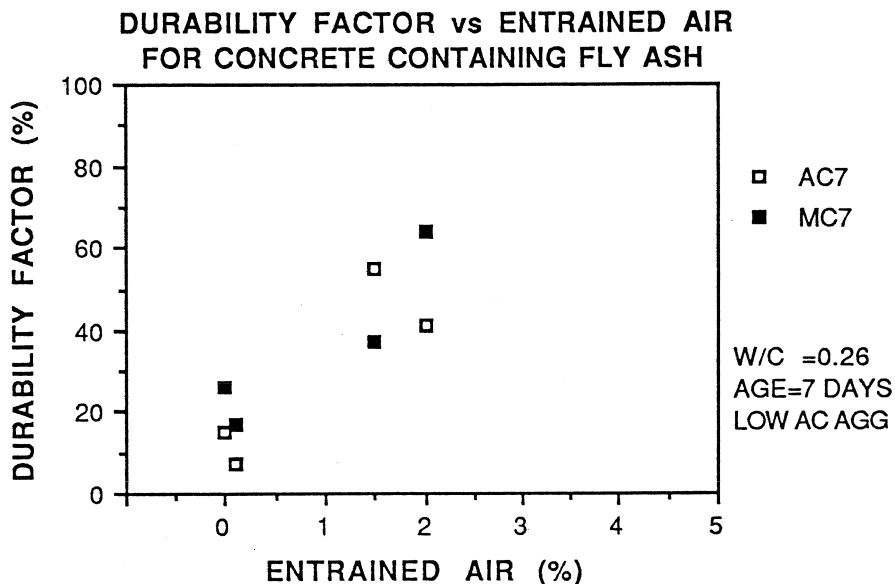
Figure 8.5 Durability Factor vs Entrained Air Content
