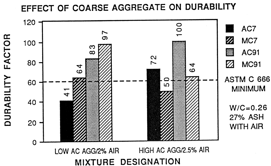
Figure 8.28 Effect of Coarse Aggregate on Durability
