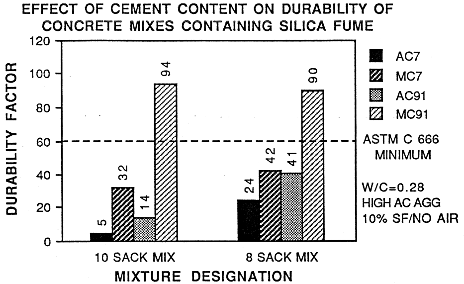
Figure 8.44 Effect of Cement Content on Durability
