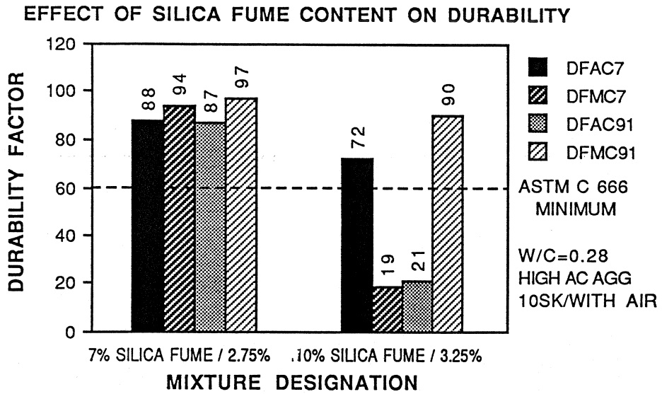
Figure 8.36 Effect of Silica Fume Content on Durability
