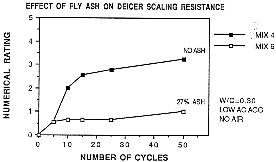
Figure 6.17 Effect of Fly Ash on Deicer Scaling Resistance
