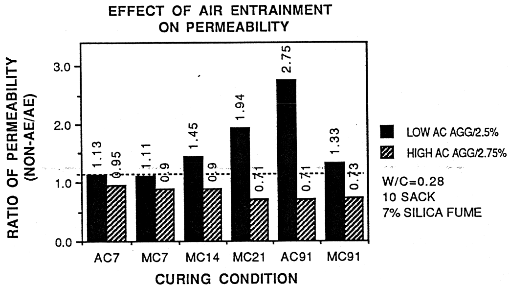
Figure 5.8 Effect of Air Entrainment on Permeability
