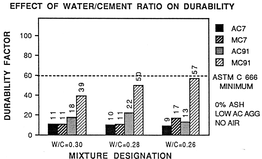
Figure 8.13 Effect of Water/Cement Ratio on Durability
