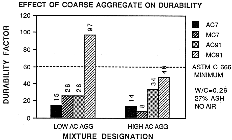
Figure 8.24 Effect of Coarse Aggregate on Durability
