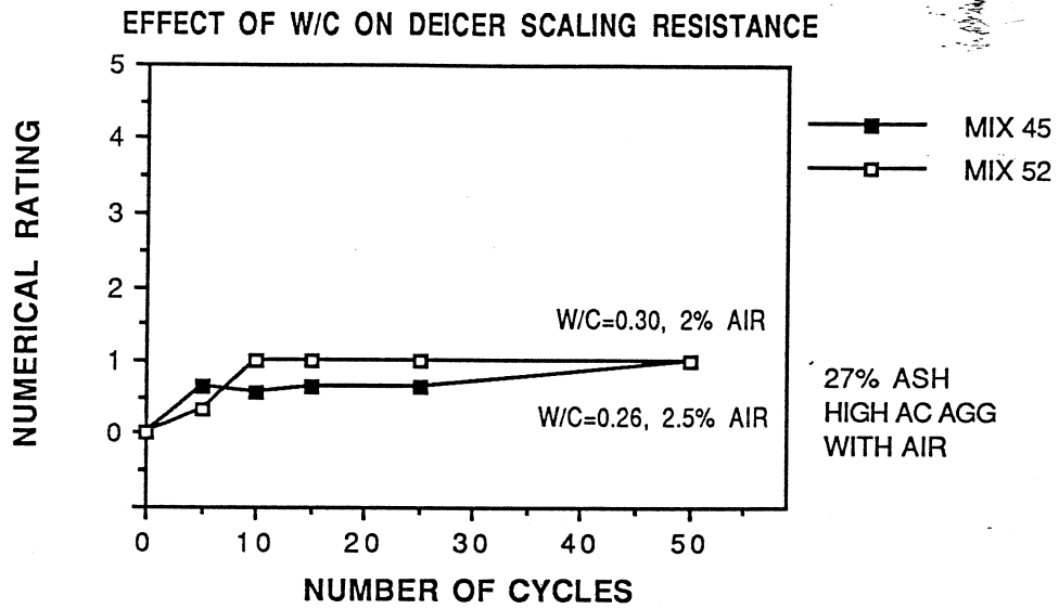
Figure 6.16 Effect of W/C Ratio on Deicer Scaling Resistance
