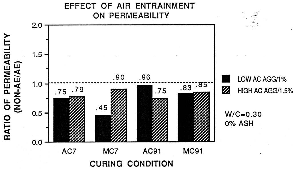
Figure 5.2 Effect of Air entrainment on Permeability.
