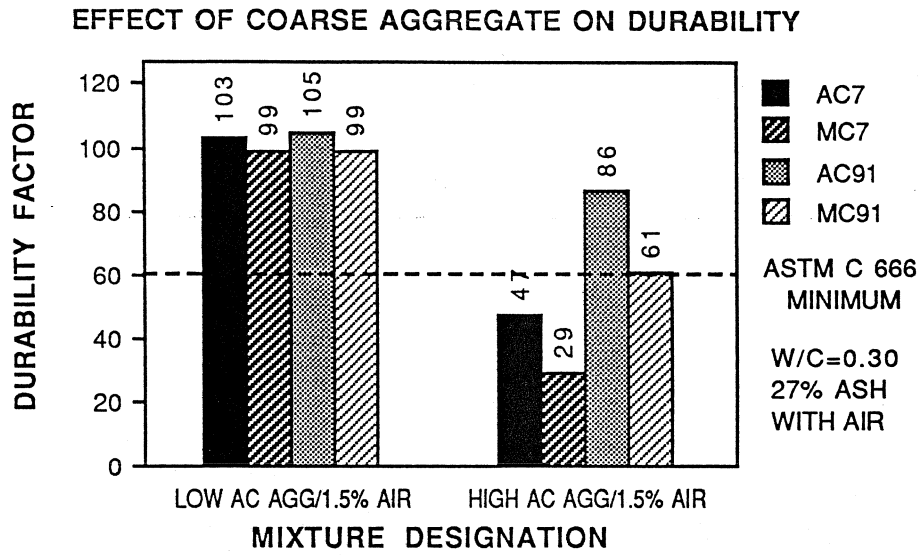
Figure 8.27 Effect of Coarse Aggregate on Durability
