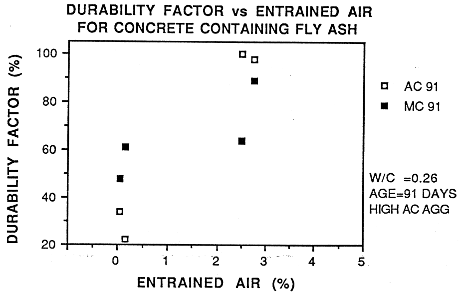
Figure 8.8 Durability Factor vs Entrained Air Content
