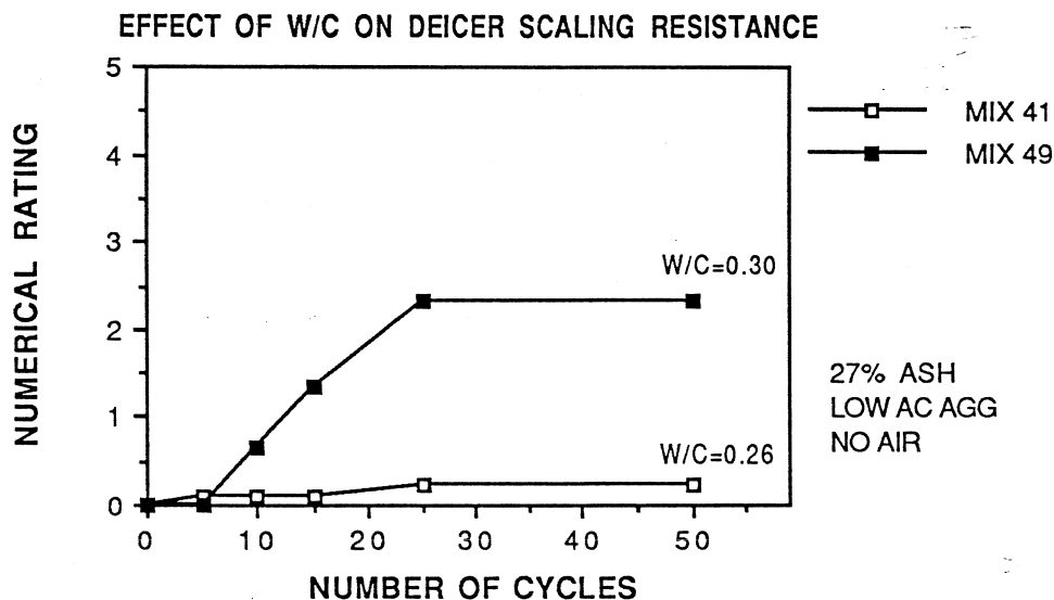
Figure 6.11 Effect of W/C Ratio on Deicer Scaling Resistance
