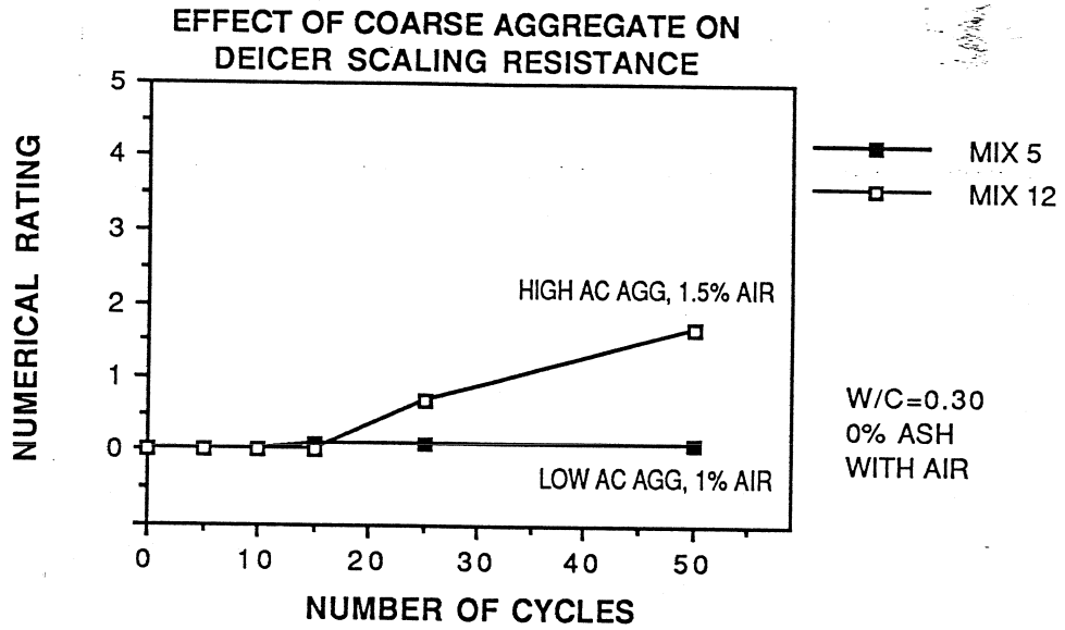
Figure 6.25 Effect of Coarse Aggregate on Scaling Resistance
