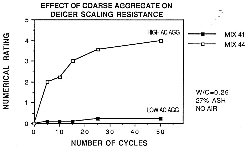
Figure 6.24 Effect of Coarse Aggregate on Scaling Resistance
