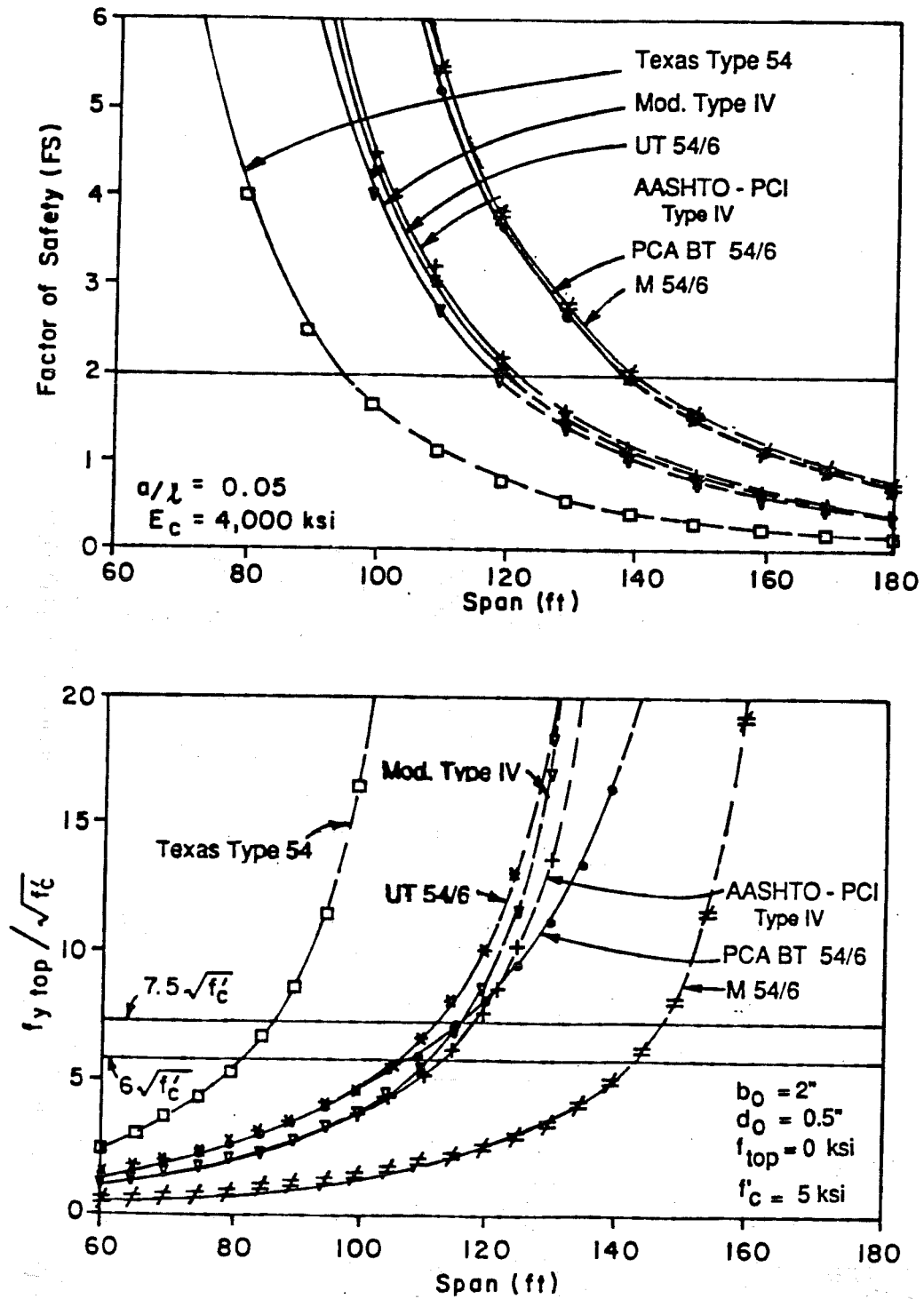
Fig. 4.62 Factor of safety and top fiber stress versus span length for 54-in. sections: a) Factor of safety (FS); b) Top fiber stress
