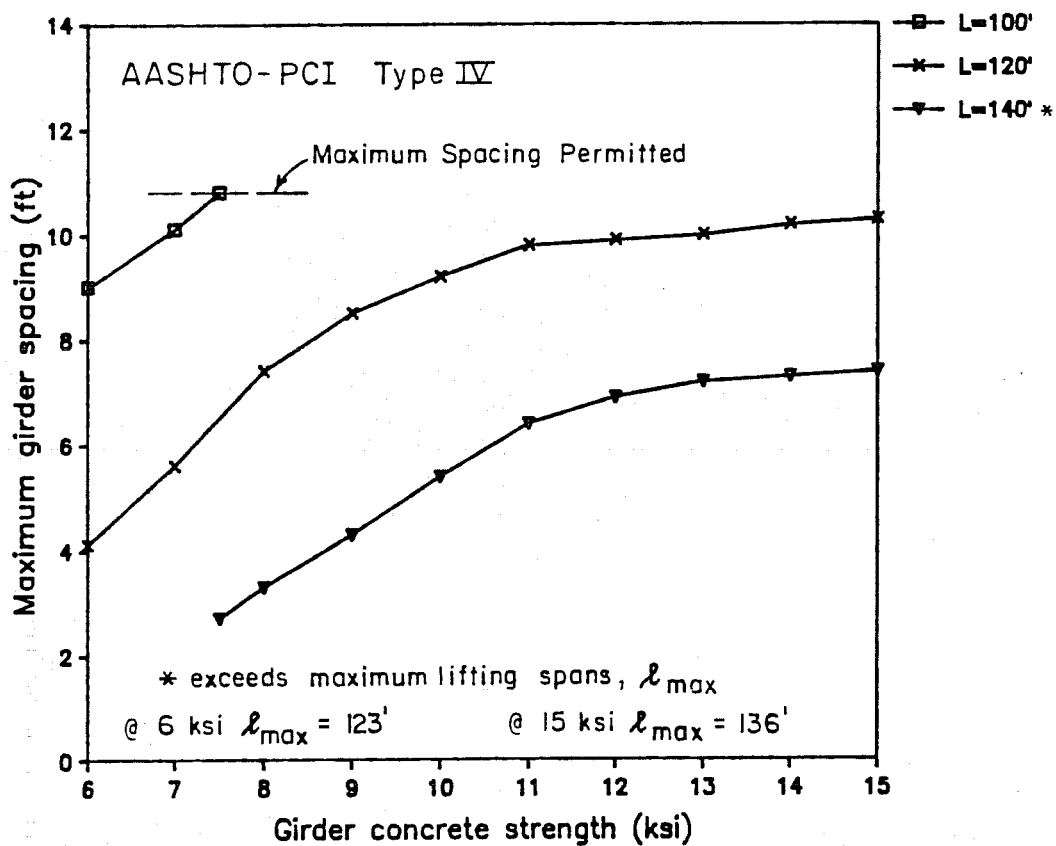
Fig. 3.15 Variation in girder spacing with concrete strength.
