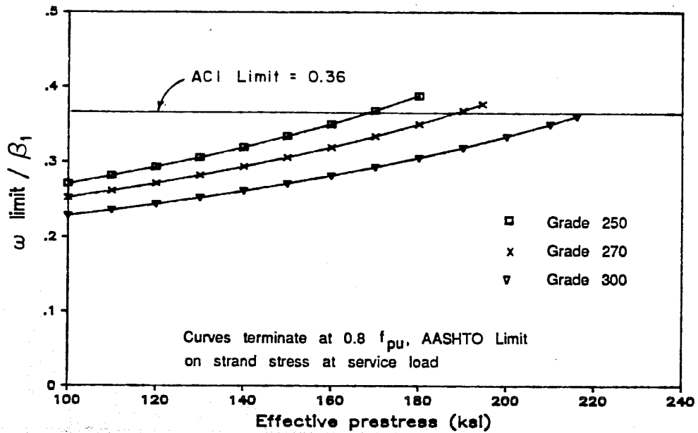
Fig. 4.49 Ratio of maximum reinforcement limit to \beta_1 versus effective prestress
