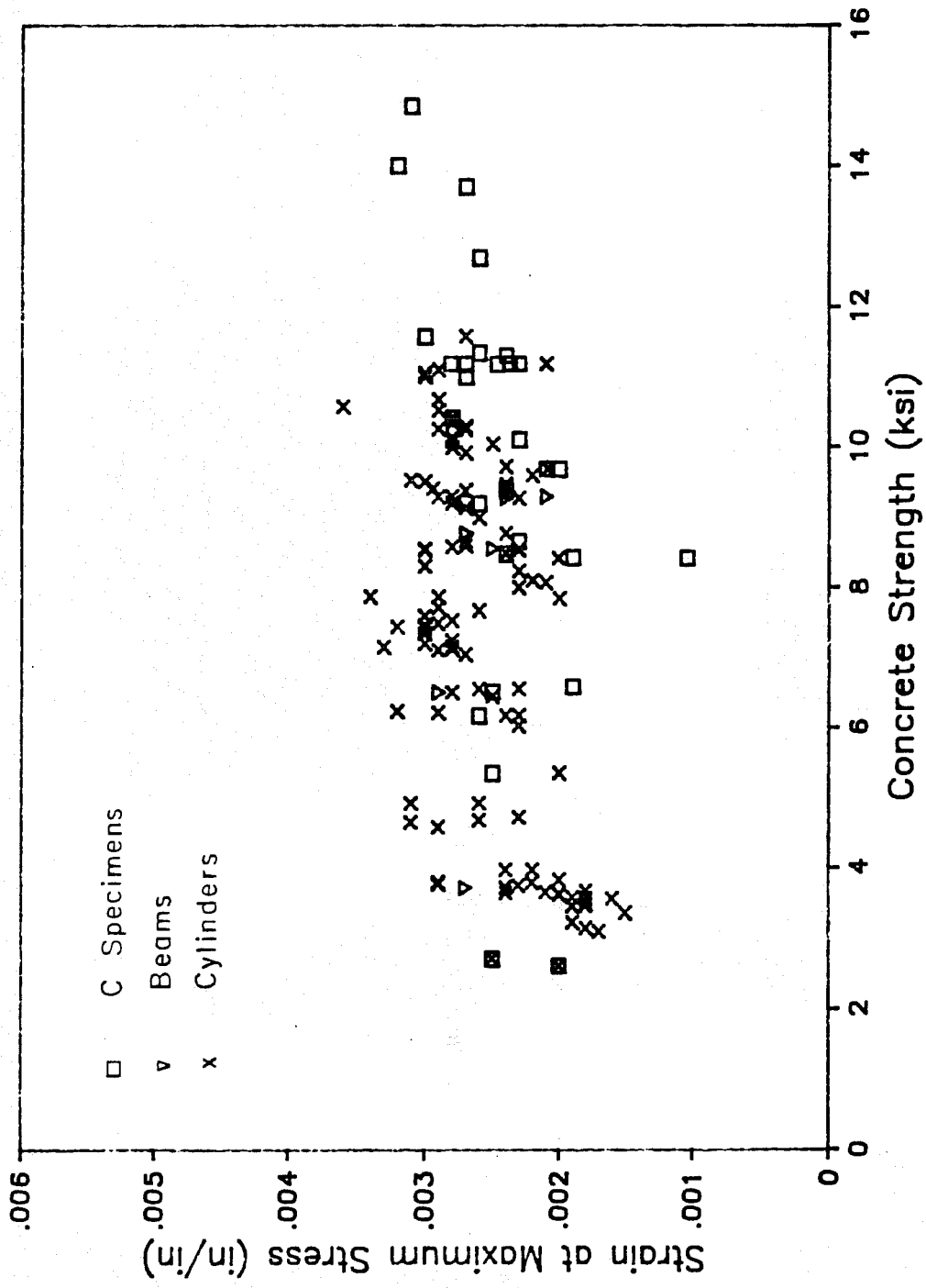
Fig. 2.6 Summary of strains at maximum stress
