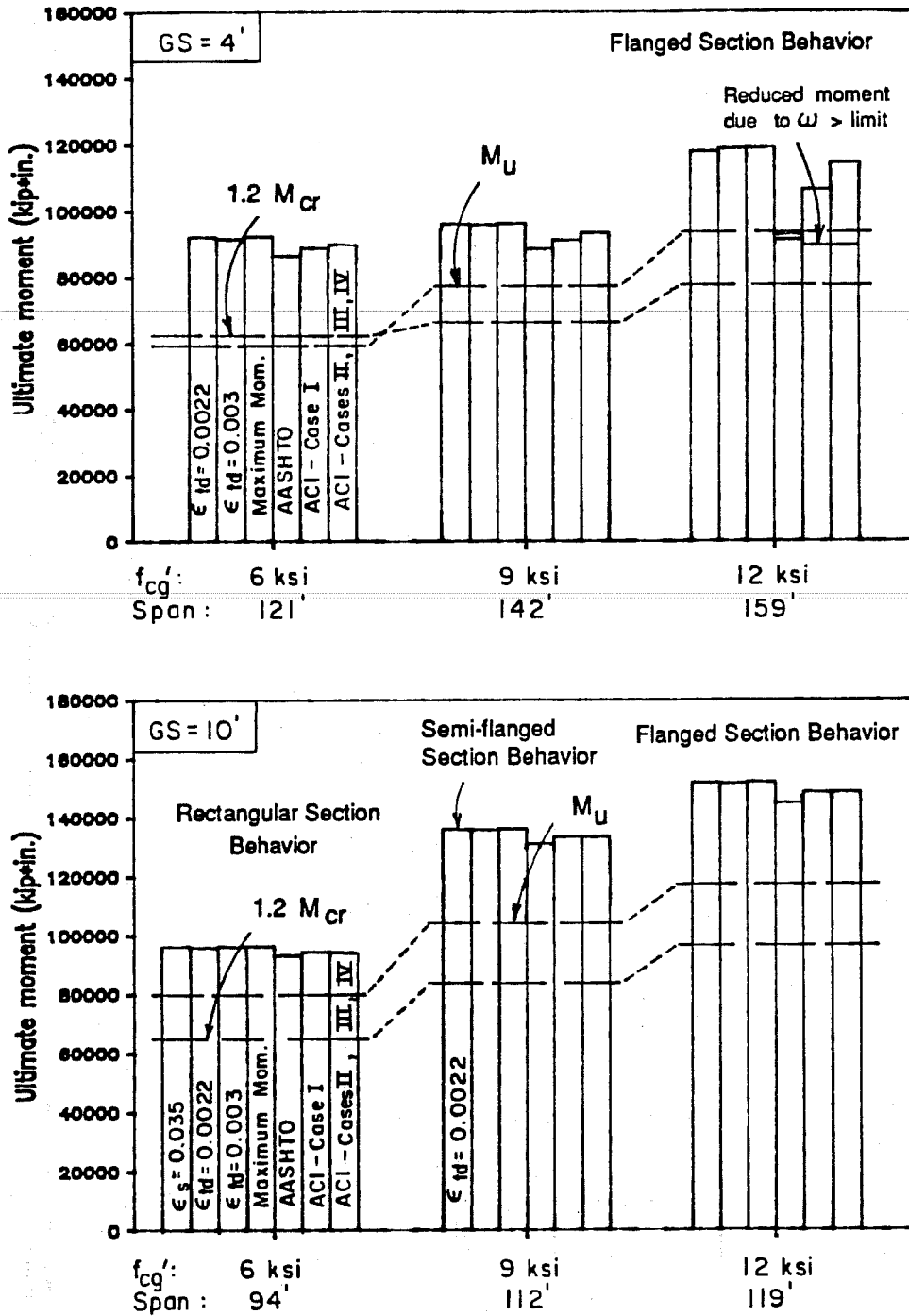
Fig. 4.31 Ultimate moment capacity for maximum span designs
