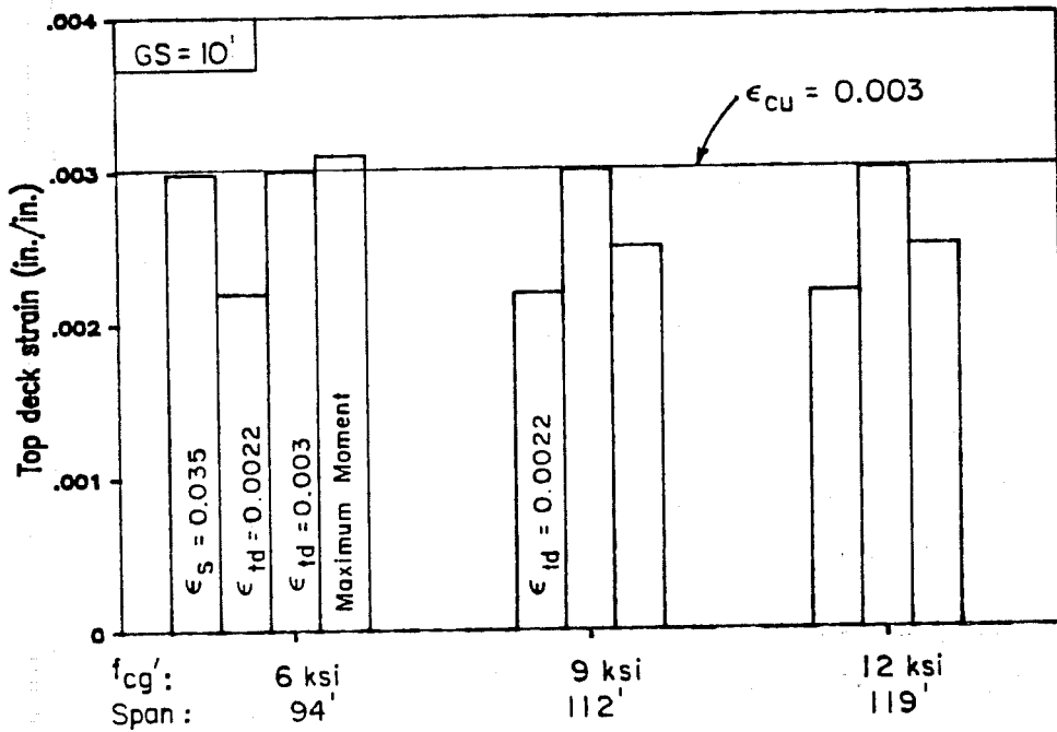
Fig. 4.35 Concrete strains at top of deck for maximum span designs
