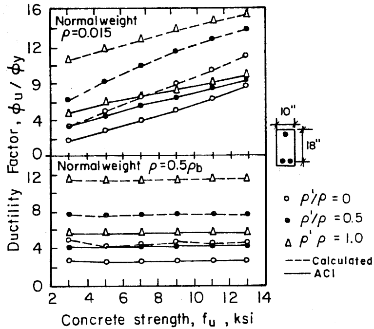
Fig. 2.23 Effect of concrete strength on the deflection ductility of a singly reinforced beam [2]
