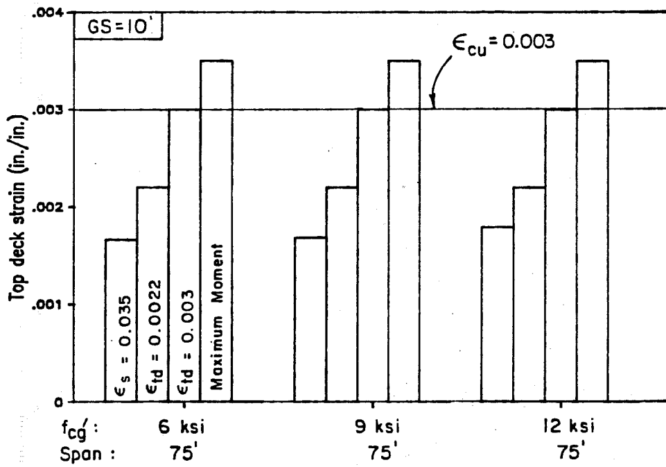
Fig. 4.36 Concrete strains at top of deck for typical span designs
