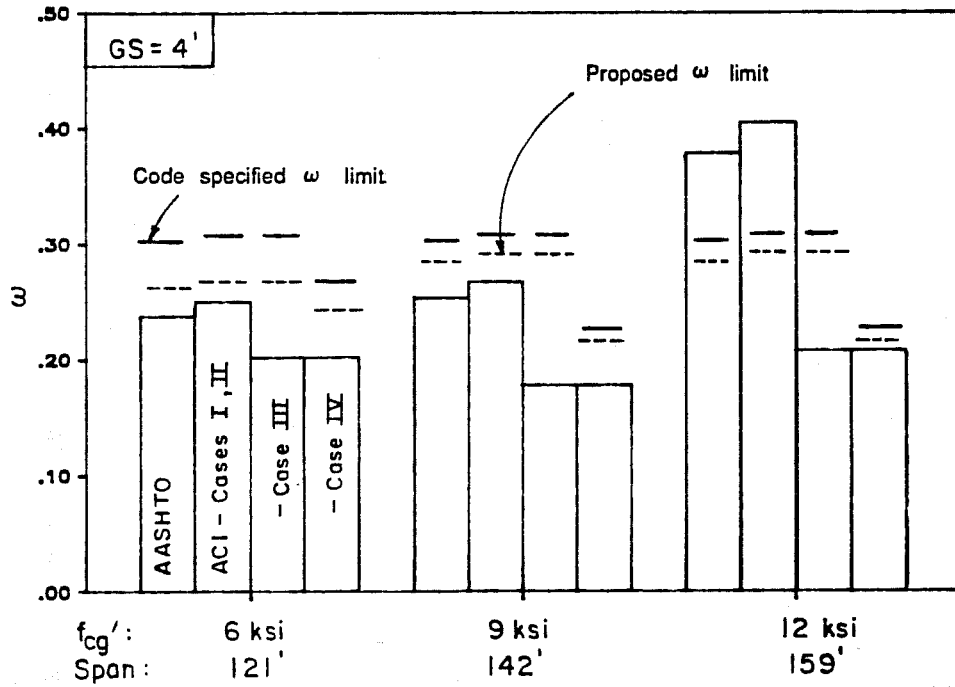
Fig. 4.51 Comparison of values and maximum limits for w for specimens and maximum span designs with GS = 4 ft
