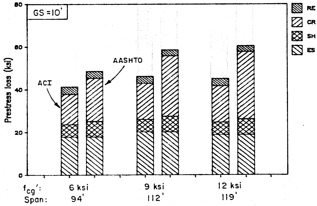
Fig. 4.71 Prestress losses for maximum span designs
