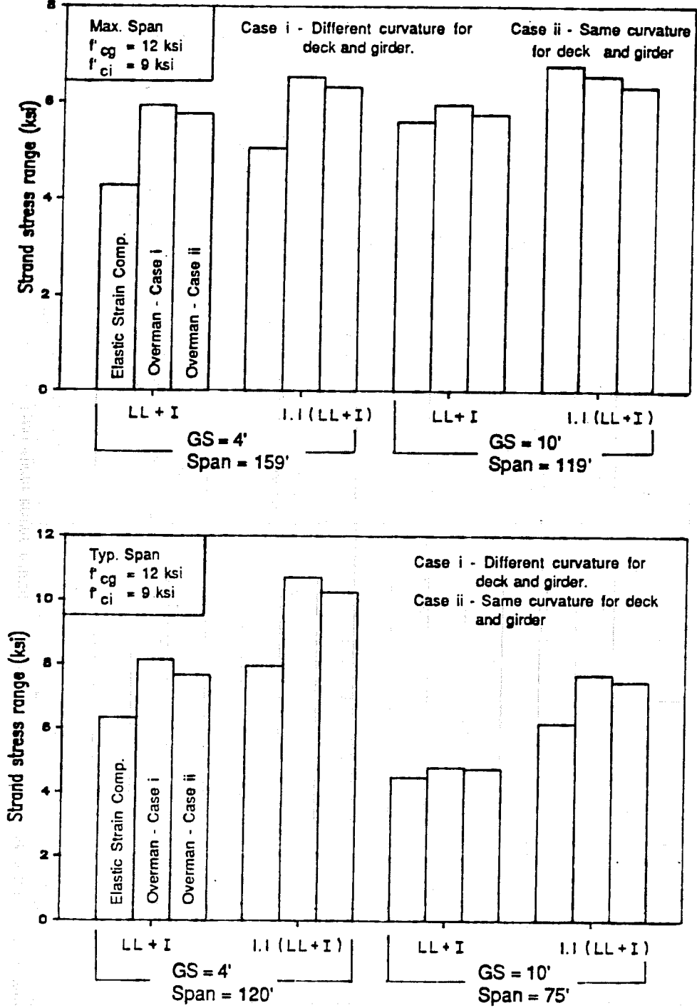
Fig. 4.66 Comparison of methods for computing strand stress range
