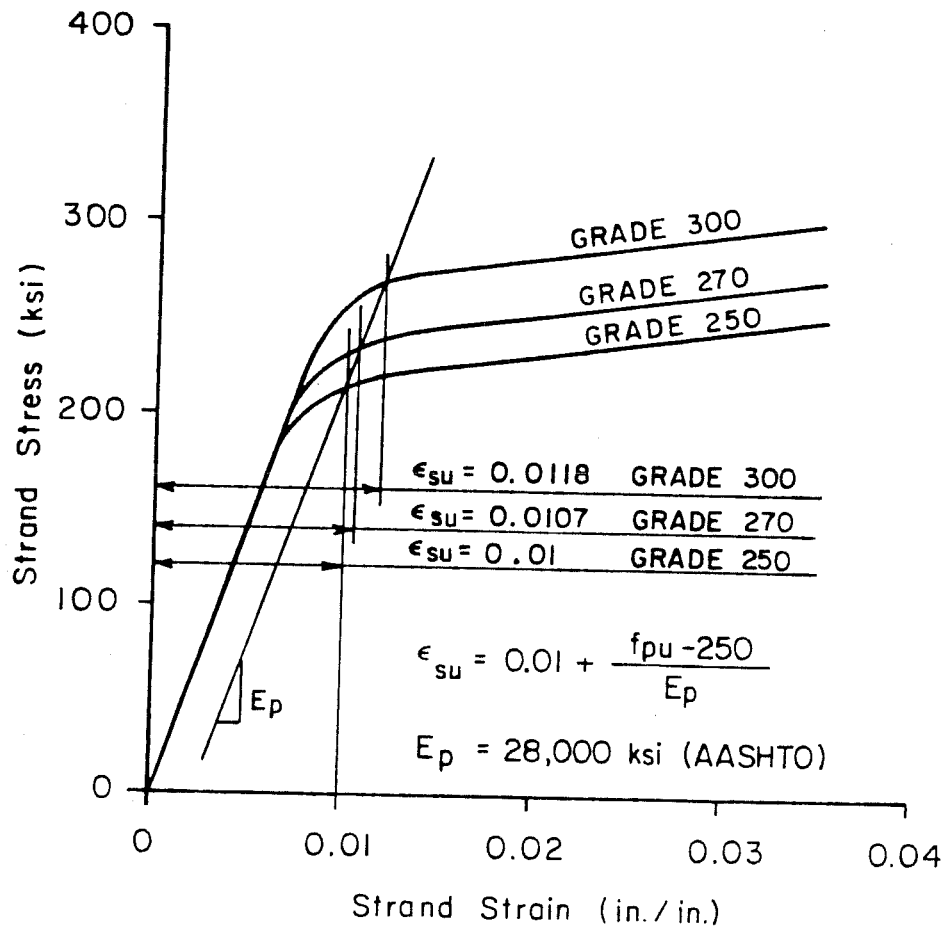
Fig. A.2 Limiting prestressed reinforcement strain for maximum reinforcement limit
