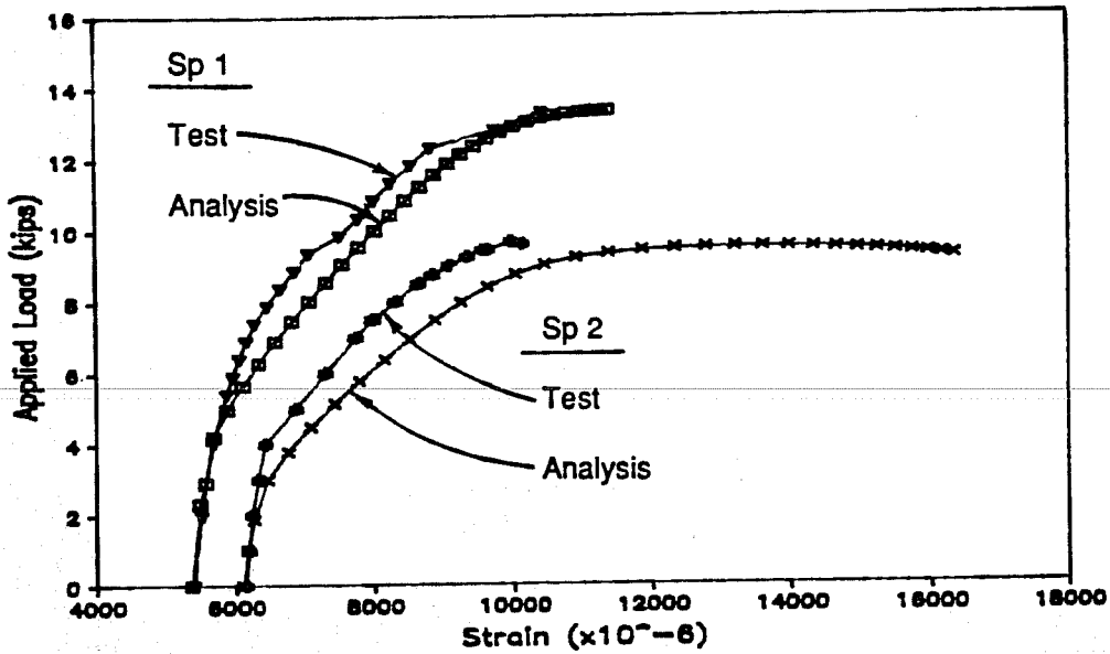
Fig. 4.13 Comparison of measured and predicted strand strains during flexure tests
