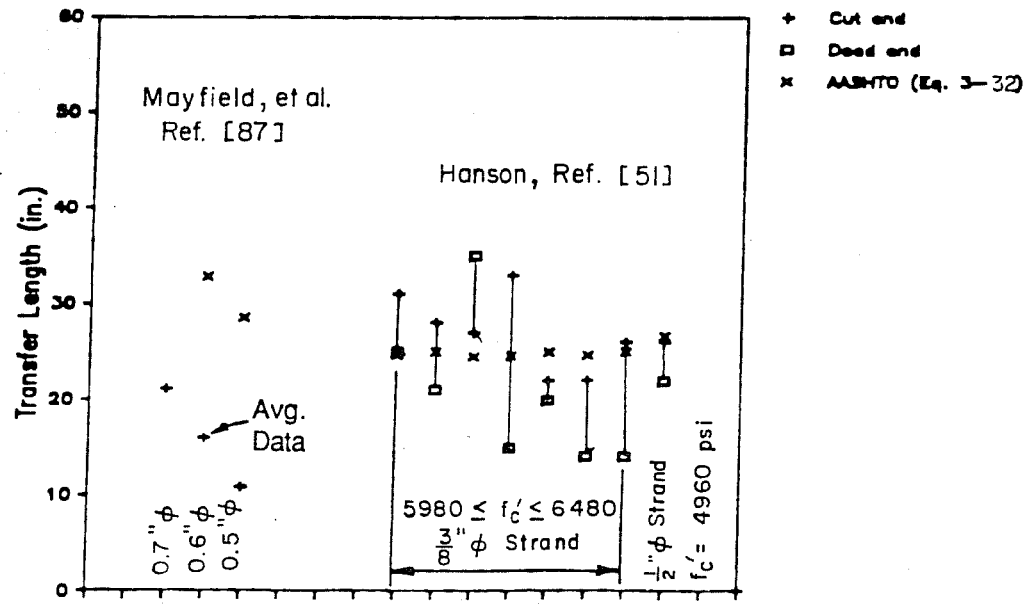
Fig. 2.27 Transfer lengths for different sizes of strand and concrete strengths [51, 87]
