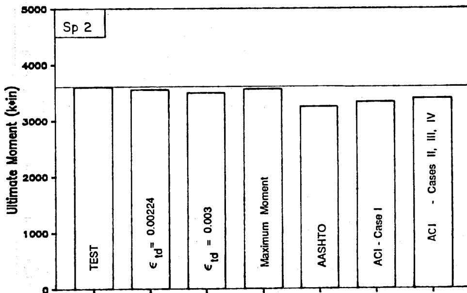
Fig. 4.21 Comparison of measured and predicted ultimate moment capacity for flexure tests
