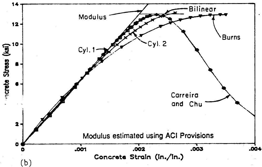
Fig. 4.5 Measured and analytical stress-strain curves for girder concrete - Specimen 1: a) Using measured E_c and \epsilon_c ; b) Using estimated E_c and \epsilon_c
