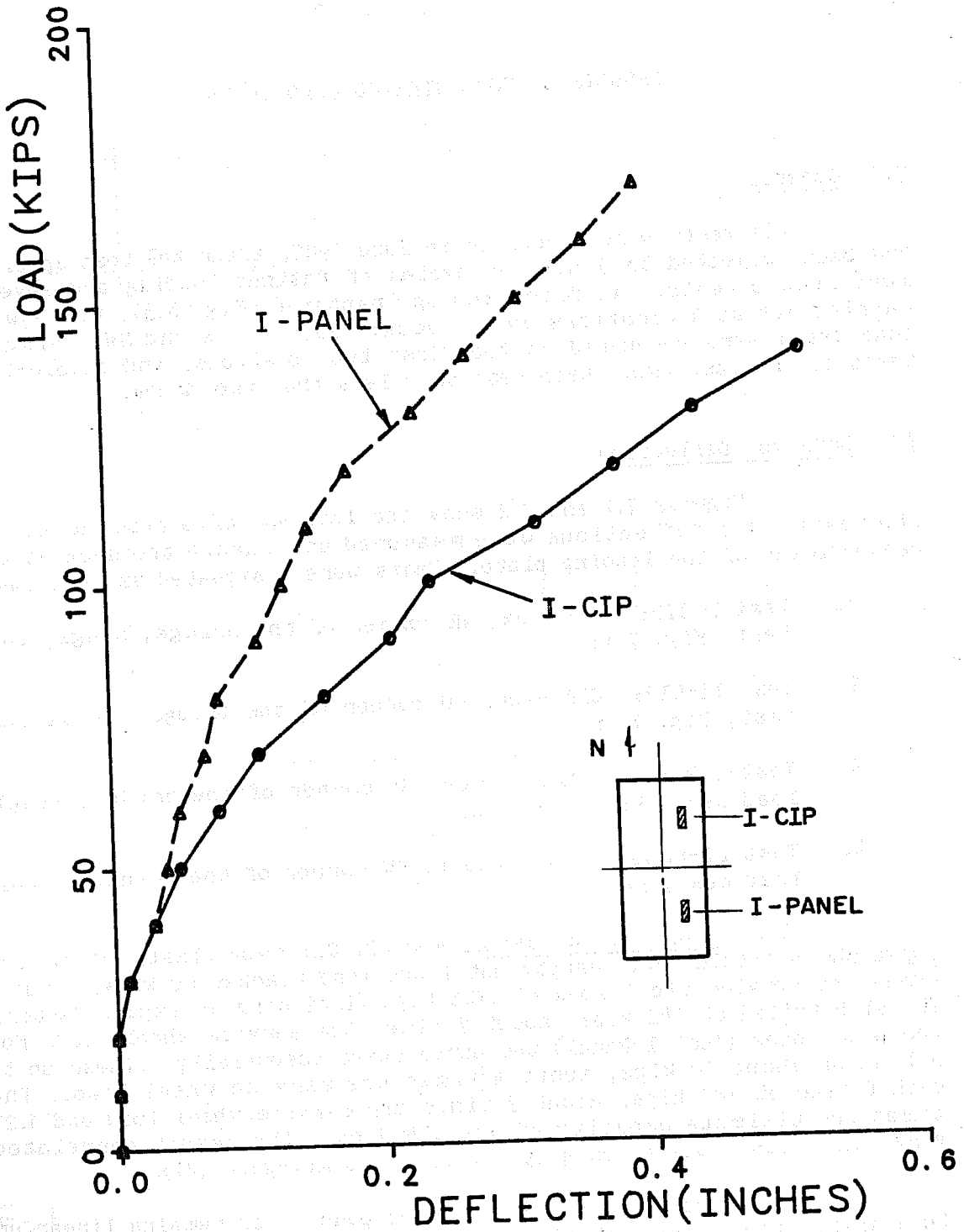
Fig. 7.1 Deflections from single load tests
