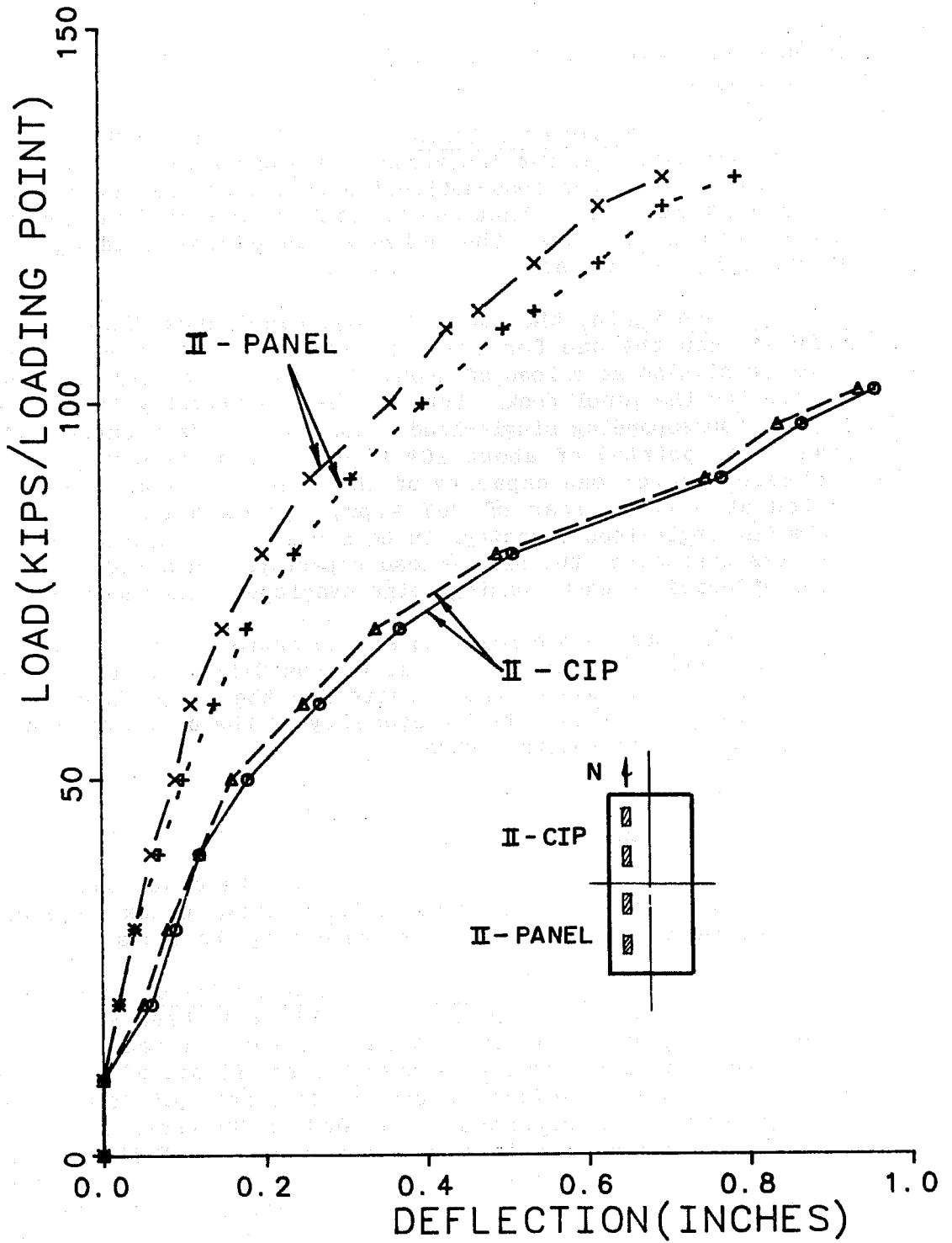
Fig. 7.2 Deflections from double load tests
