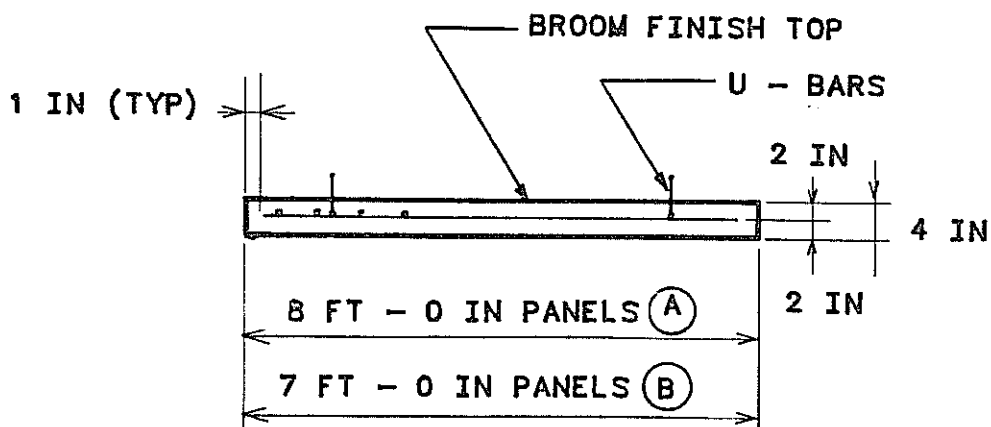
SECTION
