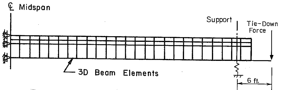
Fi.1(b) Longitudinal section of bridge model
