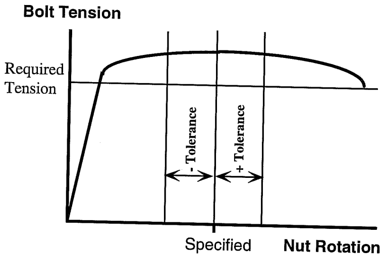
Figure 2.1 Sample tension-turn relationship for A325 bolt
