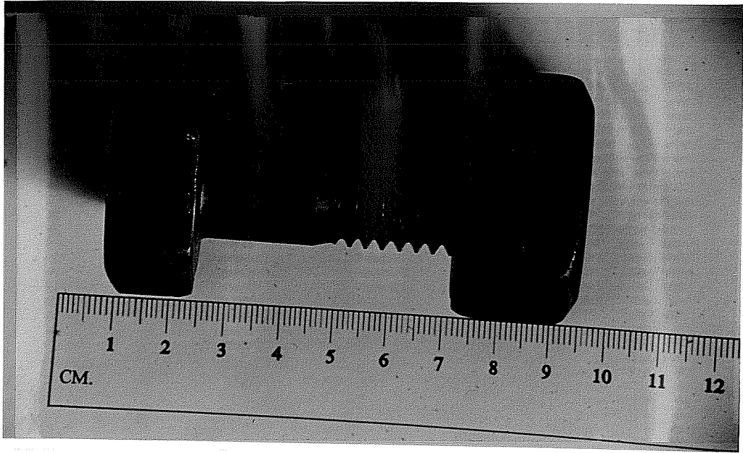
Figure 3.3 Example of flush grip for a 24 mm x 70 mm bolt
