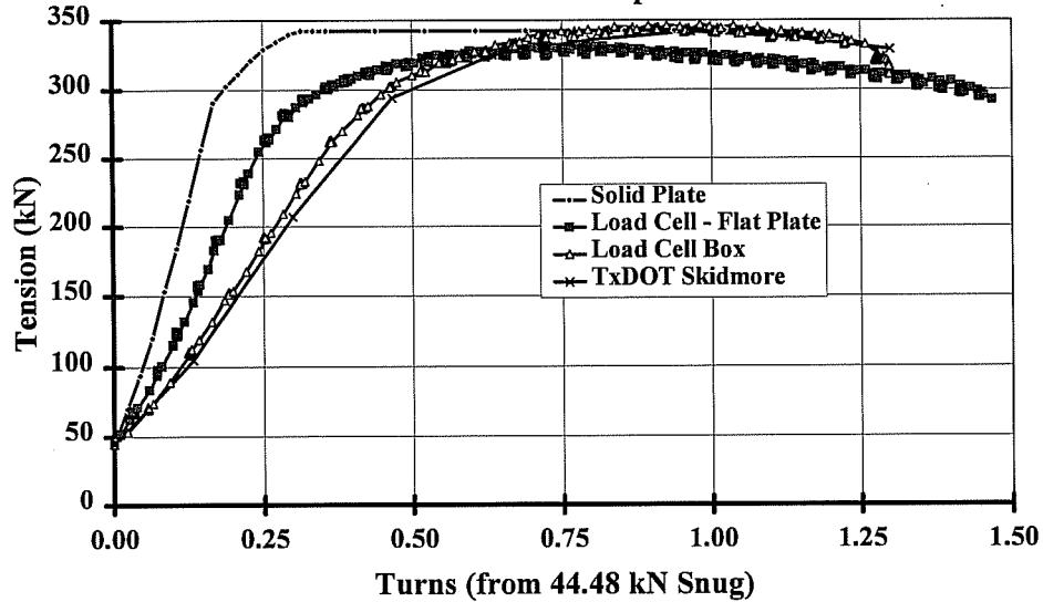
Figure 4. 6 Relative performance of 24 x 120 three turn grip bolts in different test setups
