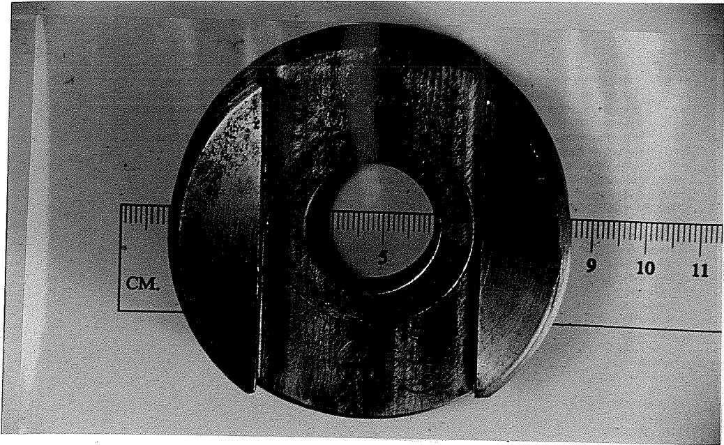
Figure 3. 10 Top view of bolt head mounting insert
