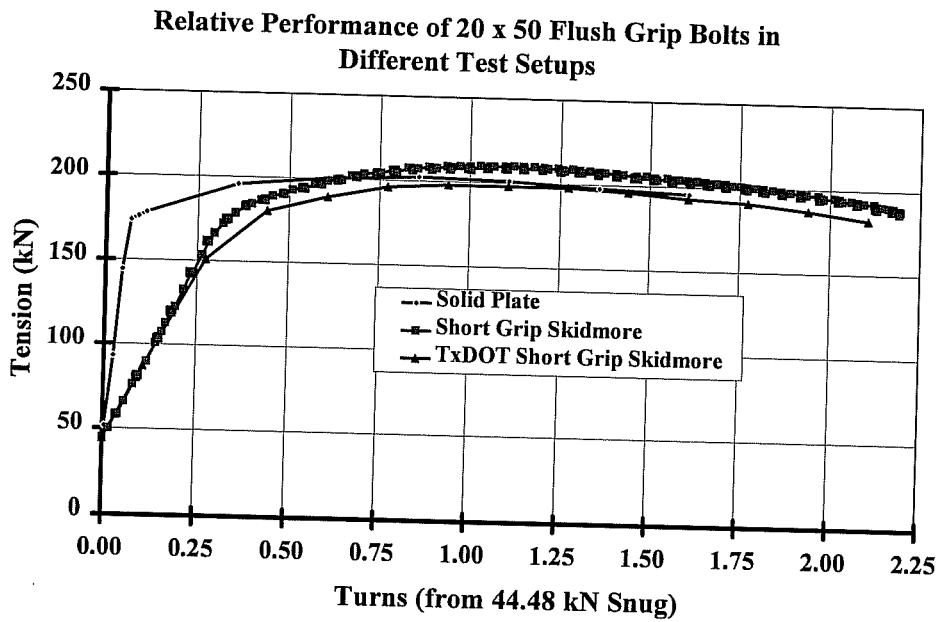
Figure 4. 8 Relative performance of 20 x 50 flush grip bolts in different test setups
