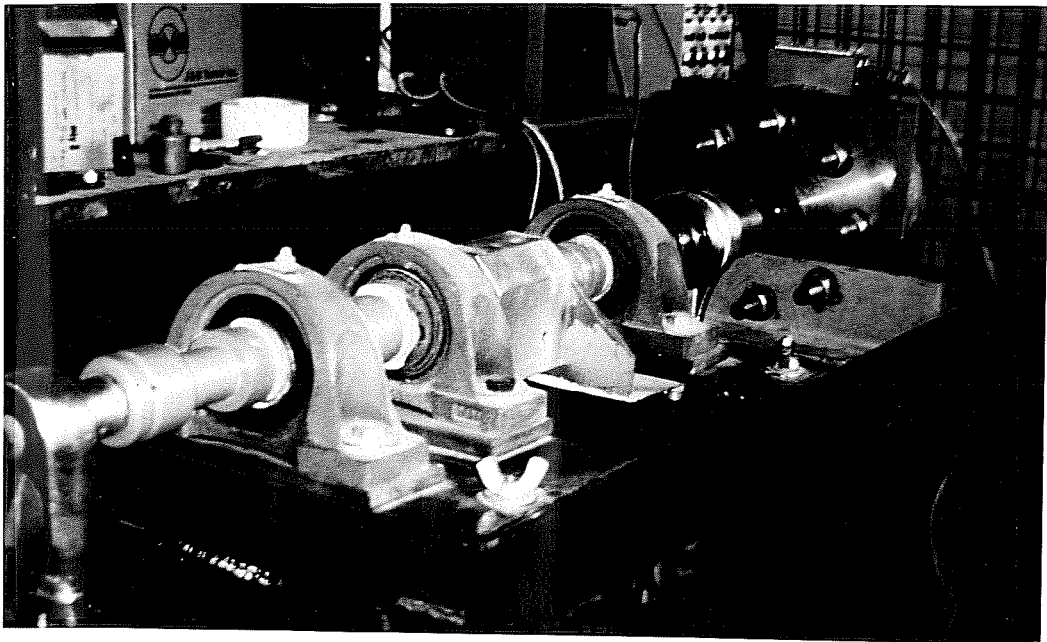
Figure 3.6 Front view of load cell - flat plate system
