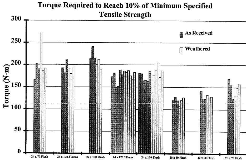
Figure 4.1 Torque required to reach 10% of minimum specified tensile strength
