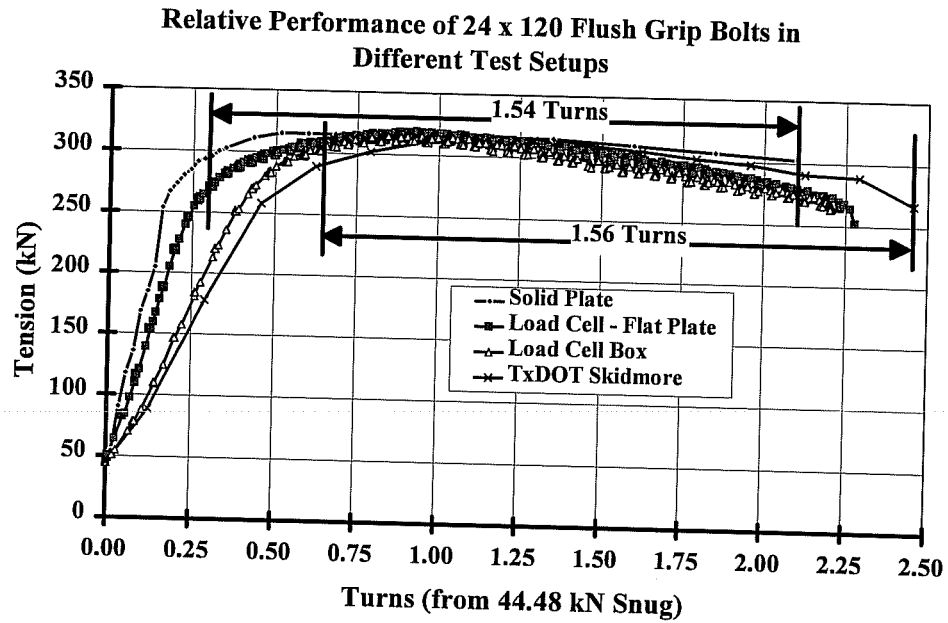
Figure 4. 7 Relative performance of 24 x 120 flush grip bolts in different test setups
