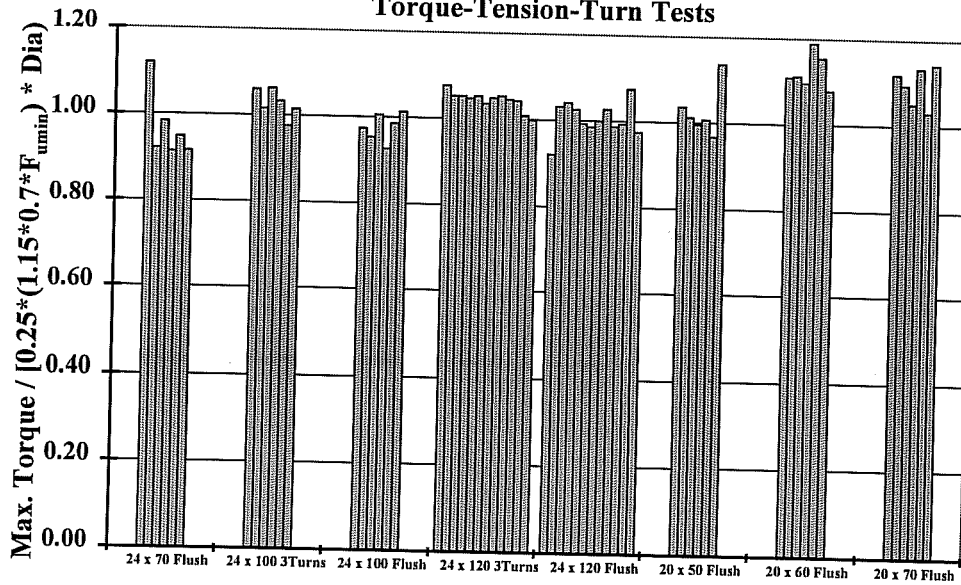
Figure 4. 26 Maximum torque in test/AASHTO maximum allowable torque
