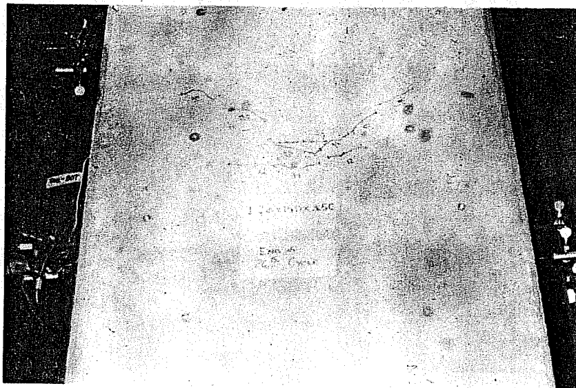
(b) Cracking at end of first set of loading cycles
