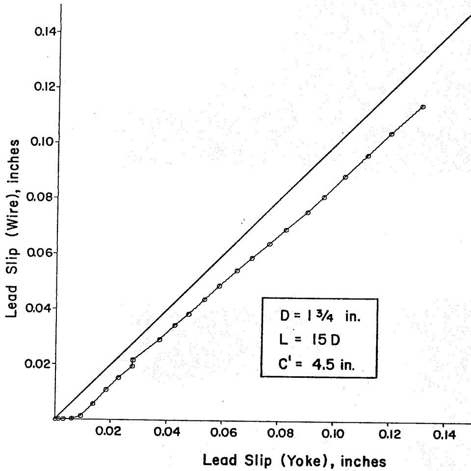
Fig. 4.2 Comparison of lead slip measuring devices-- full-scale tests
