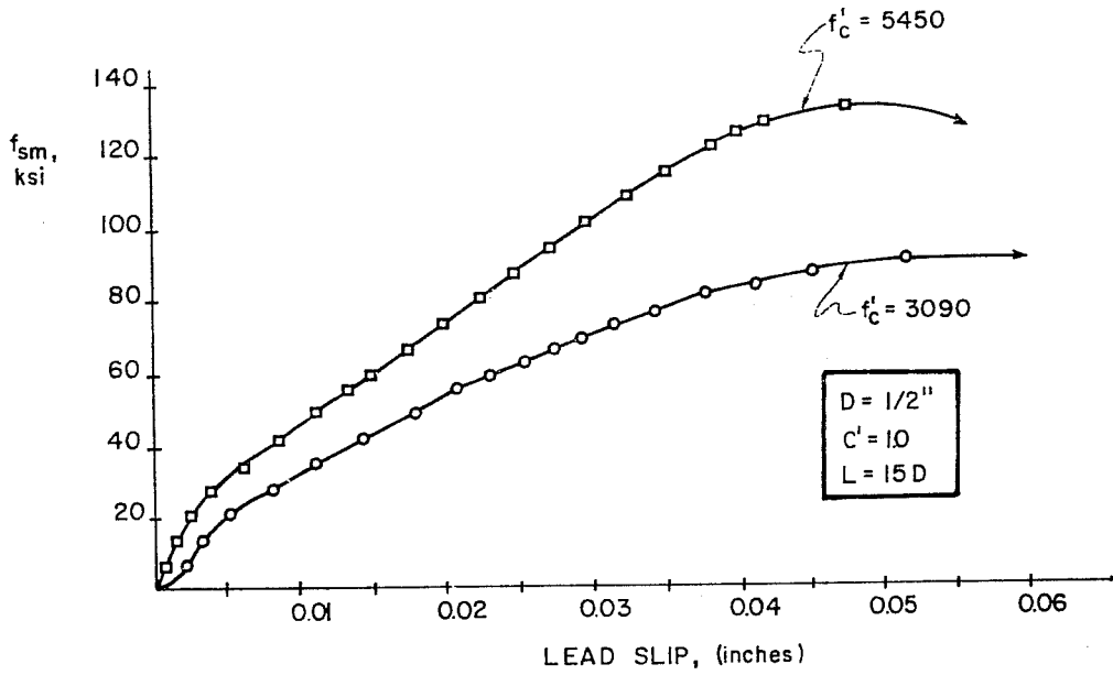
(a) Nonnormalized lead stress-lead slip curves
