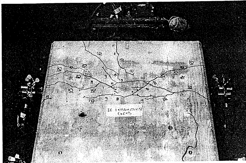
Fig. 6.18 Crack pattern at failure--bolt spacing = 5 in.
