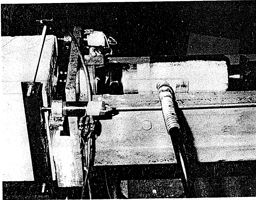
Fig. 3.7 Lead slip measuring device--model tests
