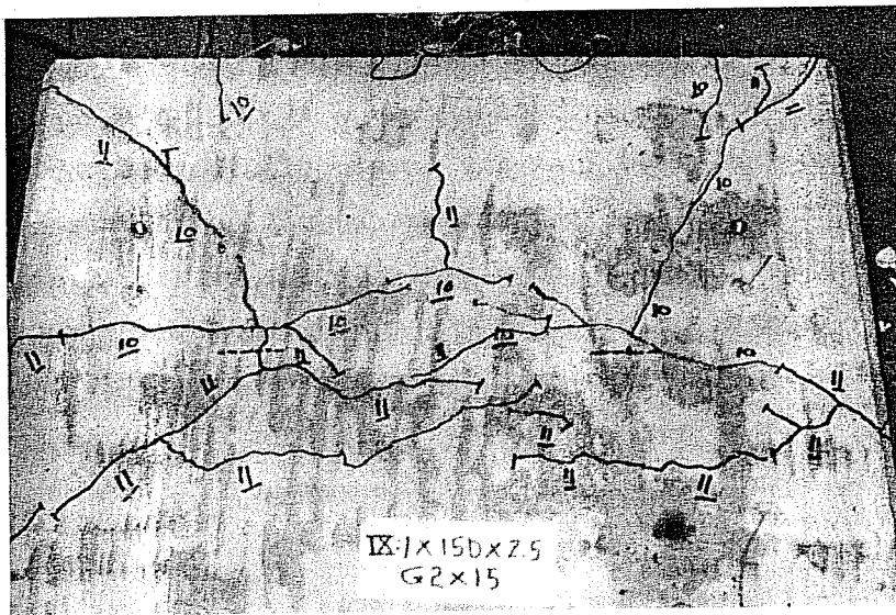
Fig. 6.20 Crack pattern at failure--bolt spacing = 15 in.
