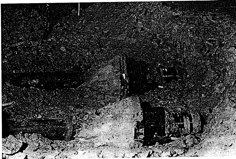
Fig. 6.17 Individual cones of crushed concrete in front of the anchorage devices--bolt spacing = 5 in.
