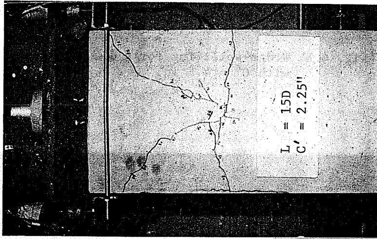
(b) Near failure
