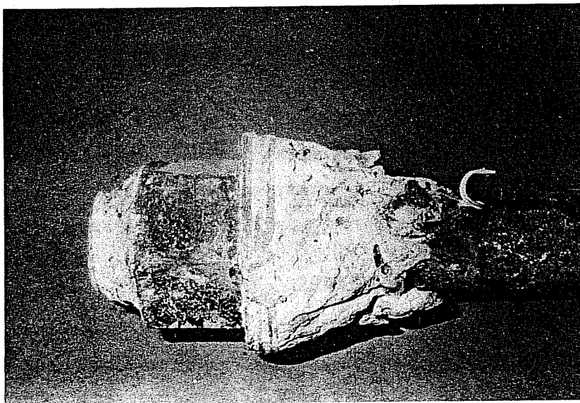
Fig. 4.6 Anchor bolt removed from specimen after failure, showing cone of crushed concrete
