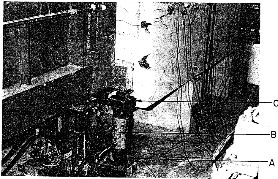
Fig. 2.14 Lateral loading assembly
