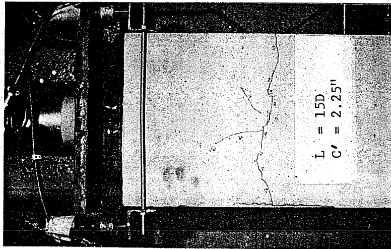
(a) Initial cracking
