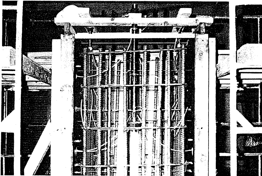
Fig. 2.6 Anchor bolts in form prior to casting
