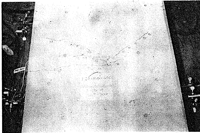
(c) Cracking at end of second set of loading cycles
