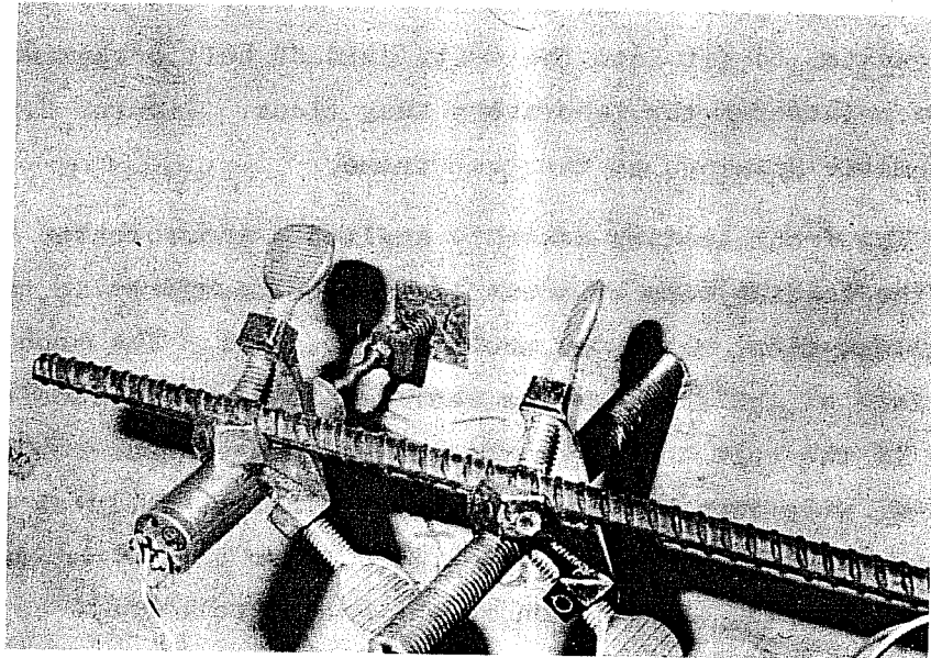
Fig. 2.7 Slip potentiometer mounting
