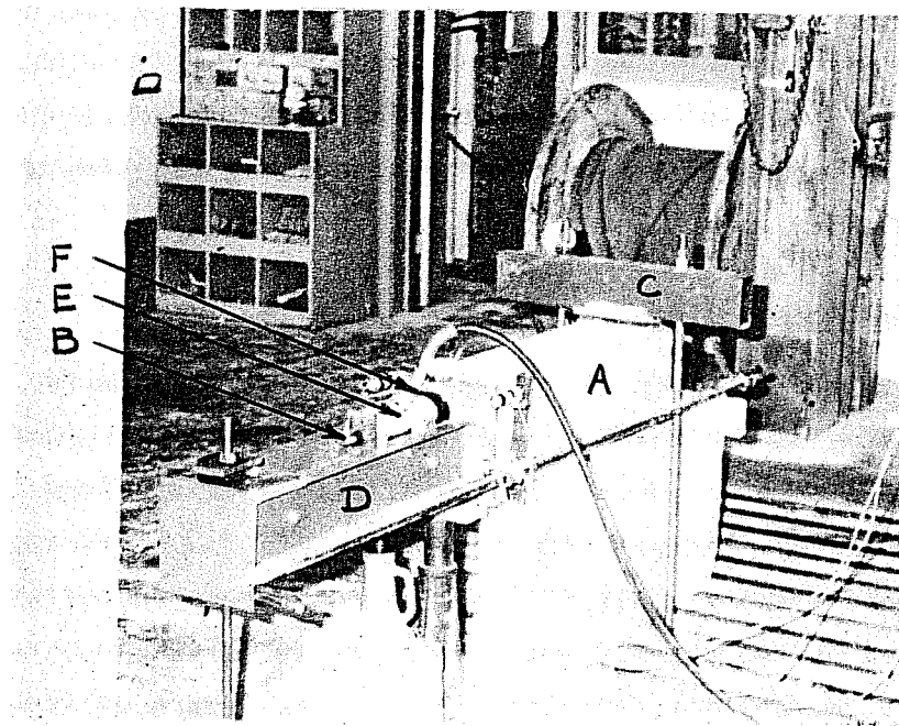
Fig. 3.4 Test setup
