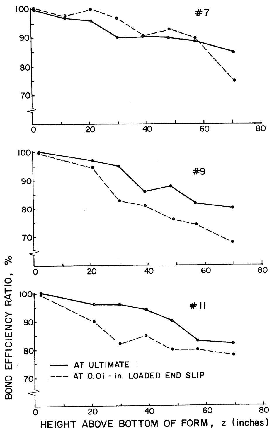
Fig. 2.5 Bond strength reduction--casting position relationship, normal slump (3") specimens
