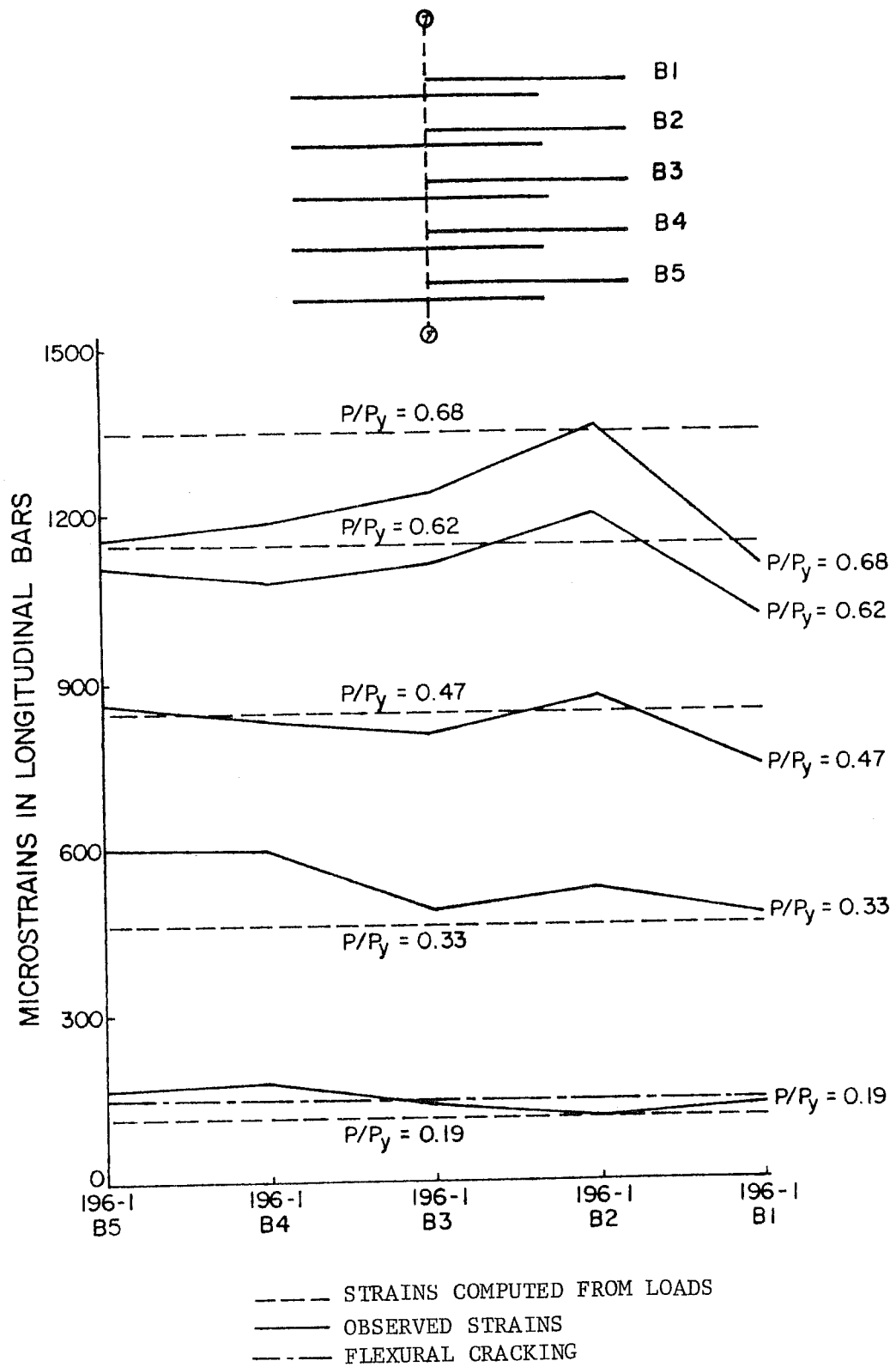
Fig. 2.15 Steel strain distribution across the end of the splice, Test 24
