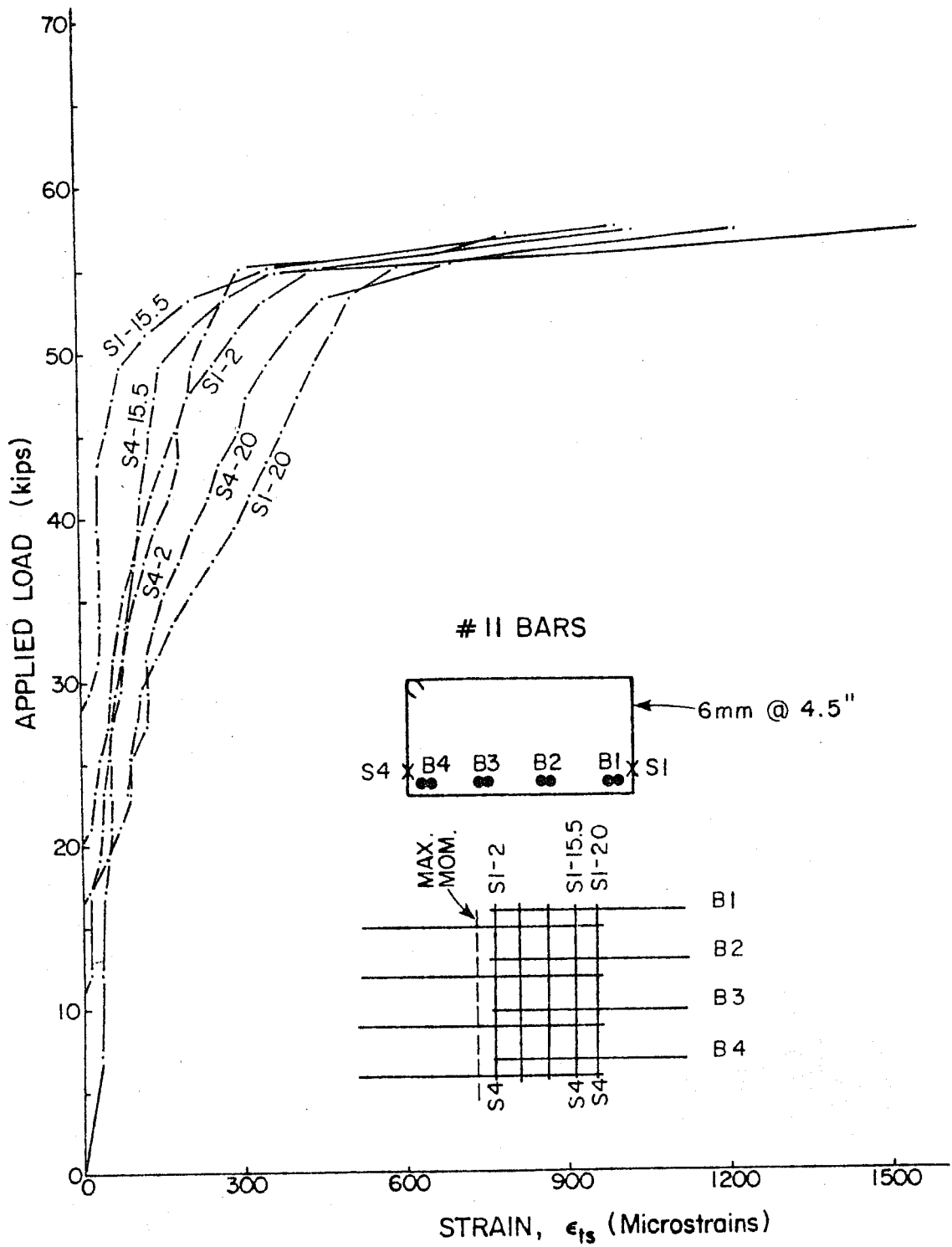
Fig. 2.17 Load vs. strain in stirrups, Test 14, bottom cast, 53-in. shear span
