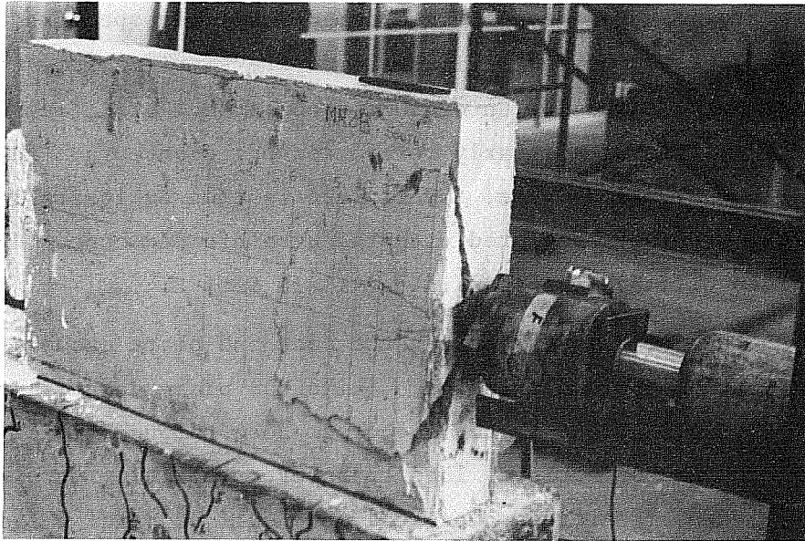
(d) t = 4\text{-}1/2 in., e = 0 in. ultimate failure after cone has been forced 2-1/2 in. into web
