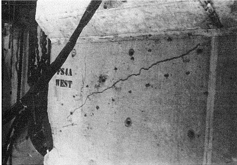
(b) Progression of tendon path crack into anchorage zone with increased load
