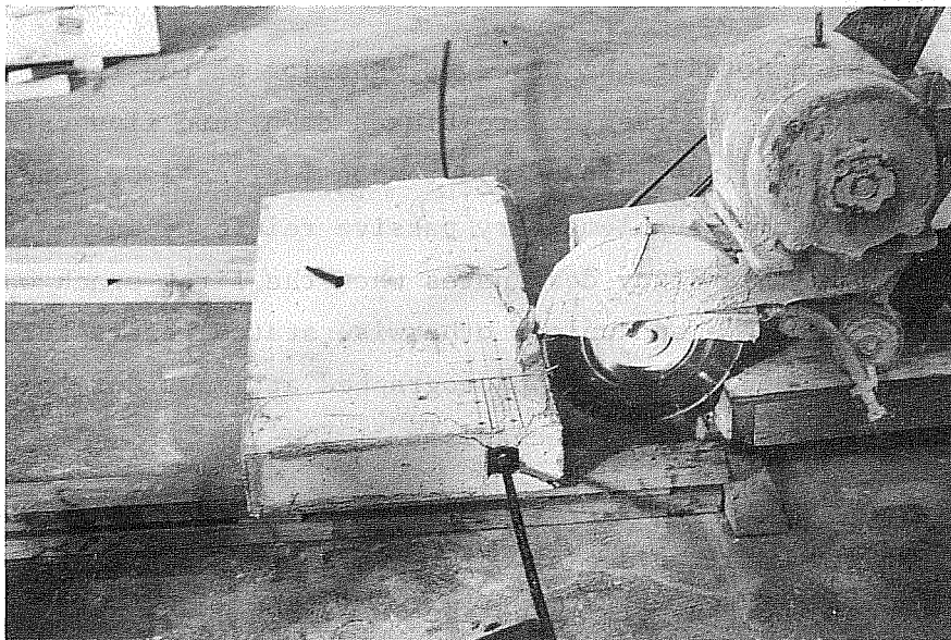
(b) Cutting off destroyed anchorage zone prior to testing of far end
