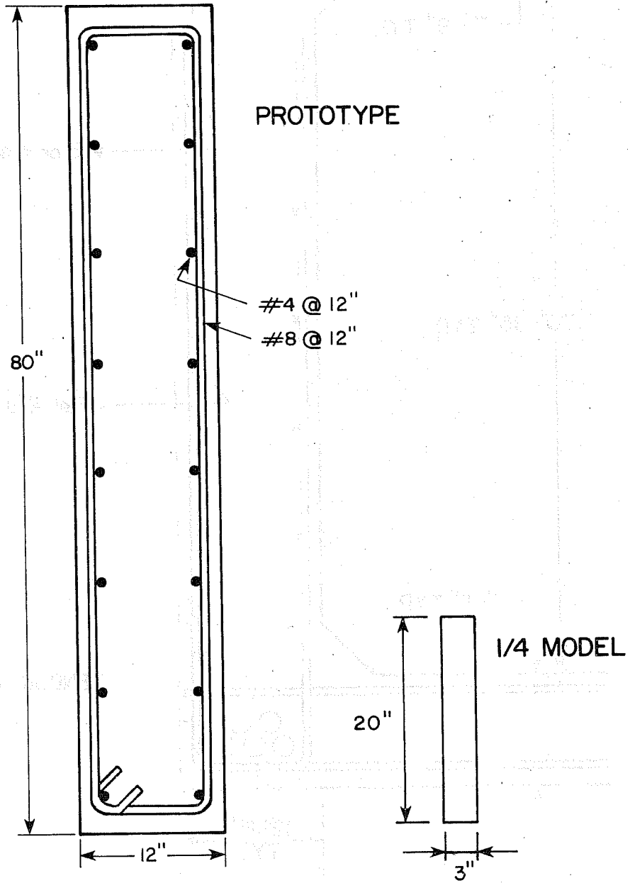
Fig. 2.2 Idealized prototype for rectangular model series
