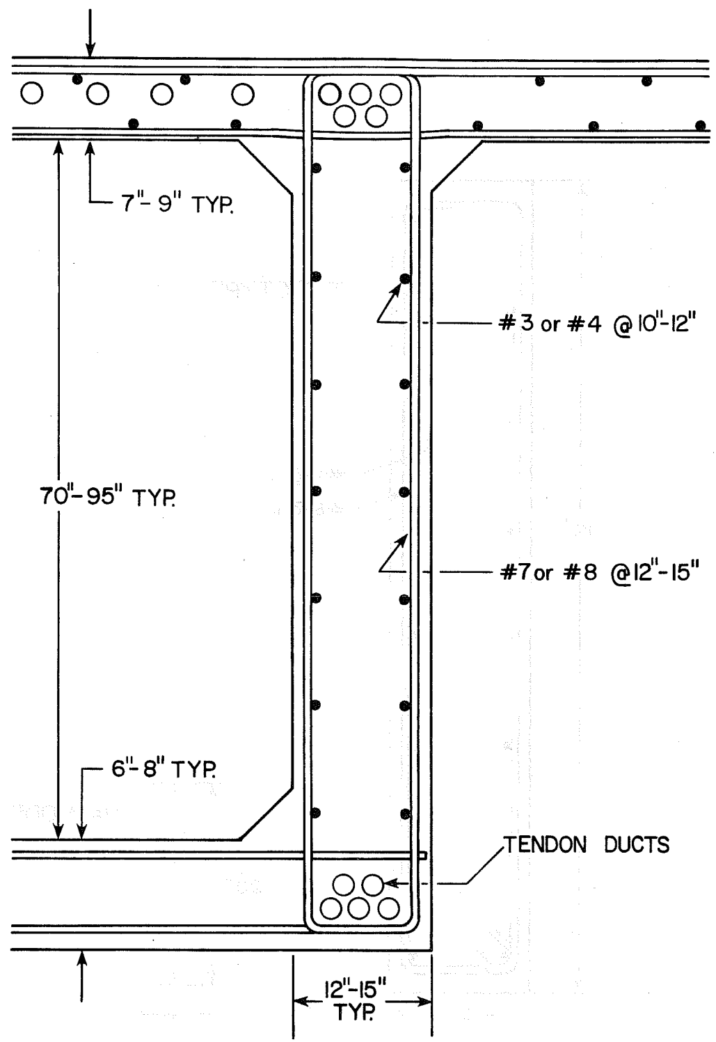
Fig. 2.1 Typical box girder details
