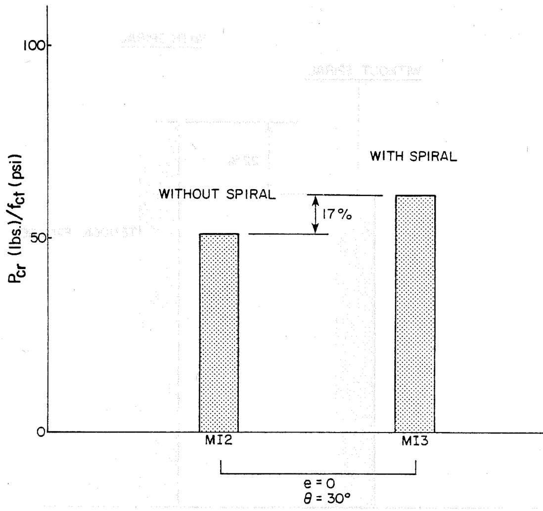
Fig. 4.29 Effect of spiral reinforcement on cracking load
