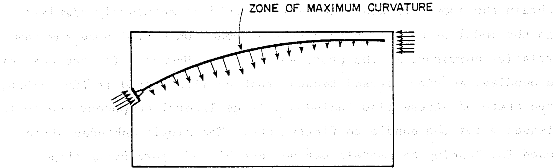
(a) RADIAL FORCES IN THE CONCRETE (ELEVATION)
