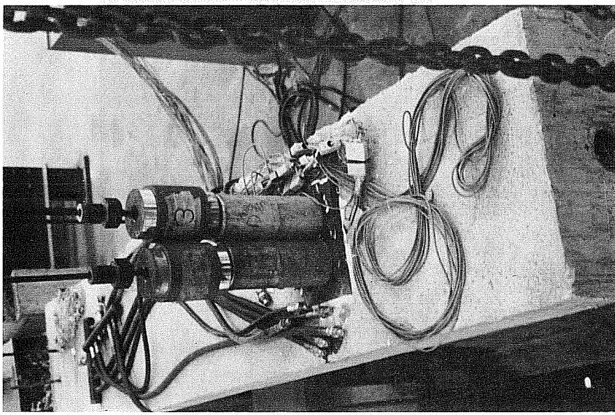
(a) FS5A: location of lateral prestress and stressing system
