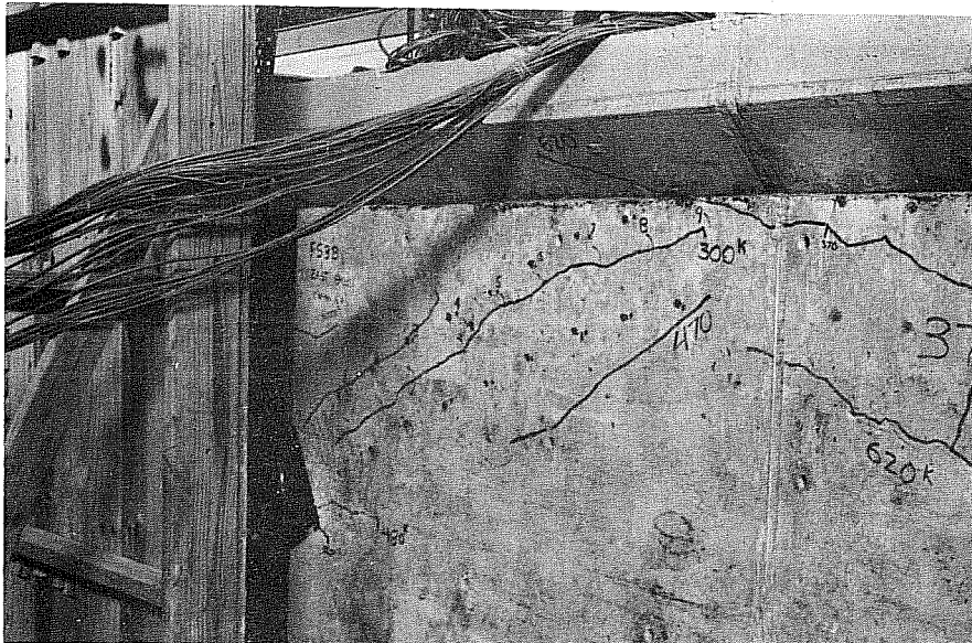
(b) Lower longitudinal crack forms at point of maximum curvature. Upper and lower diagonal cracks form shortly thereafter
