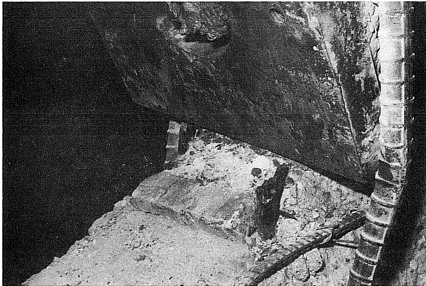
(h) Failure of lateral prestress tendons initiated explosive failure
