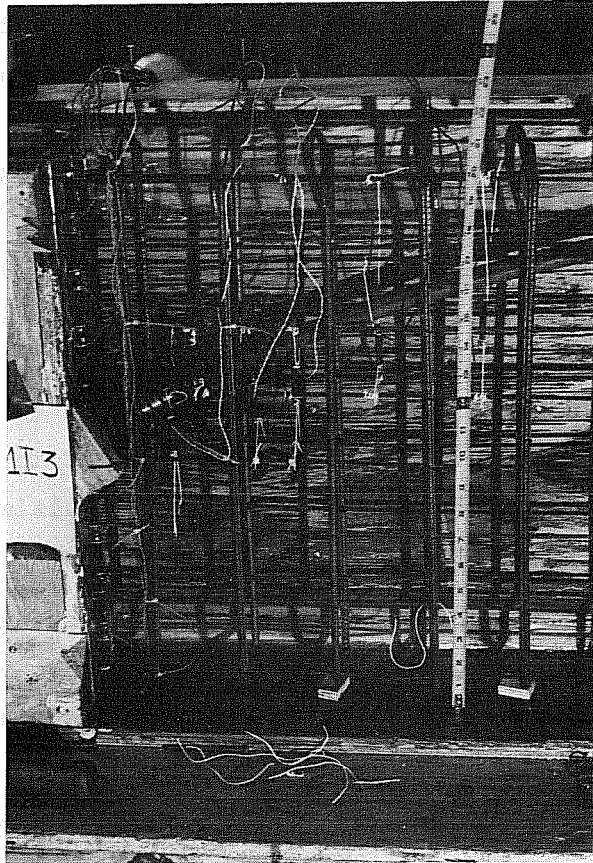
Fig. 4.7 Attachment of curved tendon to end form
