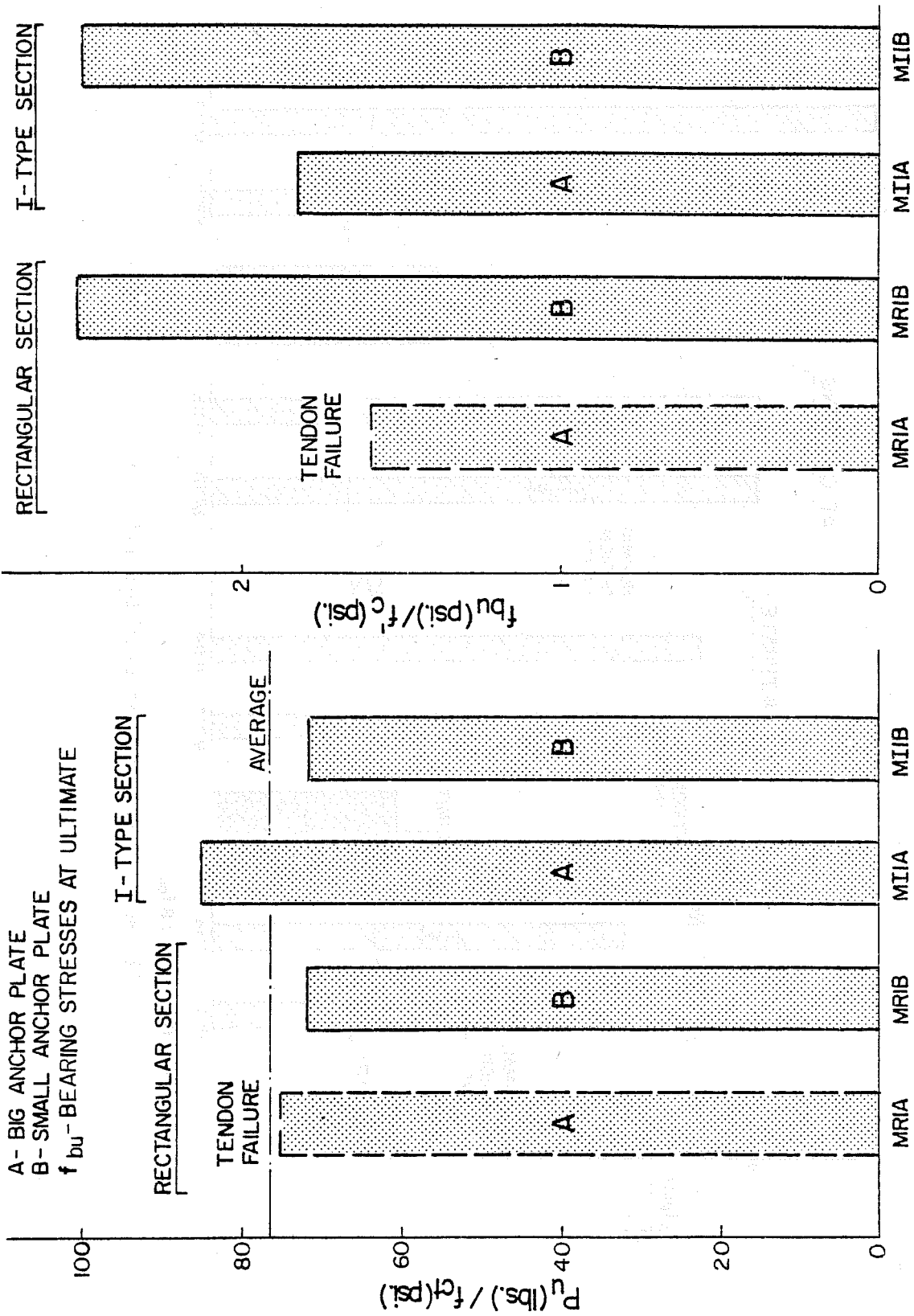
Fig. 4.21 Comparative diagrams of ultimate loads and bearing stresses at ultimate
