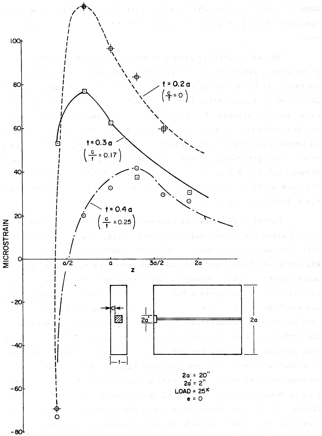
Fig. 2.25 Experimental bursting strain distribution-- cover series
