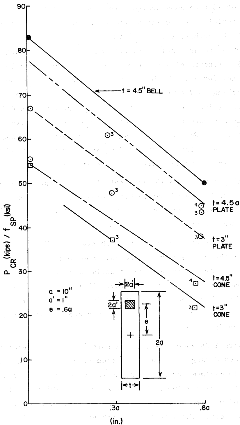
Fig. 2.26 Crack loads normalized to f_{sp} --eccentricity series
