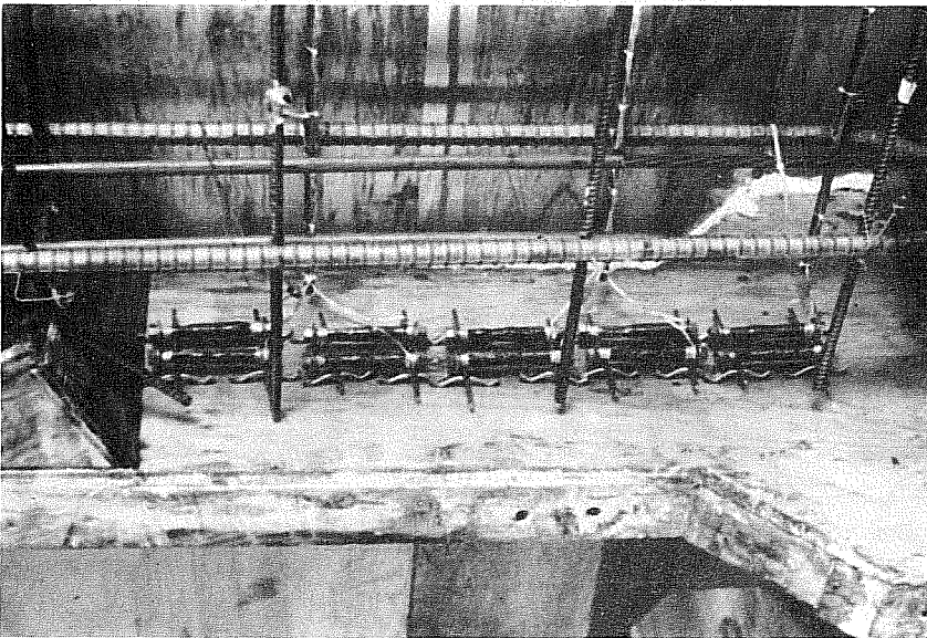
(c) Spalling strainmeters mounted on end form
