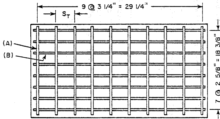
(b) ELEVATION
