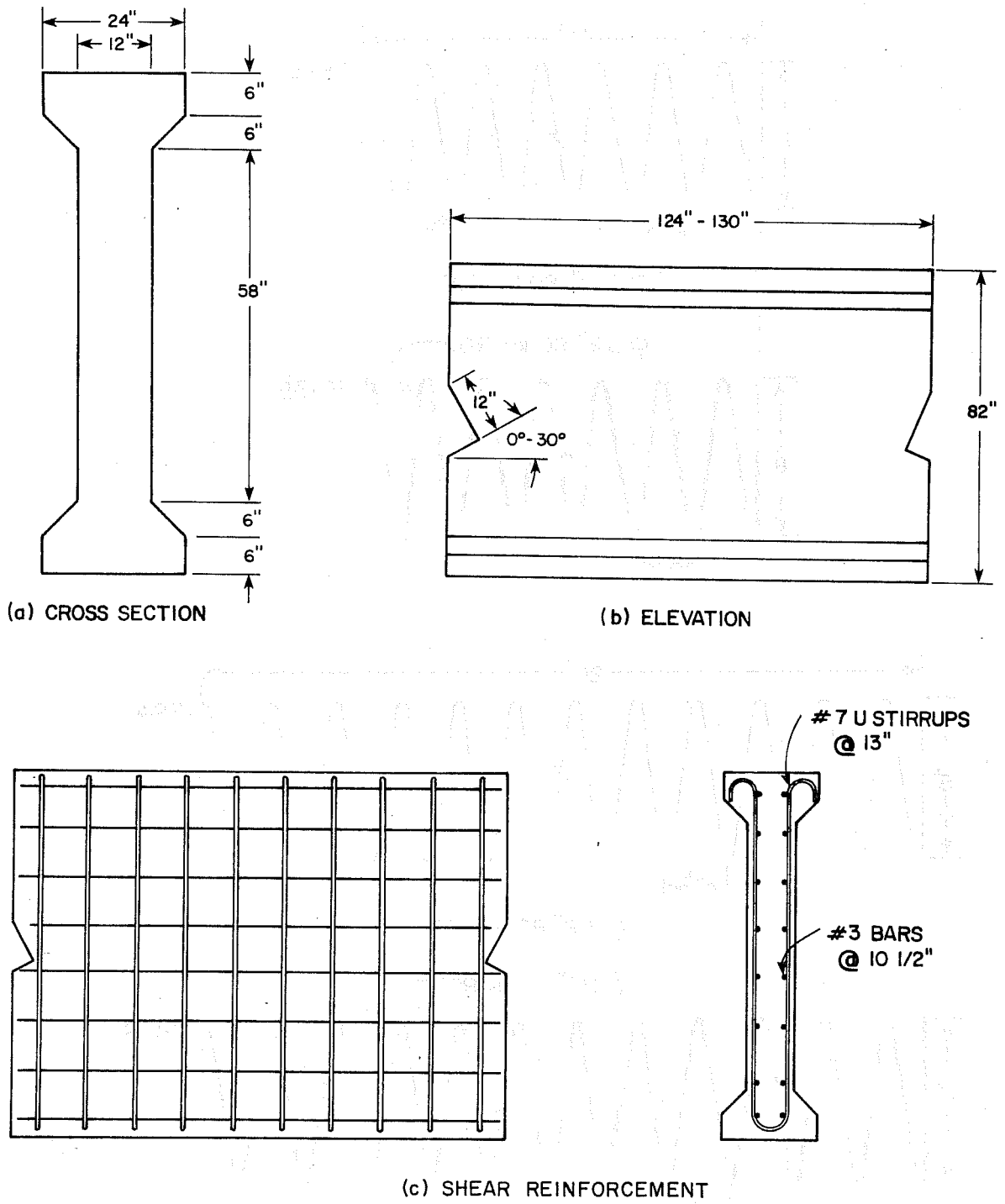
Fig. 3.1 Full-scale specimen details
