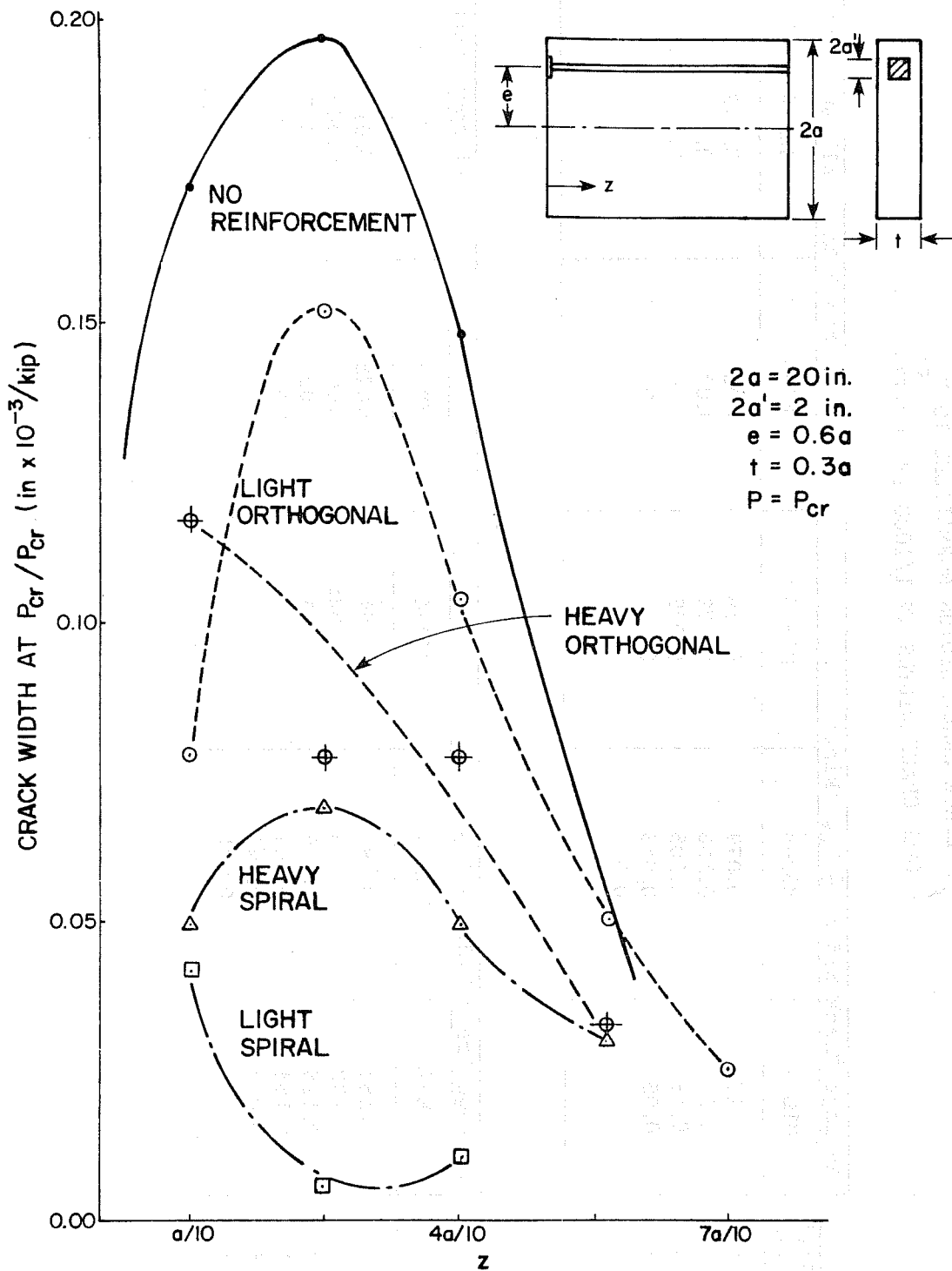
Fig. 2.37 Crack widths normalized to P_{cr} , t = 0.3a
