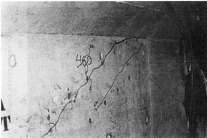
(f) Longitudinal cracks near point of maximum curvature (west side)
