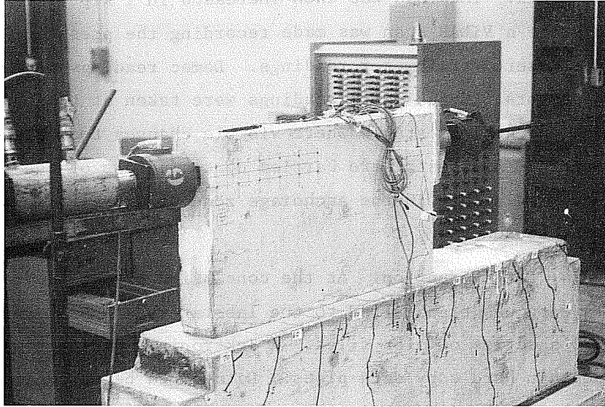
(a) Typical two-sided specimen ready for testing
