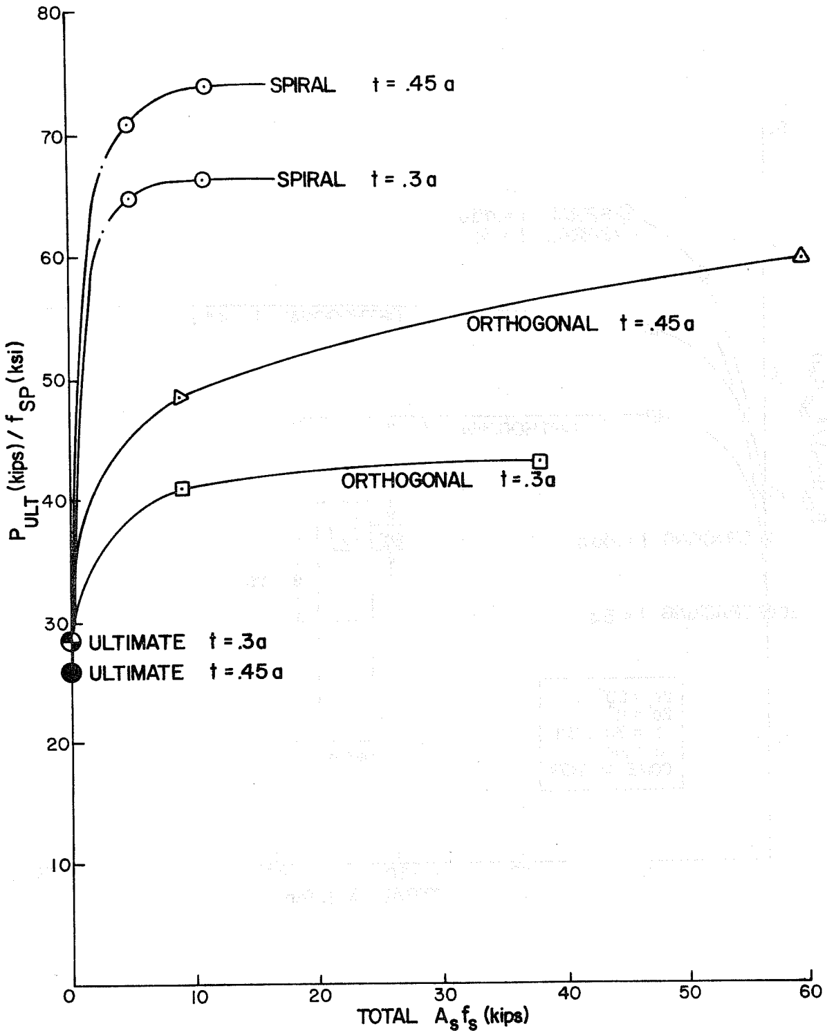
Fig. 2.36 Normalized ultimate loads--reinforcement series
