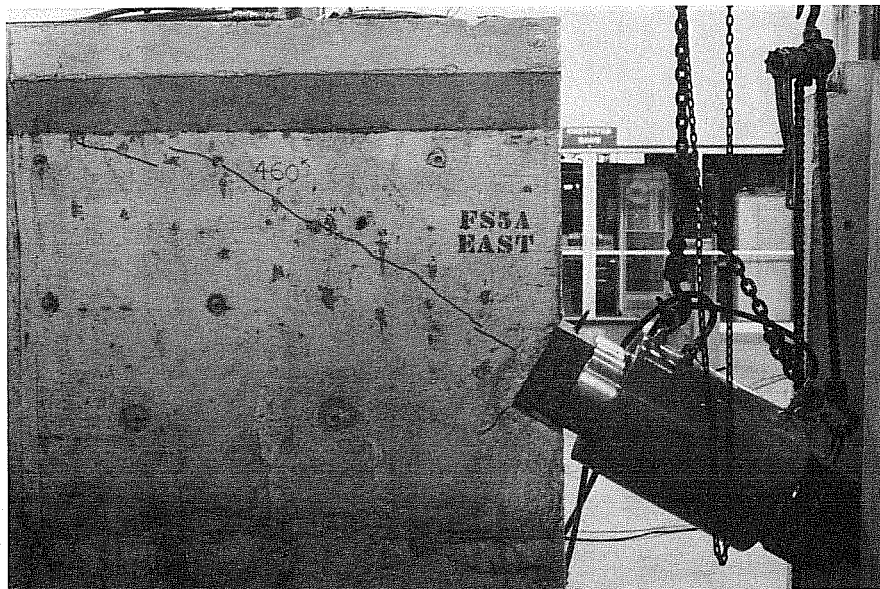
(a) First cracking along tendon path, 460 kips
