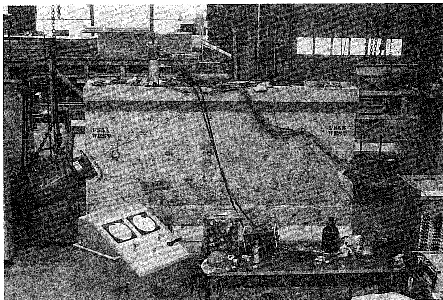
(b) Overall view FS5A showing location of LPT (lateral post-tensioning) jacking system
