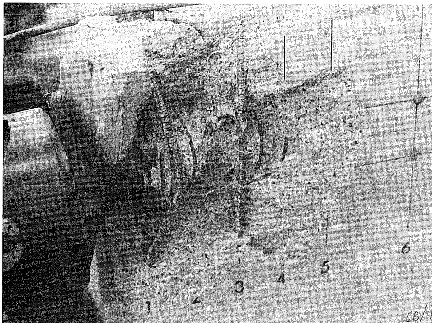
(e) Explosive failure of spiral reinforced cone t = 3 in., e = 0.6a (6 in.)
