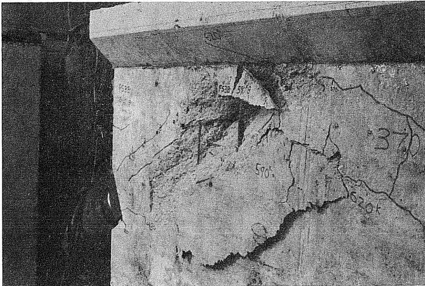
(c) Ultimate load: 590 kips. Side face rupture at point of maximum curvature
