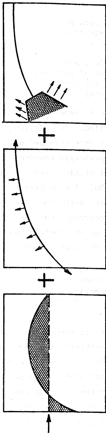
END ZONE BURSTING STRESSES RADIAL FORCES DUE TO TENDON CURVATURE INCLINED WEDGE EFFECT
