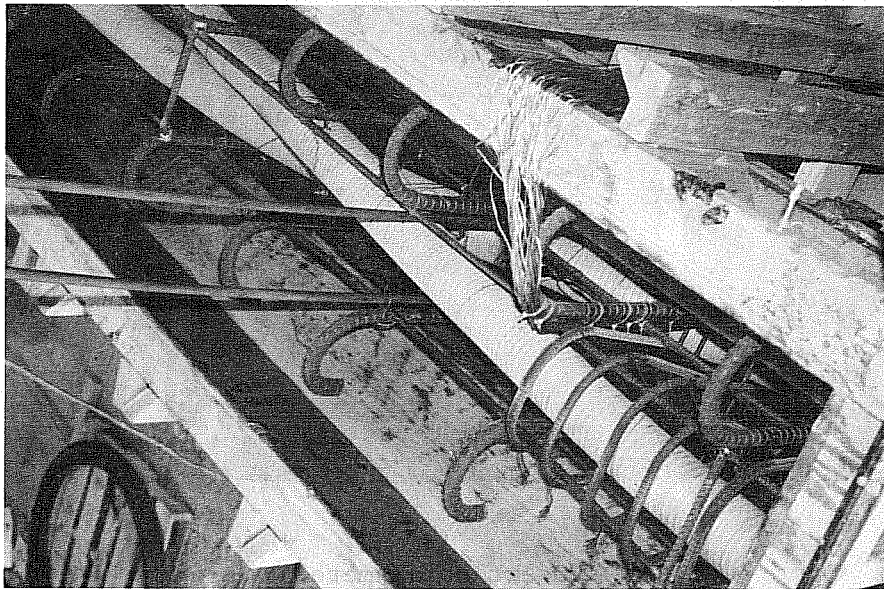
(d) Top view of closed forms showing lateral post-tensioning tendons and primary tendon duct
