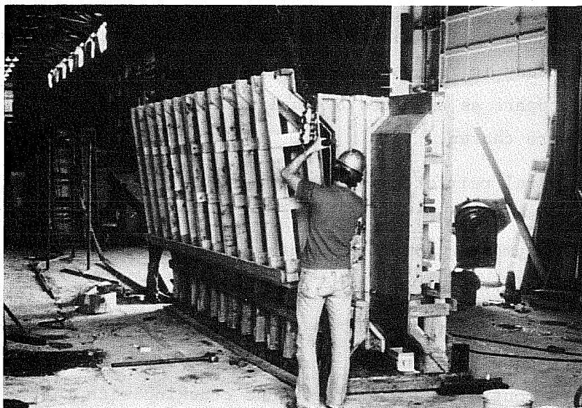
(f) Top of side form lifted into place
