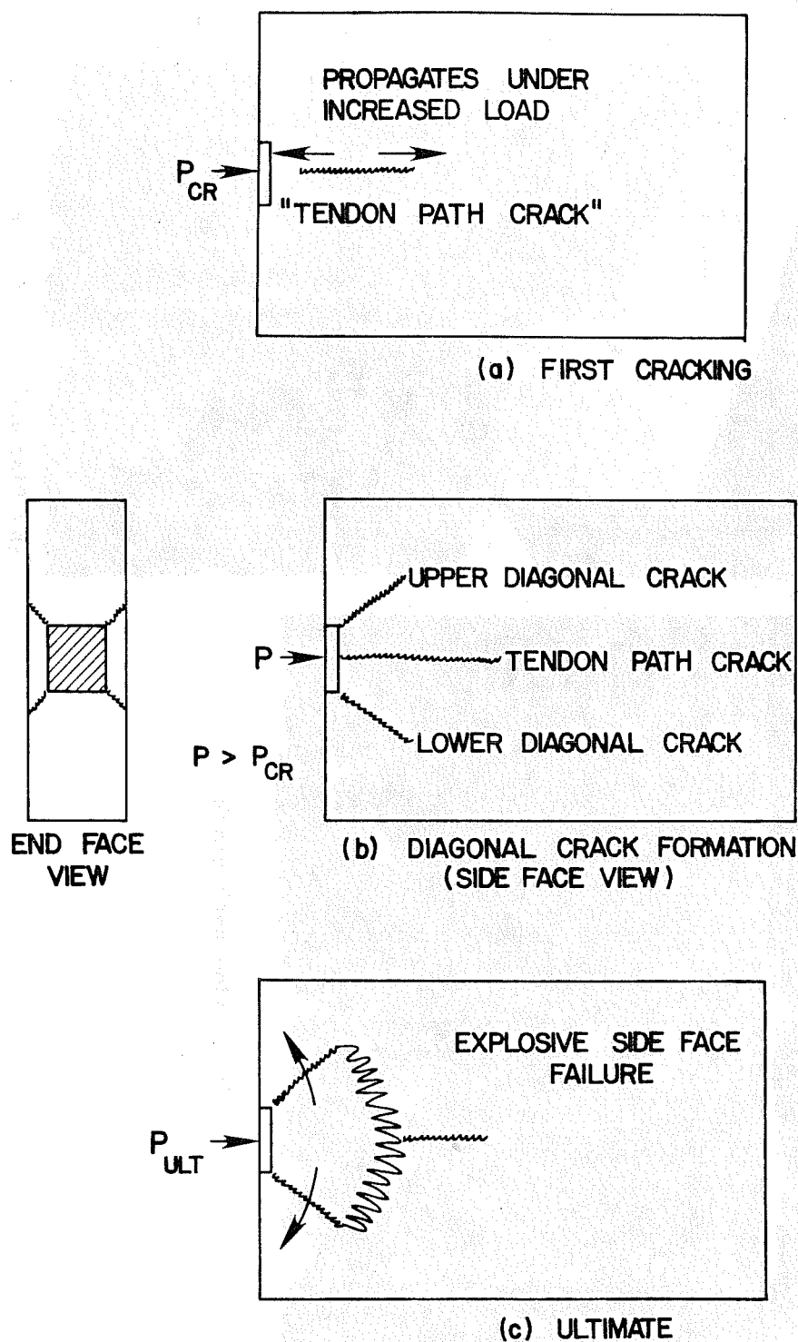
Fig. 2.15 Failure sequence for plate anchors
