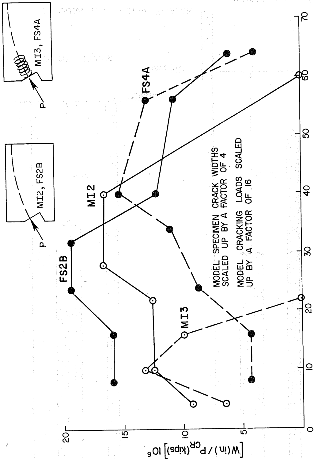
Fig. 4.31 Comparison--full-scale vs model crack widths
