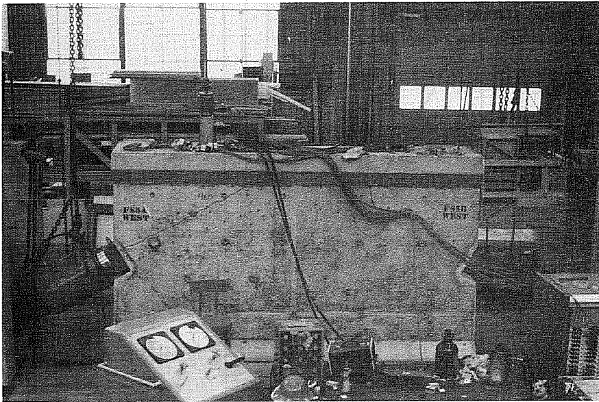
(b) Loading systems
