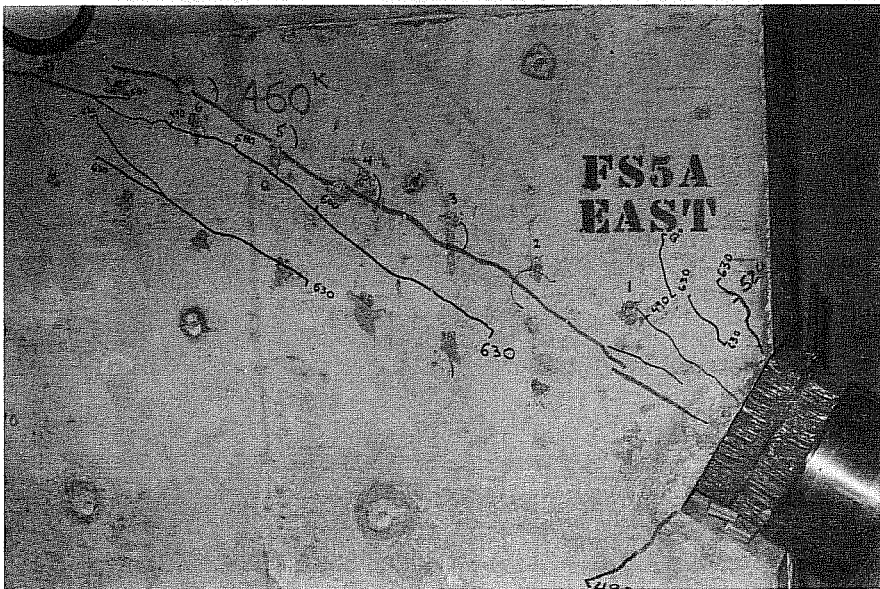
(e) Longitudinal cracks near point of maximum curvature (east side) at 630 kips
