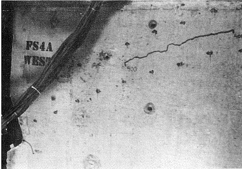
(a) First cracking at point of maximum curvature
