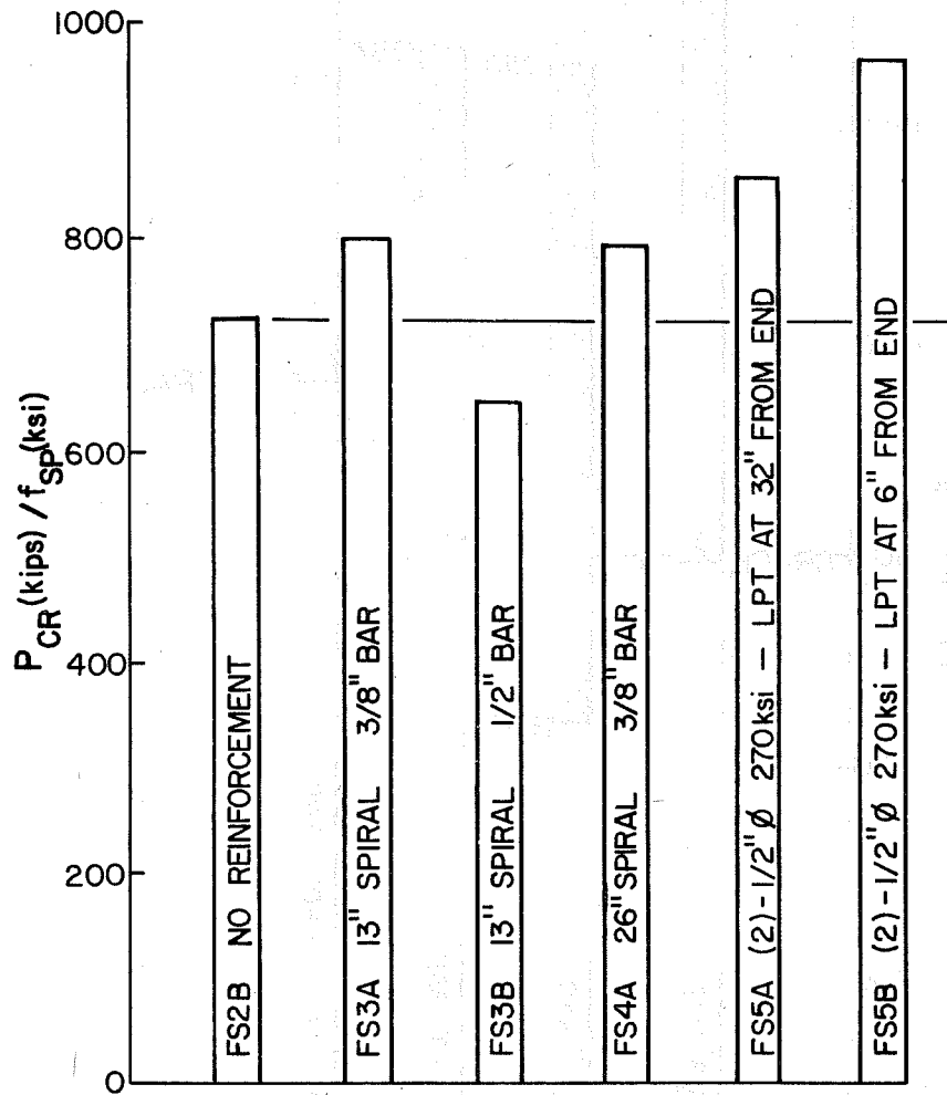
Fig. 3.47 Normalized cracking loads for reinforcement series
