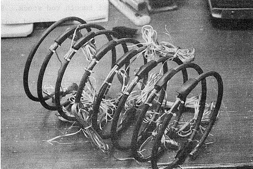
(a) Spirals with strain gages on opposing sides
