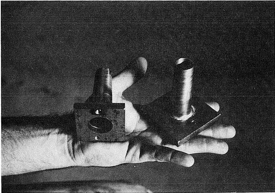
Fig. 4.5 Miniature anchorage hardware
