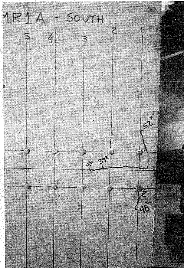
Rectangular Section Large Anchor e = 0; \theta = 0 degrees
