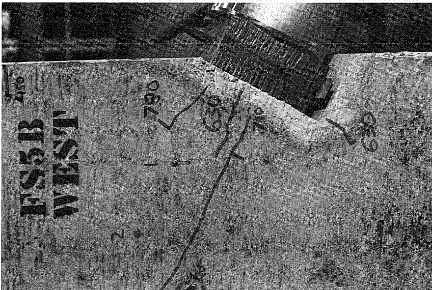
(c) Diagonal cracking, west side
