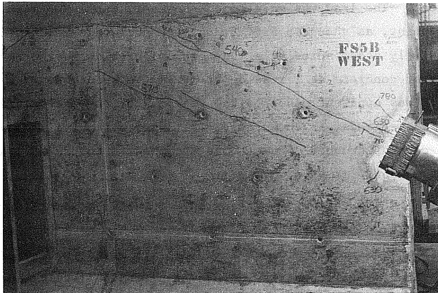
(b) Formation of multiple longitudinal cracks just prior to failure
