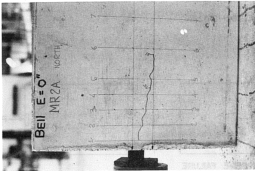
(a) North side--single tendon path crack prior to failure
