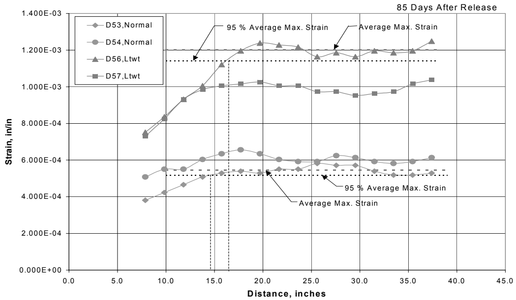
Figure 2.8 Panel Transfer Length Measurements at 85 days
