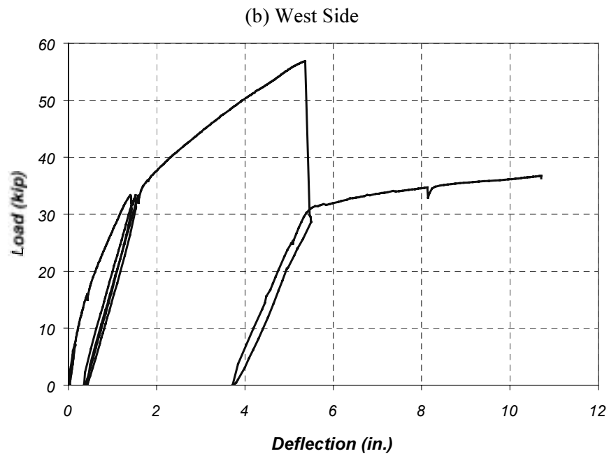
Figure 7.22 Measured Deflections at Midspan in Specimen FS-2
