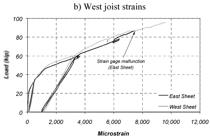
Figure D.19 Measured CFRP Strains in Specimen J-2 (Section N1)
