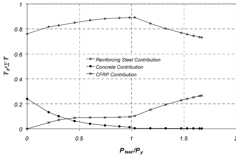
Figure 8.16 Contribution of the CFRP Sheets to the Total Internal Moment at Section N1 for Specimen FS-2
