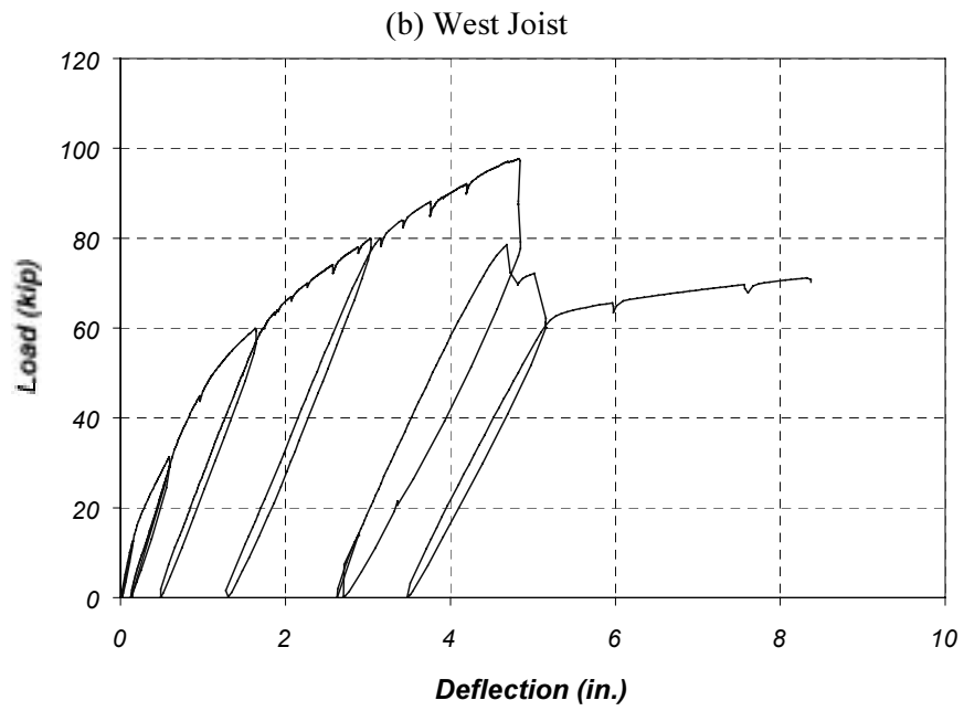
Figure 4.17 Measured Deflections at Midspan in Specimen J-1
