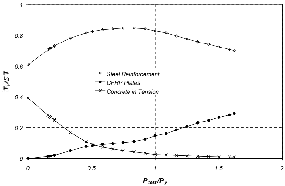
Figure 5.14 Variation of Tensile Force Components at Section N1 for Specimen J-1
