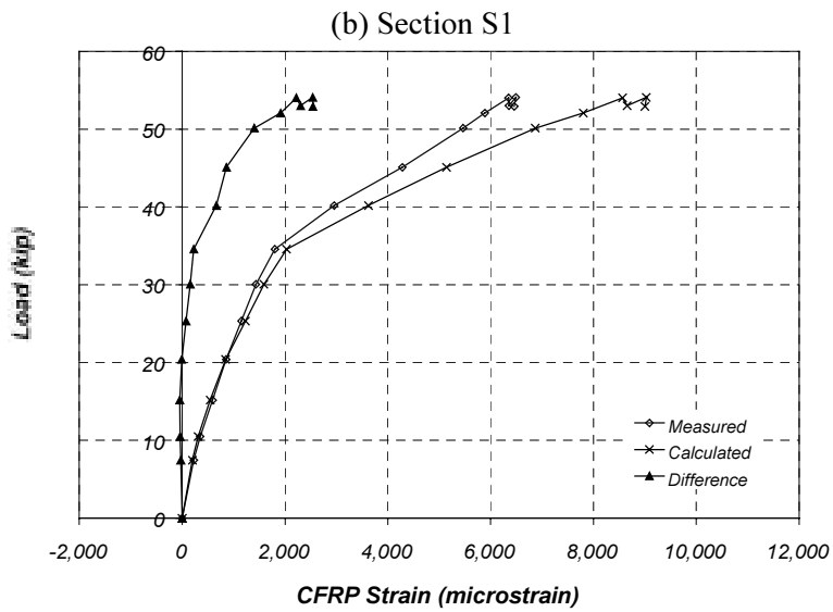
Figure 8.7 Comparison of Measured and Calculated CFRP Strains for Specimen FS-1
