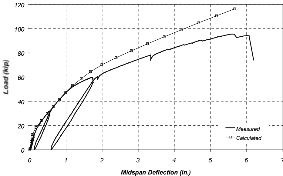
Figure 5.27 Comparison of Measured and Calculated Load-Deflection Response of Specimen J-2
