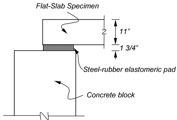
Support Detail
