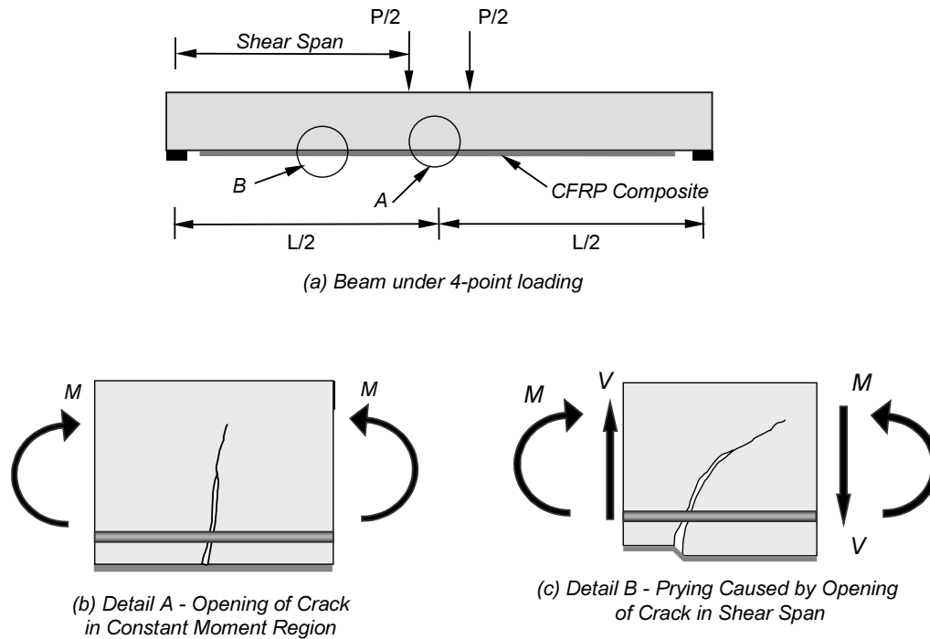
Figure 1.2 Prying Action Observed on CFRP Composite Attached to the Bottom Surface of the Beams
