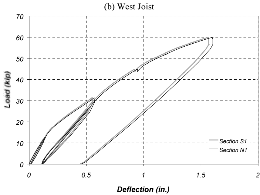
Figure 4.16 Measured Deflections at Sections N1 and S1 in Specimen J-1
