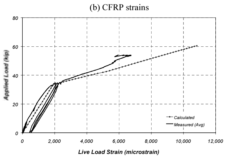
Figure 8.3 Comparison of Measured and Calculated Live-Load Strains at Section N1 (Specimen FS-1)
