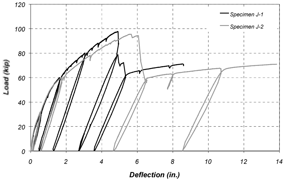
Figure 5.23 Measured Load-Deflection Response of Pan-Girder Specimens
