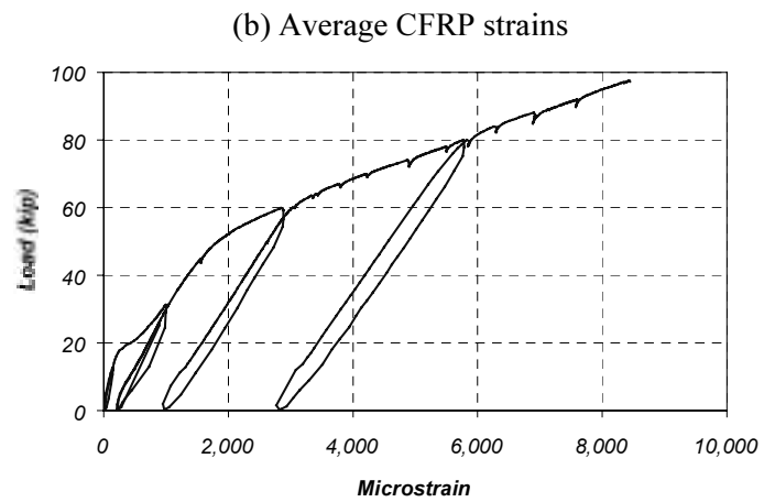
Figure 4.23 Average Strains Measured at Section N1 (Specimen J-1)
