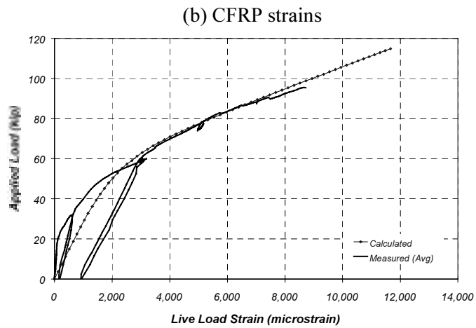
Figure 5.5 Comparison of Measured and Calculated Live-Load Strains at Section N1 (Specimen J-2)
