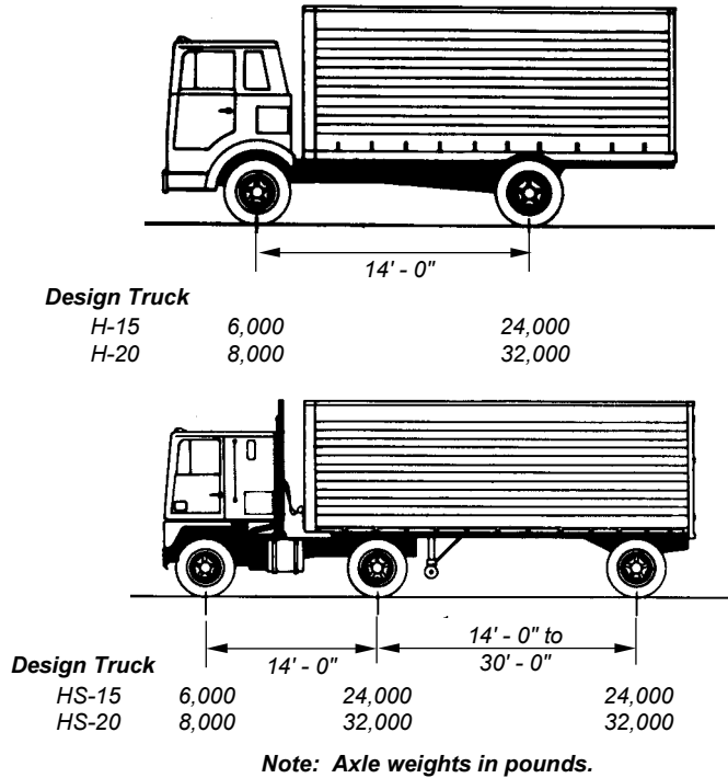
Figure B.1 Design Trucks used for Bridge Load Rating
