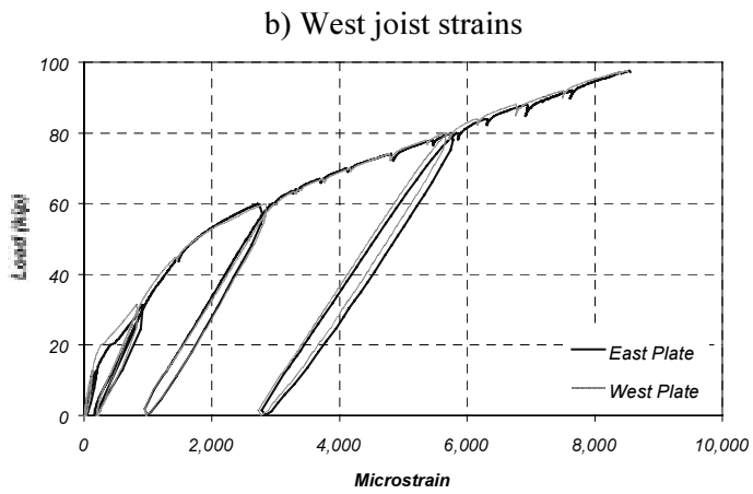
Figure D.7 Measured CFRP Strains in Specimen J-1 (Section N1)
