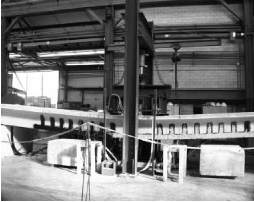
Figure 4.13 View of West Joist in Specimen J-2 at Failure
