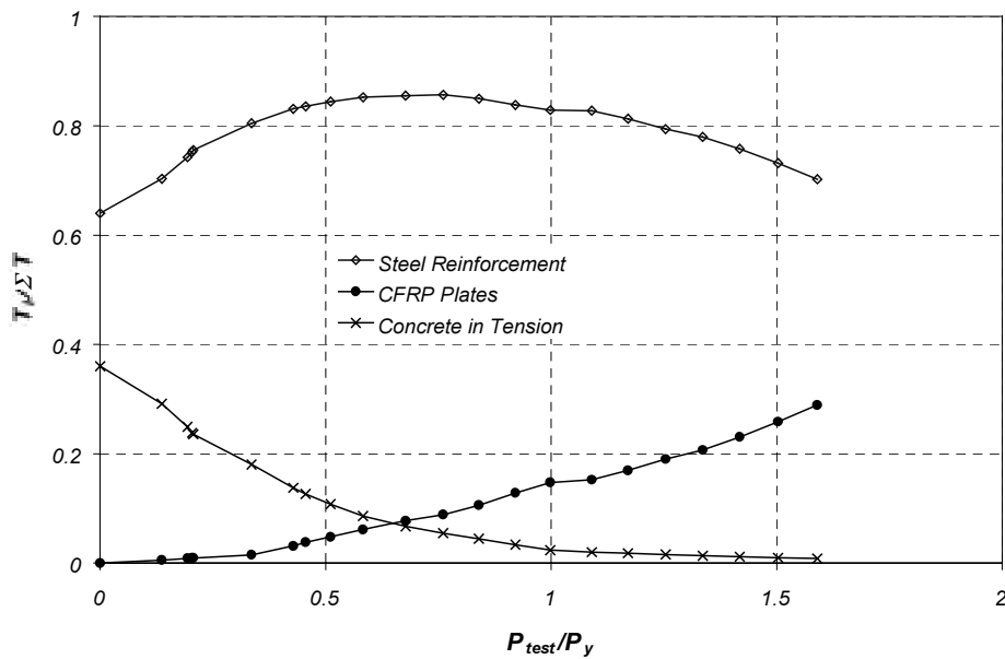
Figure 5.19 Contribution of the CFRP Sheets to the Total Internal Moment at Section N1 for Specimen J-2
