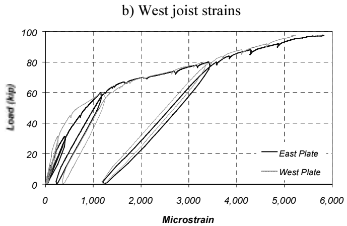
Figure D.9 Measured CFRP Strains in Specimen J-1 (Section N2)
