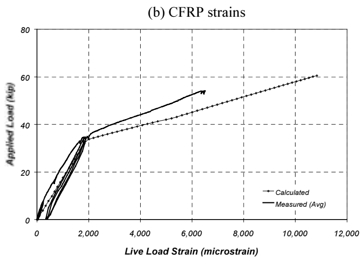
Figure 8.4 Comparison of Measured and Calculated Live-Load Strains at Section S1 (Specimen FS-1)
