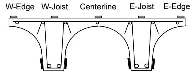
c) Location of strain gages
