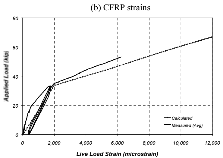
Figure 8.6 Comparison of Measured and Calculated Live-Load Strains at Section S1 (Specimen FS-2)
