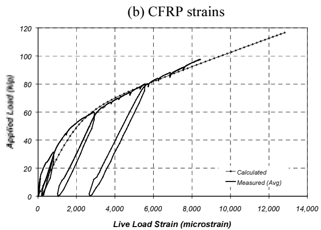
Figure 5.4 Comparison of Measured and Calculated Live-Load Strains at Section S1 (Specimen J-1)
