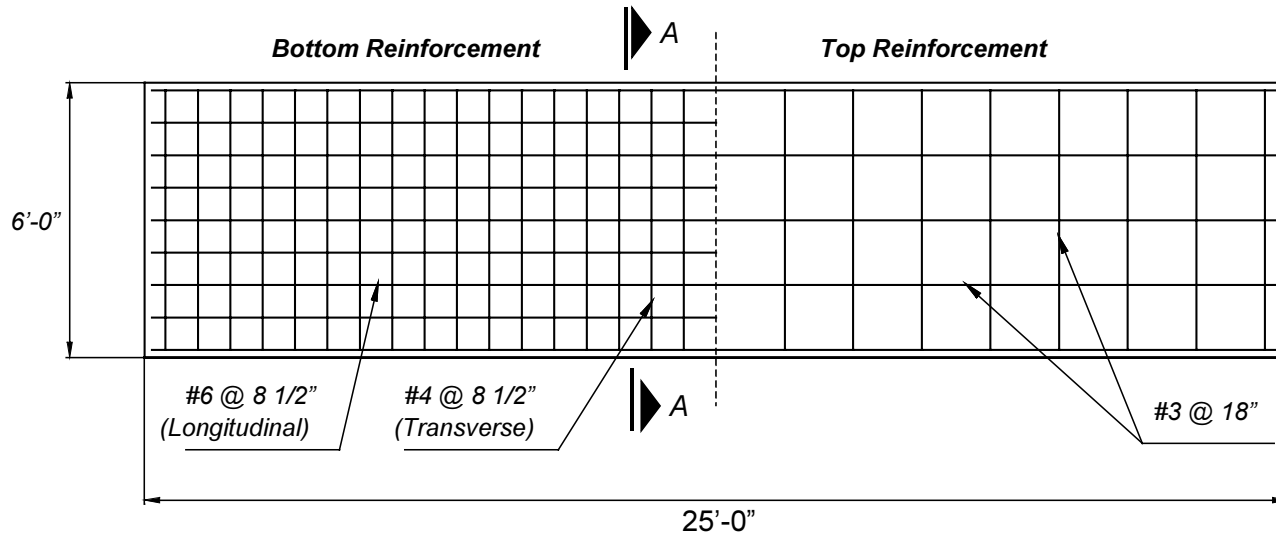
Steel Reinforcement Details (Plan)
