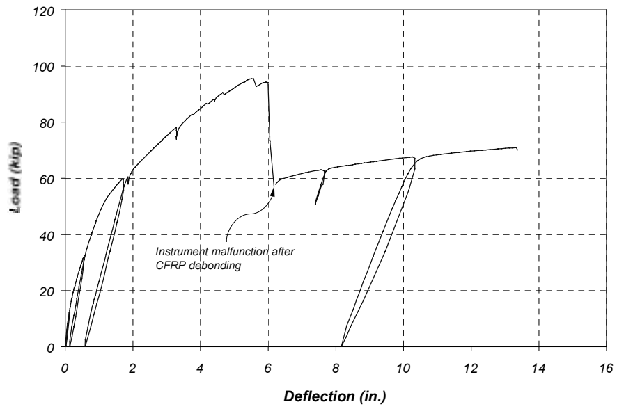
Figure 4.20 Measured Midspan Deflections in Specimen J-2
