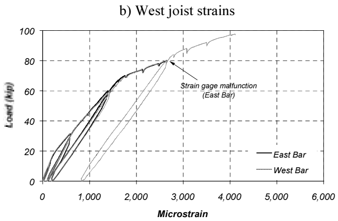
Figure D.5 Measured #8 Reinforcing Bar Strains in Specimen J-1 (Section N2)
