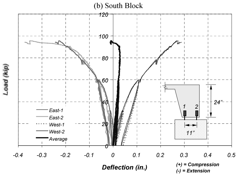
Figure 4.18 Measured Displacements at Supports in Specimen J-2
