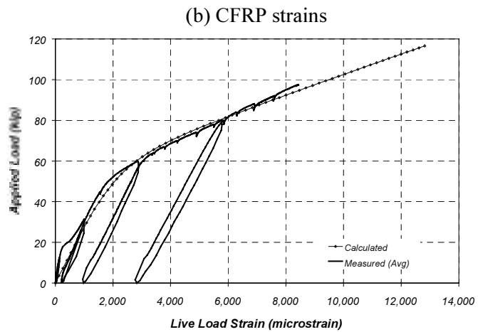
Figure 5.3 Comparison of Measured and Calculated Live-Load Strains at Section N1 (Specimen J-1)
