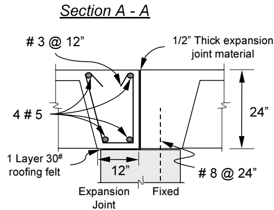
Figure 3.3 Reinforcement Details for Prototype Bridge
