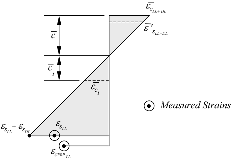
Figure 5.11 Possible Strain Distribution Corresponding to Equilibrium of Internal Forces
