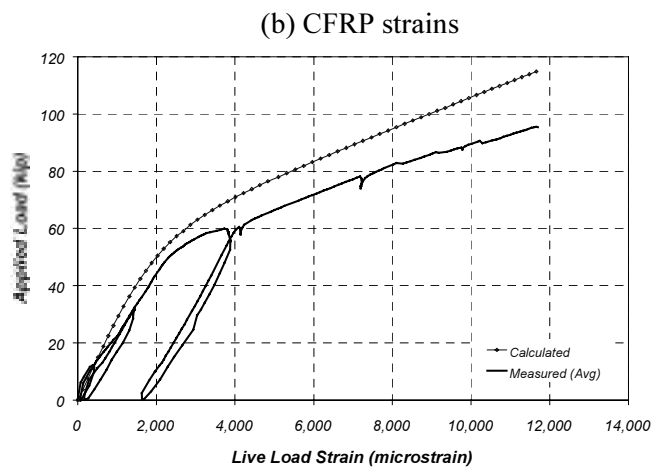
Figure 5.6 Comparison of Measured and Calculated Live-Load Strains at Section S1 (Specimen J-2)
