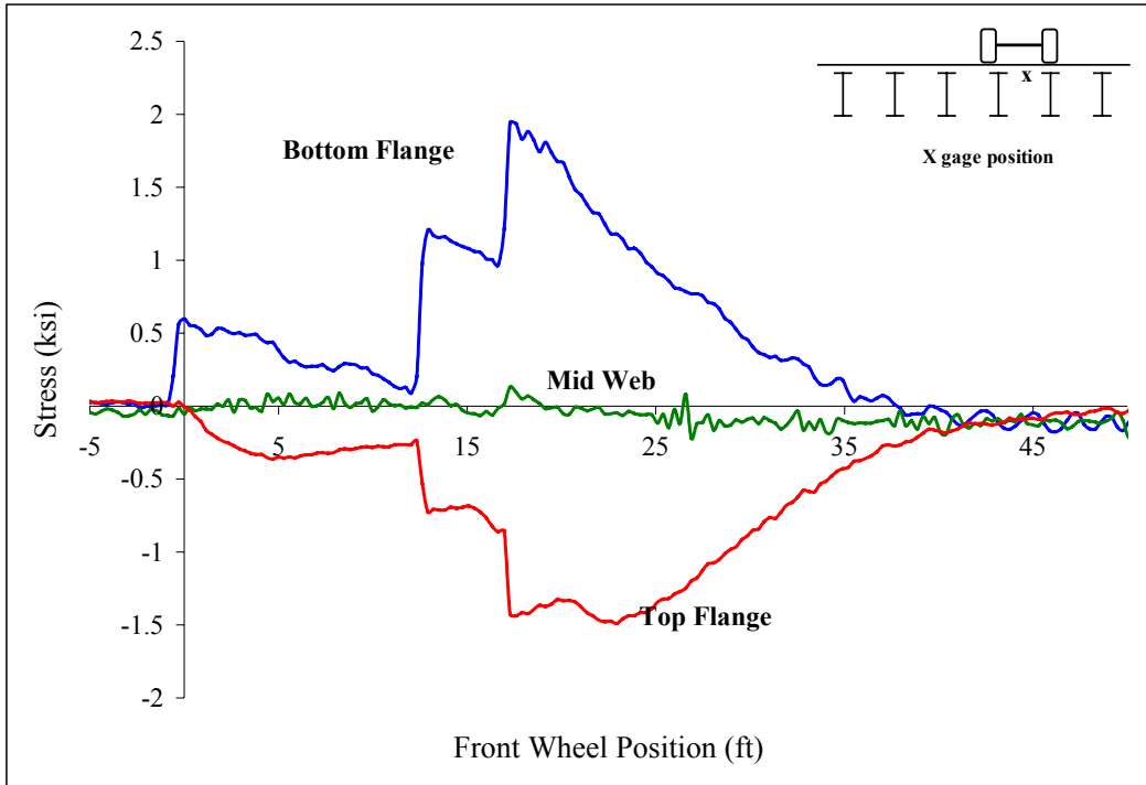
Figure B 44: Beam 1
