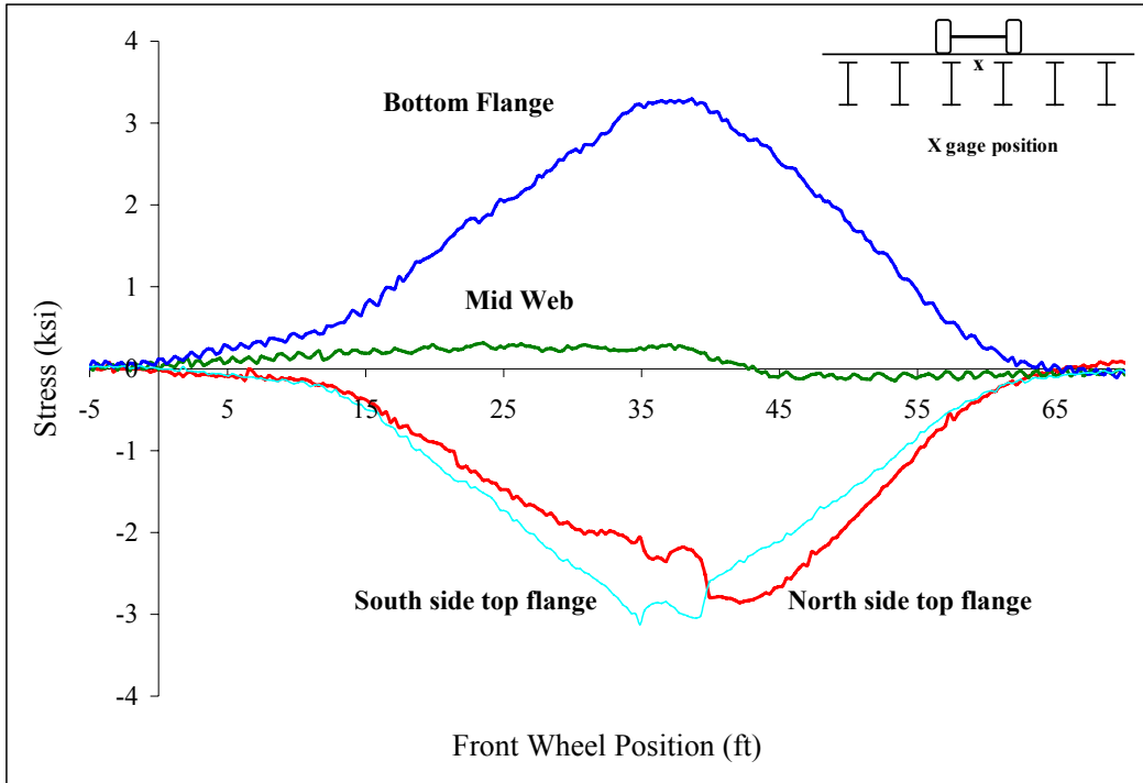
Figure A 20: Beam 2
