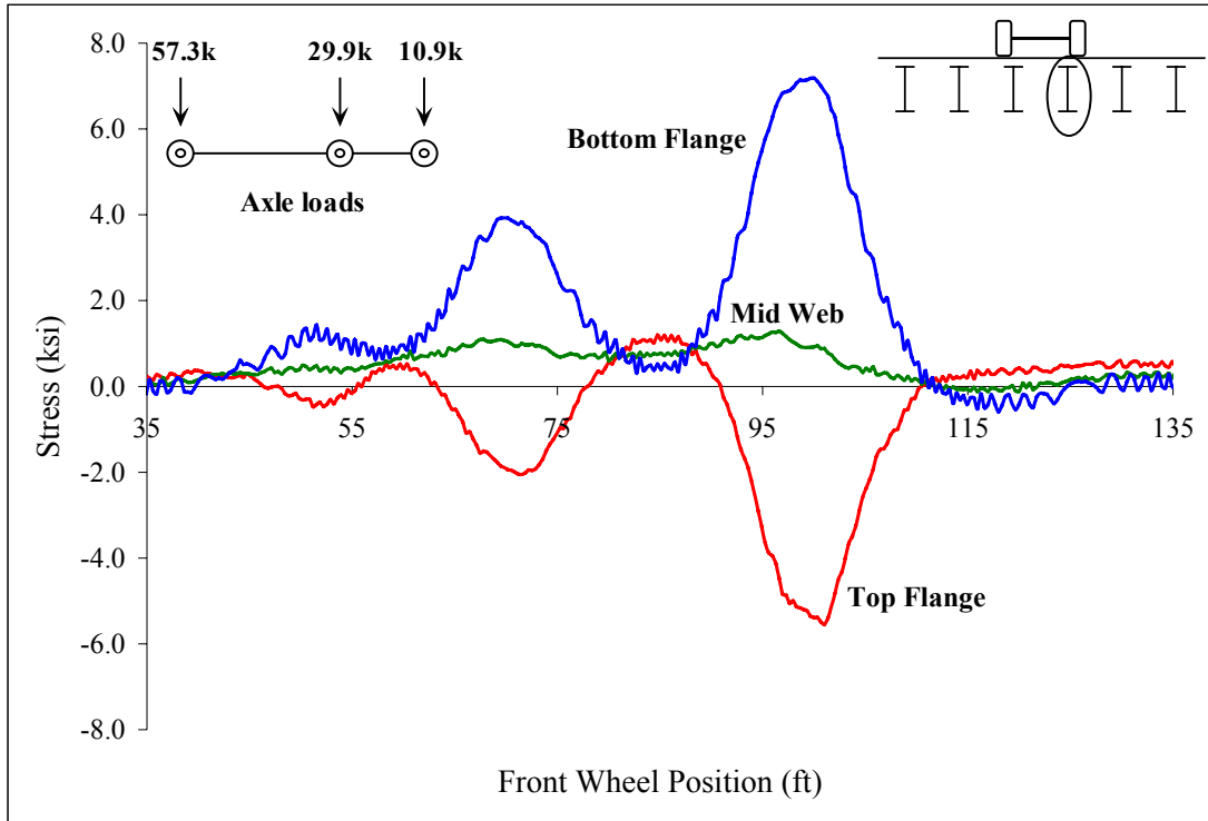
Figure C 64: Midspan stringer 4
