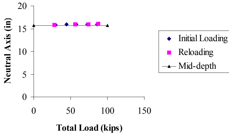
Figure 6.48 West beam: load vs. neutral axis
