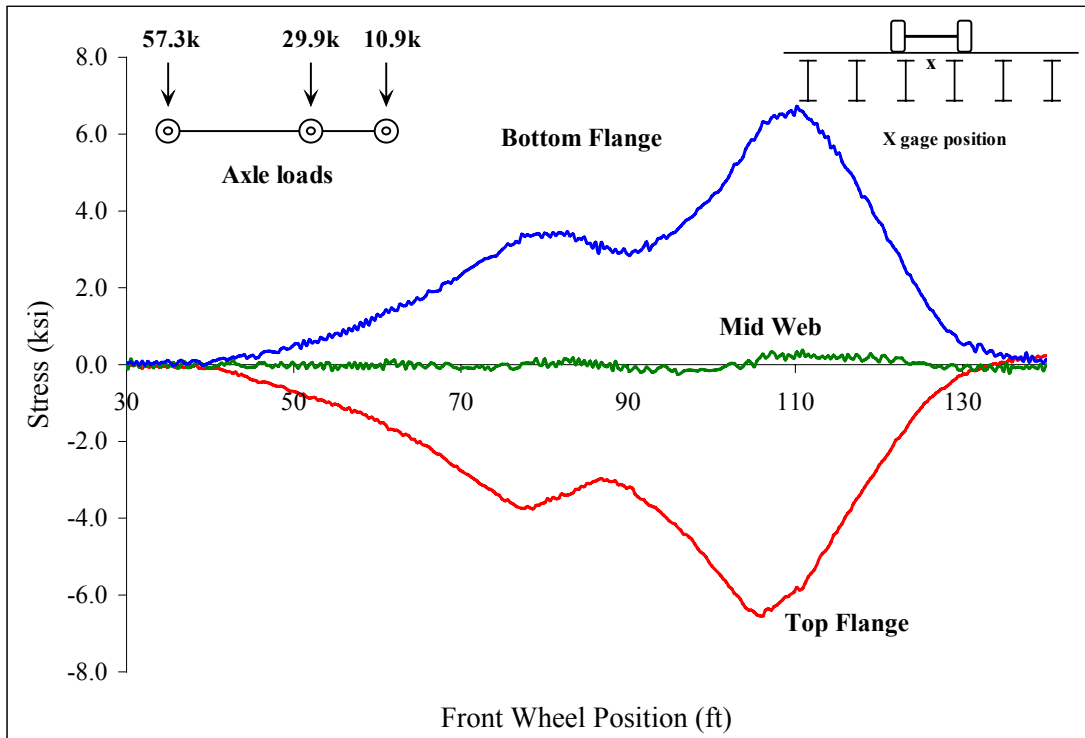
Figure C 65: Beam 5
