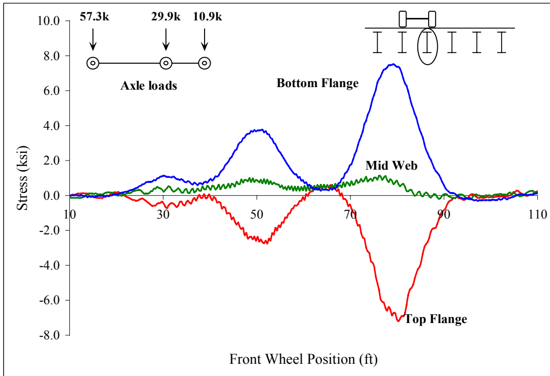
Figure C 55: Midpoint stringer 3
