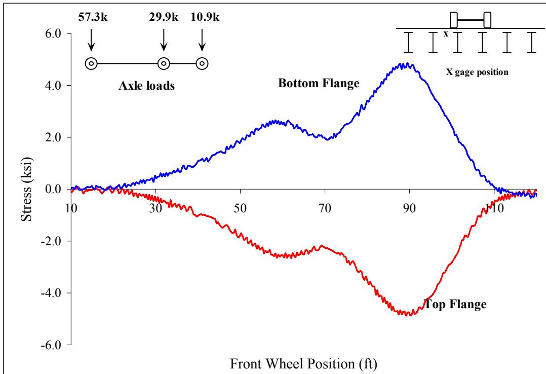
Figure C 59: Beam 4
