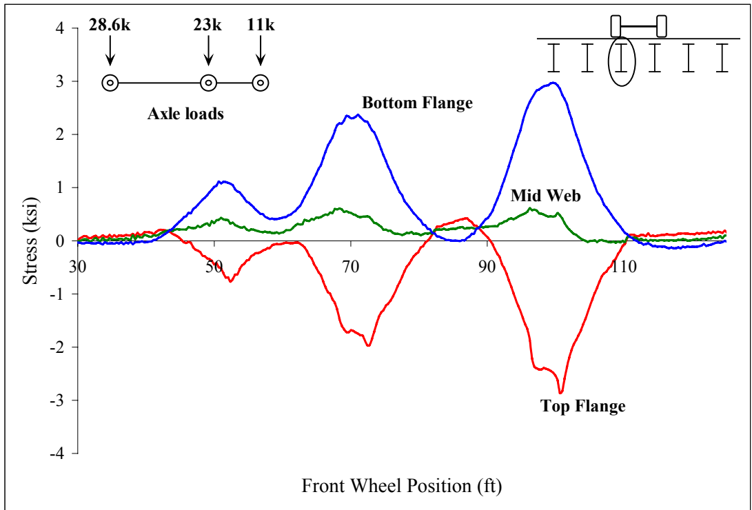
Figure C 15: Midspan stringer 3
