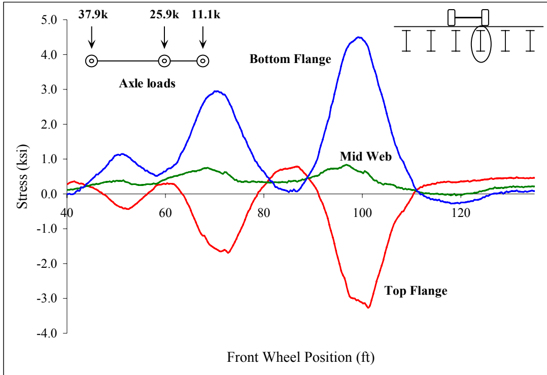
Figure C 40: Midspan stringer 4
