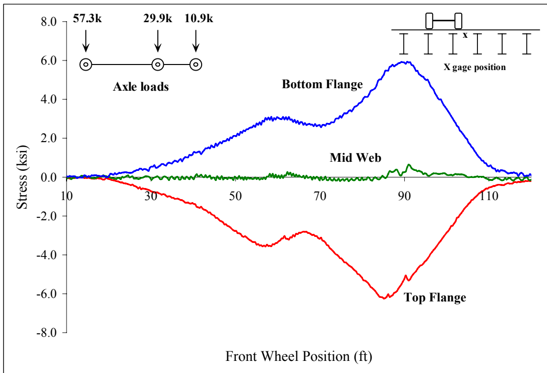
Figure C 57: Beam 5
