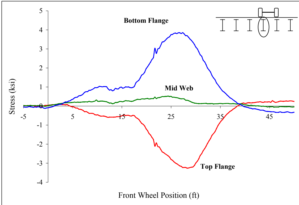
Figure A 42: Midspan stringer 3
