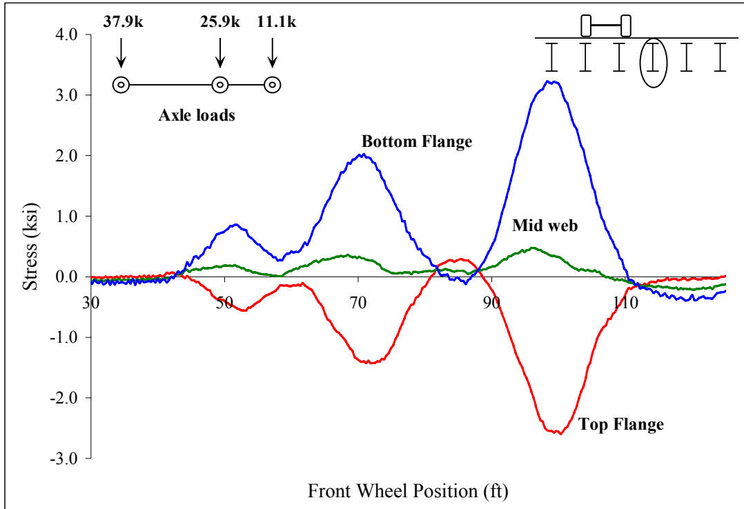
Figure C 32: Midspan stringer 4
