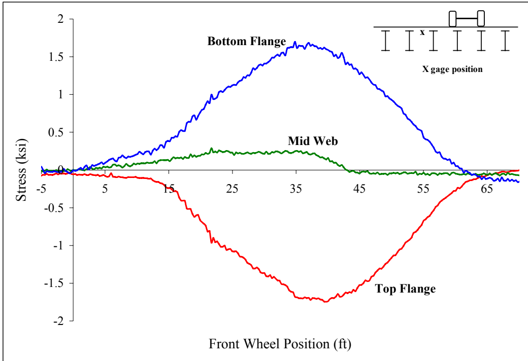
Figure A 44: Beam 2
