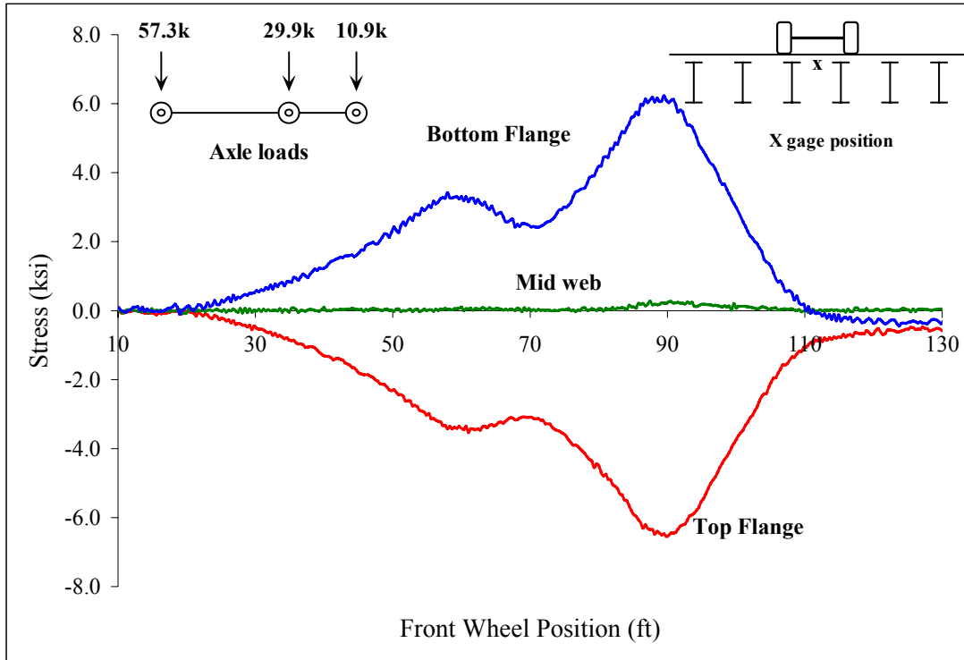
Figure C 60: Beam 4
