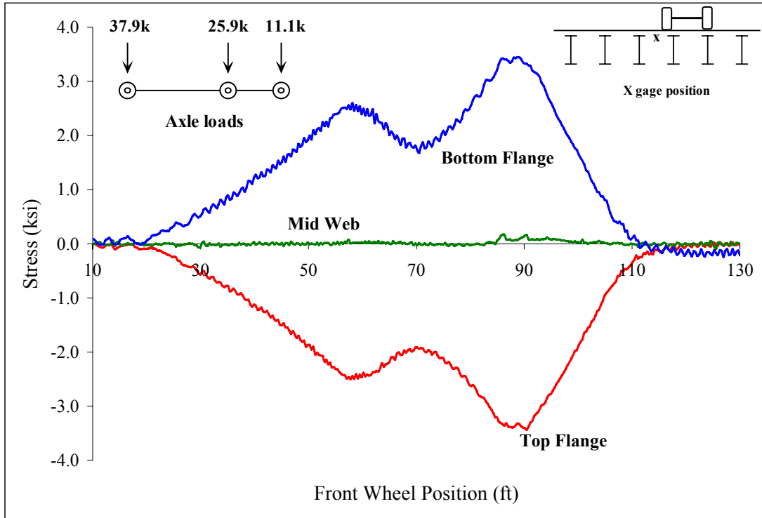
Figure C 44: Beam 4
