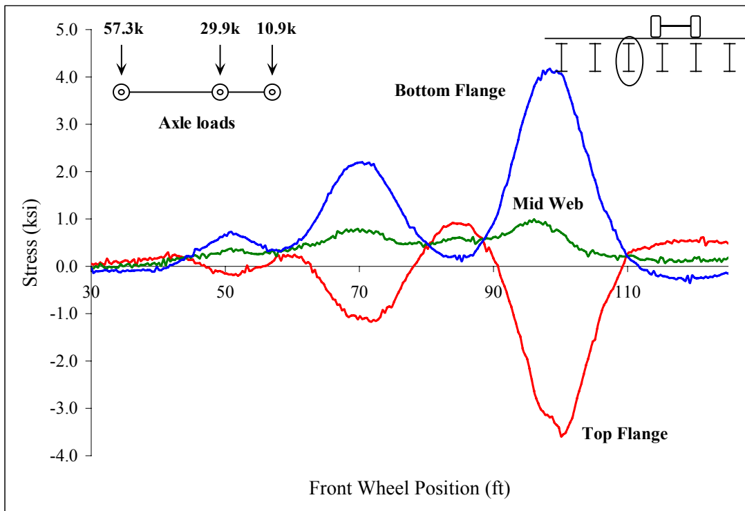
Figure C 71: Midspan stringer 3
