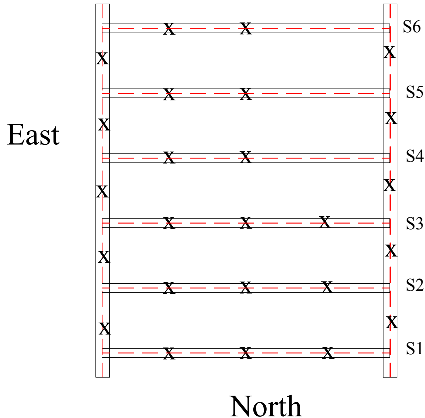
Figure 6.19 Member cross-section locations provided with strain gages
