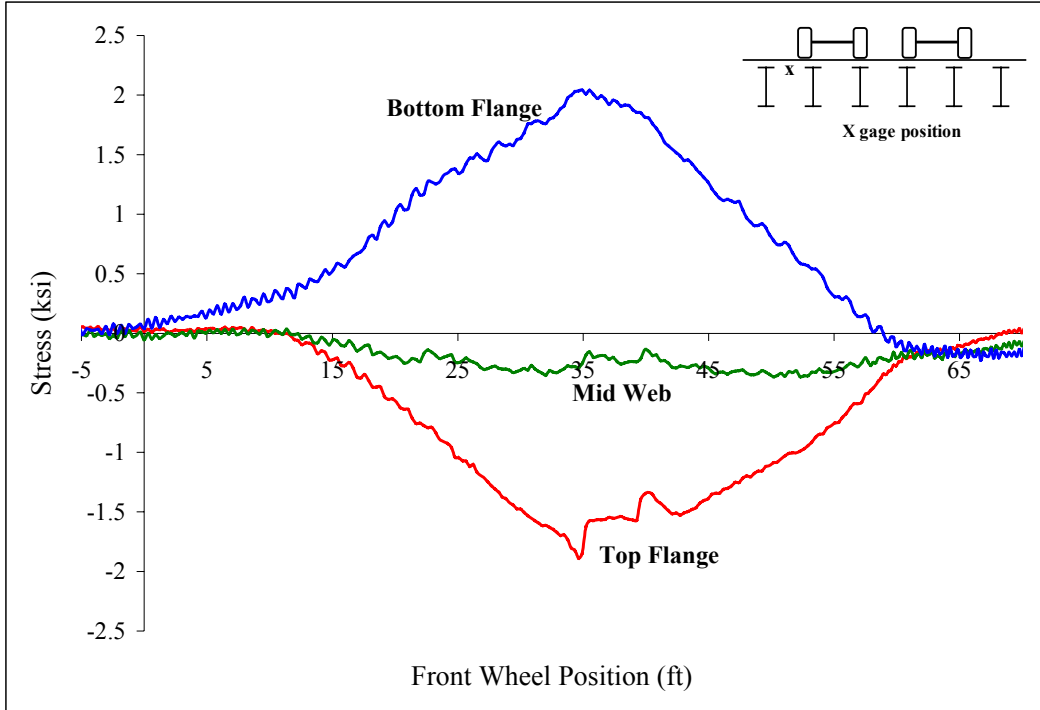
Figure B 10 Beam 2
