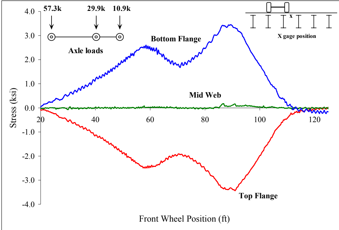
Figure C 52: Beam 4
