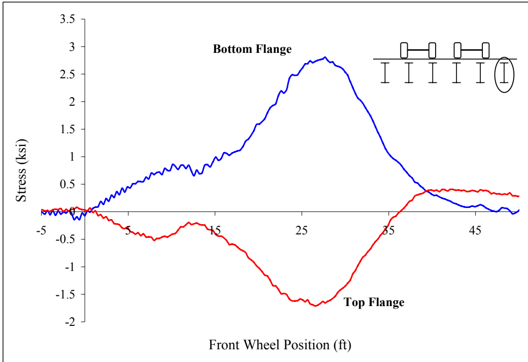
Figure B 4: Midspan stringer 1
