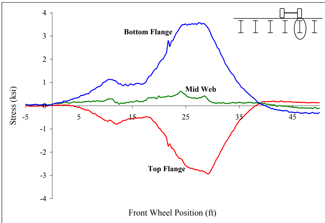
Figure A 41: Midspan stringer 2
