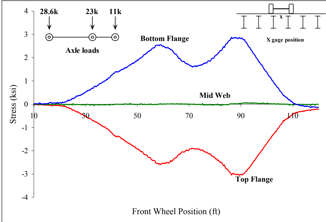
Figure C 12: Beam 4
