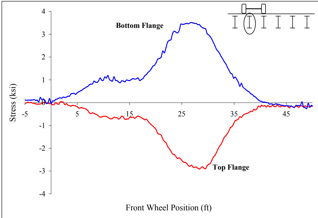
Figure B 28: Midspan stringer 5
