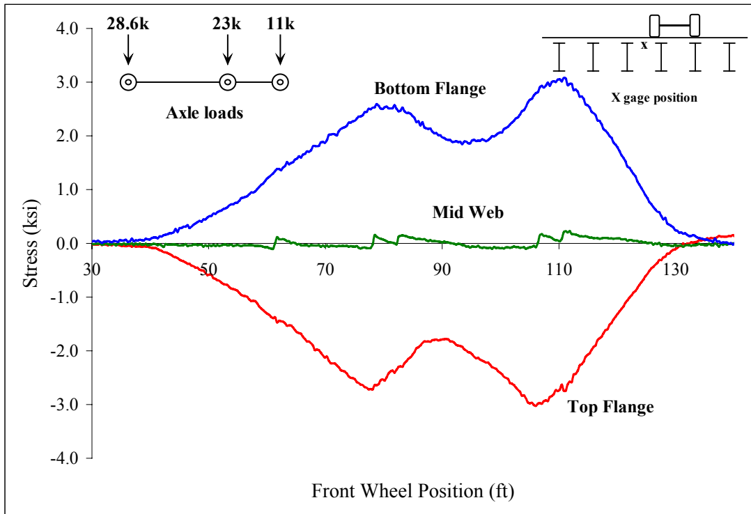
Figure C 25: Beam 5
