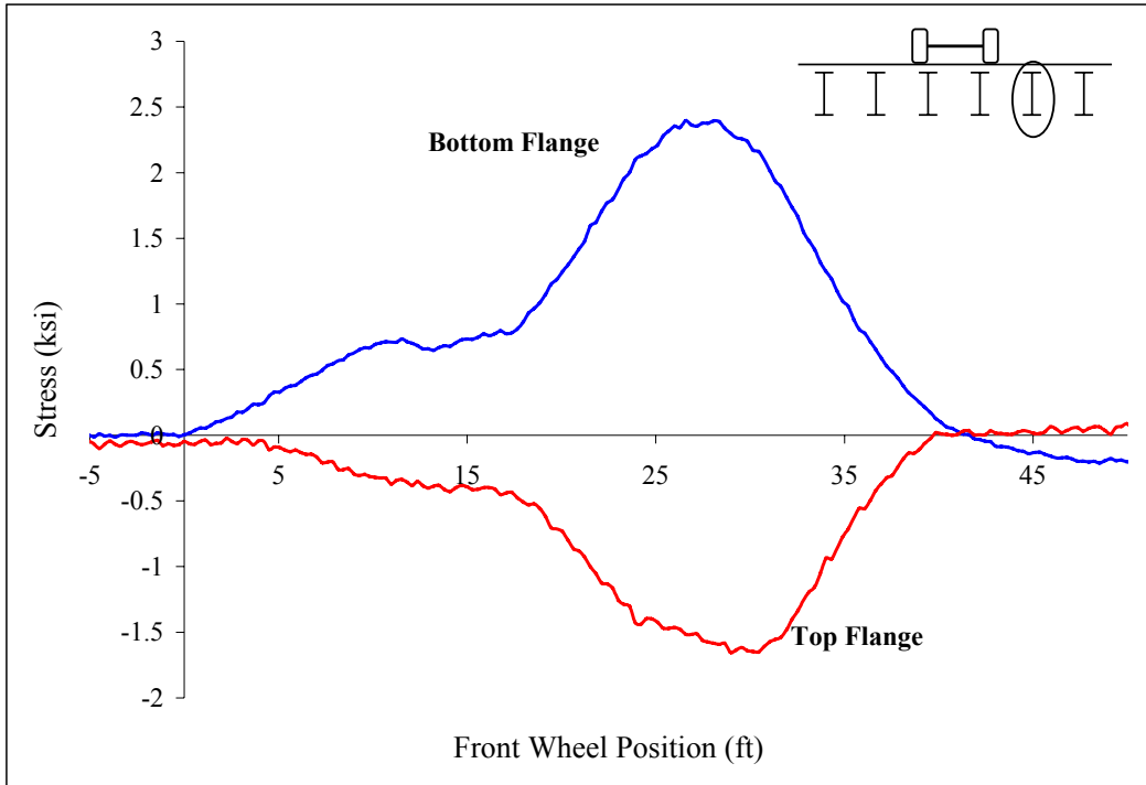
Figure B 16: Midspan stringer 2
