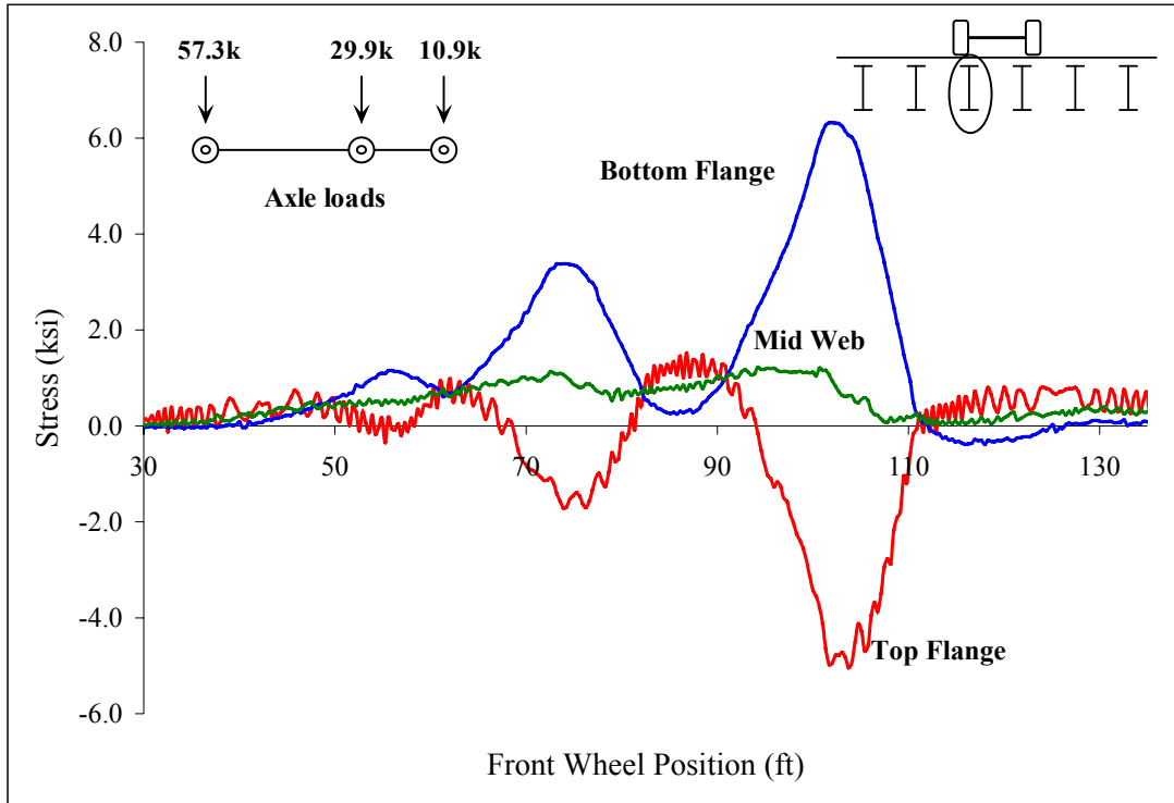
Figure C 62: North quarter point of stringer 3
