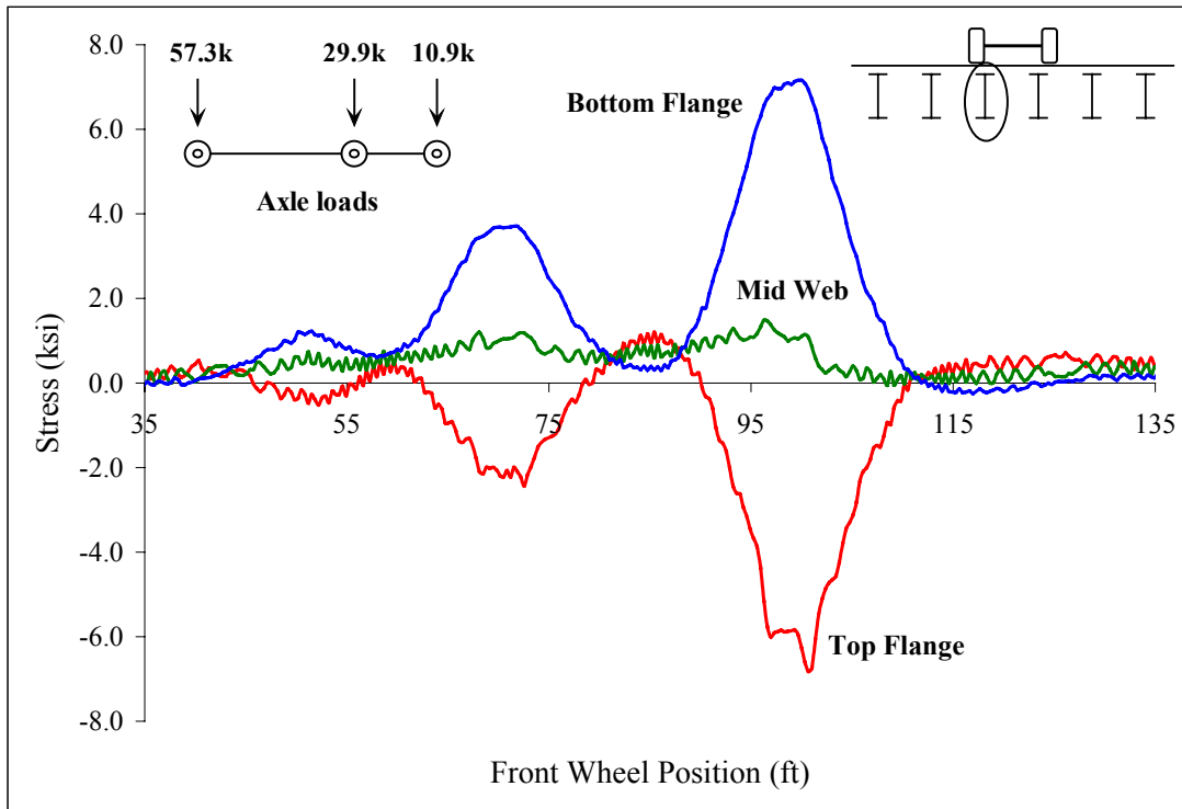
Figure C 63: Midspan stringer 3
