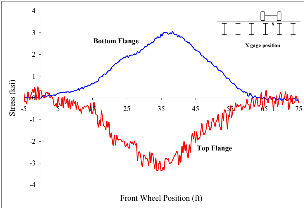
Figure B 50: Beam 2
