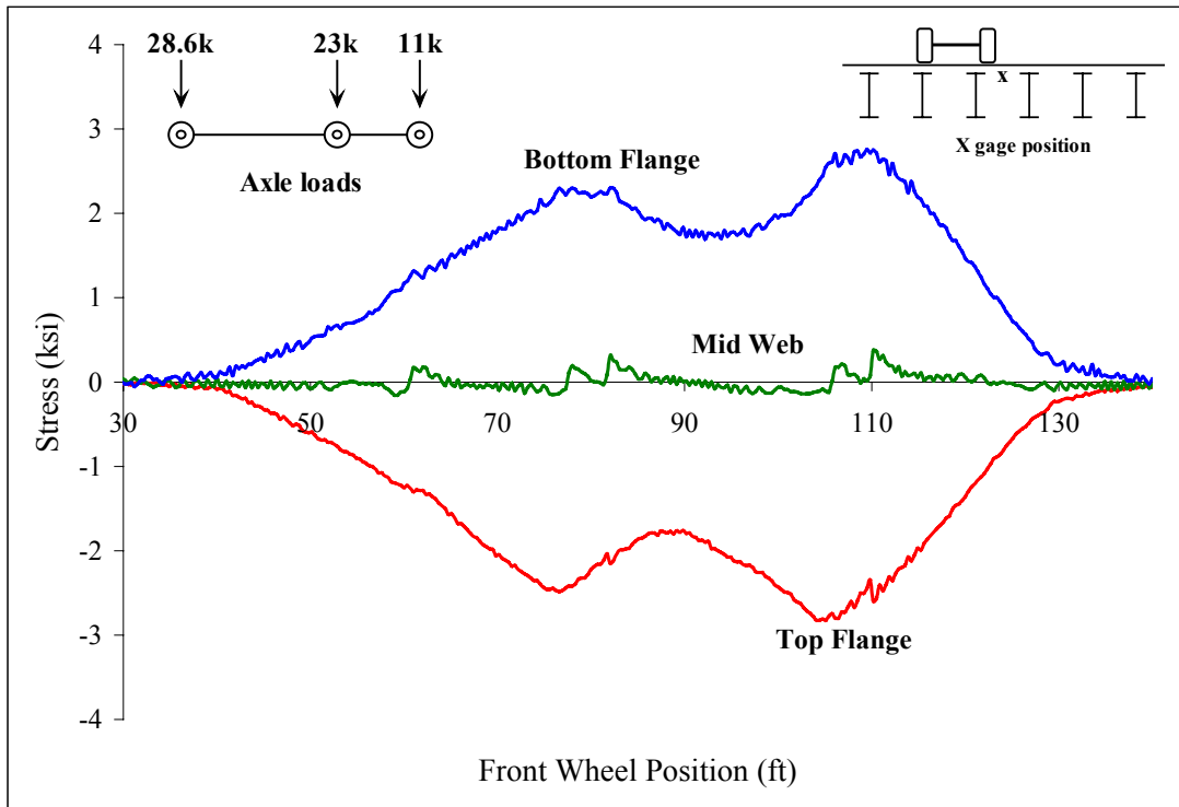
Figure C 9: Beam 5
