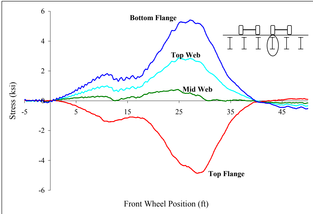
Figure B 6: Midspan stringer 3
