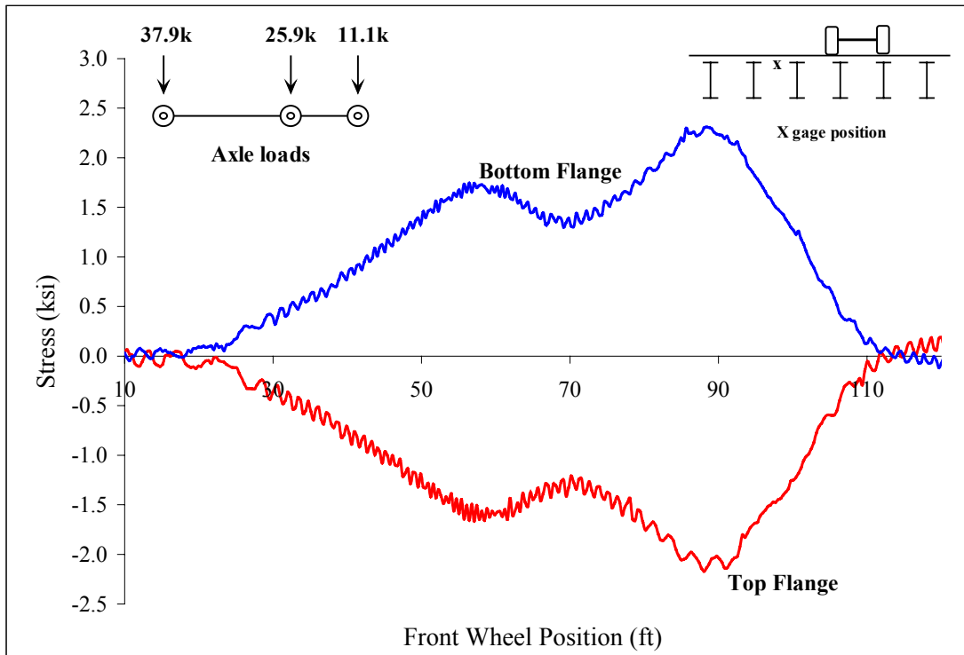
Figure C 43: Beam 4
