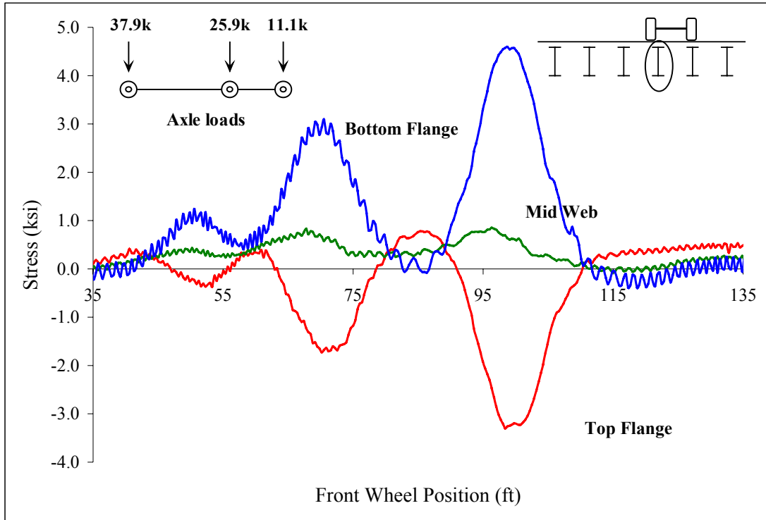
Figure C 48: Midspan stringer 4
