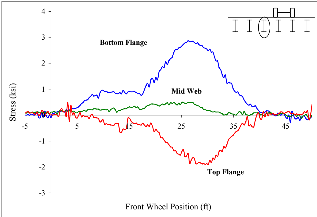
Figure B 48 Midspan stringer 4
