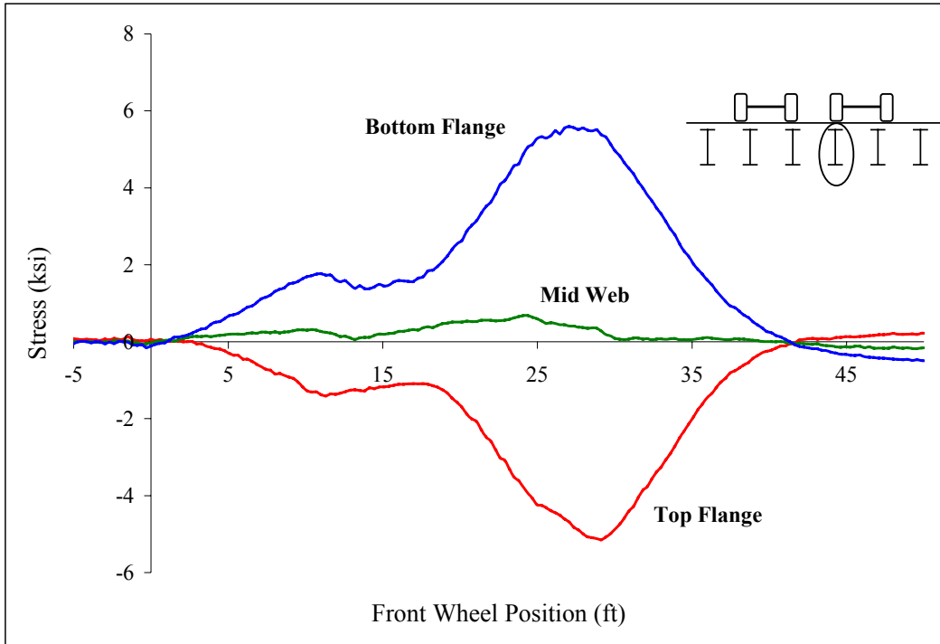
Figure A 6: Midspan stringer 3
