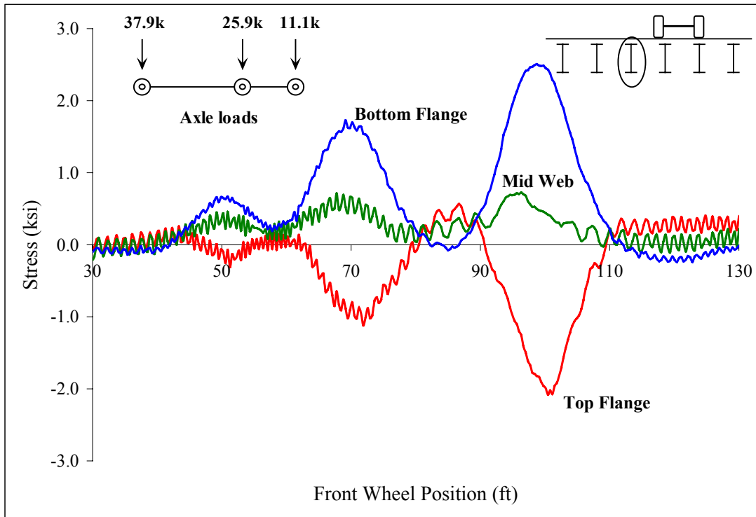
Figure C 47: Midspan stringer 3
