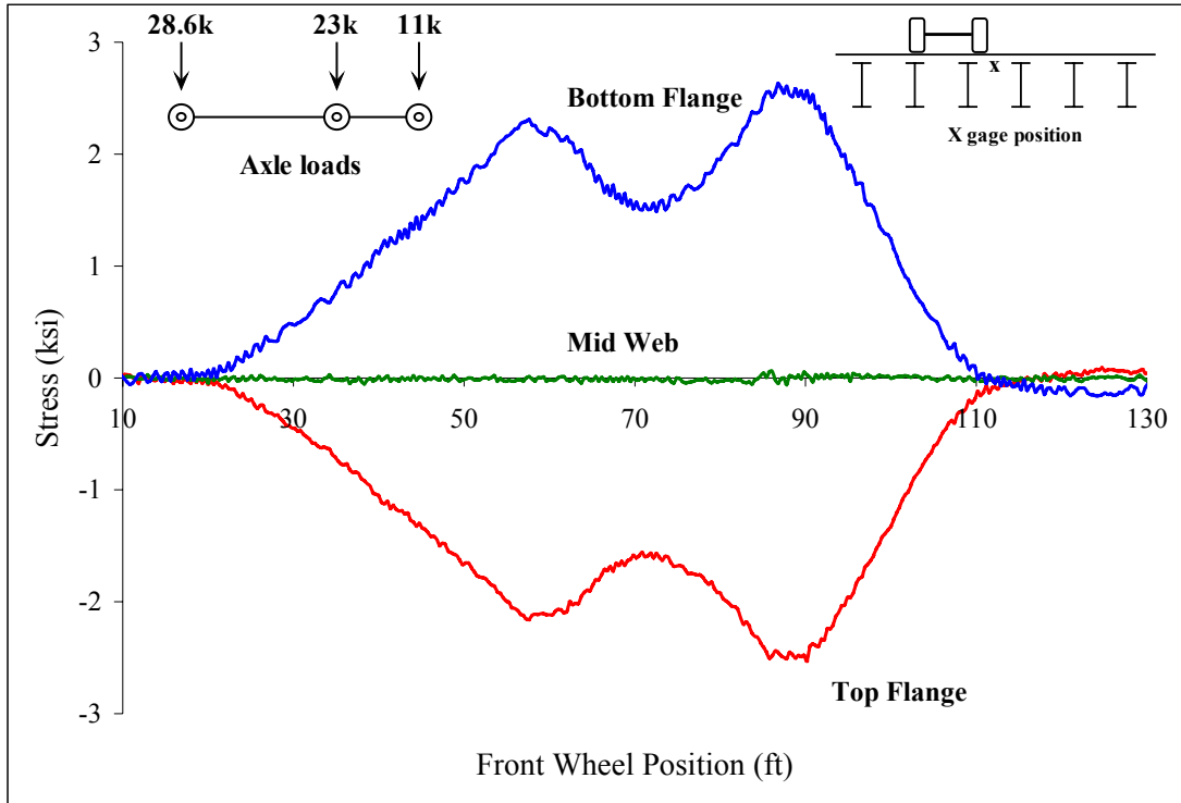
Figure C 4: Beam 4
