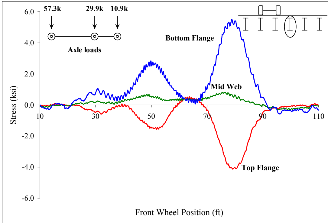
Figure C 56: Midpoint stringer 4
