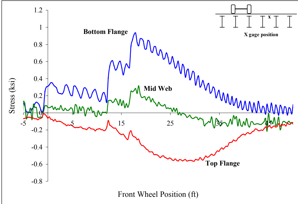
Figure B 24: Beam 1
