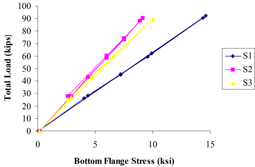
Figure 6.35 Stringers S1 to S3: load vs. stress
