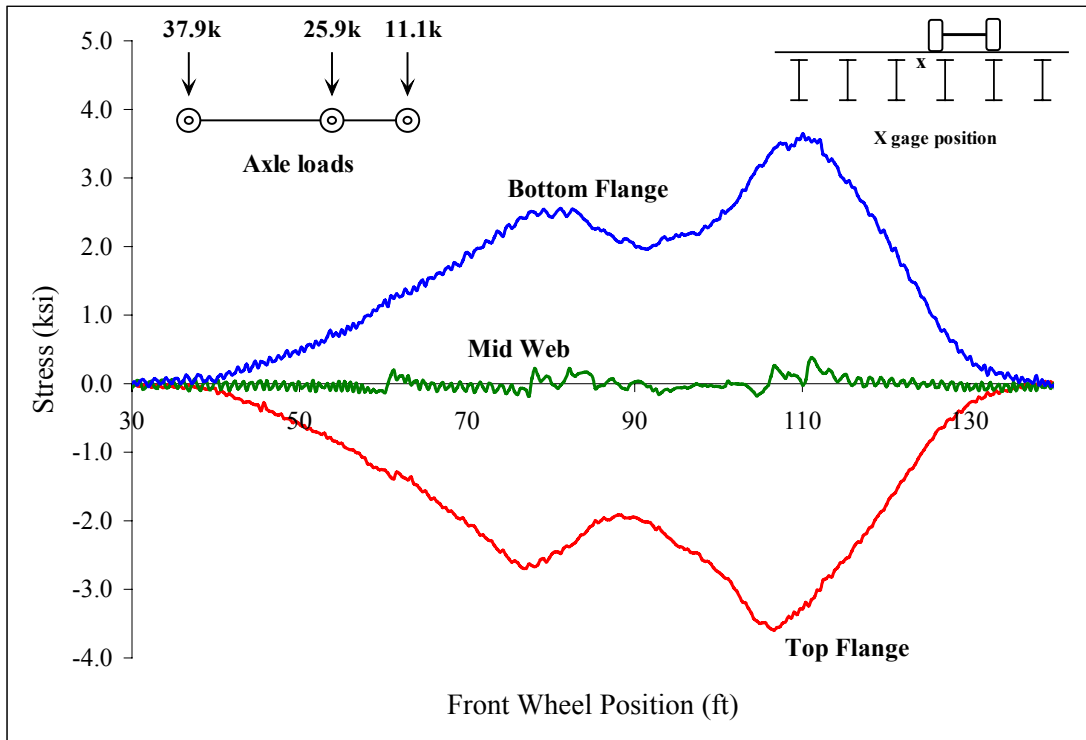
Figure C 49: Beam 5
