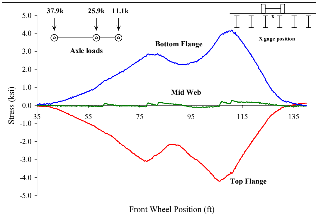
Figure C 41: Beam 5
