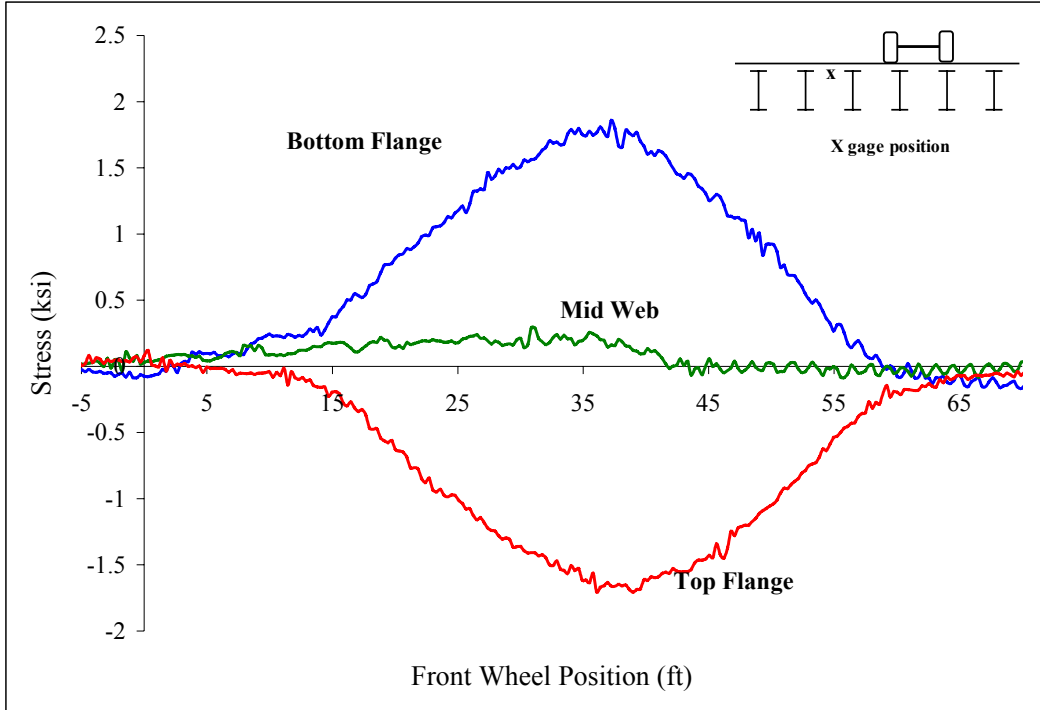
Figure B 52: Beam 2
