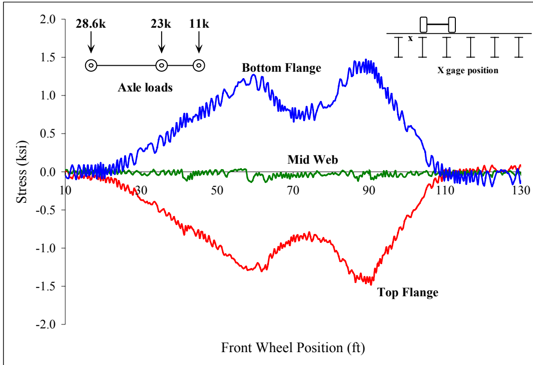
Figure C 2: Beam 4
