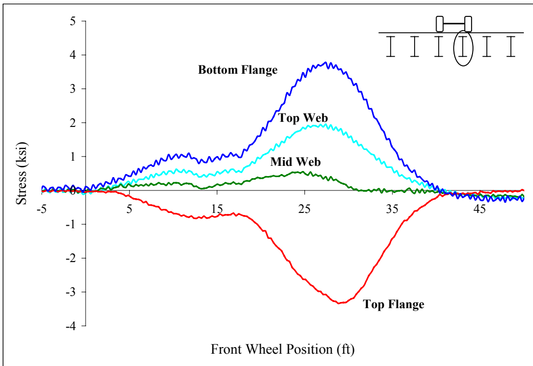
Figure B 37: Midspan stringer 3
