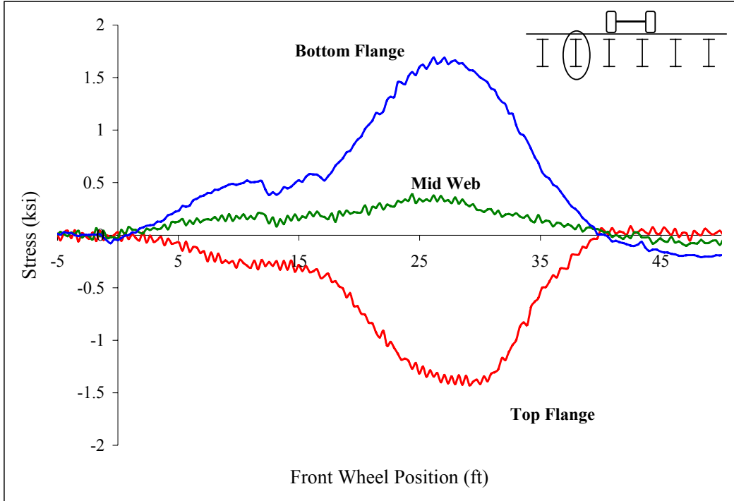
Figure A 34: Midspan stringer 5
