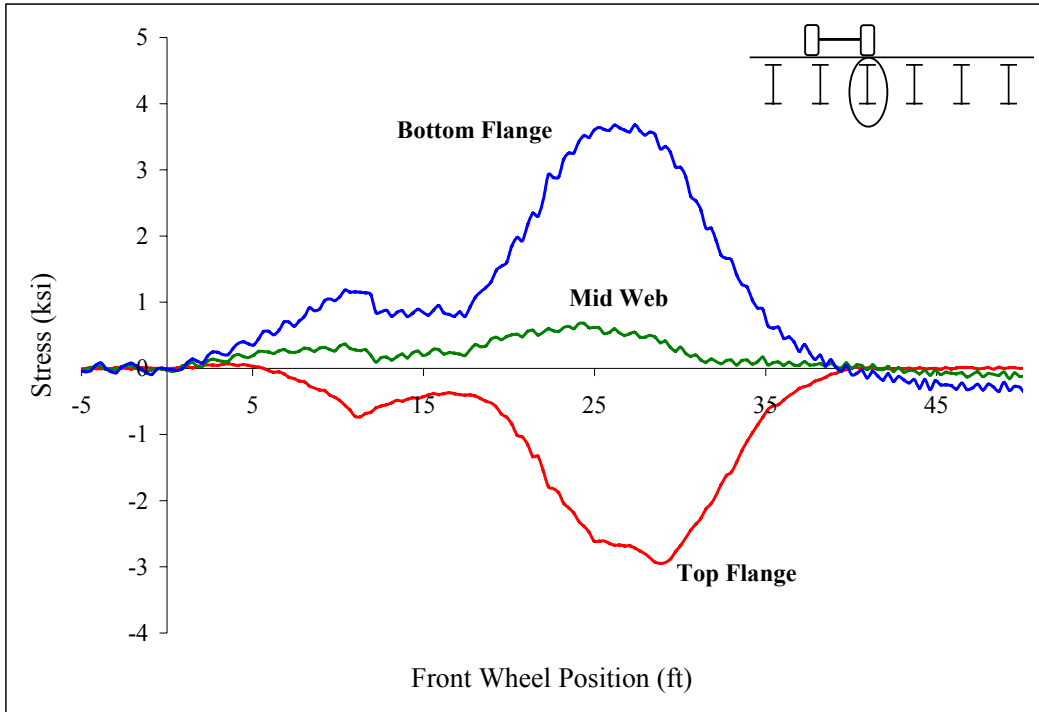
Figure A 22: Midspan stringer 4
