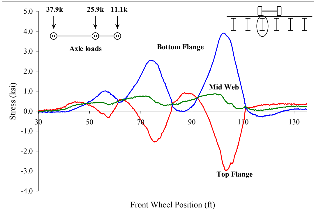
Figure C 38: North quarter point of stringer 3
