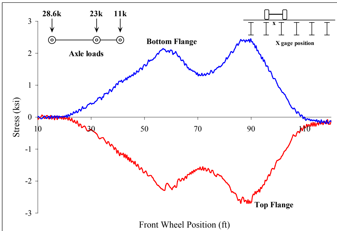
Figure C 3: Beam 4
