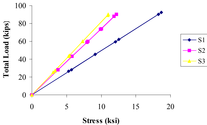
Figure 6.50 Finite element analysis prediction for load vs. midspan stress for stringers
