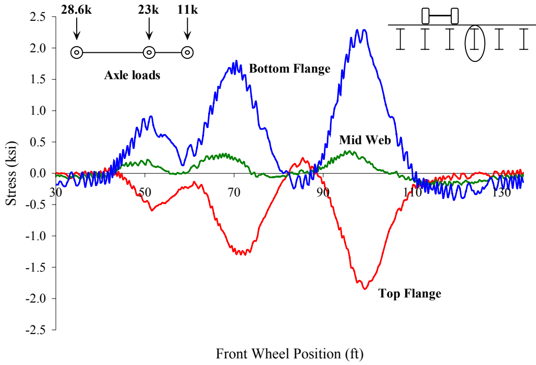
Figure C 8: Midspan stringer 4
