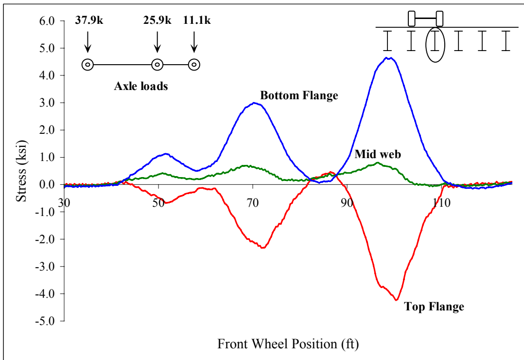
Figure C 31: Midspan stringer 3
