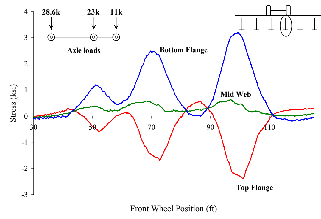
Figure C 16: Midspan stringer 4
