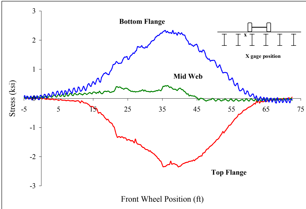
Figure A 18: Beam 2
