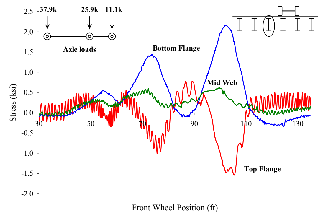
Figure C 46: North quarter point of stringer 3
