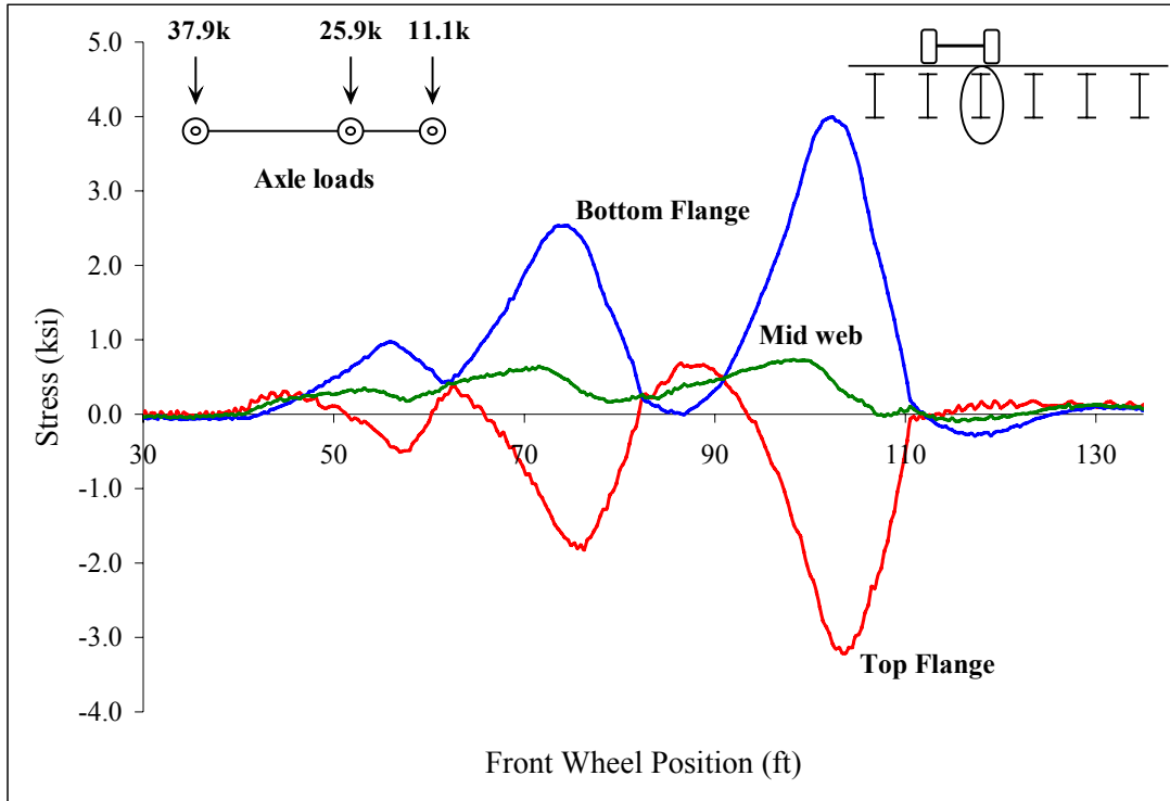
Figure C 30: North quarter point of stringer 3
