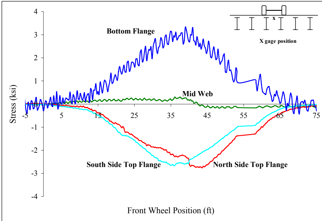
Figure B 22: Beam 2
