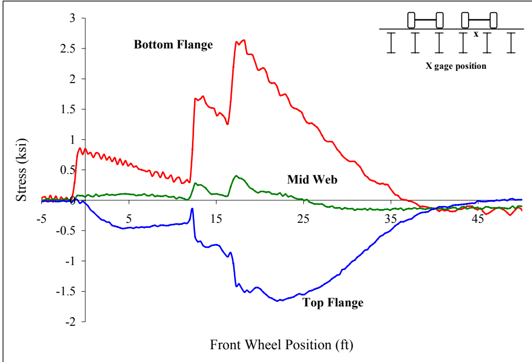
Figure B 2: Beam 1
