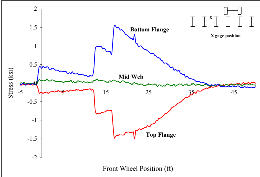
Figure A 38: Beam 1
