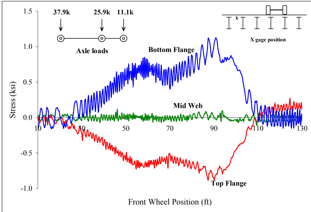
Figure C 42: Beam 4
