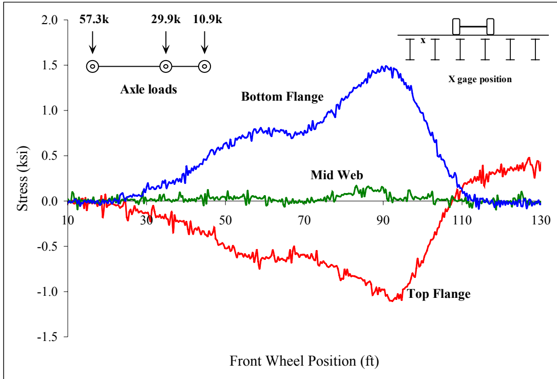
Figure C 66: Beam 4
