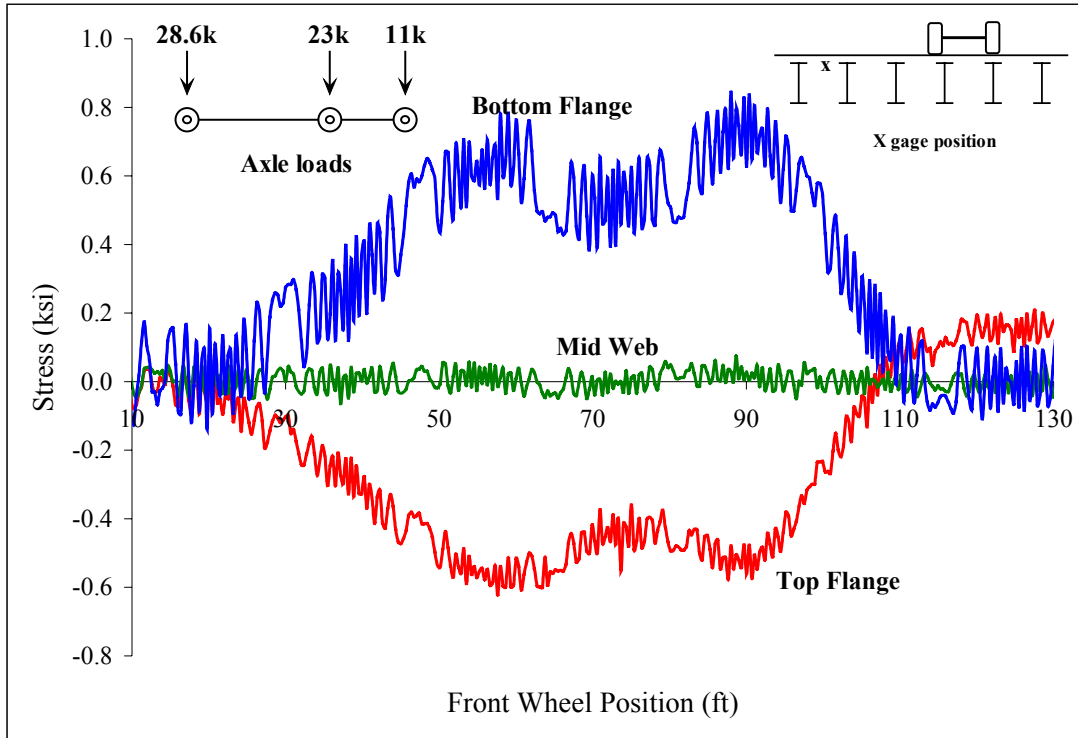
Figure C 18: Beam 4
