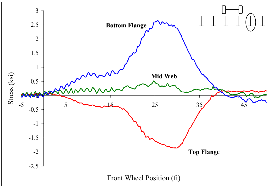
Figure A 15: Midspan stringer 2
