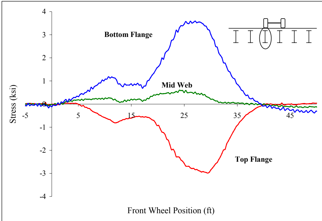
Figure A 30: Midspan stringer 4
