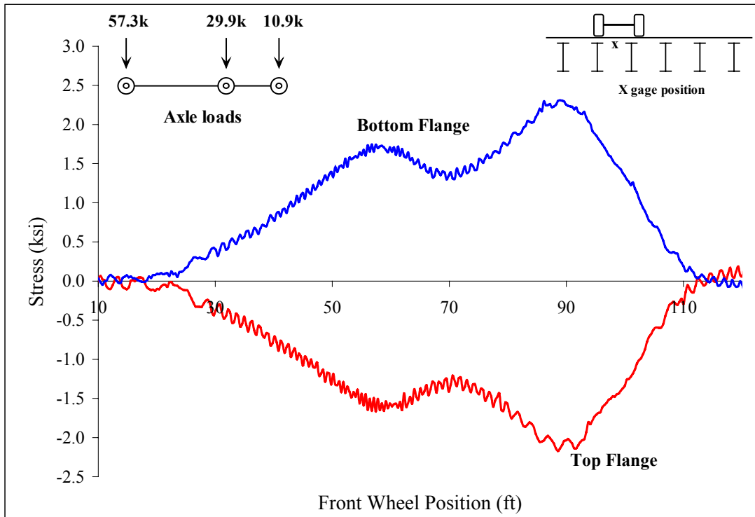
Figure C 51: Beam 4
