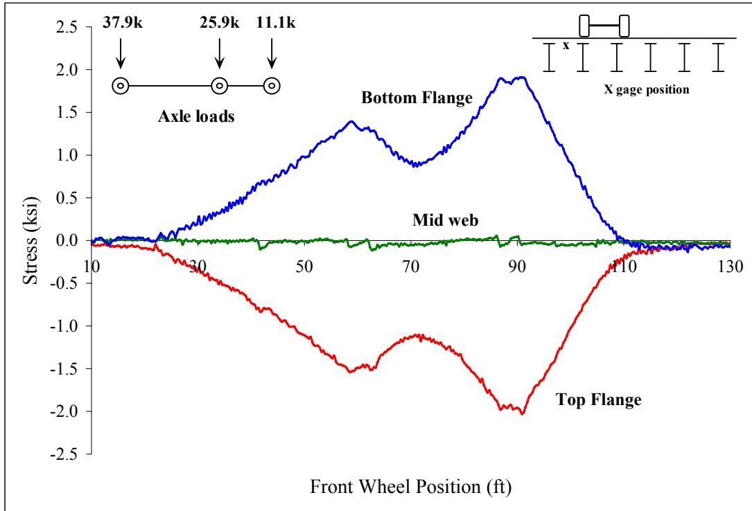
Figure C 26: Beam 4
