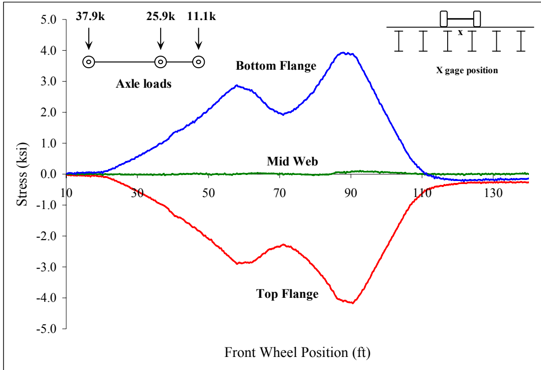
Figure C 36: Beam 4
