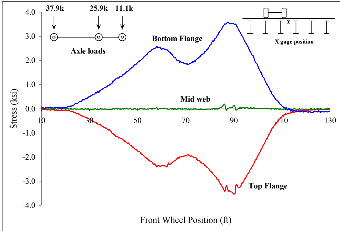
Figure C 28: Beam 4
