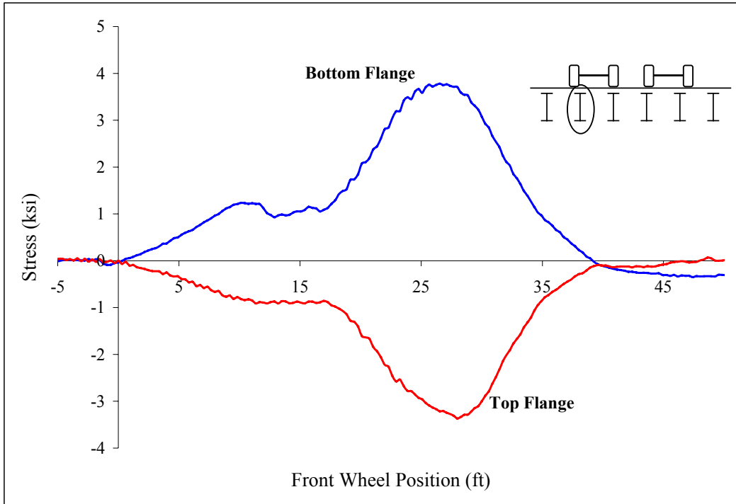
Figure B 8: Midspan stringer 5
