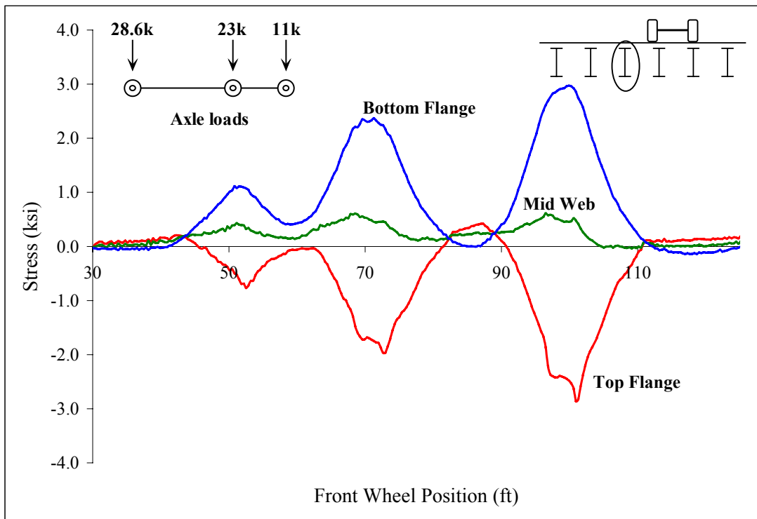
Figure C 23: Midspan stringer 3
