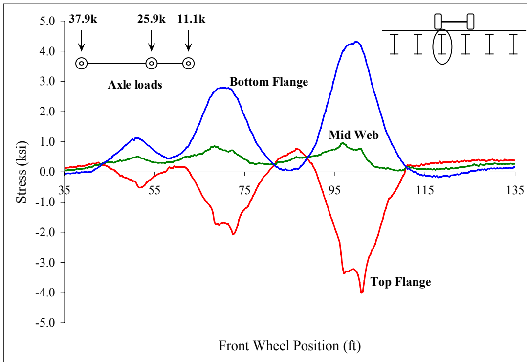
Figure C 39 Midspan stringer 3
