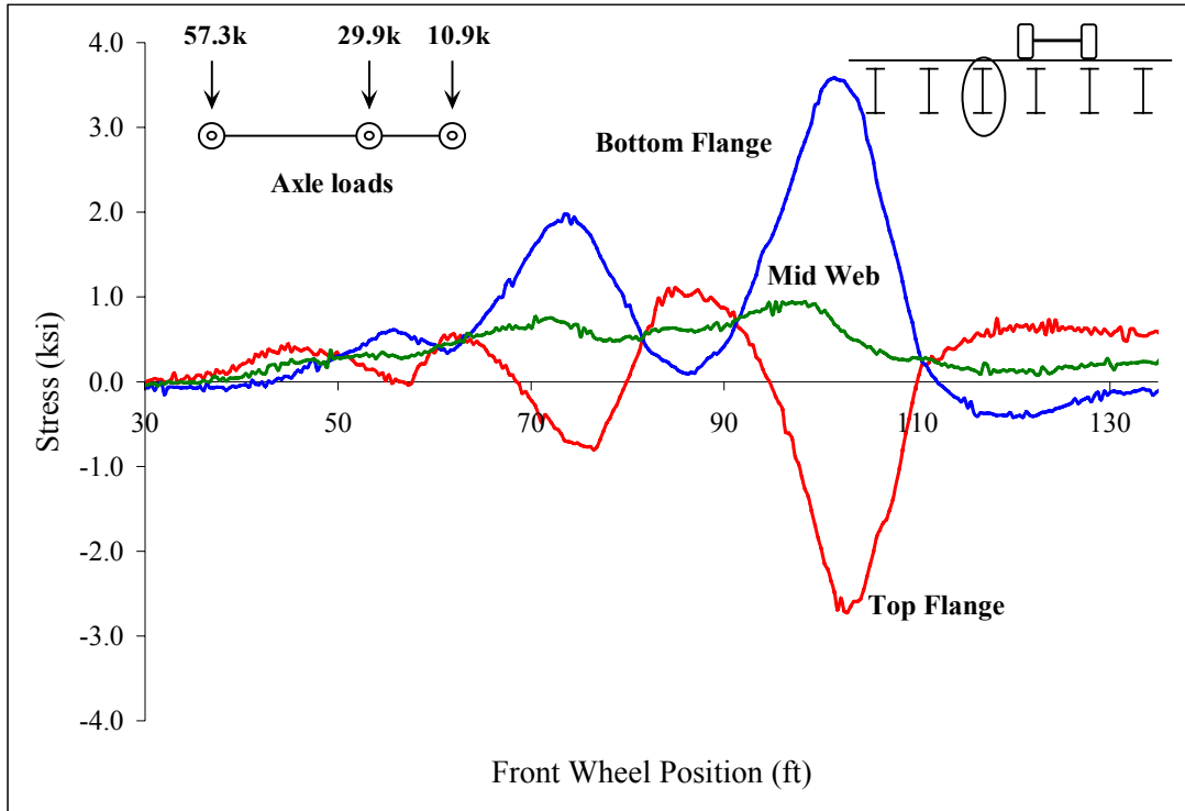
Figure C 70: North quarter point of stringer 3
