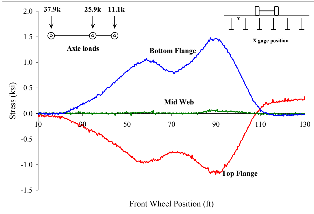
Figure C 34: Beam 4
