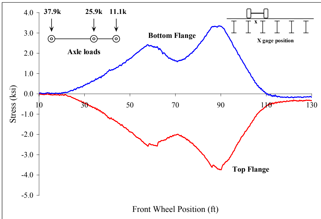
Figure C 27: Beam 4
