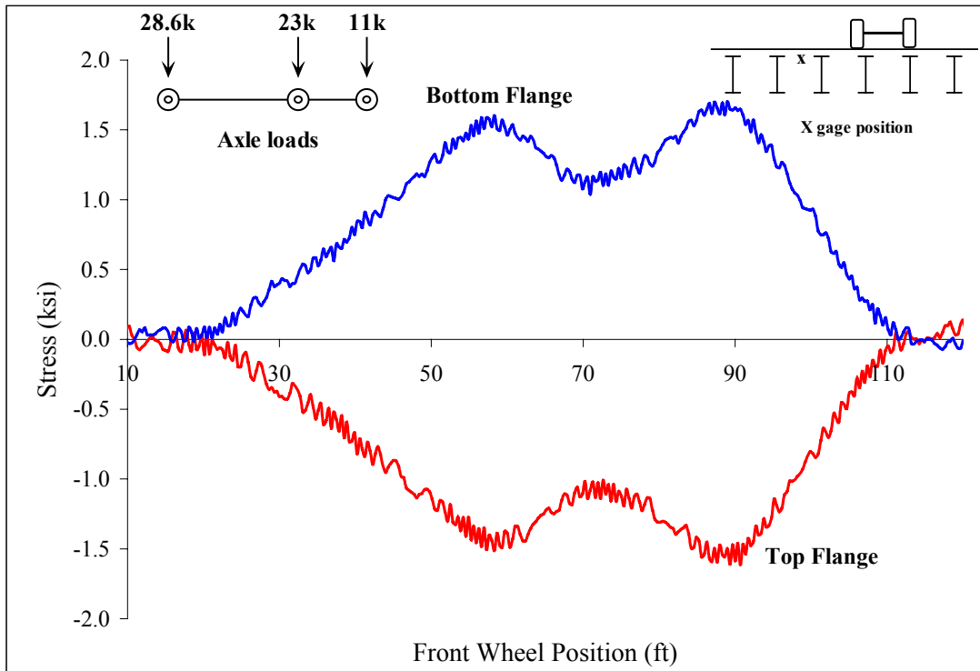
Figure C 19: Beam 4
