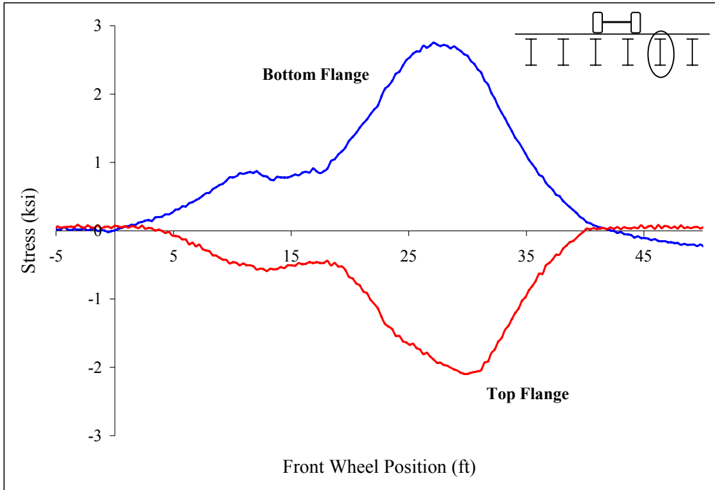
Figure B 36: Midspan stringer 2
