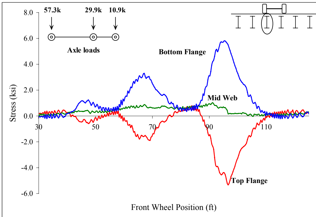
Figure C 61: South quarter point of stringer3
