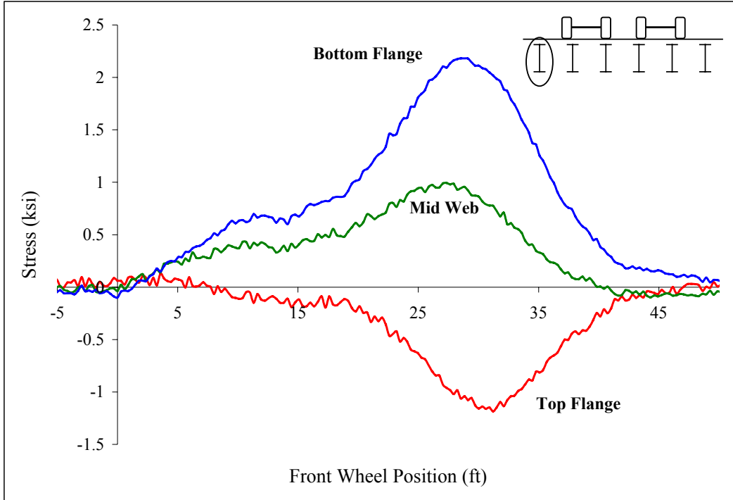
Figure A 8: Midspan stringer 6
