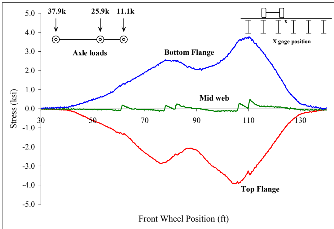
Figure C 33: Beam 5
