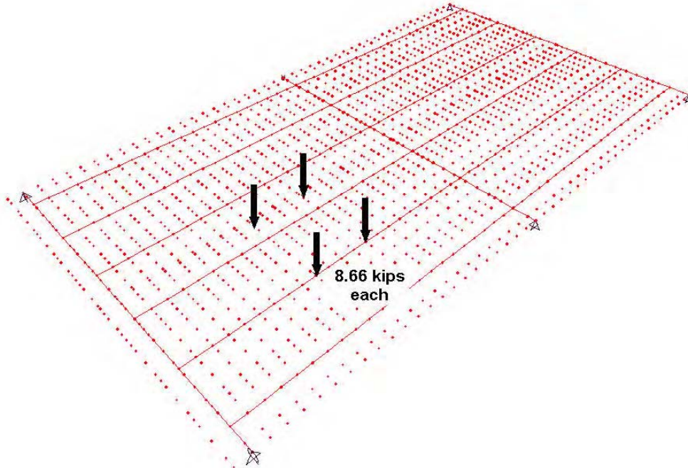
Figure 4.29 Loading for field test in stringer 2
