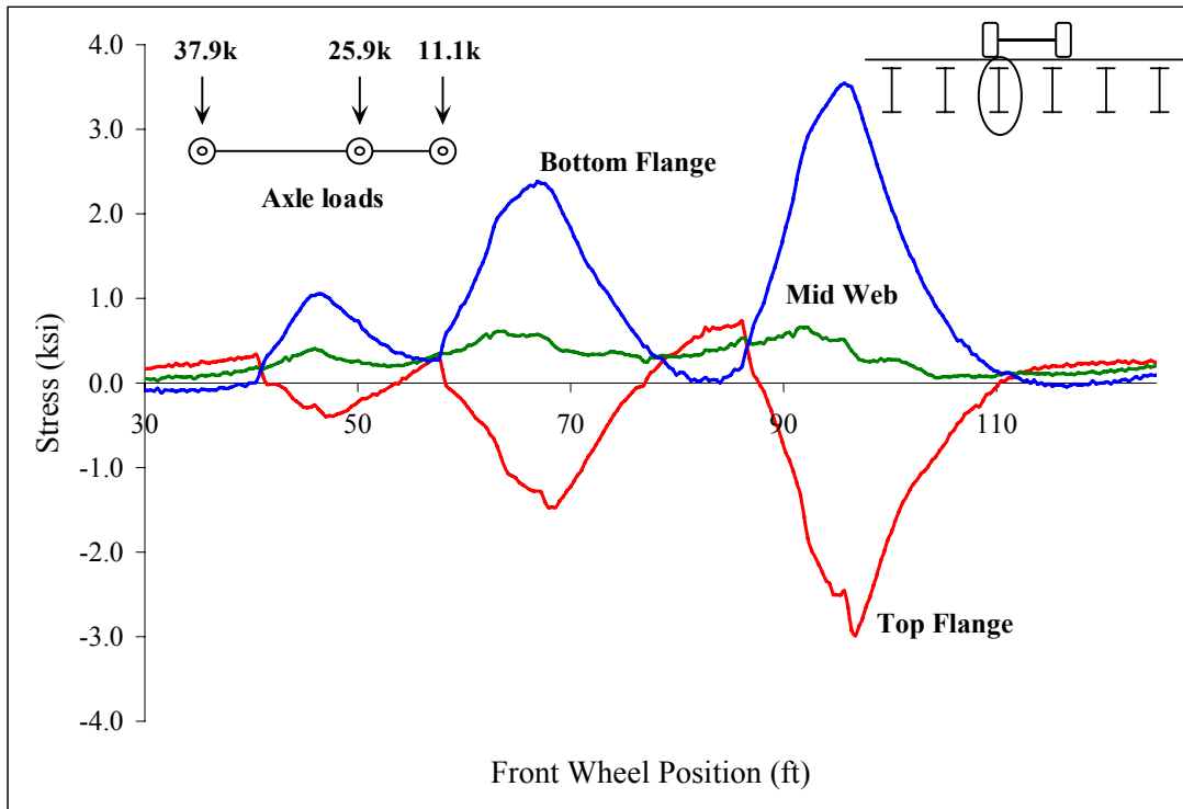
Figure C 37: South quarter point of stringer 3
