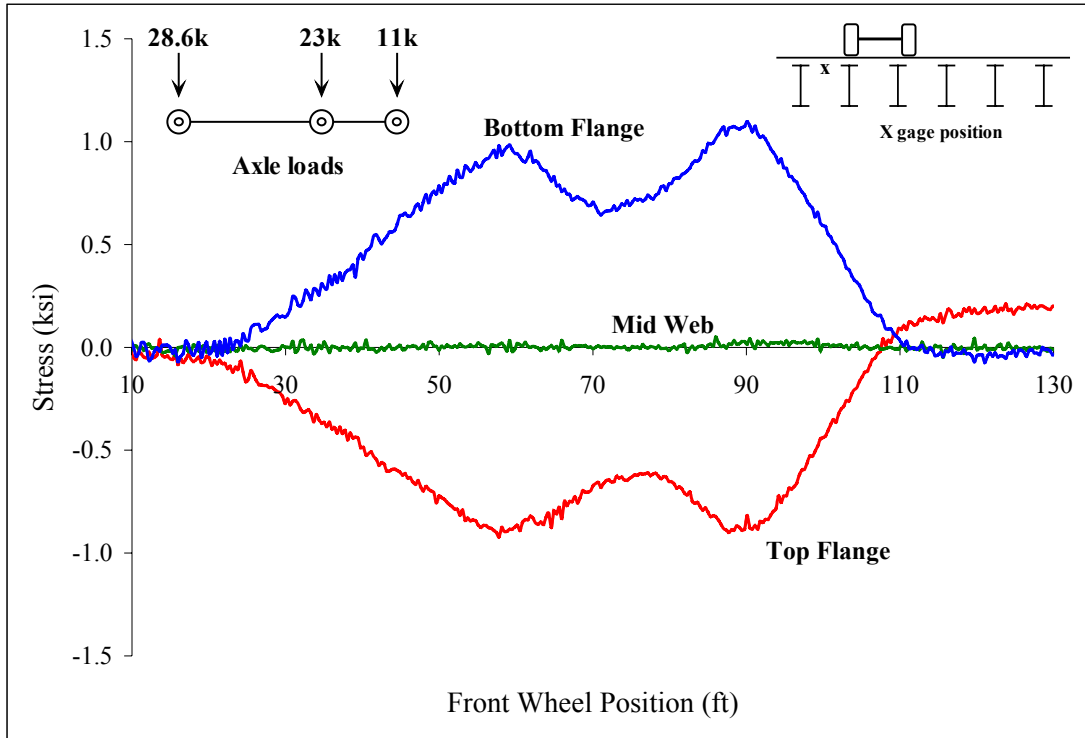
Figure C 10: Beam 4
