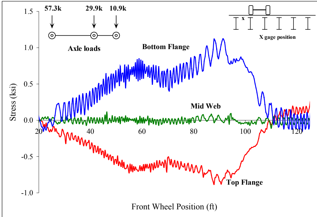
Figure C 50: Beam 4
