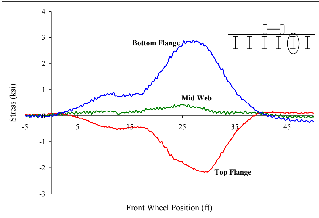
Figure A 32: Midspan stringer 2
