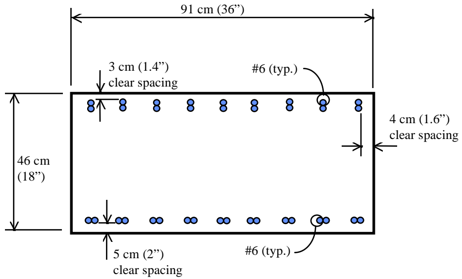
Figure 3-7 Specimen #4 cross section, as constructed
