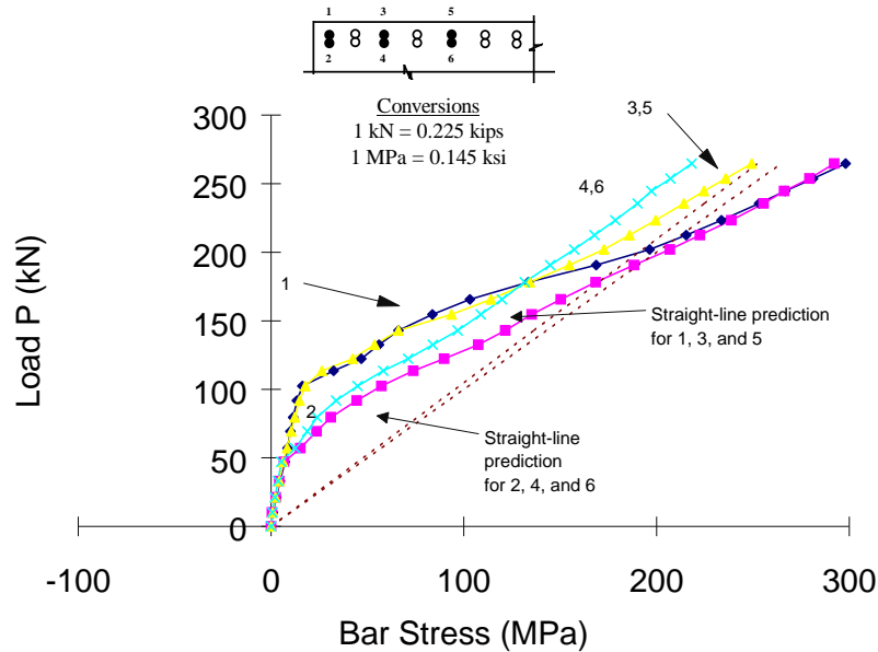
Figure 4- 31 Splice stresses for Test 12-O-A
