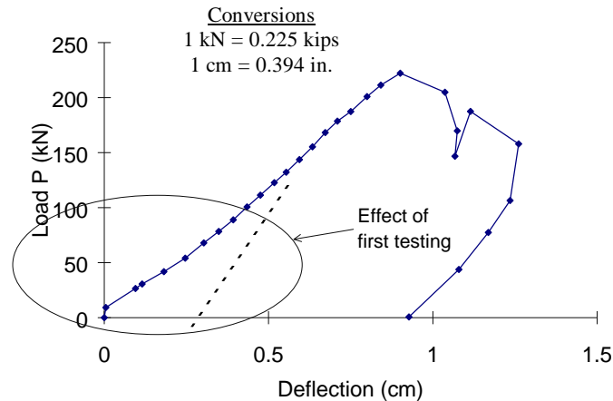
Figure 4- 22 Load-deflection plot for Test 9-O-P
