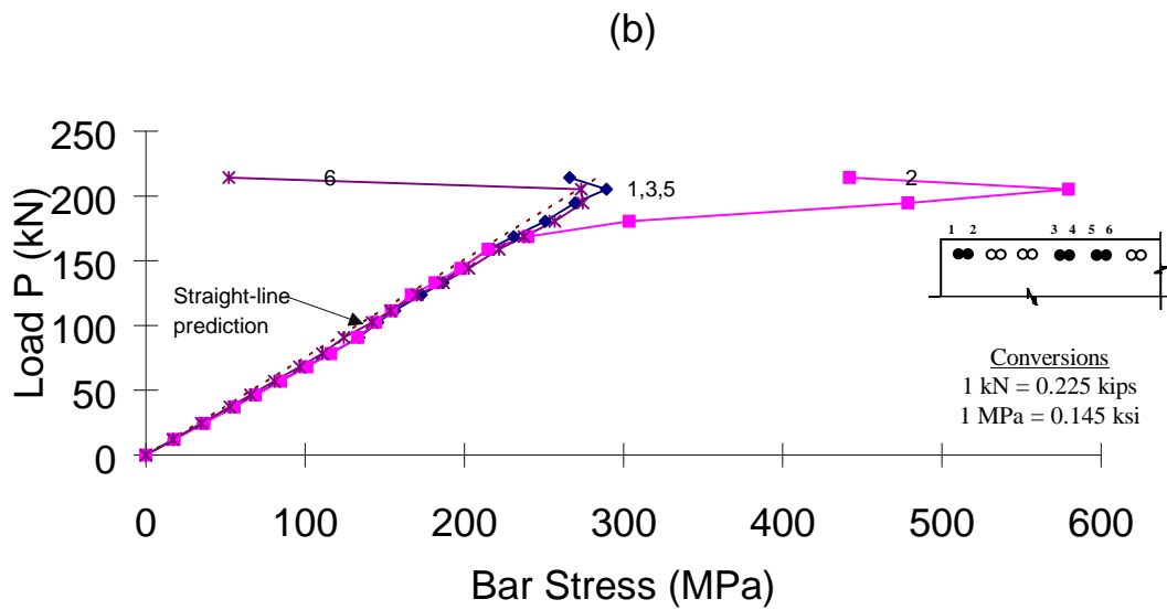
Figure 4- 43 Adjusted splice stresses for Test 9-S-A
