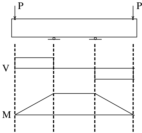
Figure 3- 3 Loading configuration
