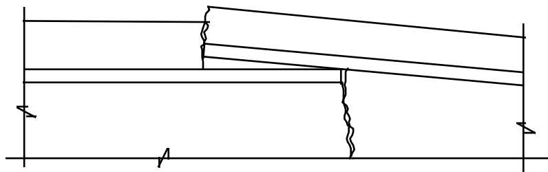
Figure 5-4 Behavior of offset splices with no stirrups in the splice region
