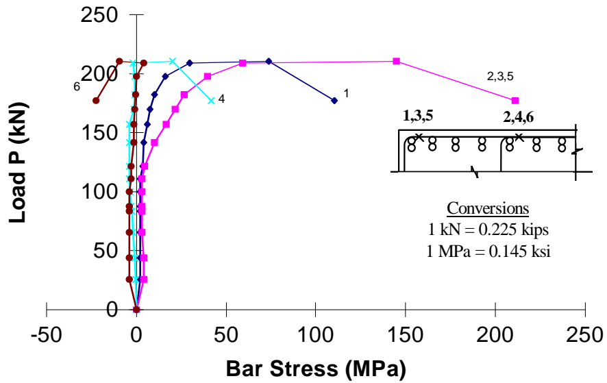
Figure 4- 11 Lateral tie leg stresses for Test 12-O-P
