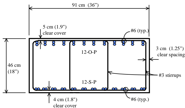
Figure 3- 4 Specimen #1 cross section, as constructed
