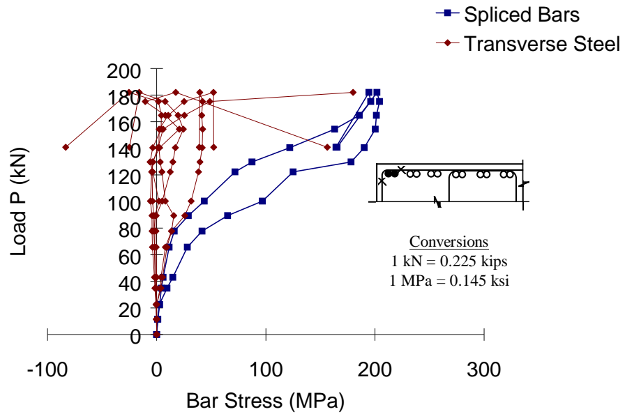
Figure 4- 28 Bar stresses for 9-S-P (edge splice)
