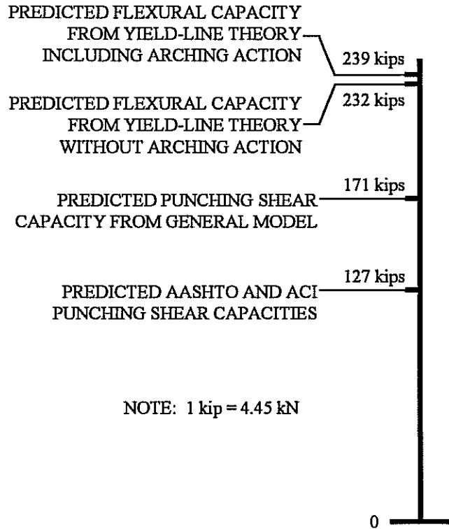
Figure 3.9: Predicted capacities for cast-in-place test specimens.
