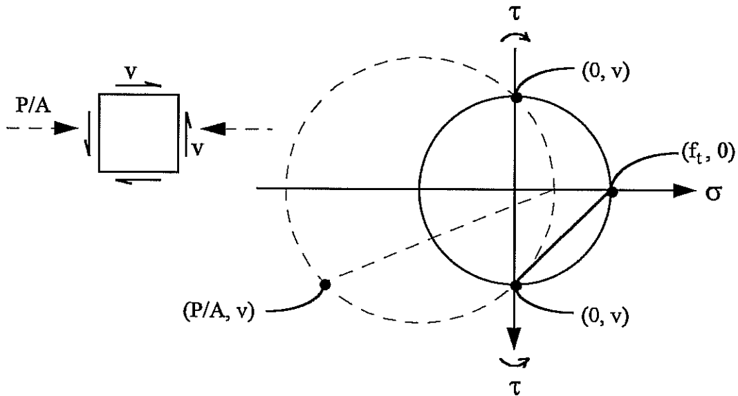
Figure 10.1: Mohr's circles for nominal stresses.
