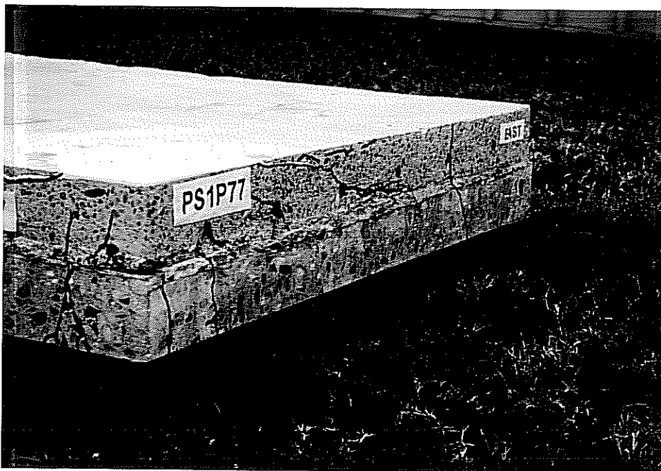
Figure 8.8: Saw cut face (transverse section) of precast prestressed panel pulsating fatigue test Specimen PS1P77.
