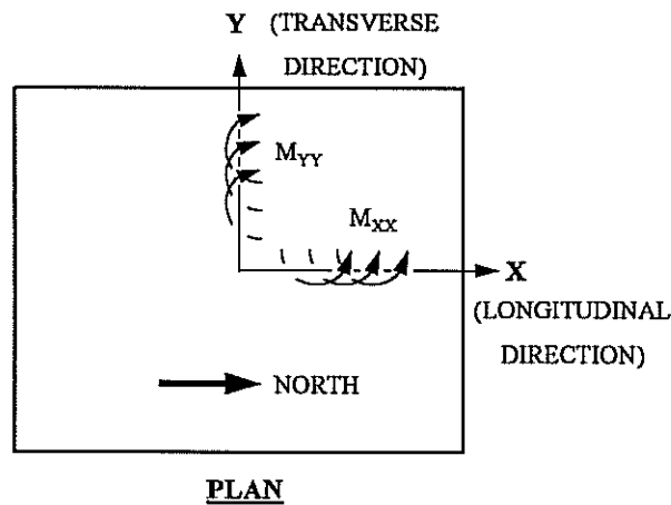
Figure 3.2: Test specimen coordinate axes and notation used for flexural capacities. Moments shown are those acting on the northwest quadrant.
