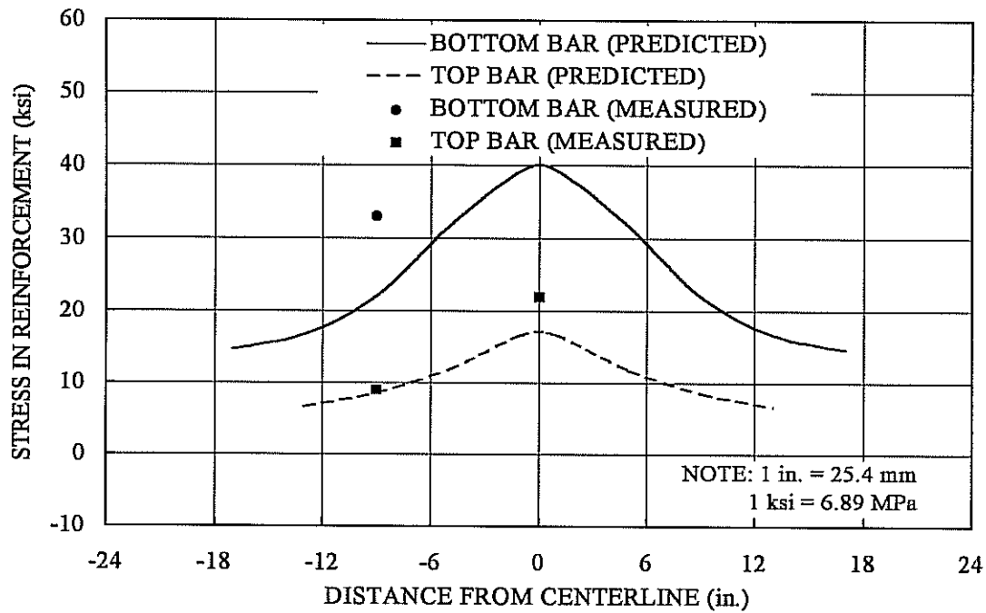
Figure 8.14: Measured and predicted reinforcing steel stresses in longitudinal bars (tension is positive).
