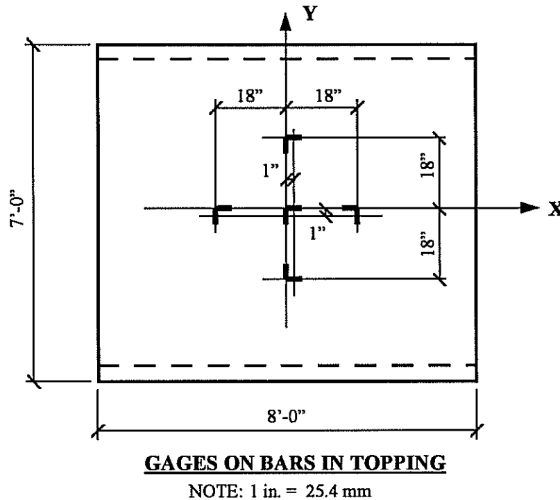
Figure 5.9: Locations of strain gages used in precast prestressed panel test specimens.
