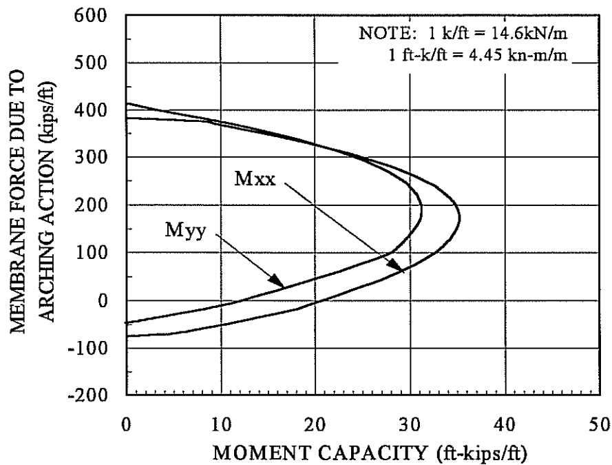
Figure 3.7: Interaction diagrams for precast prestressed panel test specimens.
