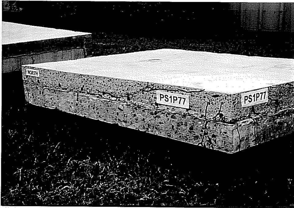
Figure 8.7: Saw cut face (longitudinal section) of precast prestressed panel pulsating fatigue test Specimen PS1P77.
