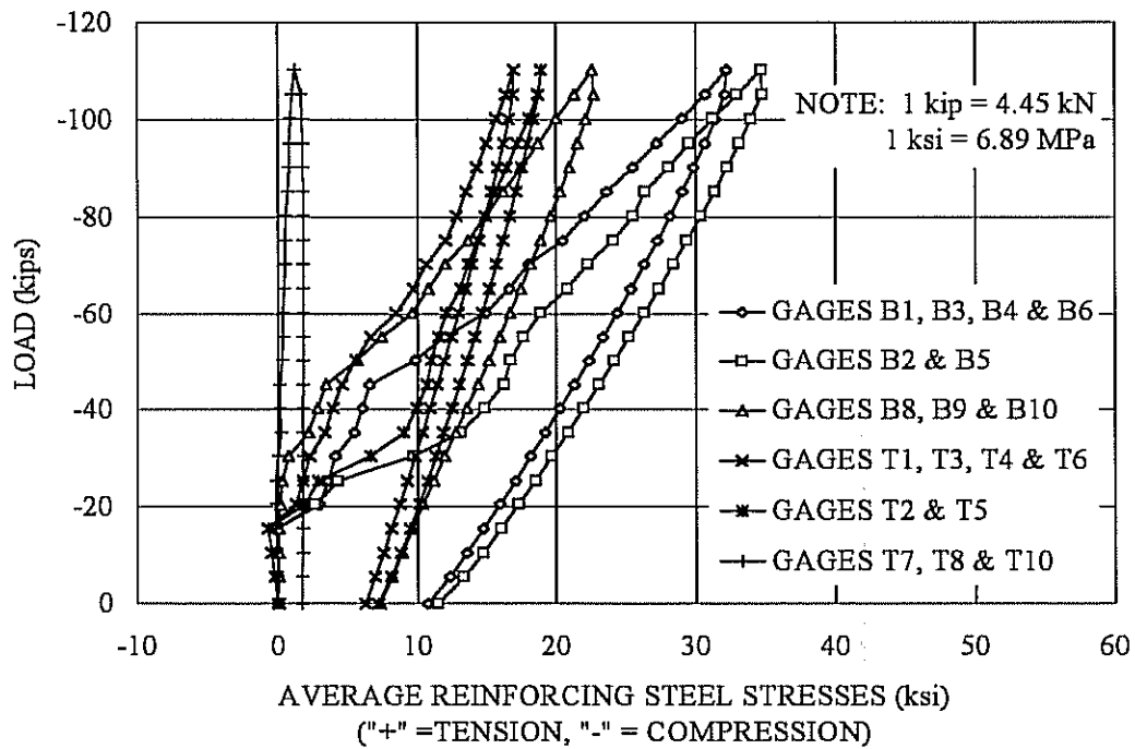
Figure 6.6: Typical reinforcing steel stresses in cast-in-place pulsating fatigue test specimens (shown is the initial loading cycle for Specimen S3P110).
