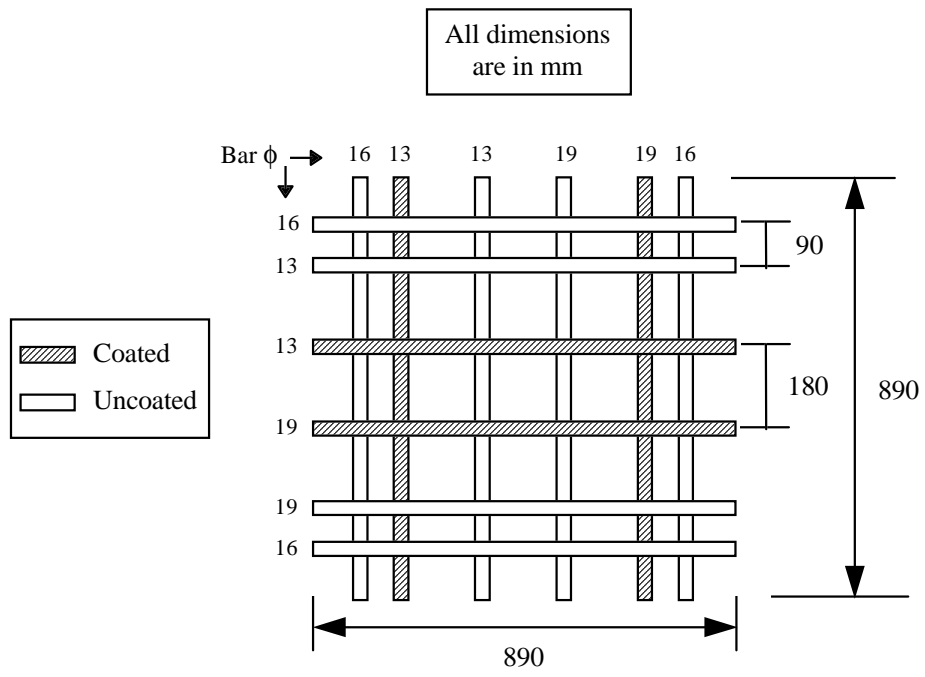
a) Reinforcement Mats
