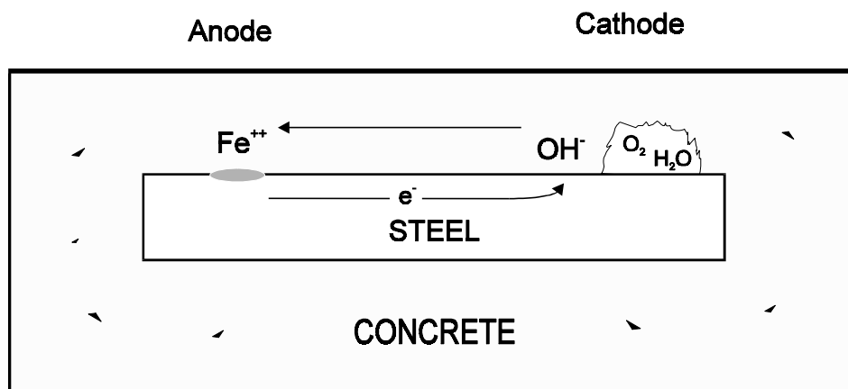
Figure 1.1 Corrosion cell in reinforced concrete
