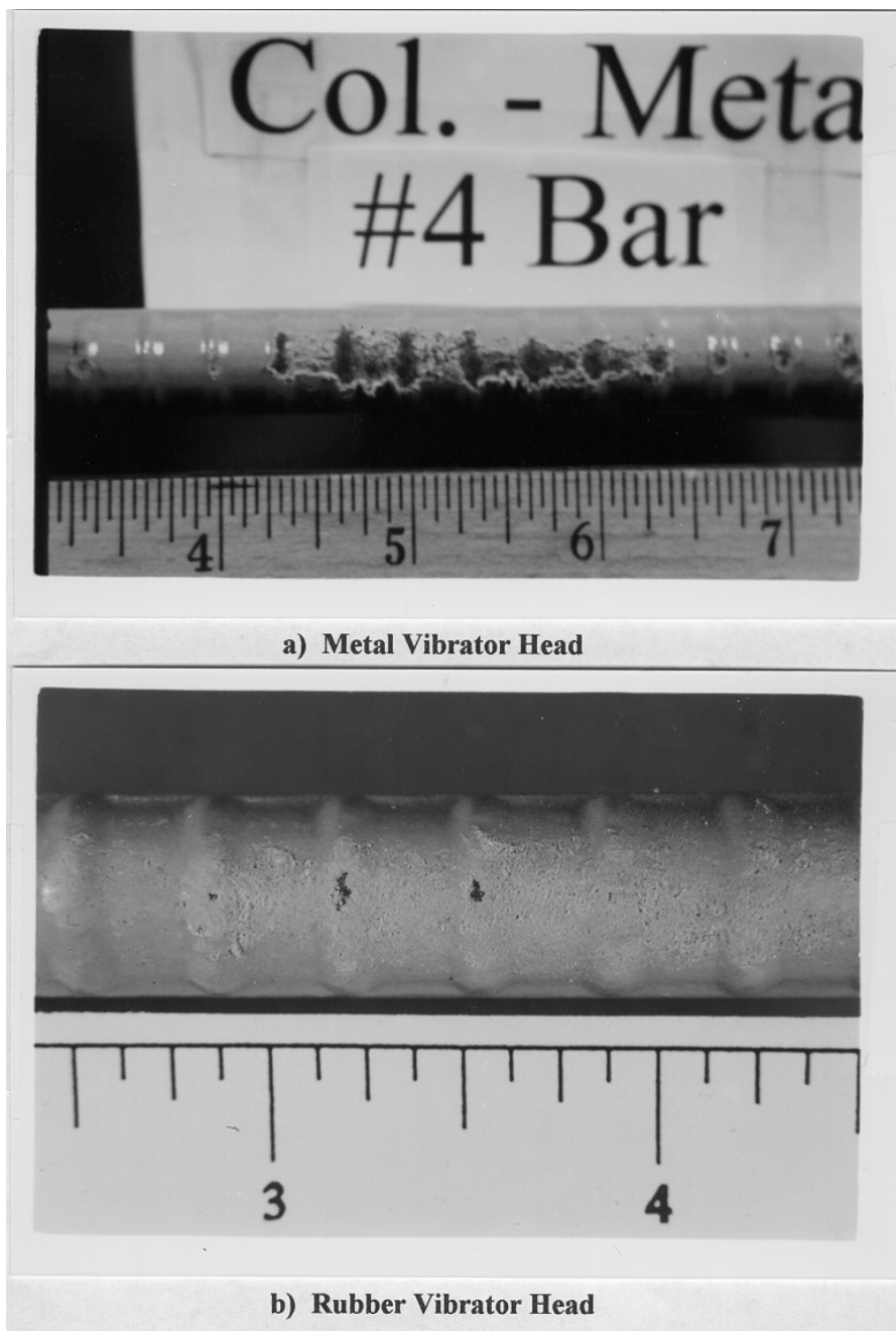
Figure 2. 19 Vibration damage to epoxy coating
