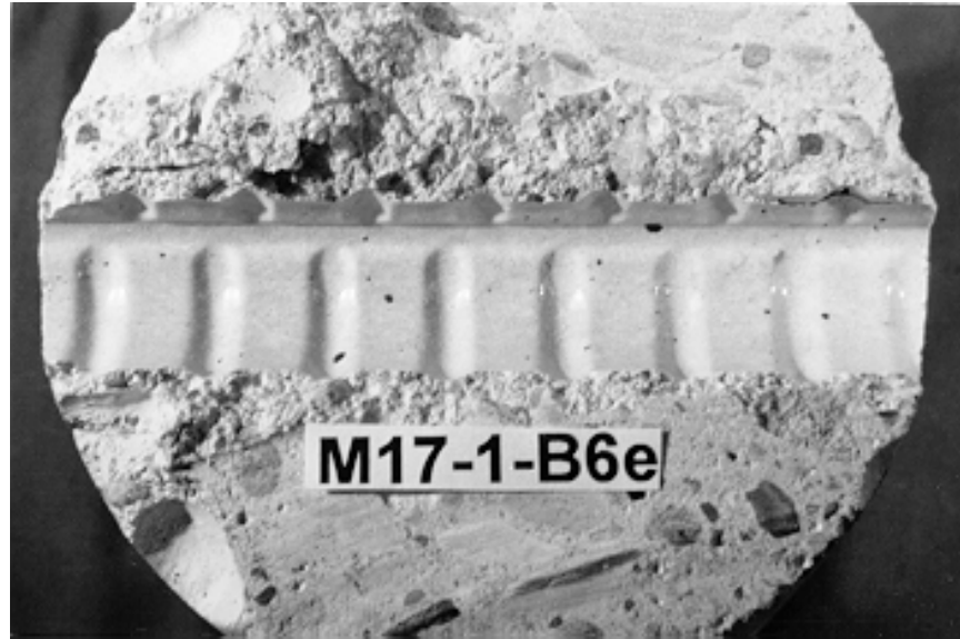
Figure 4. 19 Smooth and shiny surface under epoxy-coated rebar
