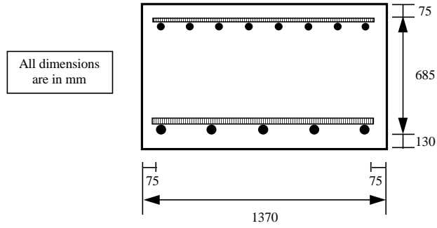
Figure 2.3 Details of footing specimen
