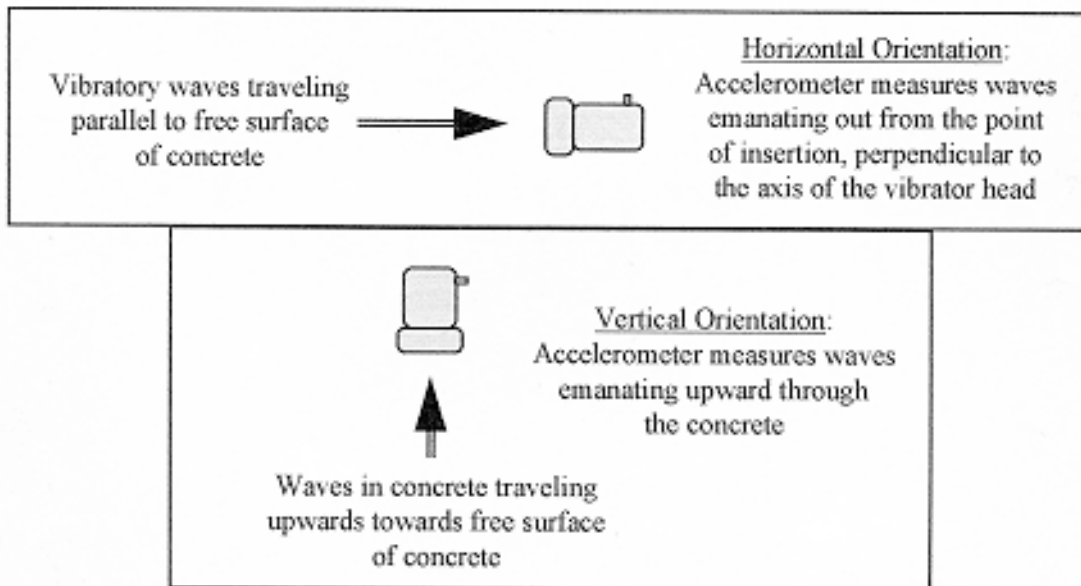
Figure 3. 5 Accelerometer orientation
