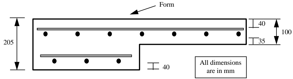
Figure 2.5 Details of deck specimen
