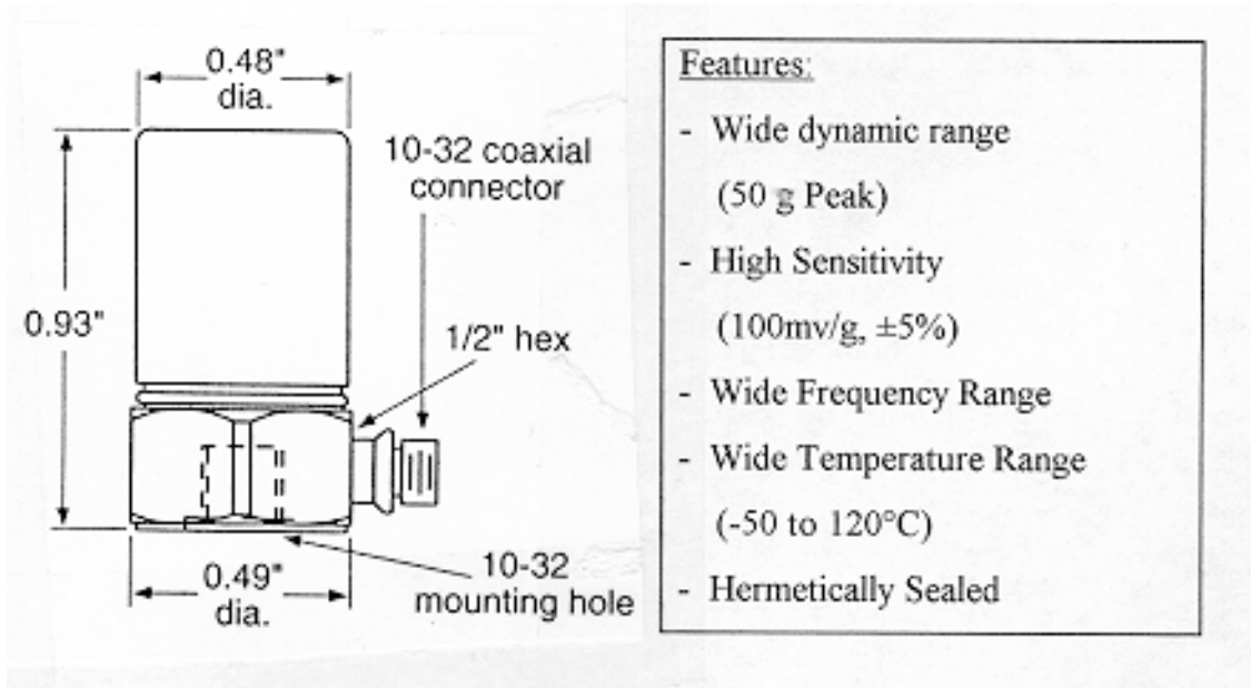
Figure 3. 4 Accelerometer features
