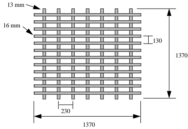
a) Upper Mat of Reinforcement
