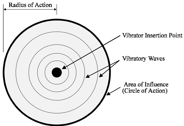
Figure 1.4 Area of influence for concrete vibrator
