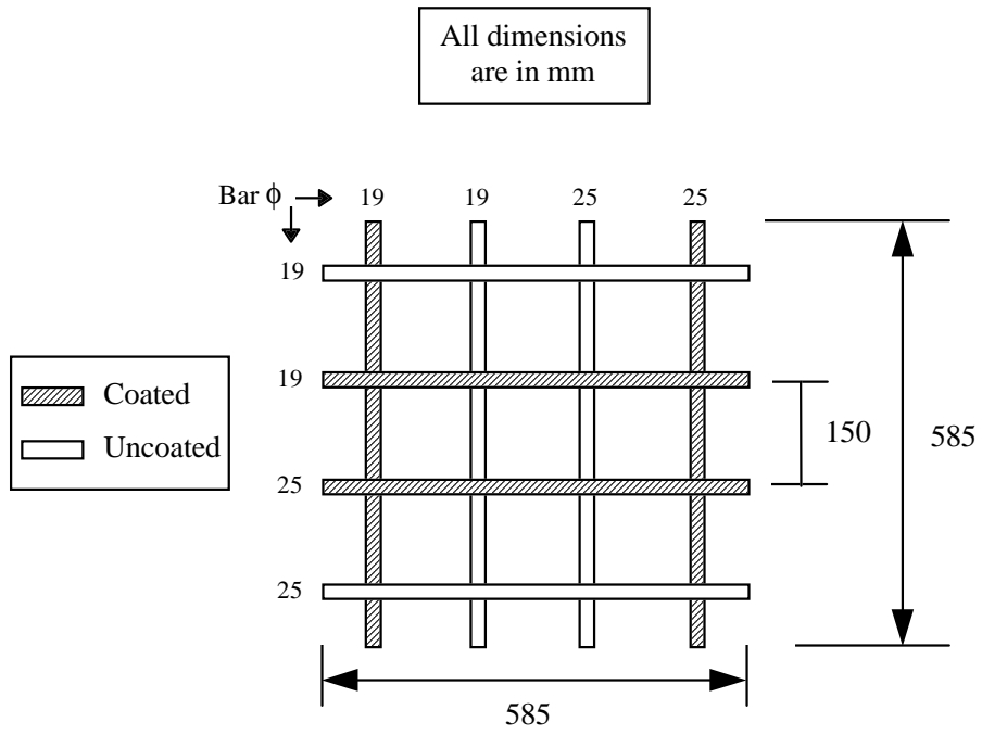
a) Reinforcement Mats
