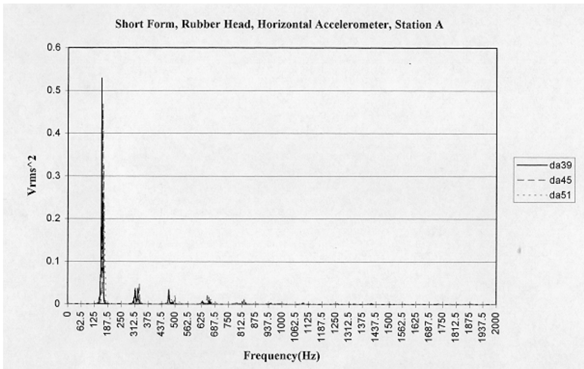
Figure 3.7 Typical power spectrum record
