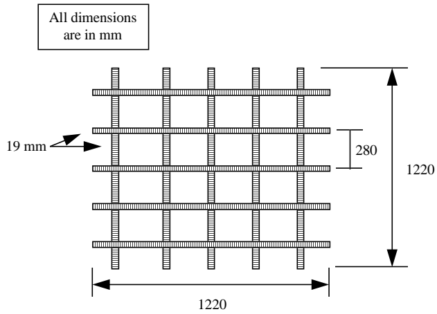
b) Lower Reinforcement Mat
