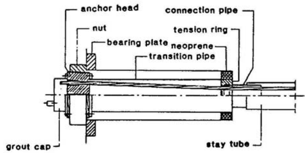
Figure 1-5 Anchor head anchorage device 90
