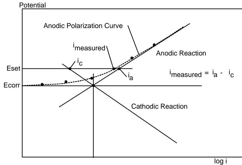
Figure 2- 8 Anodic polarization curve
