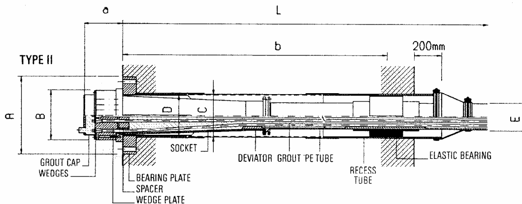
Figure 3-7 State-of-the-art stay cable anchorage developed by Dywidag 41
