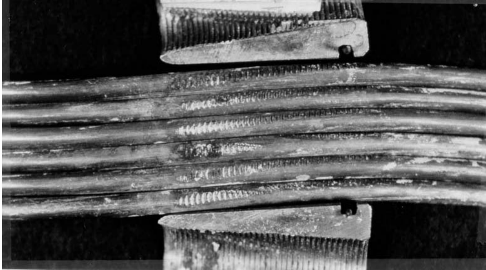
Figure 8- 24 Corrosion at the interface between the strand and wedge
