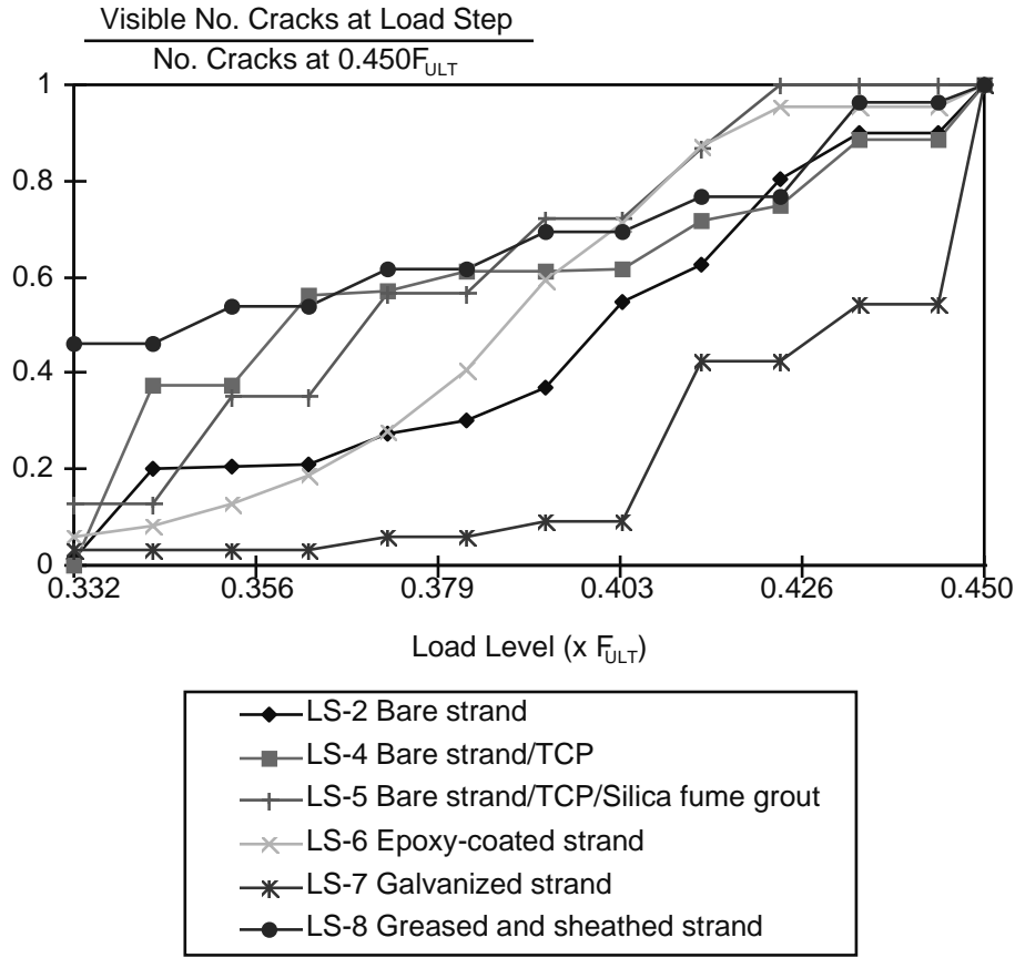
Figure 7-24 Cumulative cracking of specimens
