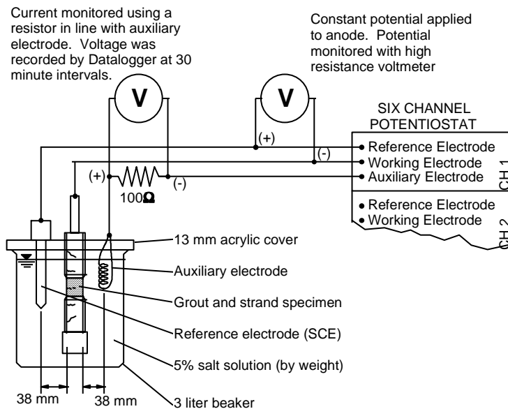
Figure 6-2 Instrumentation for anodic polarization test
