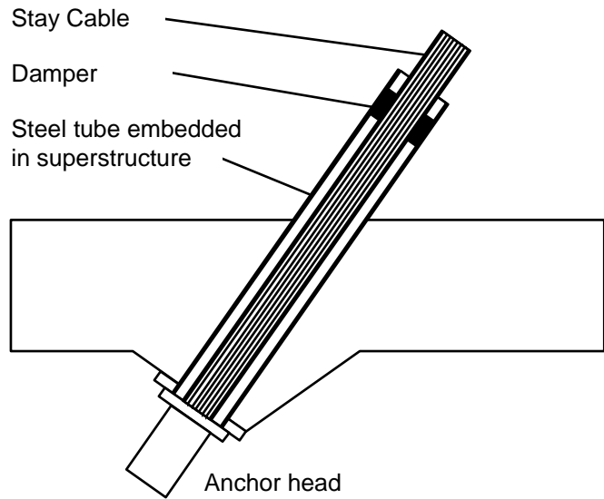
Figure 7-19 Schematic of stay damper
