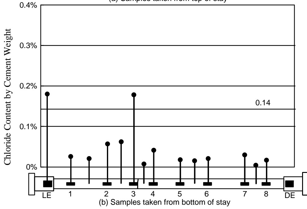
Figure 8-15 Grout chloride content for Specimen LS-6
