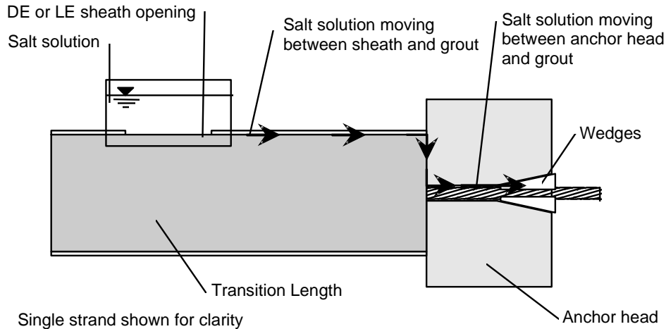
Figure 9- 12 Schematic of chloride transport mechanism
