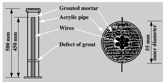
Figure 1-12 Specimen schematic for environmental tests 75
