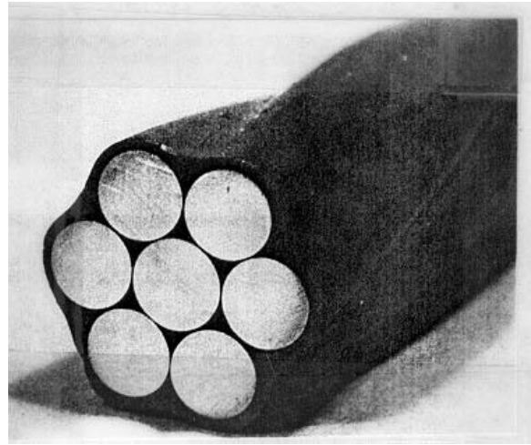
Figure 3-2 Epoxy-coated strand 45
