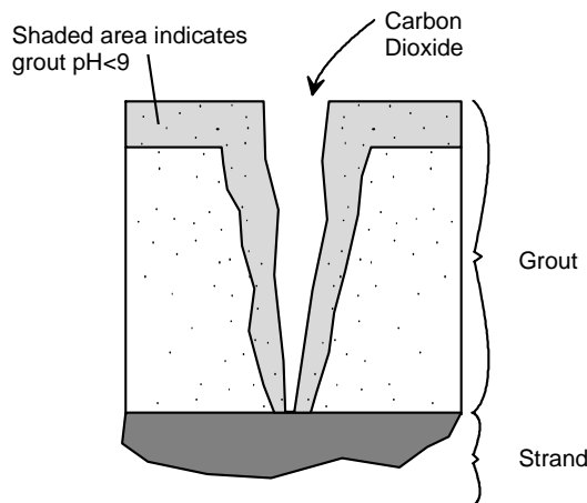
Figure 2-5 Carbonation of crack in grout
