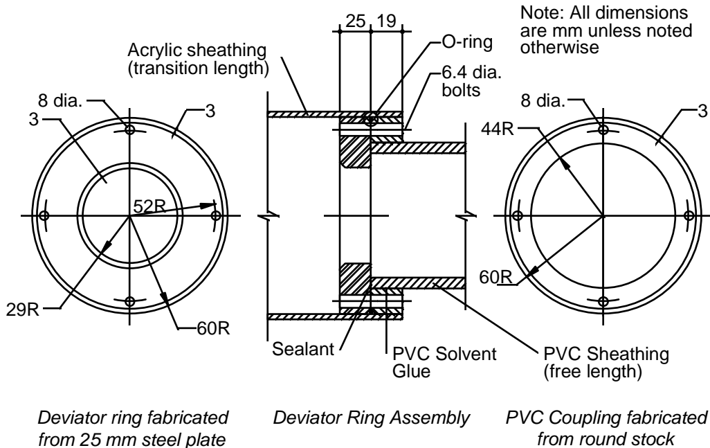
Figure 7-7 Deviator ring details
