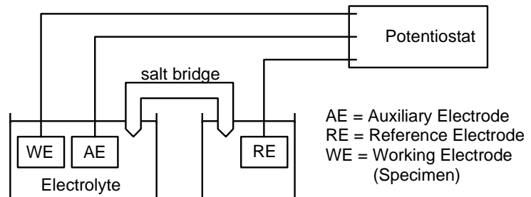
Figure 2-7 Schematic of anodic polarization with potentiostat
