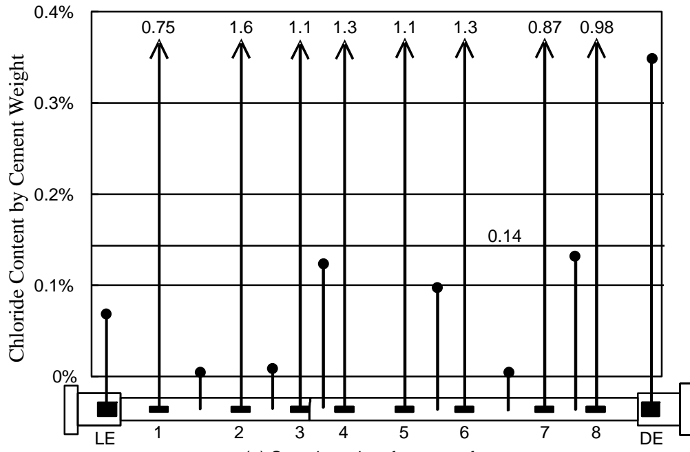
(a) Samples taken from top of stay
