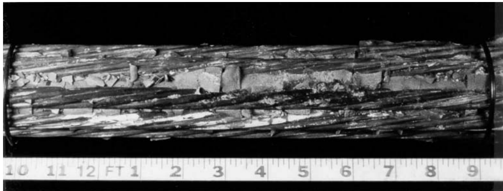
(c) Corroded strands uncovered during post-mortem examination
