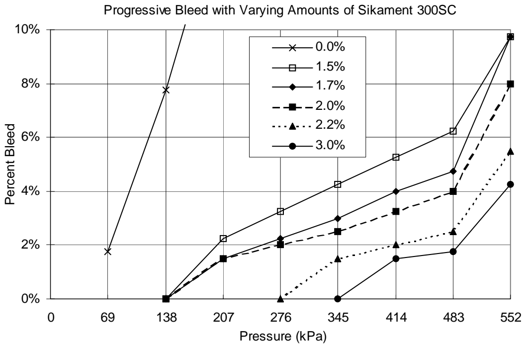
Figure 5-1 Comparison of Antibled Admixtures.
