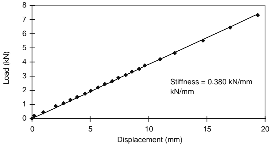
Figure 7- 23 Typical load-displacement relationship from lateral load test
