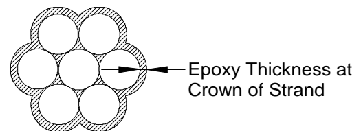
Figure 8-2 Crown thickness of epoxy-coated strand
