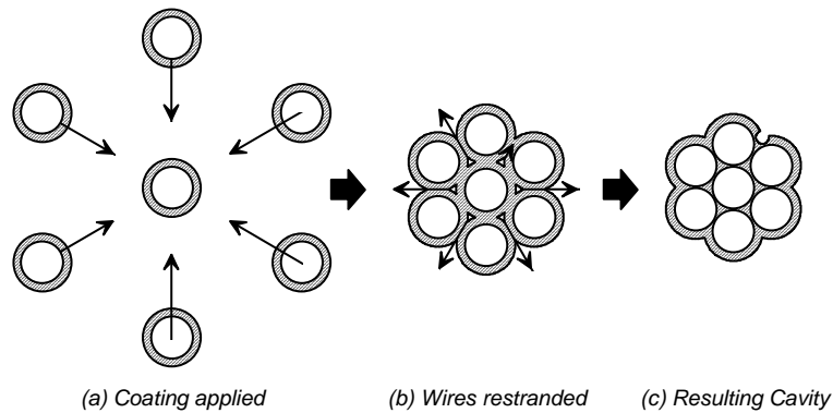
Figure 8-4 Cause of cavity in surface of epoxy-coated strand
