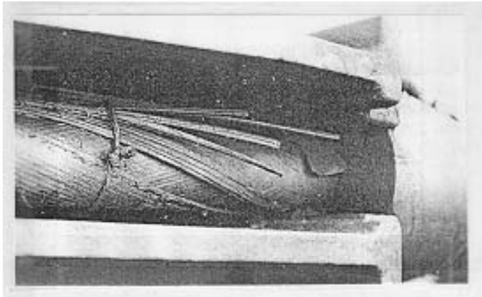
Figure 1- 11 Broken wires at lower cable anchorage on Köhlbrand Bridge
