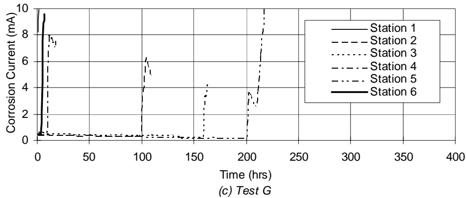
Figure 6-3 Modified ACTM results for Tests E, F, and G
