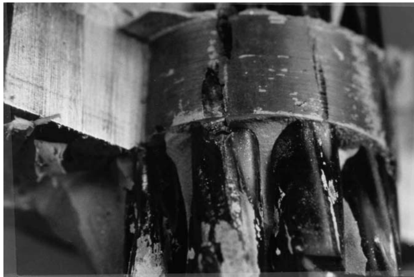
Figure 8- 32 Epoxy coating damaged by contact with deviator ring
