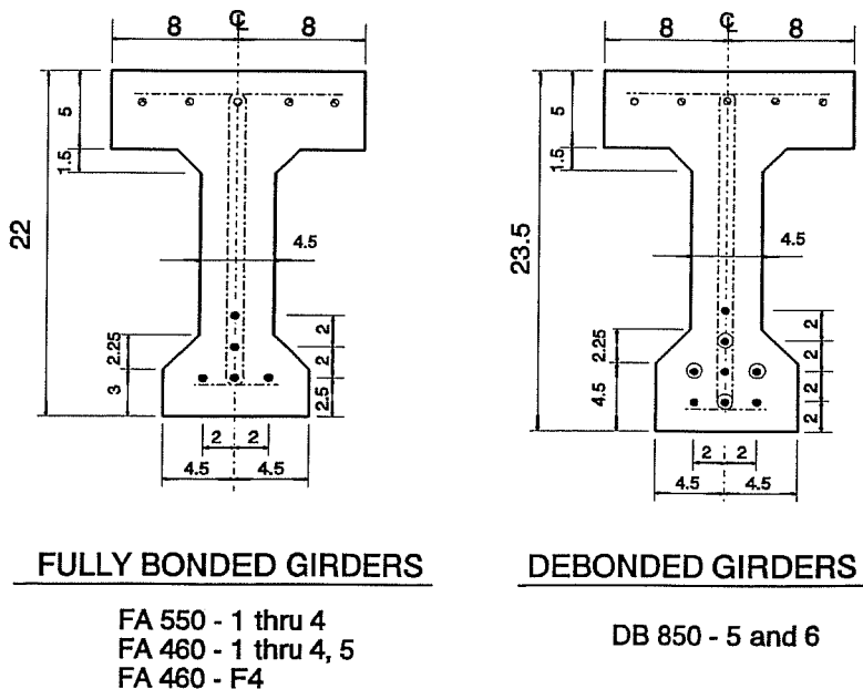
Figure 3.6 AASHTO-Type Girder Cross Sections
