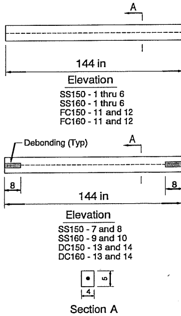
Figure 3.2 Details of Single Strand Specimens
