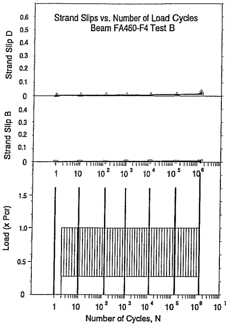
Figure 6.11 Loading History: Beam FA460-F4 Test B
