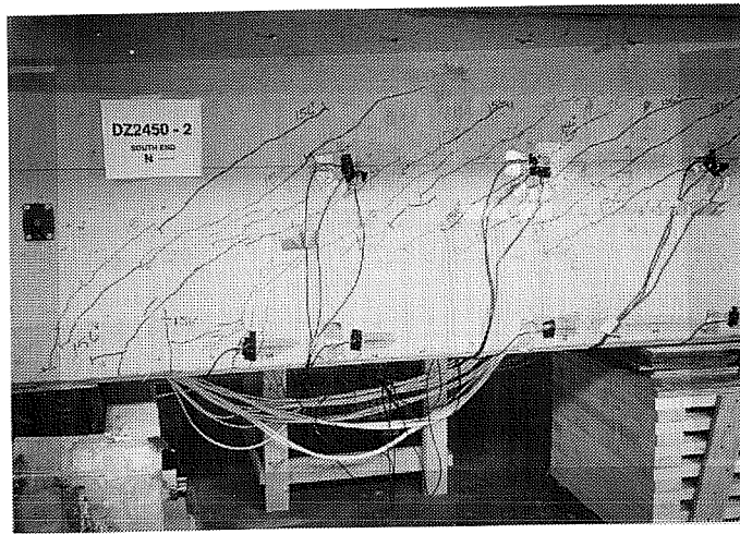
Figure 7.33 Cracking Pattern at P = 140 kips, DZ2450-2
