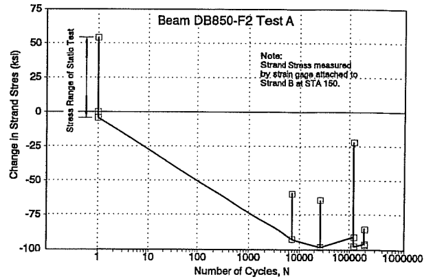
Figure 6.27 Changes in Strand Stress From Repeated Loads
