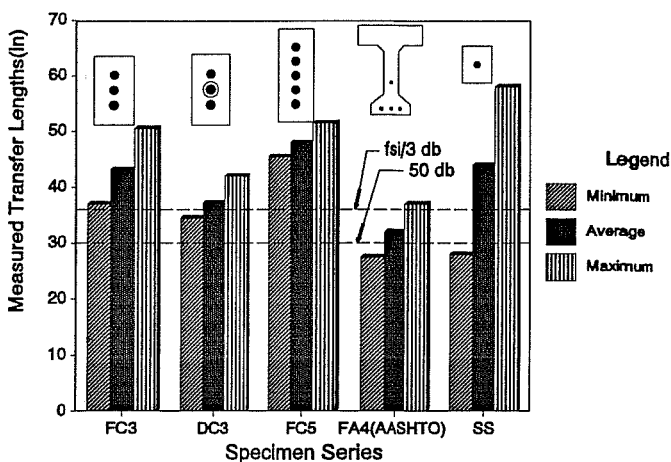
Figure 3.21 Transfer Lengths, 0.6 Inch Strand. Summary by Specimen Series
