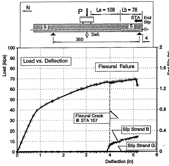
Figure 5.18 Beam DB850-3 Test B
