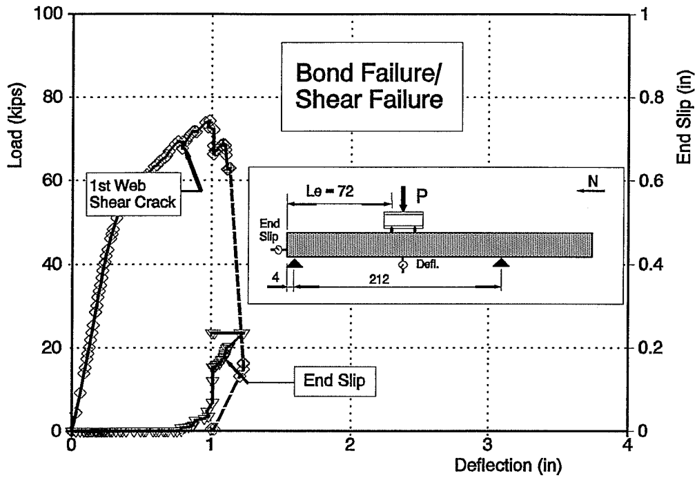
Figure C4. Beam FA550-2 Test A
