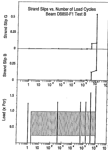
Figure 6.15 Loading History: Beam DB850-F1 Test B
