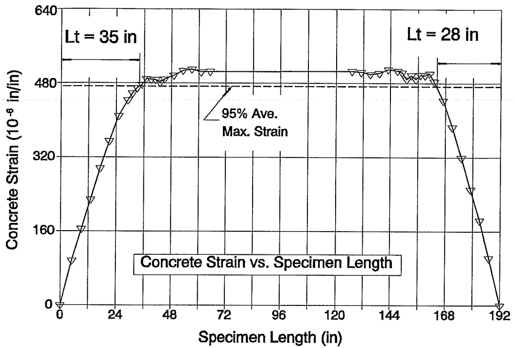
Figure A21. FC350 - 1 , Transfer Length
