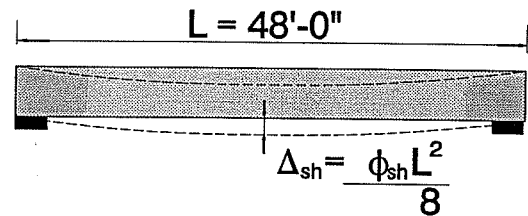
Figure 7.43 Deflection From Shrinkage
