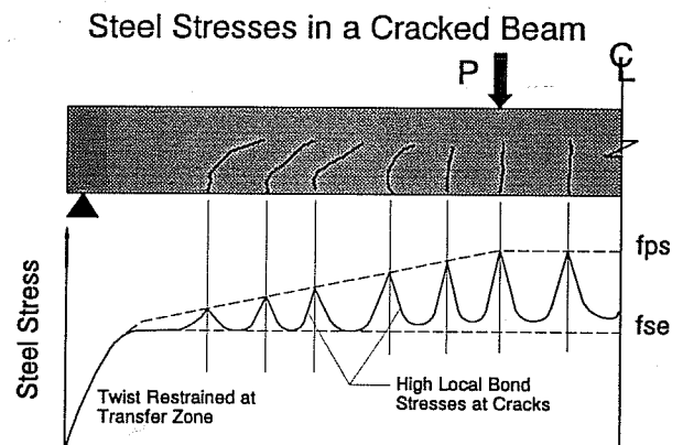
Figure 2.4 Pretensioned Steel Stresses in a Cracked Beam
