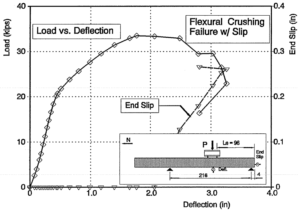
Figure C24. Beam FR350-2 Test B
