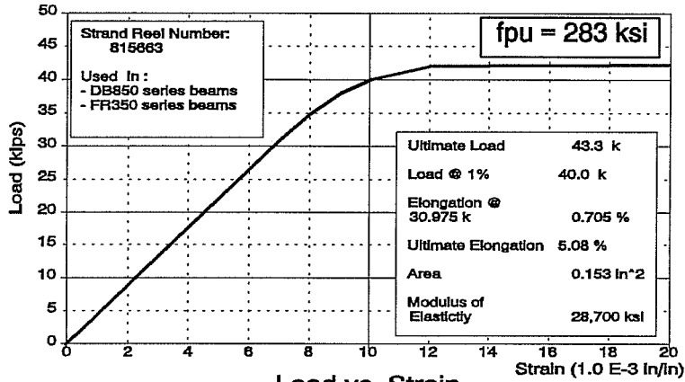
0.5 Inch Diameter Low Relaxation Strand
