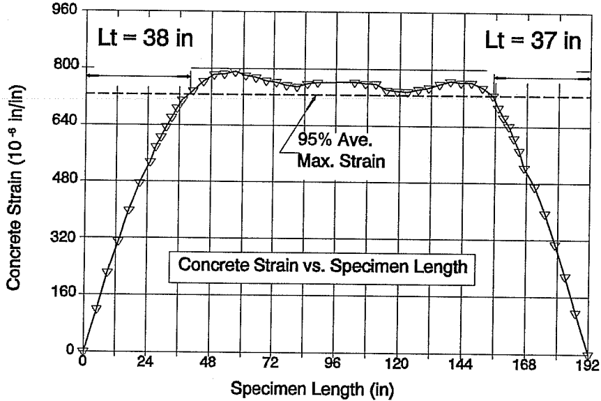
Figure A27. FC550 - 1 , Transfer Length
