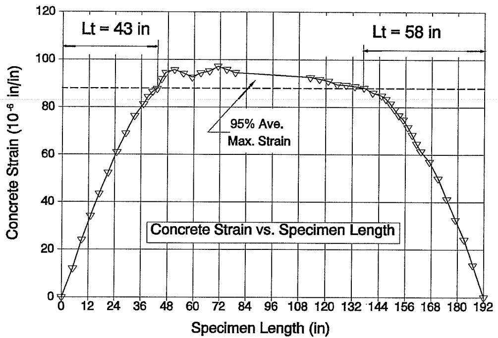
Figure A40. FCT360 - 3 , Transfer Length
