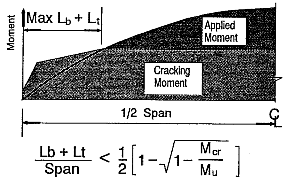
Figure 8.9 Maximum Debond Length (Applied Moment [Uniform Load] vs. Cracking Moment)
