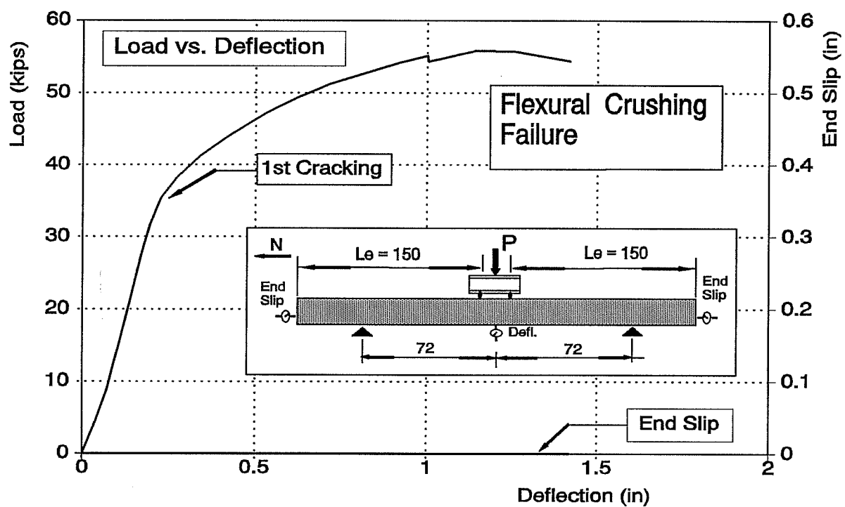
Figure C22. Beam FR350-1 Test C
