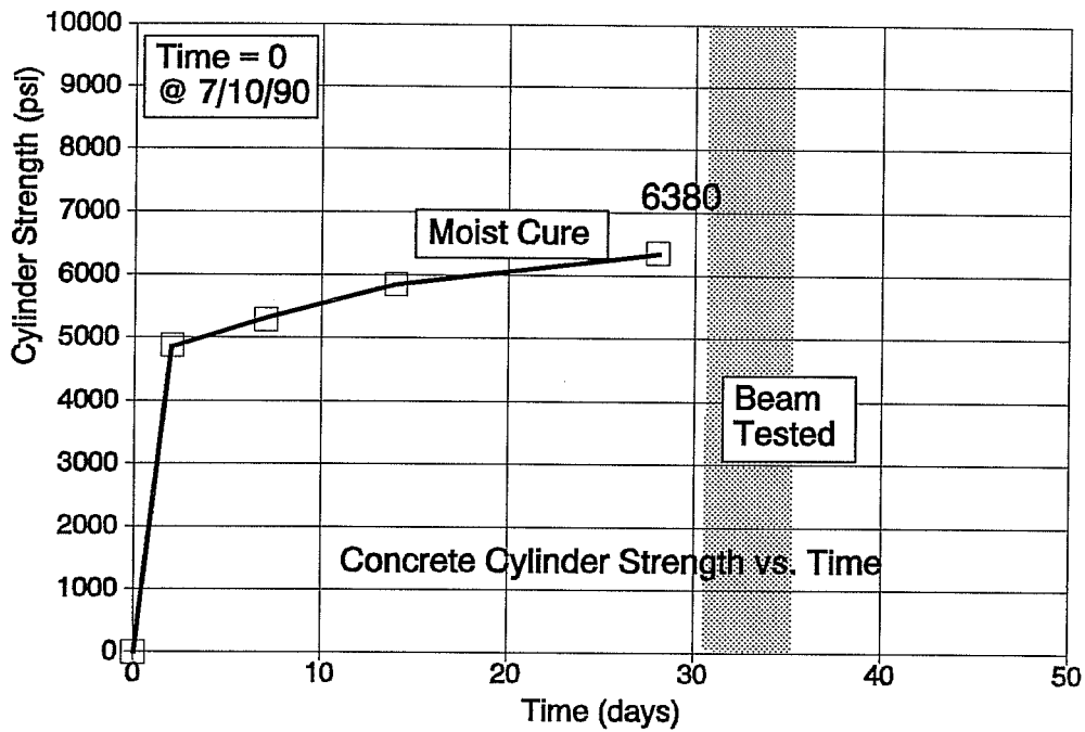
Figure B4. Beam FA460-1
