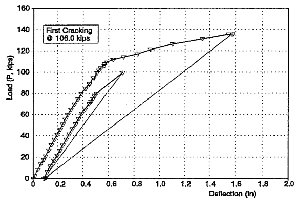
Figure 7.26 Initial Static Test, Beam FZ2450-3
