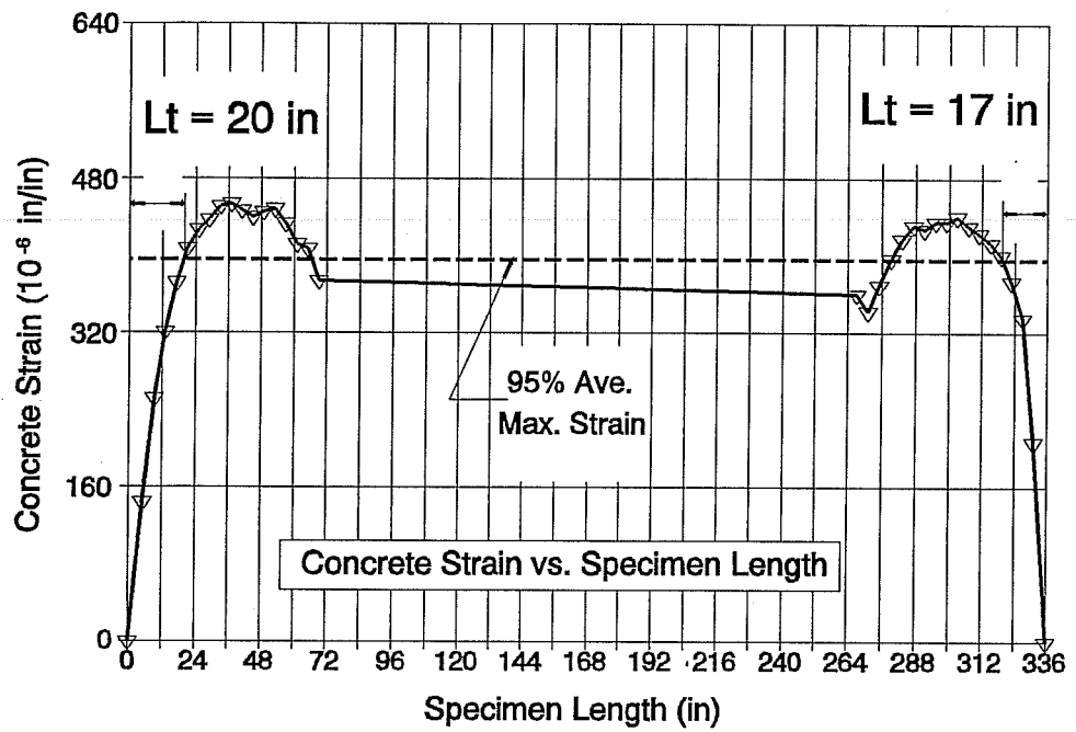
Figure A32. FA550 - 3 , Transfer Length
