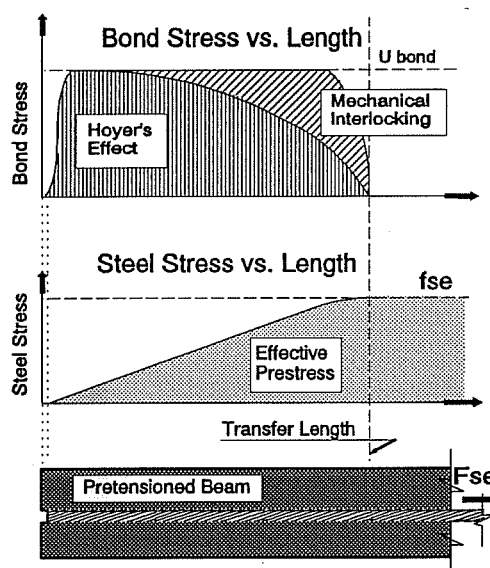
Figure 2.5 Idealization of Bond Mechanics in Transfer Zones
