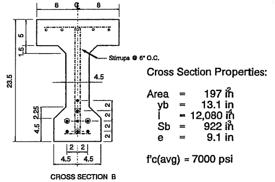
Figure 5.8 Cross Section for DB850 Beams
