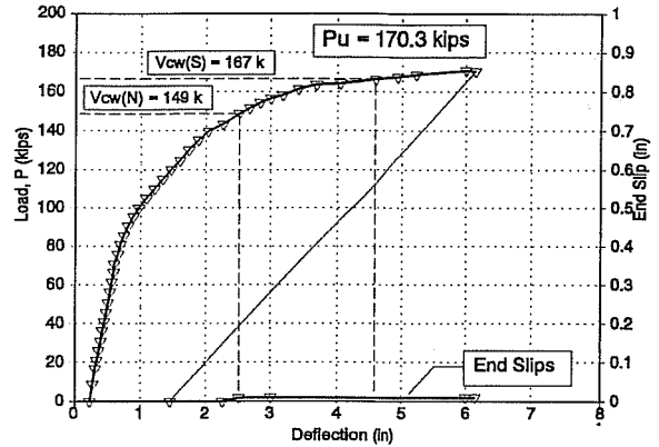
Figure 7.37 Final Static Test, Girder DZ2450-1
