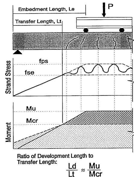
Figure 8.7 Interaction of Transfer Length and Development Length
