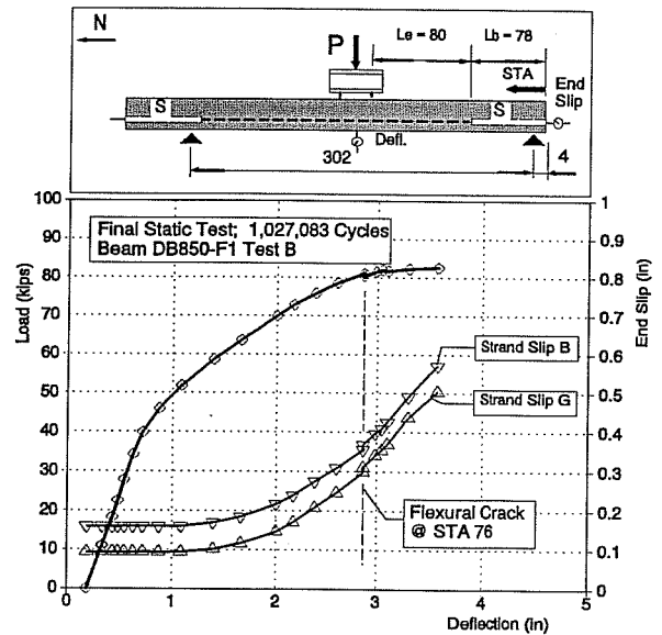
Figure 6.16 Load vs. Deflection and End Slips Beam DB850-F1 Test B
