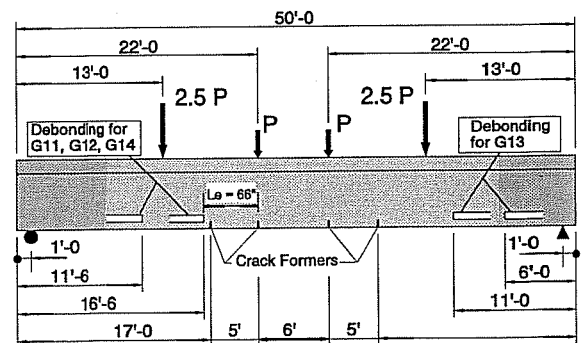
Figure 5.3 Fatigue Tests on Debonded Girders; Rabbat, Kaar, Russell and Bruce (1979)
