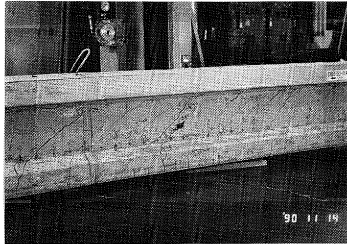
Figure 5.21 Photograph of Cracking Pattern, DB850-5A
