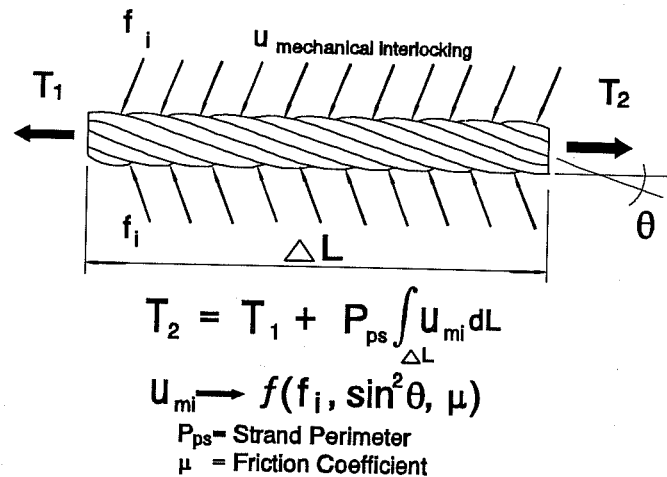
Figure 2.3 Mechanical Interlocking
