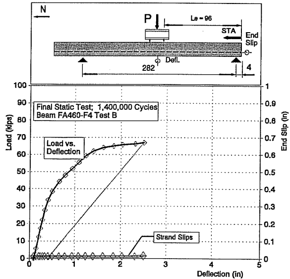
Figure 6.12 Load vs. Deflection and End Slips Beam FA460-F4 Test B
