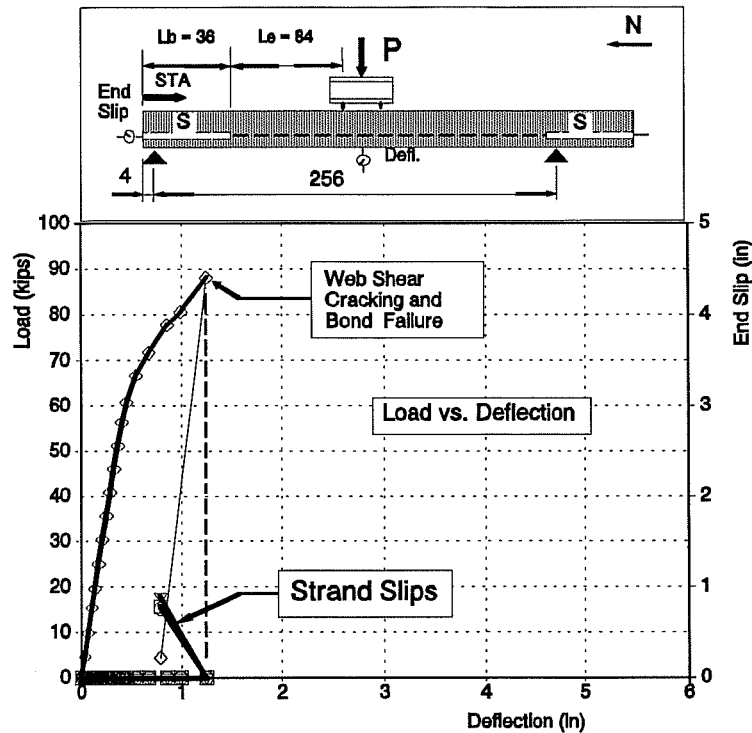
Figure 5.25 Beam DB850-1 Test A
