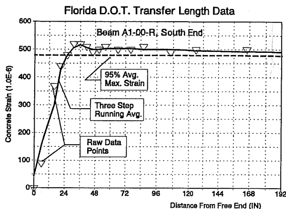
Figure 3.13 Strain Profile from FDOT Type II Girder
