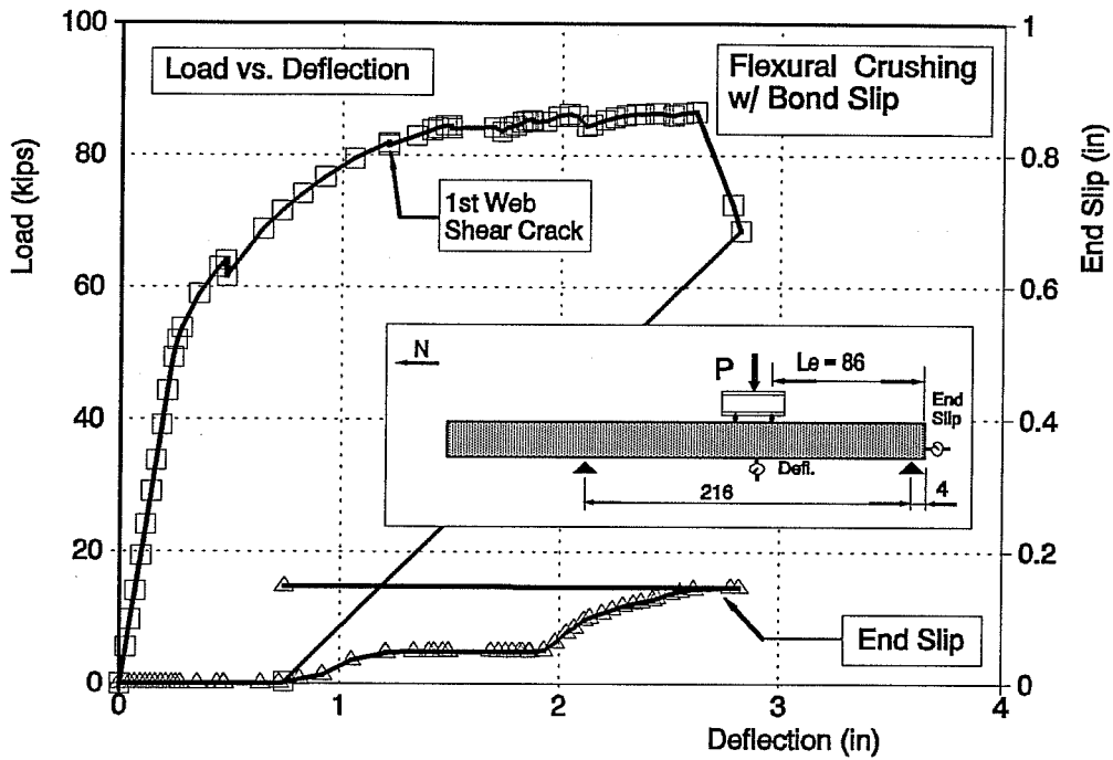
Figure C12. Beam FA460-2 Test A
