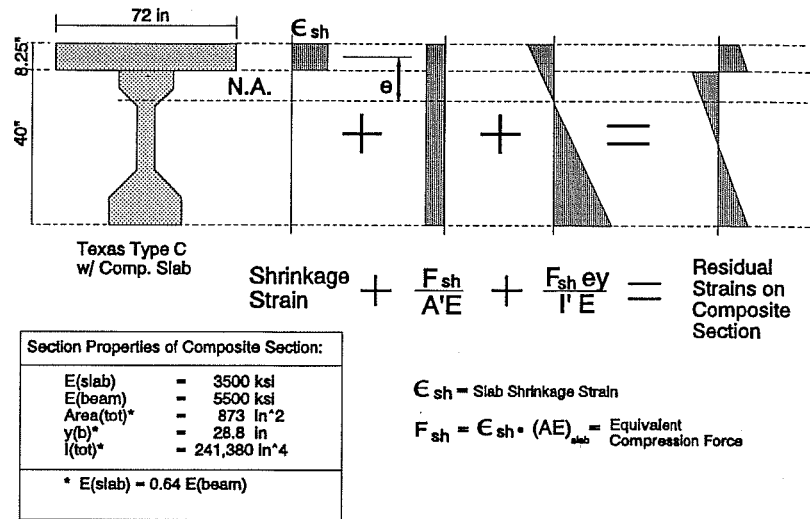
Figure 7.44 Residual Strains From Slab Shrinkage
