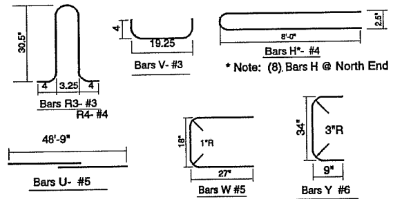
Figure 7.7 Reinforcement Details, DZ2450-2
