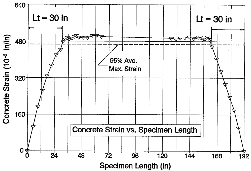
Figure A23. FCT350 - 3 , Transfer Length
