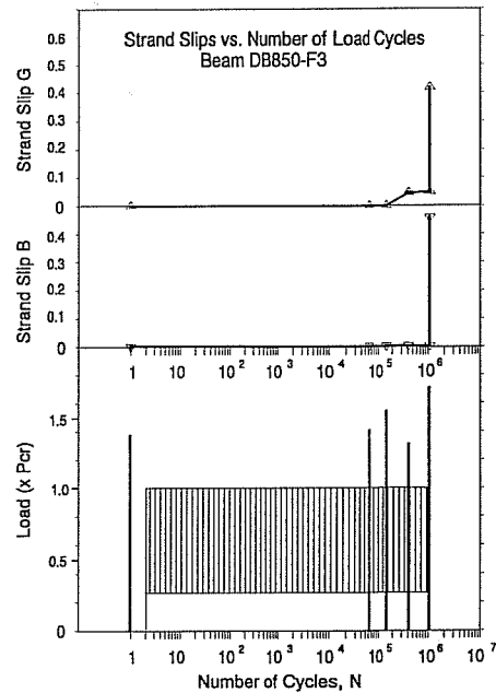
Figure 6.21 Loading History: Beam DB850-F3
