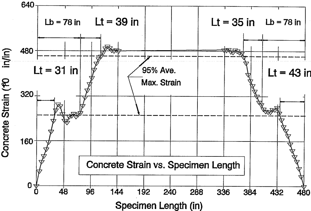
Figure A34. DB850 - 5 , Transfer Length
