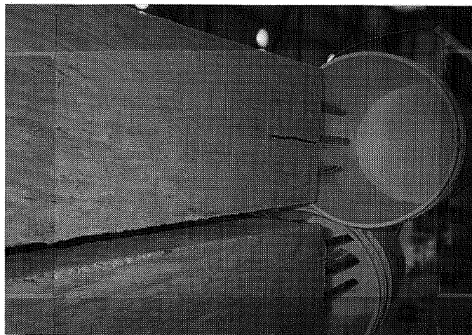
Figure 4.23 Photograph of Splitting Crack, Beam FR360-1A, Before Testing
