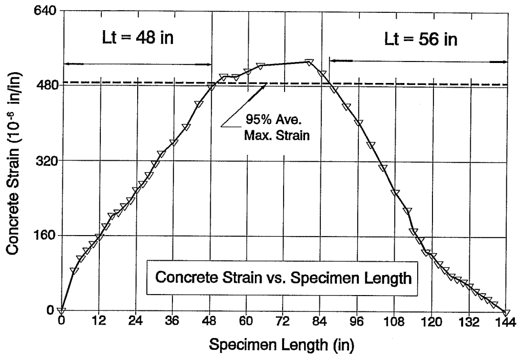
Figure A11. SS160 - 3 , Transfer Length
