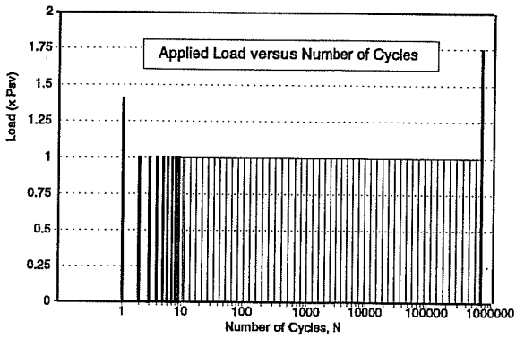
Figure 7.23 Loading History, Girder DZ2450-1
