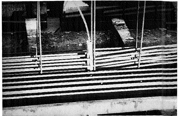
Figure 7.10 Draping Hold-Down
