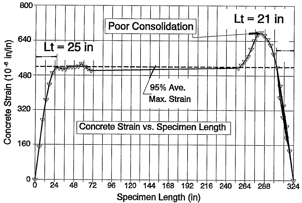
Figure A31. FA550 - 2 , Transfer Length
