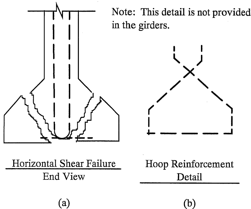
Figure 7.35 Horizontal Shear Failure, Girder DZ2450-2
