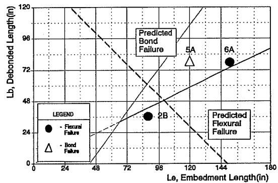
Figure 5.34 Overlay of Test Results (Concurrently Debonded Beams)
