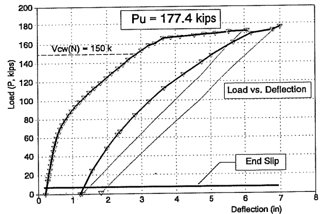
Figure 7.28 Final Static Test, Girder FZ2450-3
