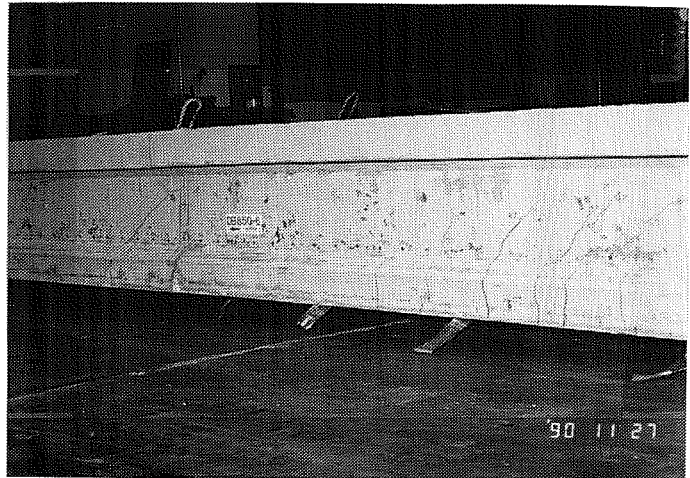
Figure 5.23 Photograph of Cracking Pattern, DB850-6A
