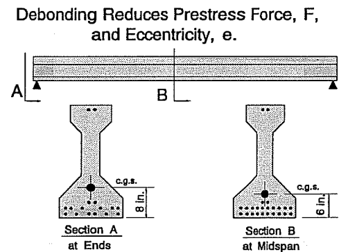
Figure 8.10 Change in Eccentricity From Two Top Strands Used With Debonded Strands
