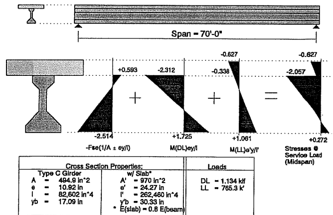
Figure 7.3 Design Stresses for Composite Section
