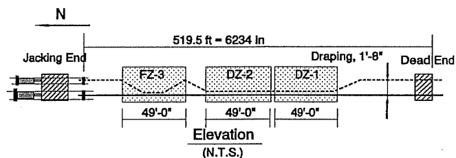
Figure 7.9 Schematic Evaluation of Pretensioning Bed
