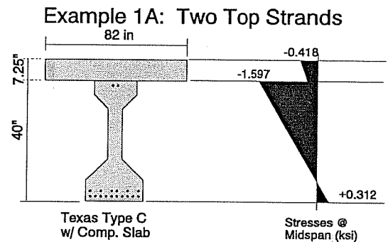
Figure 8.11 Service Load Stresses at Midspan, 60'-0 Span
