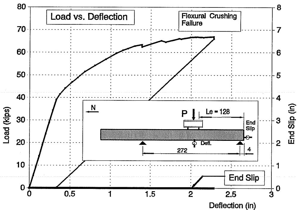
Figure C11. Beam FA460 - 1 Test B
