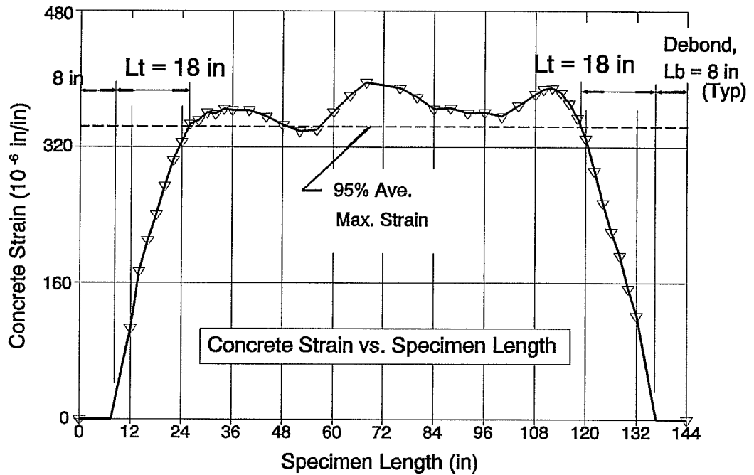
Figure A8. DC150 - 2 , Transfer Length
