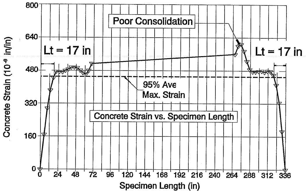
Figure A30. FA550 - 1 , Transfer Length
