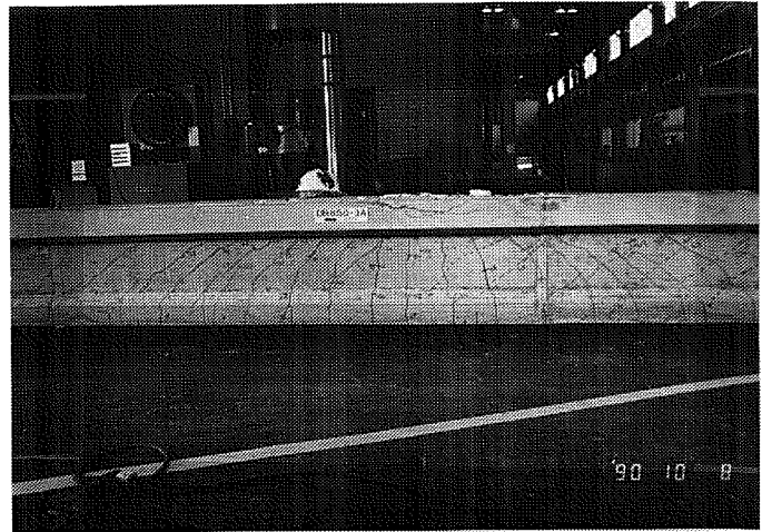
Figure 5.15 Photograph of Test DB850-3A Cracking Patterns
