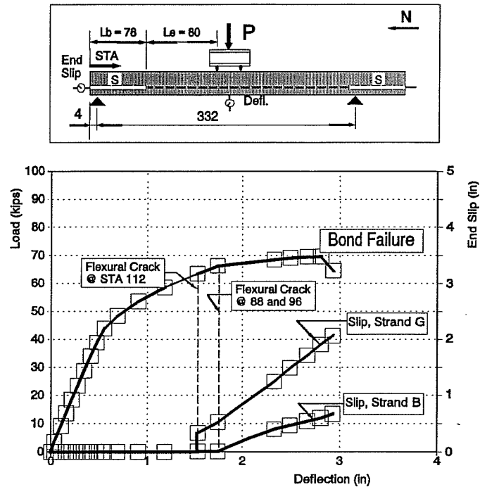
Figure 5.13 Beam DB850-3 Test A
