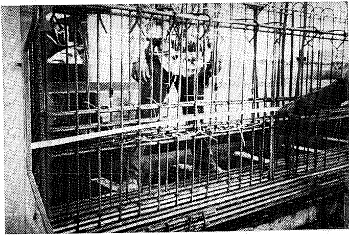
Figure 7.11 Photograph of Shear Reinforcement
