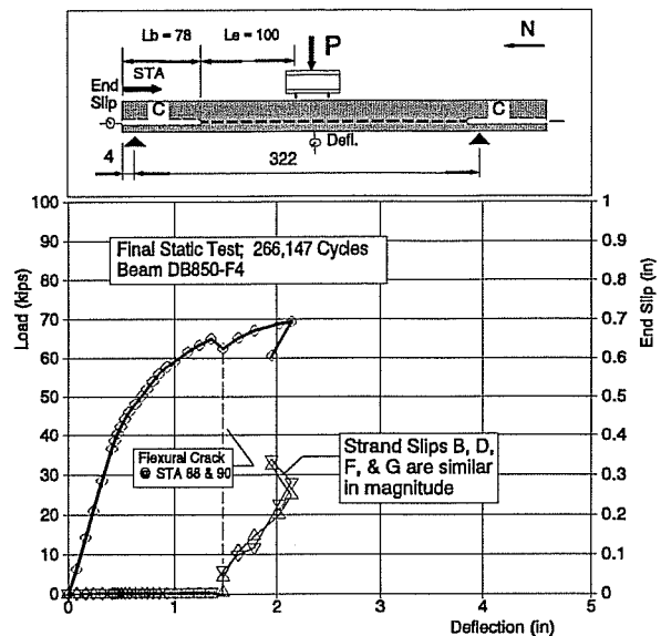
Figure 6.24 Load vs. Deflection and End Slips Beam DB850-F4
