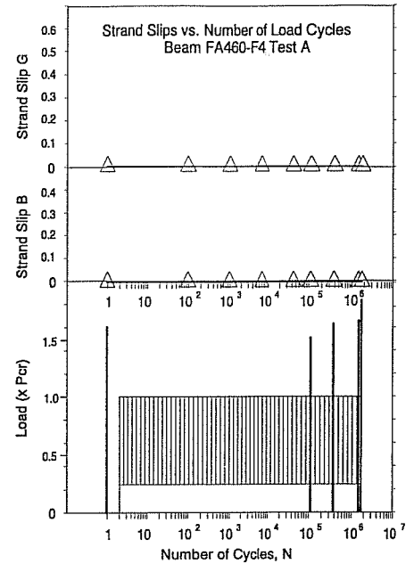
Figure 6.9 Loading History: Beam FA460-F4 Test A
