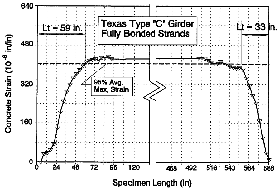
Figure 3.19 Strain Profile for FZ2450-3
