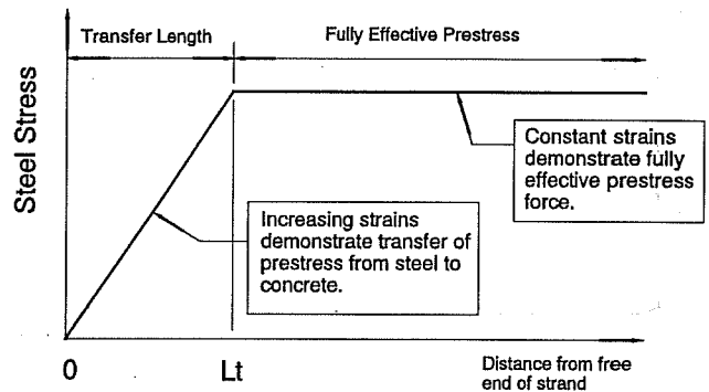
Figure 1.1 Idealized Steel Stress vs. Length for Pretensioned Concrete Member
