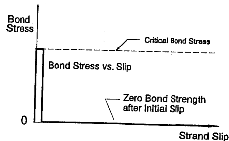
Figure 2.1 Adhesion: Rigid - Brittle Behavior
