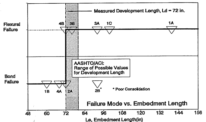
Figure 4.7 Development Length Tests: 0.5 Inch Strands in AASHTO-Type Beams
