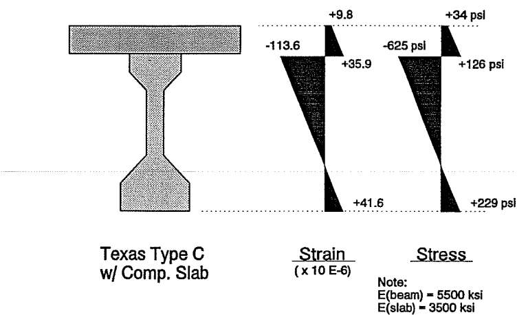
Figure 7.45 Residual Stresses and Strains From Slab Shrinkage, FZ2450-3
