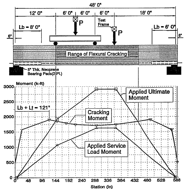
Figure 7.5 Applied Moment vs. Cracking Moment, Full-Sized Composite Girders
