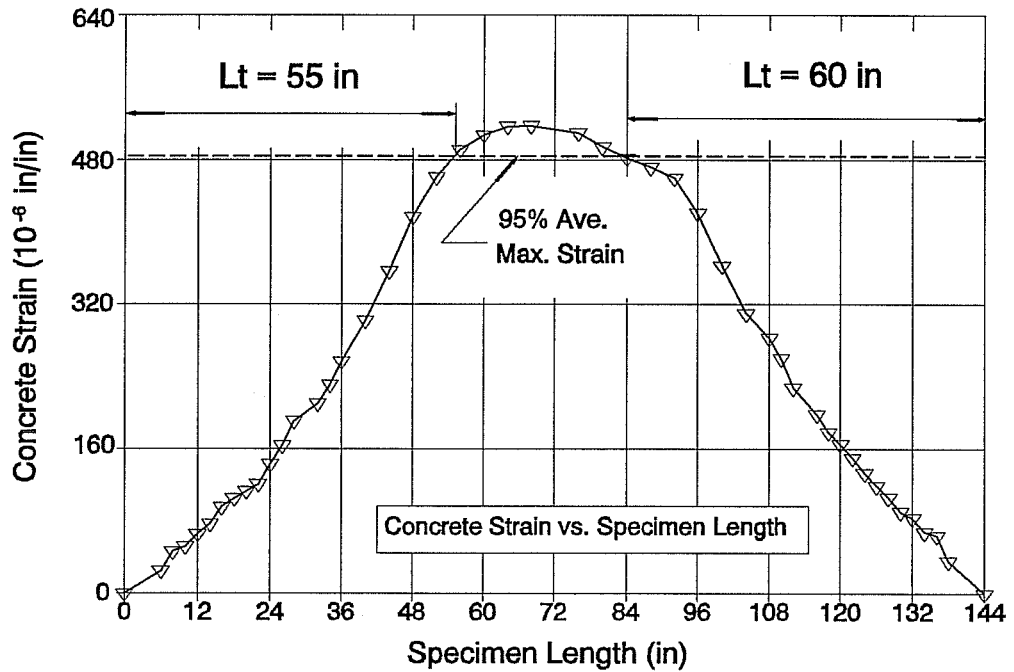
Figure A2. SS150 - 2 , Transfer Length
