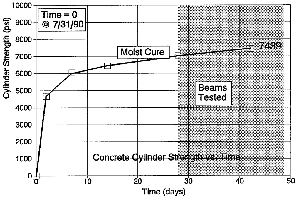
Figure B7. Beams FA460-5 and 6
