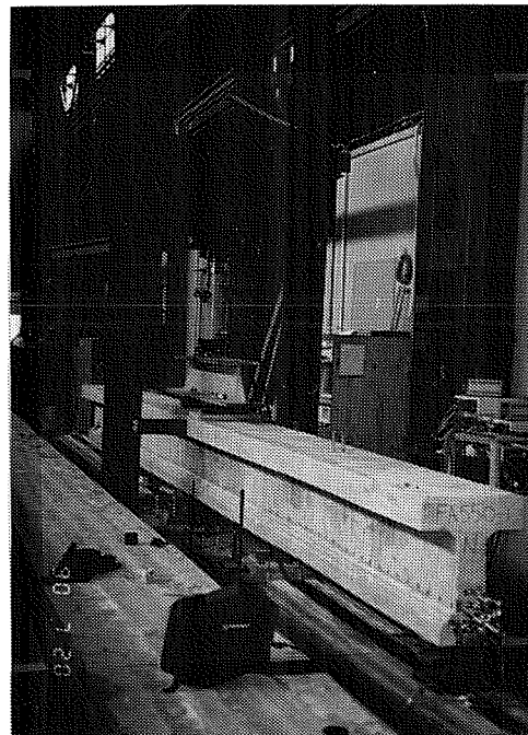
Figure 4.4 Testing Apparatus
