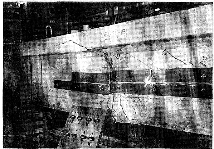
Figure 5.27 Web Shear Cracking and Bond Failure DB850-1B
