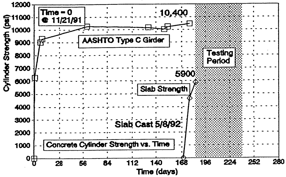
Figure 7.16 Concrete Cylinder Strengths: Girder DZ2450-1 and Bridge Deck
