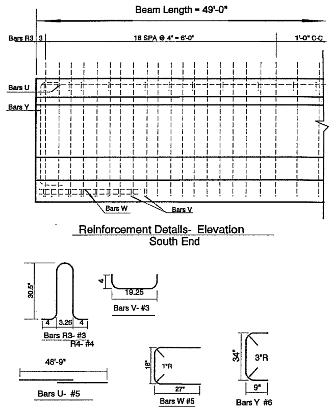
Figure 7.8 Reinforcement Details, FZ2450-3
