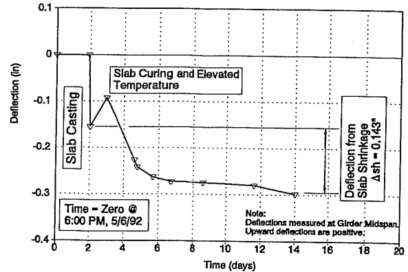
Figure 7.42 Time Dependent Deflections: DZ2450-1
