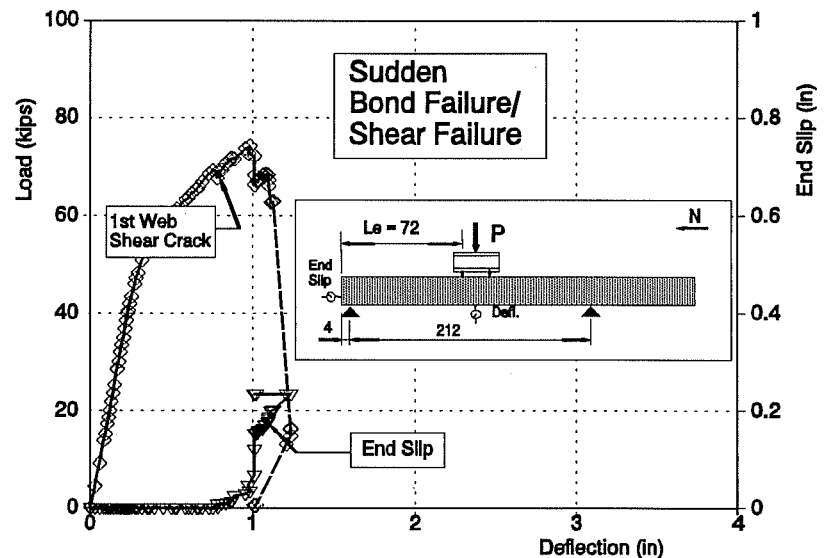
Figure 4.14 Beam FA550-2 Test B: Sudden Collapse Simultaneous Bond Failure and Shear Failure
