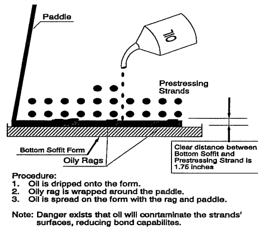
Figure 3.22 Form Oil Applied to Bottom Soffit Form in Pretensioning Plant
