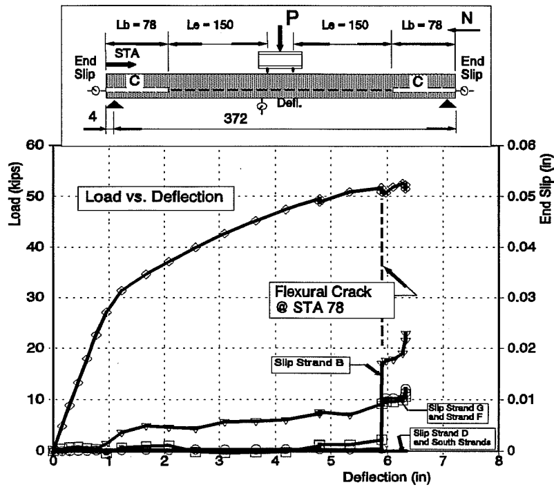
Figure 5.22 Beam DB850-6 Test A
