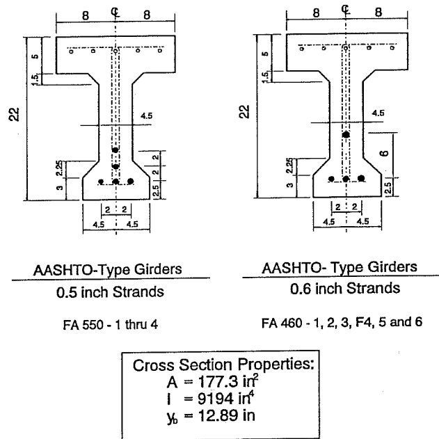
Figure 4.1 AASHTO-Type Girder Cross Sections
