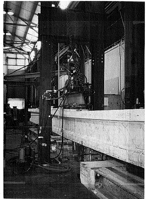
Figure 6.4 Photograph of Testing Apparatus
