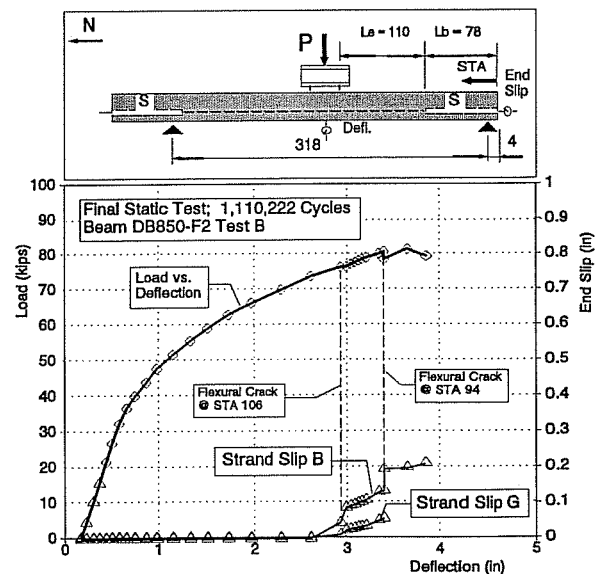
Figure 6.20 Load vs. Deflection and End Slips Beam DB850-F2 Test B
