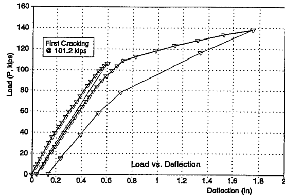
Figure 7.29 Initial Static Test, Beam DZ2450-2
