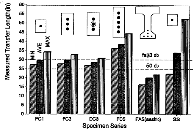
Figure 3.20 Transfer Lengths, 0.5 Inch Strands. Summary by Specimen Series, Fully Bonded
