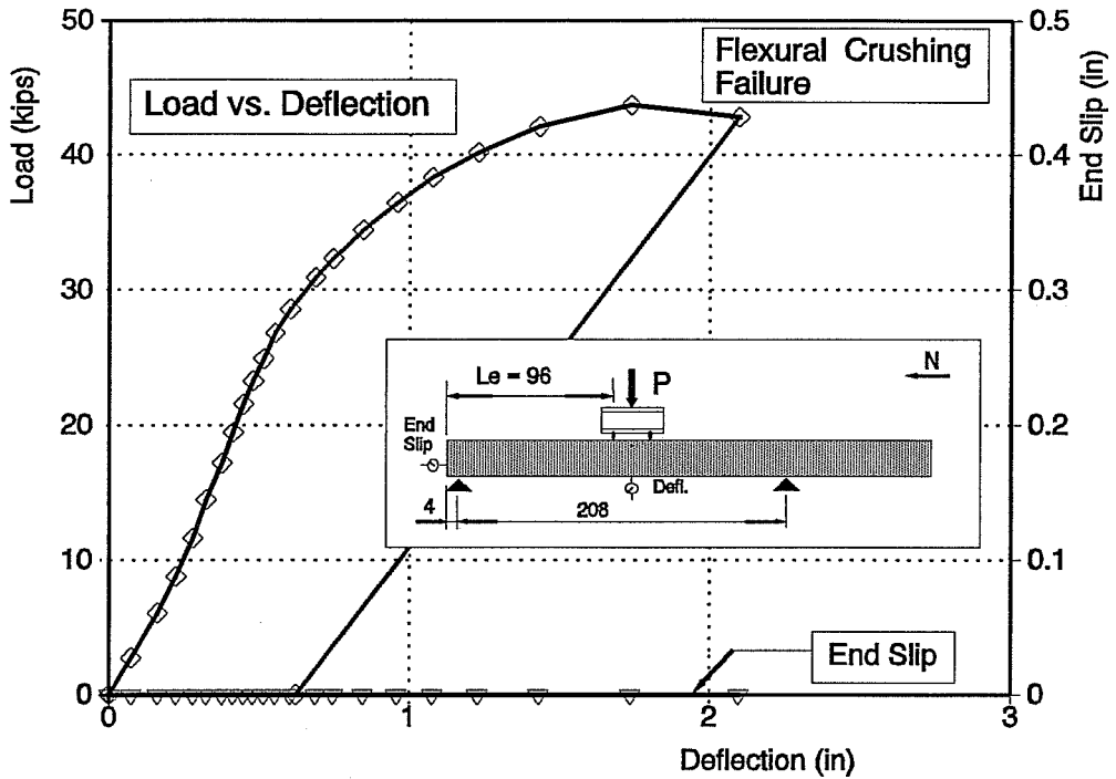
Figure C25. Beam FR360-1 Test A
