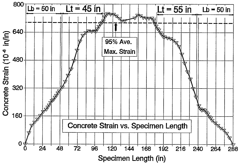
Figure A49. DCT360 - 10 , Transfer Length
