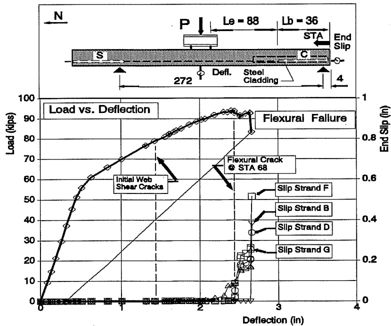
Figure 5.32 Beam DB850-2 Test B
