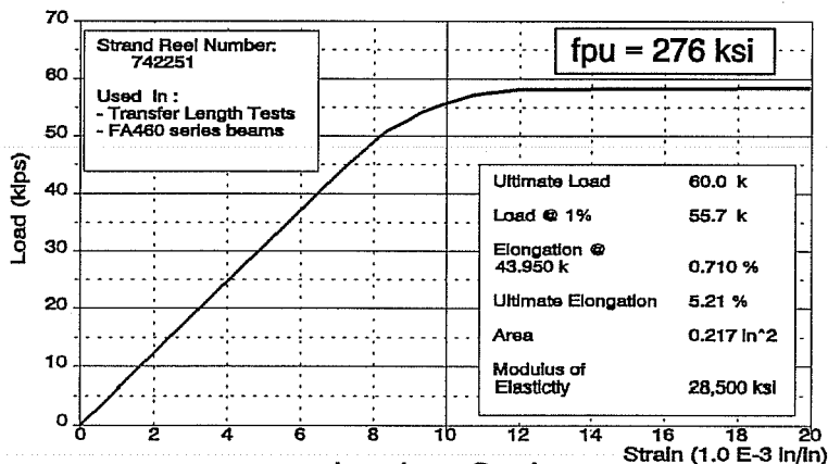
0.6 inch Diameter Low Relaxation Strand
