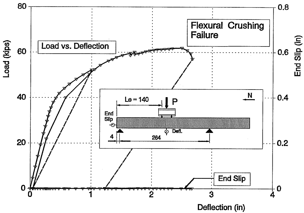
Figure C1. Beam FA550-1 Test A
