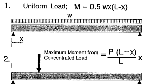
Figure 8.8 Loadings for Parabolic Moment Distributions
