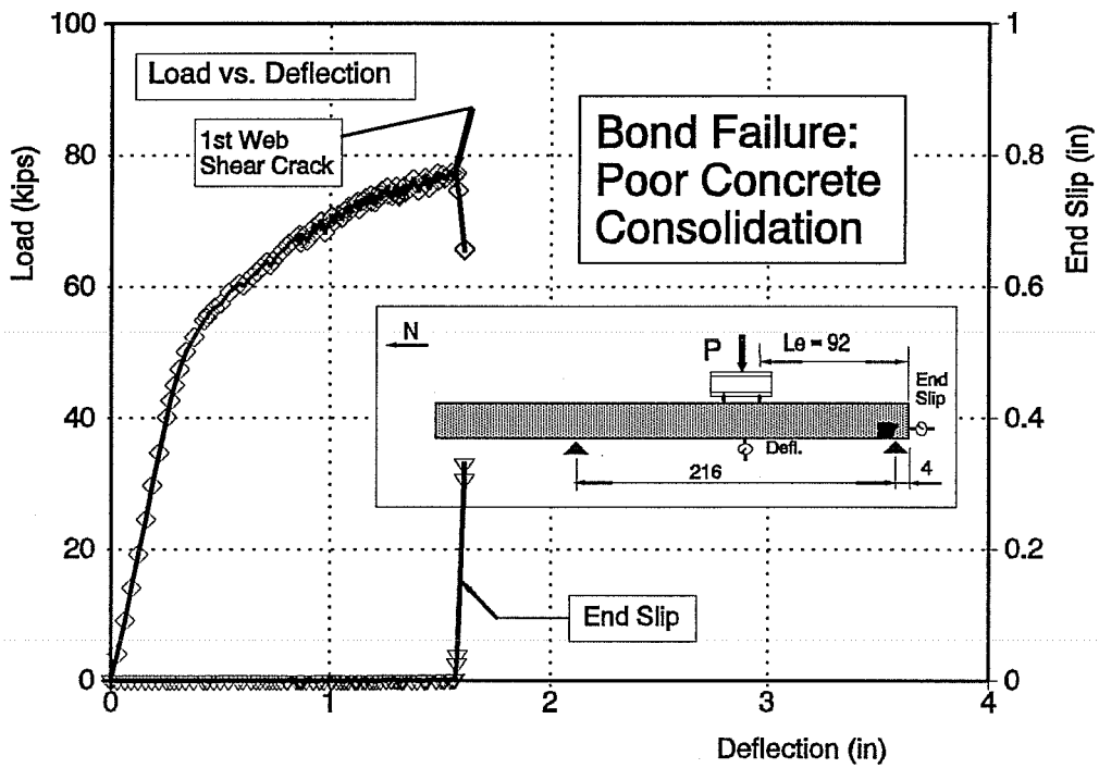
Figure C5. Beam FA550-2 Test B
