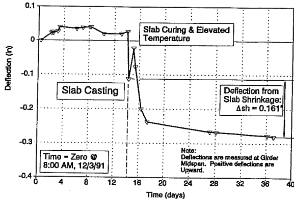
Figure 7.41 Time Dependent Deflections: FZ2450-3
