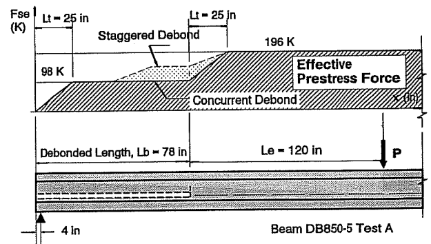
Figure 5.4 Effective Prestress Force (Beams With Debonded Strands)
