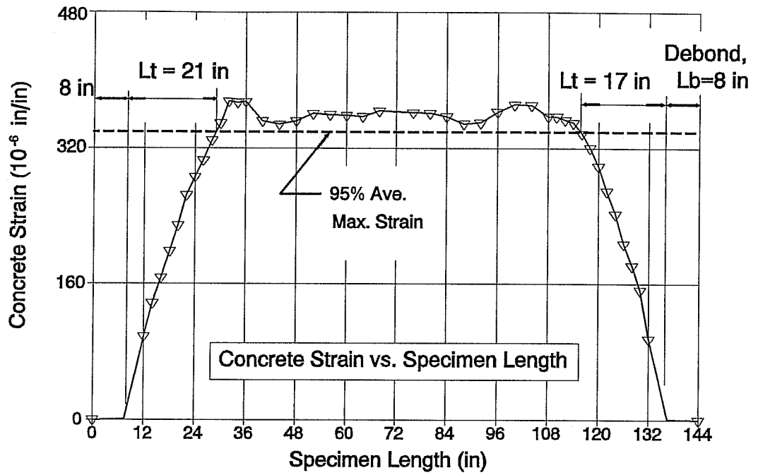
Figure A7. DC150 - 1 , Transfer Length
