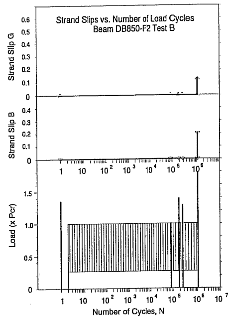
Figure 6.19 Loading History: Beam DB850-F2 Test B
