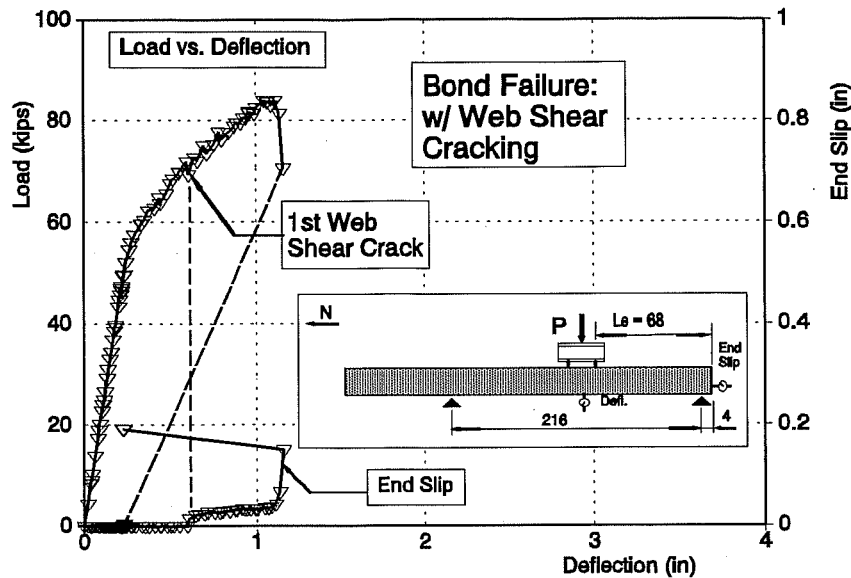
Figure 4.11 Beam FA550-4 Test A: Typical Shear/Bond Failure
