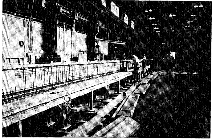
Figure 4.3 Fabrication of AASHTO-Type Beams
