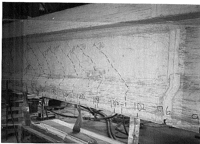
Figure 6.28 Test DB850-F2B at Load = 76 kips
