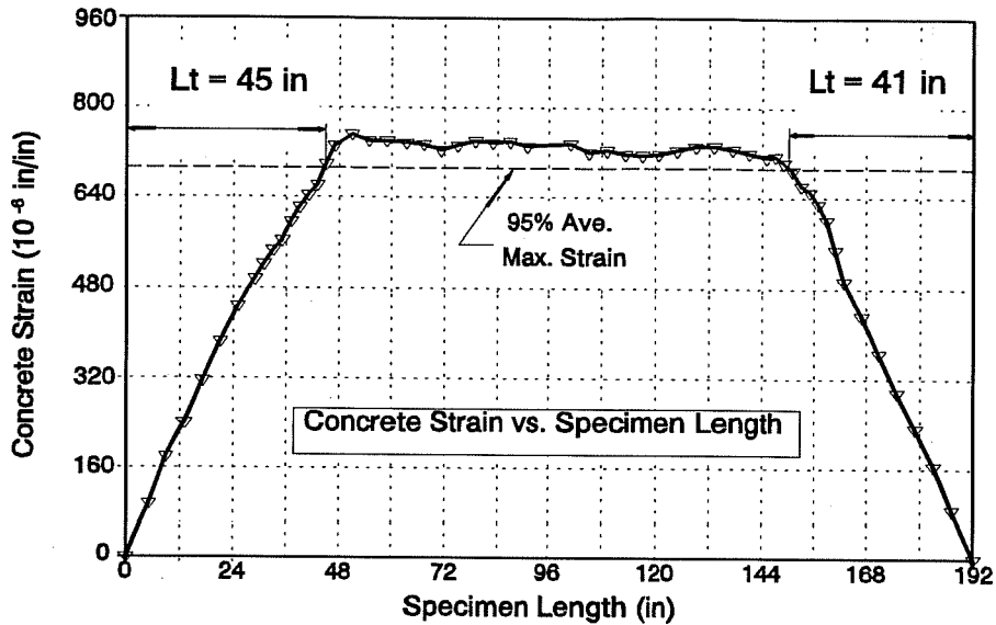
Figure 3.15 FC362-13, Transfer Length
