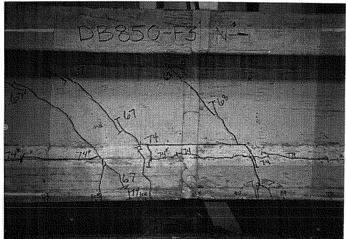
Figure 6.30 Cracking in the Debond/Transfer Zone of DB850-F3
