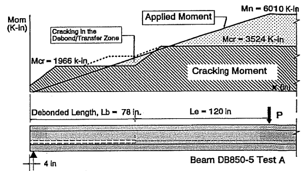
Figure 5.5 Applied Moment vs. Cracking Moment (Beams With Debonded Strand)
