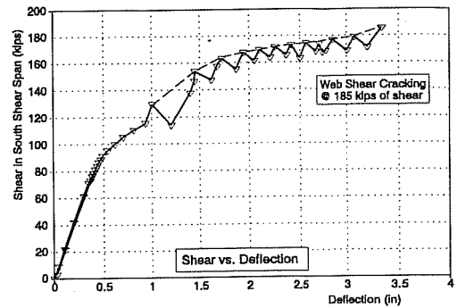
Figure 7.27 Static Test to Web Shear Cracking, Beam FZ2450-3
