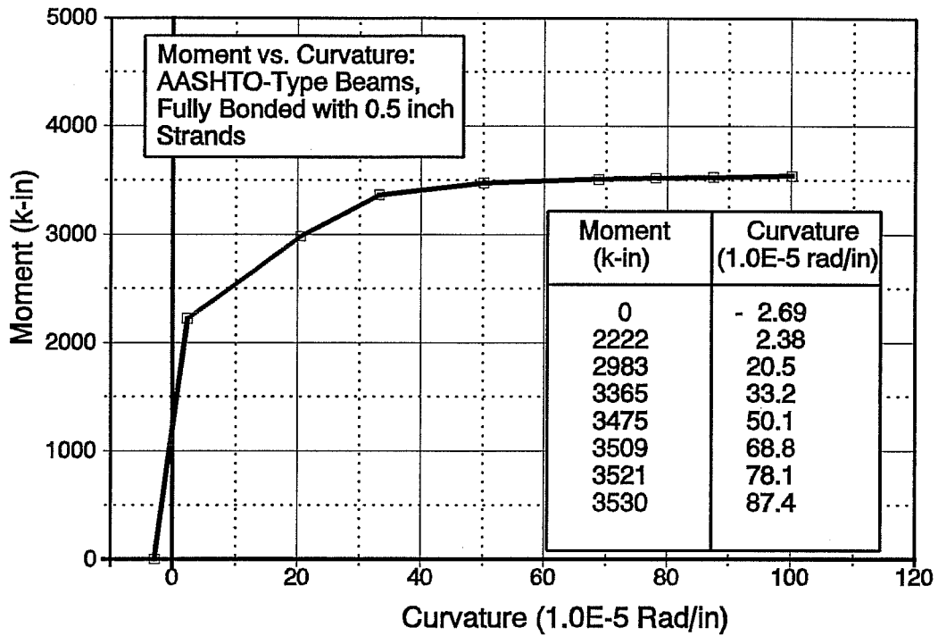
Figure D1. Moment Curvature, Beams FA550
