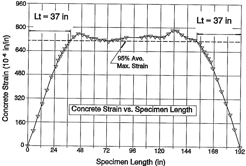
Figure A28. FCT550 - 2 , Transfer Length
