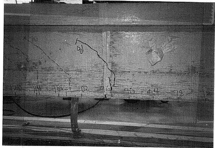
Figure 6.29 Test DB850-F2B at Load = 81 kips
