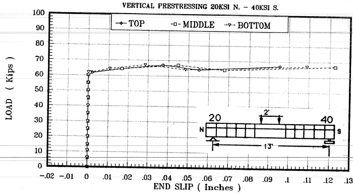
Figure 5.5e Load vs. end slip (north end).
