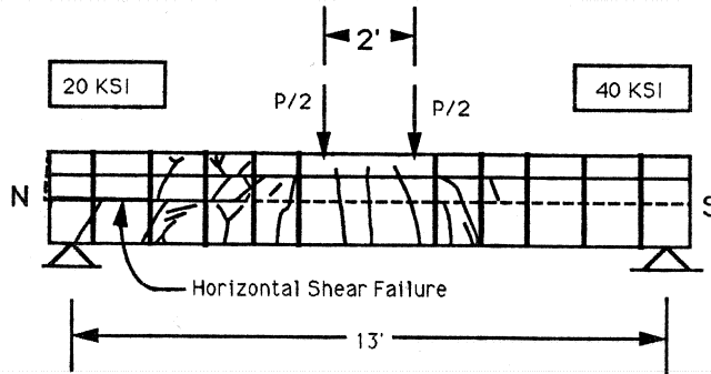
Figure 5.5c Loading and cracking patterns (Beam R4).
