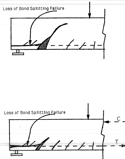
Figure 2.3c Bond failure.
