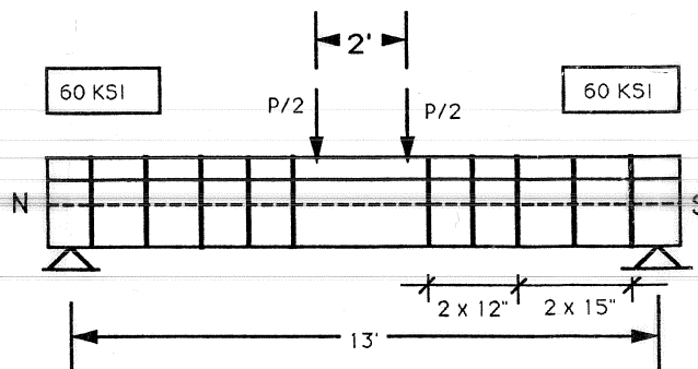
Figure 5.3a Loading pattern.
