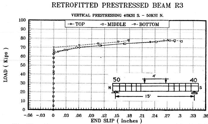
Figure 5.4b Load vs. end slip (north end).
