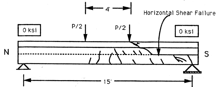
Figure 5.1c Crack pattern, Beam B1.
