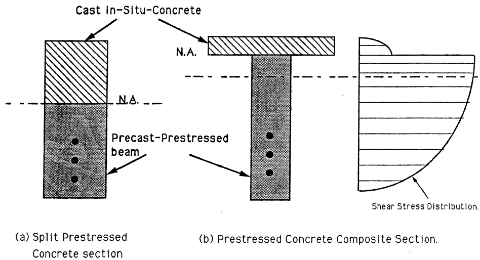
Figure 1.1 Prestressed concrete composite sections.
