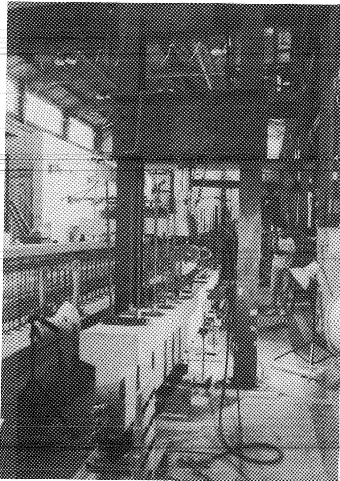
Figure 4.3(b) Test specimen under testing frame.
