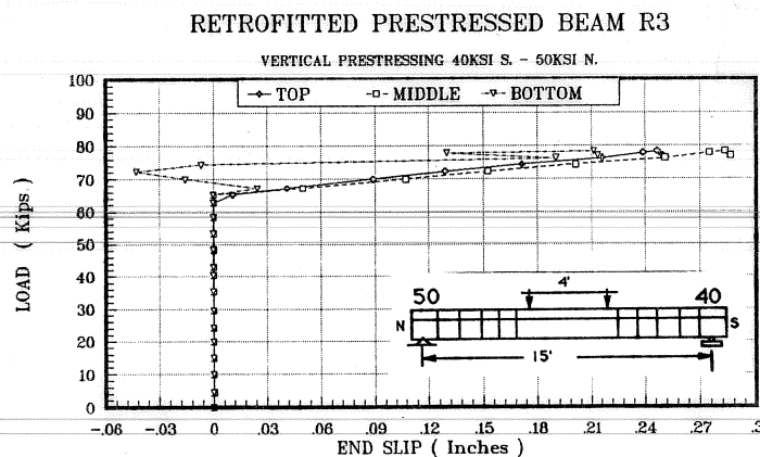
Figure 5.4a Load vs. end slip (south end).
