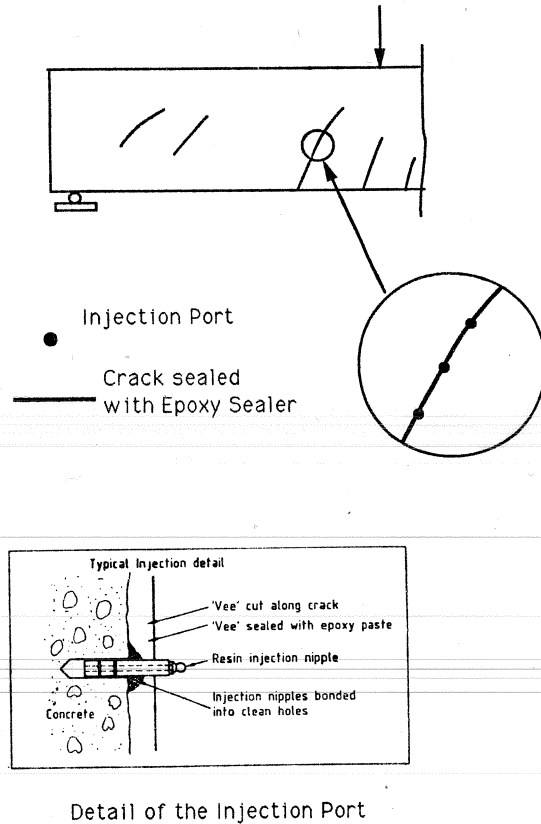
Figure 3.1 Epoxy resin injection technique.
