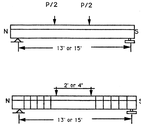
Figure 1.3 Test beam before and after retrofitting.
