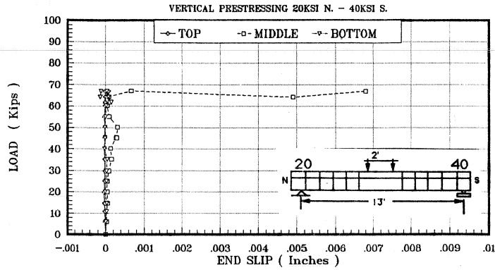
Figure 5.5d Load vs. end slip (south end).
