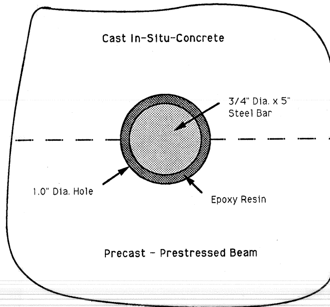
Figure 5.2b Detail of horizontal shear insert.
