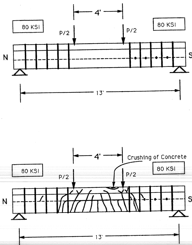
Figure 5.2a Loading and cracking pattern, Beam R1.
