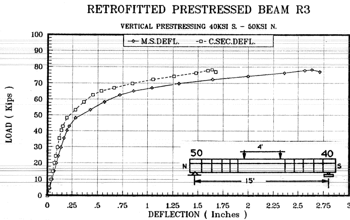
Figure 5.4c Load - Deflection curve.
