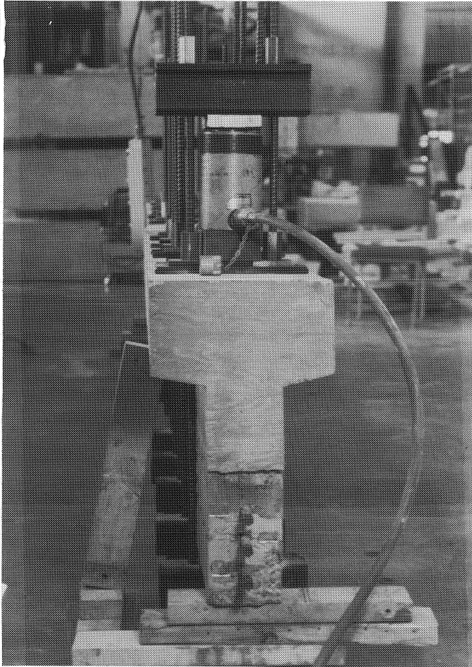
Figure 4.2(d) Tensioning system.
