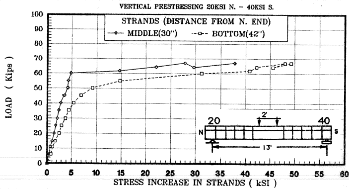
Figure 5.5f Load vs. stresses in strands (north 20 ksi end).
