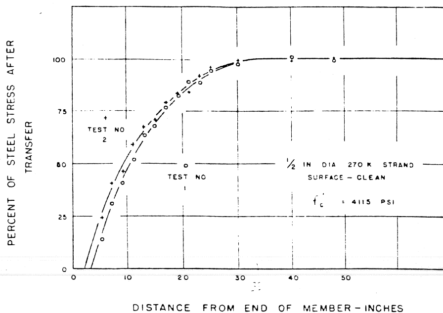
Figure 2.6 Steel stress profile of 0.5-inch diameter Grade 270K strand (7) .
