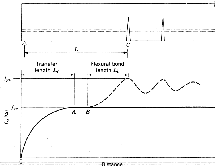
Figure 2.2 Flexural bond overlapping with transfer length (15) .
