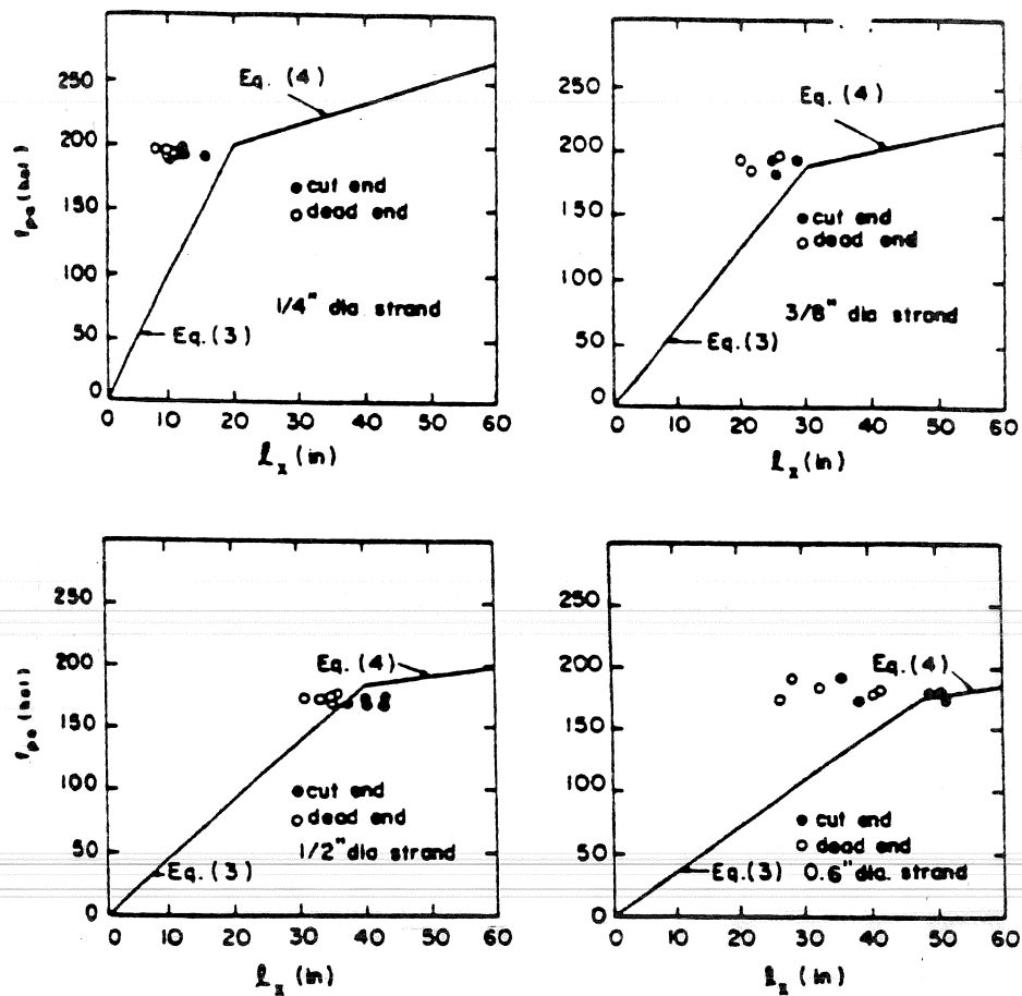
Figure 2.9 Comparison of the Martin-Scott equations with test results by Kaar, LaFraugh and Mass (10) .
