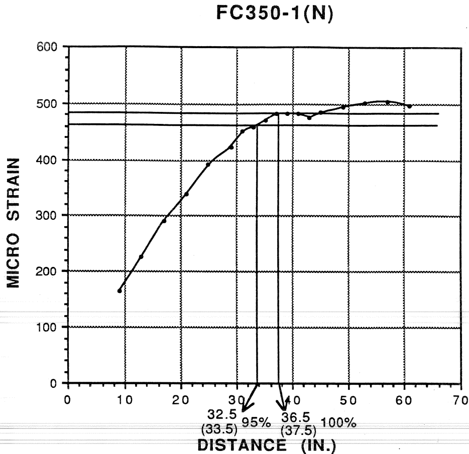
Figure 4.4 Typical concrete strain profile and techniques of obtaining transfer length.
