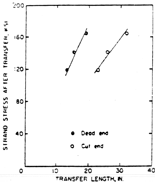
Figure 2.5 Effect of strand tension on transfer length specimens prestressed with 3/8-inch diameter strand (6) .
