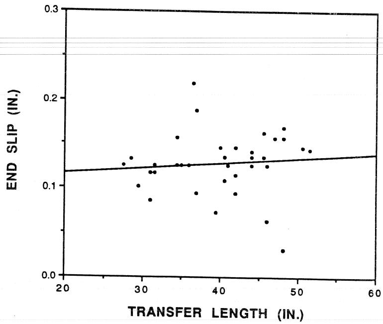
Figure 5.4 Measured transfer length vs. end slip, 0.6-inch diameter strand.
