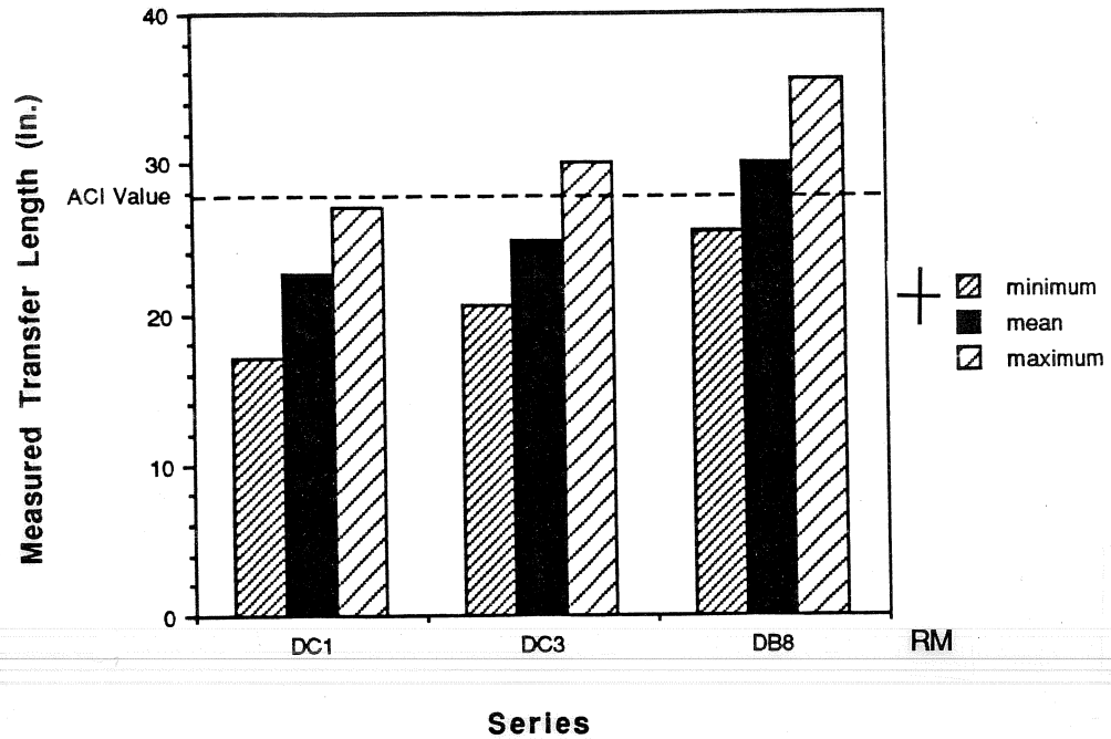
Figure 4.7 Measured transfer length, 0.5-inch debonded strand (minimum, mean and maximum values compared with ACI required value).
