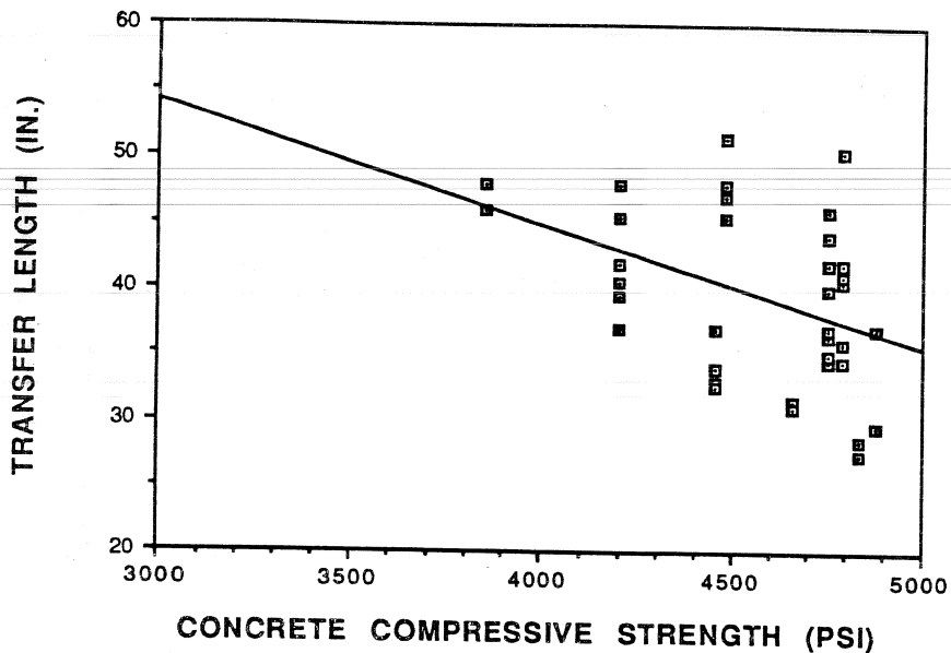
Figure 5.2 Measured transfer length vs. concrete compressive strength, 0.6-inch diameter strand.
