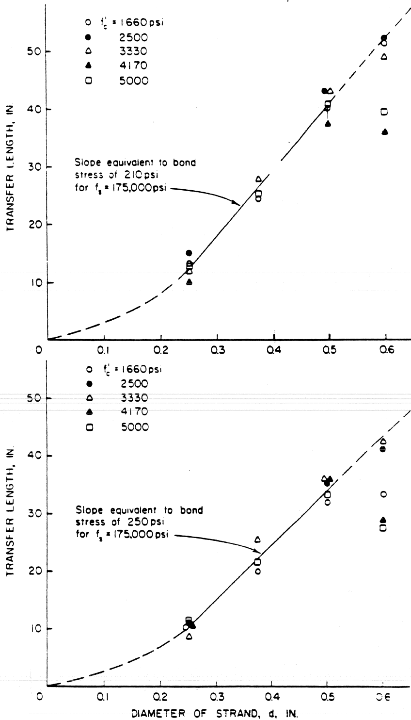
Figure 2.3 Relation of prestress transfer length to strand diameter at a) cut end and b) dead end (6) .
