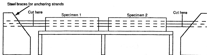
Figure 3.5 Test setup (figure not drawn to scale).
