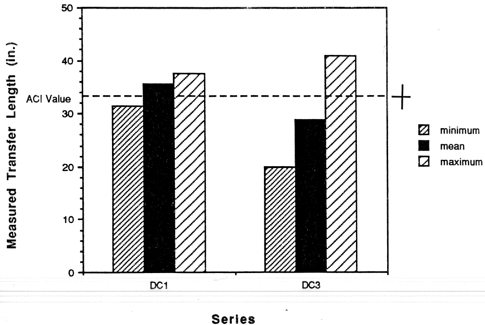
Figure 4.8 Measured transfer length, 0.6-inch debonded strand (minimum, mean and maximum values compared with ACI required value).
