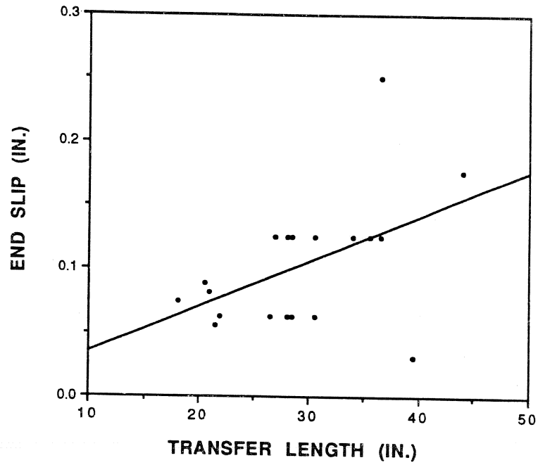
Figure 5.3 Measured transfer length vs. end slip, 0.5-inch diameter strand.
