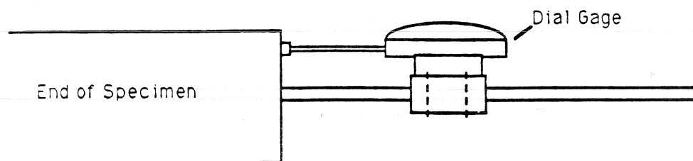
Figure 3.6 End slip device.
