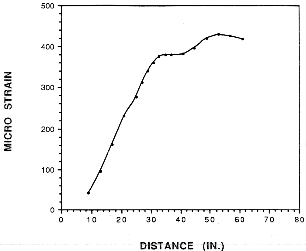
Figure 4.3 Typical concrete strain profile obtained by smoothed data.
