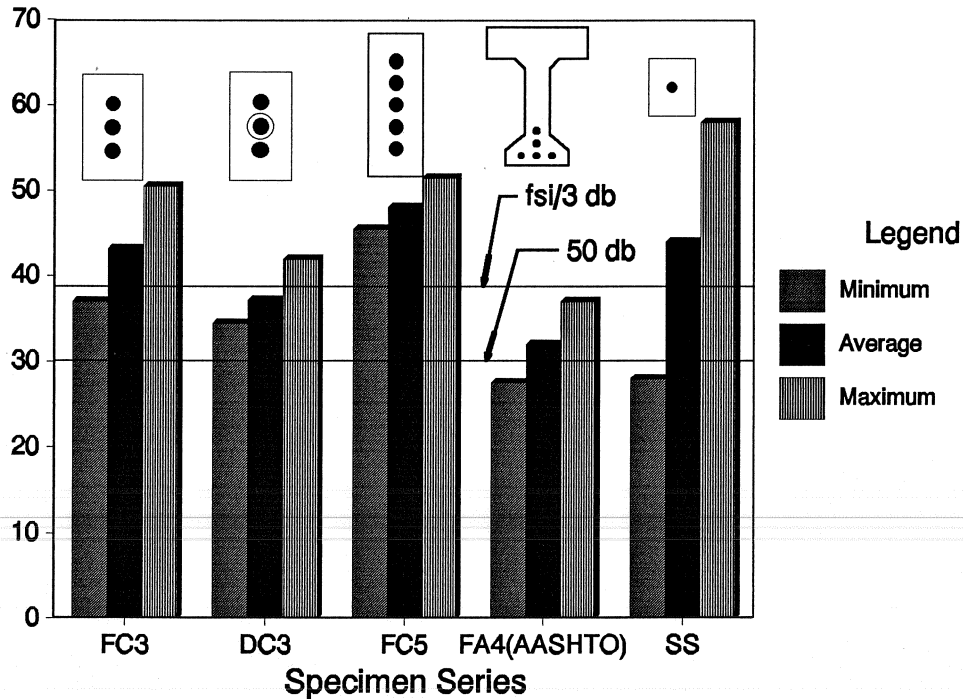
Figure 4.6 Measured transfer length, 0.6-inch fully bonded strand (minimum mean and maximum values compared with ACI required value).
