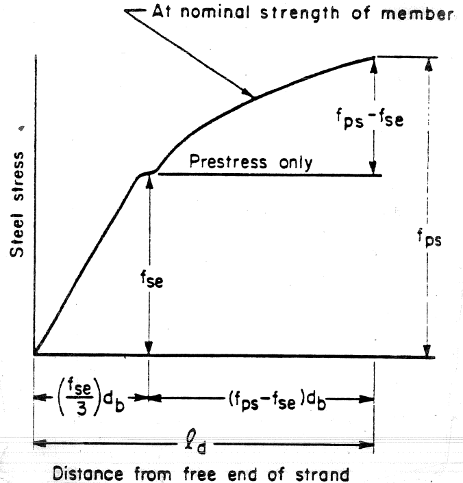
Figure 2.1 Variation of steel stress with distance from free end of strand. Used as the basis for ACI/AASHTO formula (21,22) .
