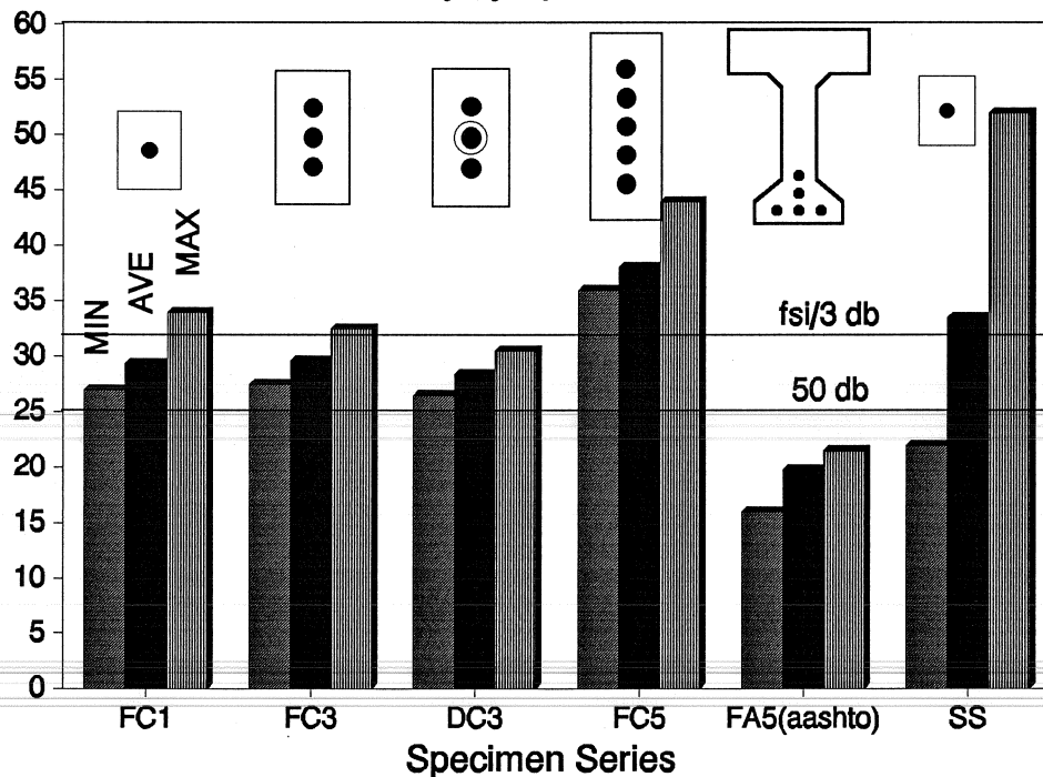
Figure 4.5 Measured transfer length, 0.5-inch fully bonded strand (minimum, mean and maximum values compared with ACI required value).
