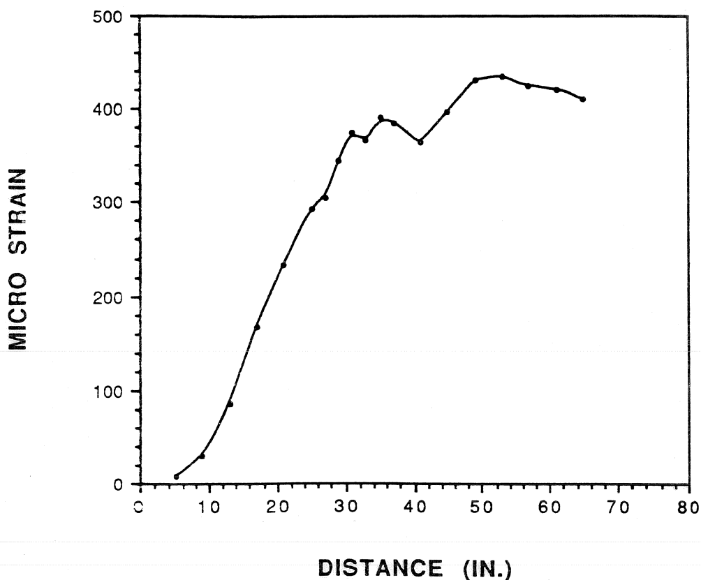
Figure 4.2 Typical concrete strain profile obtained by raw data.
