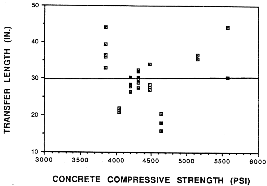
Figure 5.1 Measured transfer length vs. concrete compressive strength, 0.5-inch diameter strand.
