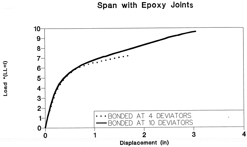
Figure 4.17 Effect of bonding on load-deflection response during flexureal strength tests on epoxy joints span.
