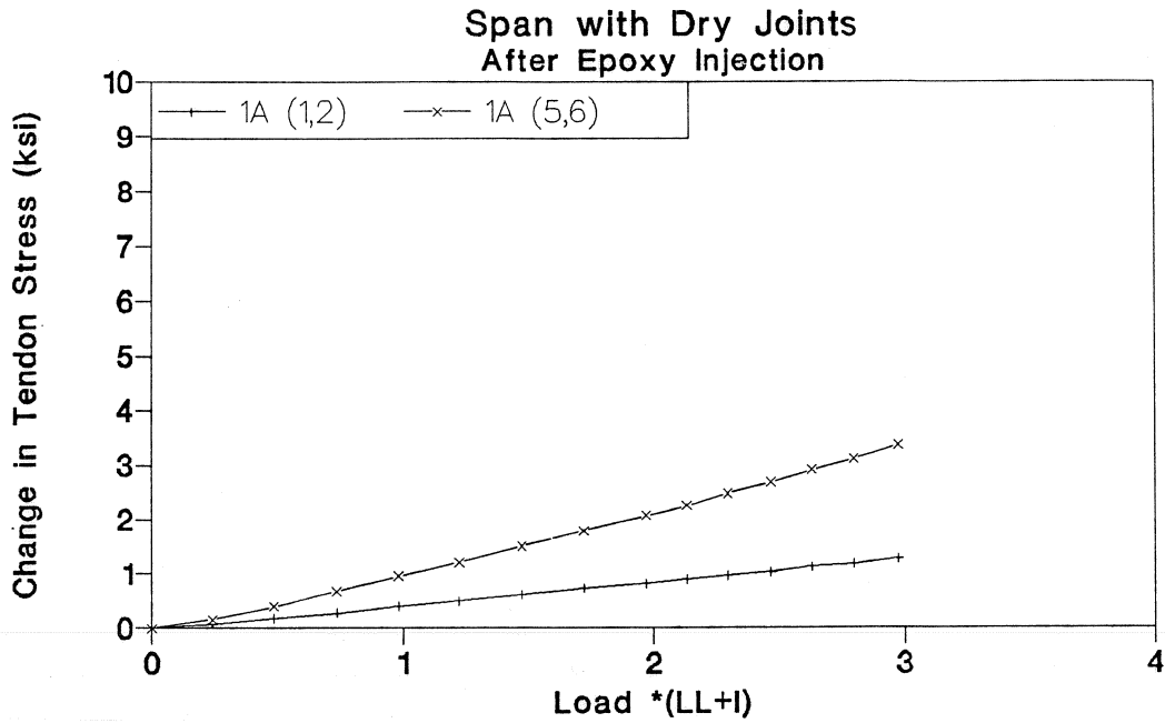
Figure 3.88 Tendon 1A stress-load of injection cycle in dry joints span.
