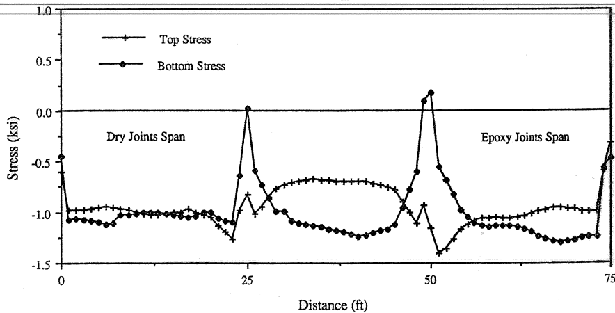
Figure 2.35 Flexural stresses without center span dead load blocks.
