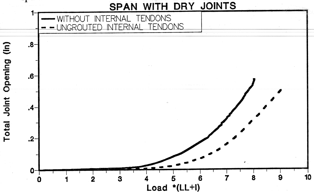
Figure 4.40 UngROUTED internal tendon effect on total joint opening-load for dry joints span.
