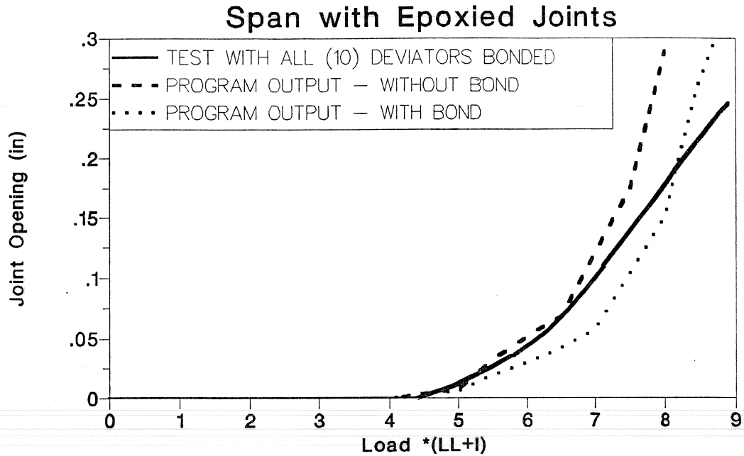
Figure 6.10 Joint opening response (epoxy joints span without internal tendons).
