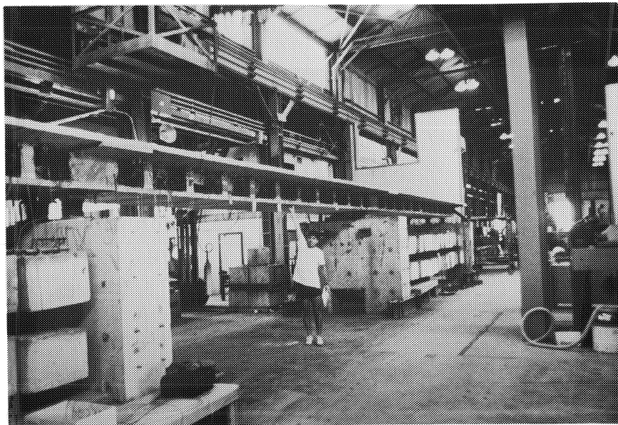
Figure 2.34 Middle span dead load blocks removed.
