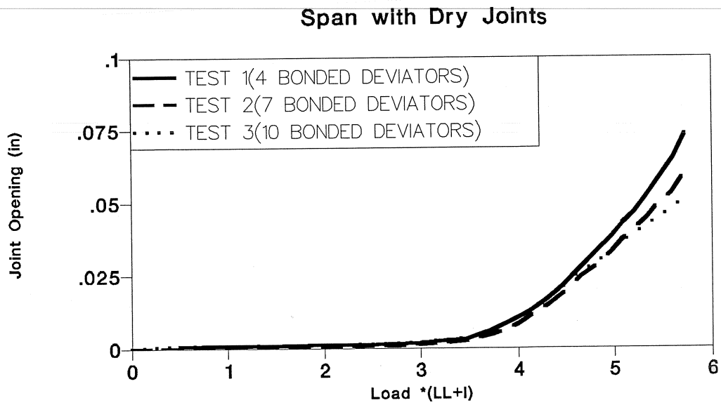
Figure 4.14 Effect of bonding on joint opening in dry joints span.
