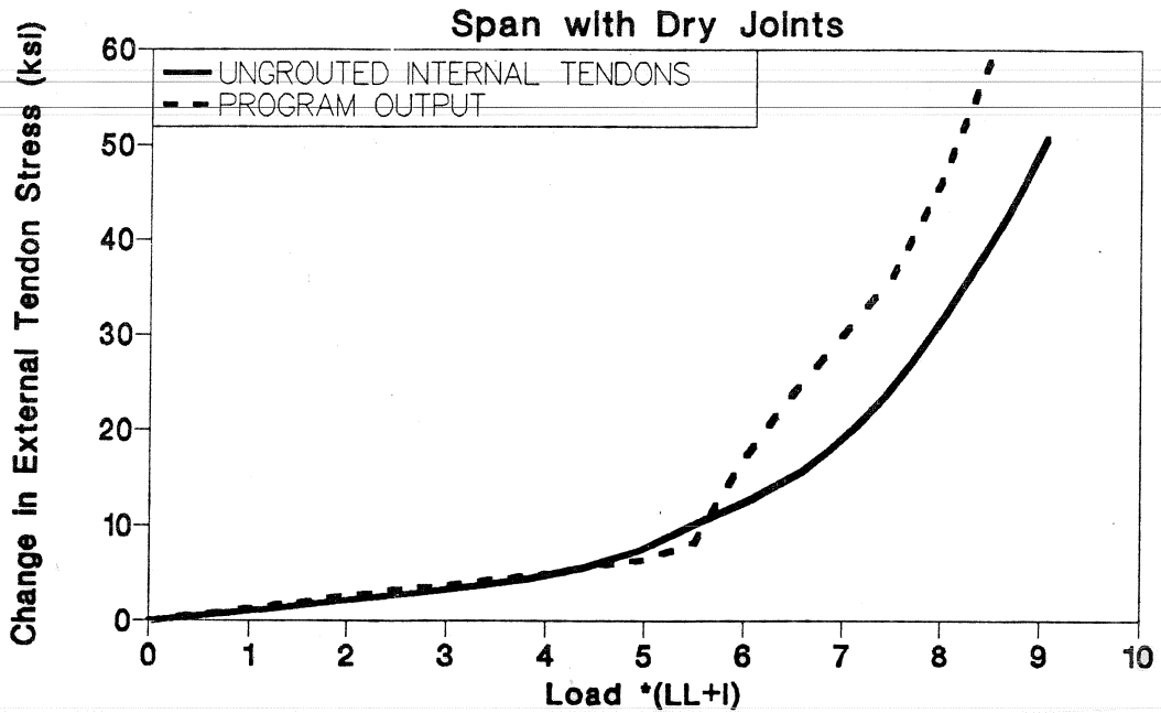
Figure 6.20 Change in external tendon stress (dry joints span - ungrouted internal tendons).
