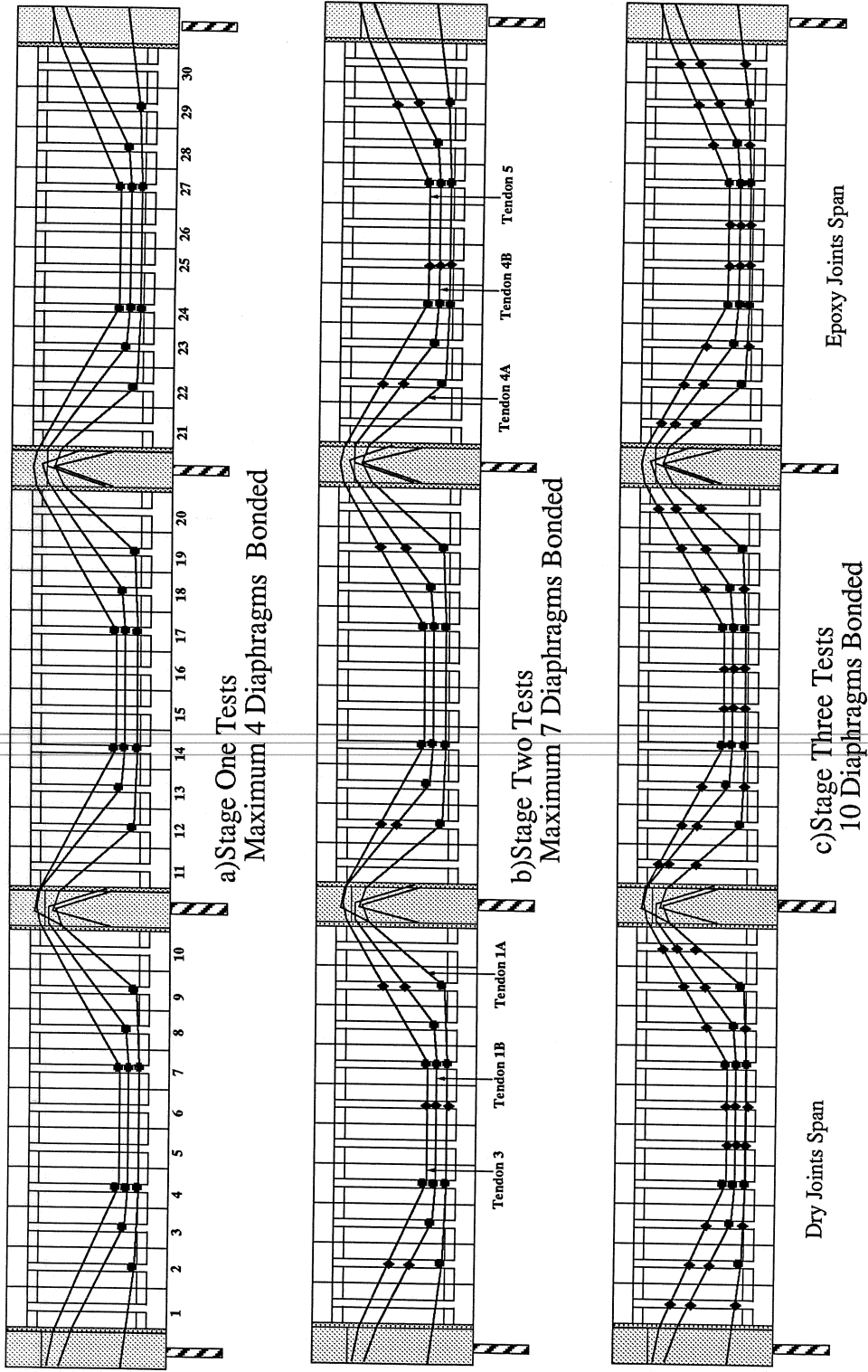
■ : Interior Diaphragm Originally Bonded ◆ : Interior Diaphragm Bonded Figure 3.25 Bonding stages of external tendons.
