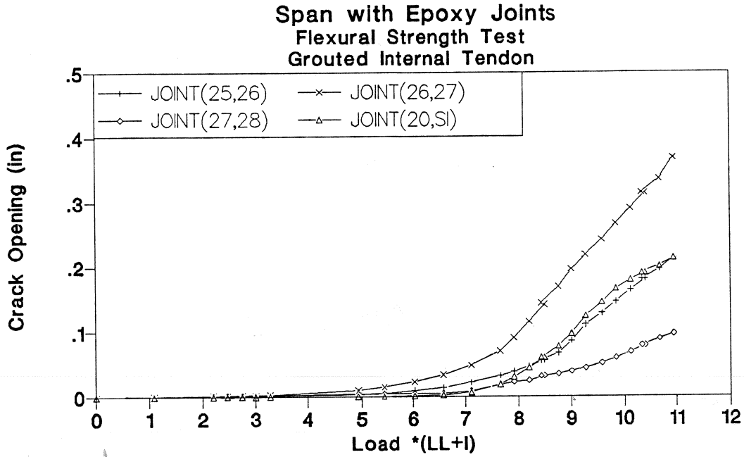
Figure 3.77 Crack opening-load of grouted internal tendons test in epoxy joints span.
