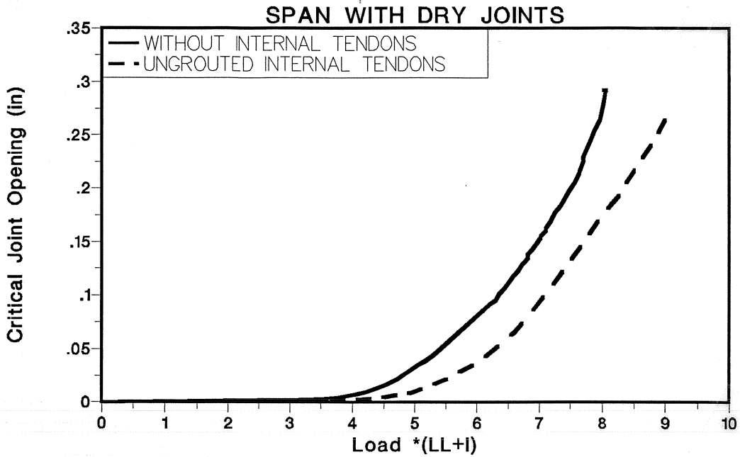
Figure 4.37 UngROUTED internal tendon effect on critical joint opening-load for dry joints span.
