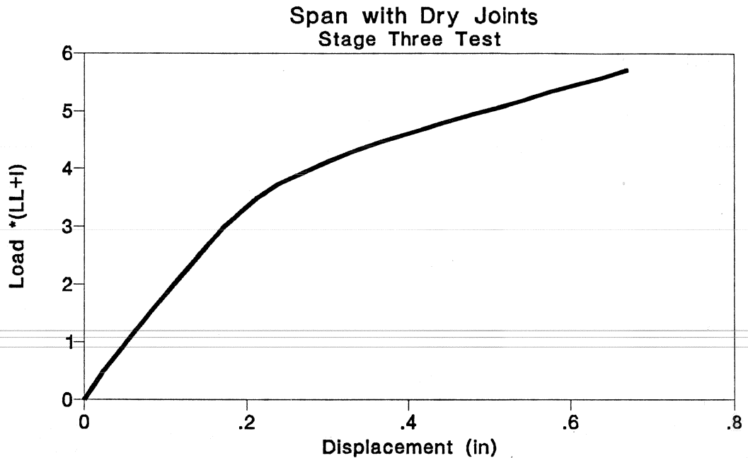
Figure 3.106 Load-deflection of Stage Three test in dry joints span.
