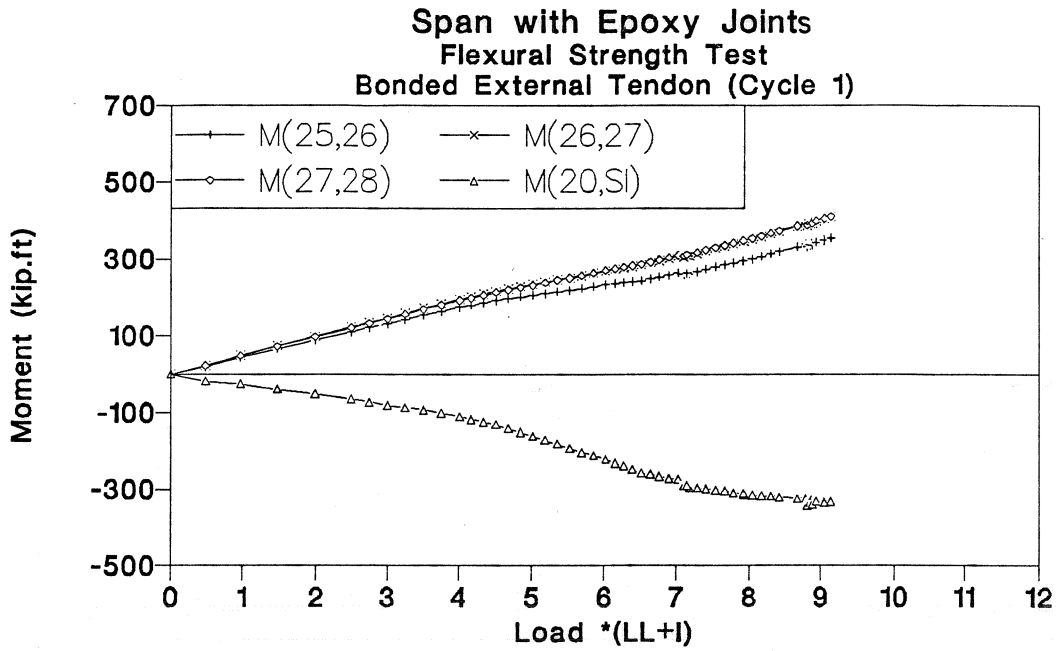
Figure 3.49 Moment-load of flexural strength test (cycle 1) in epoxy joints span.
