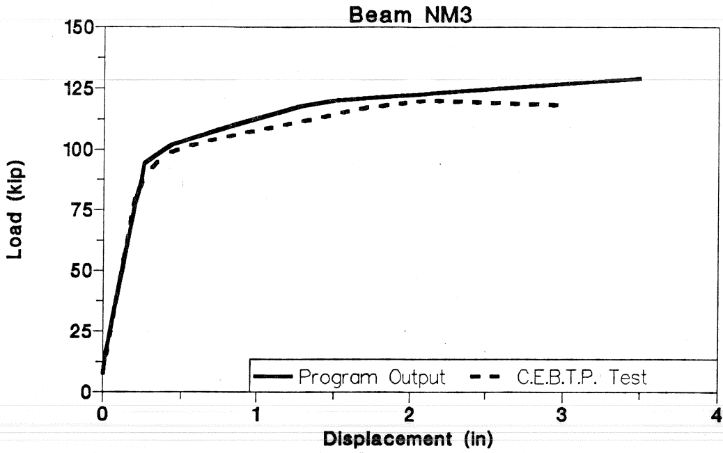
Figure 6.31 Load-deflection response (Beam NM3).
