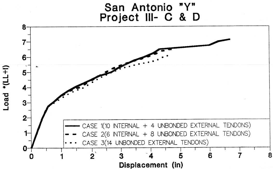
Figure 7.16 Load-displacement (effect of internal tendons - unbonded external tendons).
