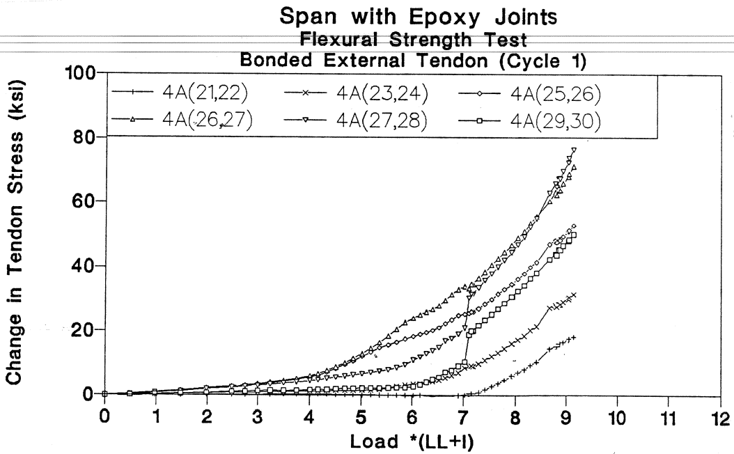
Figure 3.50 Tendon 4A stress-load of flexural strength test (cycle 1) in epoxy joints span.
