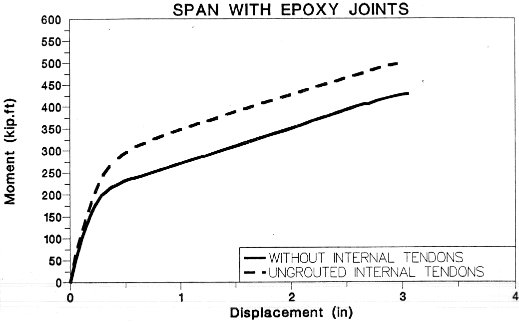
Figure 4.42 UngROUTED tendon effect on moment-deflection response of epoxy joints span.
