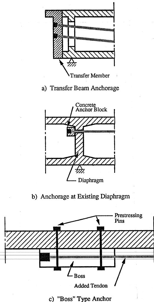
Figure 1.2 Anchorage schemes for retrofit external tendons [From Ref. (2)].
