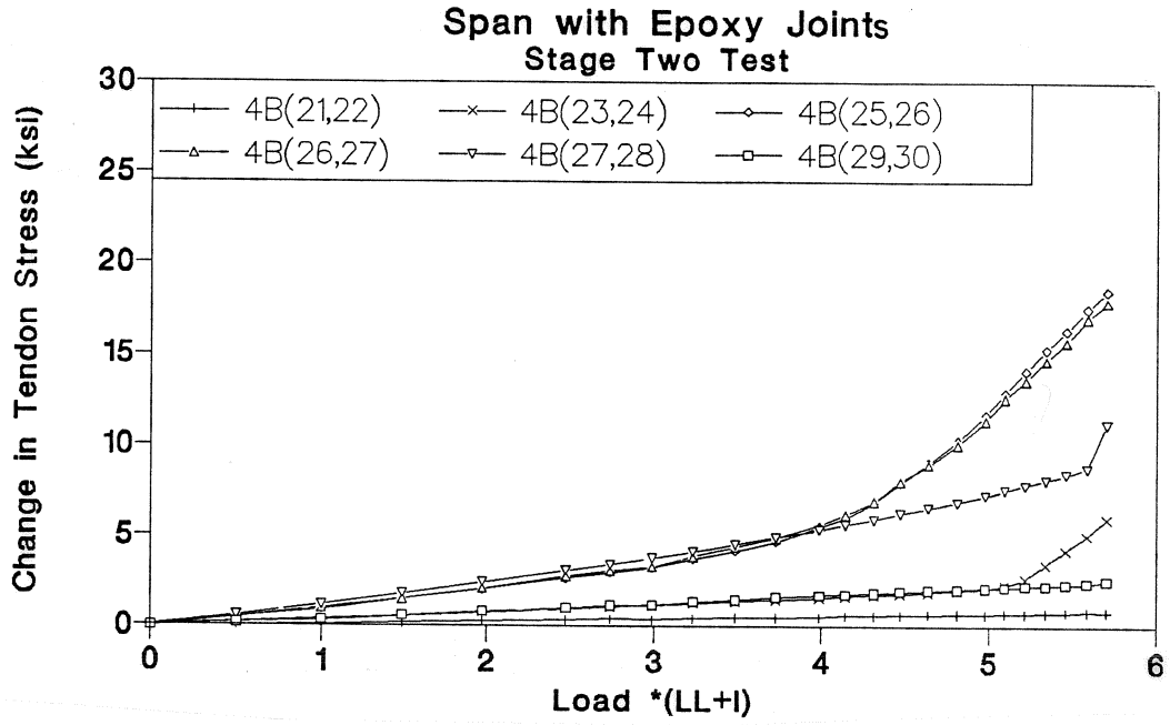
Figure 3.37 Tendon 4B stress-load of Stage Two test in epoxy joints span.
