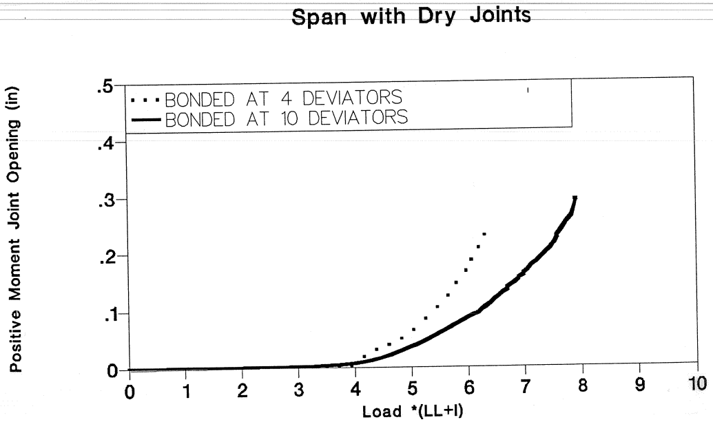
Figure 4.27 Effect of bonding on positive moment joint opening-load response for flexural strength tests of dry joints span.
