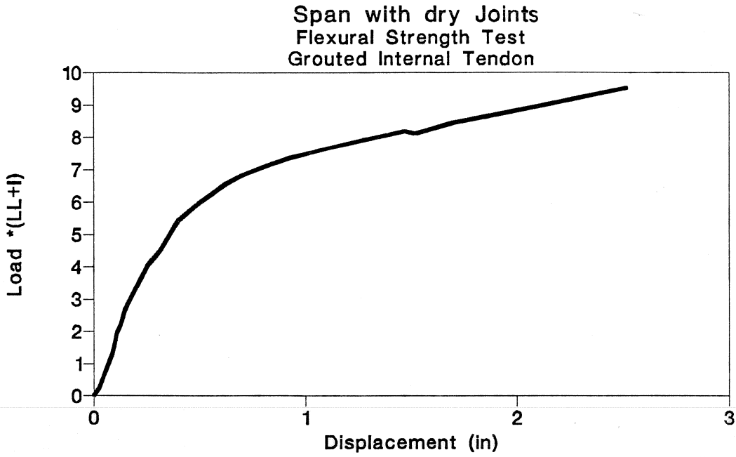
Figure 3.130 Load-deflection of grouted internal tendon test in dry joints span.
