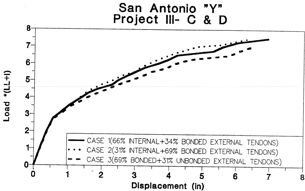
b) Load-displacement (bonded external tendons)
