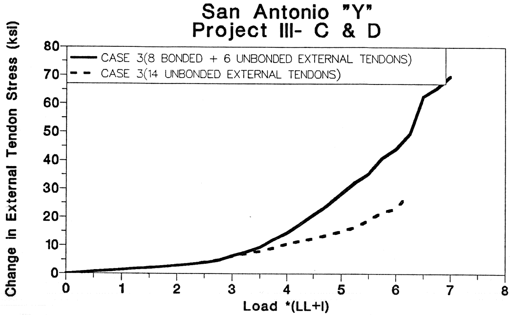
Figure 7.13 External tendon stress (Case Three - Effect of bonding).
