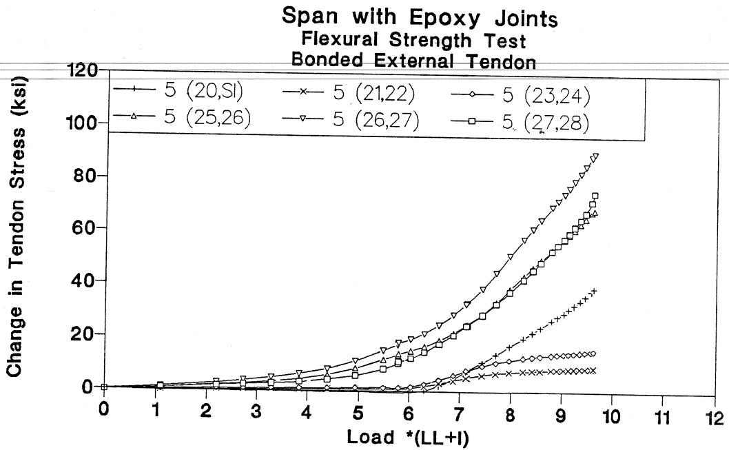
Figure 3.59 Tendon 5 stress-load of flexural strength test (cycle 2) in epoxy joints span.
