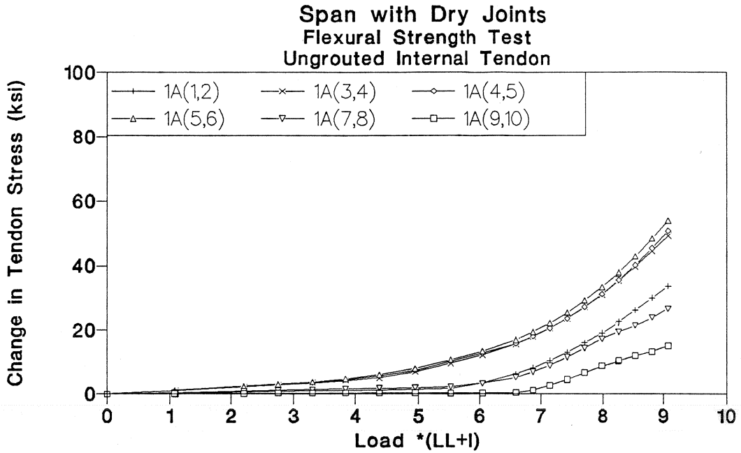
Figure 3.124 Tendon 1A stress-load of ungrouted internal tendon test in dry joints span.
