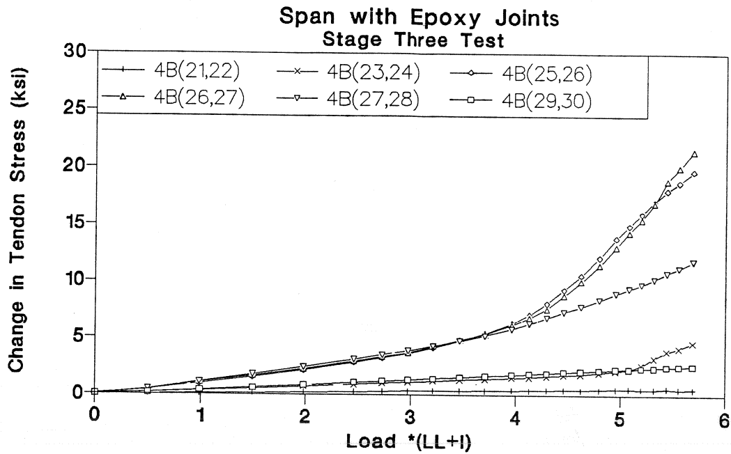
Figure 3.44 Tendon 4B stress-load of Stage Three test in epoxy joints span.
