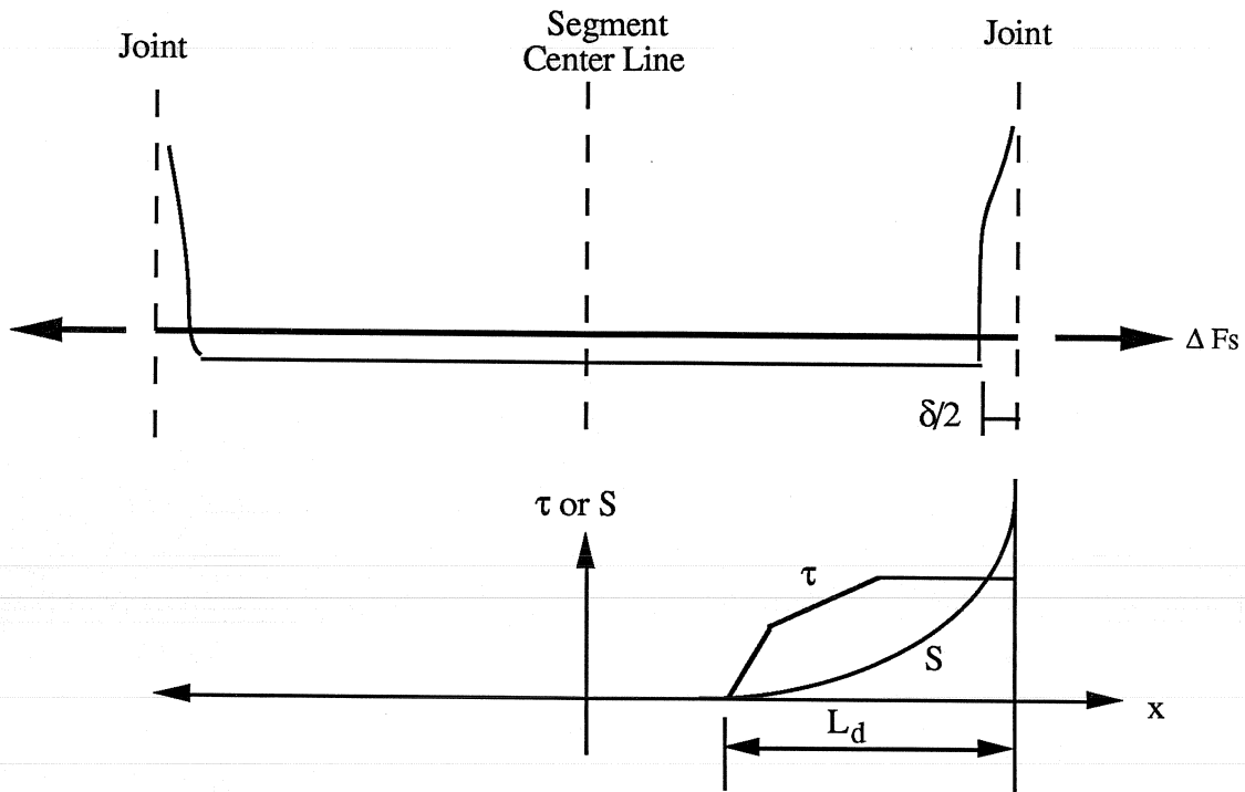
Bond &amp; Slip along the segment
