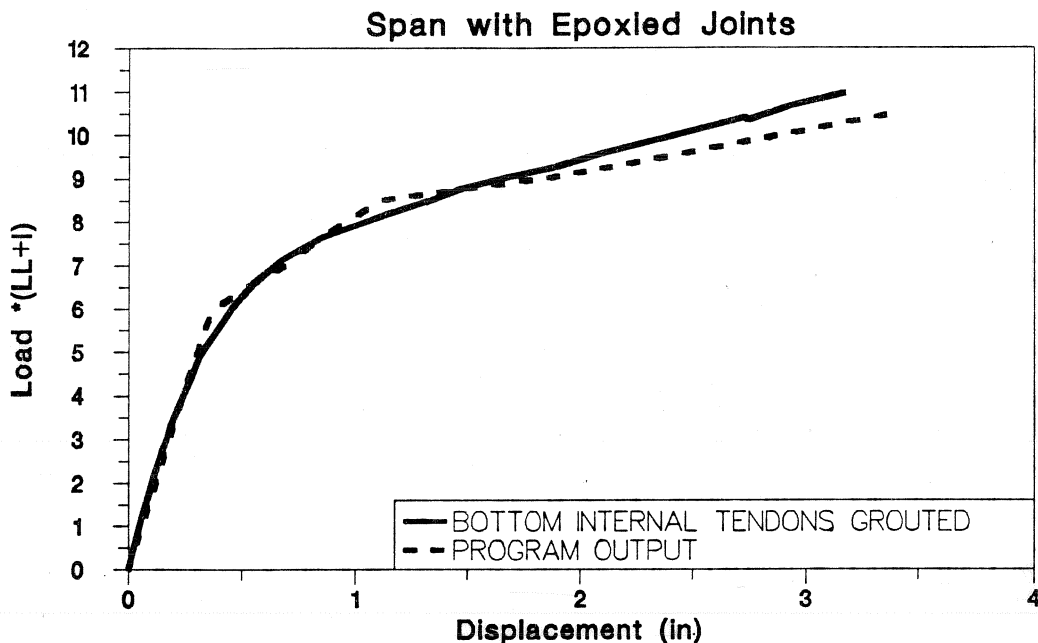
Figure 6.21 Load-deflection response (epoxy joints span - grouted internal tendons).
