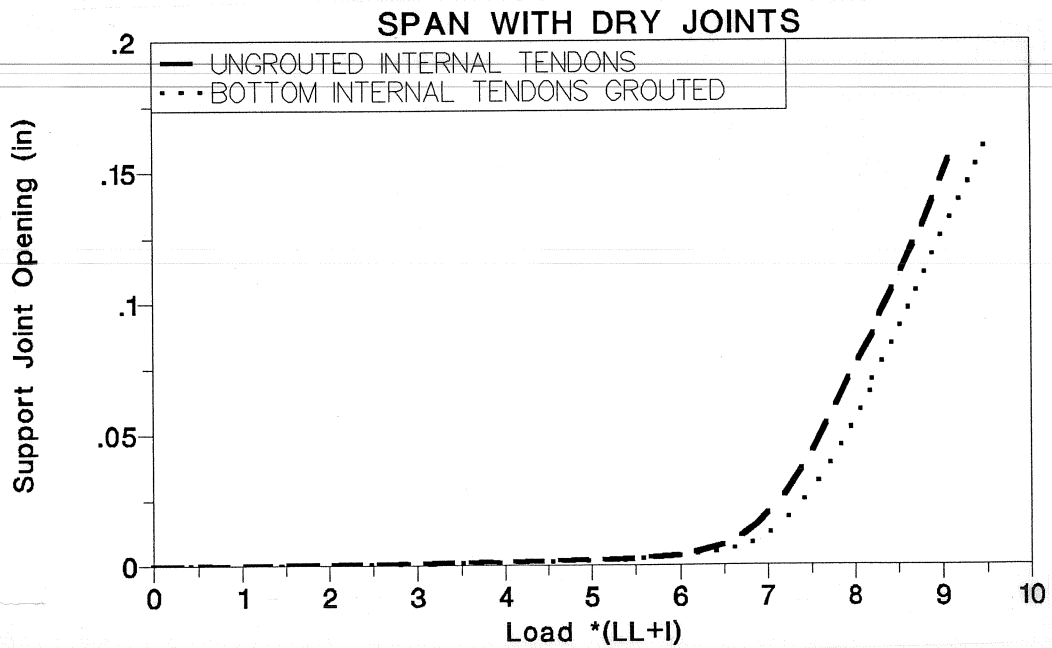
Figure 4.54 Grouted tendon effect on support joint opening-load for dry joints span.
