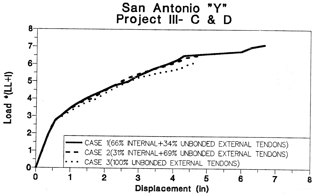
a) Load-displacement (unbonded external tendons)
