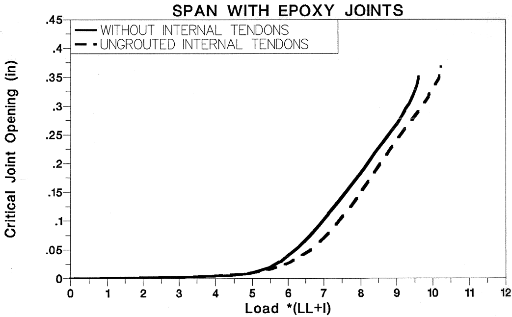
Figure 4.45 UngROUTed tendon effect on critical joint opening-load for epoxy joints span.
