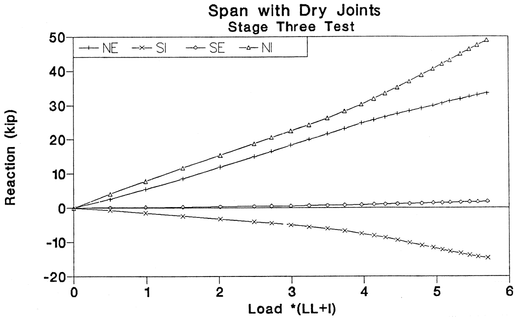
Figure 3.107 Reaction-load of Stage Three test in dry joints span.
