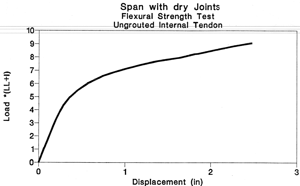
Figure 3.121 Load-deflection of ungrouted internal tendon test in dry joints span.
