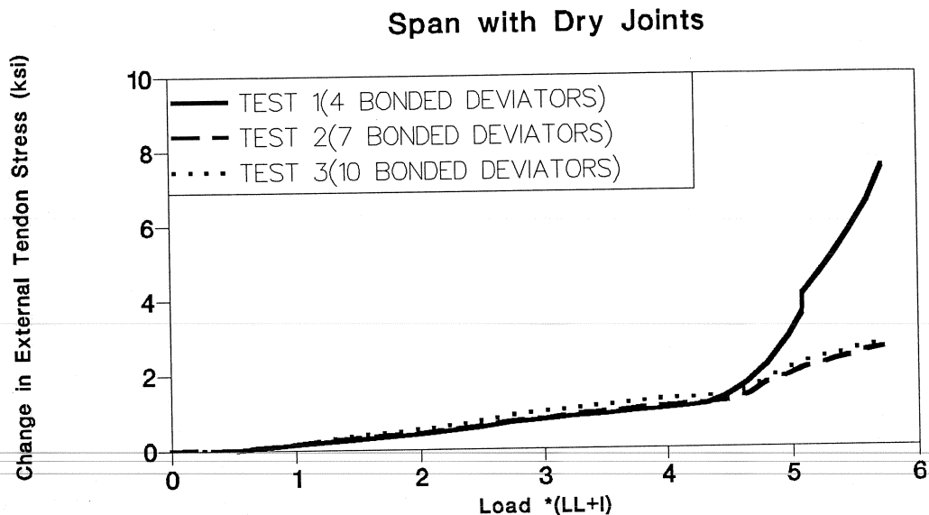
Figure 4.8 Effect of bonding on tendon slip in dry joints span.
