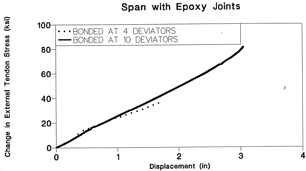
Figure 4.21 Effect of bonding on tendon stress-displacement for flexural strength tests of epoxy joints span.
