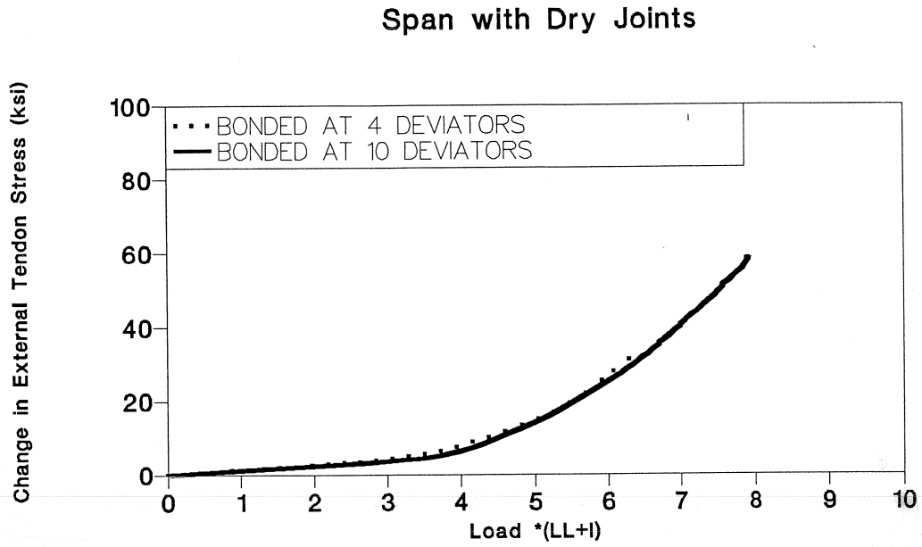
Figure 4.26 Effect of bonding on tendon stress-load during flexural strength tests of dry joints span.
