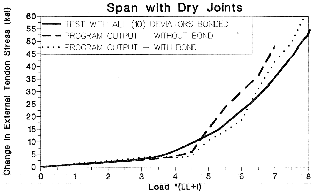
Figure 6.14 Change in external tendon stress (dry joints span without internal tendons).
