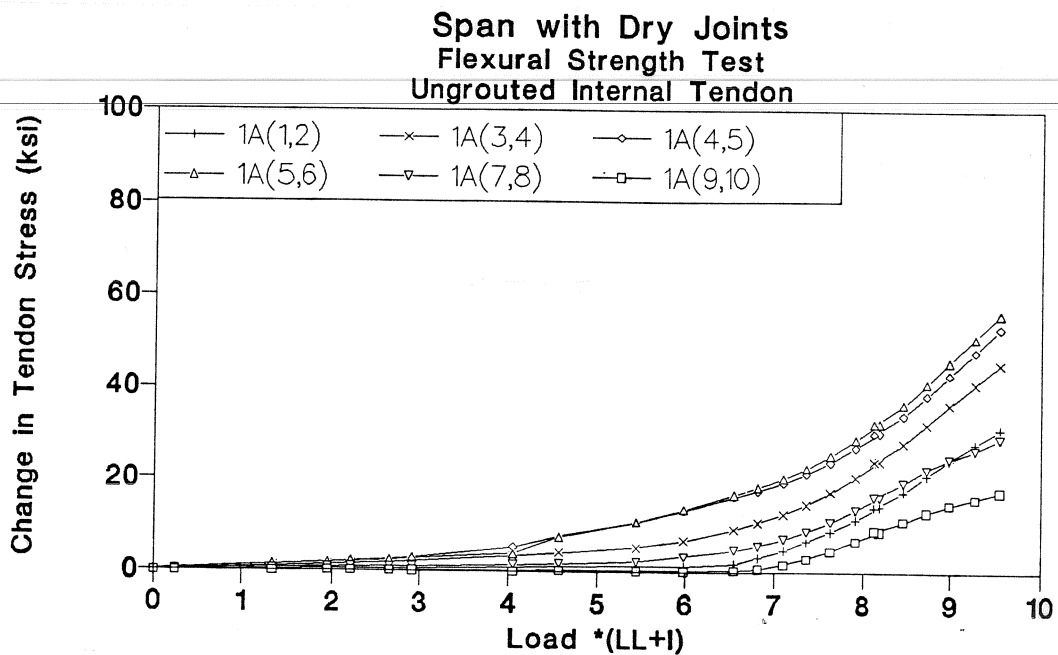
Figure 1.33 Tendon 1A stress-load of grouted internal tendon test in dry joints span.
