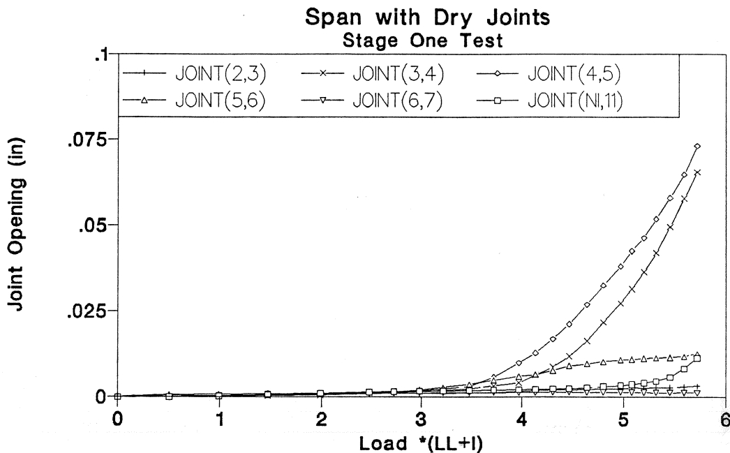
Figure 3.98 Joint opening-load of Stage One test in dry joints span.
