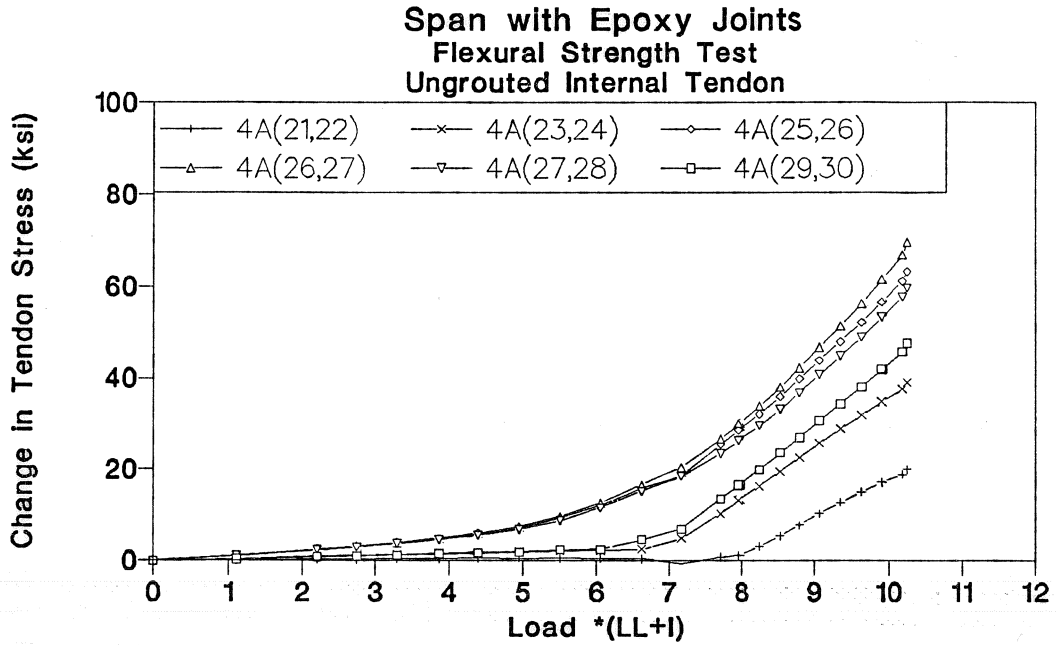
Figure 3.138 Change in Tendon 4A stress in epoxy joints span.
