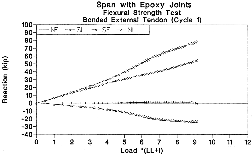
Figure 3.48 Reaction-load of flexural strength test (cycle 1) in epoxy joints span.
