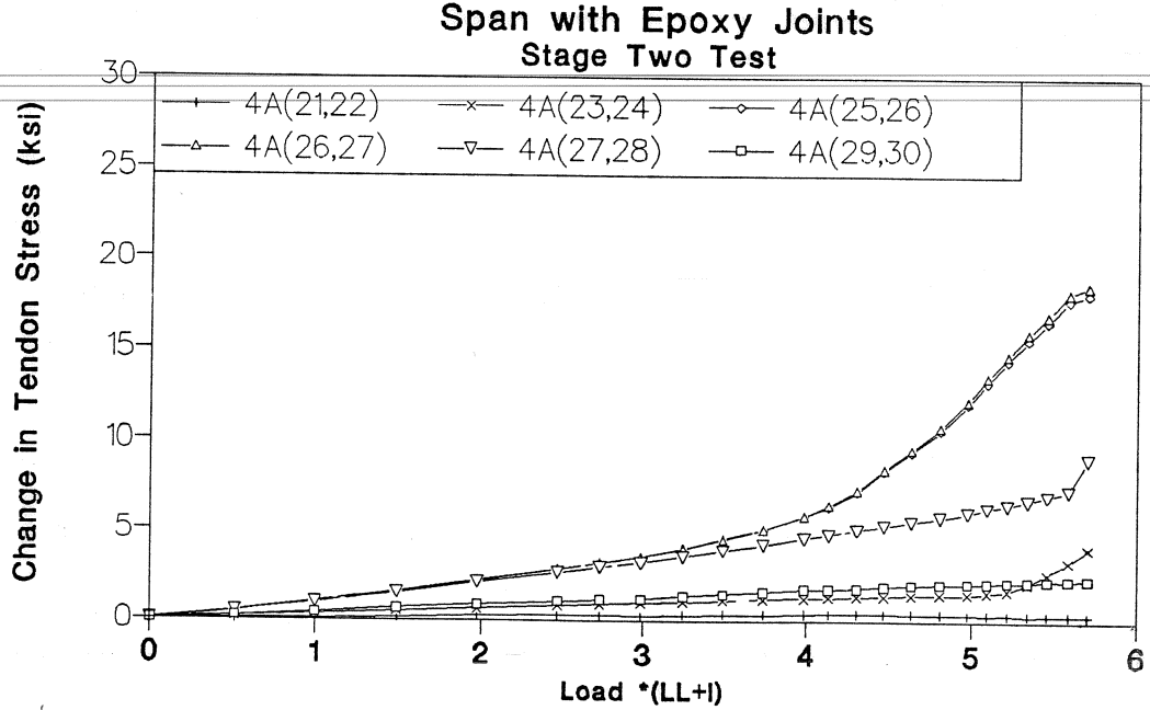
Figure 3.36 Tendon 4A stress-load of Stage Two test in epoxy joints span.
