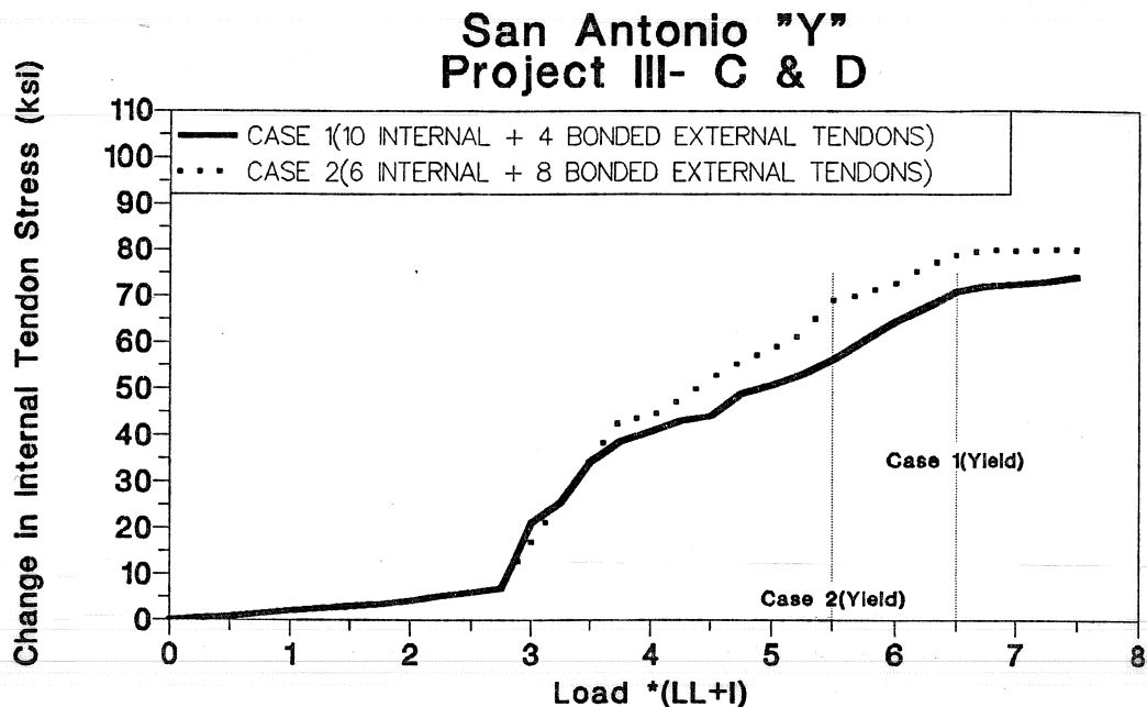
Figure 7.21 Internal tendon stress (effect of internal tendons - bonded external tendons).
