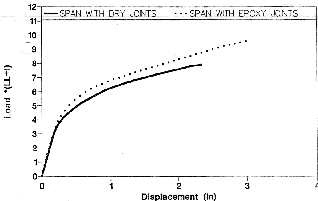
Figure 4.65 Effective prestress effect on load-deflection response.
