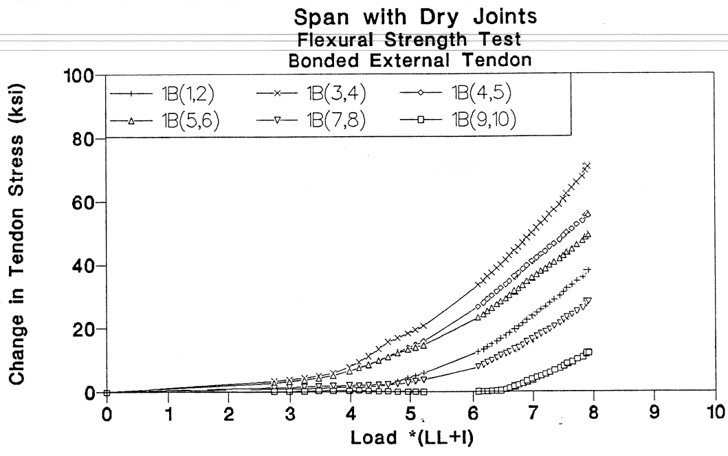
Figure 3.117 Tendon 1B stress-load of flexural strength test in dry joints span.
