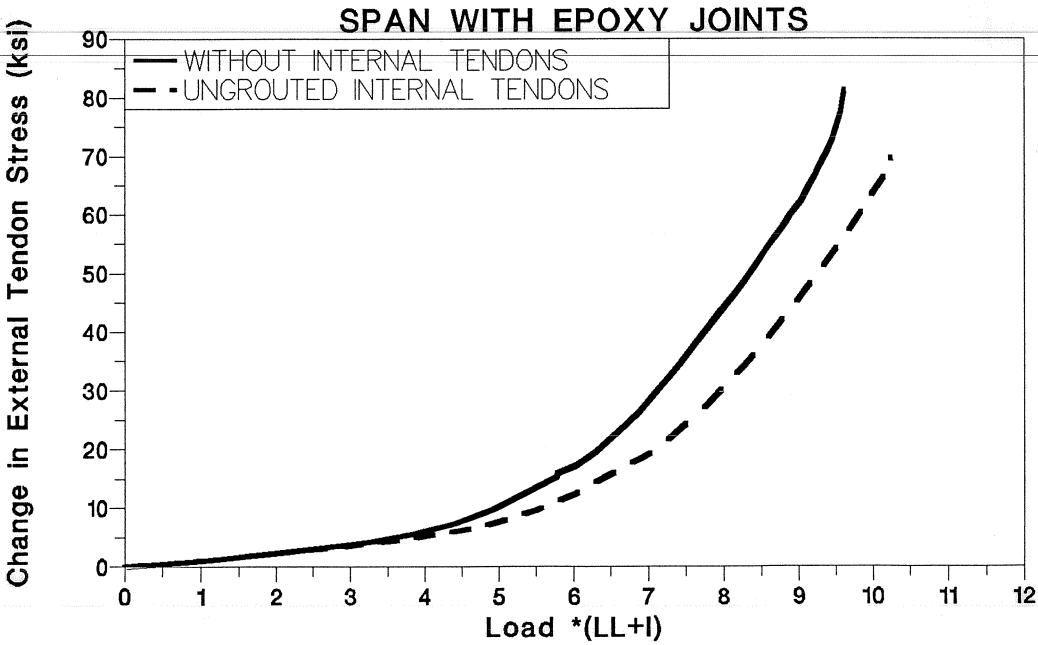
Figure 4.43 UngROUTED tendon effect on tendon stress-load for epoxy joints span.
