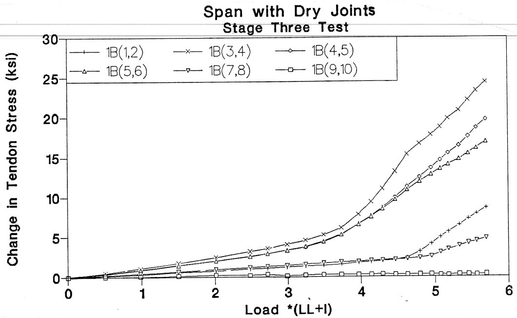
Figure 3.110 Tendon 1B stress-load of Stage Three in dry joints span.
