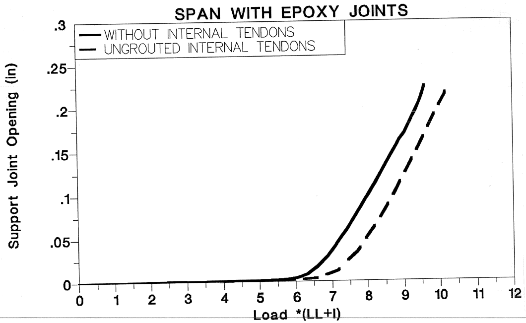
Figure 4.47 UngROUTed tendon effect on support joint opening-load for epoxy joints span.
