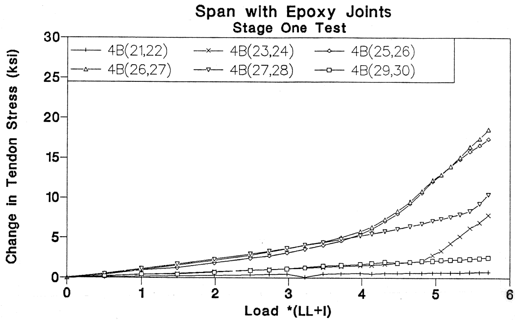
Figure 3.30 Tendon 4B stress-load of Stage One test in epoxy joints span.
