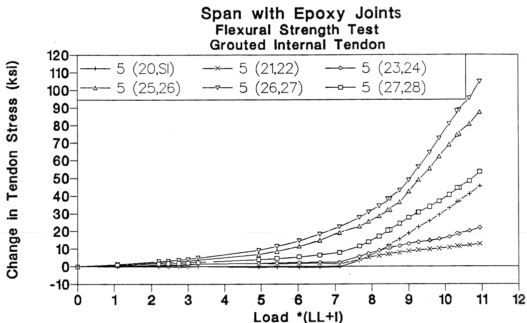
Figure 3.76 Tendon 5 stress-load grouted internal tendons test in epoxy joints span.
