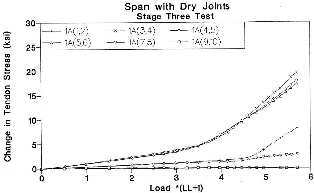
Figure 3.109 Tendon 1A stress load of Stage Three test in dry joints span.
