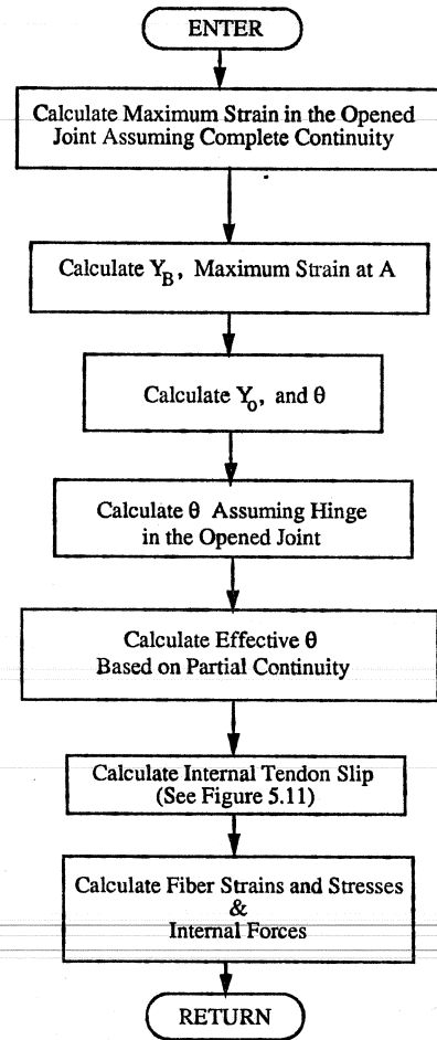
Figure 5.7 Internal forces for cracked or opened joint element.
