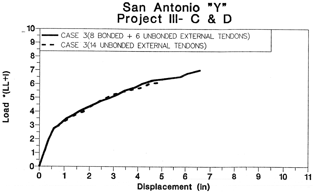
Figure 7.11 Load-displacement (Case Three - Effect of bonding).
