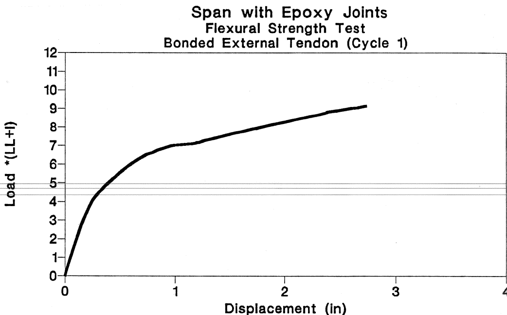
Figure 3.47 Load-deflection of flexural strength test (cycle 1) in epoxy joints span.
