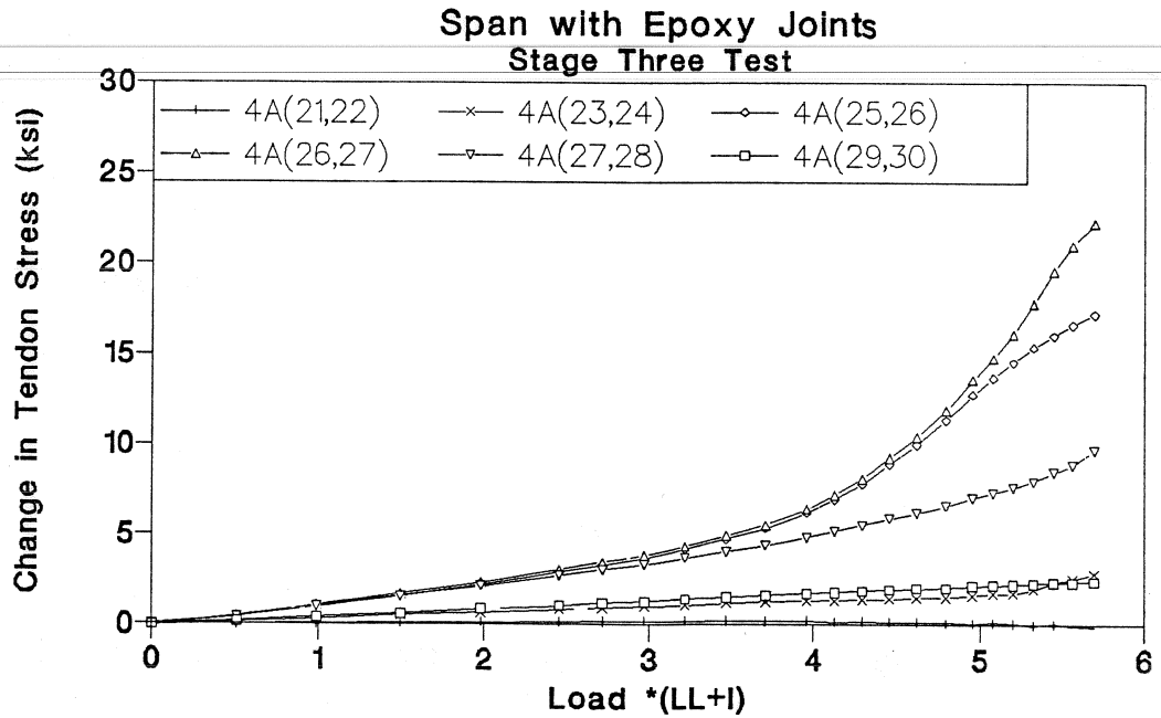
Figure 3.43 Tendon 4A stress-load of Stage Three test in epoxy joints span.
