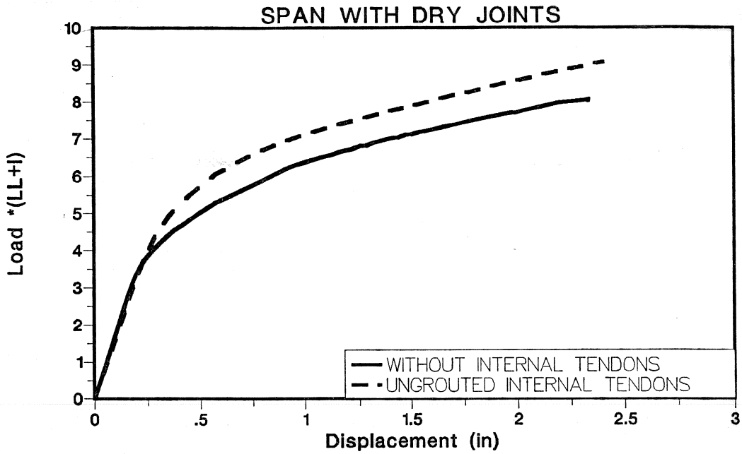
Figure 4.33 UngROUTed internal tendon effect on load-deflection response of dry joints span.
