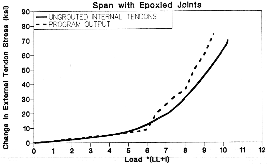
Figure 6.17 Change in external tendon stress (epoxy joints span - ungrouted internal tendons).
