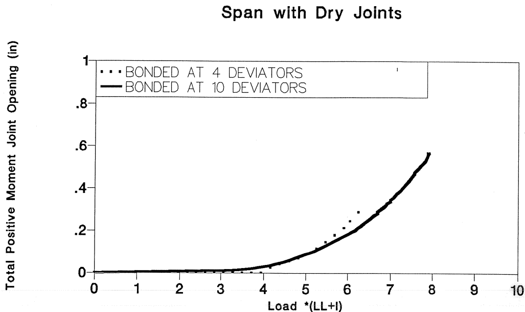
Figure 4.32 Effect of bonding on total positive moment joint opening for flexural strength tests of dry joints span.
