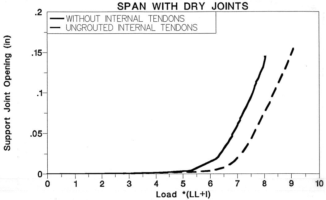
Figure 4.39 UngROUTED internal tendon effect on support joint opening-load for dry joints span.
