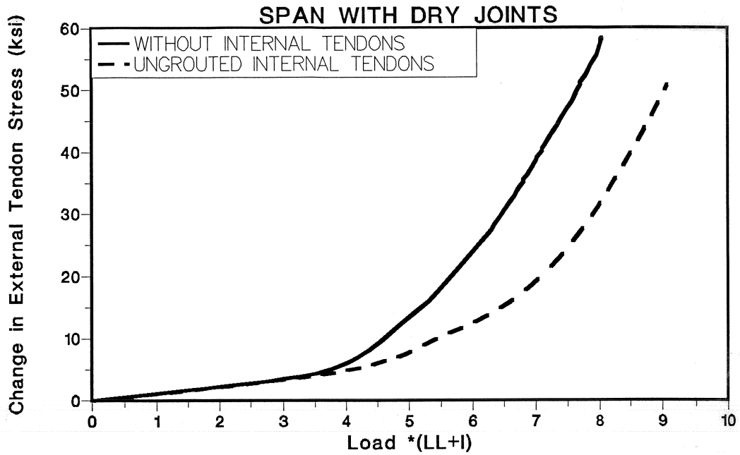
Figure 4.35 UngROUTed internal tendon effect on tendon stress-load for dry joints span.
