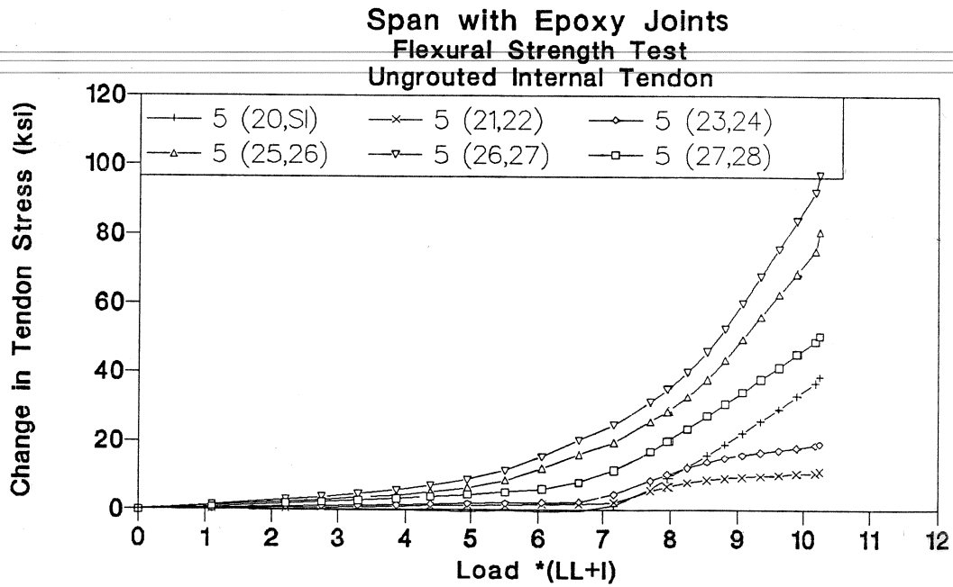
Figure 3.67 Tendon 5 stress-load ungrouted internal tendons test in epoxy joints span.
