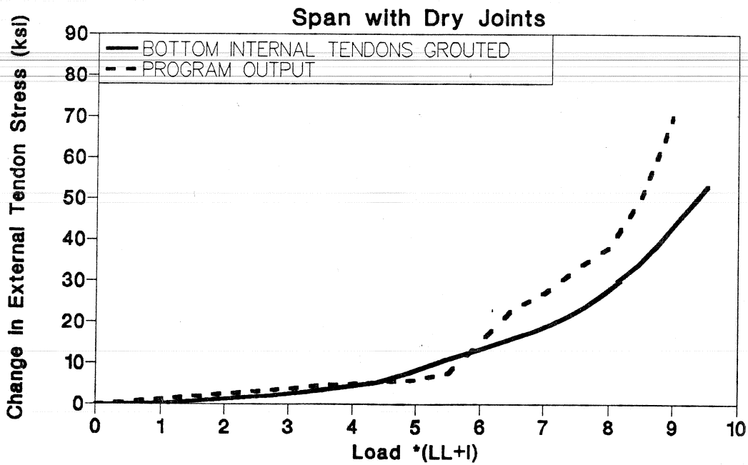
Figure 6.27 Change in external tendon stress (dry joints span - grouted internal tendons).
