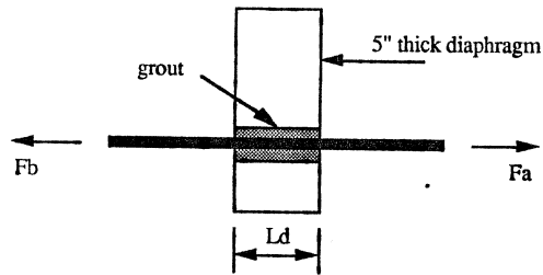
Elevation of Strand &amp; Intermediate Diaphragm
