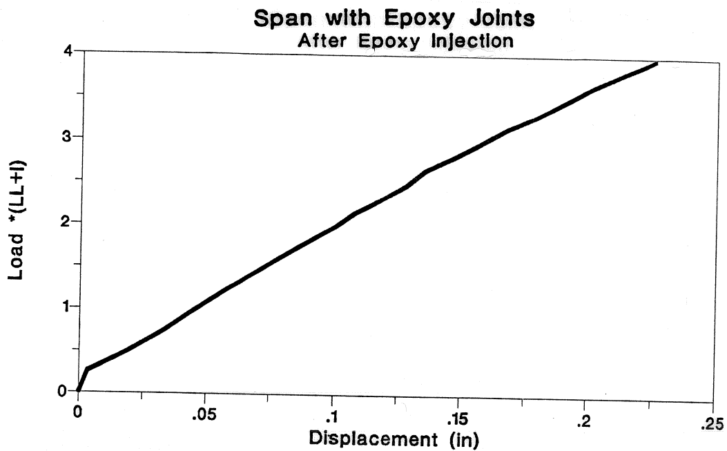
Figure 3.11 Load-deflection of injection cycle in epoxy joints span.
