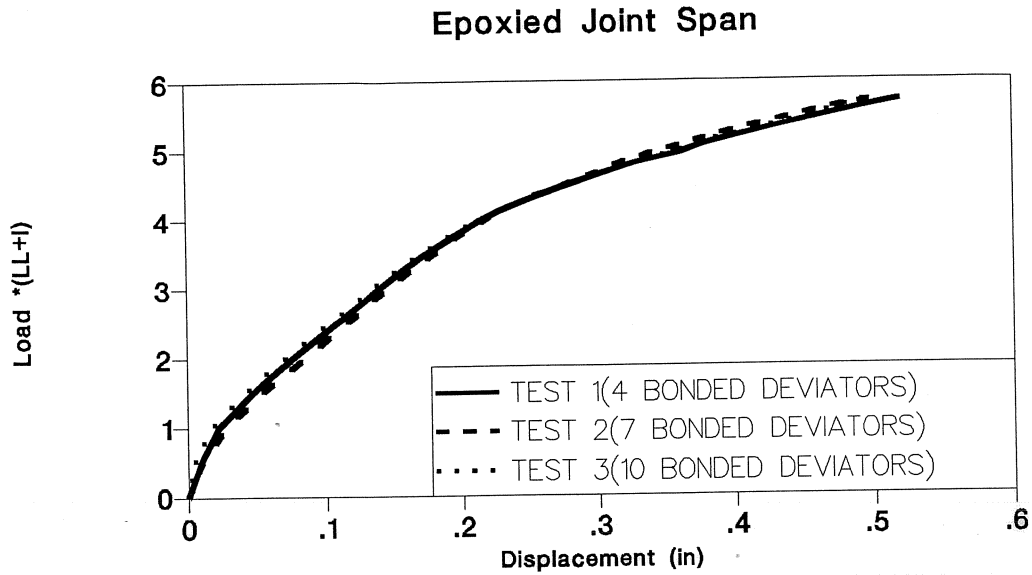
Figure 4.9 Effect of bonding on load-deflection response in epoxy joints span.
