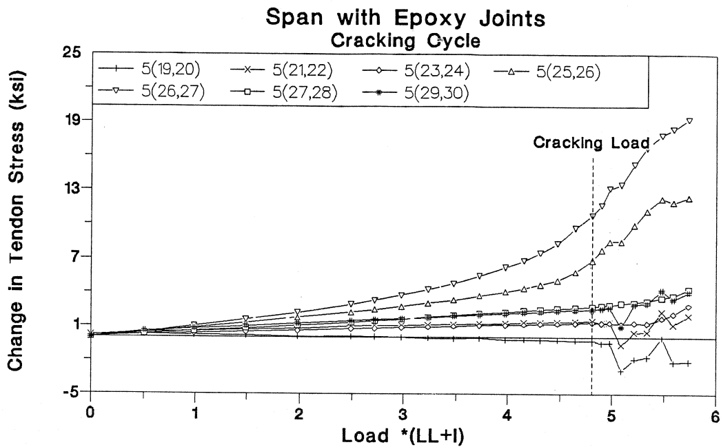
Figure 3.23 Tendon 5 stress-load of cracking cycle in epoxy joints span.
