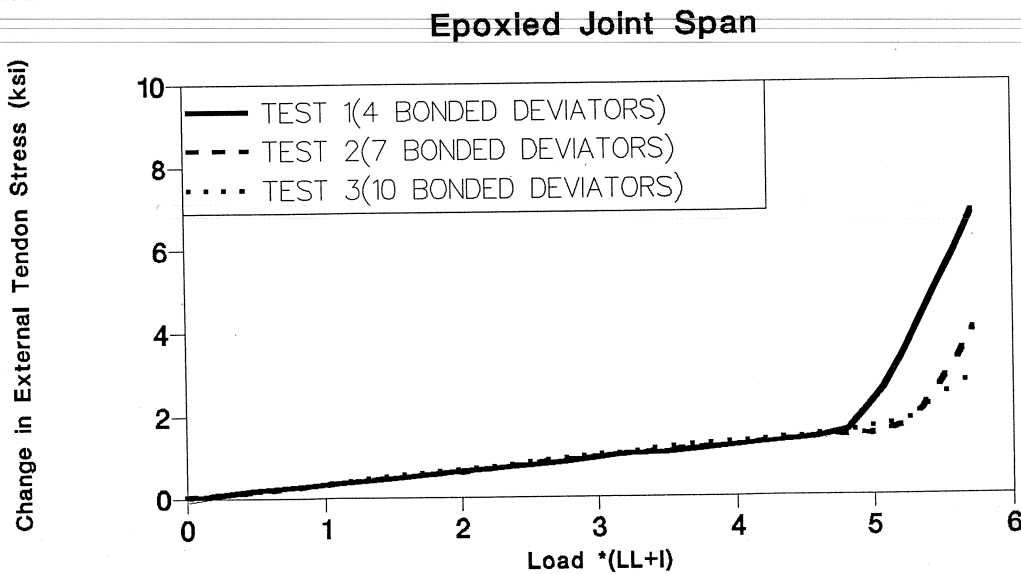
Figure 4.7 Effect of bonding on tendon slip in epoxy joints span.
