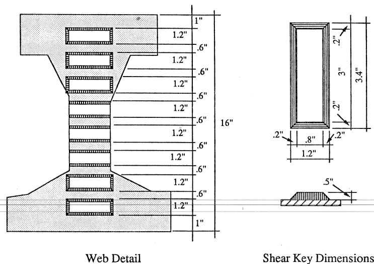
Figure 2.11 Shear key details [from Ref. (1)].
