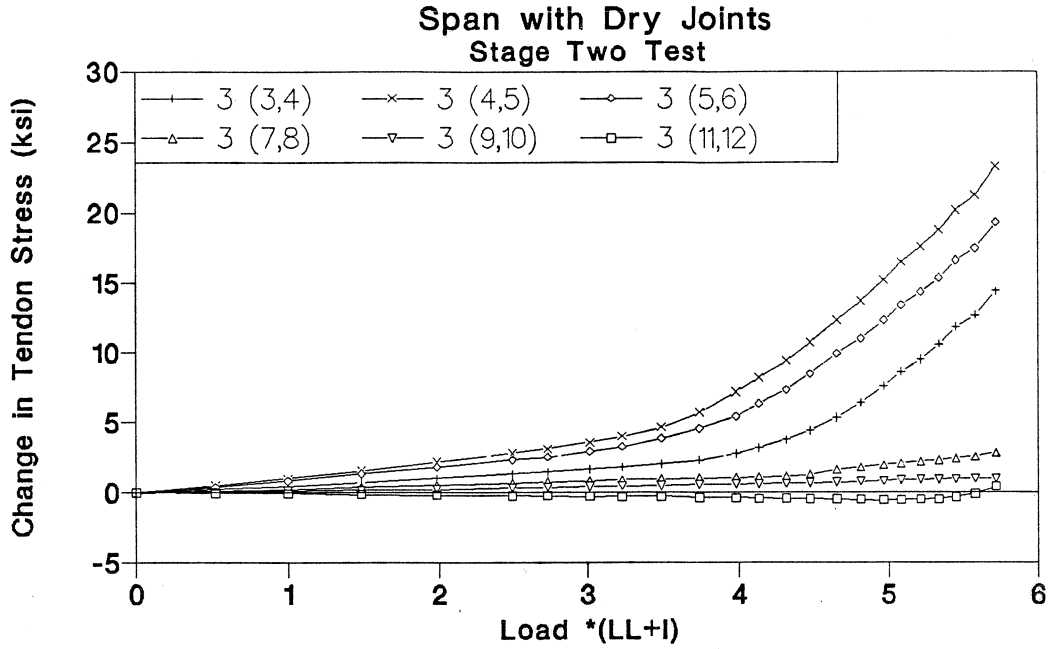
Figure 3.104 Tendon 3 stress-load of Stage Two in dry joints span.
