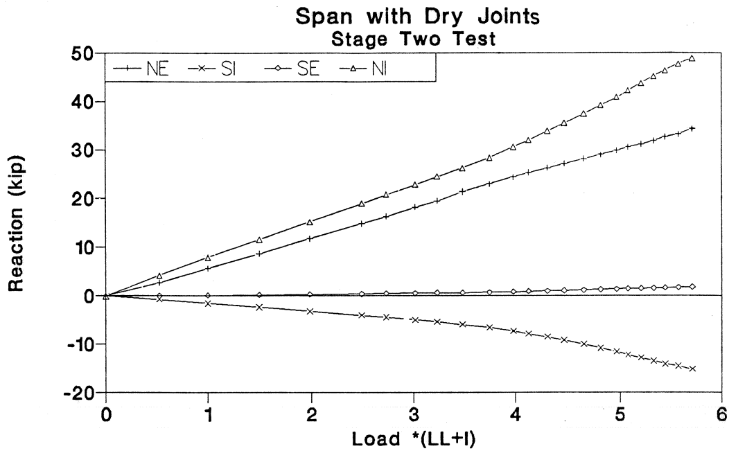
Figure 3.100 Reaction-load of Stage Two test in dry joints span.
