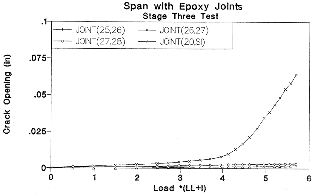
Figure 3.46 Crack opening-load of Stage Three test in epoxy joints span.
