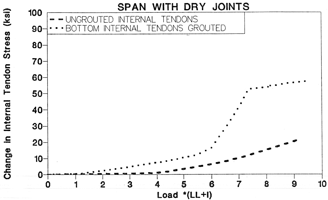
Figure 4.53 Grouted tendon effect on critical joint opening-load for dry joints span.
