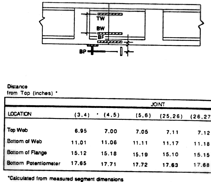
Figure 2.29 Web distortion and joint opening instrumentation [Ref. (1)].
