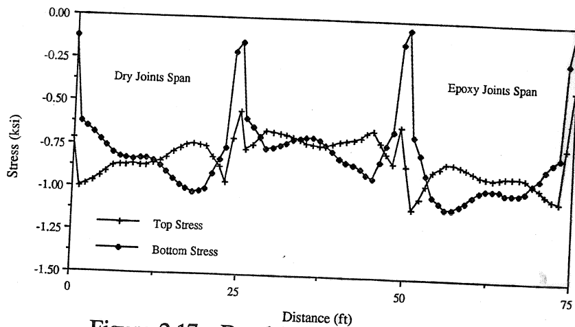
Figure 2.17 Dead load plus prestress stresses.
