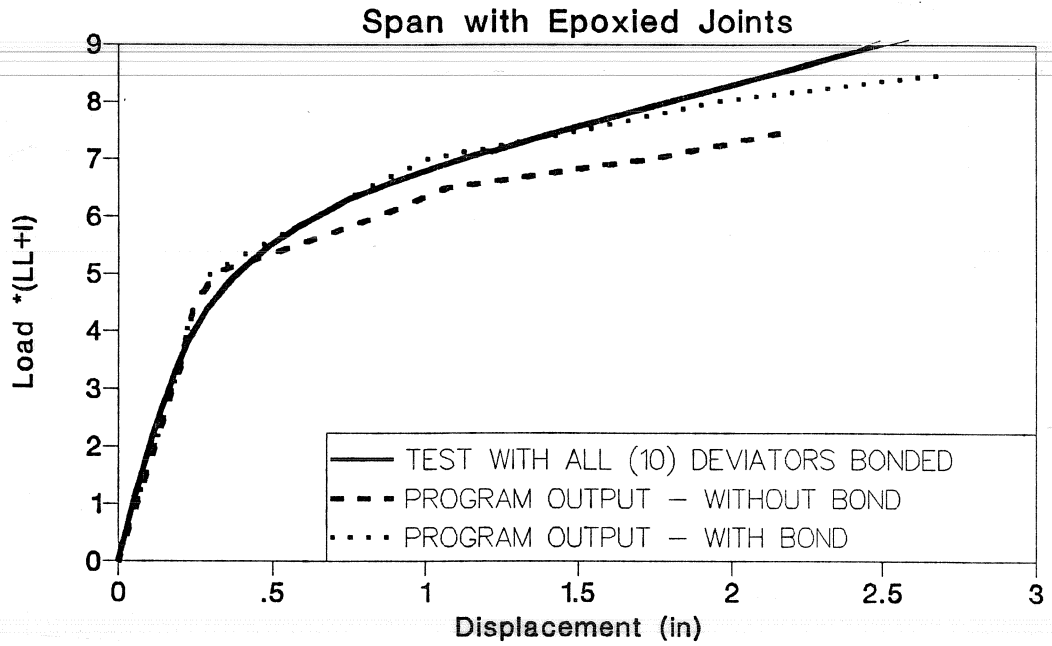
Figure 6.9 Load-deflection response (epoxy joints span without internal tendons).
