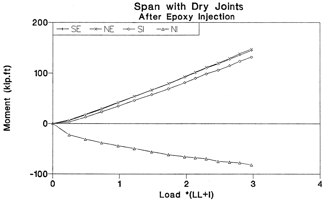
Figure 3.87 Moment-load of injection cycle in dry joints span.
