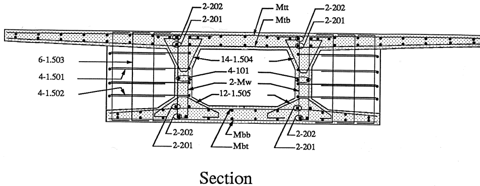
Figure 2.7 Typical segment reinforcement [from Ref. (1)].
