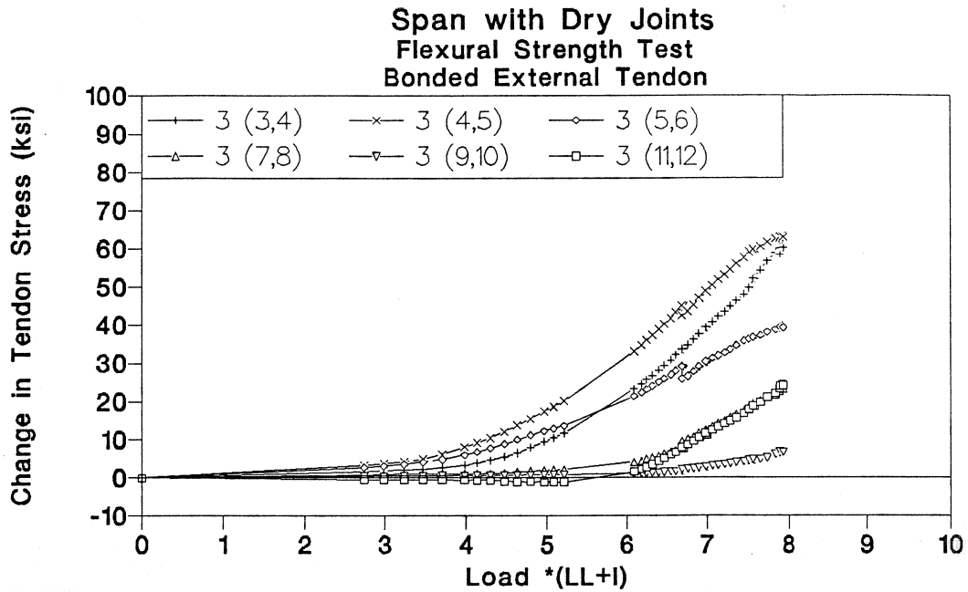
Figure 3.118 Tendon 3 stress-load of flexural strength test in dry joints span.
