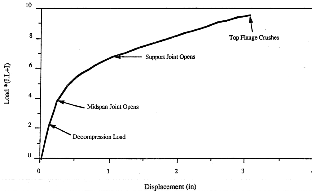
Figure 4.64 Stages of flexural behavior (epoxy joints span) for fully bonded external tendons.
