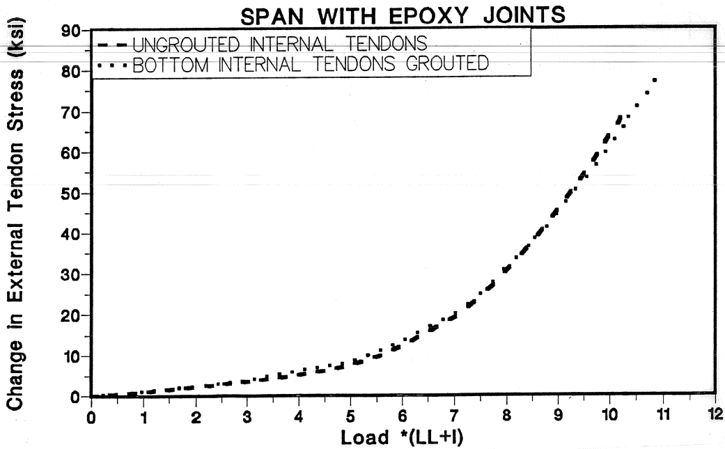
Figure 4.58 Grouted tendon effect on tendon stress-load for epoxy joints span.
