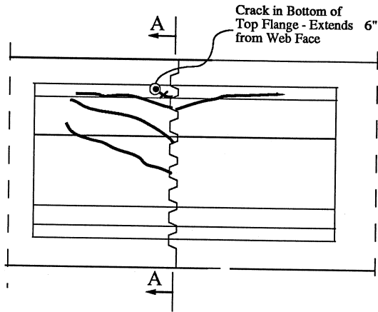
a) Crack in Dry Joints Span
