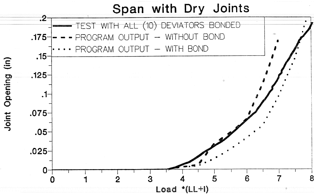
Figure 6.13 Joint opening response (dry joints span without internal tendons).
