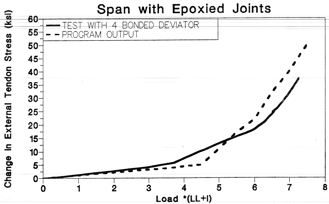
Figure 6.5 Change in external tendon stress (epoxy joints span - initial strength test).
