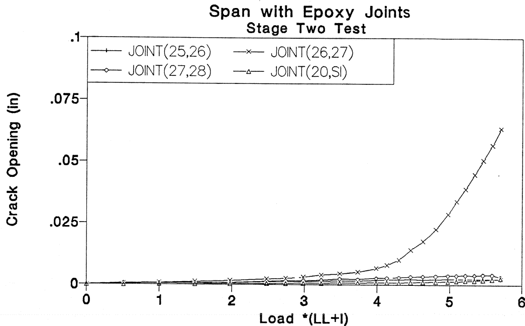
Figure 3.39 Crack opening-load of Stage Two test in epoxy joints span.
