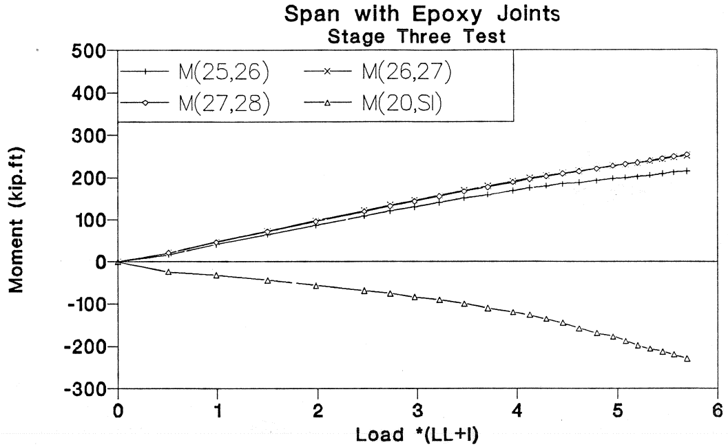
Figure 3.42 Moment-load of Stage Three test in epoxy joints span.
