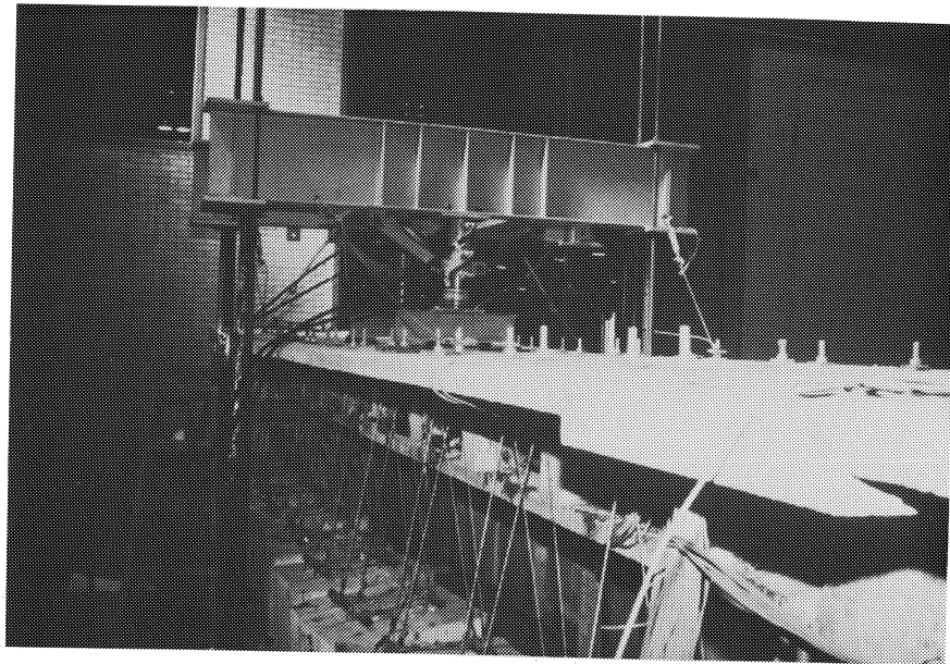
Figure 3.3 Load frame.
