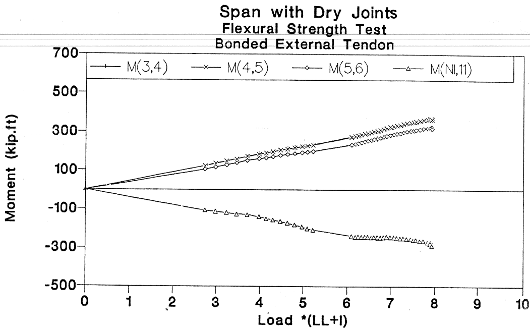
Figure 3.115 Moment-load of flexural strength test in dry joints span.
