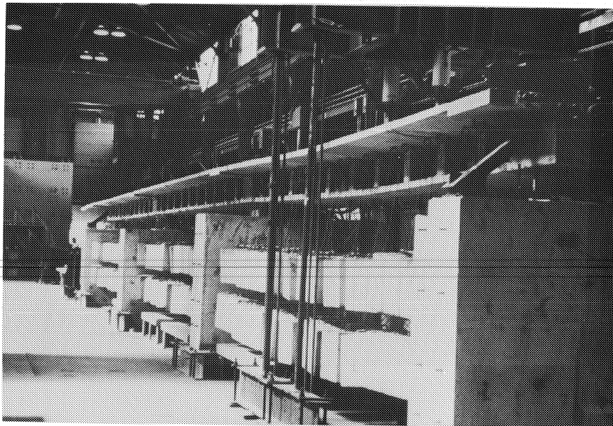
Figure 1. Model of externally post-tensioned bridge.
