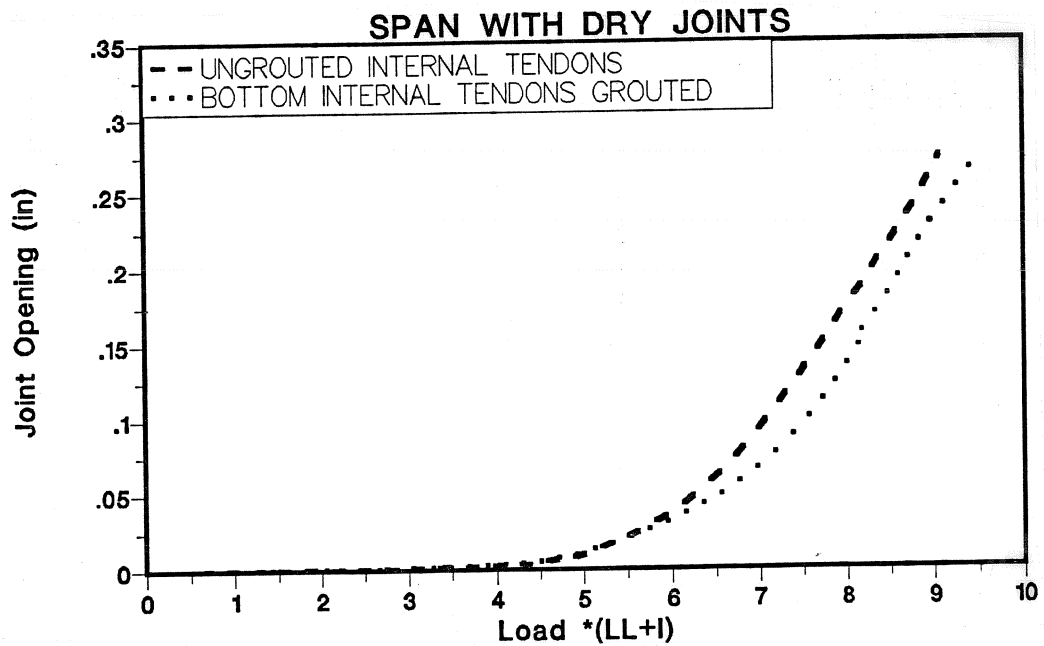
Figure 4.52 Grouted tendon effect on internal tendon stress-load for dry joints span.
