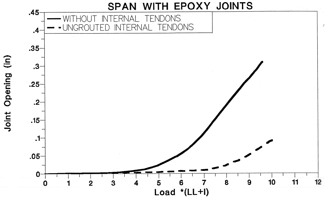
Figure 4.46 UngROUTed tendon effect on adjacent joint opening-load for epoxy joints span.
