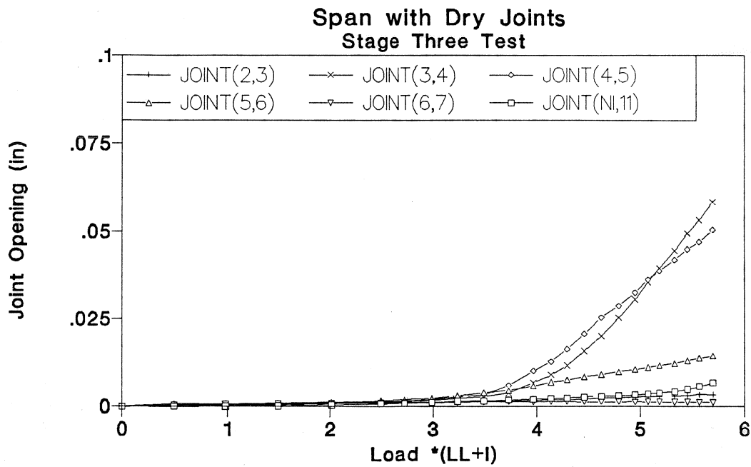
Figure 3.112 Joint opening-load of Stage Three test in dry joints span.
