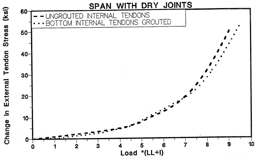
Figure 4.51 Grouted tendon effect on tendon stress-load for dry joints span.
