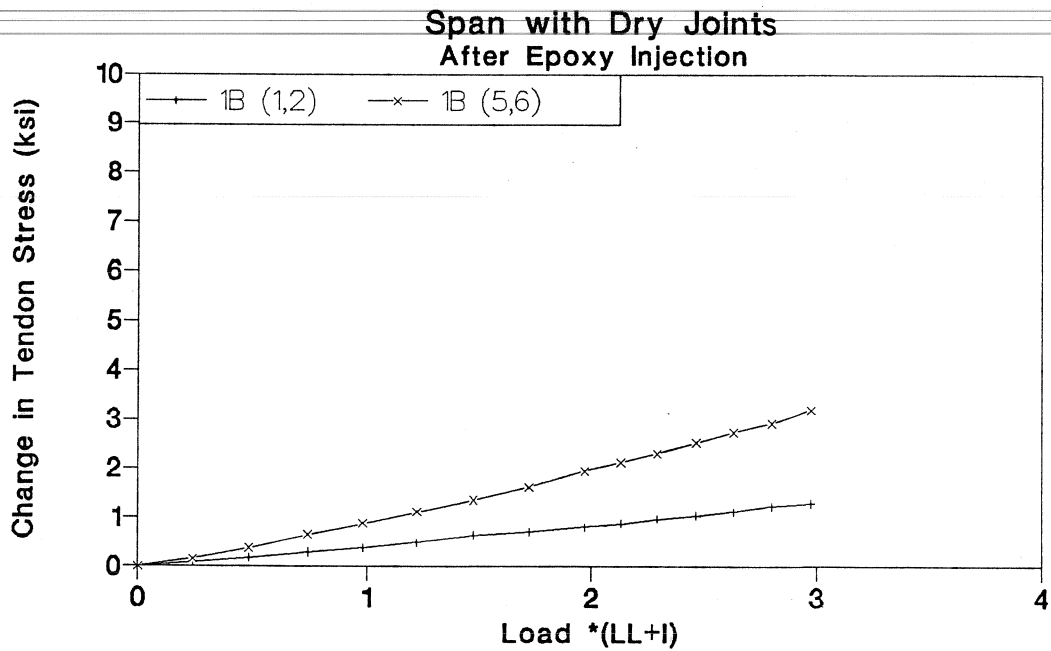
Figure 3.89 Tendon 1B stress-load of inject cycle in dry joints span.
