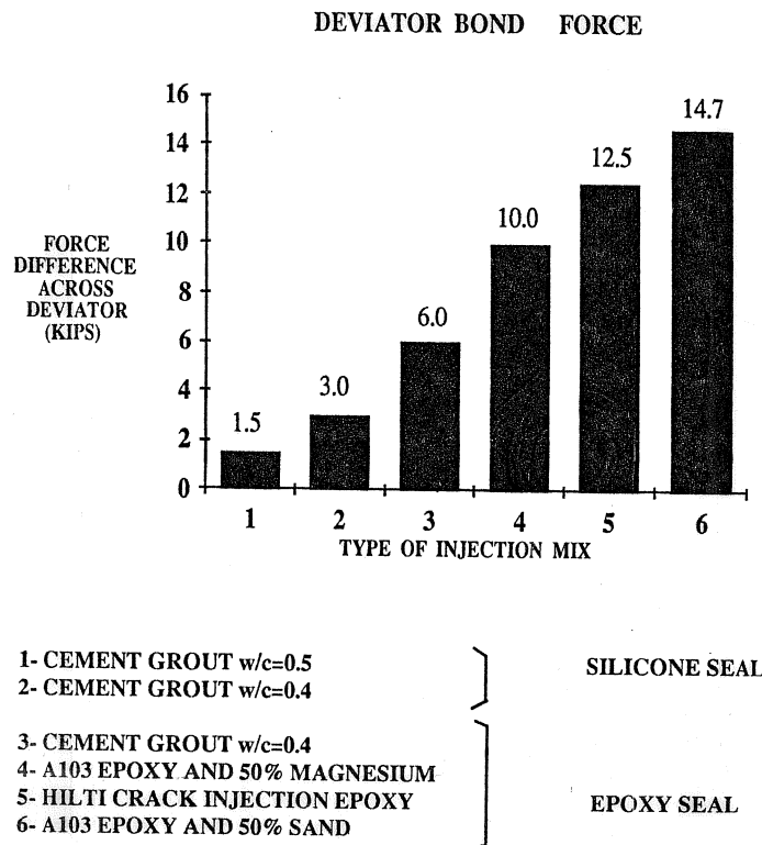
Figure 2.25 Bond tests.
