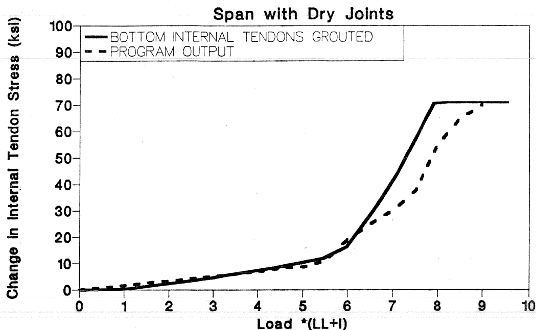
Figure 6.28 Internal tendon stress (dry joints span - gouted internal tendons).
