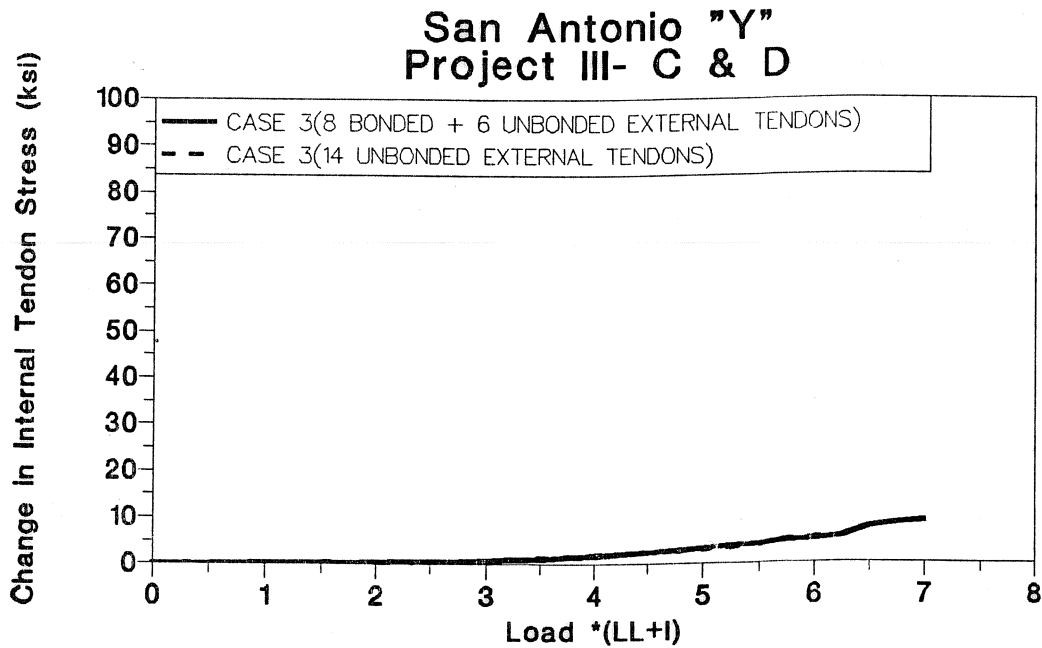
Figure 7.12 Internal tendon stress (Case Three - Effect of bonding).
