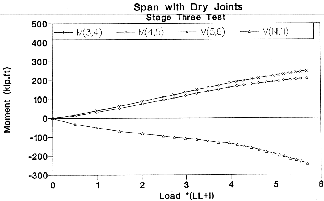
Figure 3.108 Moment-load of Stage Three in dry joints span.
