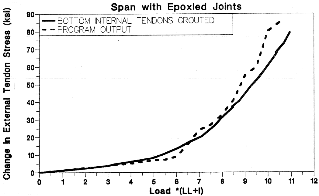
Figure 6.23 Change in external tendon stress (epoxy joints span - grouted internal tendons).
