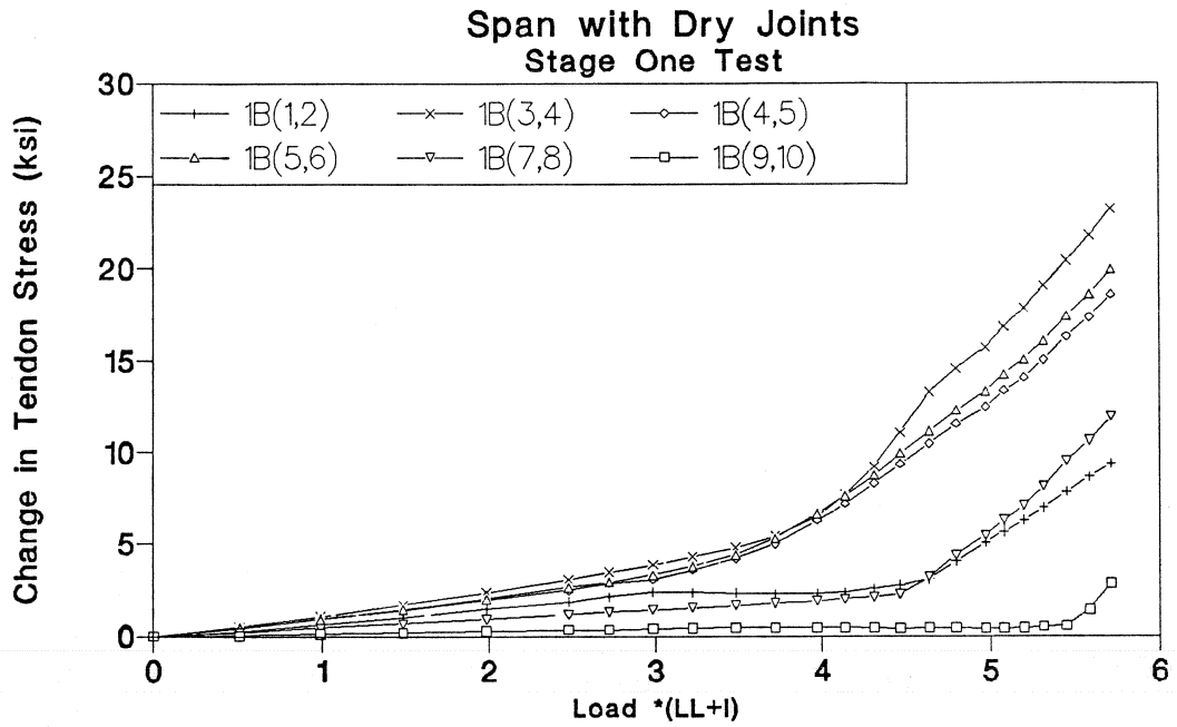
Figure 3.96 Tendon 1B stress-load of Stage One test in dry joints span.
