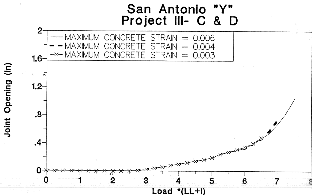
Figure 7.26 Joint opening (maximum concrete strain).
