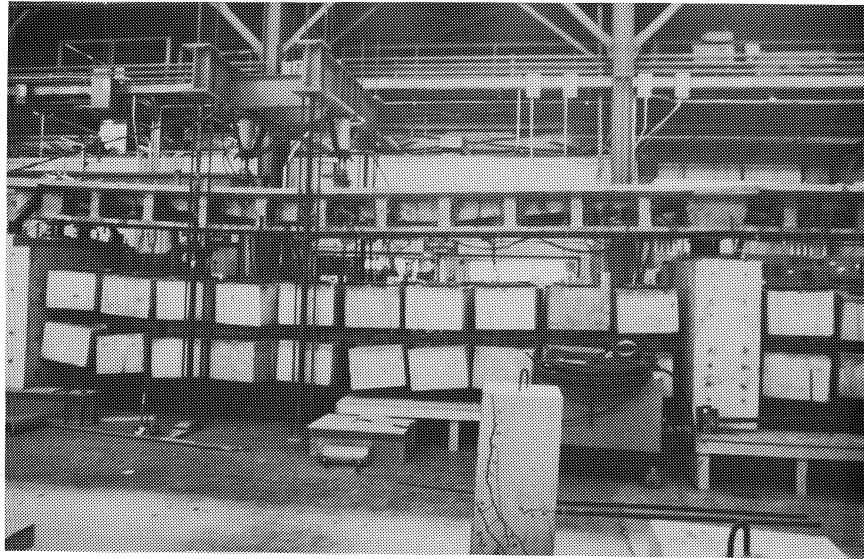
Figure 4.63 Deflection of the model at ultimate load.
