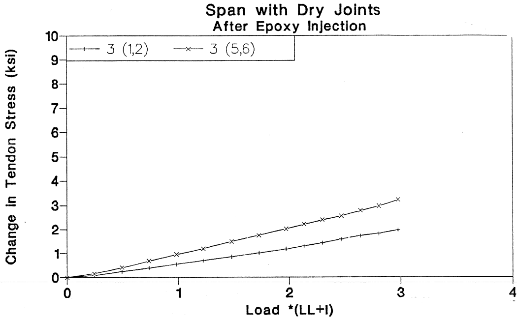
Figure 3.90 Tendon 3 stress-load of injection cycle in dry joints span.
