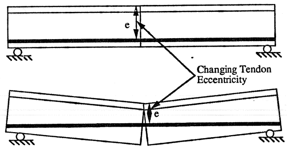
a) Without Intermediate Deviators
