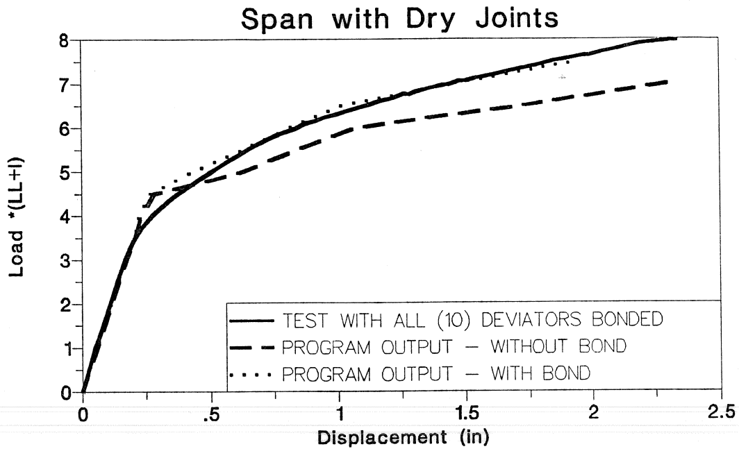
Figure 6.12 Load-deflection response (dry joints span without internal tendons).
