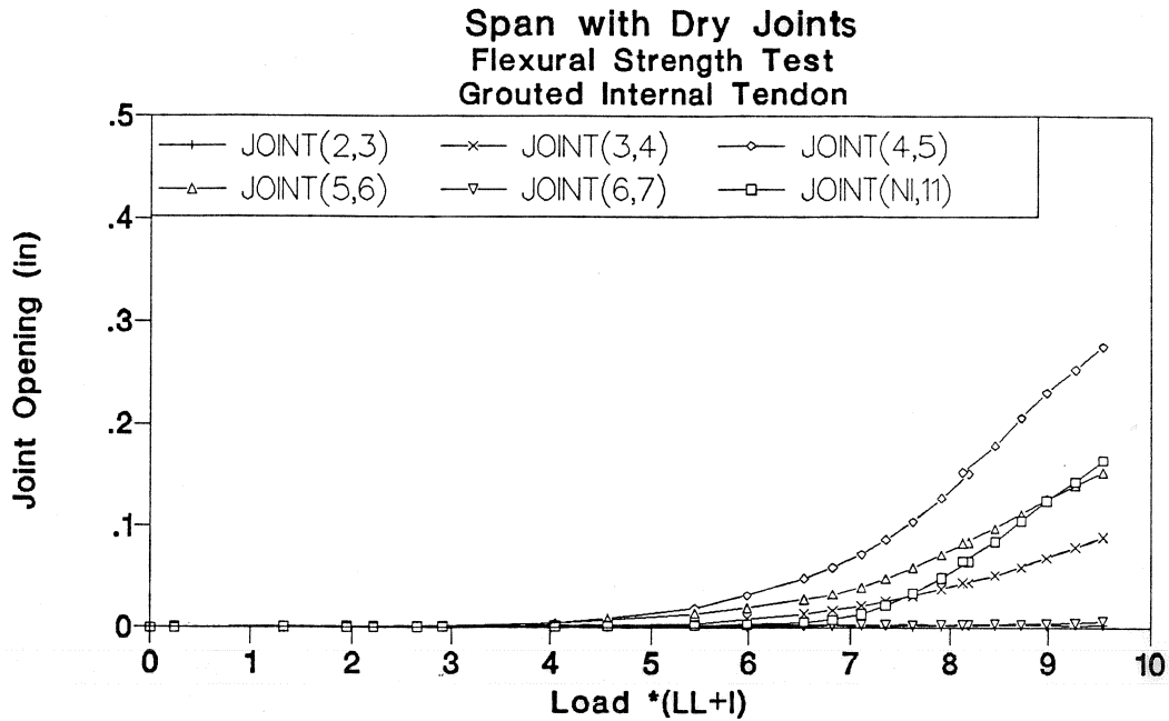
Figure 1.136 Joint opening-load of grouted internal tendon test in dry joints span.
