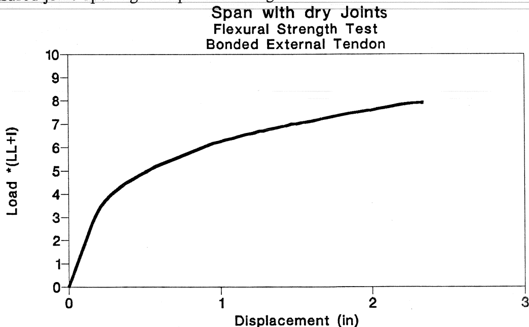
Figure 3.113 Load-deflection of flexural strength test in dry joints span.
