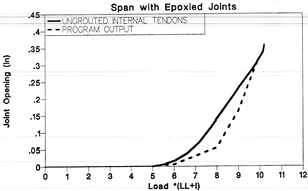
Figure 6.16 Joint opening response (epoxy joints span - ungrouted internal tendons).
