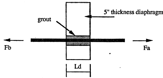
Elevation of Strand & Intermediate Diaphragm
