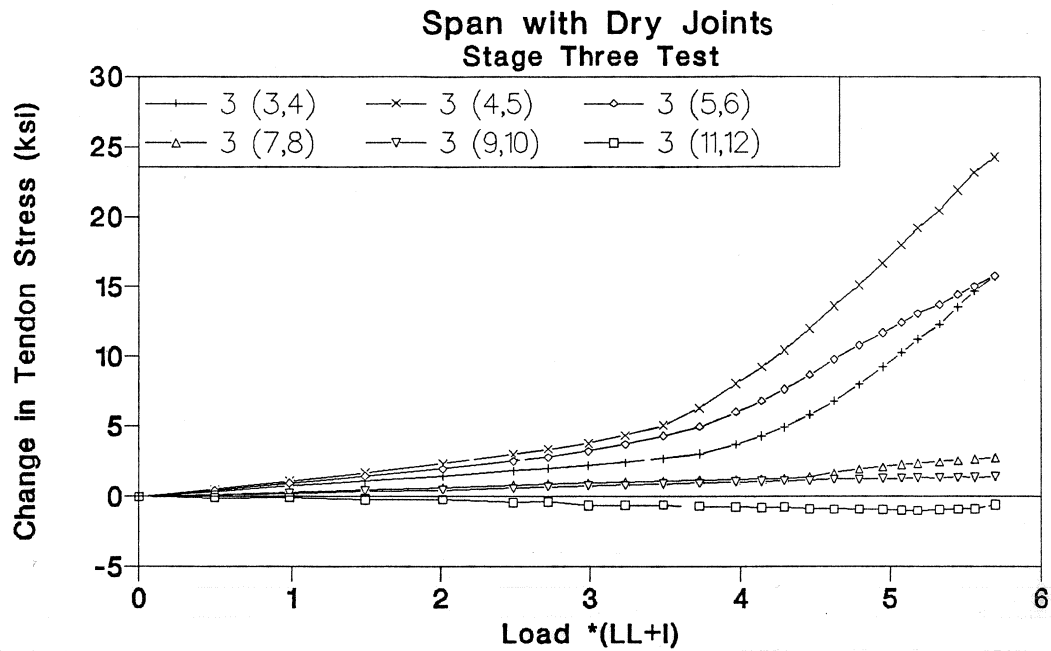
Figure 3.111 Tendon 3 stress-load of Stage Three test in dry joints span.
