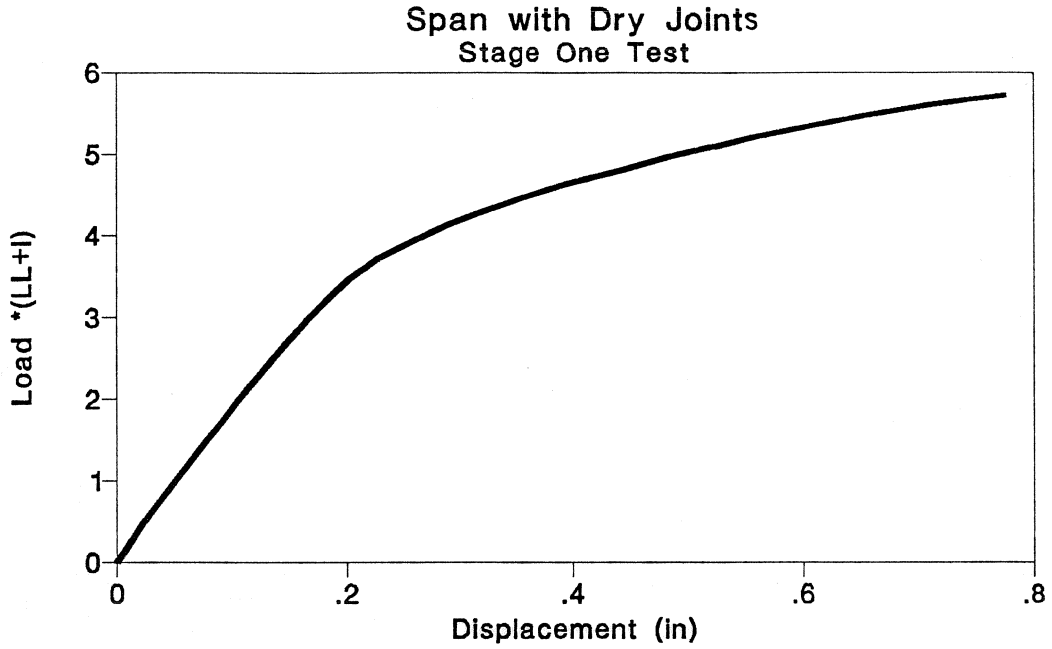
Figure 3.92 Load-deflection of Stage One test in dry joints span.
