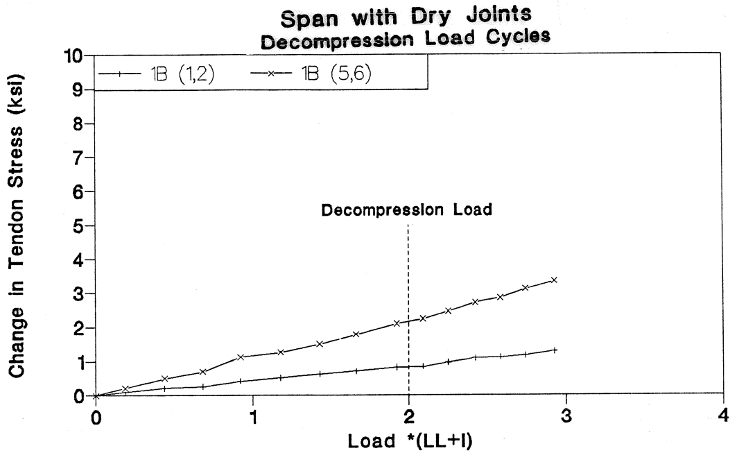
Figure 3.83 Tendon 1B stress-load of decompression cycle in dry joints span.
