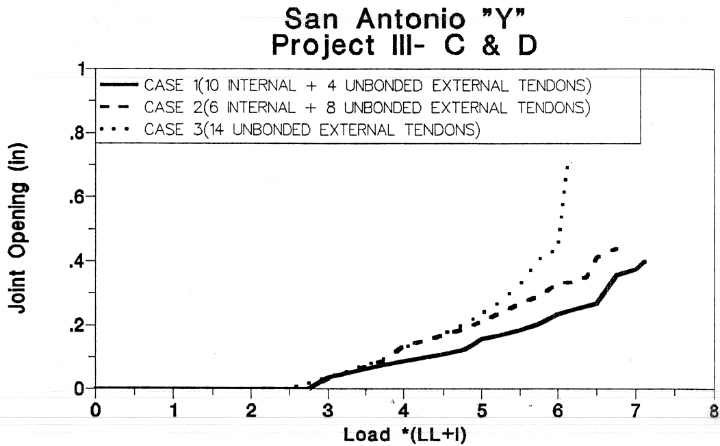
Figure 7.19 Joint opening (effect of internal tendons - unbonded external tendons).
