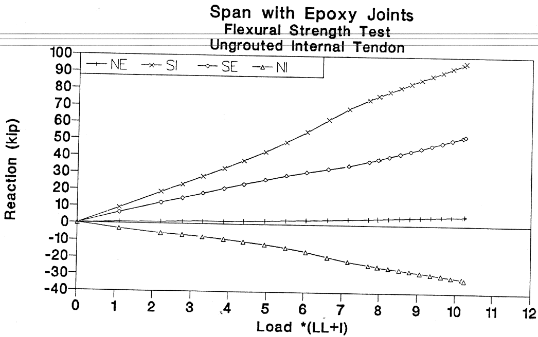
Figure 3.63 Reaction-load of ungrouted internal tendons test in epoxy joints span.
