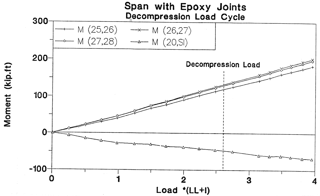
Figure 3.7 Moment-load of decompression cycle in epoxy joints span.
