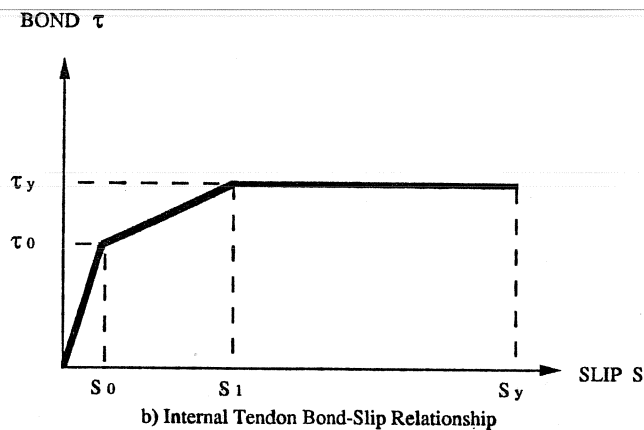
Figure 5.3 Bond-slip relationships.
