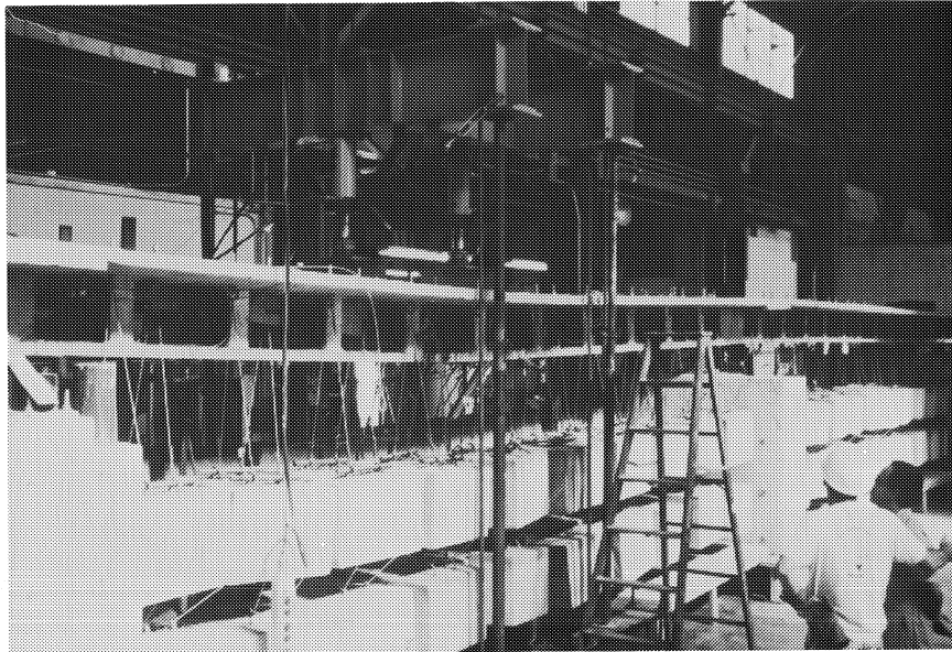
Figure 4.15 Deflected shape of the model for the fully bonded strength test.
