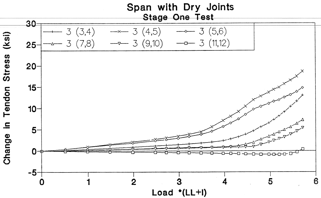
Figure 3.97 Tendon 3 stress-load of Stage One test in dry joints span.
