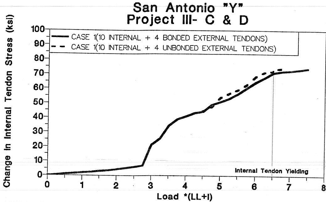
Figure 7.4 Internal tendon stress (Case One - Effect of bonding).
