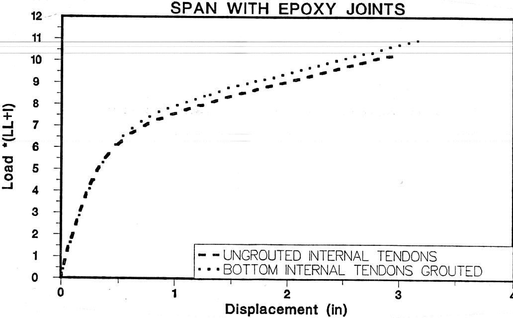
Figure 4.56 Grouted tendon effect on load-deflection response of epoxy joints span.
