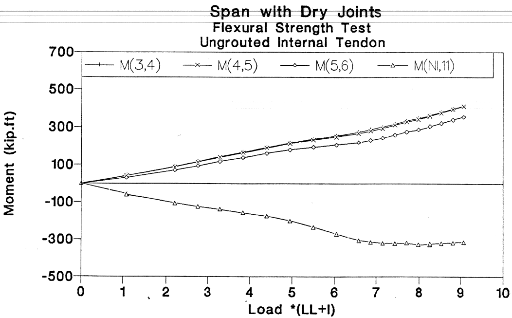
Figure 3.123 Moment-load of ungrouted internal tendon test in dry joints span.
