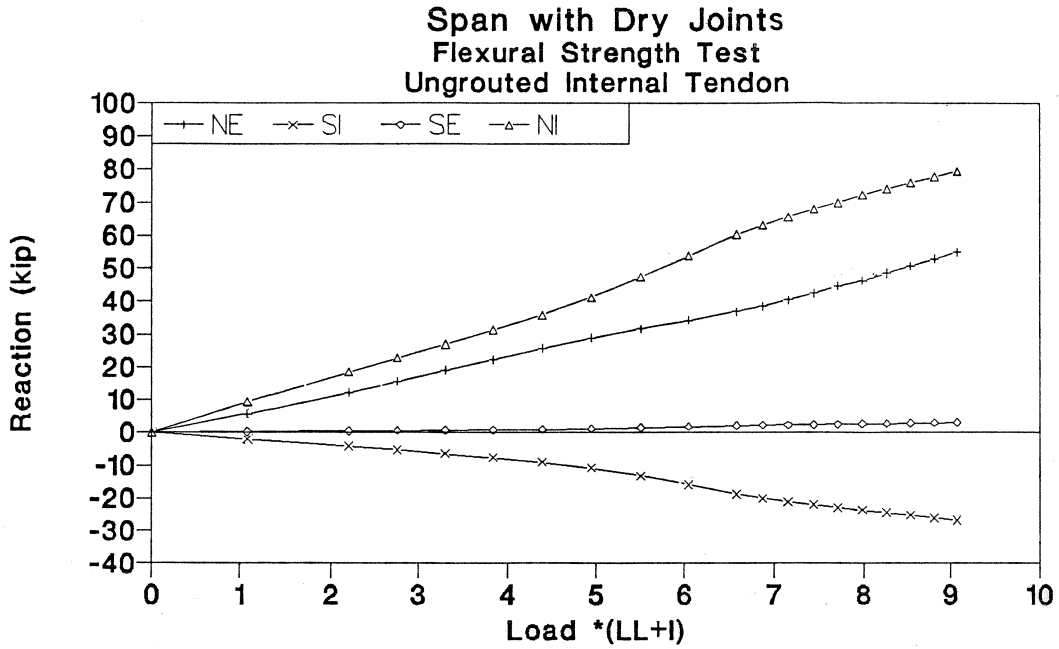
Figure 3.122 Reaction-load of ungrouted internal tendon test in dry joints span.
