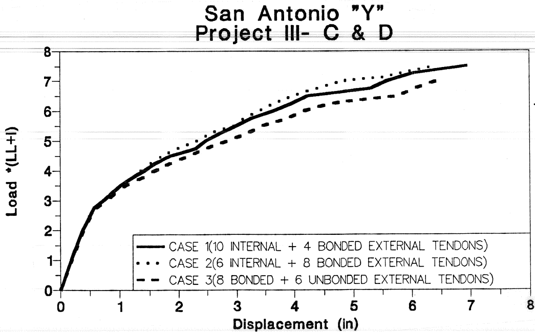
Figure 7.20 Load-displacement (effect of internal tendons - bonded external tendons).
