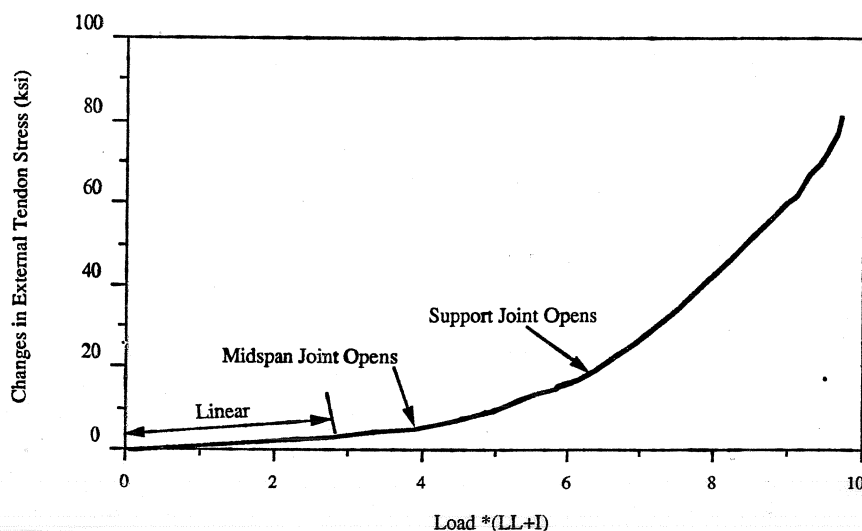
Figure 4.80 Typical tendon stress response (epoxy joints span).
