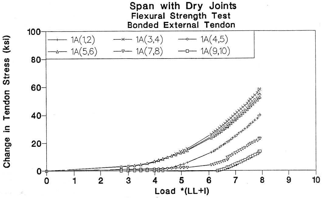
Figure 3.116 Tendon 1A stress-load of flexural strength test in dry joints span.
