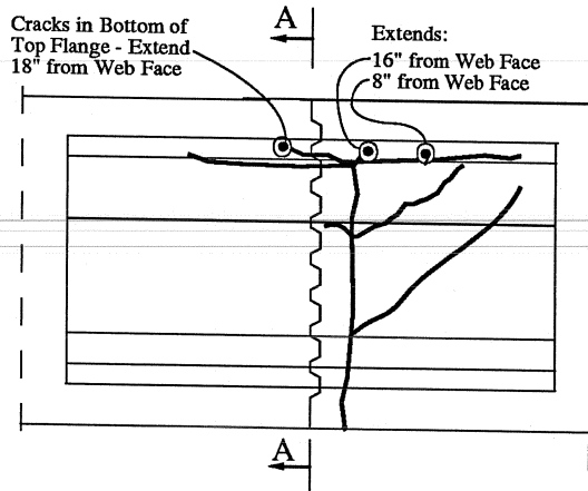
b) Crack in Epoxy Joints Span
