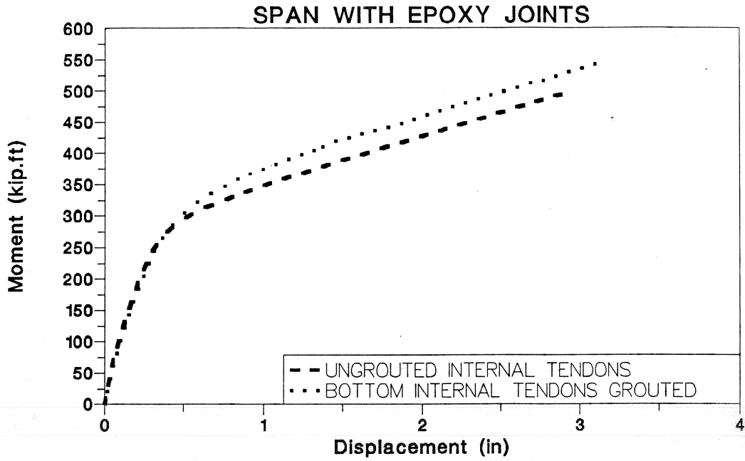
Figure 4.57 Grouted tendon effect on moment-deflection for epoxy joints span.
