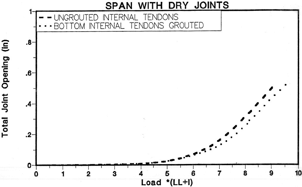
Figure 4.55 Grouted tendon effect on total joint opening-load for dry joints span.
