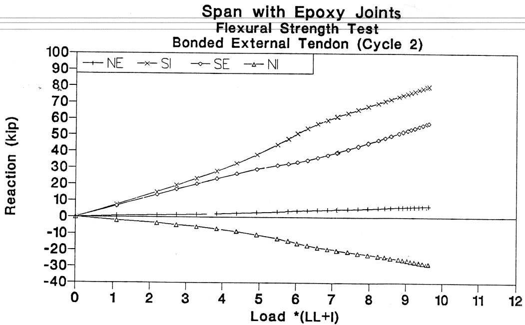
Figure 3.55 Reaction-load of flexural strength test (cycle 2) in epoxy joints span.
