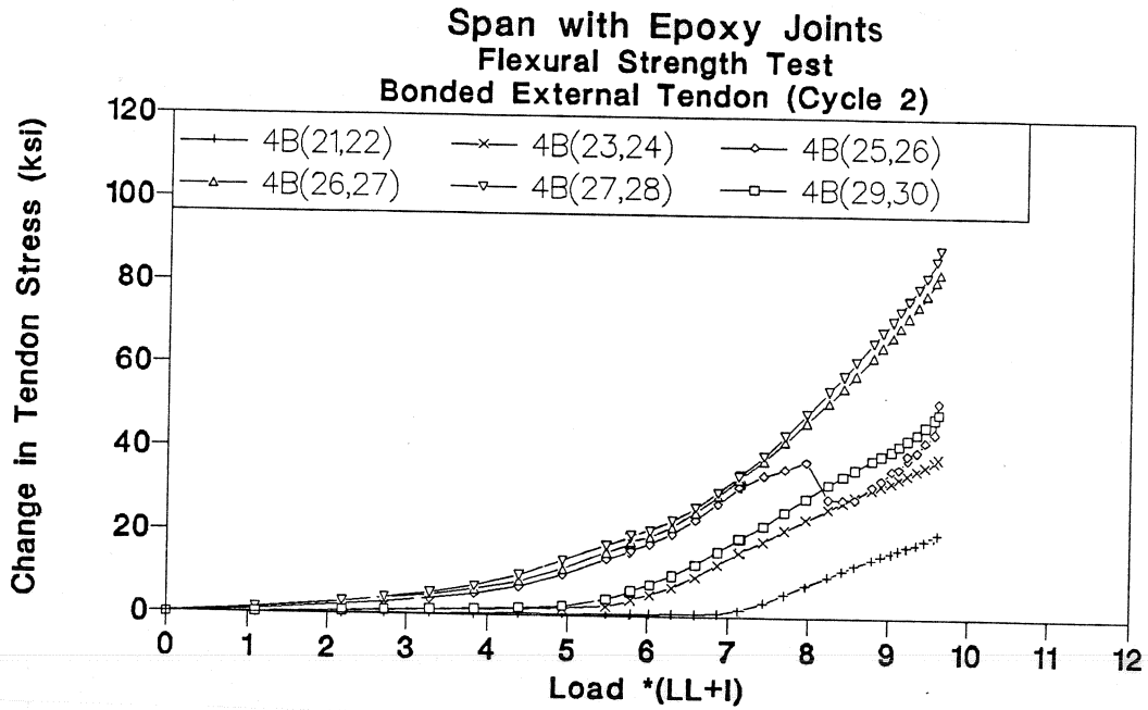
Figure 3.58 Tendon 4B stress-load of flexural strength test (cycle 2) in epoxy joints span.
