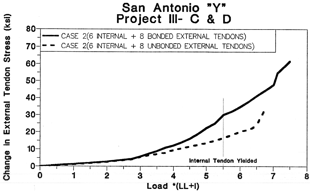
Figure 7.9 External tendon stress (Case Two - Effect of bonding).
