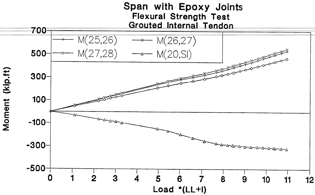
Figure 3.73 Moment-load of grouted internal tendons test in epoxy joints span.
