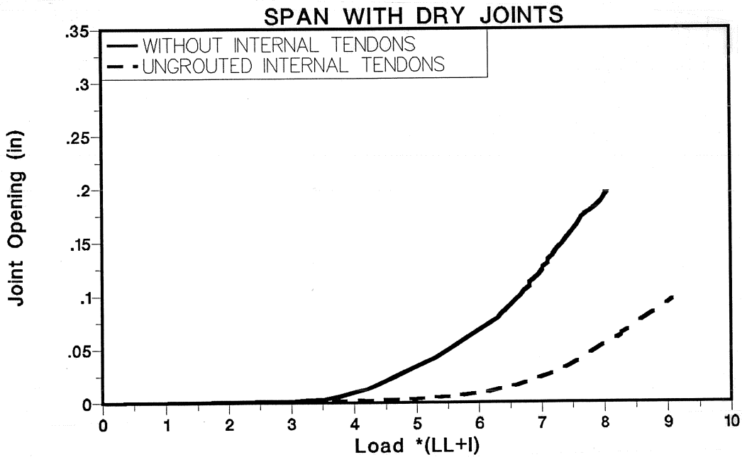
Figure 4.38 UngROUTED internal tendon effect on adjacent joint opening-load for dry joints span.
