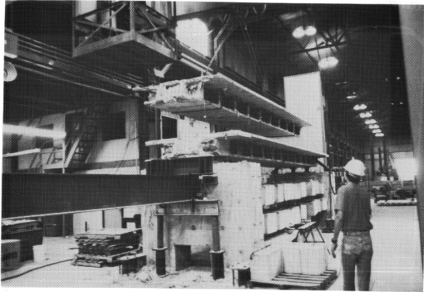
Figure 2.36 Supporting beams.
