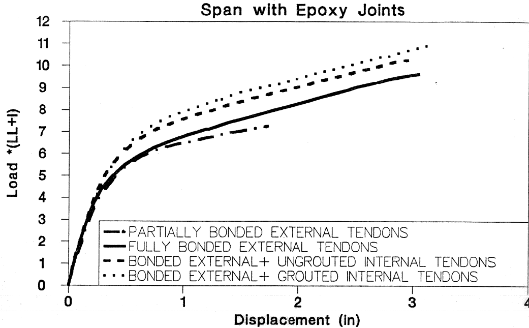
Figure 4.76 Effect of bonding and grouted internal tendons on strength and ductility of epoxy joints span.
