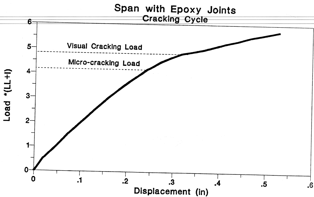
Figure 3.18 Load-deflection of cracking cycle in epoxy joints span.
