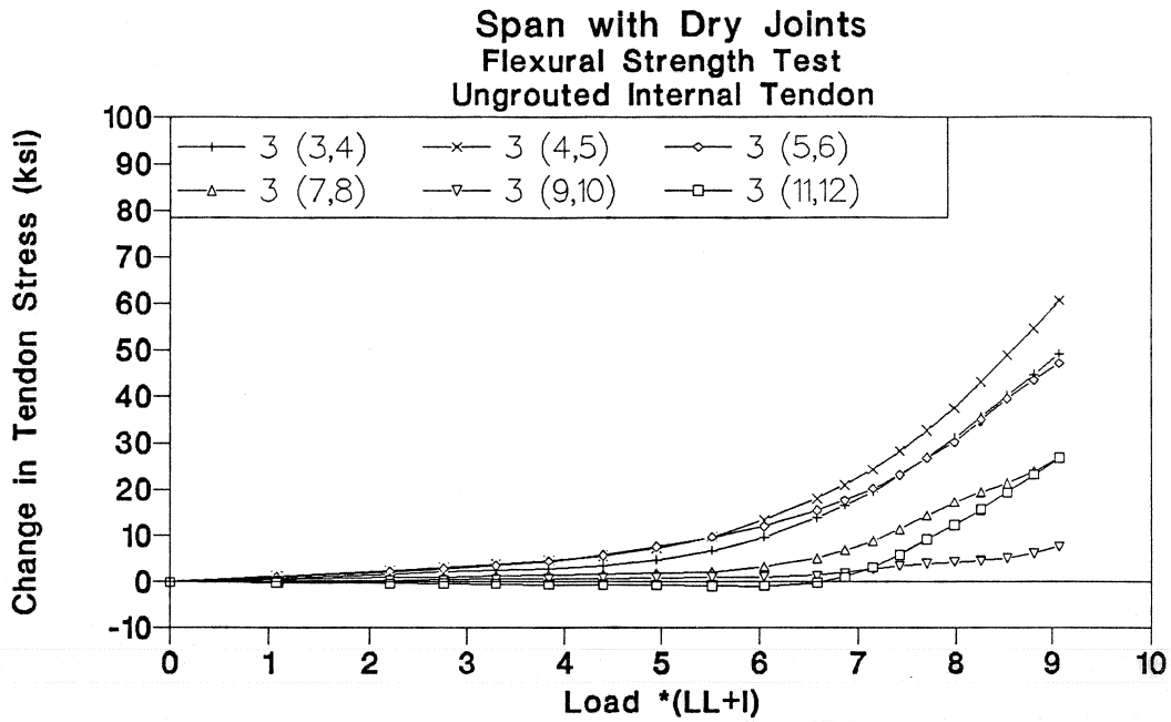
Figure 3.126 Tendon 3 stress-load of ungrouted internal tendon test in dry joints span.
