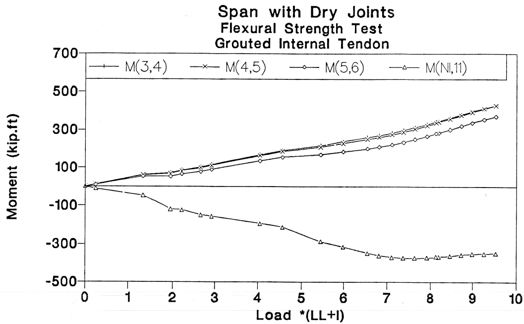
Figure 3.132 Moment-load of grouted internal tendon test in dry joints span.
