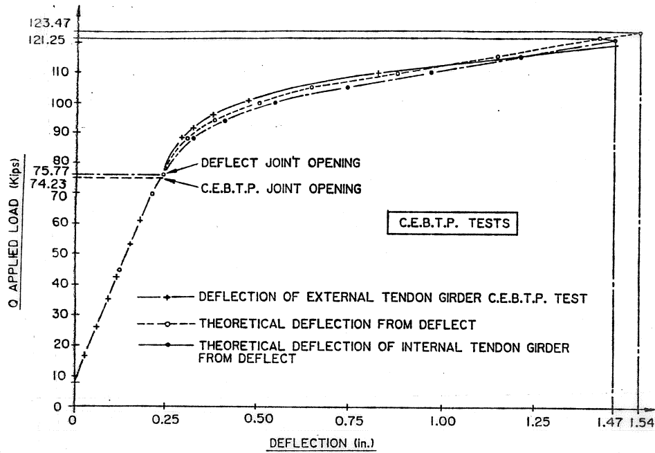
Figure 1.12 Load-deflection response predictions by defect for CEBTP test specimen [From Ref. (6)].
