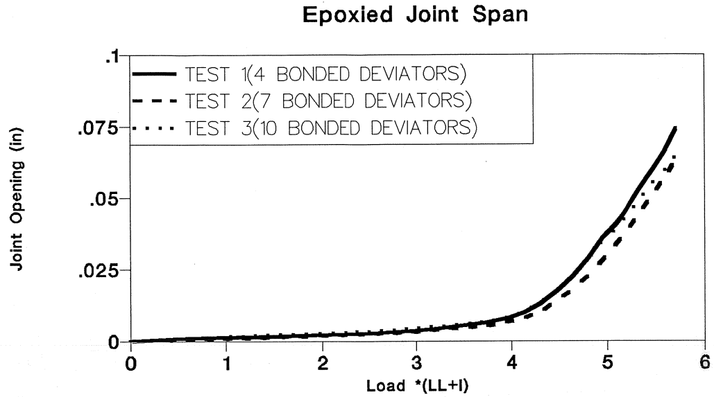
Figure 4.11 Effect of bonding on joint opening in epoxy joints span.
