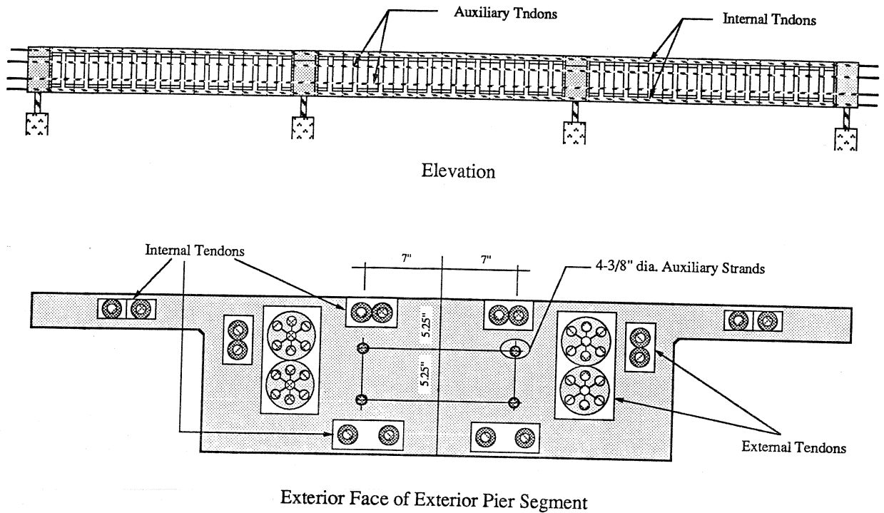
Figure 2.5 Internal and auxiliary tendons.
