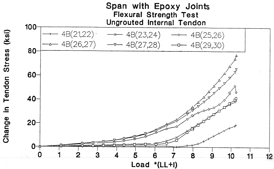
Figure 3.66 Tendon 4B stress-load of ungrouted internal tendons test in epoxy joints span.
