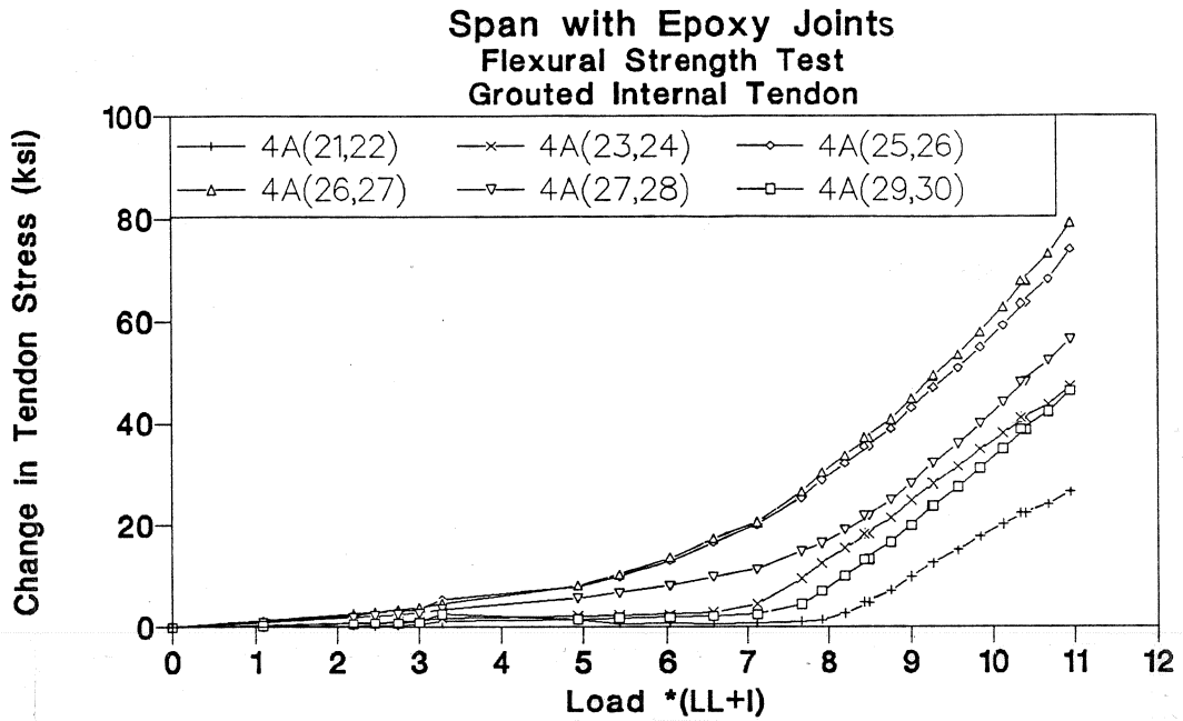
Figure 3.74 Tendon 4A stress-load of grouted internal tendons test in epoxy joints span.
