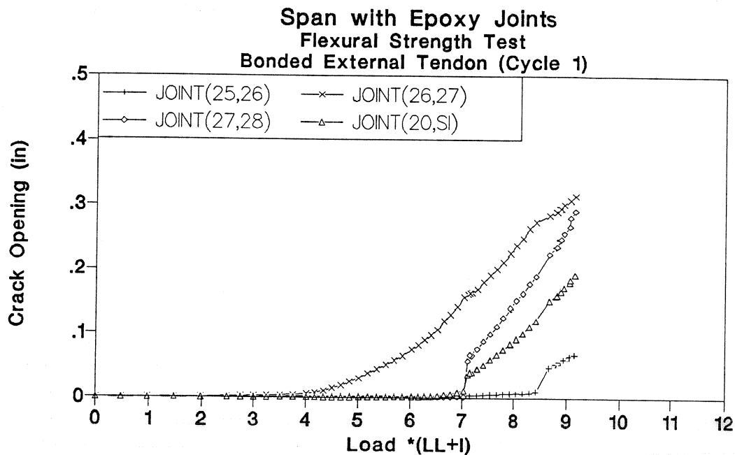
Figure 3.53 Crack opening-load of flexural strength test (cycle 1) in epoxy joints span.
