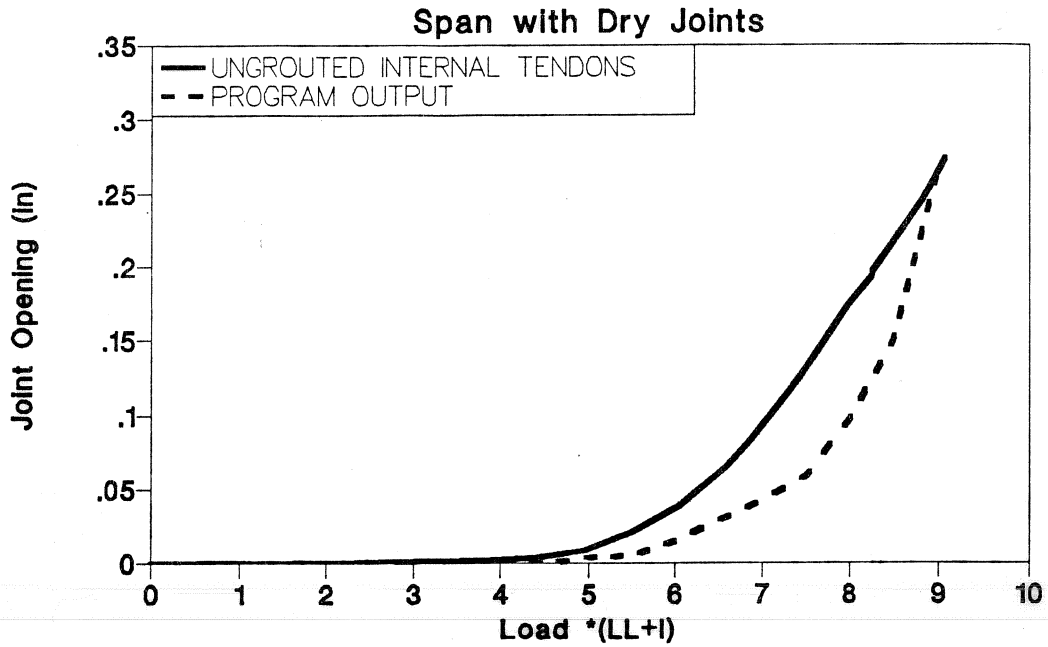
Figure 6.19 Joint opening response (dry joints span - ungrouted internal tendons).
