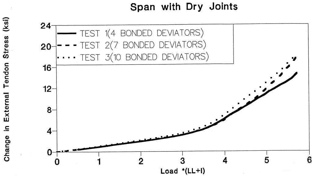
Figure 4.13 Effect of bonding on change in tendon stress in dry joints span.
