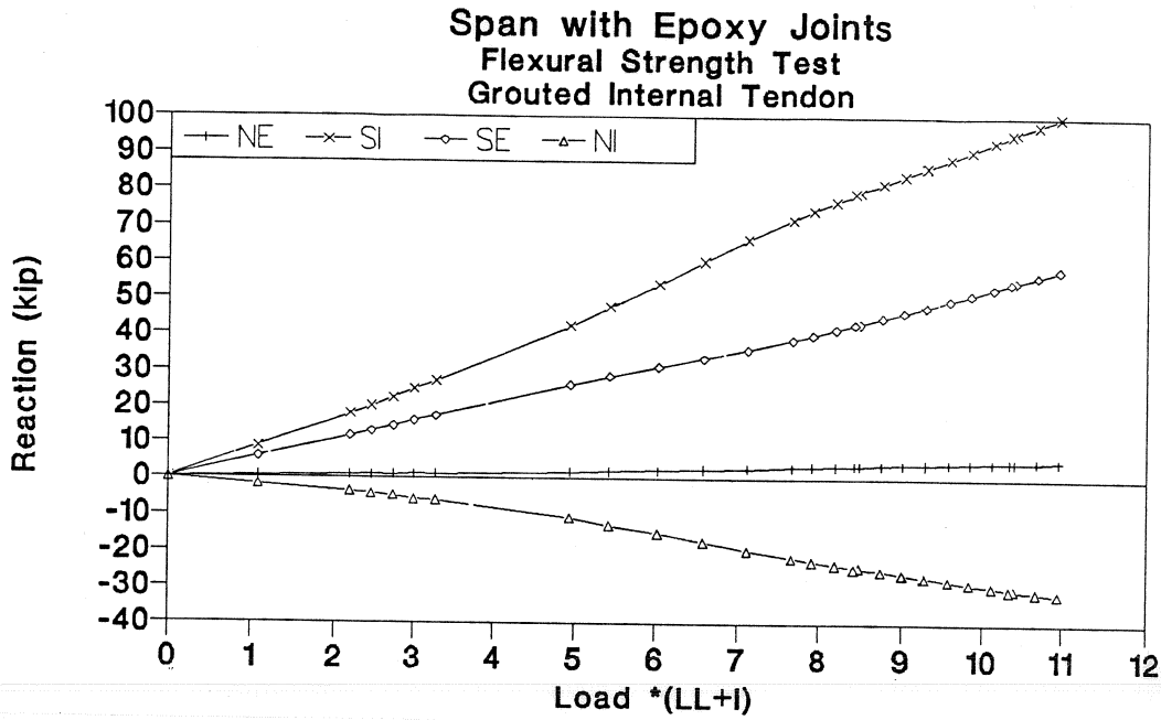
Figure 3.72 Reaction-load of grouted internal tendons test in epoxy joints span.
