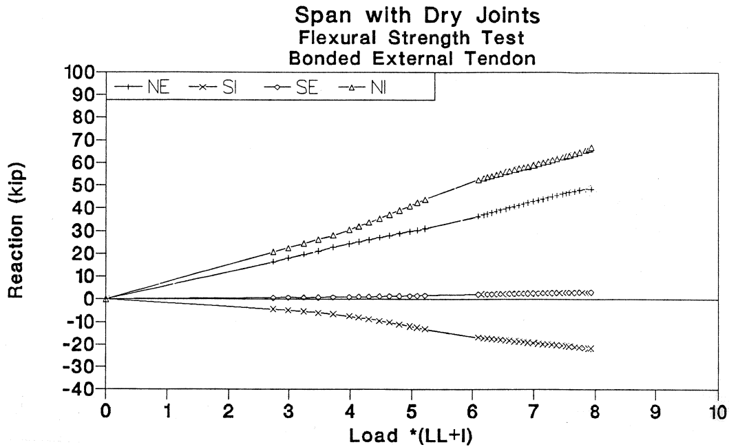
Figure 3.114 Reaction-load of flexural strength test in dry joints span.
