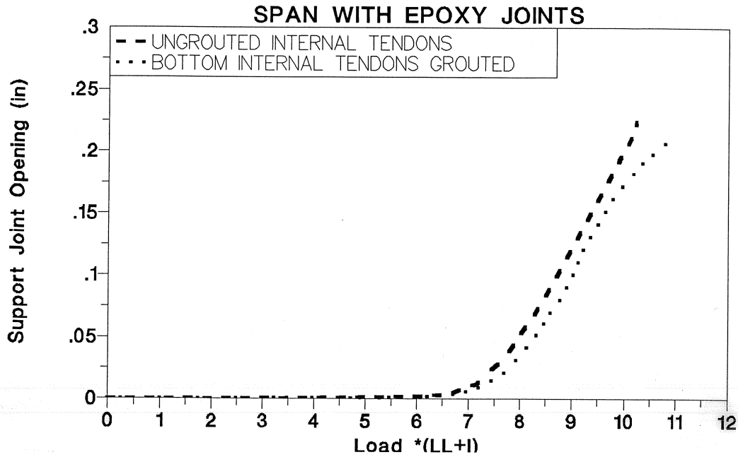
Figure 4.61 Grouted tendon effect on support joint opening-load for epoxy joints span.
