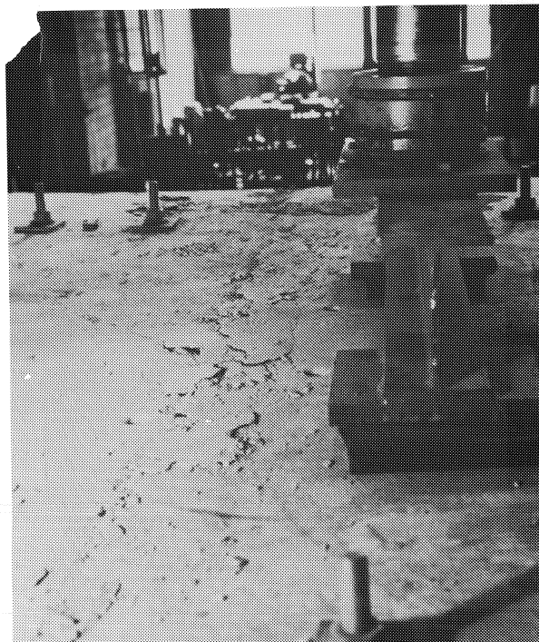
Figure 3.129 Crushed critical joints top flange.
