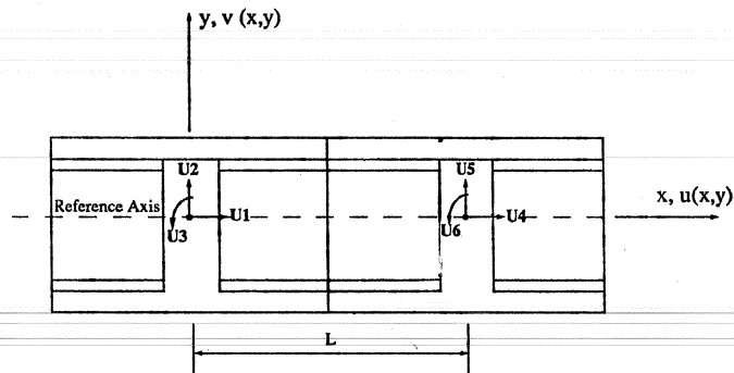
Figure 5.4 Beam element model.
