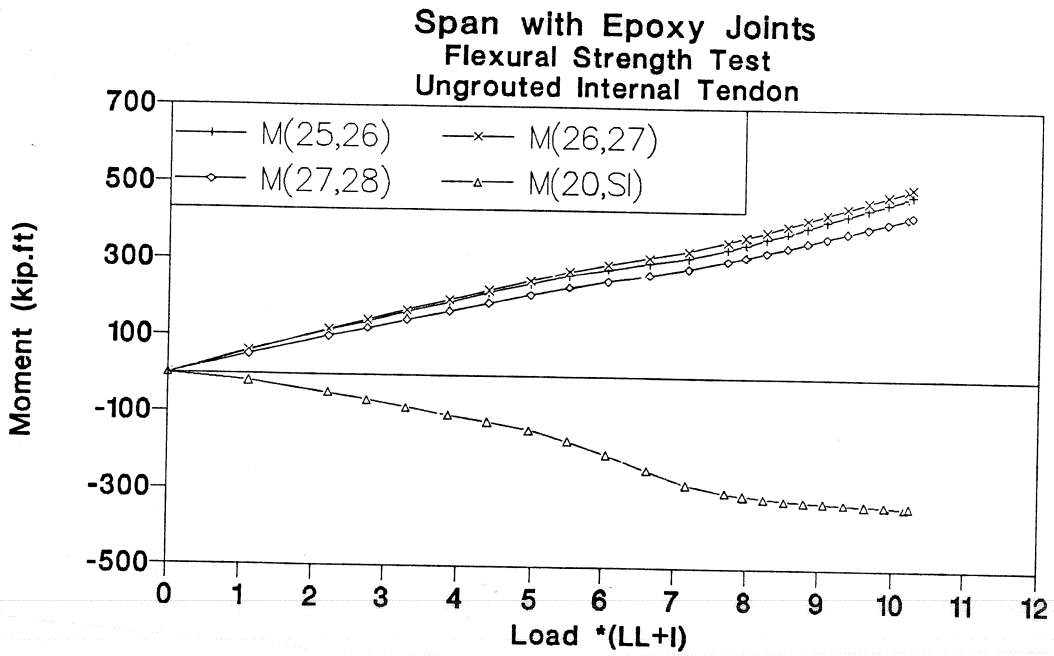
Figure 3.64 Moment-load of ungrouted internal tendons test in epoxy joints span.
