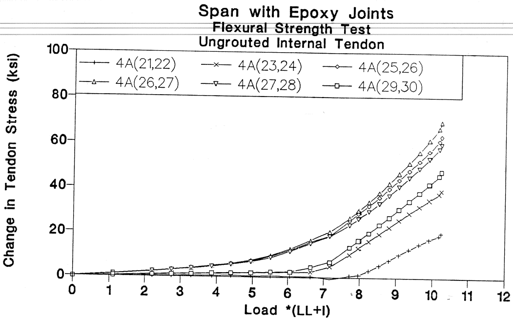
Figure 3.65 Tendon 4A stress-load of ungrouted internal tendons test in epoxy joints span.
