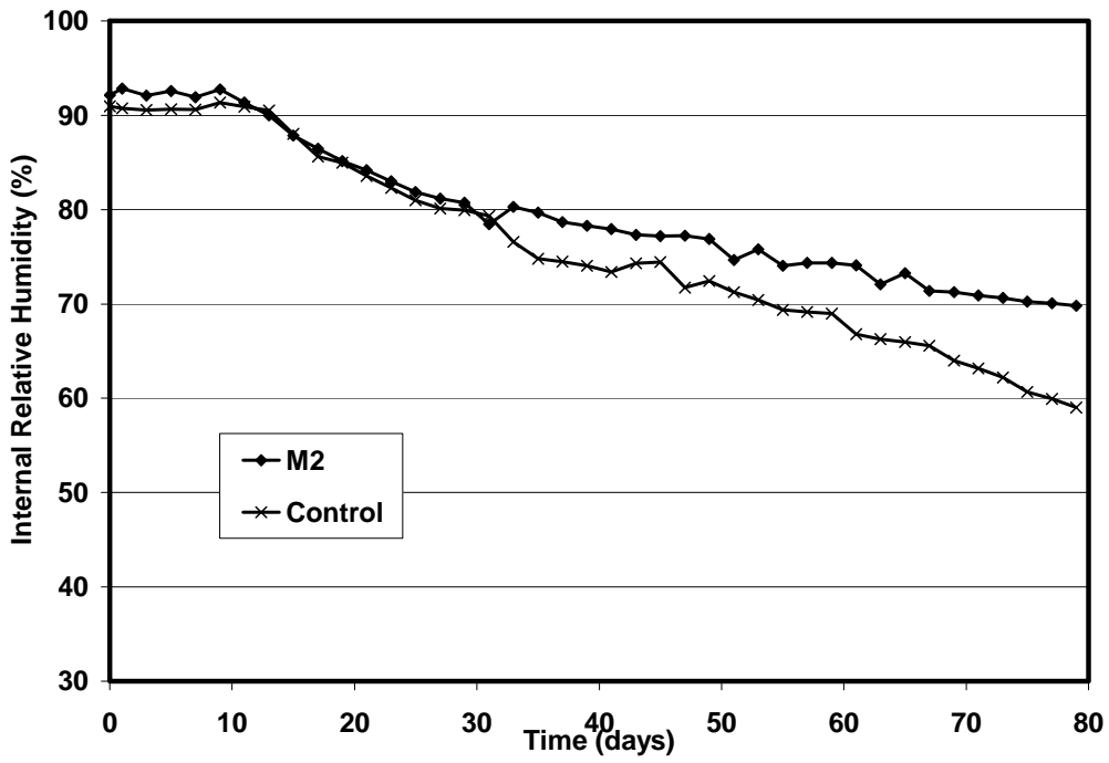
Figure D-4 Average internal RH of M2 replicates and control replicates at 1.5-in. depth
