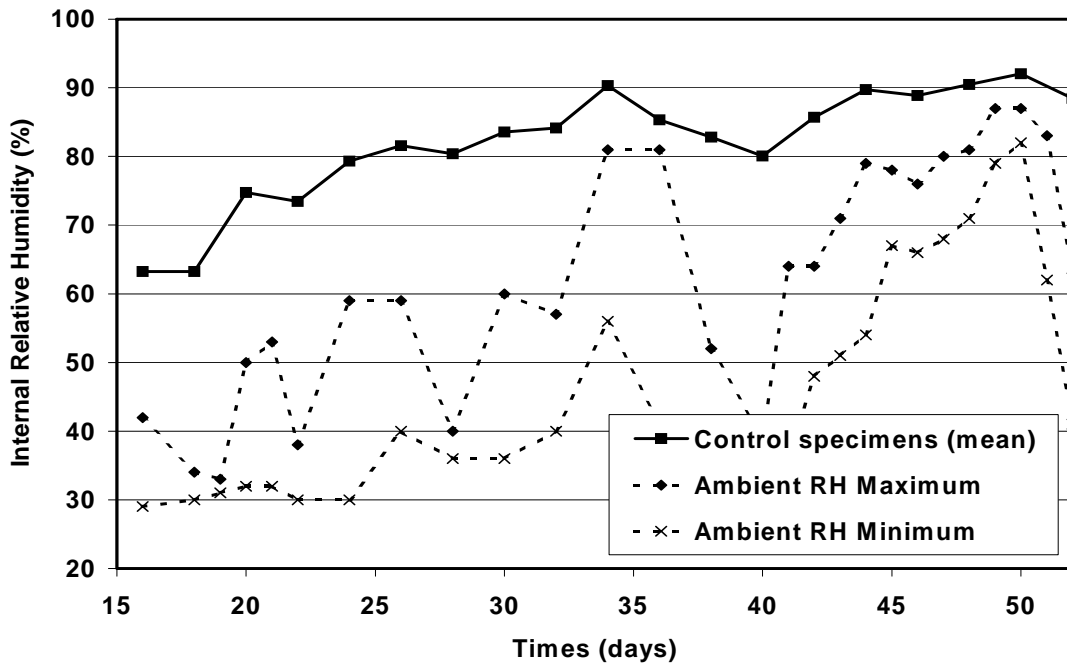
Figure 5.7 Average internal RH of control specimens at 0.5-in. depth and ambient RH during Wetting Stage #1 (Confirmatory Test)
